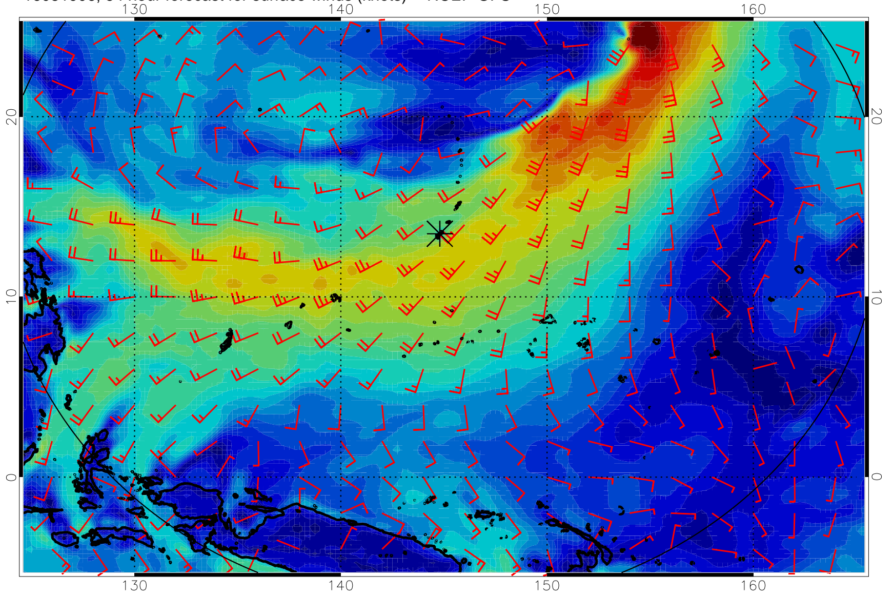
16081906, 54 hour forecast for surface winds (knots) -- NCEP GFS
