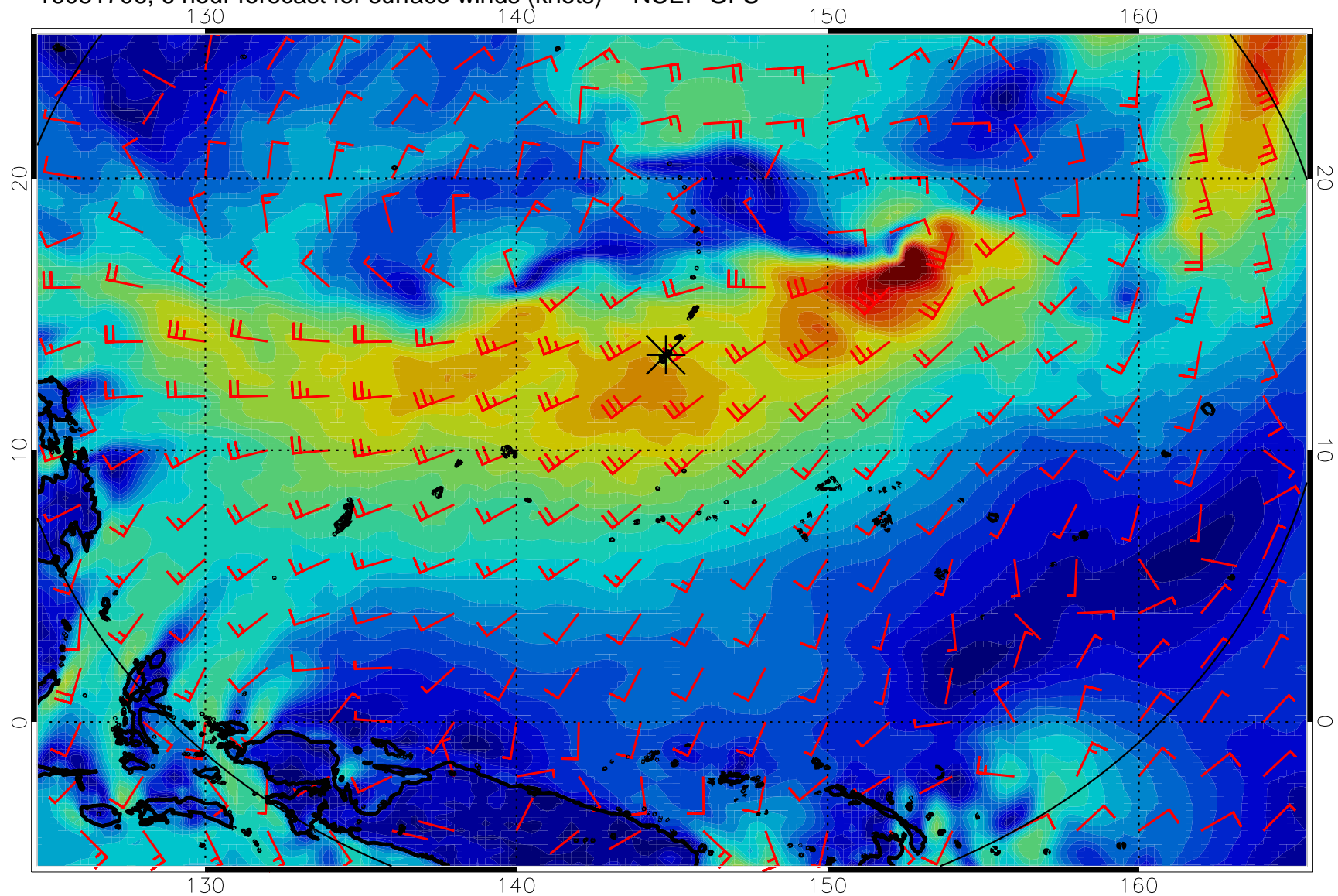
16081706, 6 hour forecast for surface winds (knots) -- NCEP GFS
