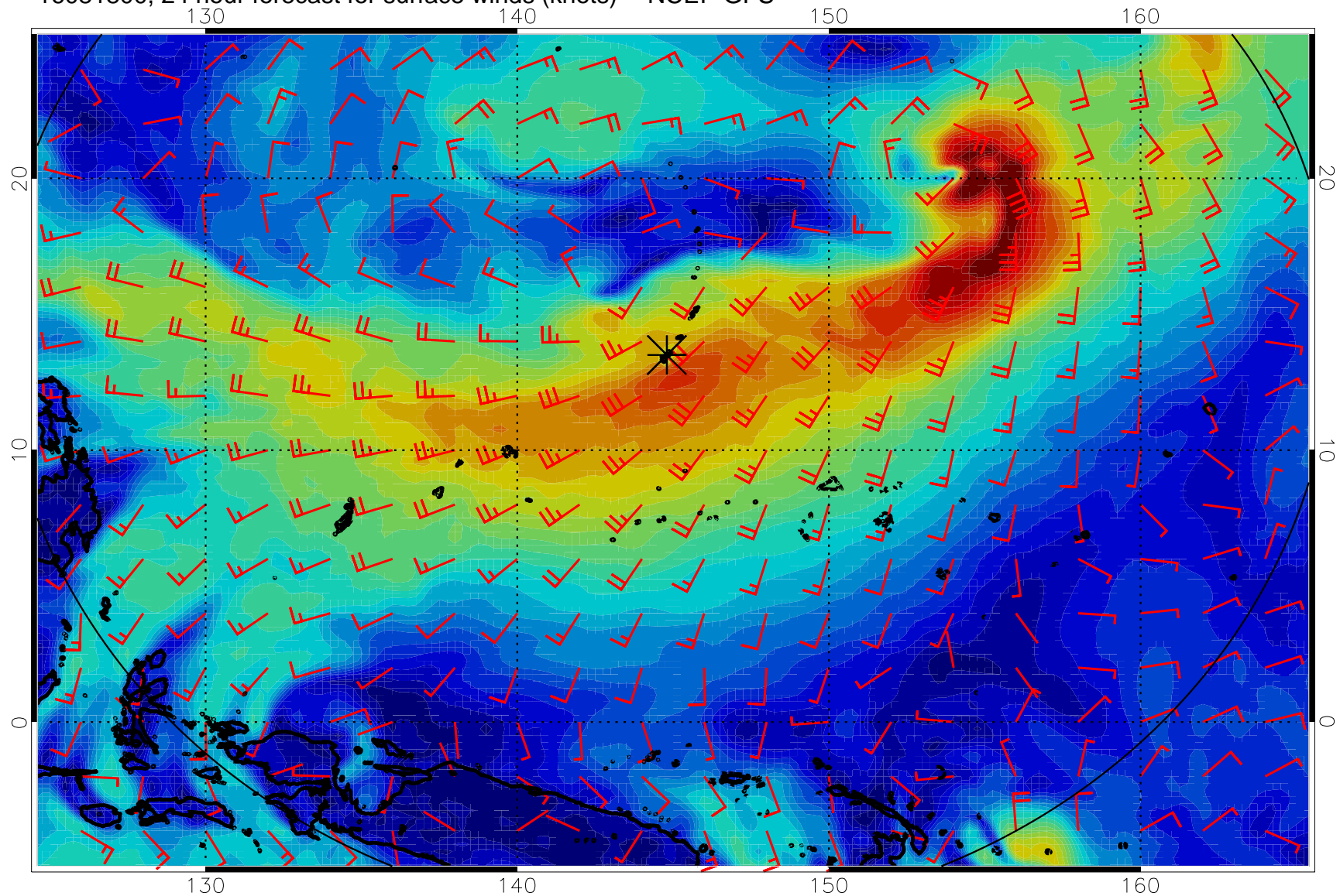
16081800, 24 hour forecast for surface winds (knots) -- NCEP GFS
