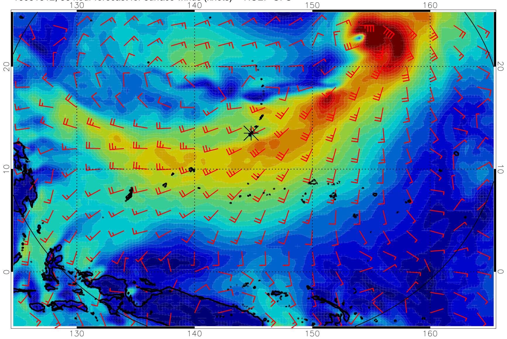
16081812, 36 hour forecast for surface winds (knots) -- NCEP GFS
