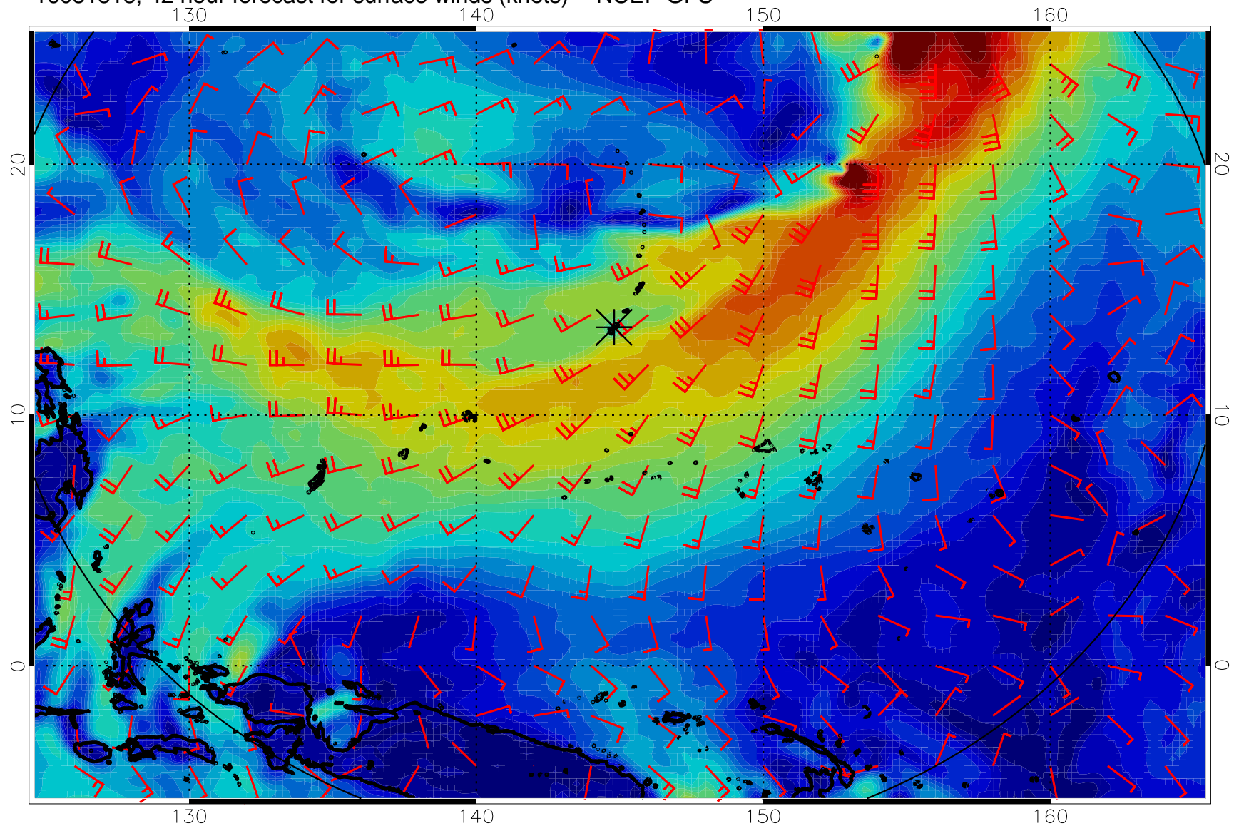
16081818, 42 hour forecast for surface winds (knots) -- NCEP GFS
