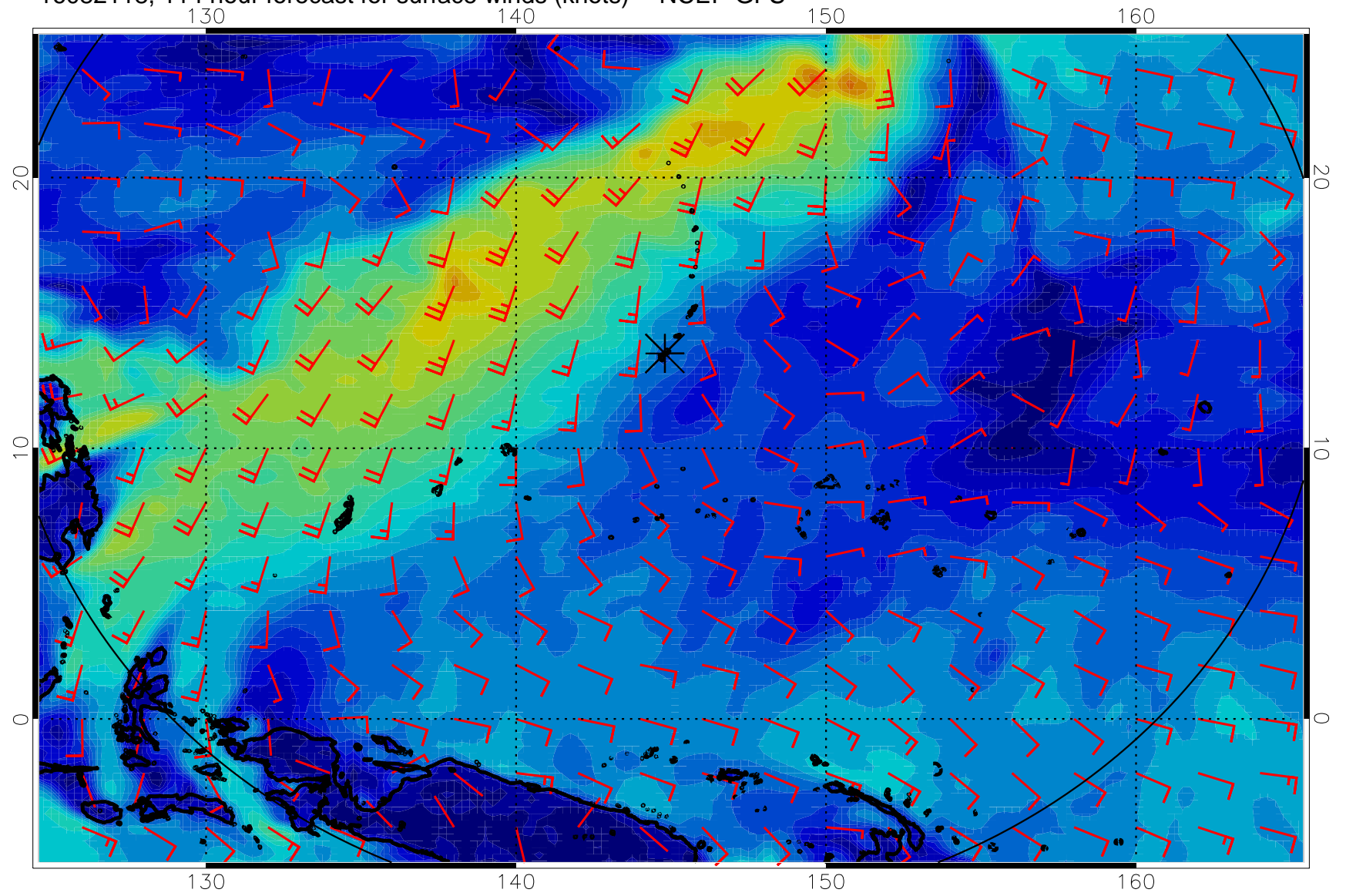
16082118, 114 hour forecast for surface winds (knots) -- NCEP GFS
