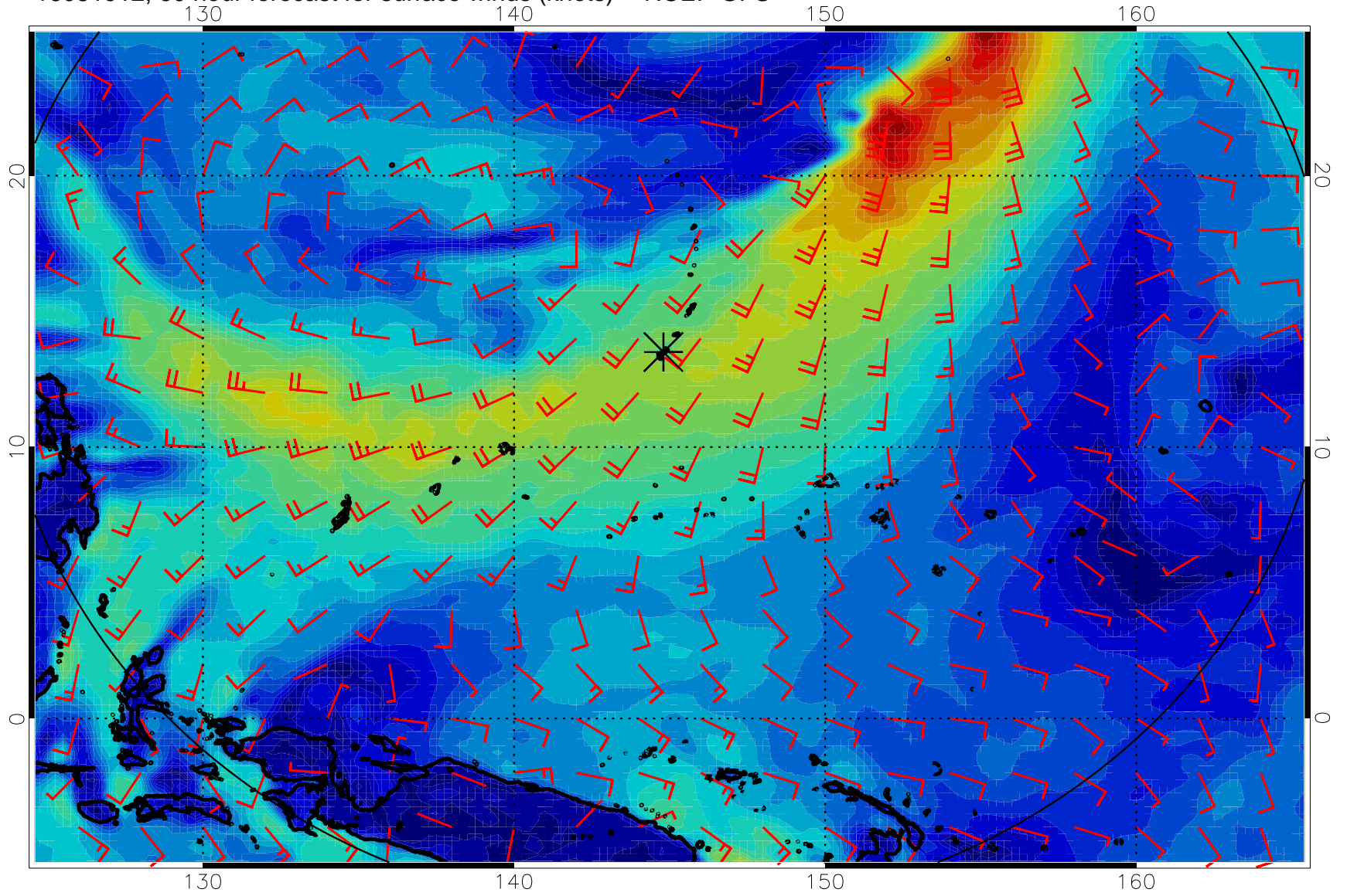
16081912, 60 hour forecast for surface winds (knots) -- NCEP GFS
