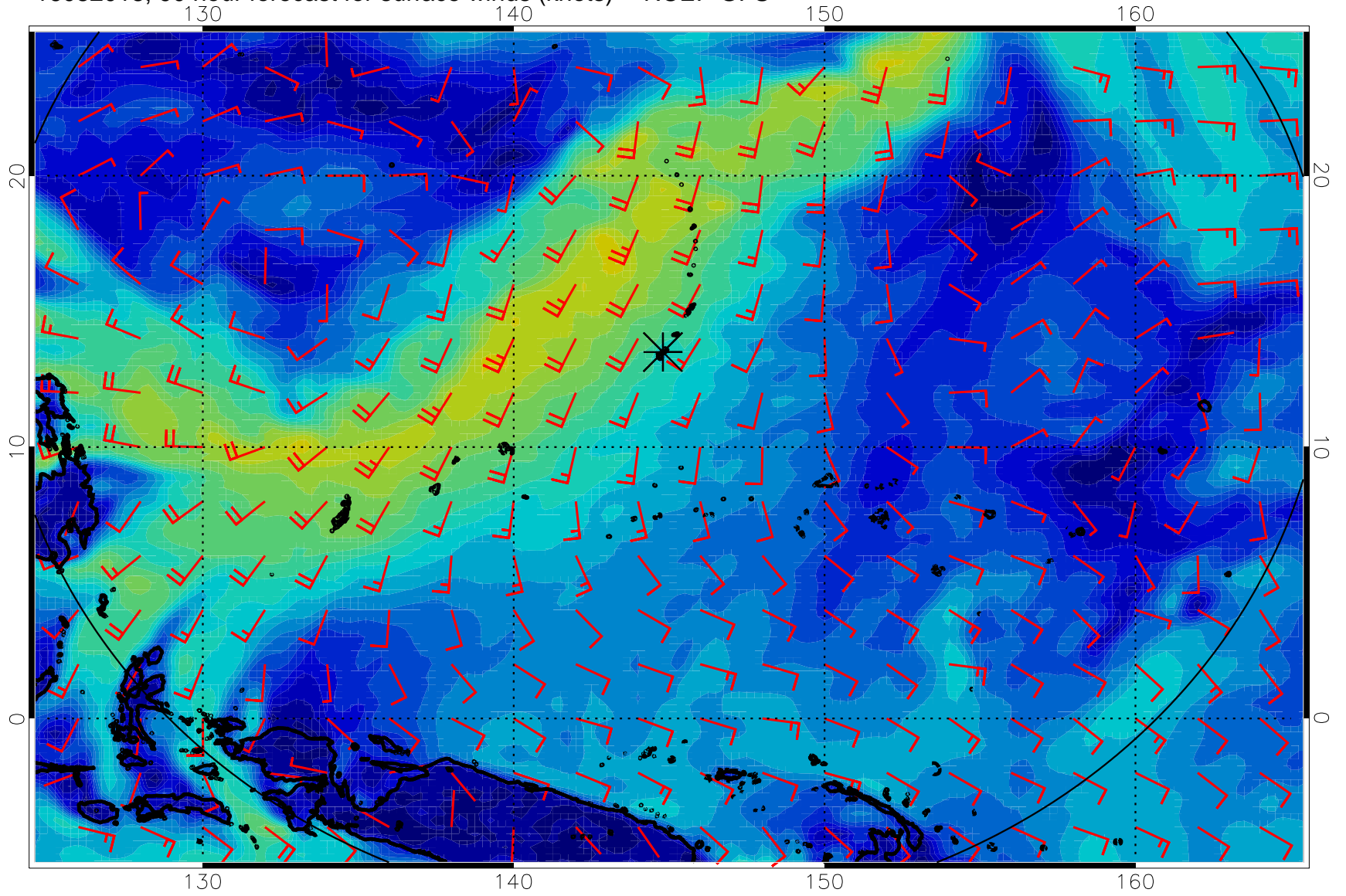
16082018, 90 hour forecast for surface winds (knots) -- NCEP GFS
