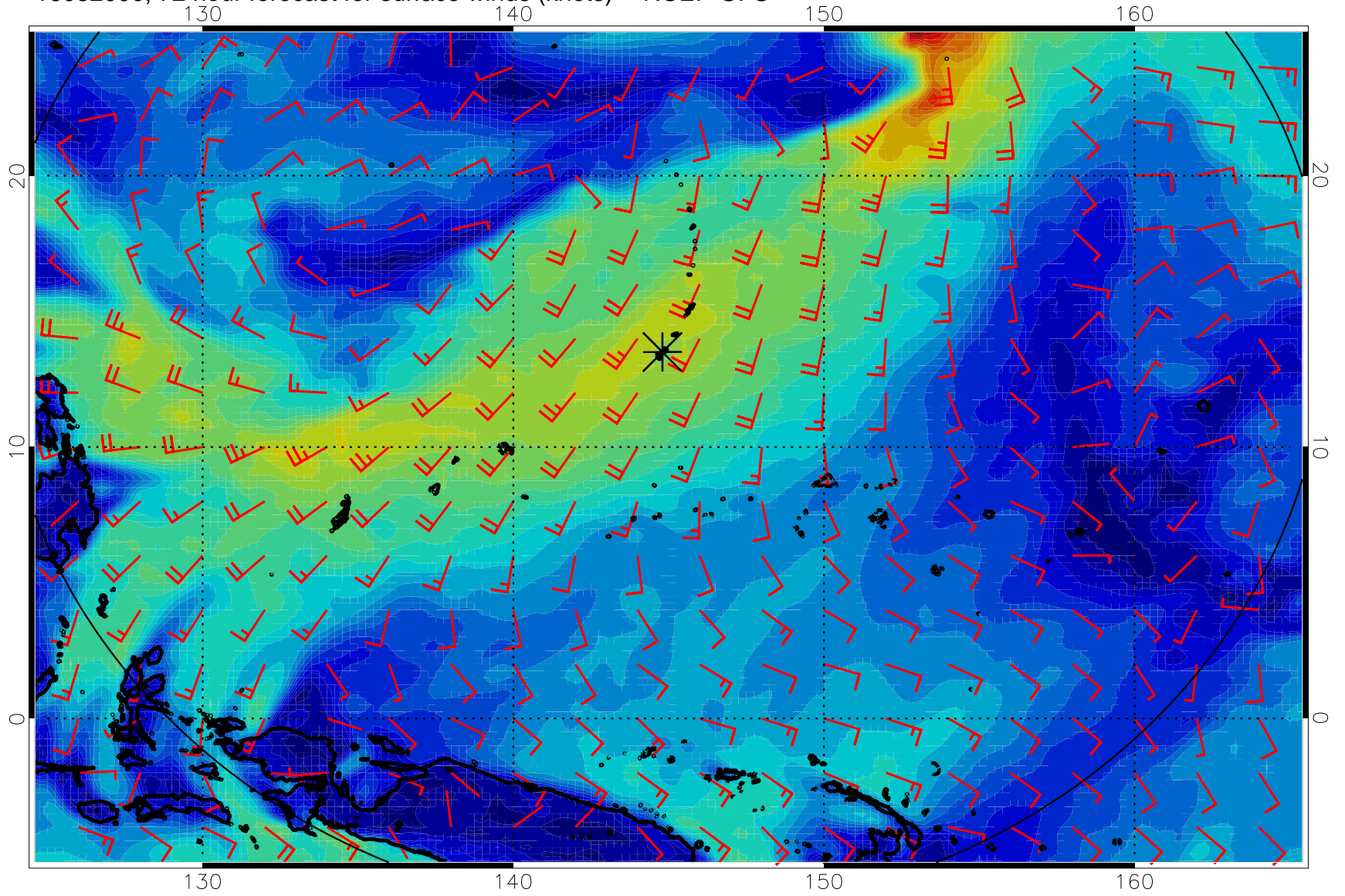
16082000, 72 hour forecast for surface winds (knots) -- NCEP GFS
