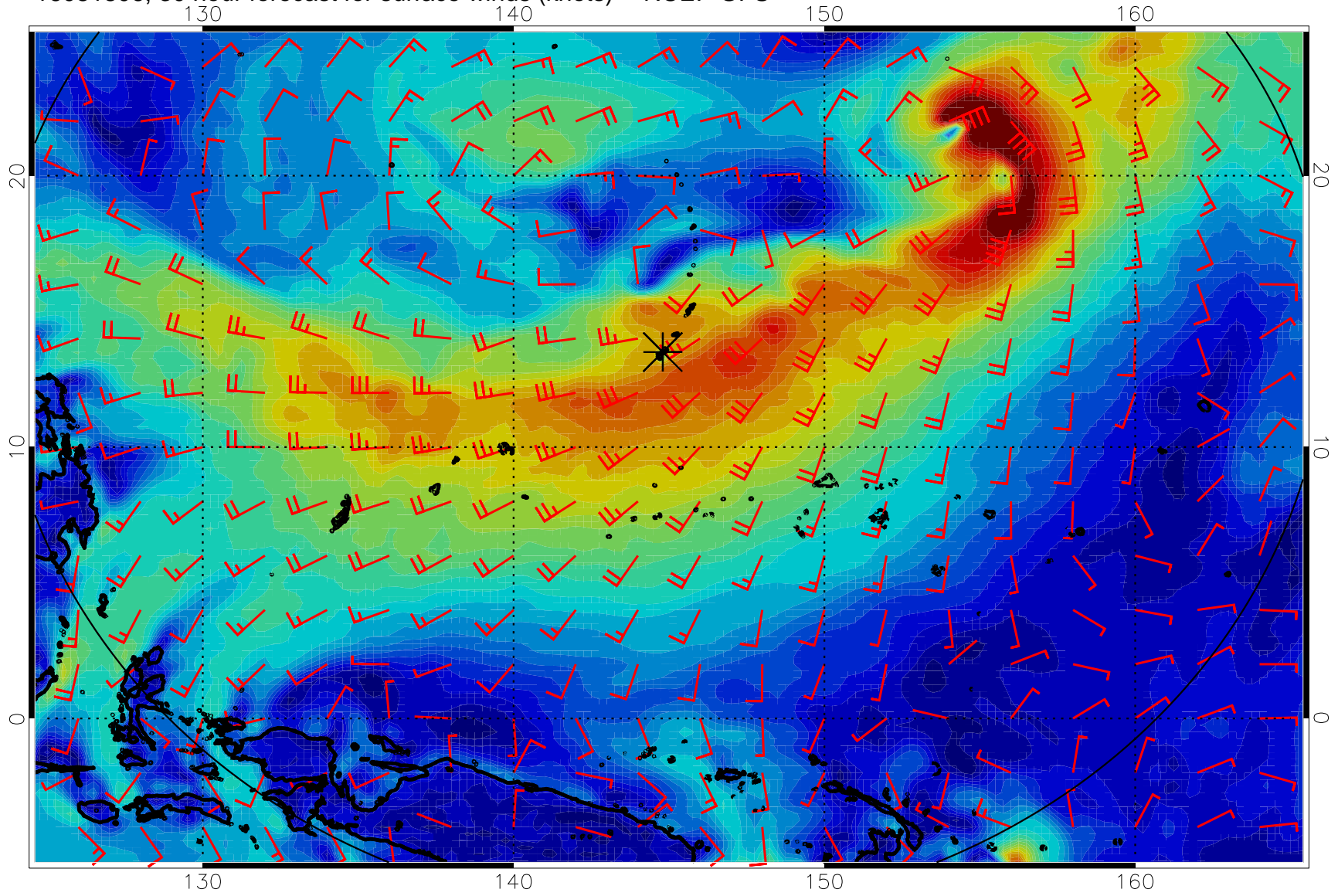
16081806, 30 hour forecast for surface winds (knots) -- NCEP GFS
