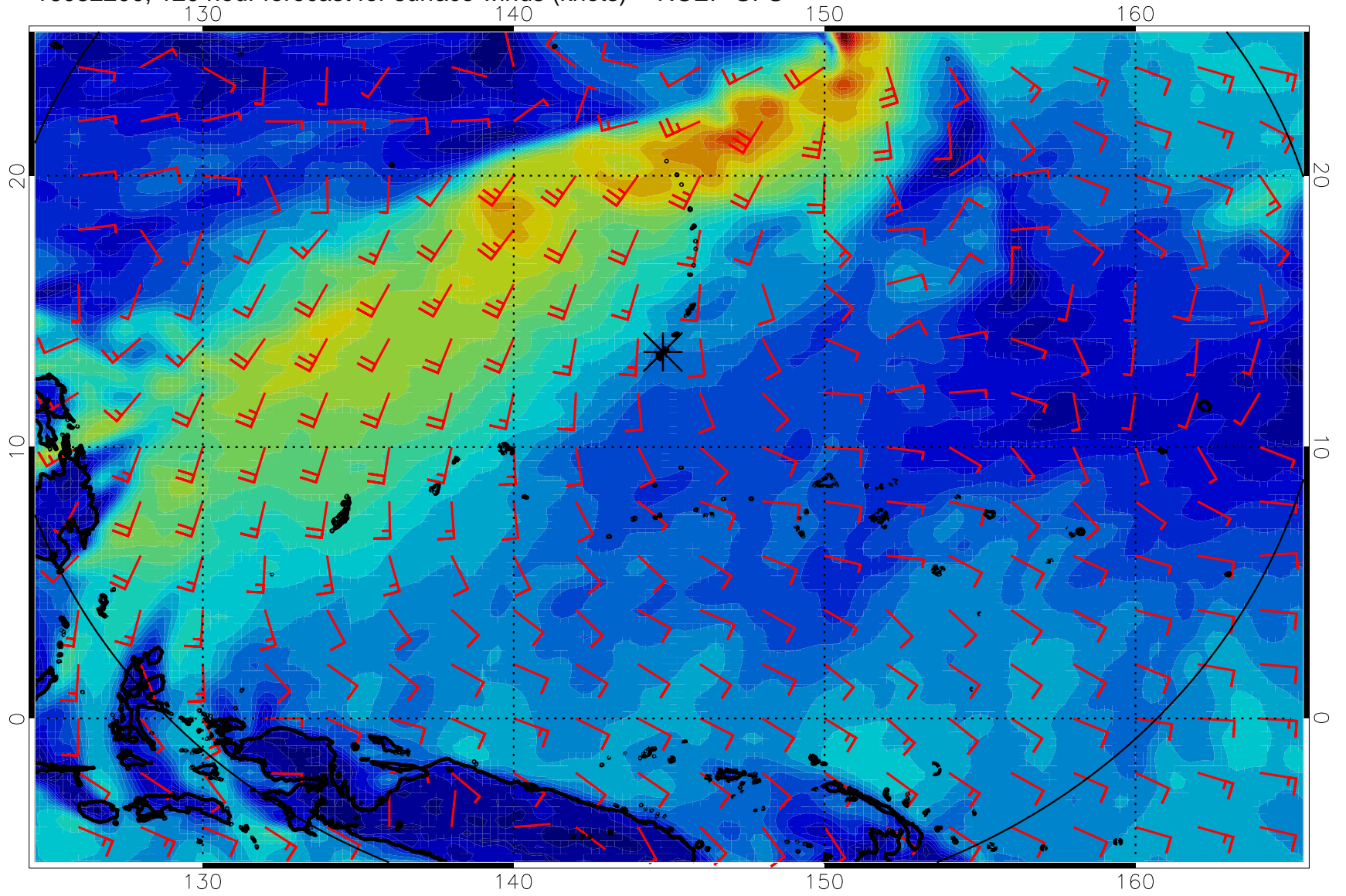
16082200, 120 hour forecast for surface winds (knots) -- NCEP GFS
