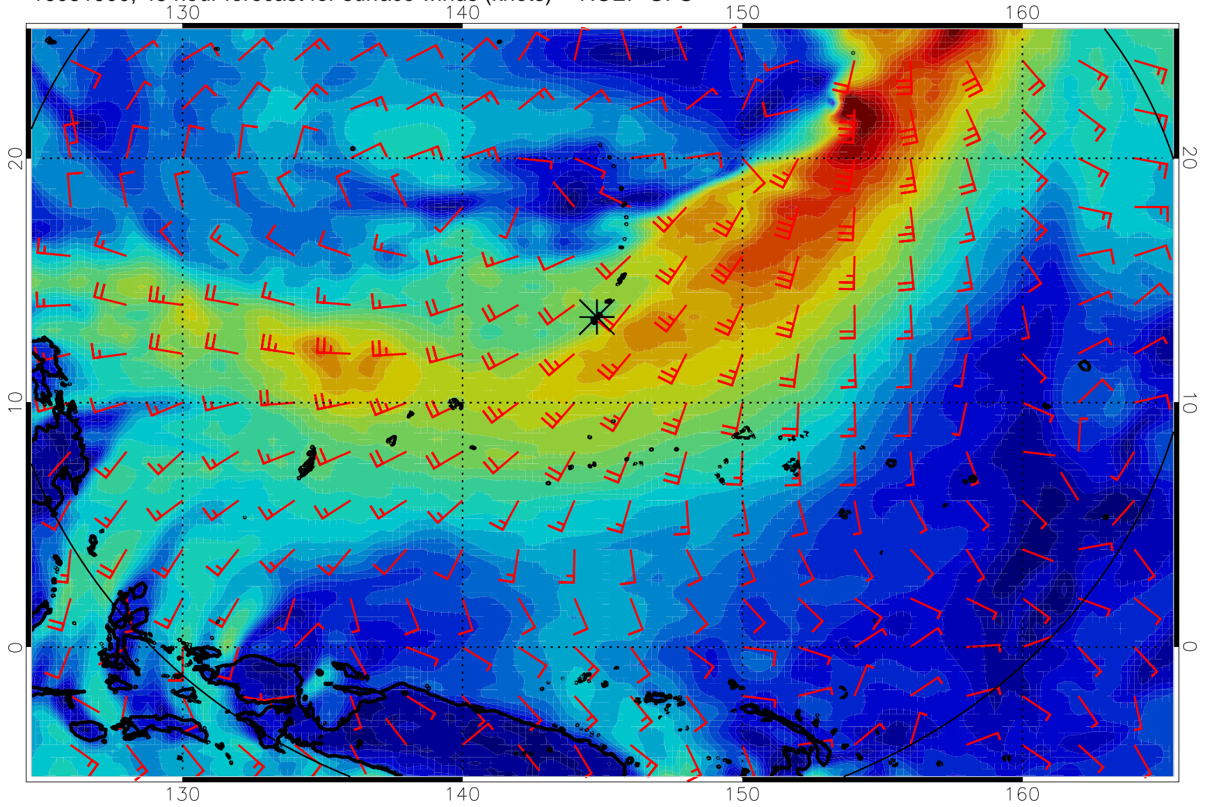
16081900, 48 hour forecast for surface winds (knots) -- NCEP GFS
