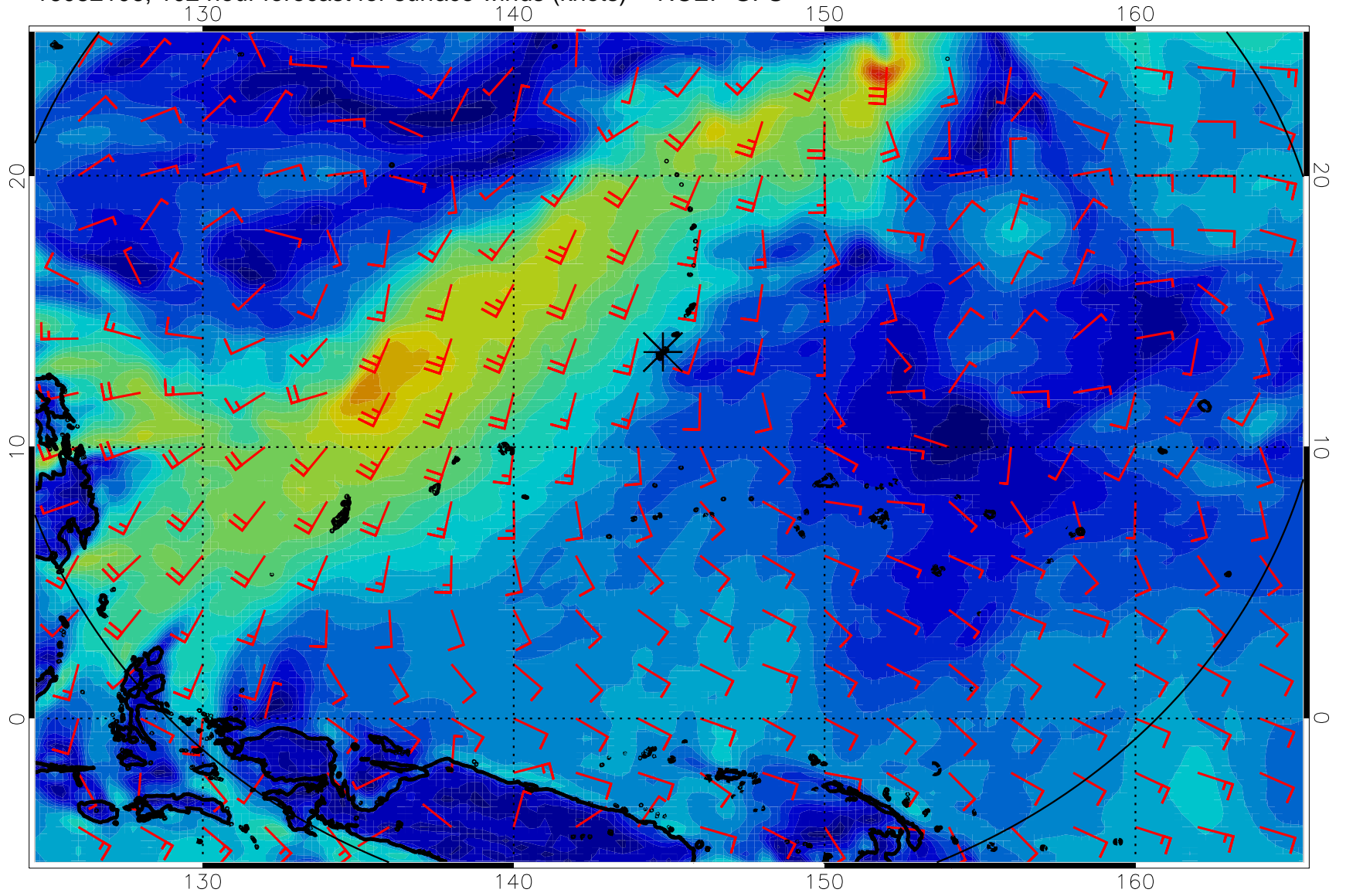
16082106, 102 hour forecast for surface winds (knots) -- NCEP GFS
