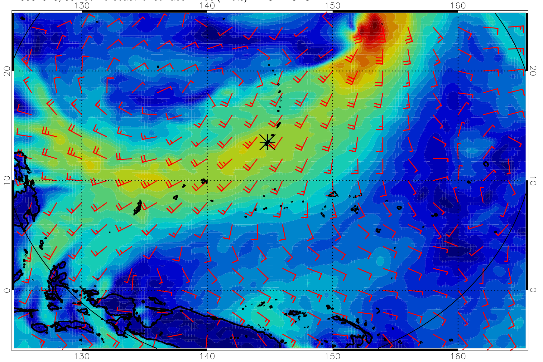
16081918, 66 hour forecast for surface winds (knots) -- NCEP GFS
