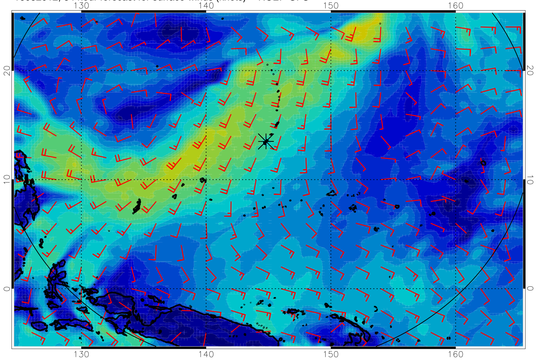
16082012, 84 hour forecast for surface winds (knots) -- NCEP GFS
