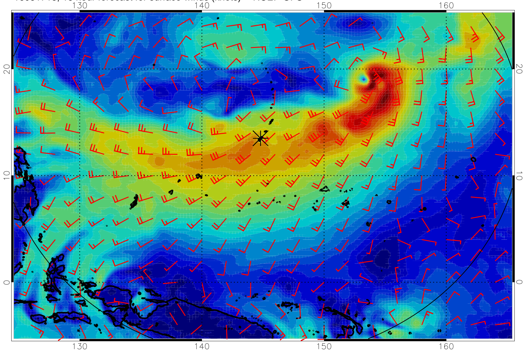
16081718, 18 hour forecast for surface winds (knots) -- NCEP GFS
