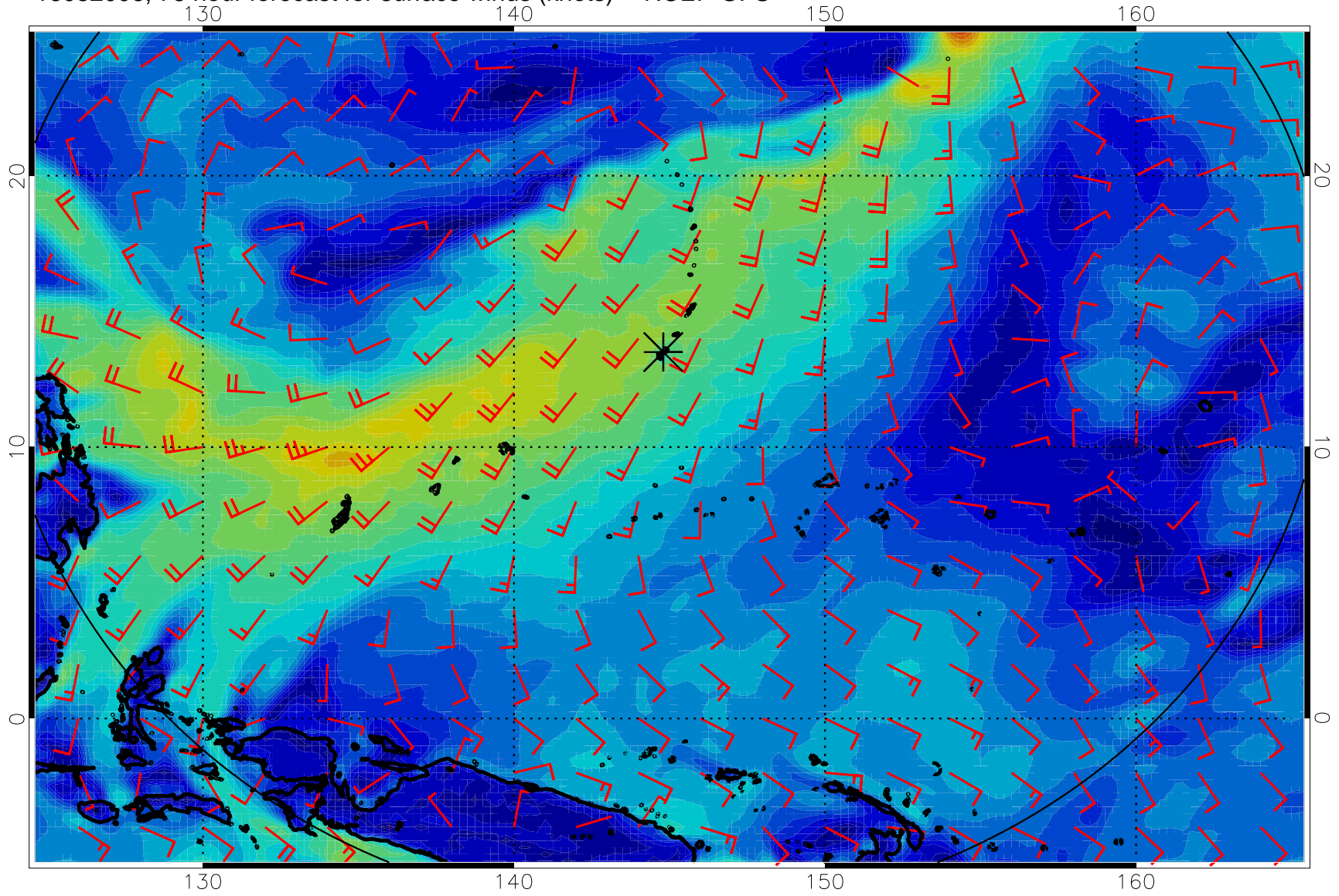
16082006, 78 hour forecast for surface winds (knots) -- NCEP GFS
