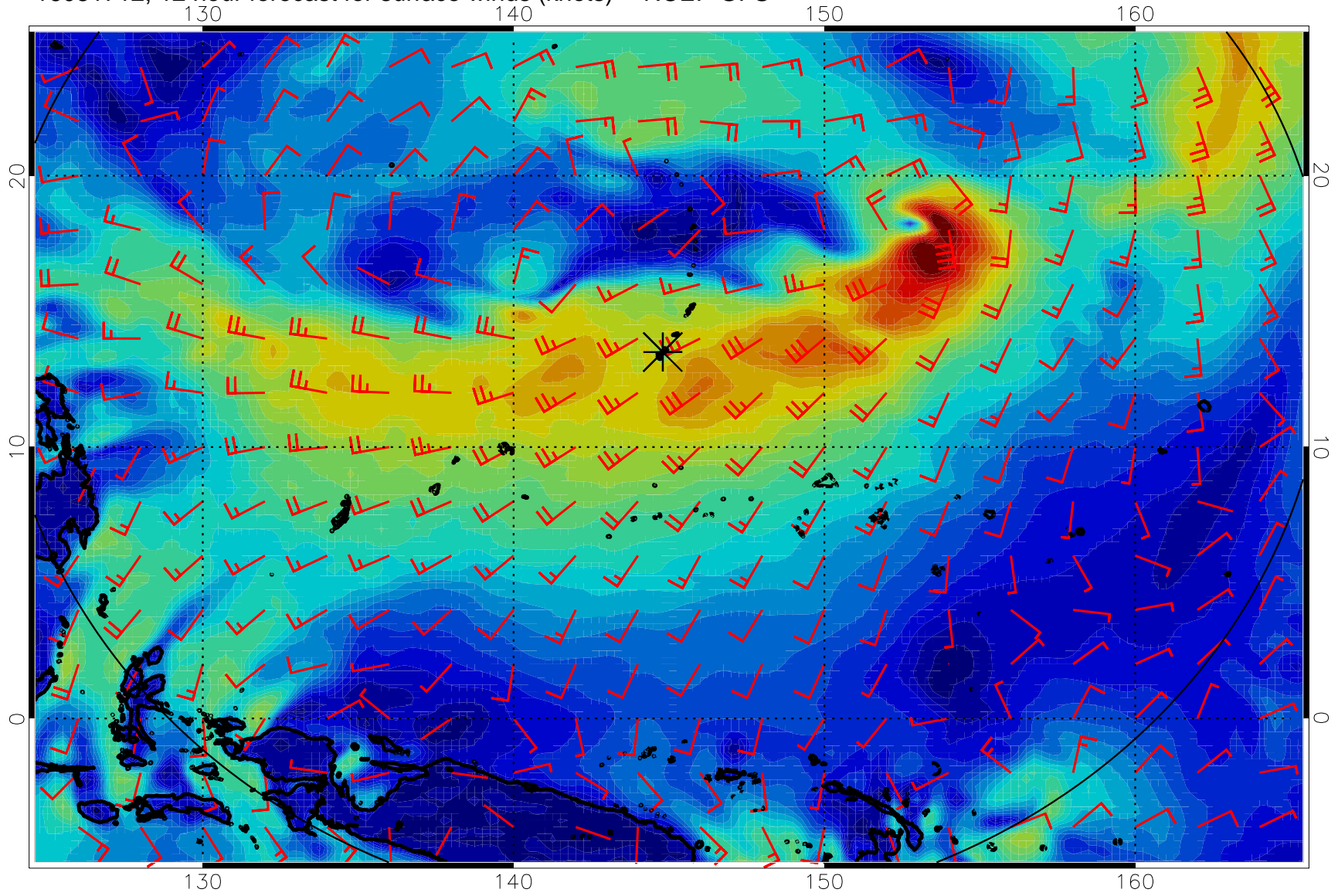
16081712, 12 hour forecast for surface winds (knots) -- NCEP GFS
