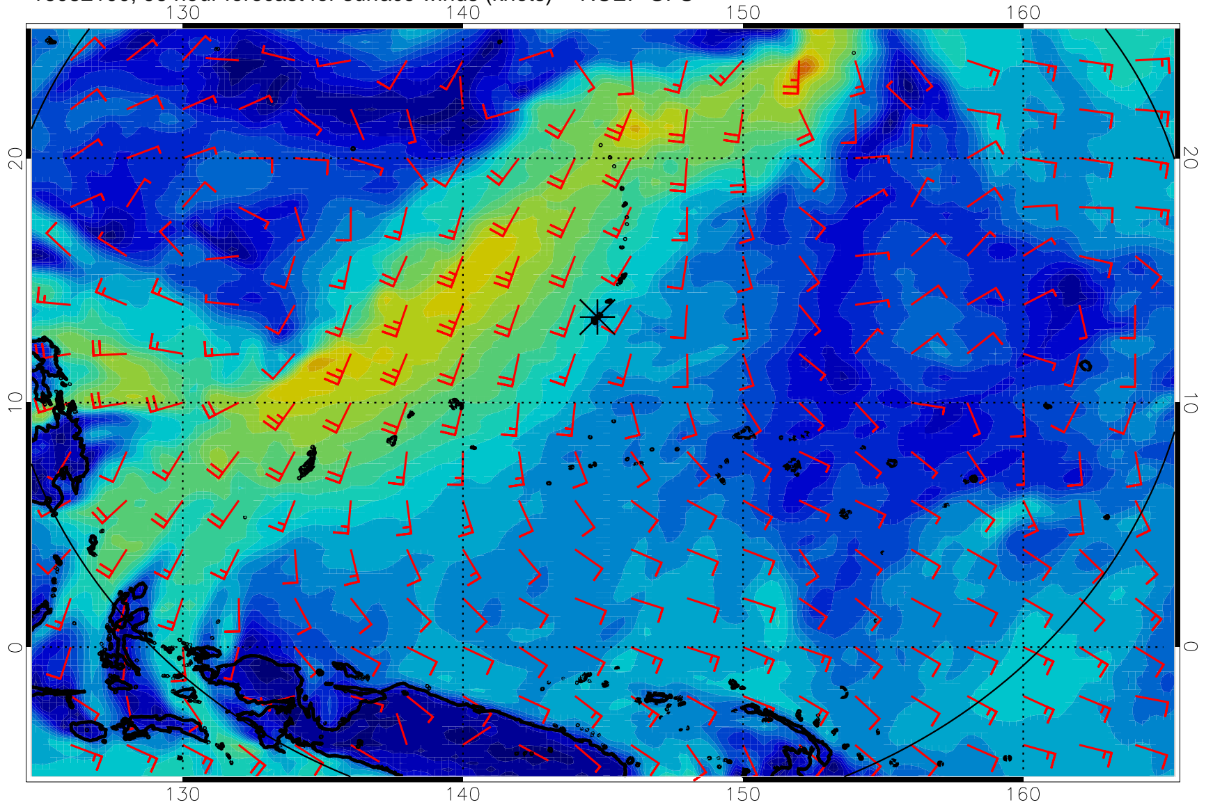
16082100, 96 hour forecast for surface winds (knots) -- NCEP GFS
