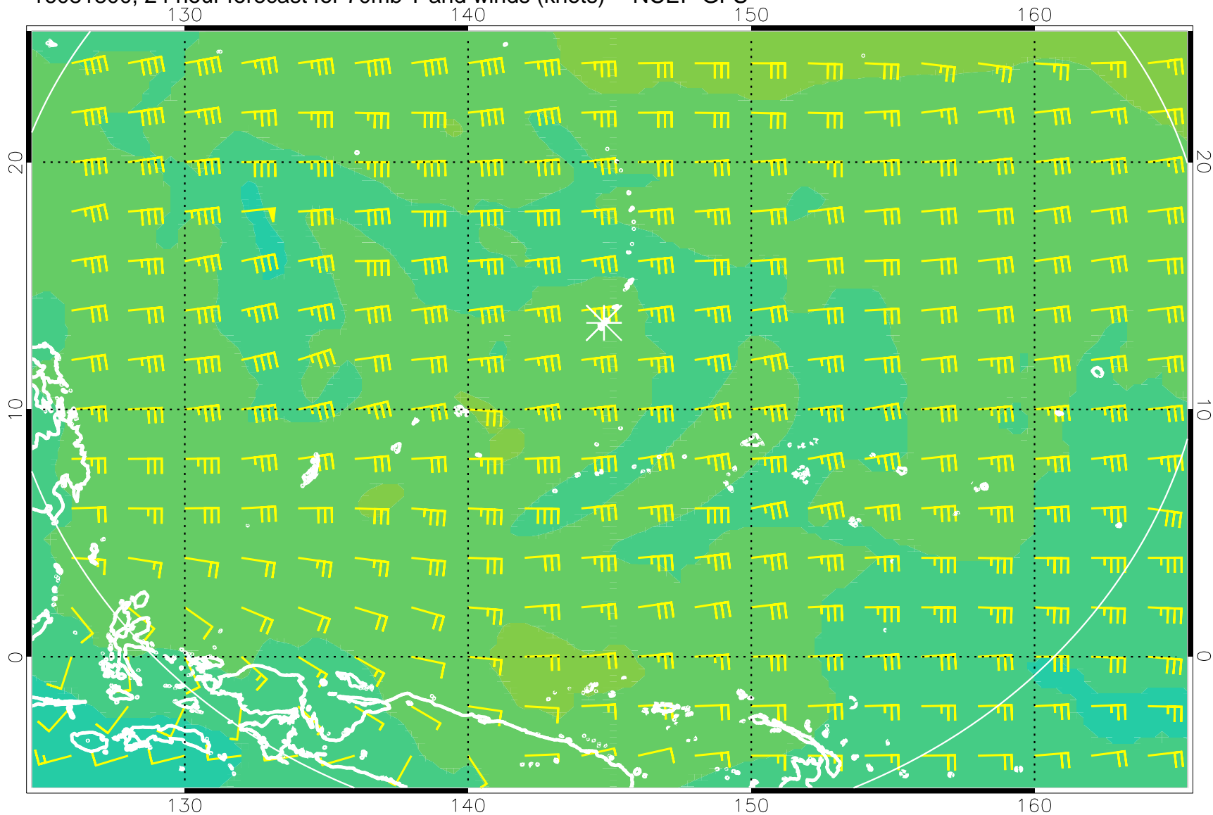
16081800, 24 hour forecast for 70mb T and winds (knots) -- NCEP GFS
