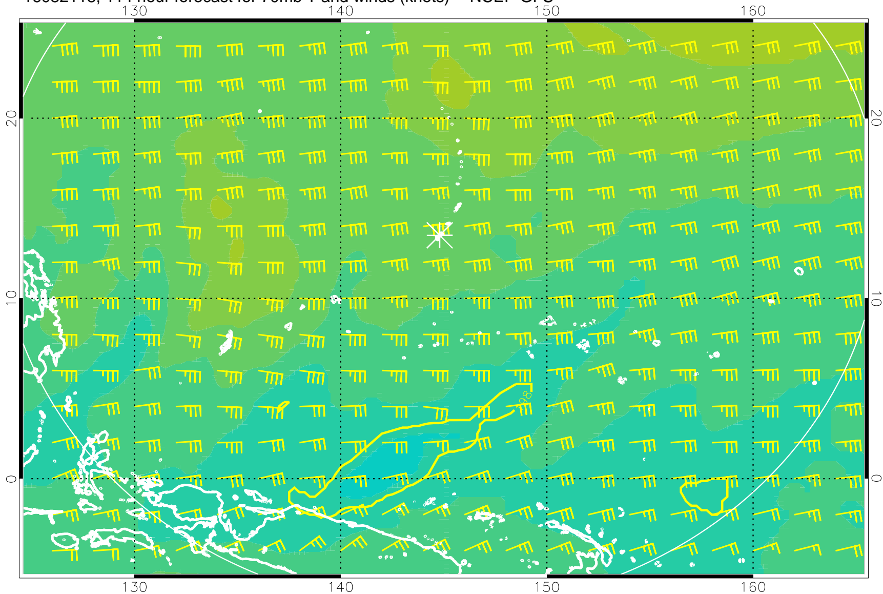
16082118, 114 hour forecast for 70mb T and winds (knots) -- NCEP GFS
