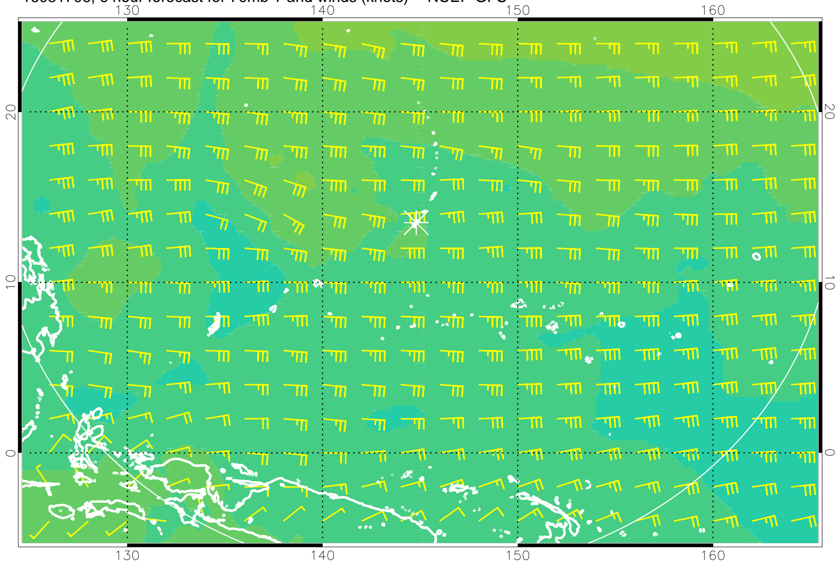
16081706, 6 hour forecast for 70mb T and winds (knots) -- NCEP GFS
