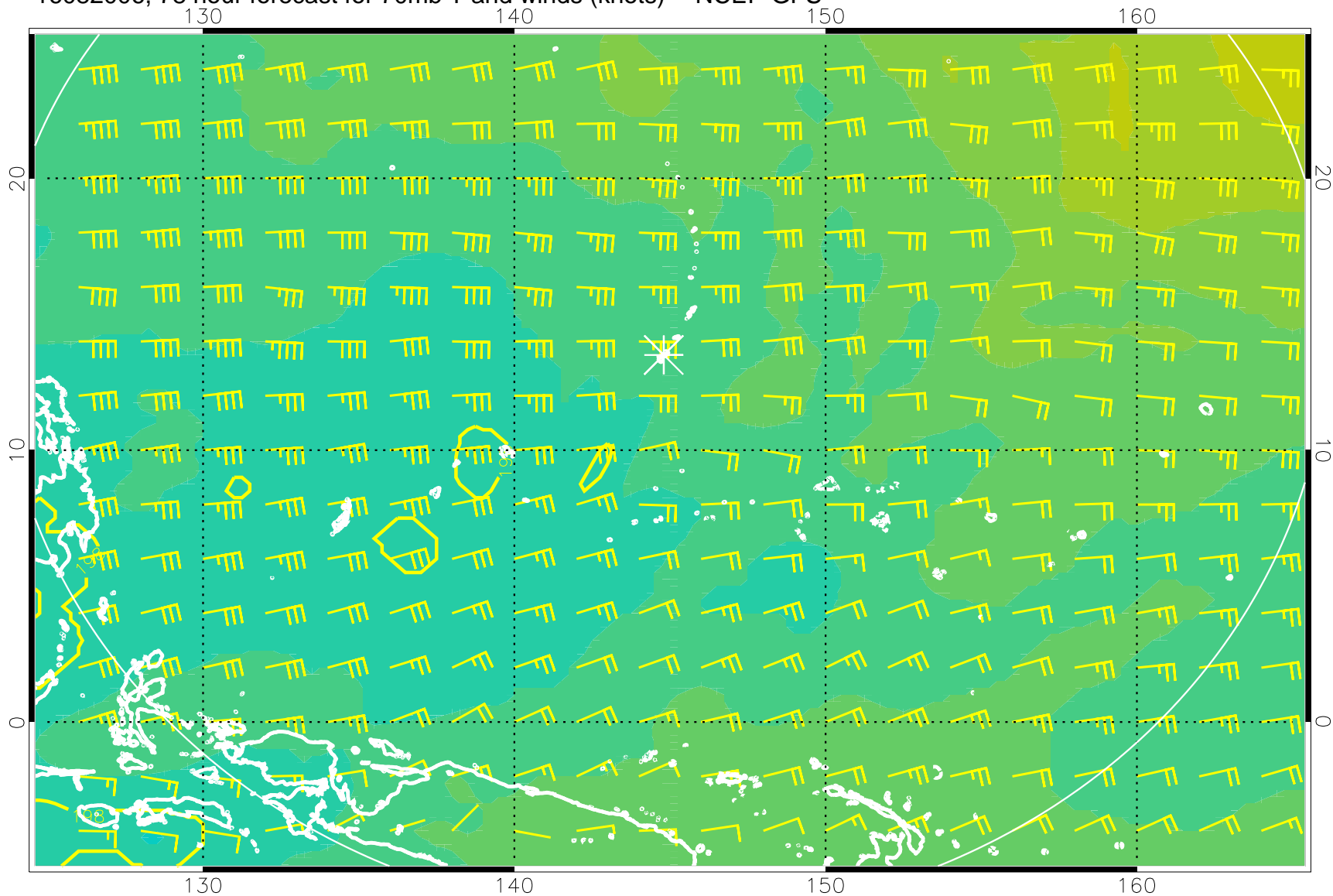
16082006, 78 hour forecast for 70mb T and winds (knots) -- NCEP GFS
