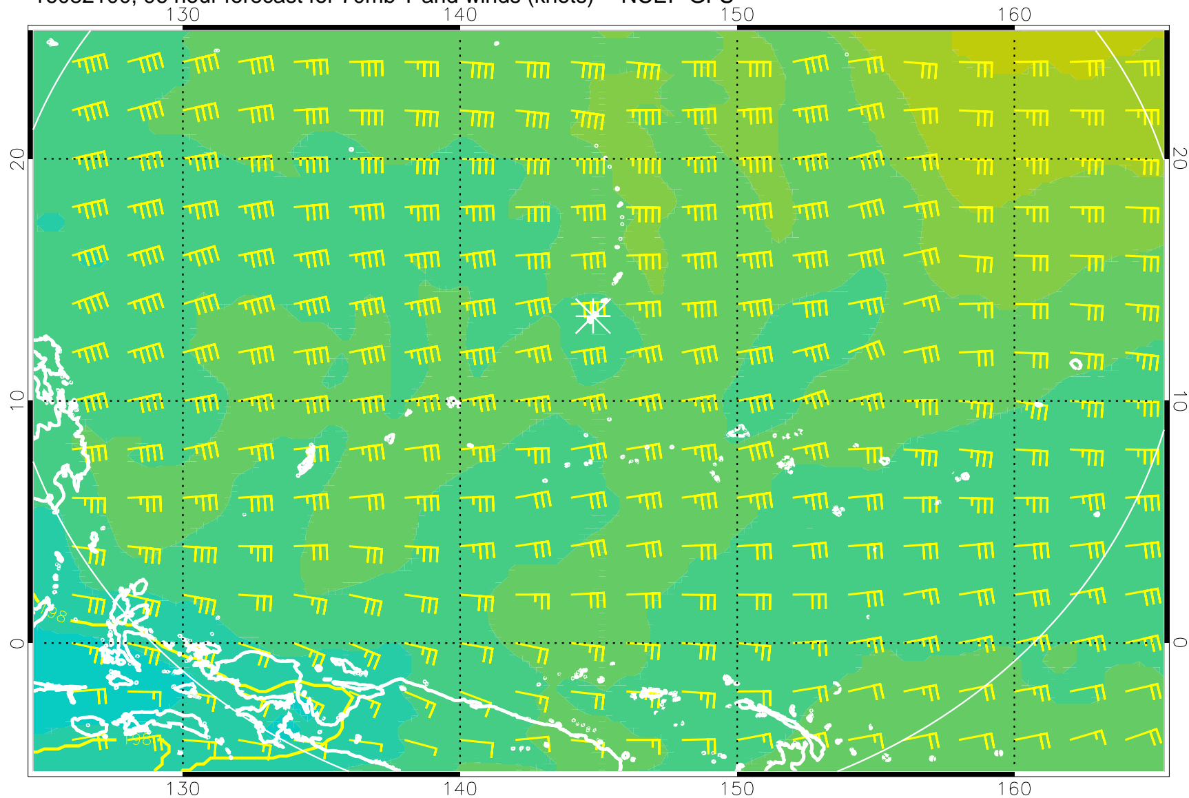
16082100, 96 hour forecast for 70mb T and winds (knots) -- NCEP GFS
