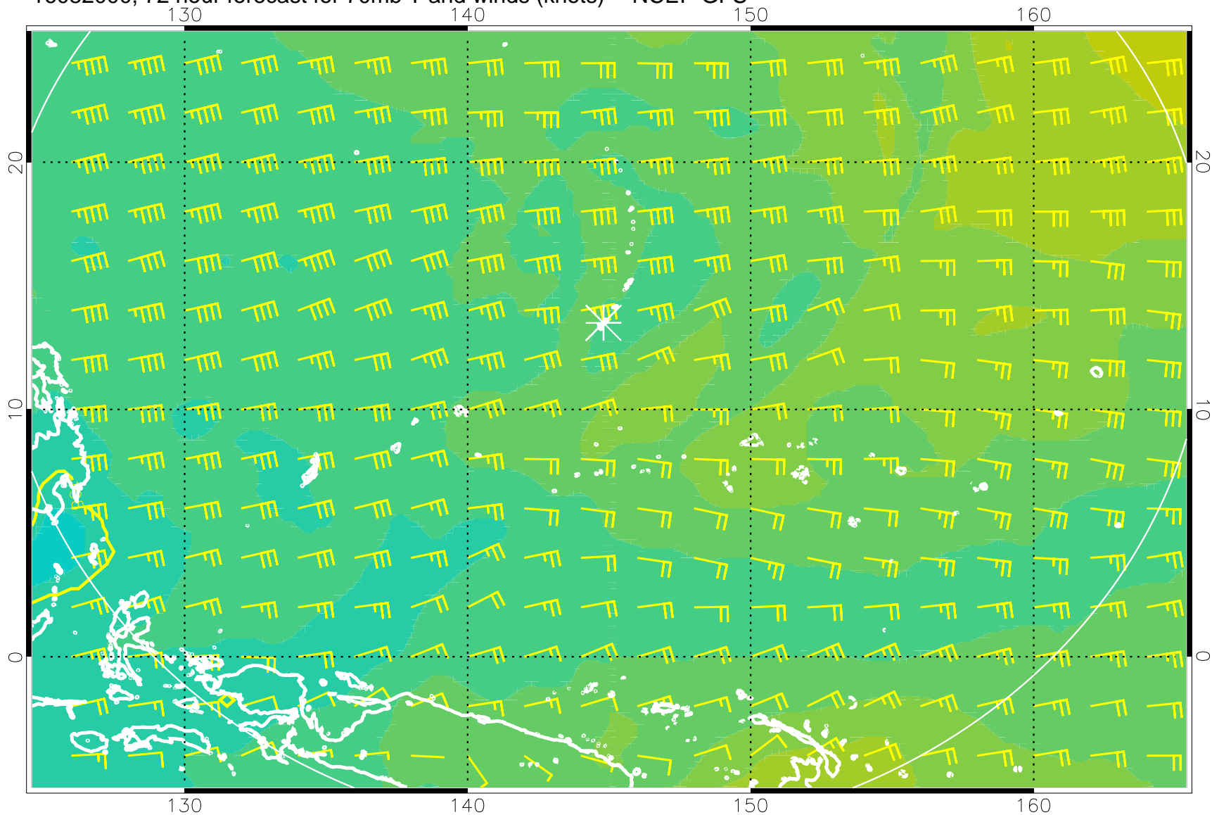
16082000, 72 hour forecast for 70mb T and winds (knots) -- NCEP GFS
