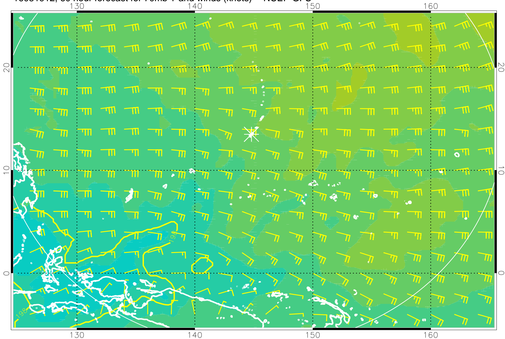
16081912, 60 hour forecast for 70mb T and winds (knots) -- NCEP GFS
