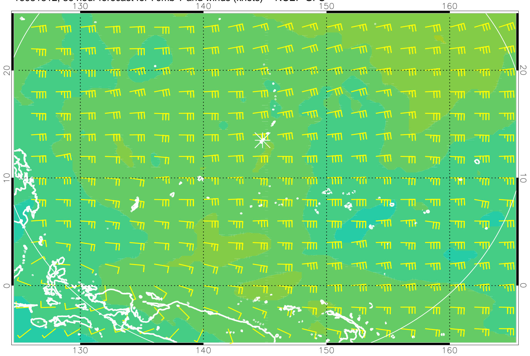
16081812, 36 hour forecast for 70mb T and winds (knots) -- NCEP GFS
