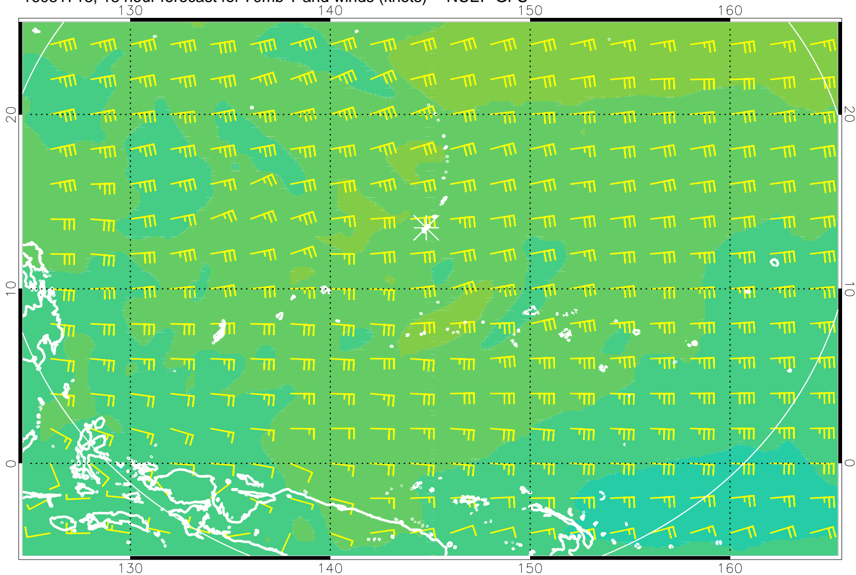
16081718, 18 hour forecast for 70mb T and winds (knots) -- NCEP GFS
