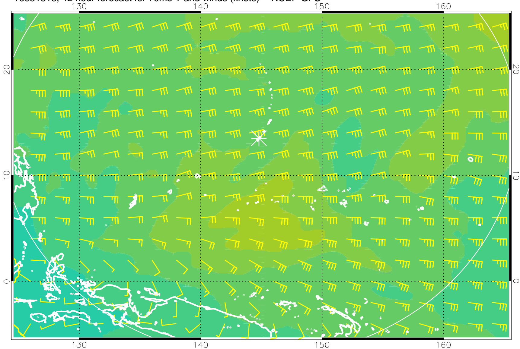
16081818, 42 hour forecast for 70mb T and winds (knots) -- NCEP GFS
