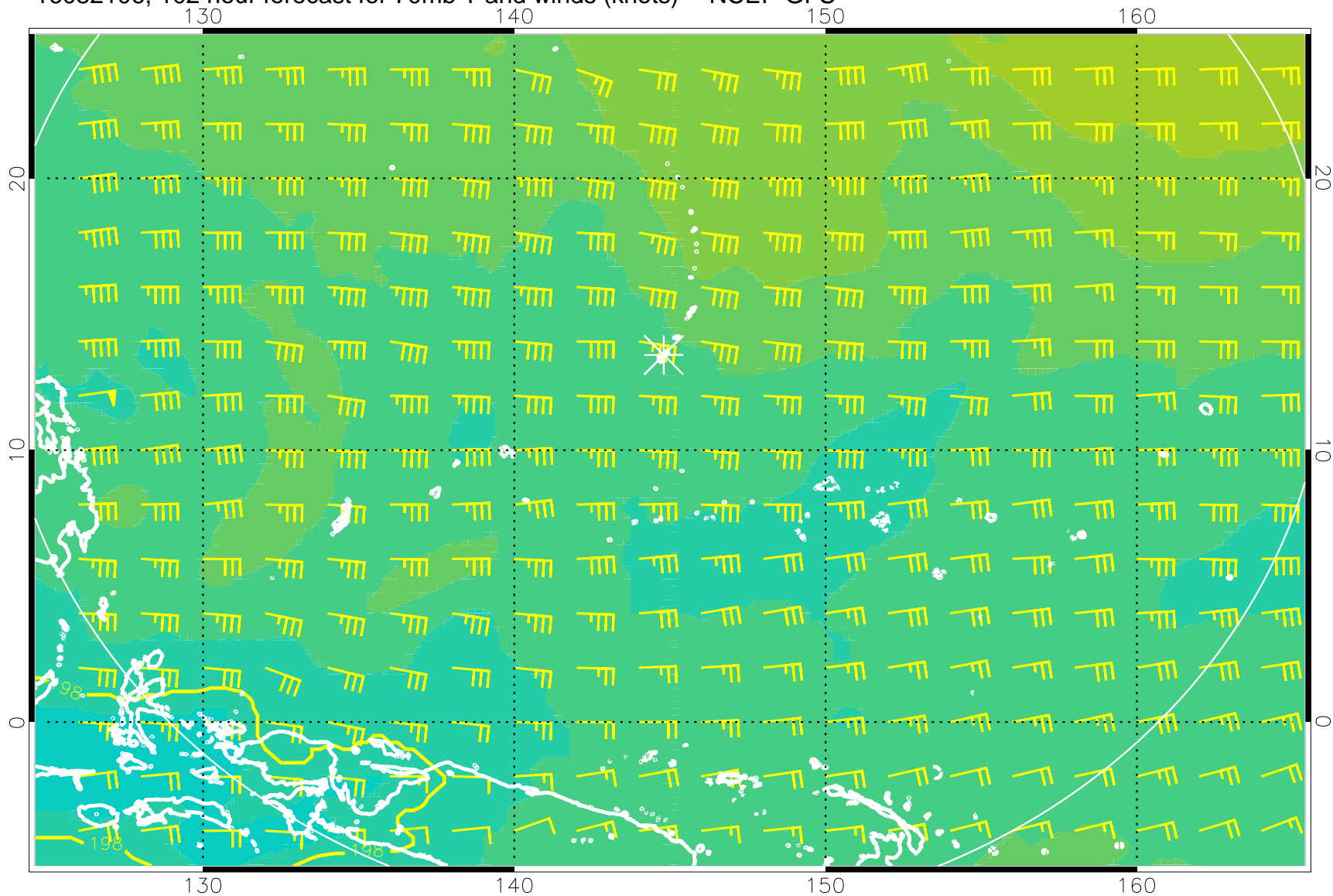
16082106, 102 hour forecast for 70mb T and winds (knots) -- NCEP GFS
