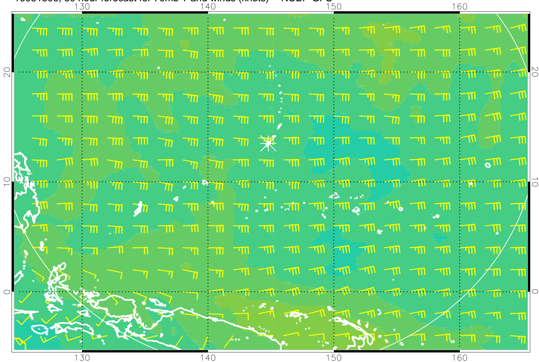
16081806, 30 hour forecast for 70mb T and winds (knots) -- NCEP GFS
