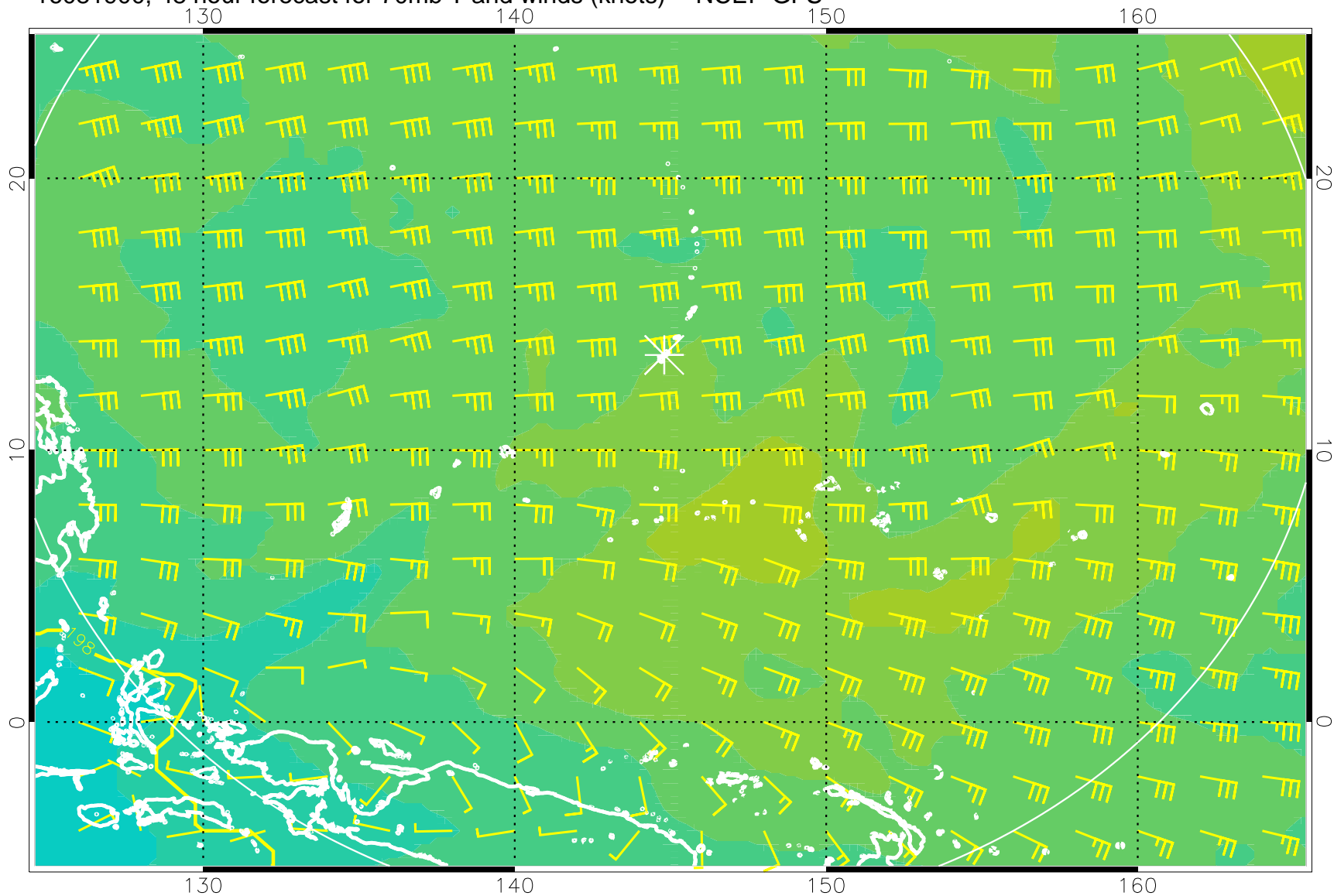
16081900, 48 hour forecast for 70mb T and winds (knots) -- NCEP GFS
