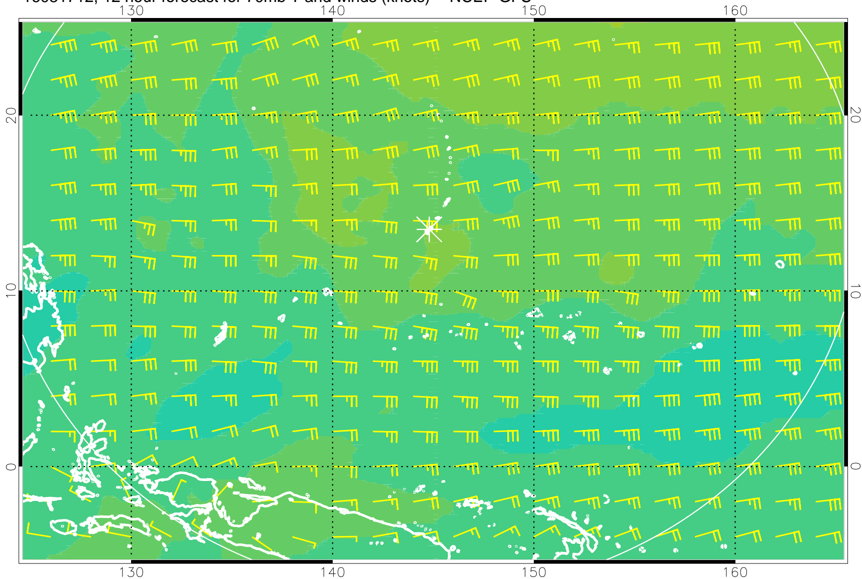
16081712, 12 hour forecast for 70mb T and winds (knots) -- NCEP GFS
