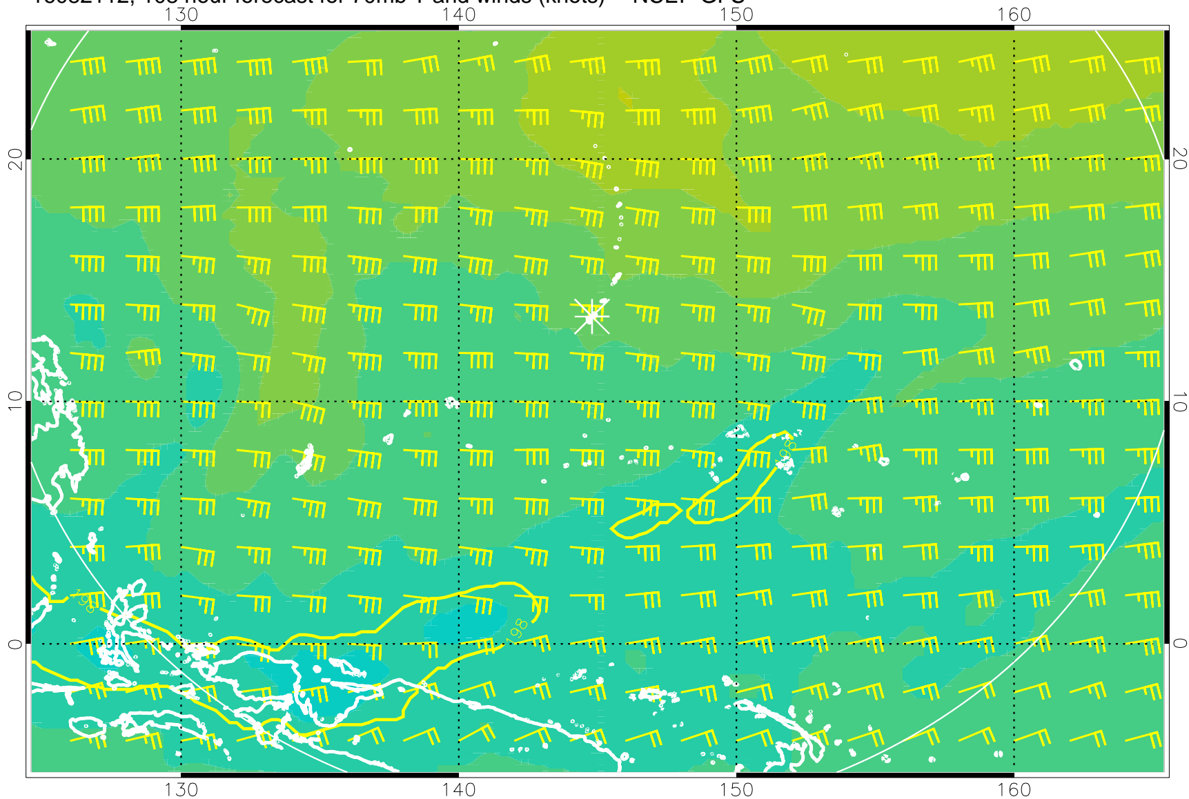
16082112, 108 hour forecast for 70mb T and winds (knots) -- NCEP GFS
