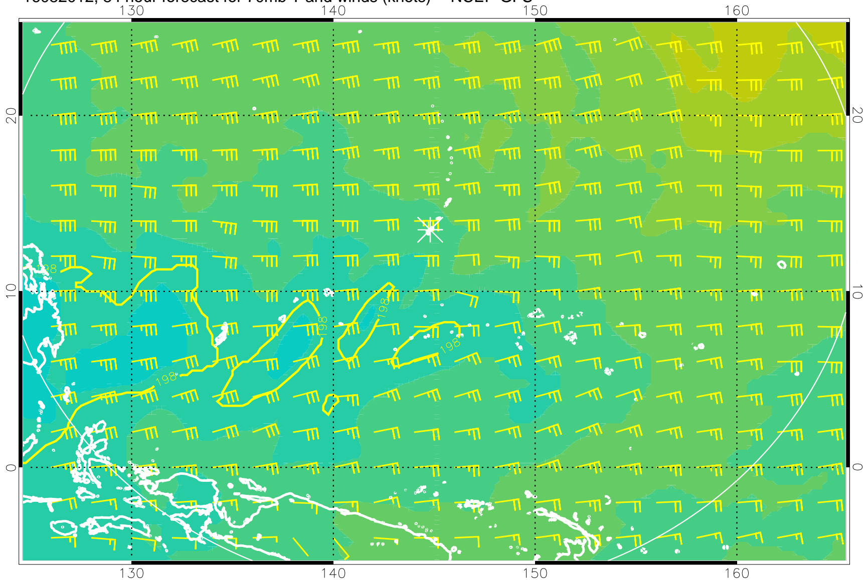
16082012, 84 hour forecast for 70mb T and winds (knots) -- NCEP GFS
