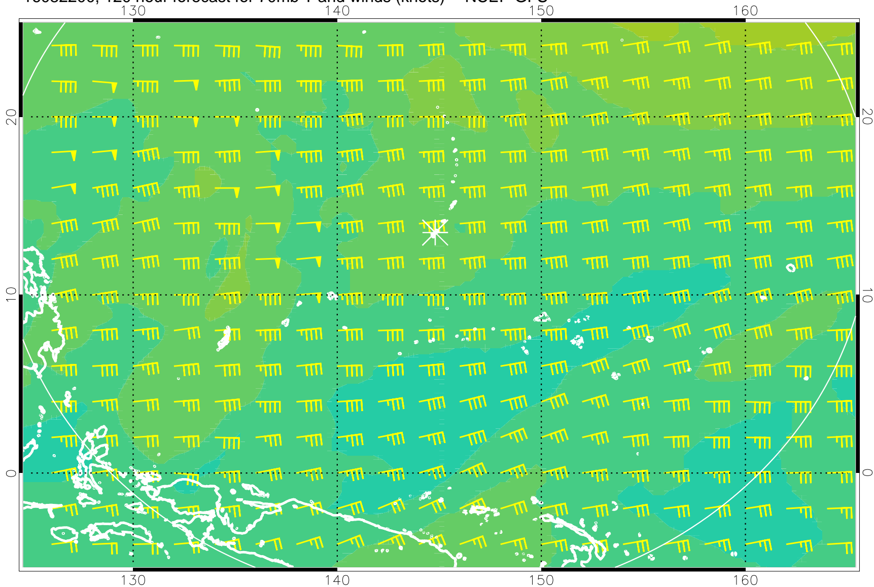
16082200, 120 hour forecast for 70mb T and winds (knots) -- NCEP GFS
