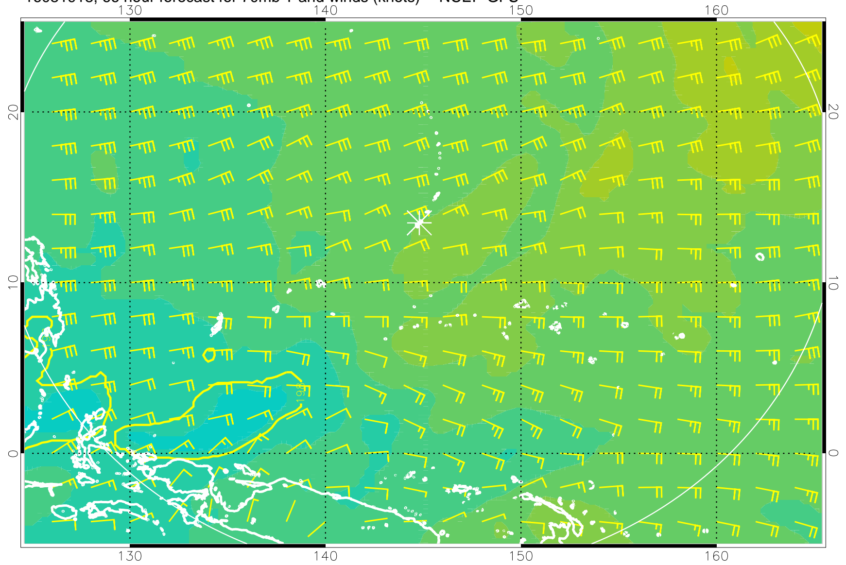
16081918, 66 hour forecast for 70mb T and winds (knots) -- NCEP GFS
