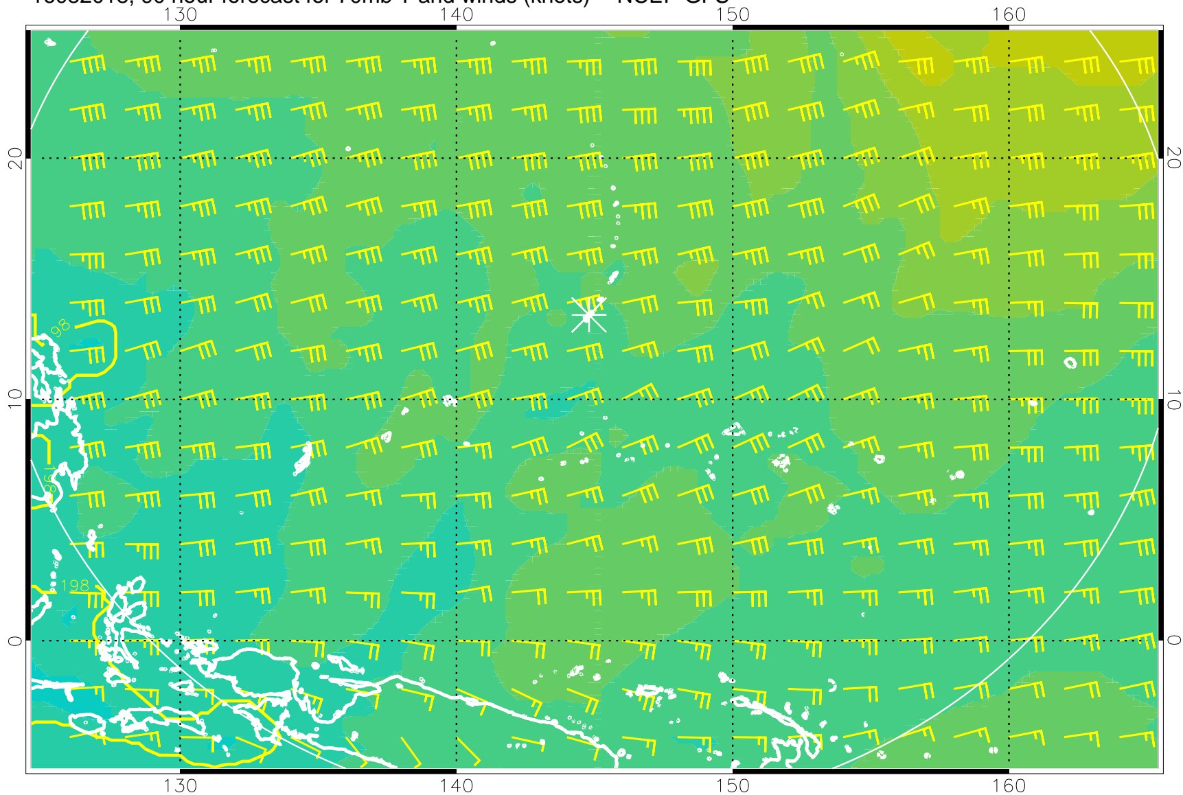
16082018, 90 hour forecast for 70mb T and winds (knots) -- NCEP GFS
