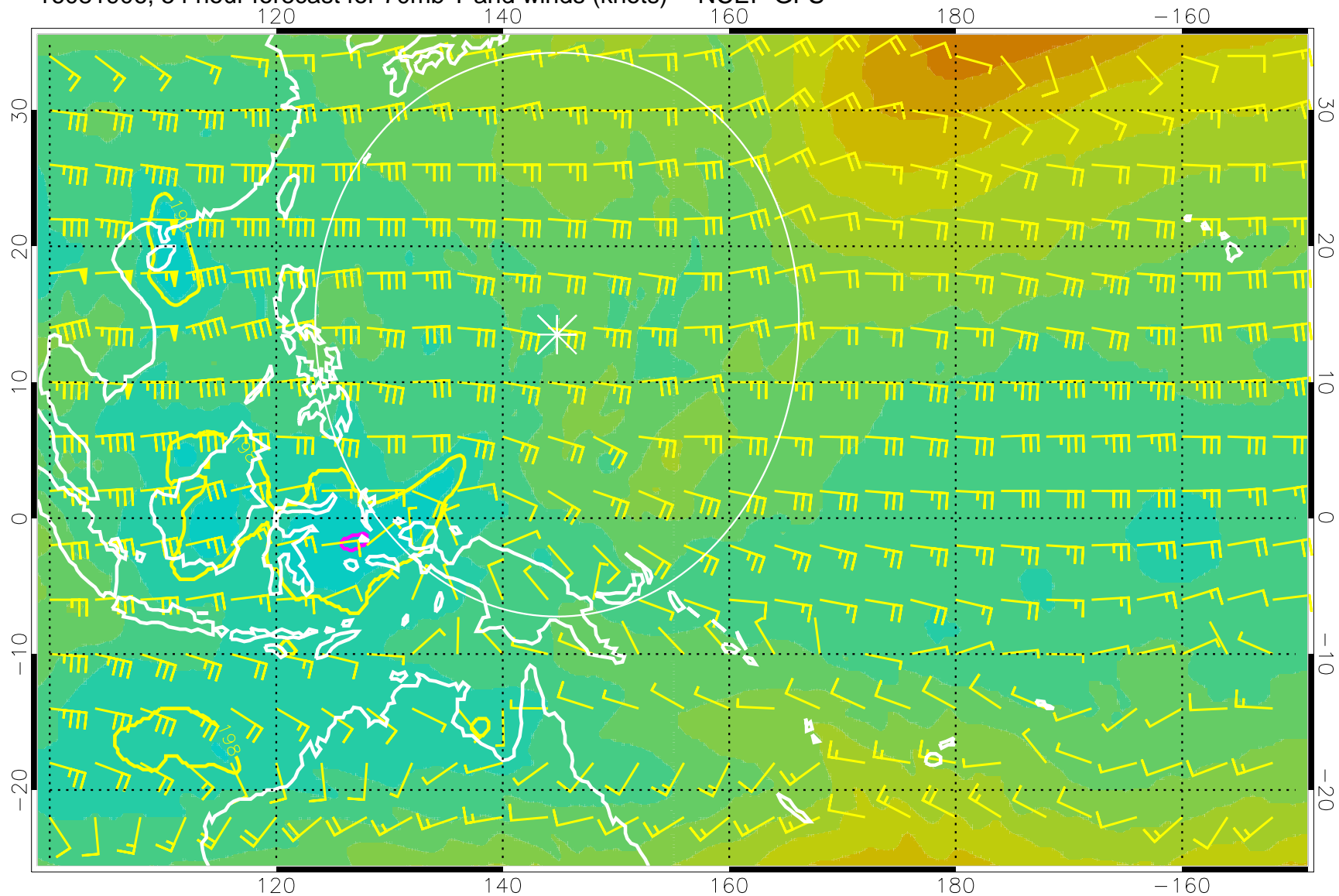
16081906, 54 hour forecast for 70mb T and winds (knots) -- NCEP GFS
