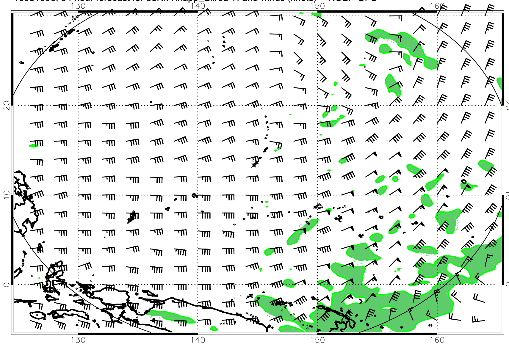
16081906, 54 hour forecast for 53Kft Knapp_Ellrod TI and winds (knots) -- NCEP GFS
