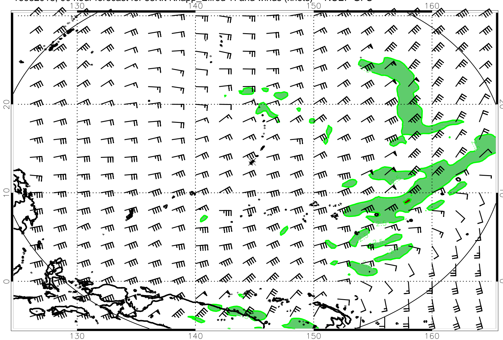
16082018, 90 hour forecast for 53Kft Knapp_Ellrod TI and winds (knots) -- NCEP GFS
