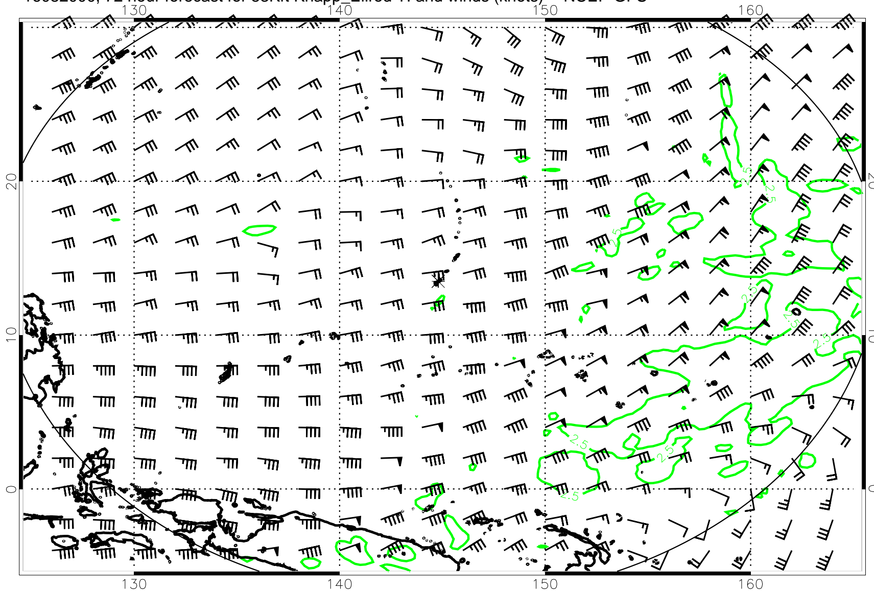
16082000, 72 hour forecast for 53Kft Knapp_Ellrod TI and winds (knots) -- NCEP GFS
