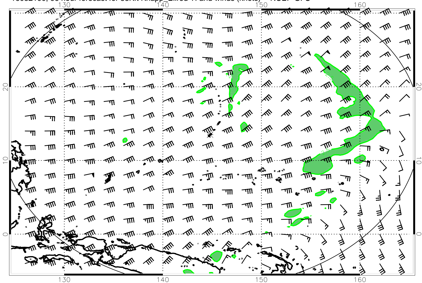
16082100, 96 hour forecast for 53Kft Knapp_Ellrod TI and winds (knots) -- NCEP GFS
