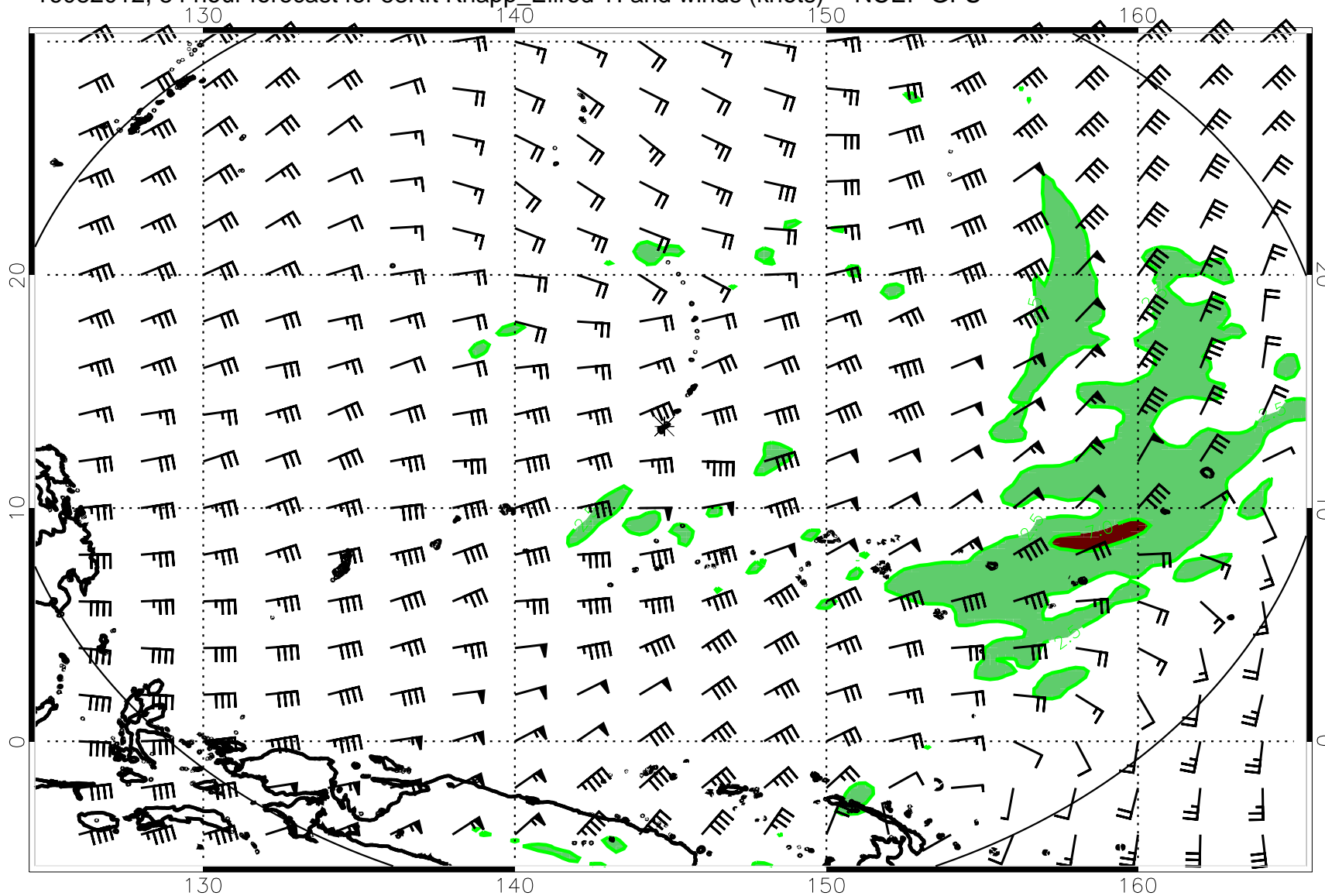
16082012, 84 hour forecast for 53Kft Knapp_Ellrod TI and winds (knots) -- NCEP GFS
