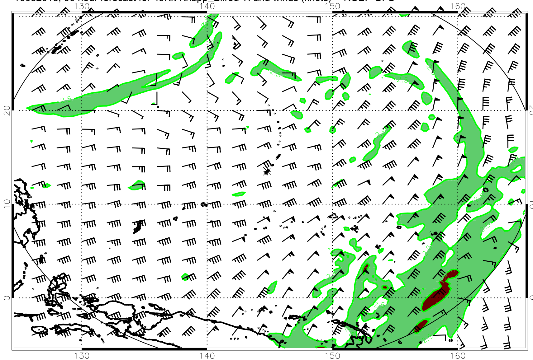
16082018, 90 hour forecast for 49Kft Knapp_Ellrod TI and winds (knots) -- NCEP GFS
