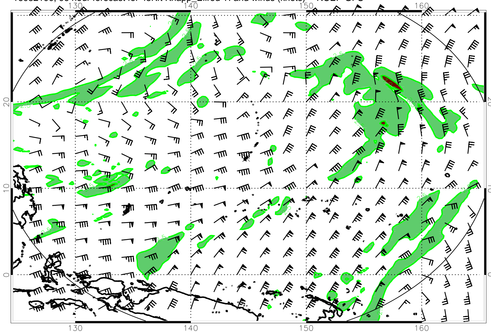
16082100, 96 hour forecast for 45Kft Knapp_Ellrod TI and winds (knots) -- NCEP GFS
