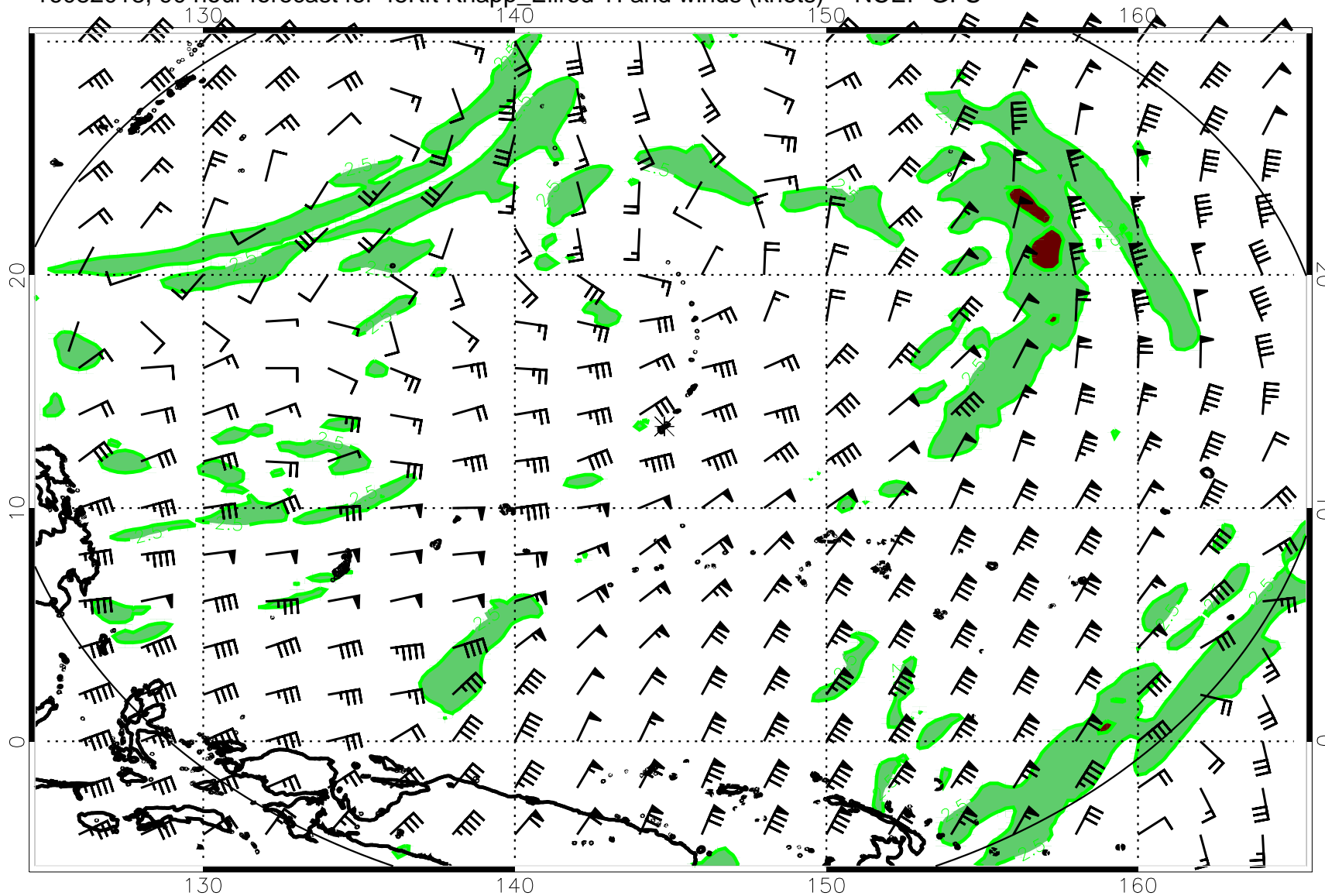
16082018, 90 hour forecast for 45Kft Knapp_Ellrod TI and winds (knots) -- NCEP GFS
