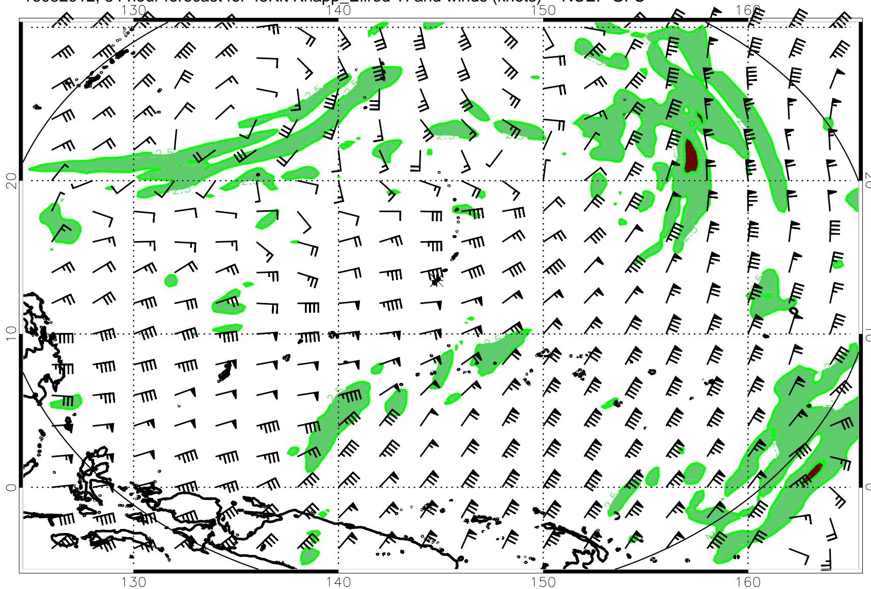
16082012, 84 hour forecast for 45Kft Knapp_Ellrod TI and winds (knots) -- NCEP GFS
