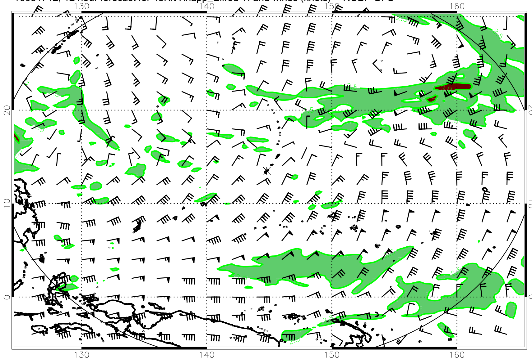
16081712, 12 hour forecast for 45Kft Knapp_Ellrod TI and winds (knots) -- NCEP GFS
