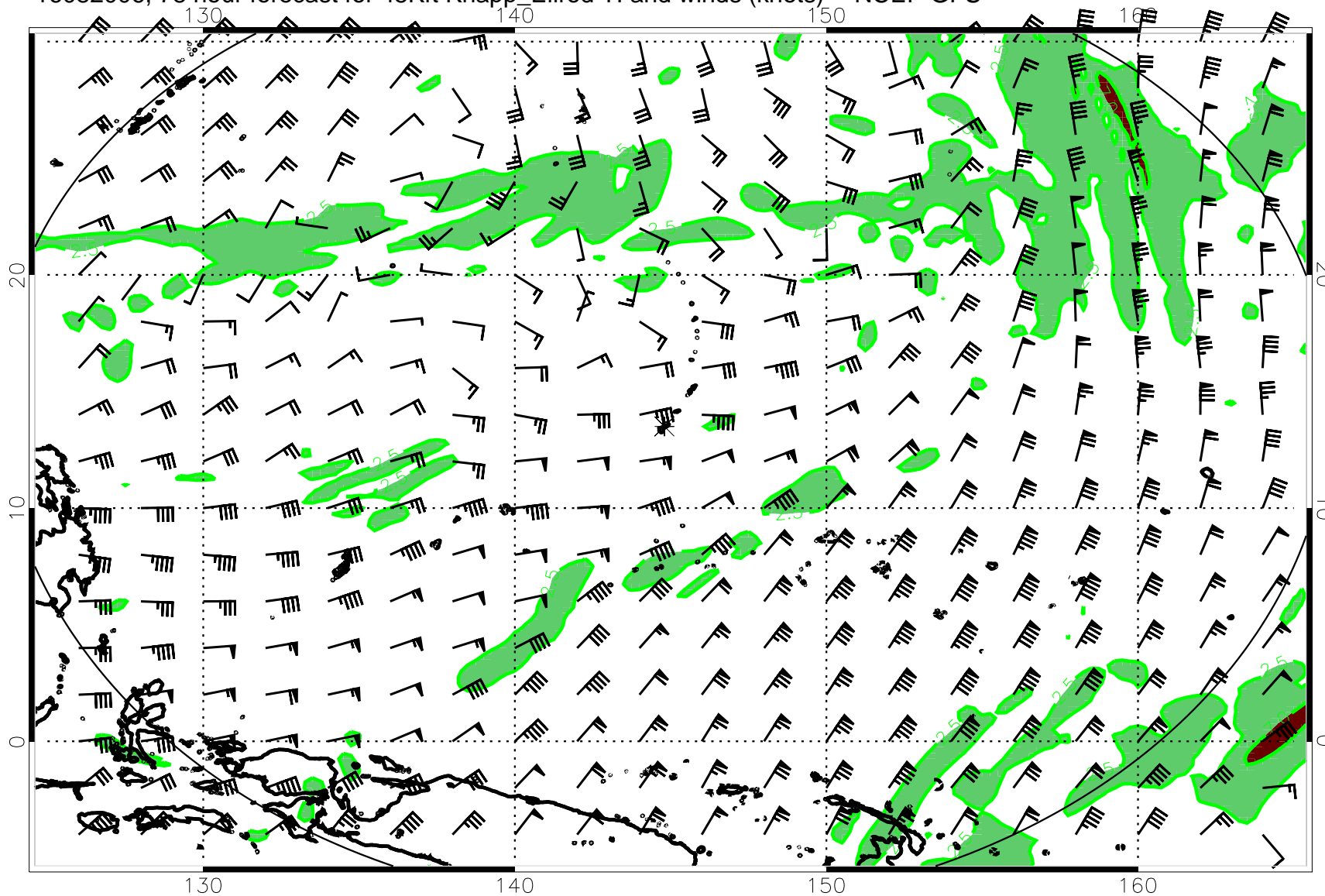
16082006, 78 hour forecast for 45Kft Knapp_Ellrod TI and winds (knots) -- NCEP GFS
