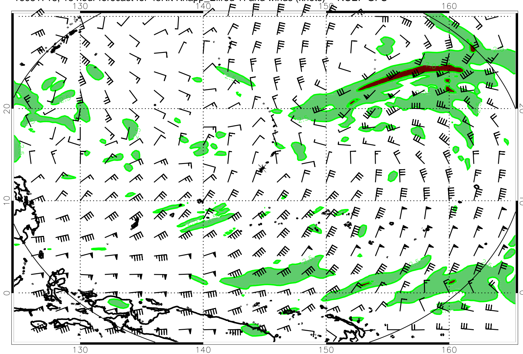
16081718, 18 hour forecast for 45Kft Knapp_Ellrod TI and winds (knots) -- NCEP GFS
