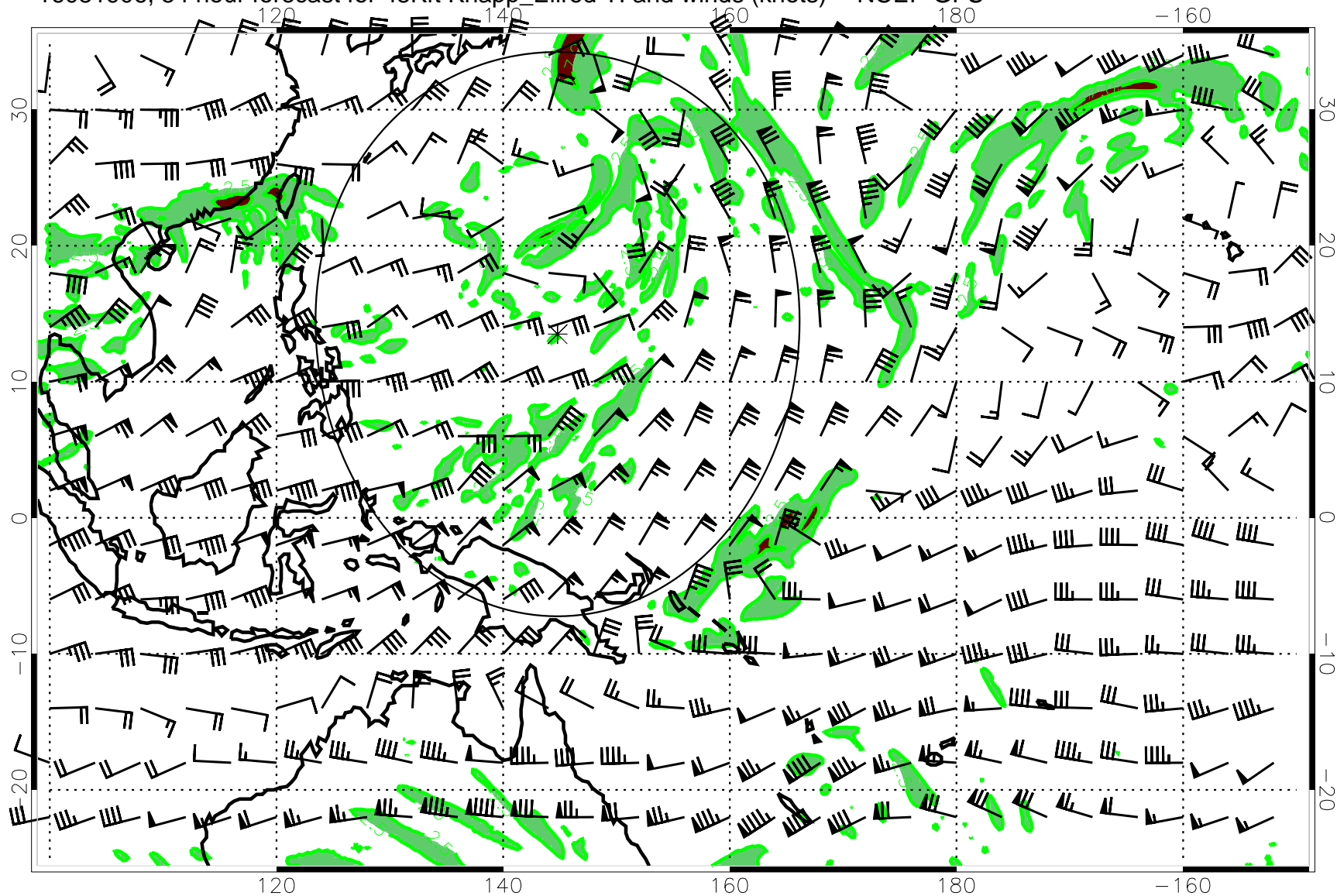
16081906, 54 hour forecast for 45Kft Knapp_Ellrod TI and winds (knots) -- NCEP GFS
