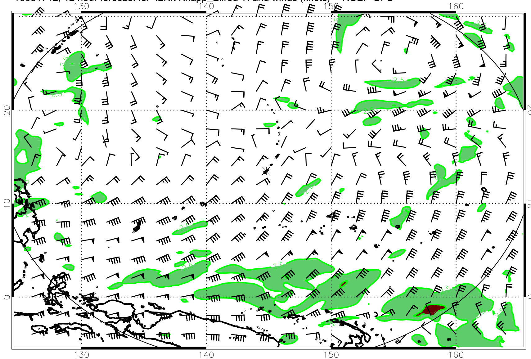
16081712, 12 hour forecast for 42Kft Knapp_Ellrod TI and winds (knots) -- NCEP GFS
