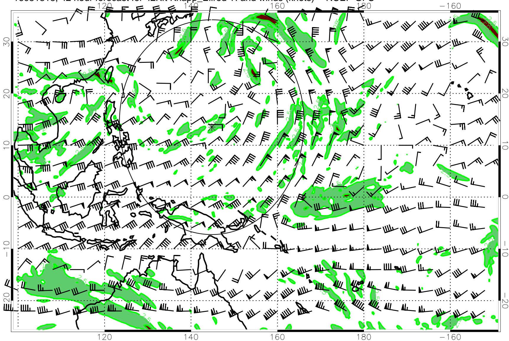
16081818, 42 hour forecast for 42Kft Knapp_Ellrod TI and winds (knots) -- NCEP GFS
