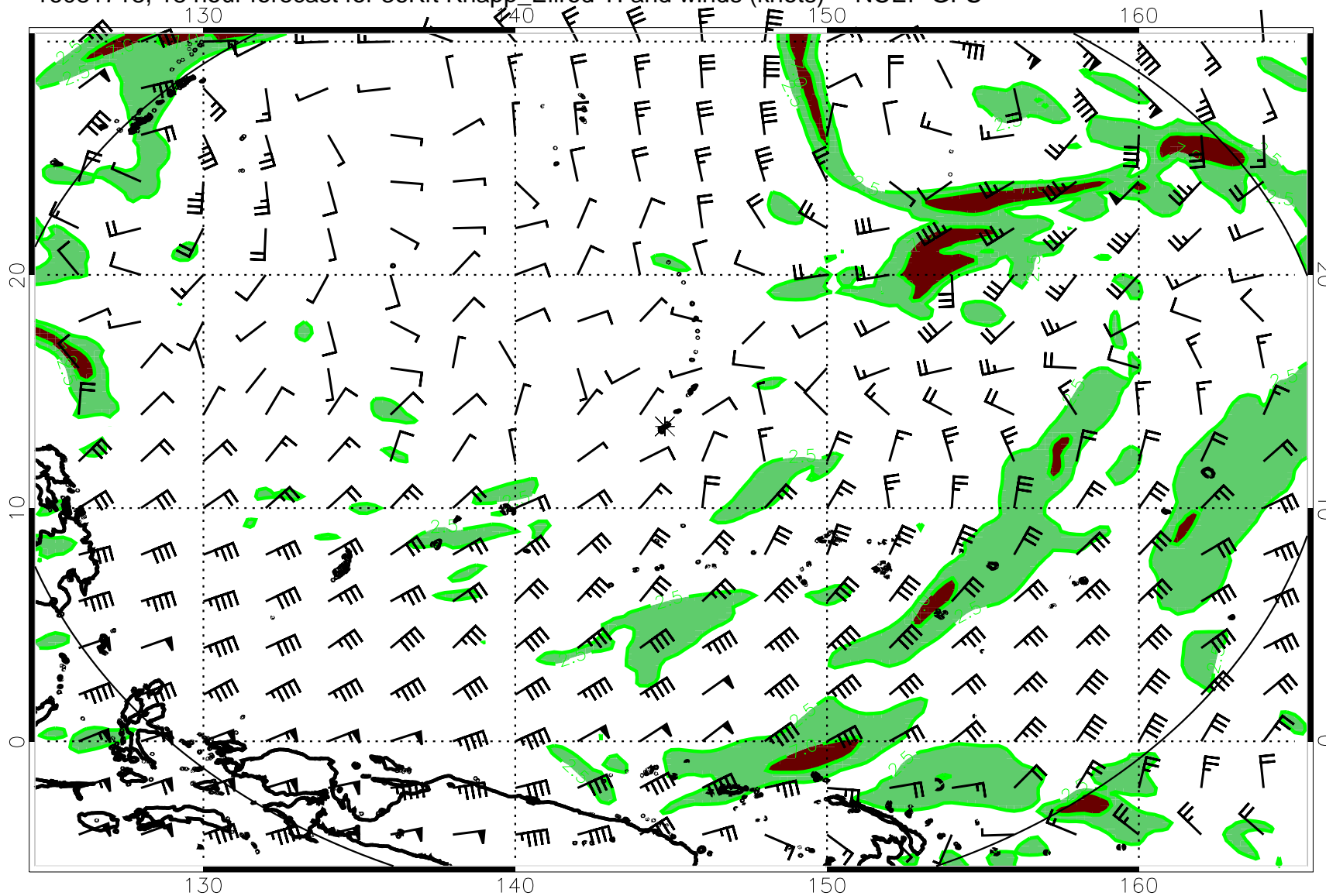
16081718, 18 hour forecast for 36Kft Knapp_Ellrod TI and winds (knots) -- NCEP GFS
