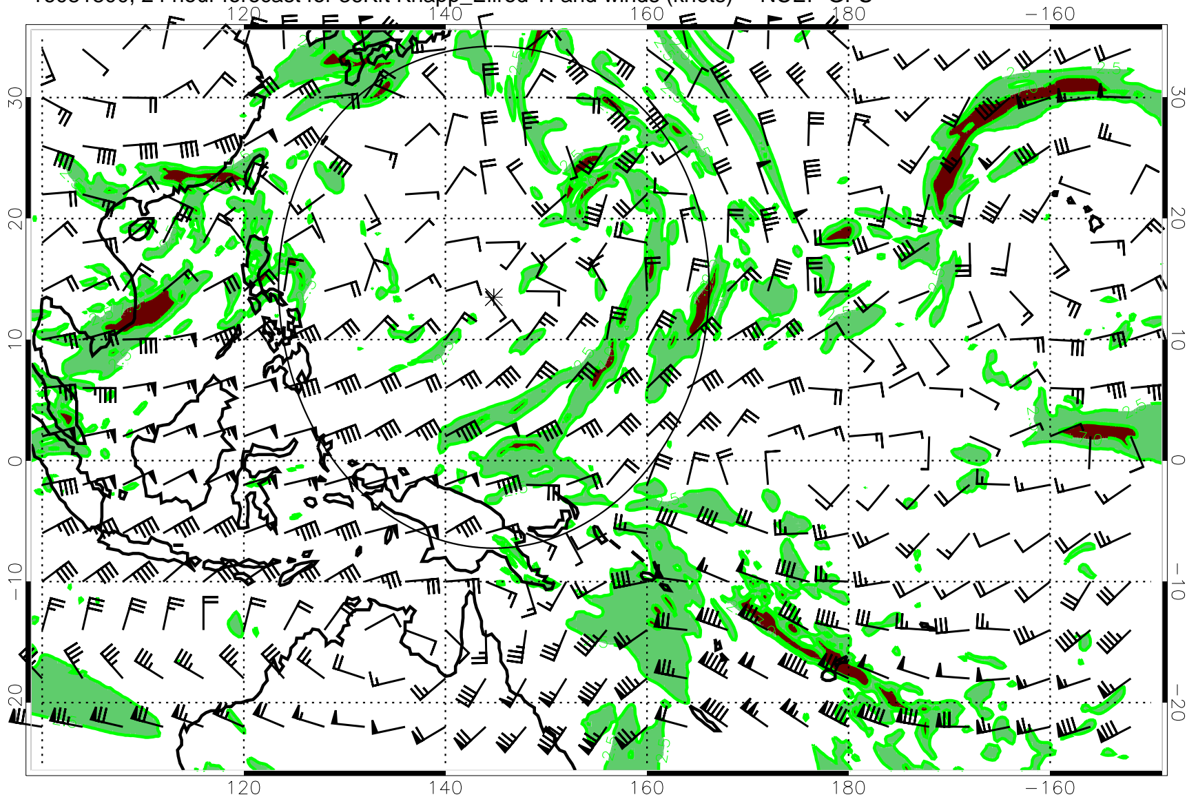
16081800, 24 hour forecast for 36Kft Knapp_Ellrod TI and winds (knots) -- NCEP GFS
