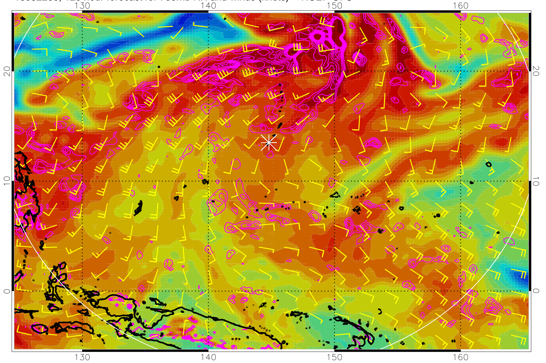
16082200, 120 hour forecast for 700mb RH and winds (knots) -- NCEP GFS
