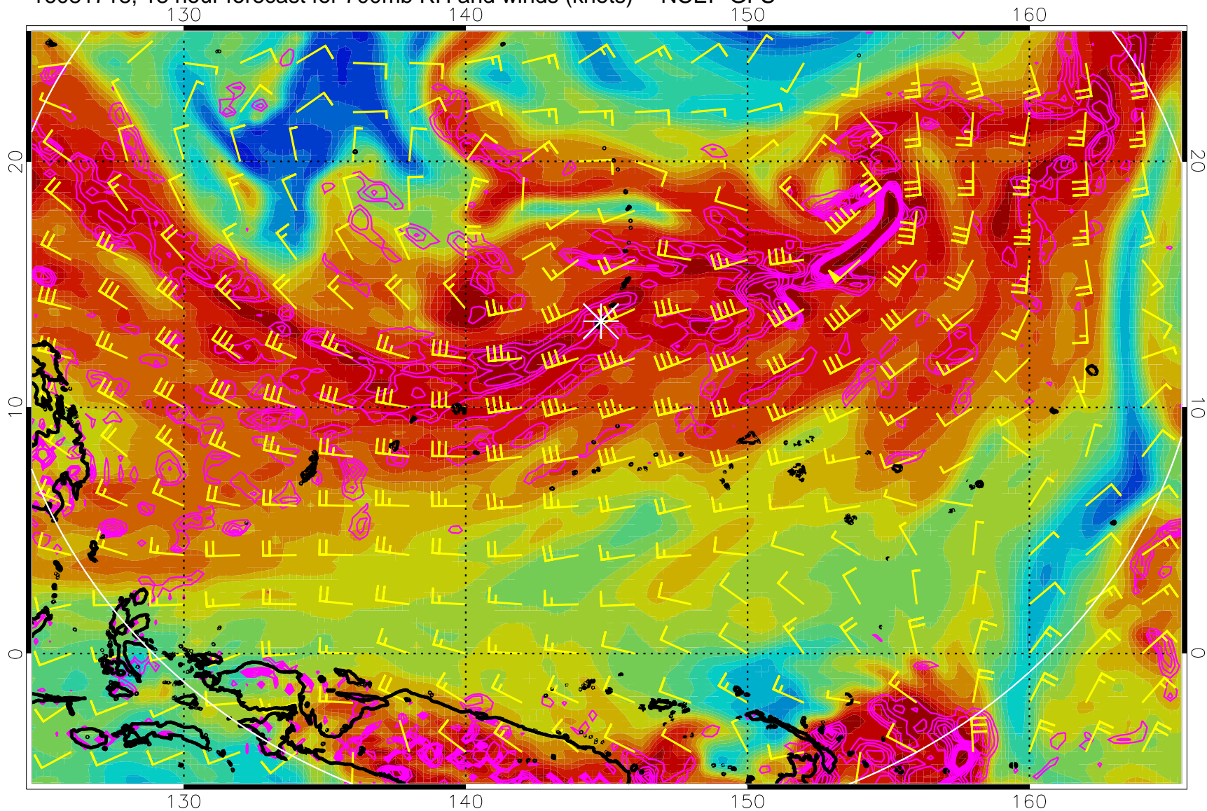
16081718, 18 hour forecast for 700mb RH and winds (knots) -- NCEP GFS
