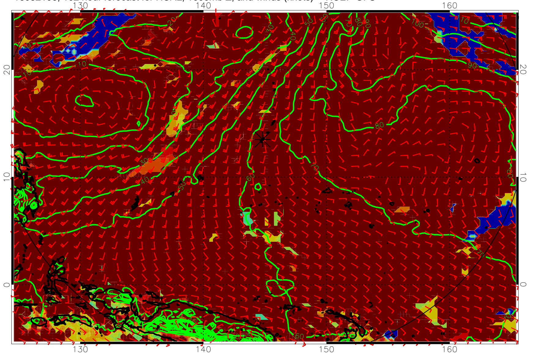
16082106, 102 hour forecast for HCAL, 1000mb Z, and winds (knots) -- NCEP GFS
