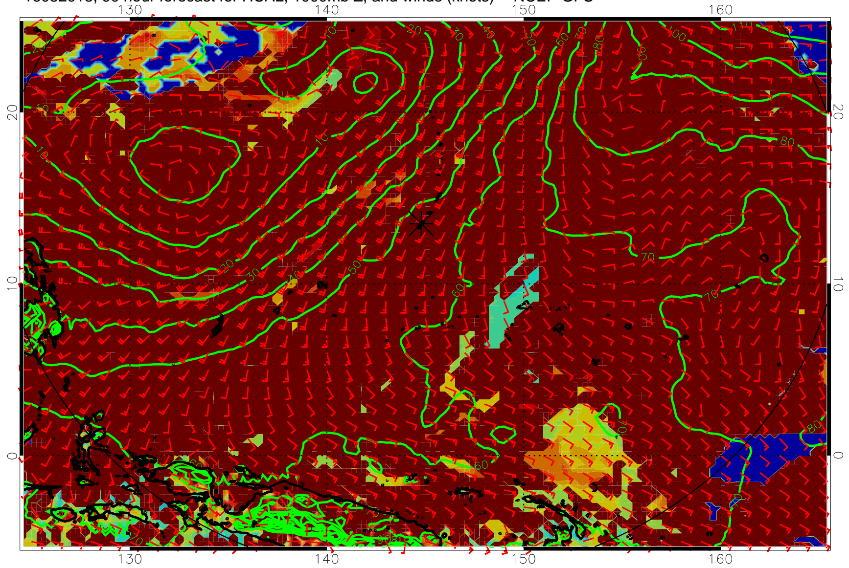
16082018, 90 hour forecast for HCAL, 1000mb Z, and winds (knots) -- NCEP GFS
