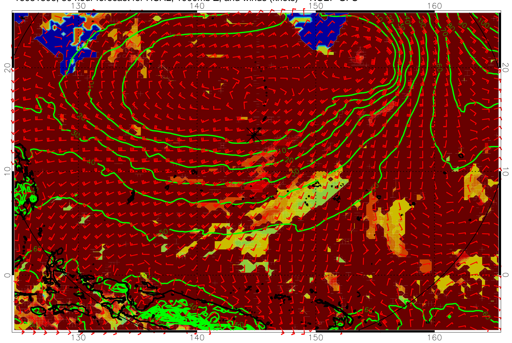
16081806, 30 hour forecast for HCAL, 1000mb Z, and winds (knots) -- NCEP GFS
