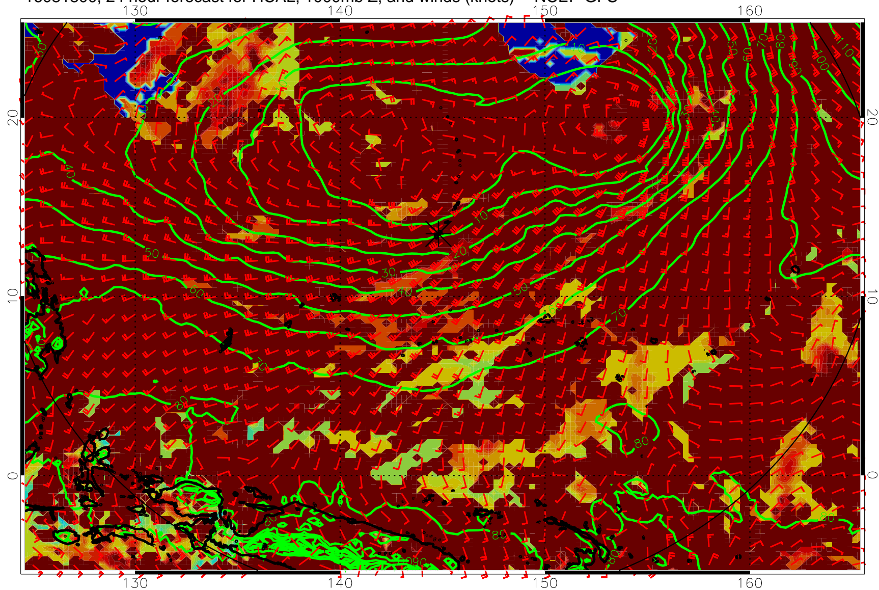
16081800, 24 hour forecast for HCAL, 1000mb Z, and winds (knots) -- NCEP GFS
