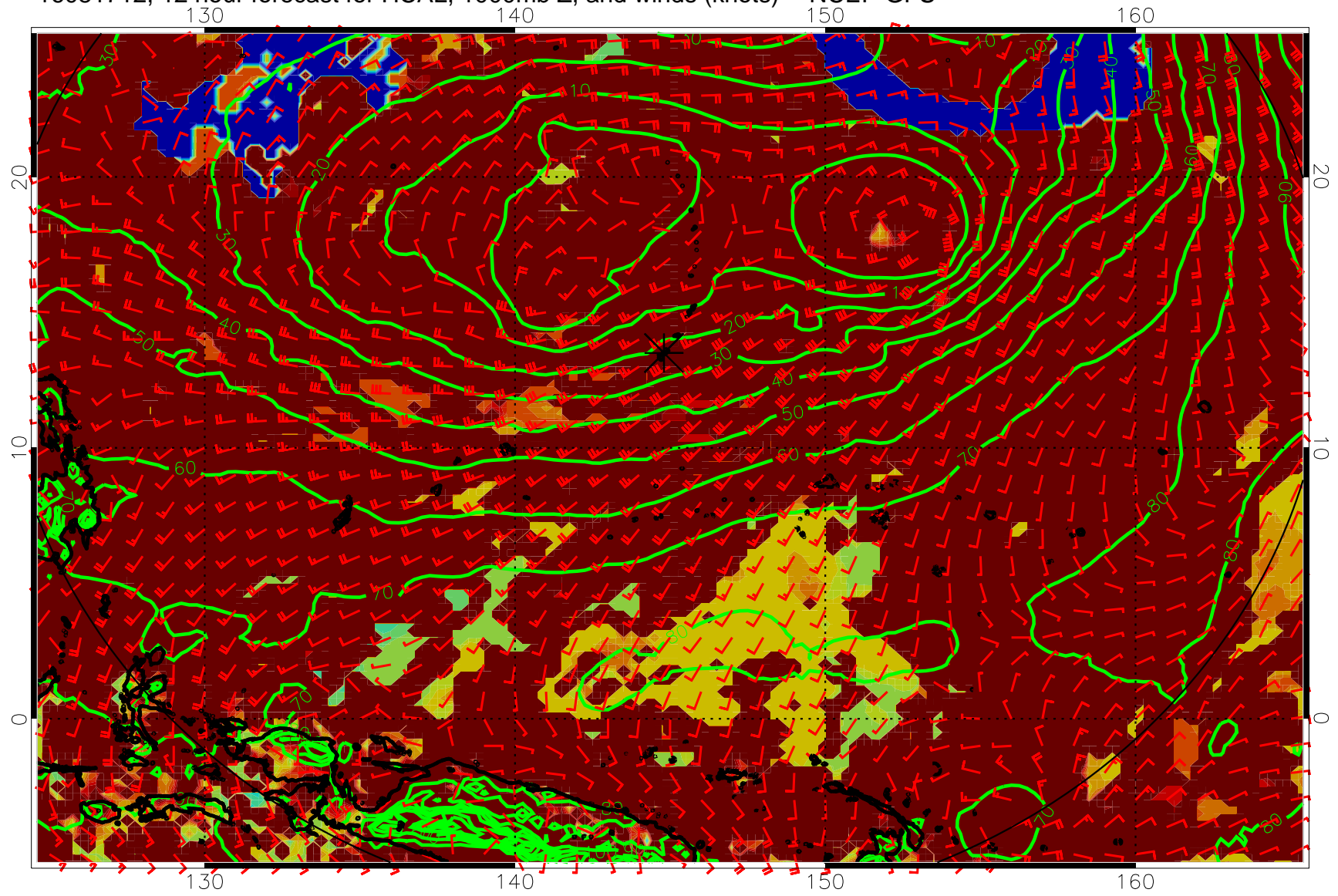
16081712, 12 hour forecast for HCAL, 1000mb Z, and winds (knots) -- NCEP GFS
