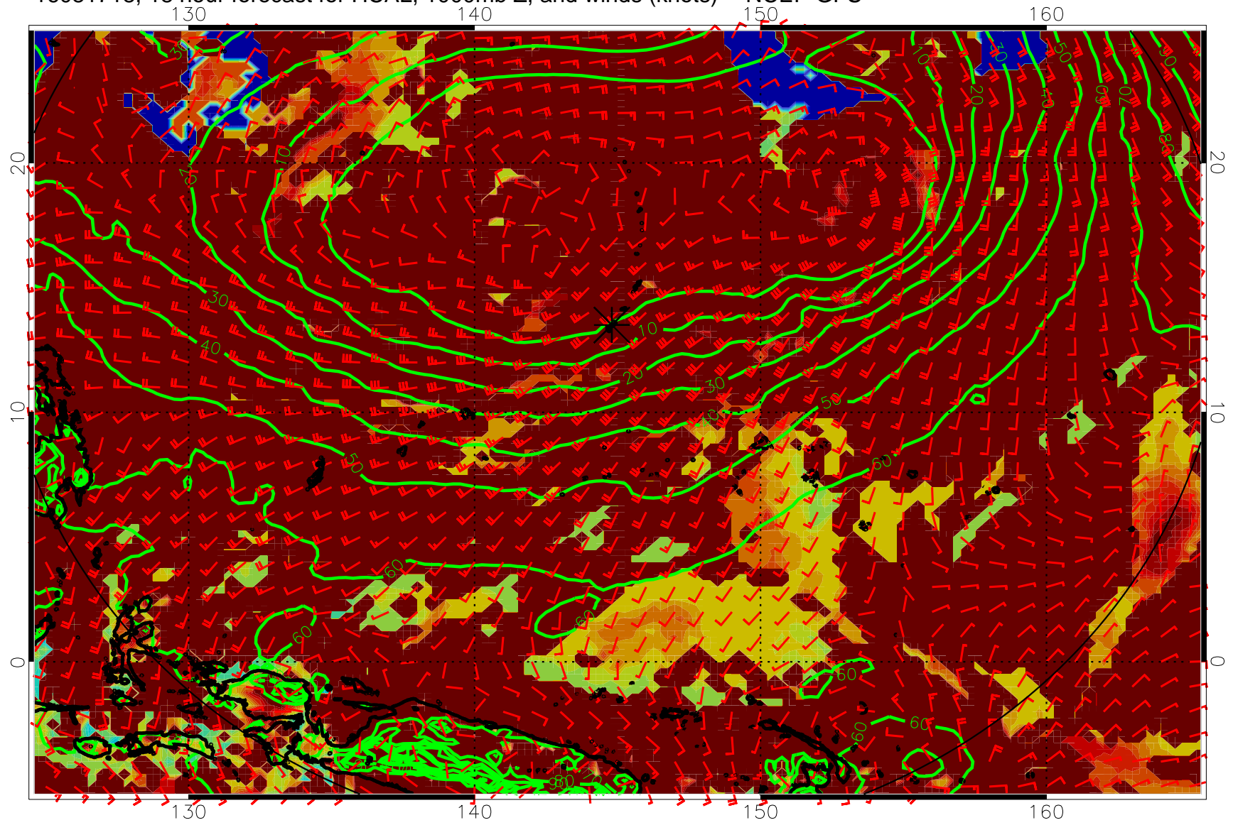
16081718, 18 hour forecast for HCAL, 1000mb Z, and winds (knots) -- NCEP GFS
