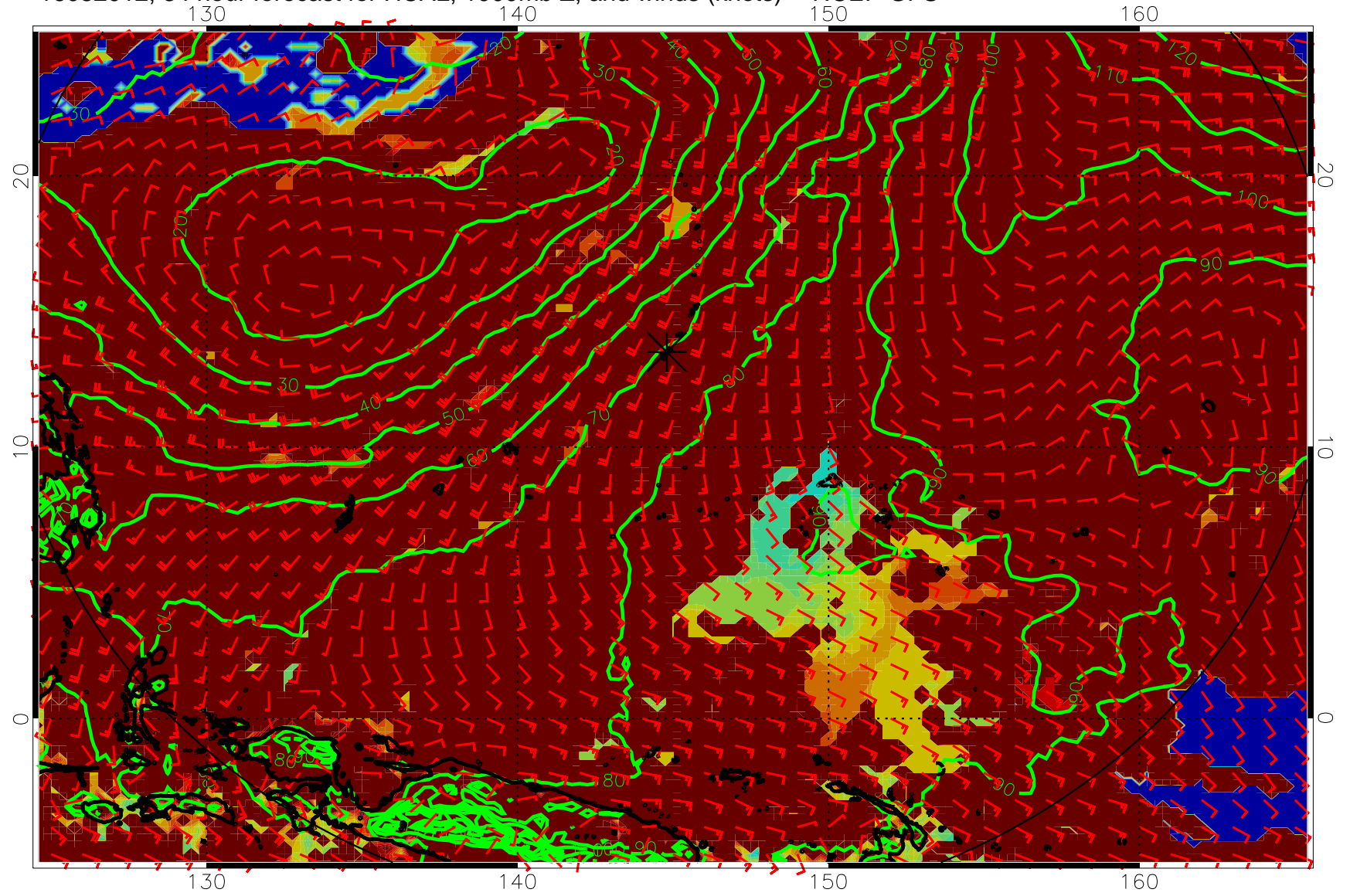
16082012, 84 hour forecast for HCAL, 1000mb Z, and winds (knots) -- NCEP GFS
