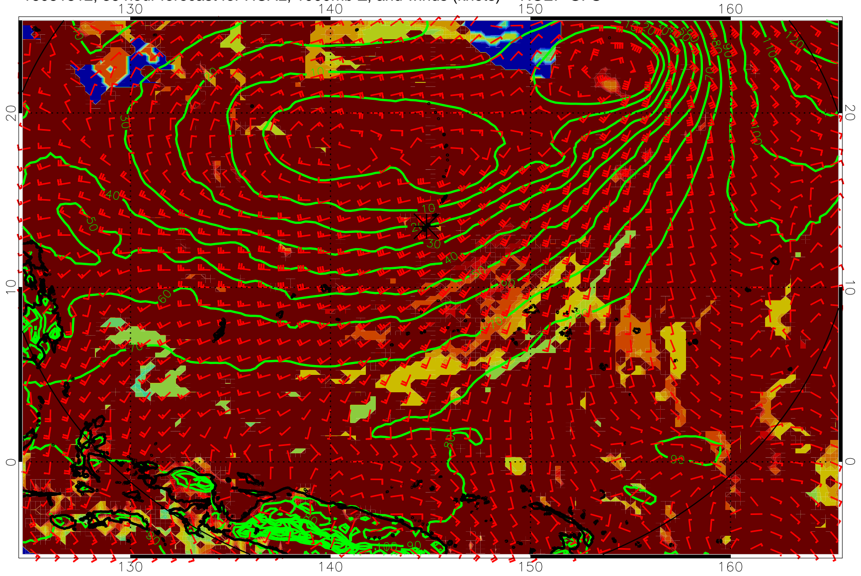
16081812, 36 hour forecast for HCAL, 1000mb Z, and winds (knots) -- NCEP GFS
