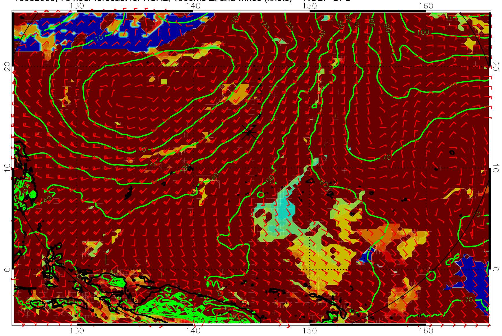
16082006, 78 hour forecast for HCAL, 1000mb Z, and winds (knots) -- NCEP GFS
