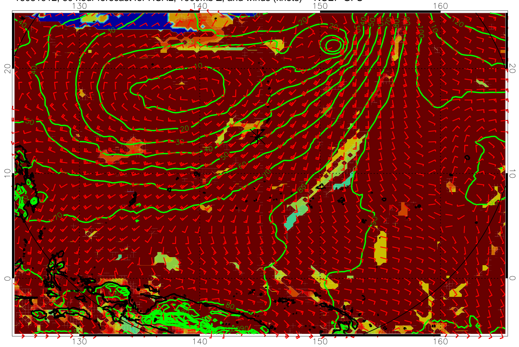
16081912, 60 hour forecast for HCAL, 1000mb Z, and winds (knots) -- NCEP GFS
