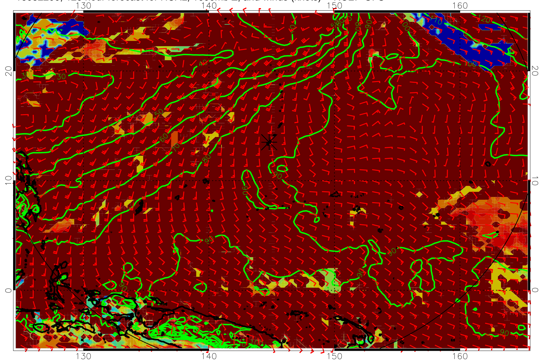
16082200, 120 hour forecast for HCAL, 1000mb Z, and winds (knots) -- NCEP GFS
