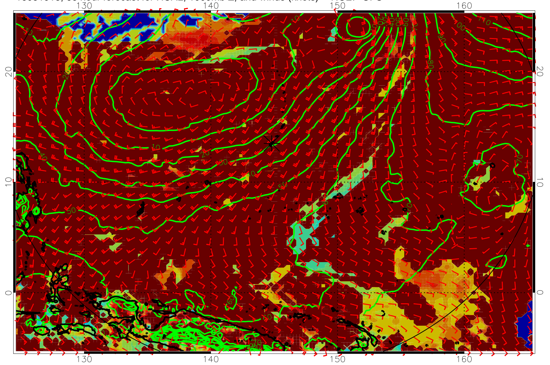
16081918, 66 hour forecast for HCAL, 1000mb Z, and winds (knots) -- NCEP GFS
