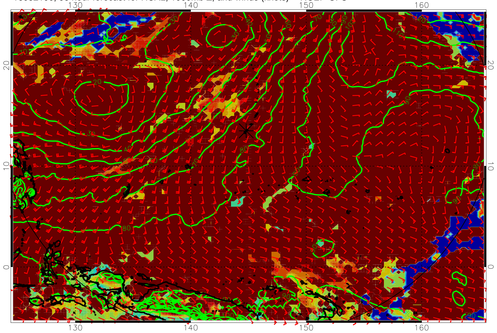
16082100, 96 hour forecast for HCAL, 1000mb Z, and winds (knots) -- NCEP GFS
