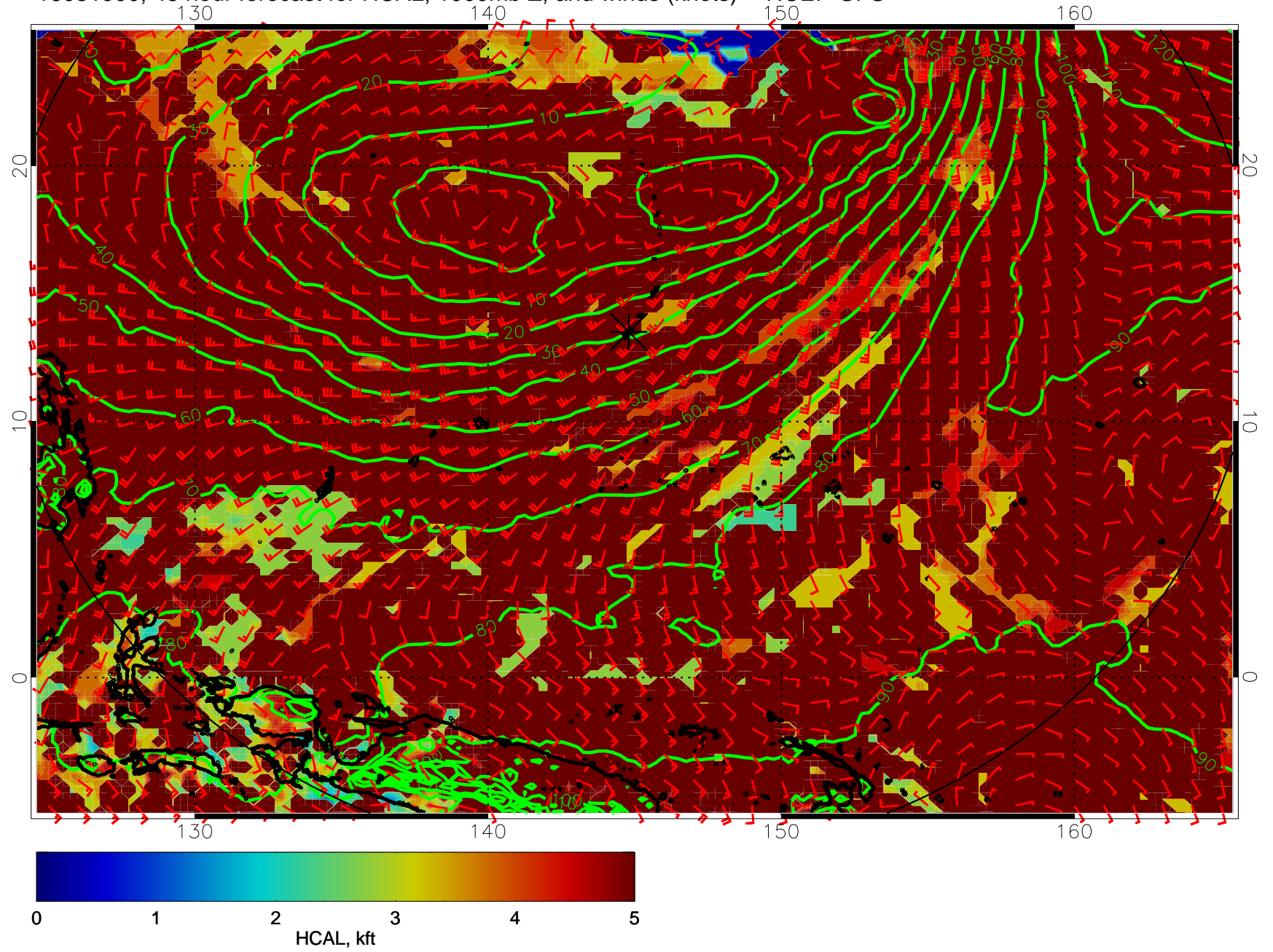
16081900, 48 hour forecast for HCAL, 1000mb Z, and winds (knots) -- NCEP GFS
