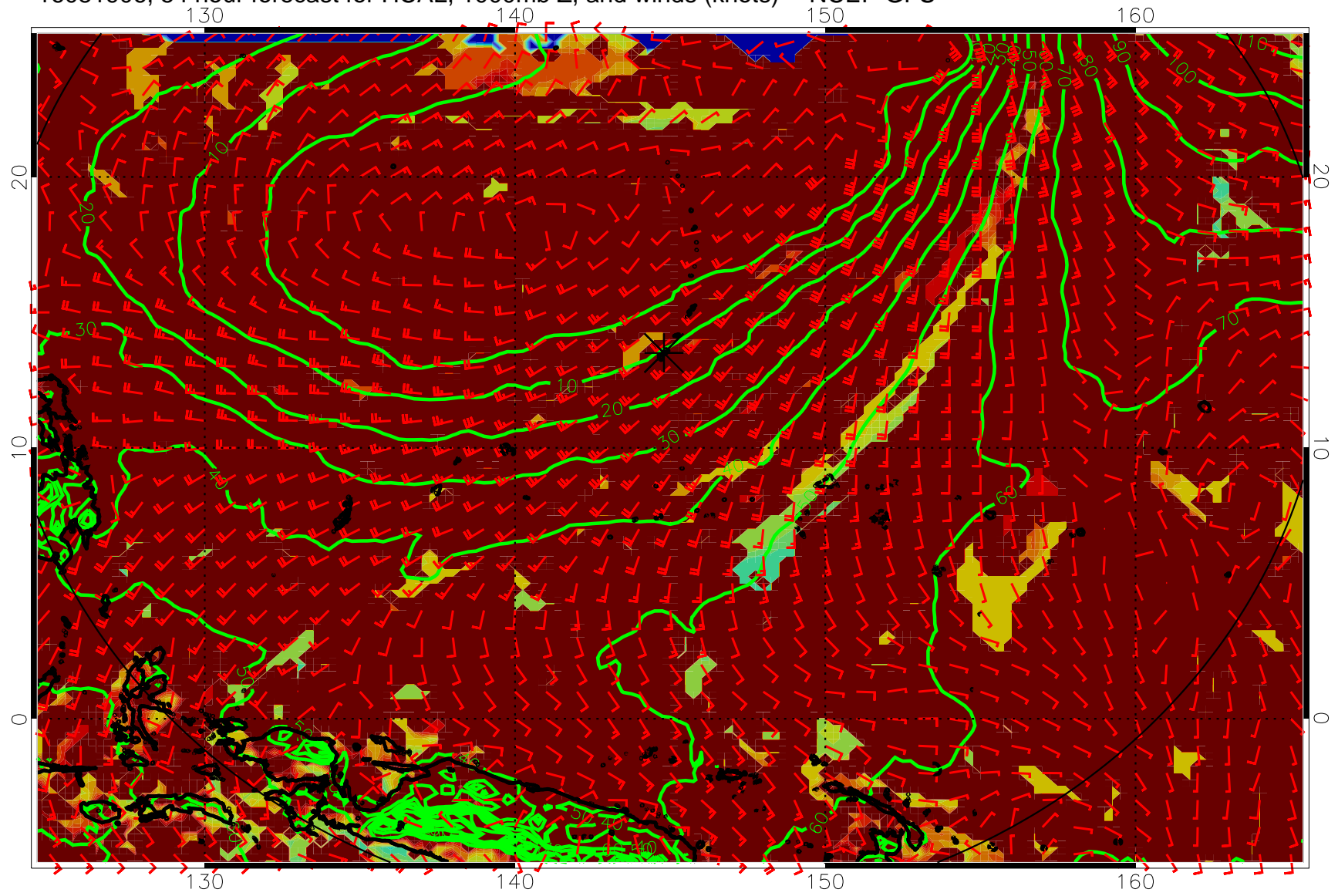
16081906, 54 hour forecast for HCAL, 1000mb Z, and winds (knots) -- NCEP GFS
