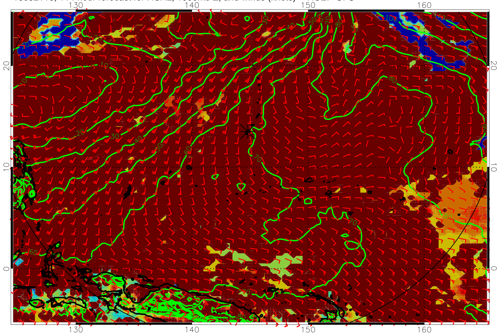
16082118, 114 hour forecast for HCAL, 1000mb Z, and winds (knots) -- NCEP GFS
