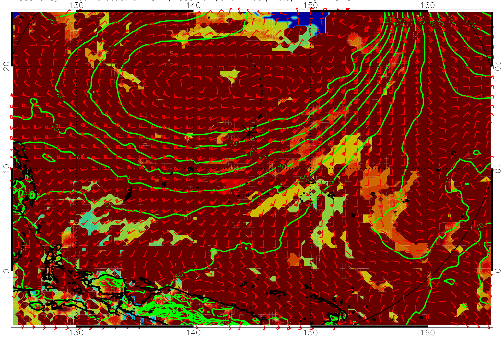
16081818, 42 hour forecast for HCAL, 1000mb Z, and winds (knots) -- NCEP GFS
