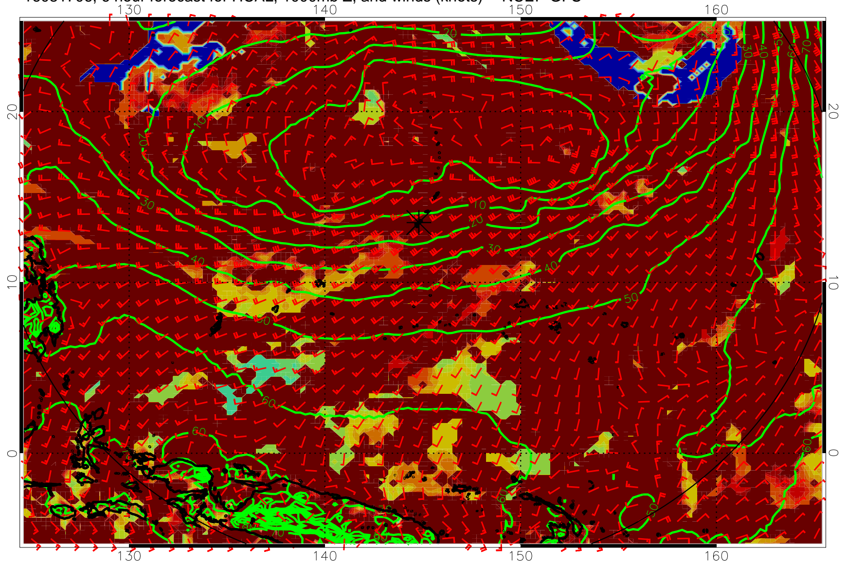
16081706, 6 hour forecast for HCAL, 1000mb Z, and winds (knots) -- NCEP GFS
