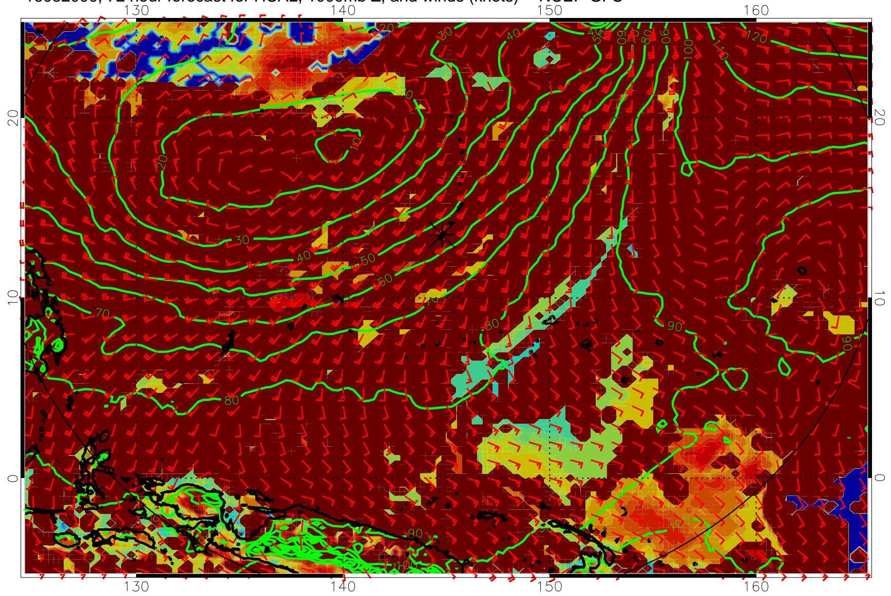
16082000, 72 hour forecast for HCAL, 1000mb Z, and winds (knots) -- NCEP GFS
