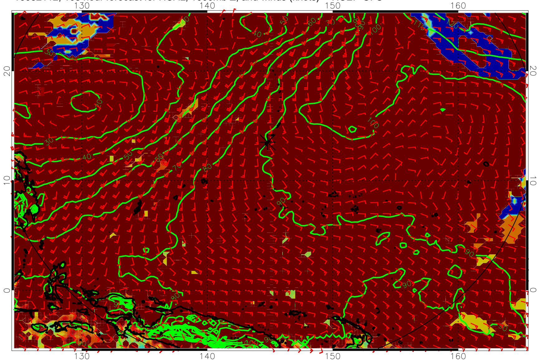
16082112, 108 hour forecast for HCAL, 1000mb Z, and winds (knots) -- NCEP GFS
