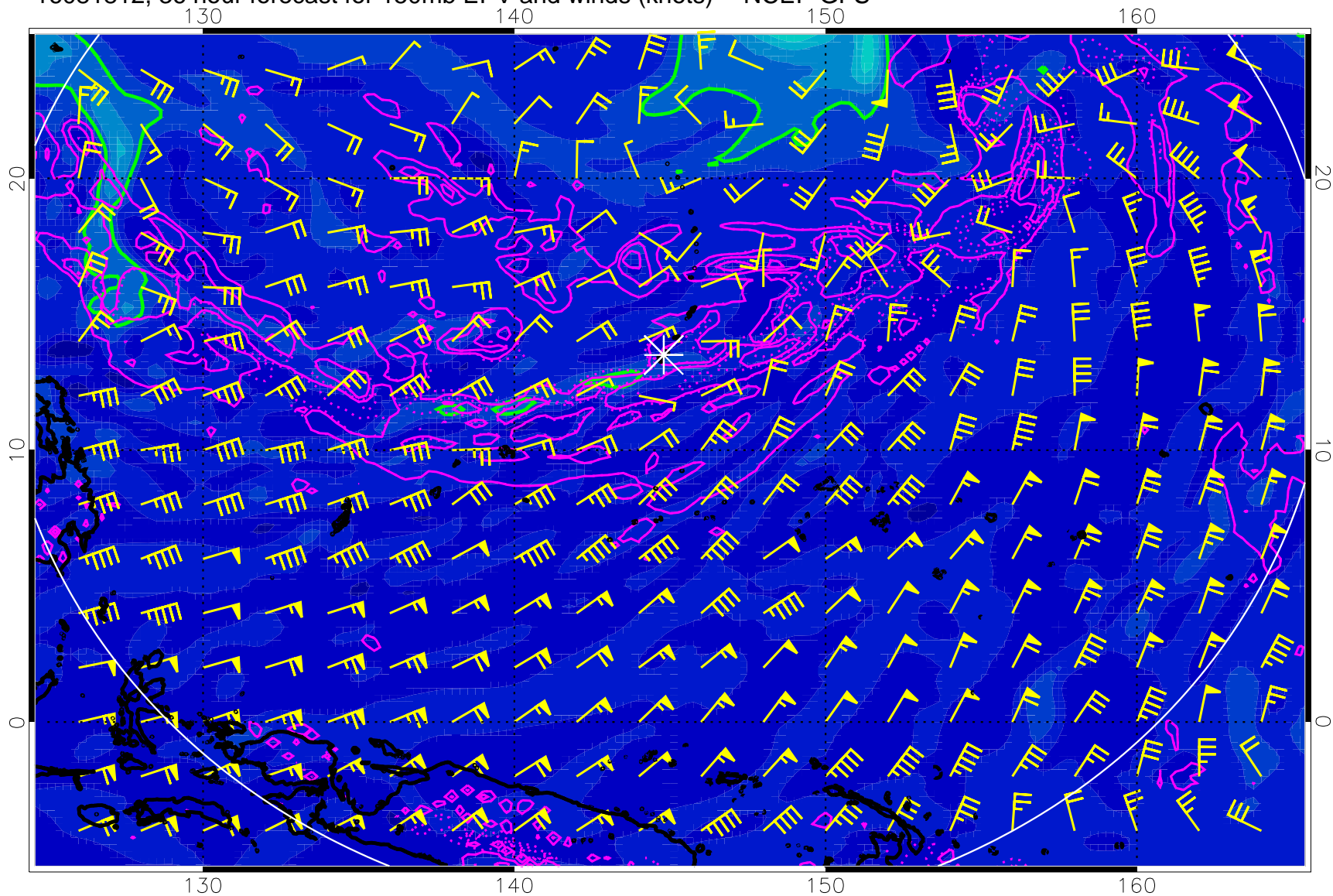
16081812, 36 hour forecast for 150mb EPV and winds (knots) -- NCEP GFS
