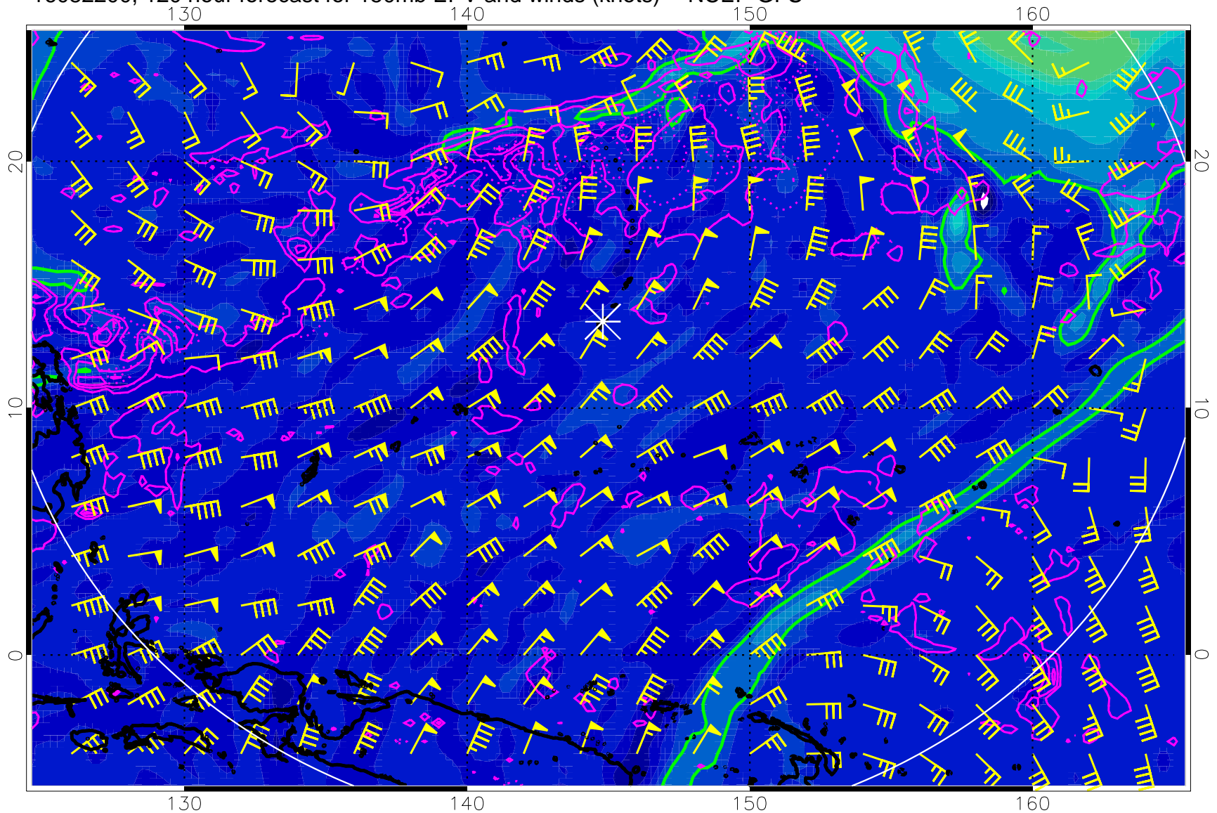
16082200, 120 hour forecast for 150mb EPV and winds (knots) -- NCEP GFS
