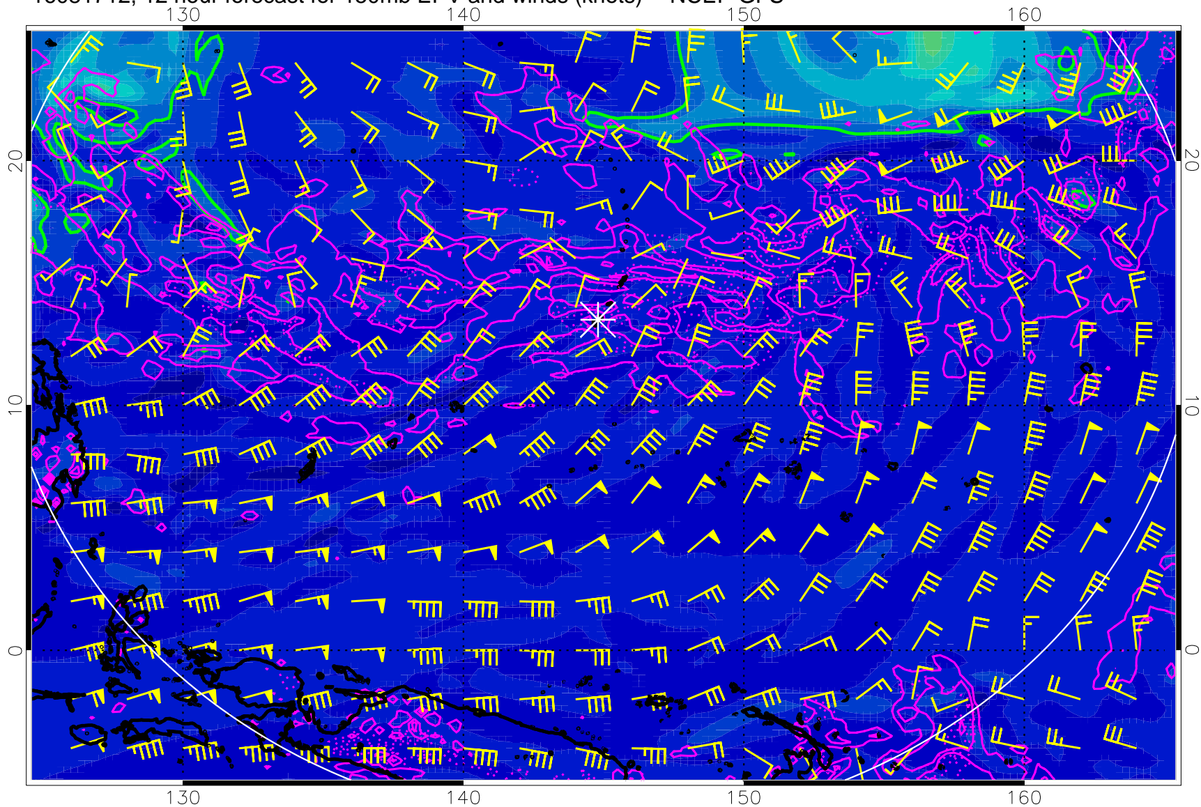
16081712, 12 hour forecast for 150mb EPV and winds (knots) -- NCEP GFS
