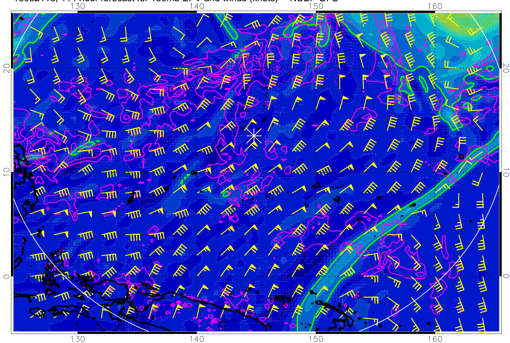
16082118, 114 hour forecast for 150mb EPV and winds (knots) -- NCEP GFS
