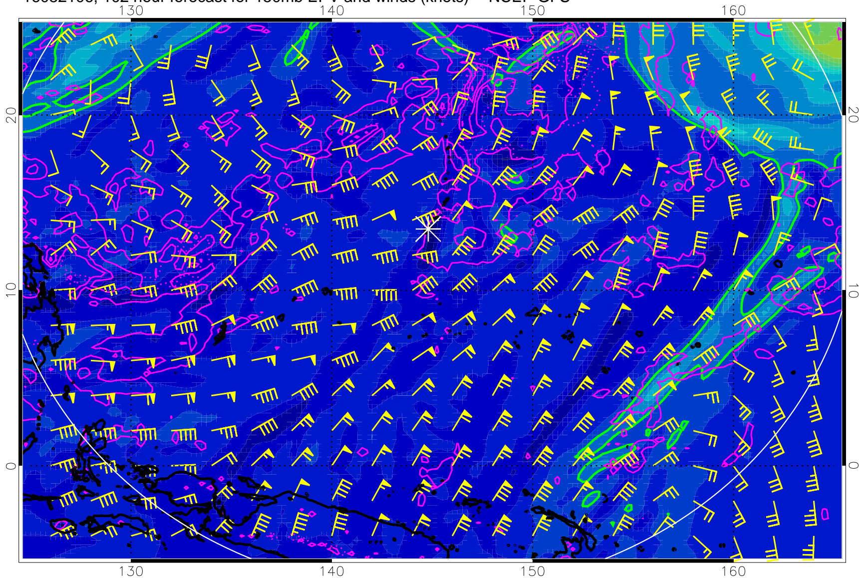
16082106, 102 hour forecast for 150mb EPV and winds (knots) -- NCEP GFS
