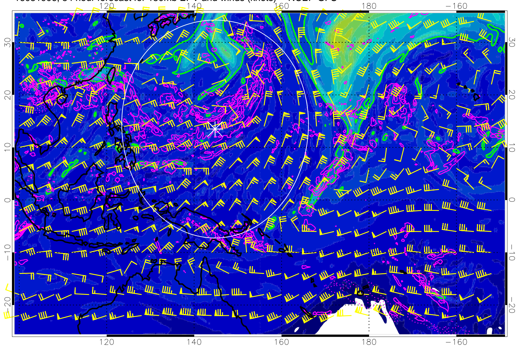
16081906, 54 hour forecast for 150mb EPV and winds (knots) -- NCEP GFS
