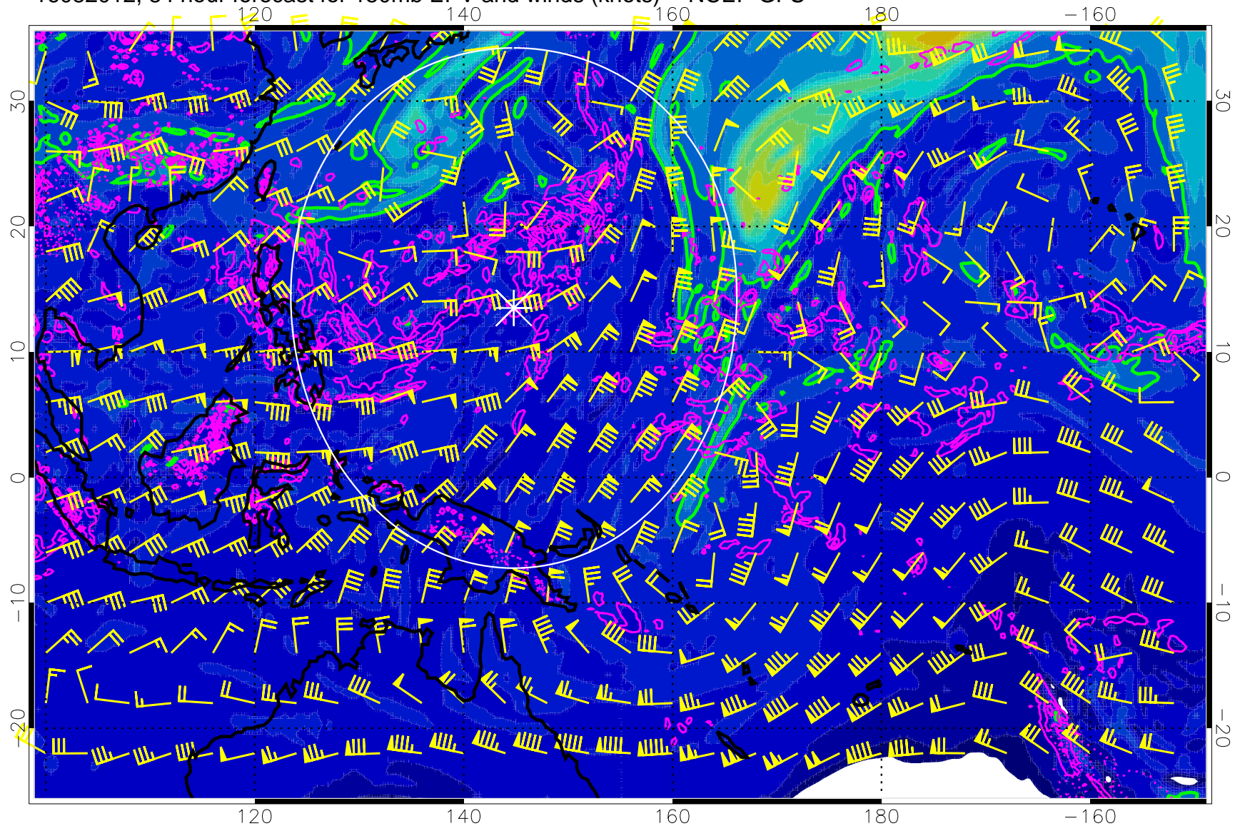
16082012, 84 hour forecast for 150mb EPV and winds (knots) -- NCEP GFS
