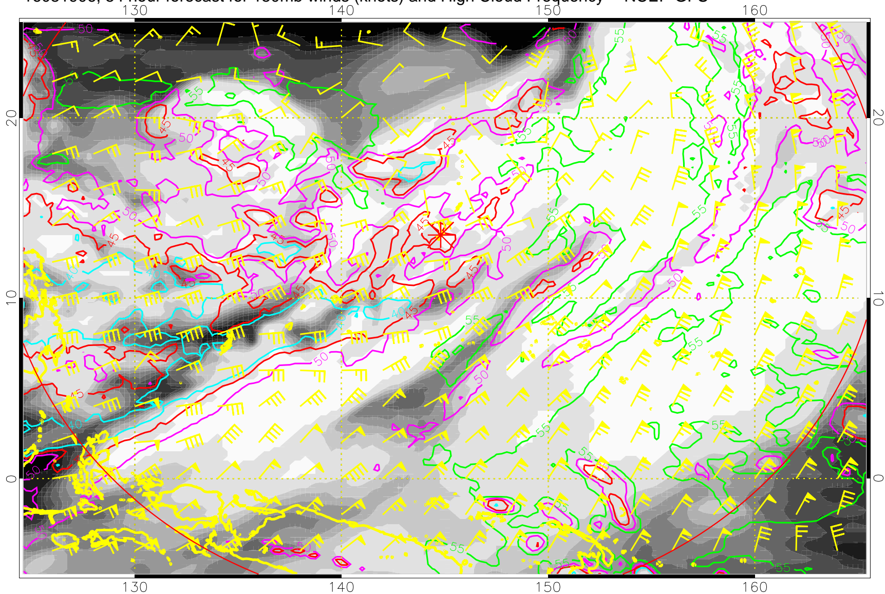
16081906, 54 hour forecast for 150mb winds (knots) and High Cloud Frequency -- NCEP GFS
