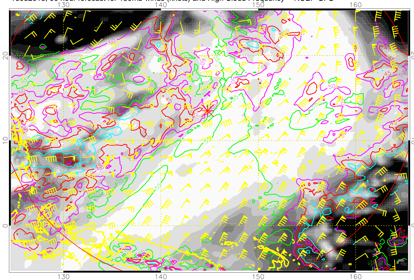
16082018, 90 hour forecast for 150mb winds (knots) and High Cloud Frequency -- NCEP GFS
