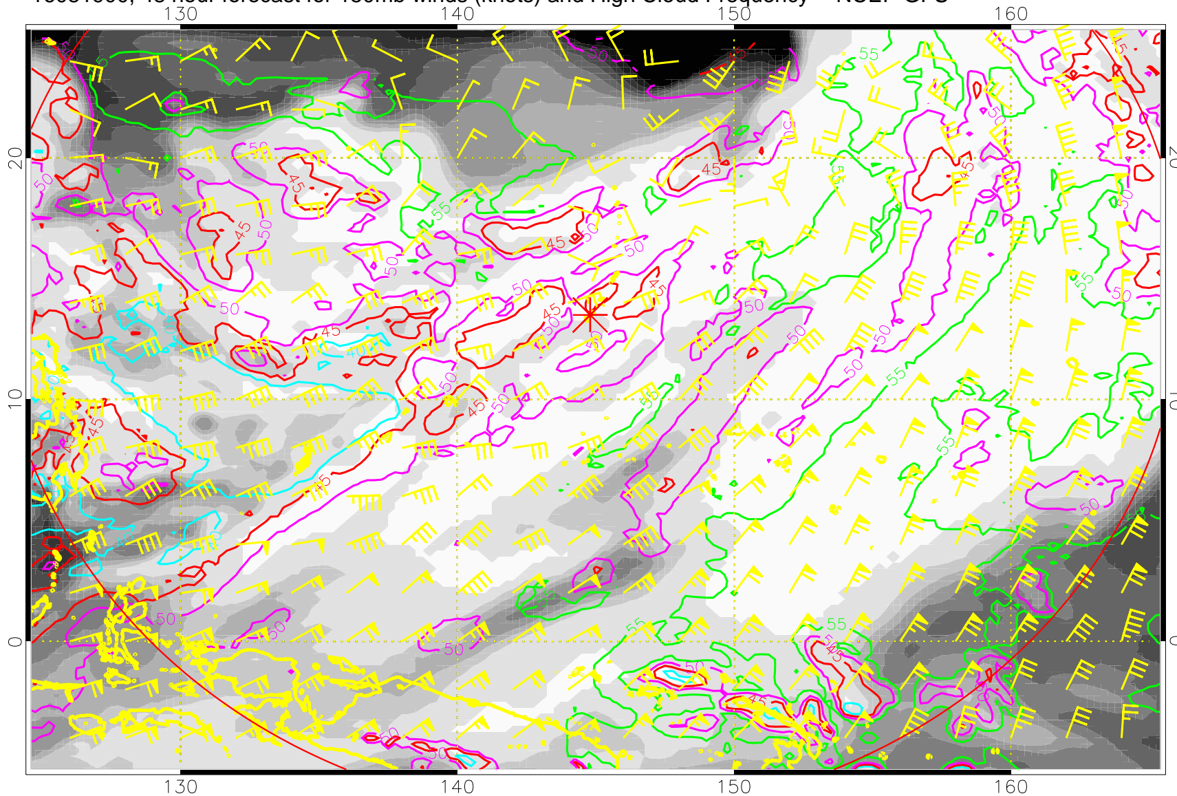
16081900, 48 hour forecast for 150mb winds (knots) and High Cloud Frequency -- NCEP GFS
