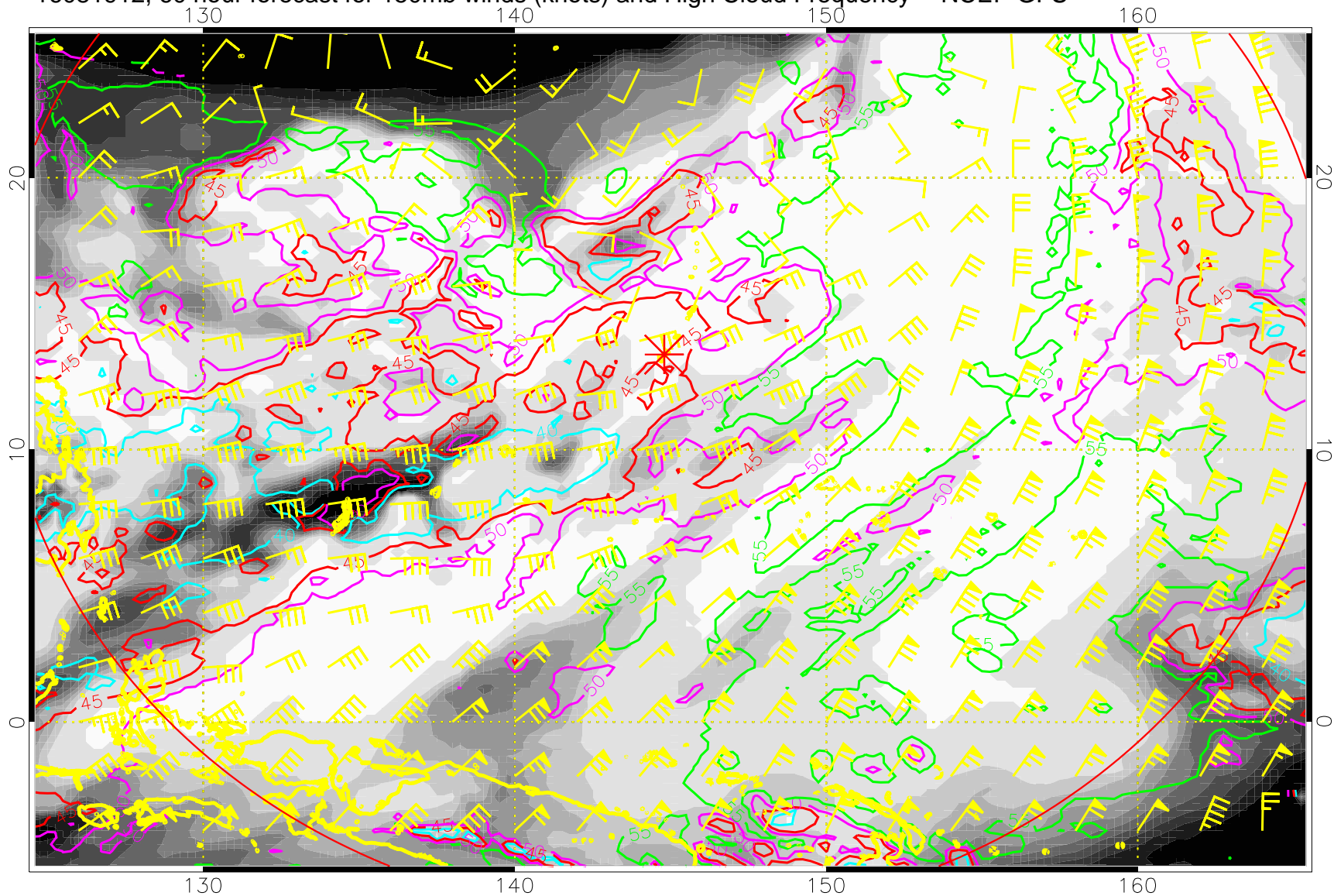
16081912, 60 hour forecast for 150mb winds (knots) and High Cloud Frequency -- NCEP GFS
