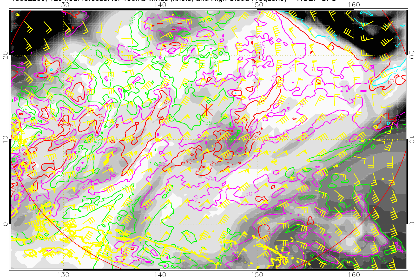
16082200, 120 hour forecast for 150mb winds (knots) and High Cloud Frequency -- NCEP GFS
