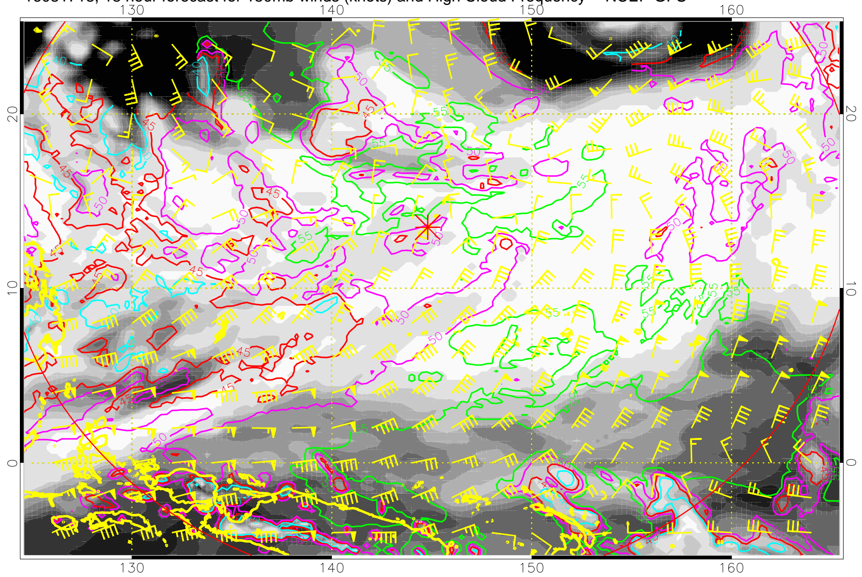
16081718, 18 hour forecast for 150mb winds (knots) and High Cloud Frequency -- NCEP GFS
