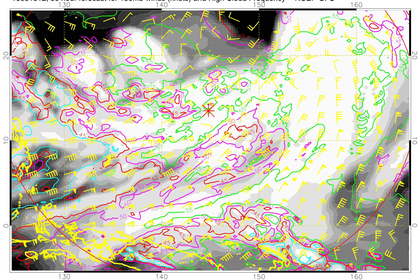
16081812, 36 hour forecast for 150mb winds (knots) and High Cloud Frequency -- NCEP GFS
