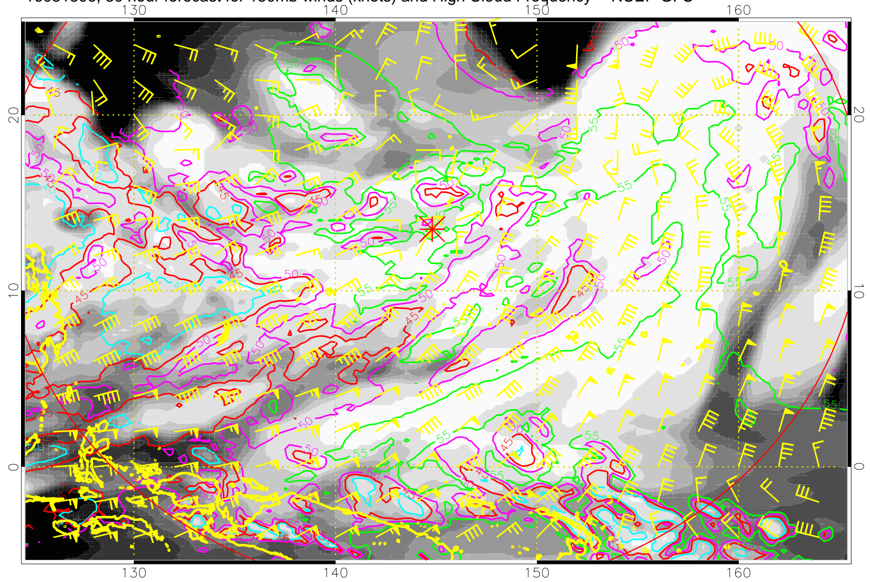
16081806, 30 hour forecast for 150mb winds (knots) and High Cloud Frequency -- NCEP GFS
