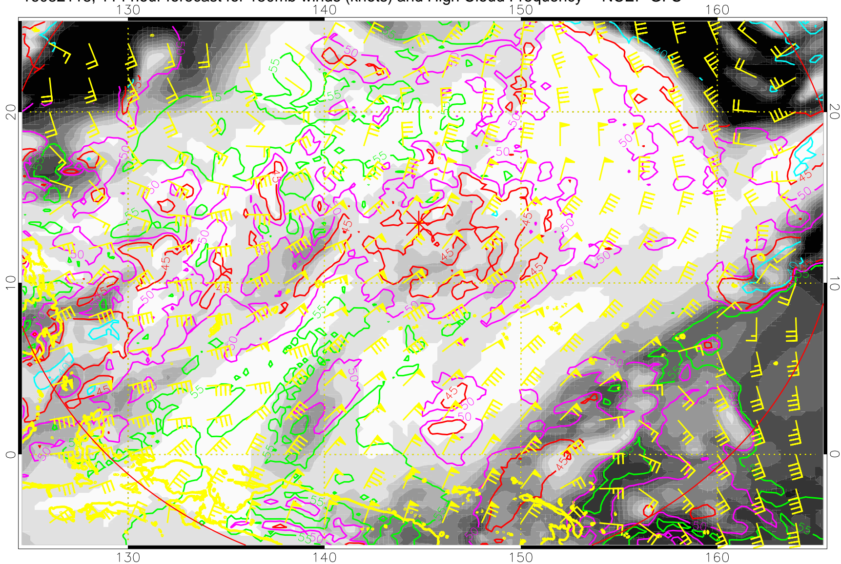
16082118, 114 hour forecast for 150mb winds (knots) and High Cloud Frequency -- NCEP GFS
