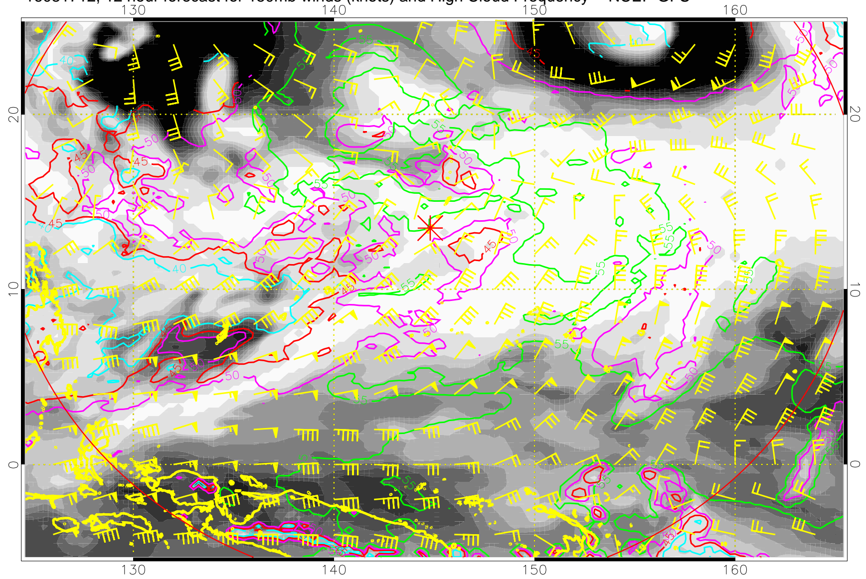
16081712, 12 hour forecast for 150mb winds (knots) and High Cloud Frequency -- NCEP GFS
