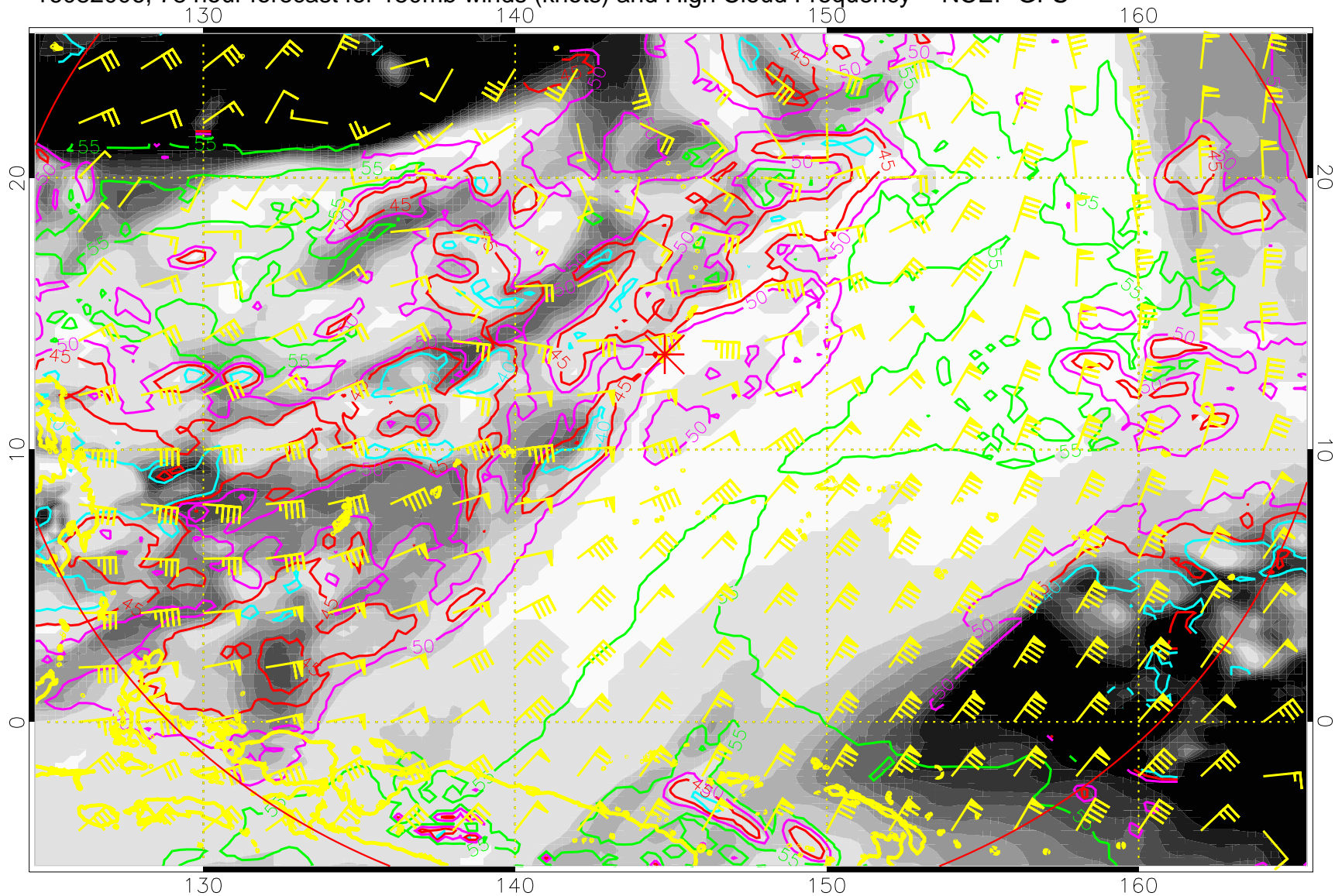
16082006, 78 hour forecast for 150mb winds (knots) and High Cloud Frequency -- NCEP GFS
