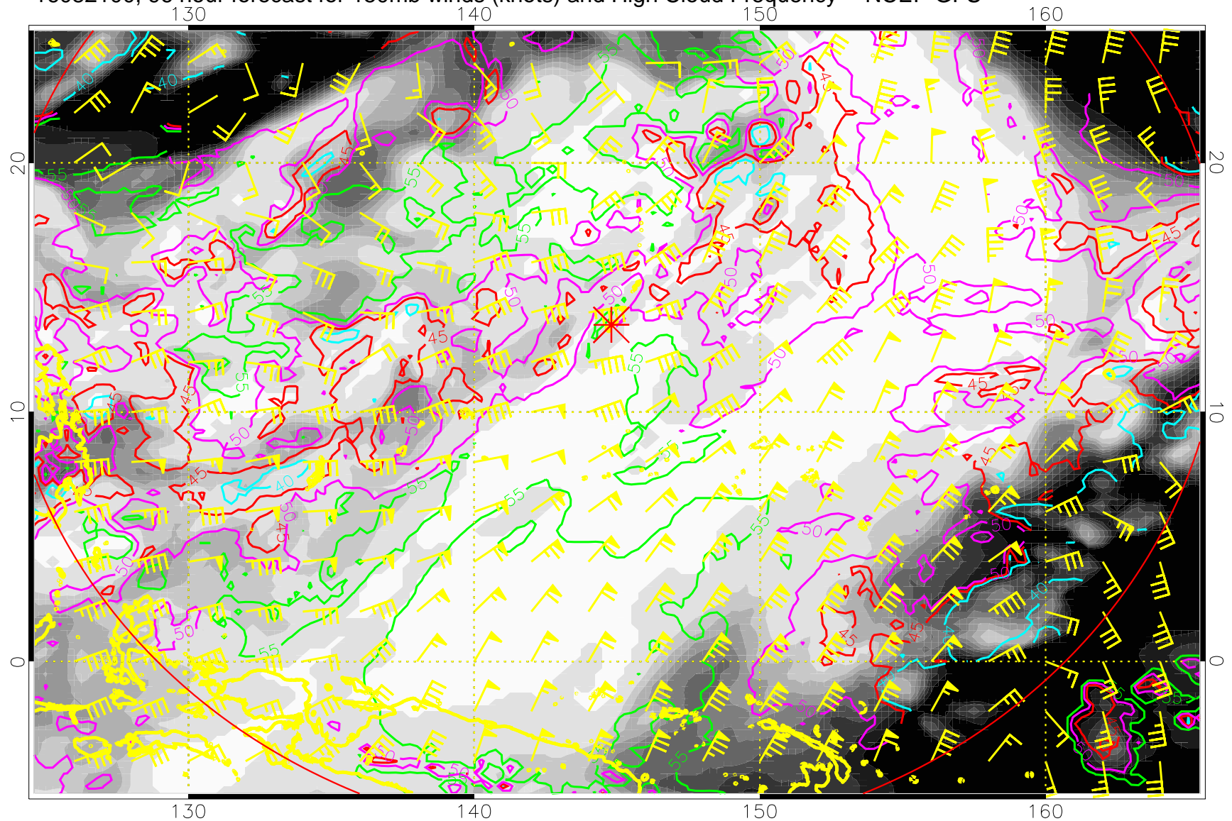
16082100, 96 hour forecast for 150mb winds (knots) and High Cloud Frequency -- NCEP GFS
