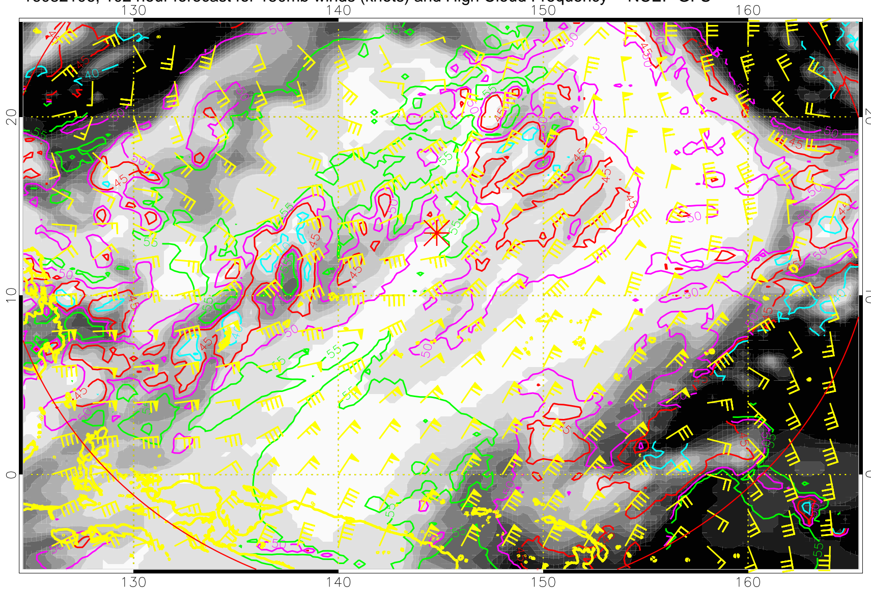
16082106, 102 hour forecast for 150mb winds (knots) and High Cloud Frequency -- NCEP GFS
