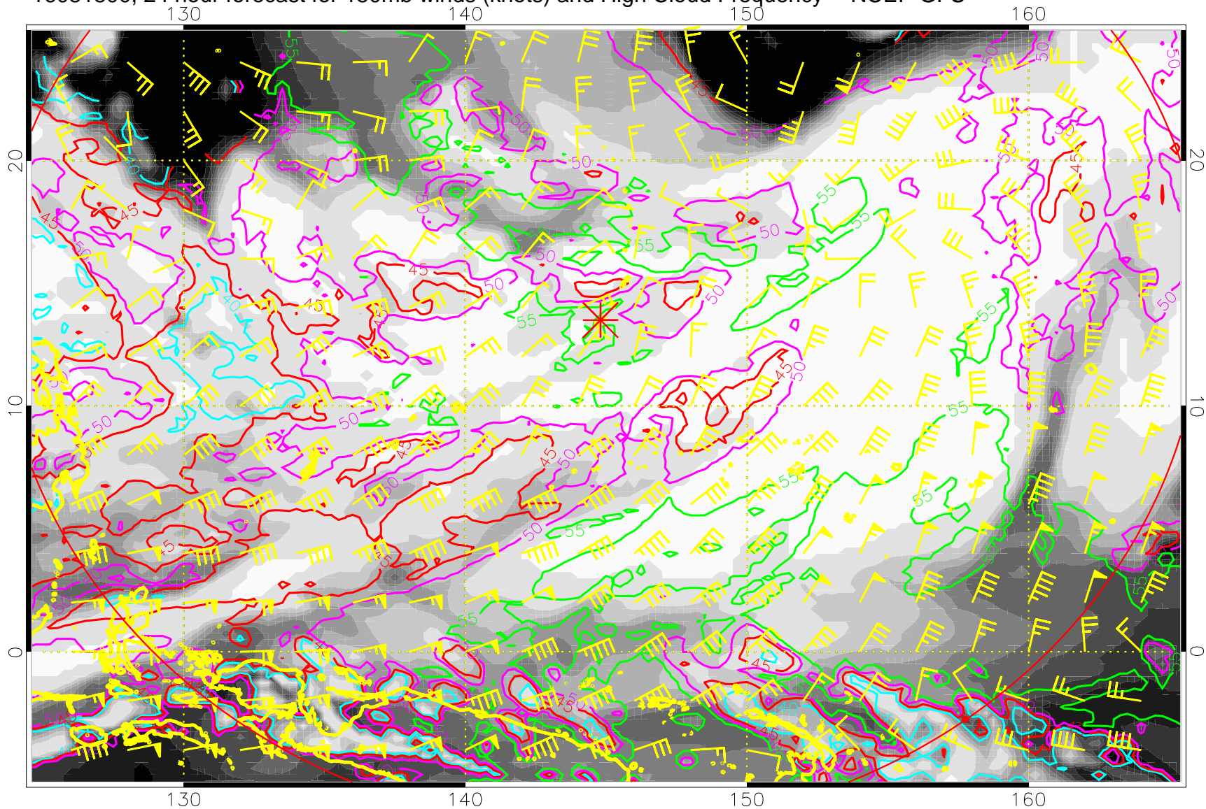
16081800, 24 hour forecast for 150mb winds (knots) and High Cloud Frequency -- NCEP GFS
