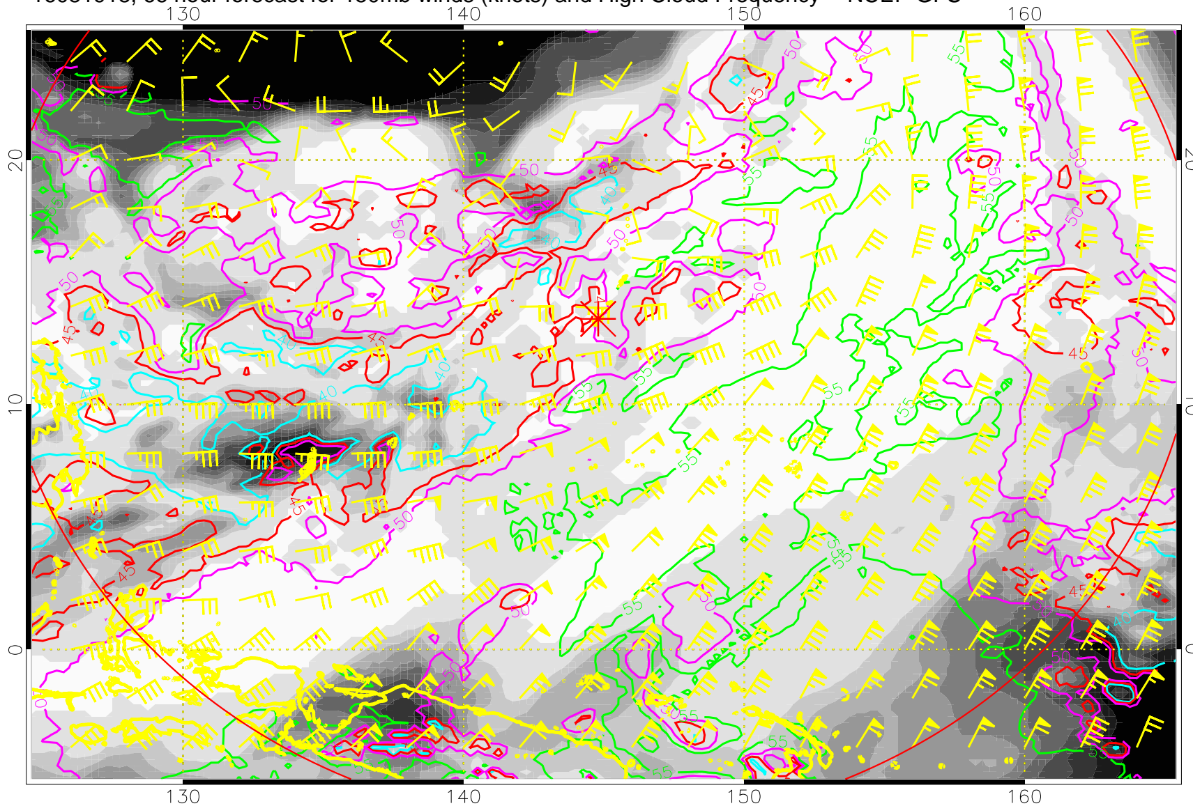
16081918, 66 hour forecast for 150mb winds (knots) and High Cloud Frequency -- NCEP GFS
