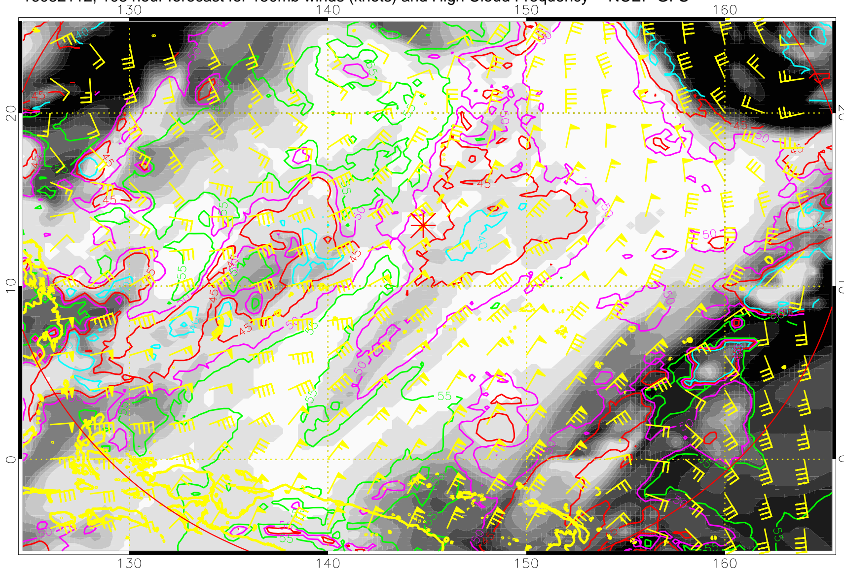
16082112, 108 hour forecast for 150mb winds (knots) and High Cloud Frequency -- NCEP GFS
