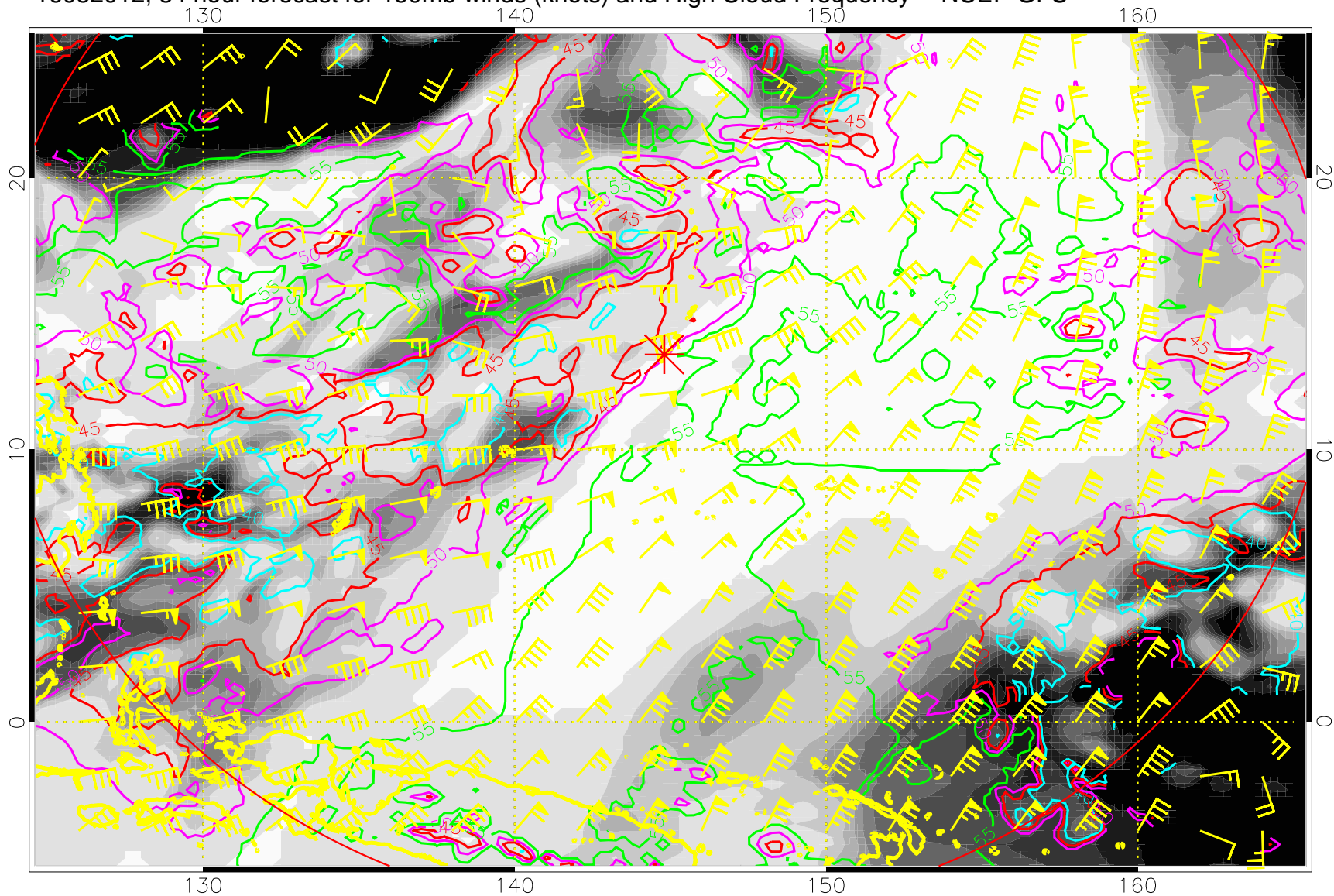
16082012, 84 hour forecast for 150mb winds (knots) and High Cloud Frequency -- NCEP GFS
