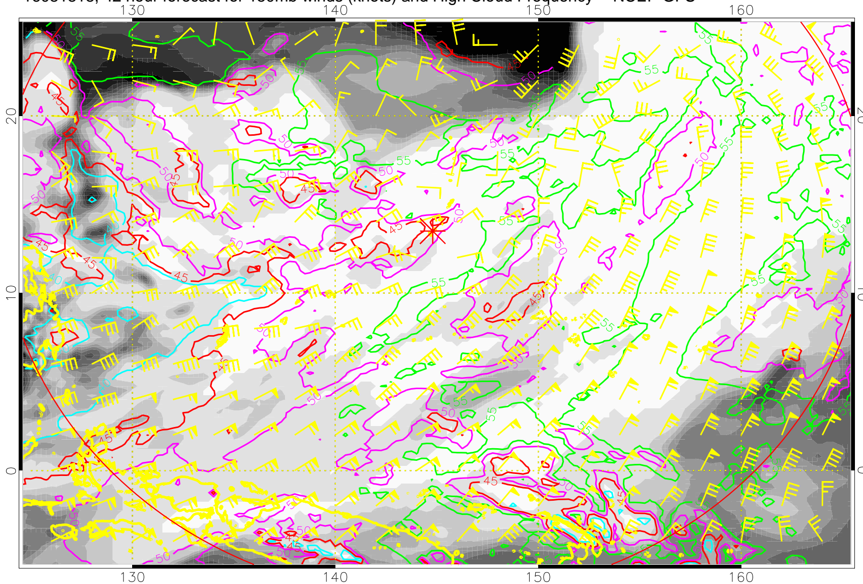
16081818, 42 hour forecast for 150mb winds (knots) and High Cloud Frequency -- NCEP GFS
