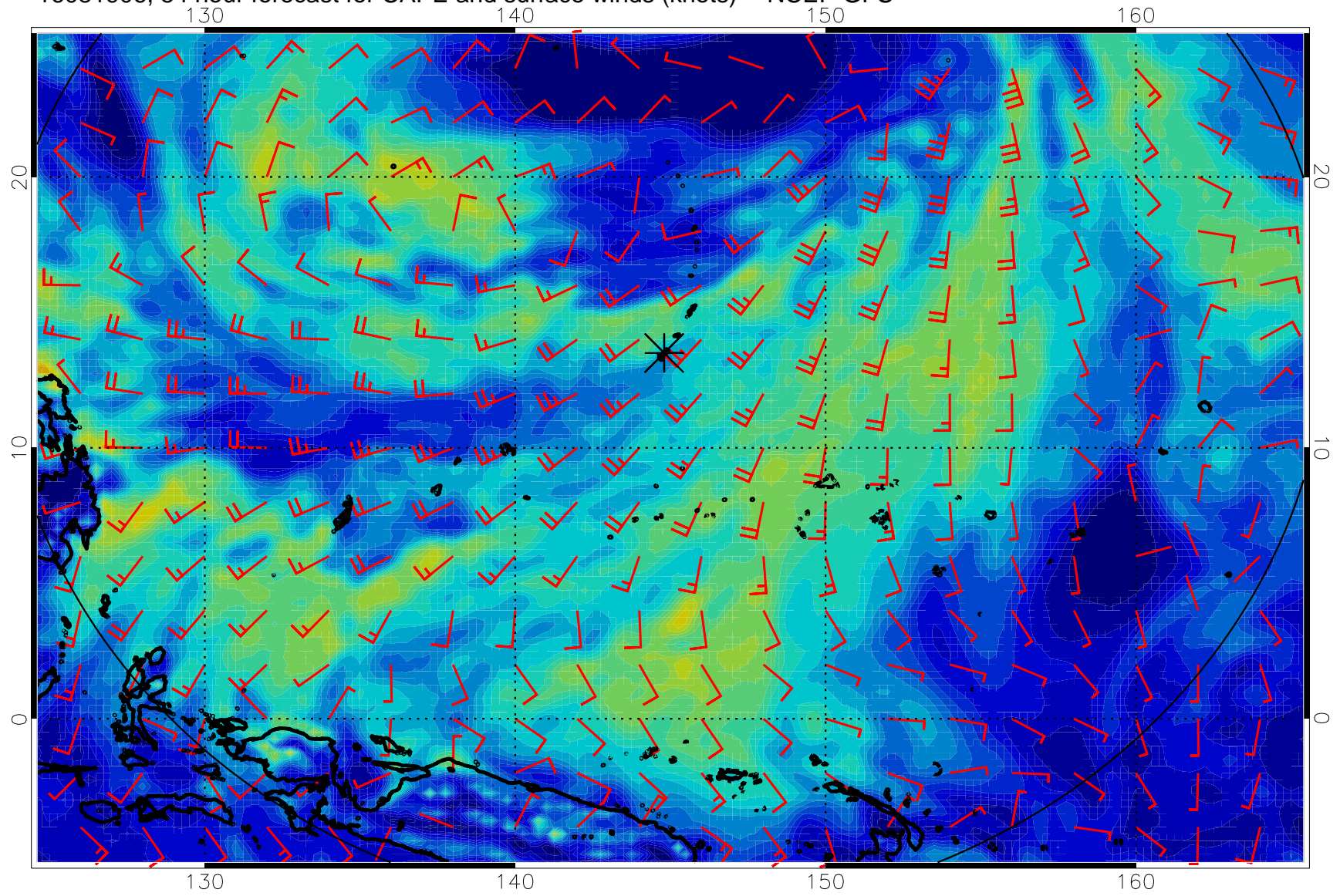
16081906, 54 hour forecast for CAPE and surface winds (knots) -- NCEP GFS
