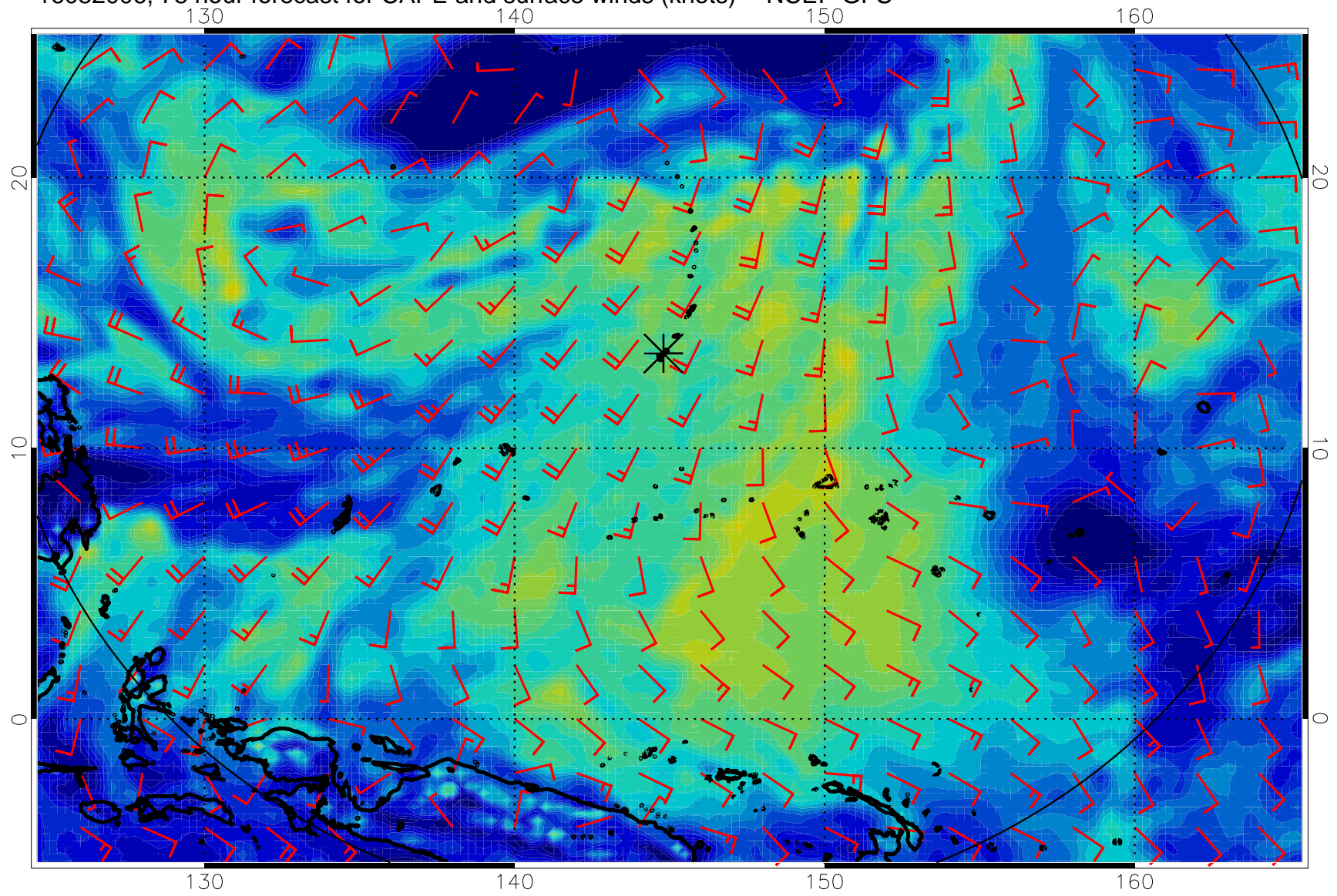
16082006, 78 hour forecast for CAPE and surface winds (knots) -- NCEP GFS
