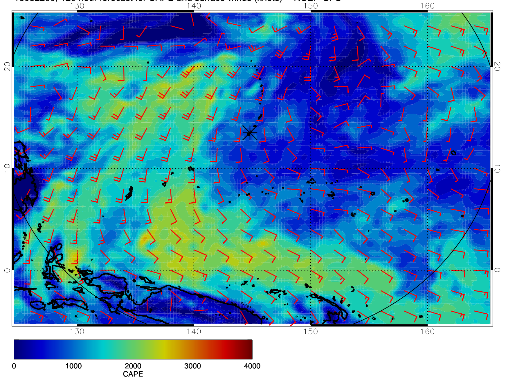
16082200, 120 hour forecast for CAPE and surface winds (knots) -- NCEP GFS
