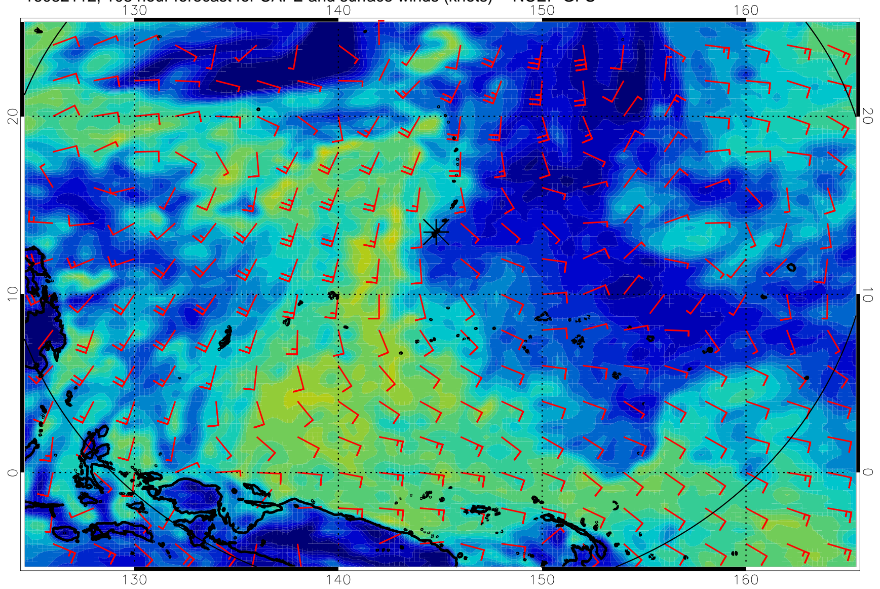
16082112, 108 hour forecast for CAPE and surface winds (knots) -- NCEP GFS
