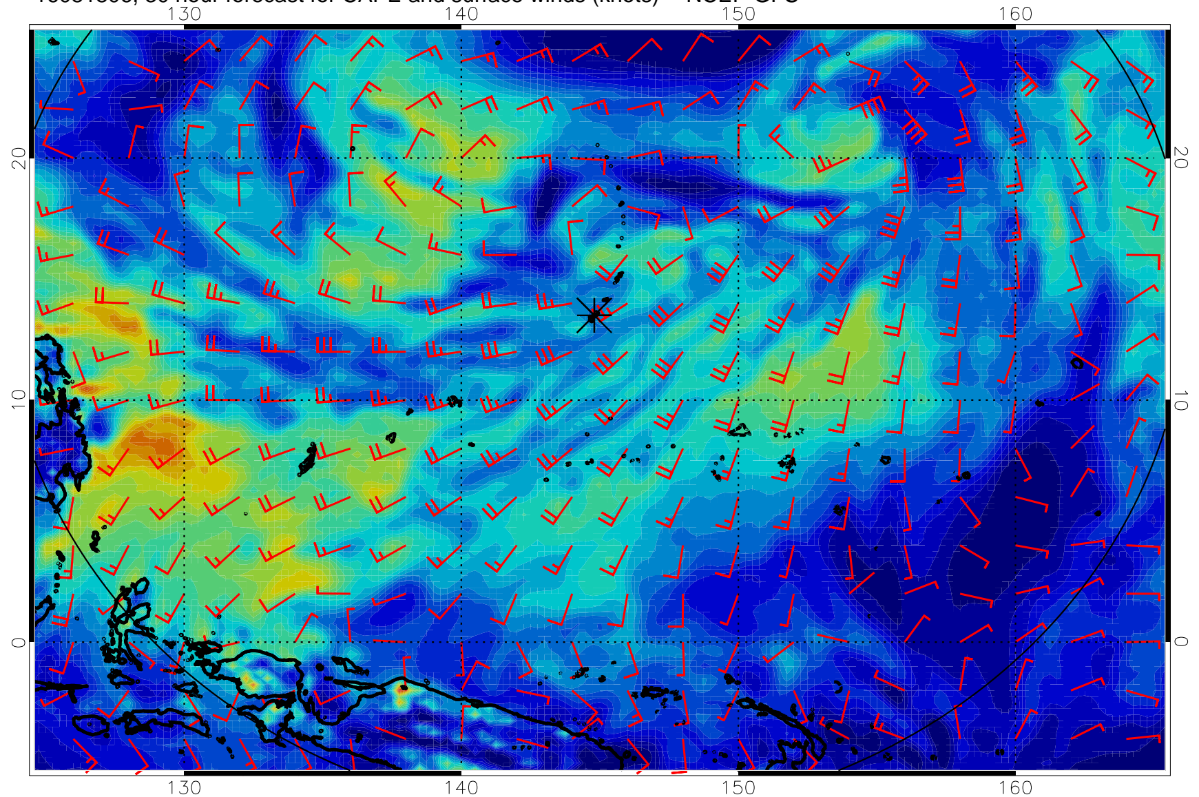
16081806, 30 hour forecast for CAPE and surface winds (knots) -- NCEP GFS
