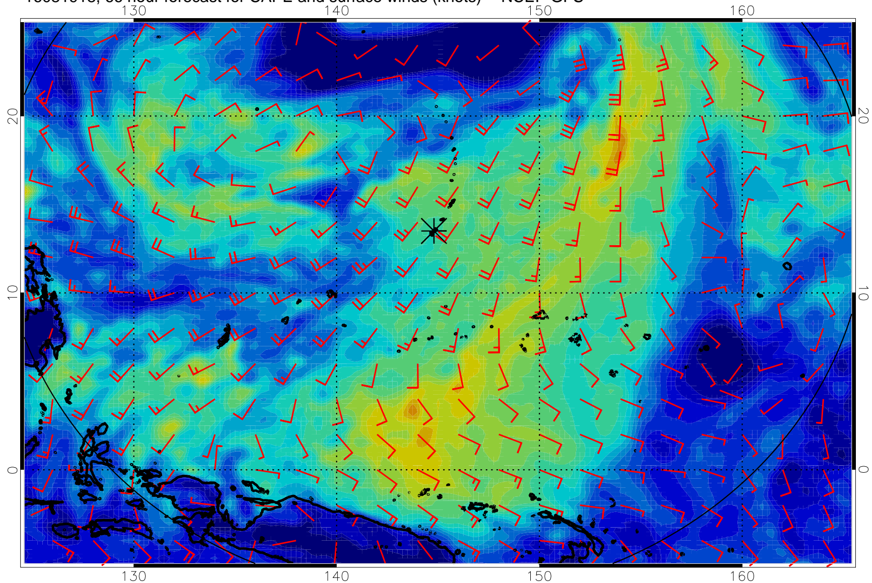
16081918, 66 hour forecast for CAPE and surface winds (knots) -- NCEP GFS
