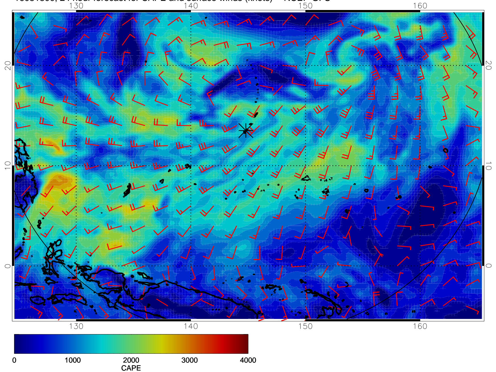
16081800, 24 hour forecast for CAPE and surface winds (knots) -- NCEP GFS
