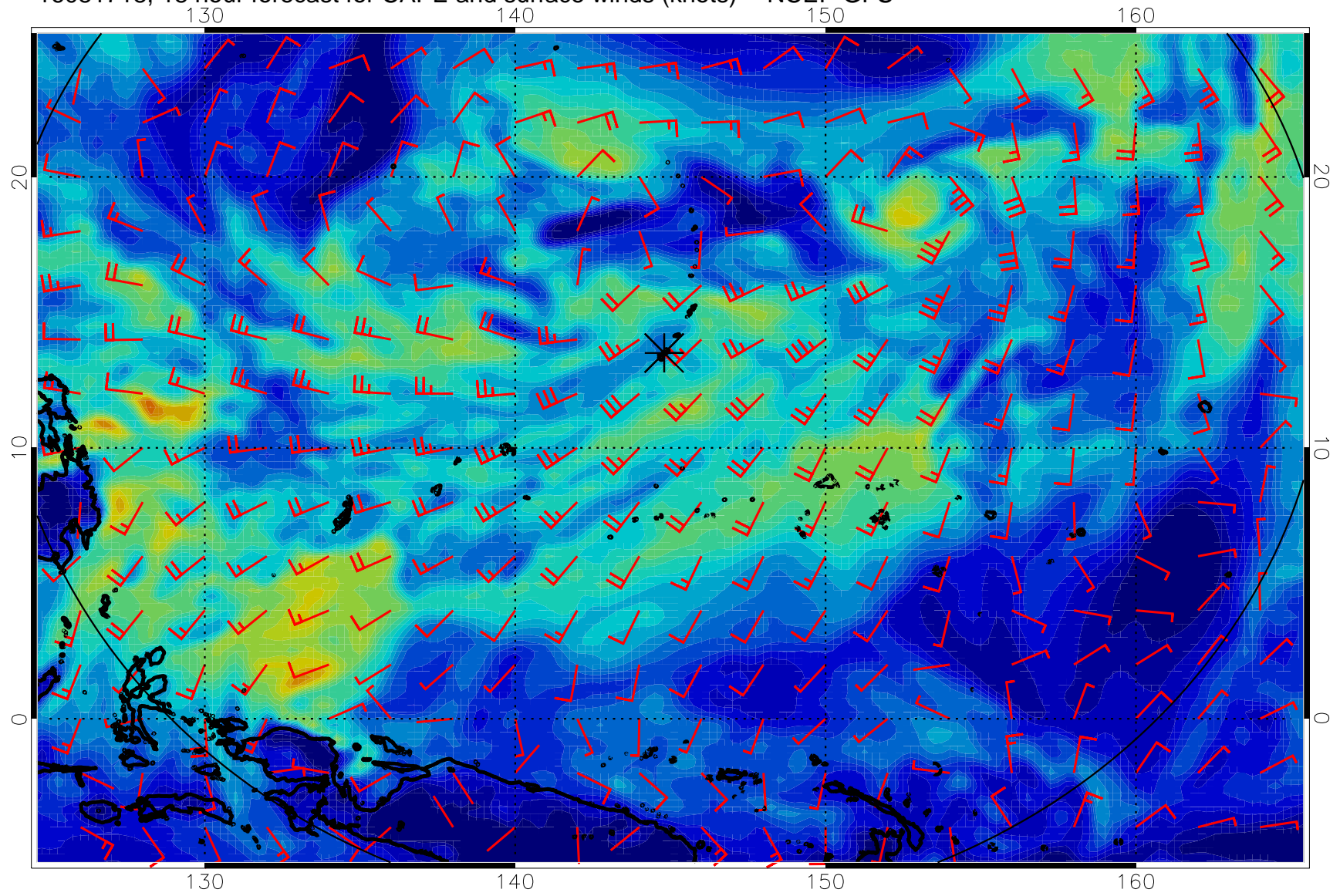
16081718, 18 hour forecast for CAPE and surface winds (knots) -- NCEP GFS
