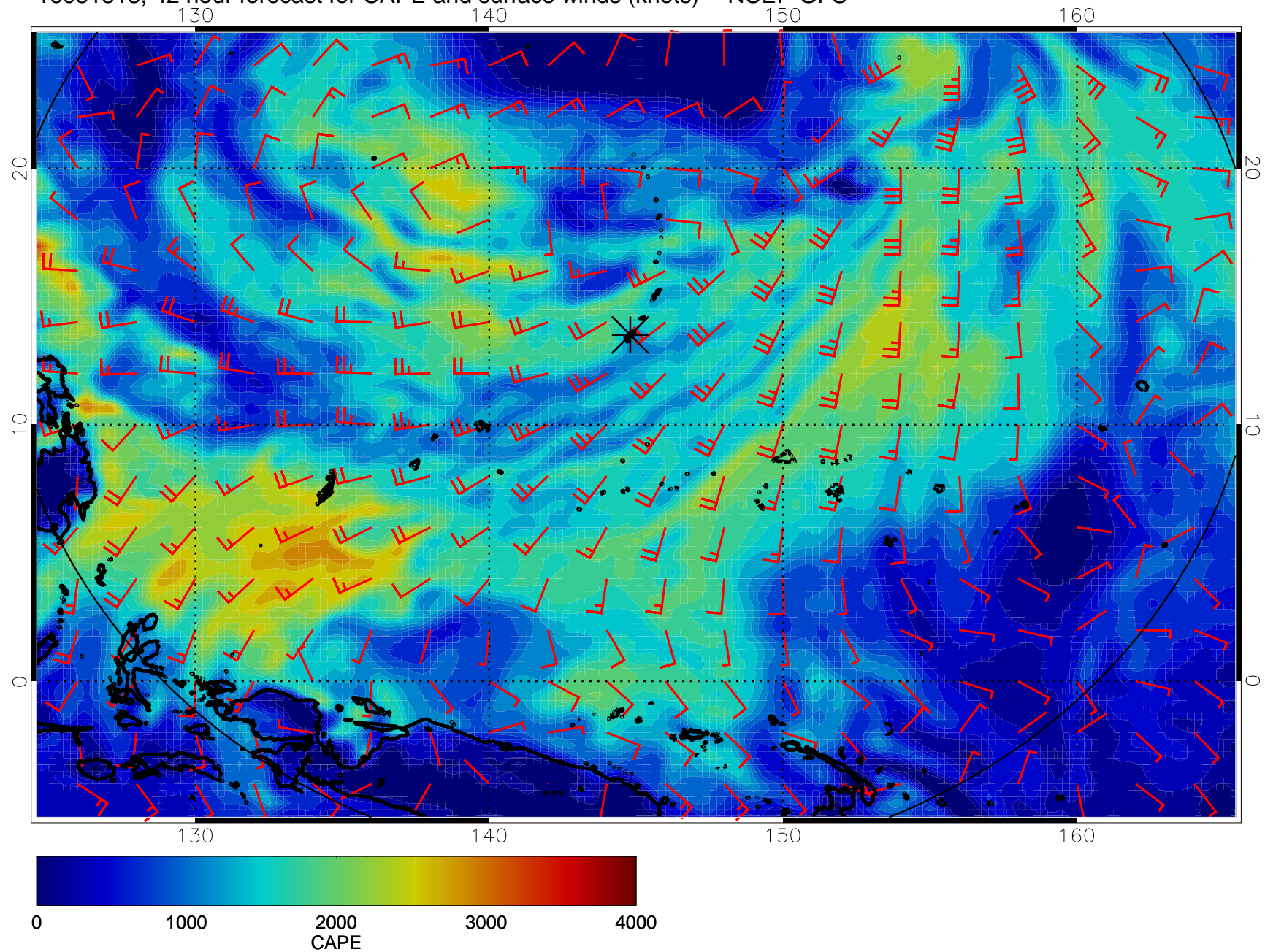
16081818, 42 hour forecast for CAPE and surface winds (knots) -- NCEP GFS
