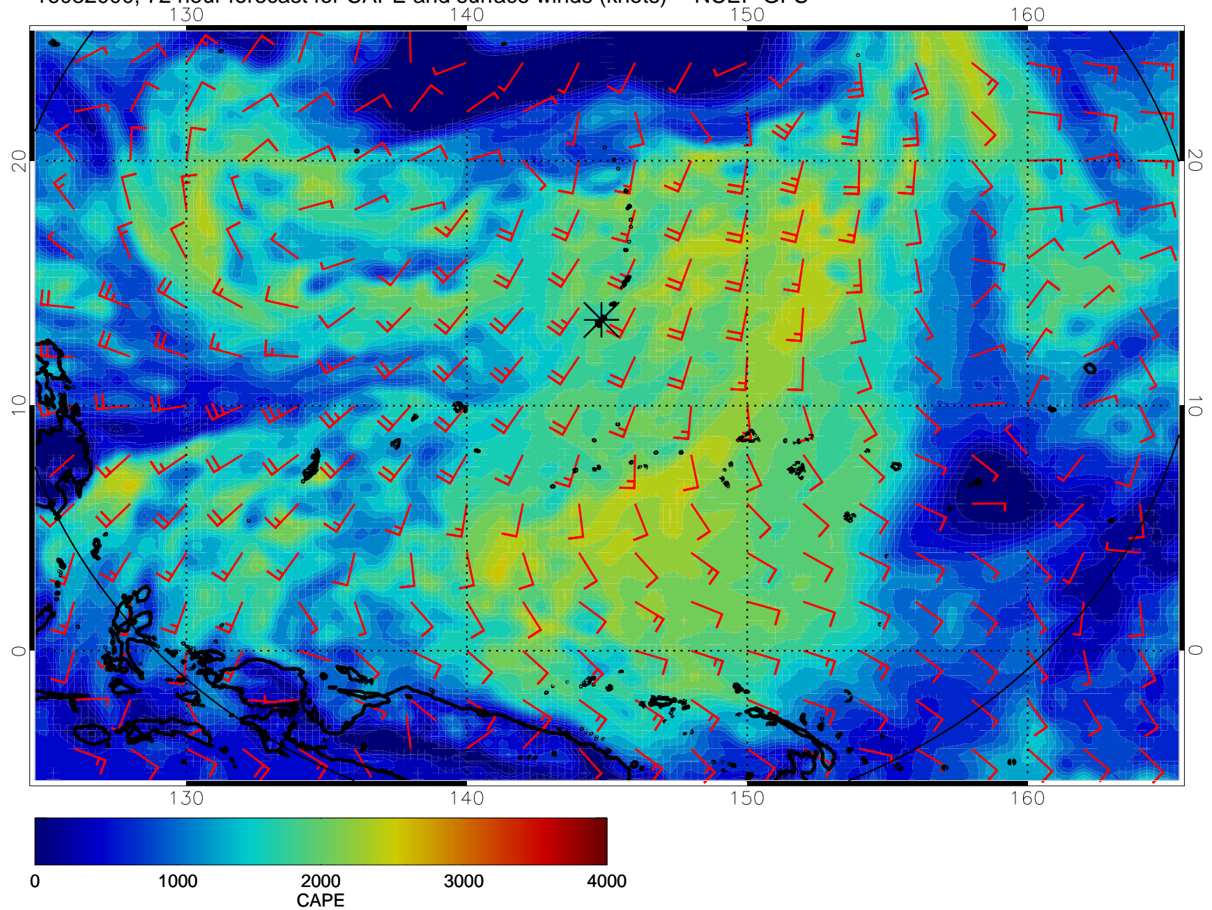
16082000, 72 hour forecast for CAPE and surface winds (knots) -- NCEP GFS
