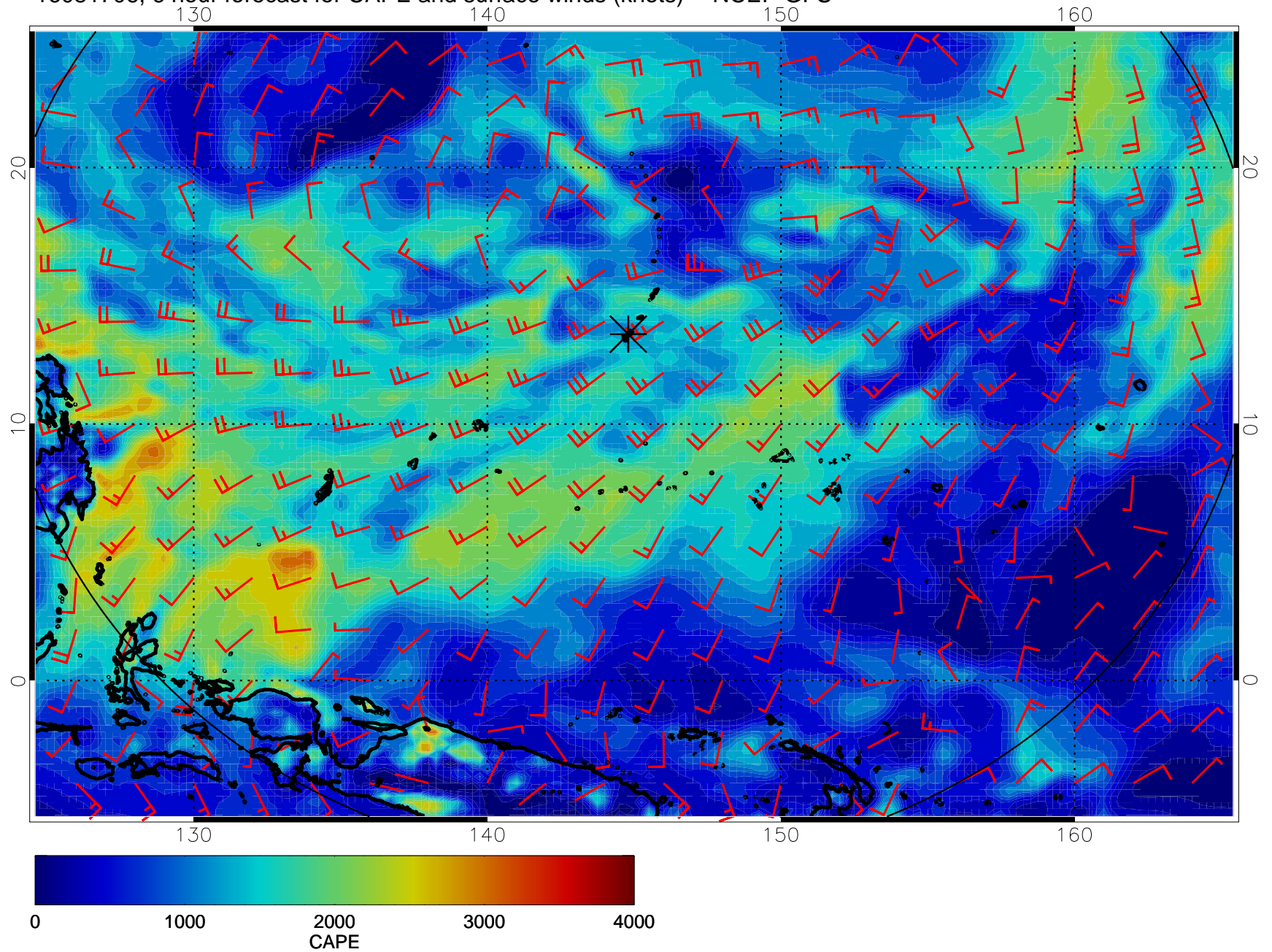
16081706, 6 hour forecast for CAPE and surface winds (knots) -- NCEP GFS
