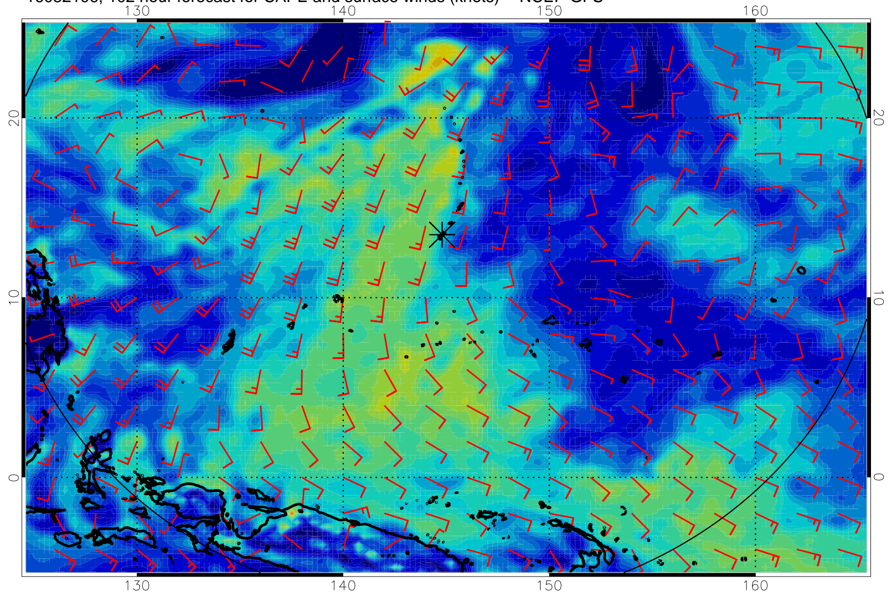
16082106, 102 hour forecast for CAPE and surface winds (knots) -- NCEP GFS
