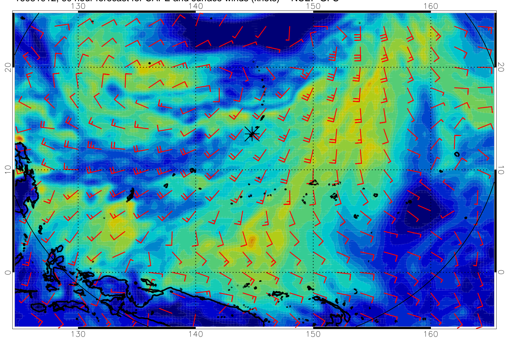
16081912, 60 hour forecast for CAPE and surface winds (knots) -- NCEP GFS
