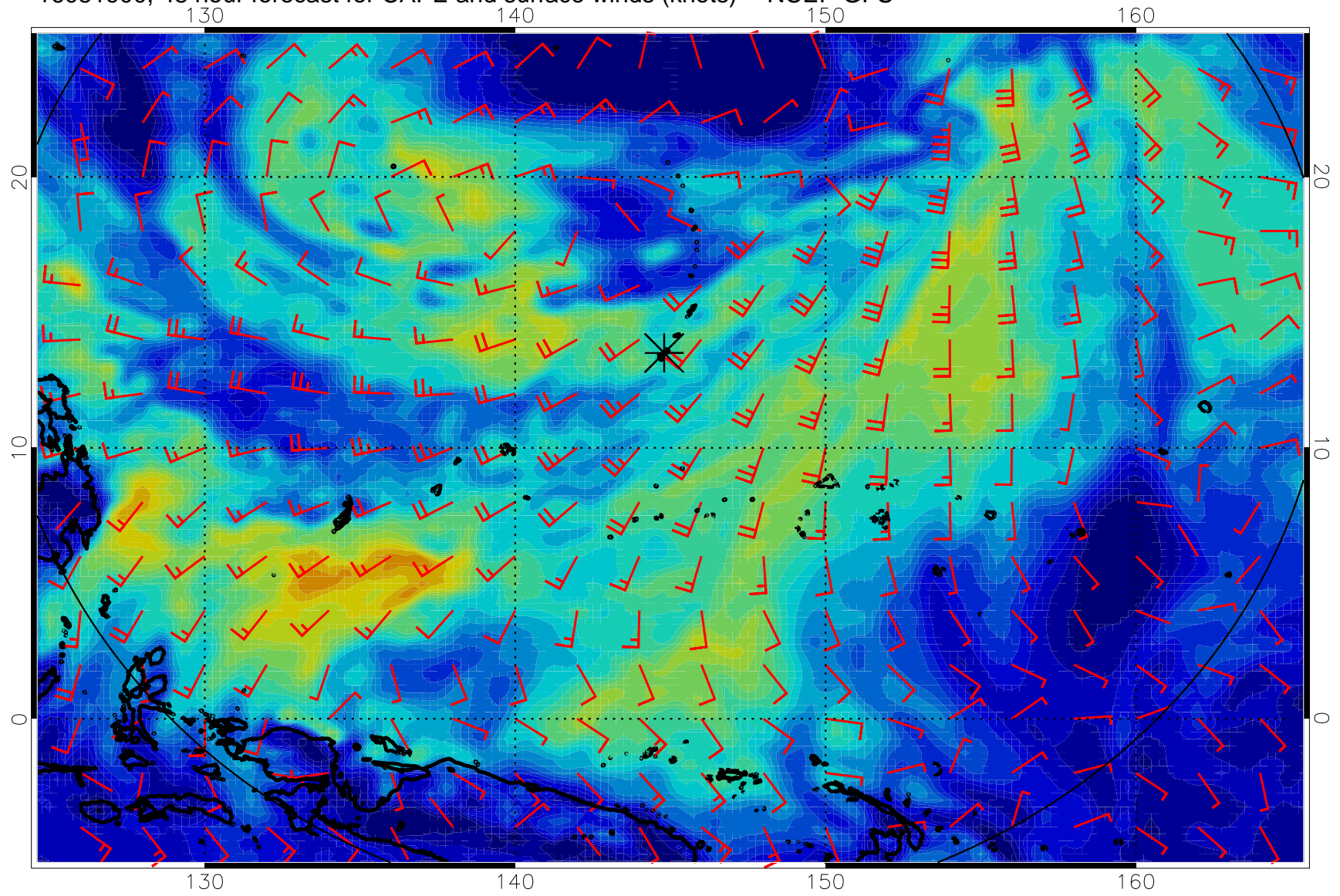
16081900, 48 hour forecast for CAPE and surface winds (knots) -- NCEP GFS
