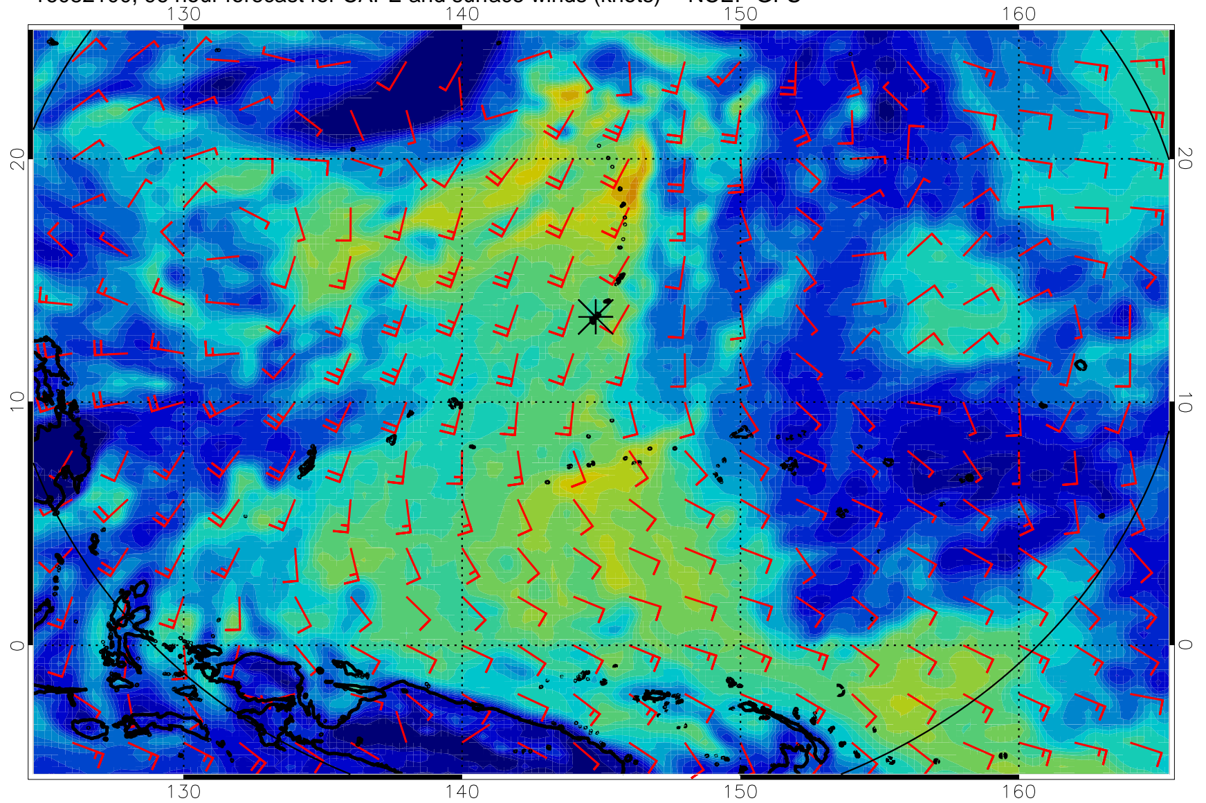
16082100, 96 hour forecast for CAPE and surface winds (knots) -- NCEP GFS
