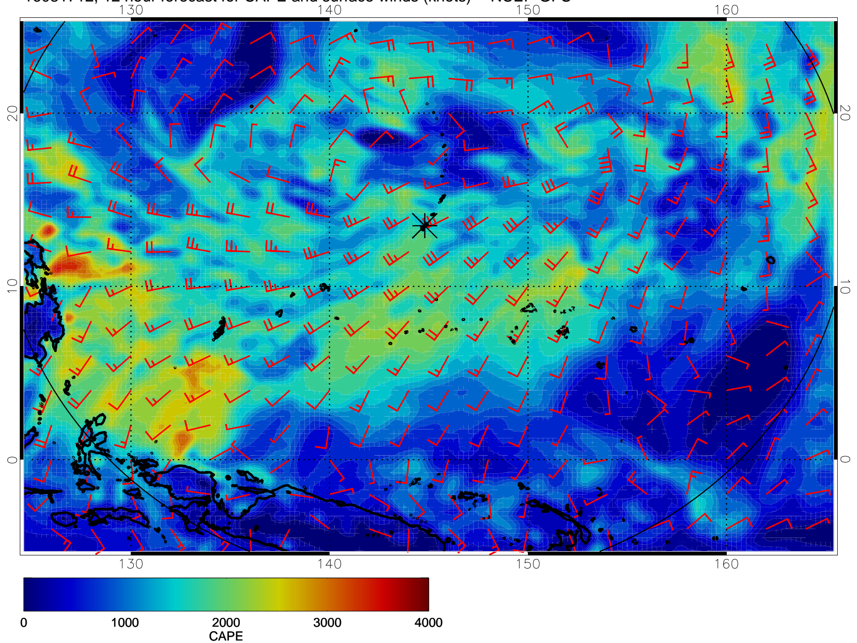
16081712, 12 hour forecast for CAPE and surface winds (knots) -- NCEP GFS
