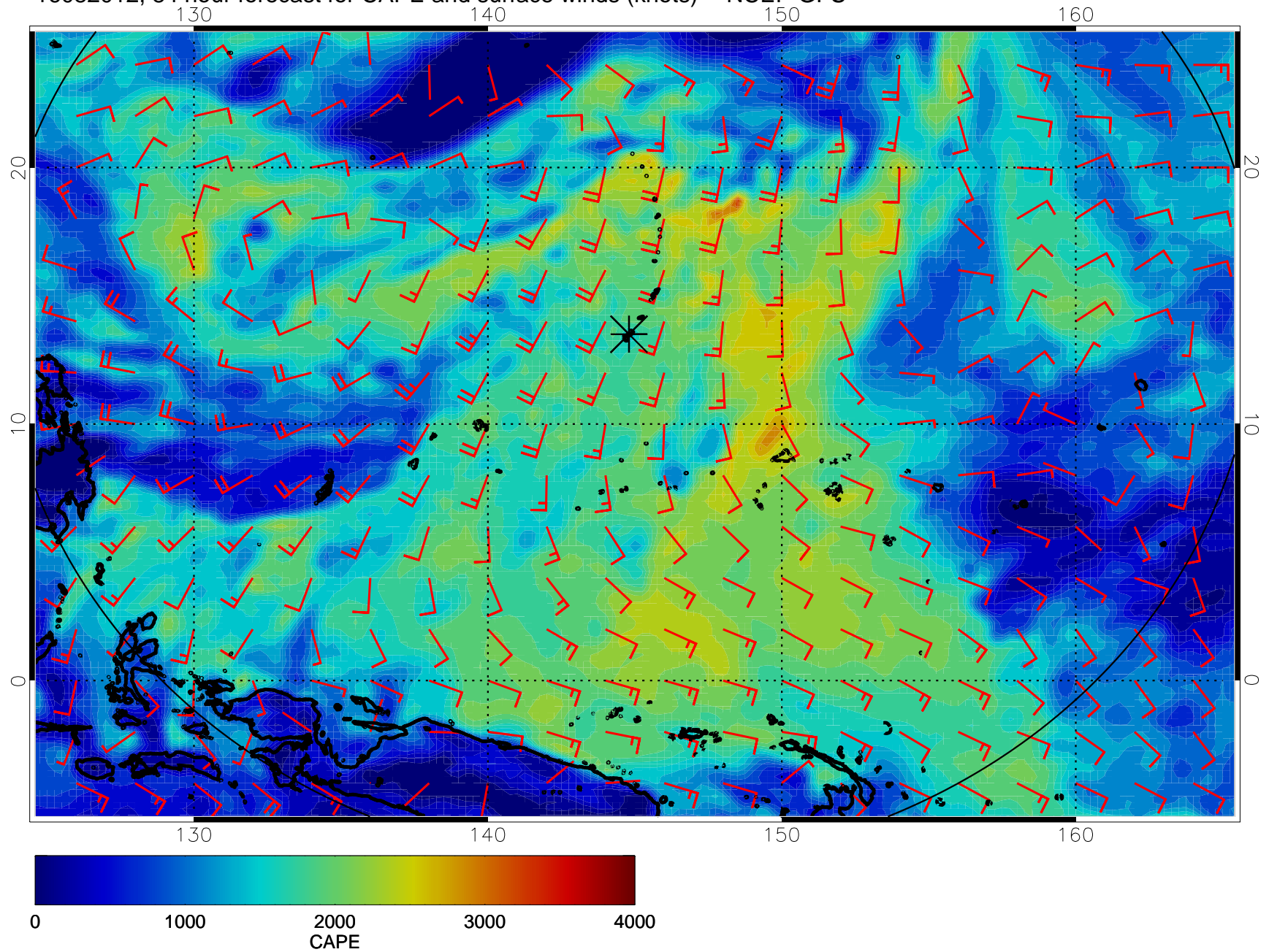
16082012, 84 hour forecast for CAPE and surface winds (knots) -- NCEP GFS
