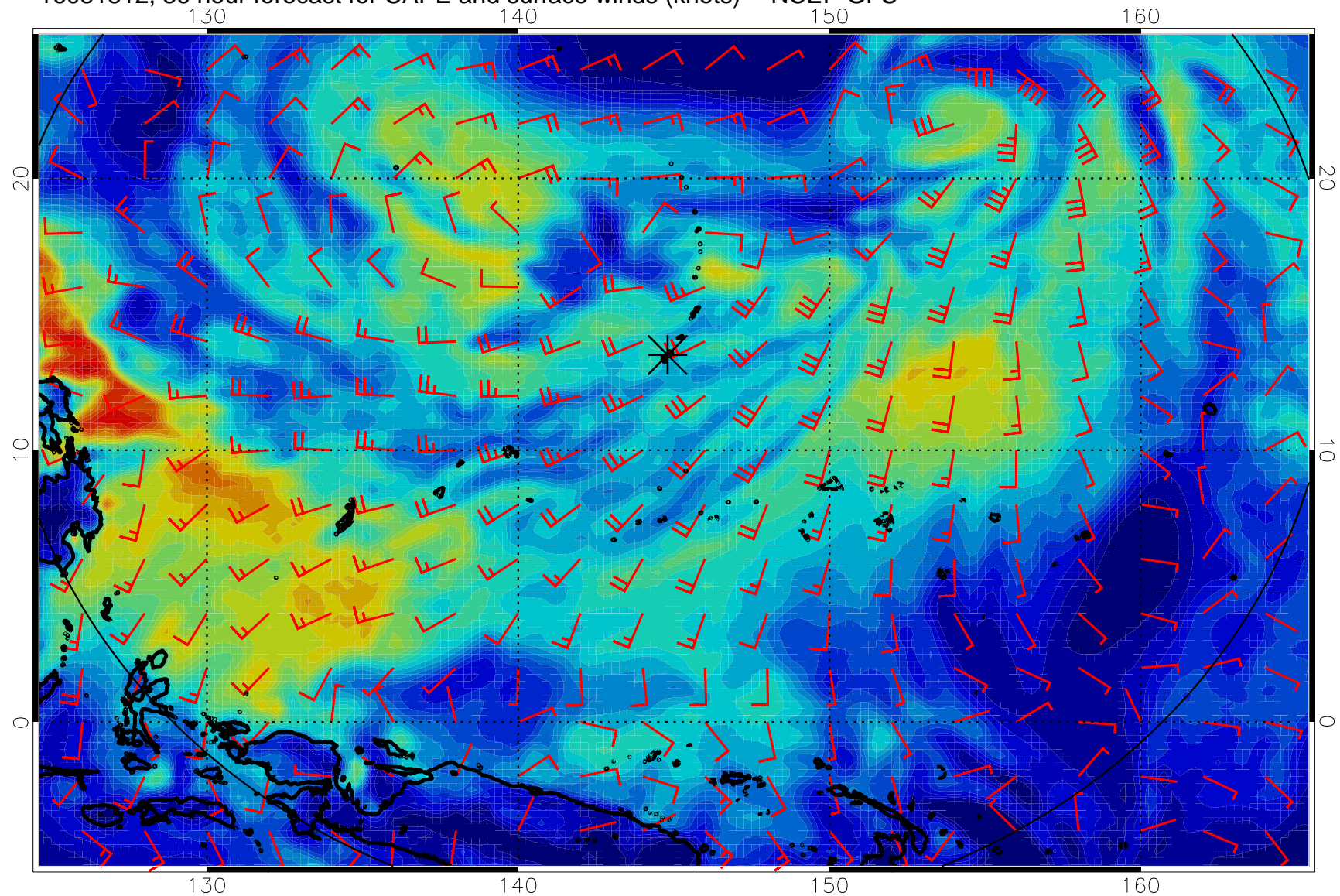
16081812, 36 hour forecast for CAPE and surface winds (knots) -- NCEP GFS
