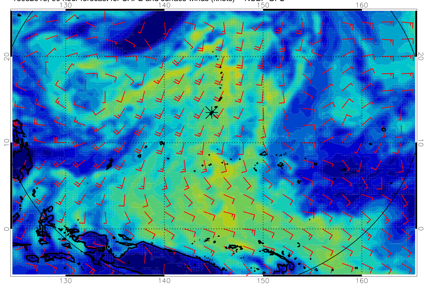
16082018, 90 hour forecast for CAPE and surface winds (knots) -- NCEP GFS
