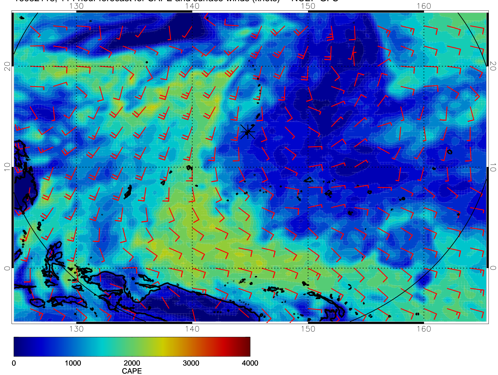
16082118, 114 hour forecast for CAPE and surface winds (knots) -- NCEP GFS
