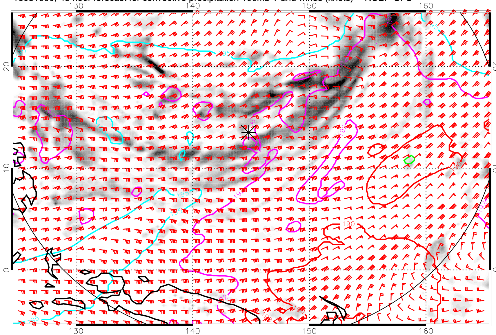
16081900, 48 hour forecast for convective precipitation 100mb T and winds (knots) -- NCEP GFS
