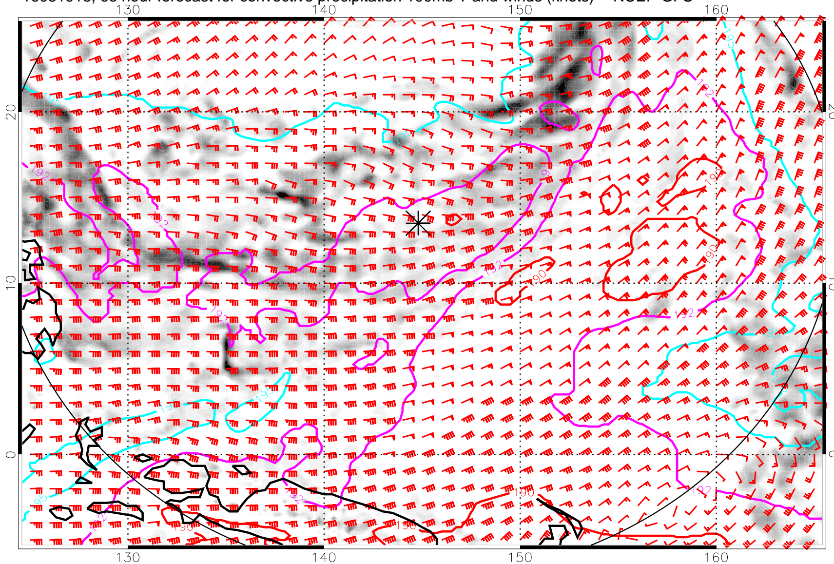
16081918, 66 hour forecast for convective precipitation 100mb T and winds (knots) -- NCEP GFS
