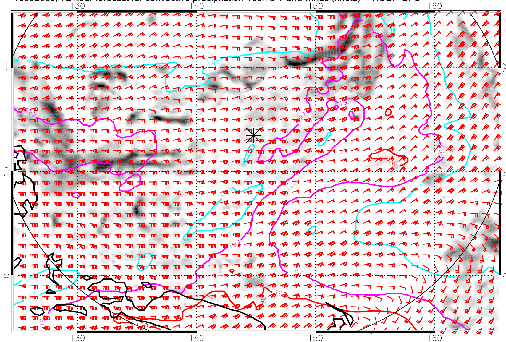
16082000, 72 hour forecast for convective precipitation 100mb T and winds (knots) -- NCEP GFS
