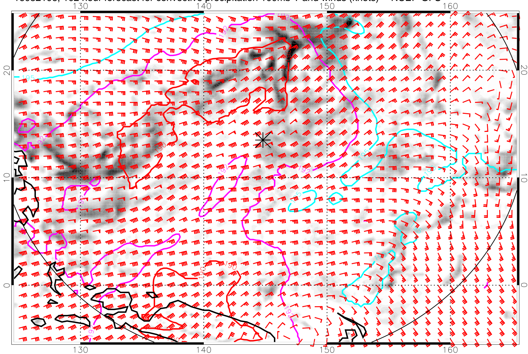
16082106, 102 hour forecast for convective precipitation 100mb T and winds (knots) -- NCEP GFS
