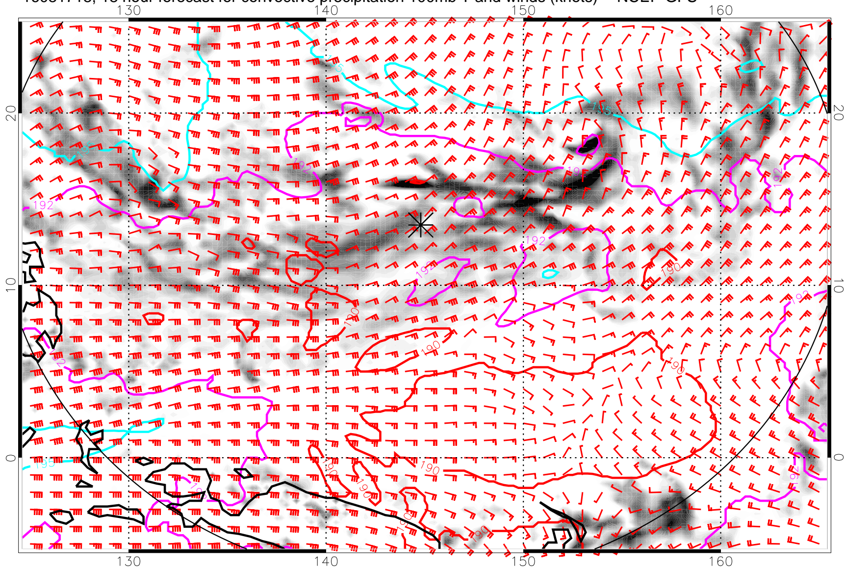
16081718, 18 hour forecast for convective precipitation 100mb T and winds (knots) -- NCEP GFS
