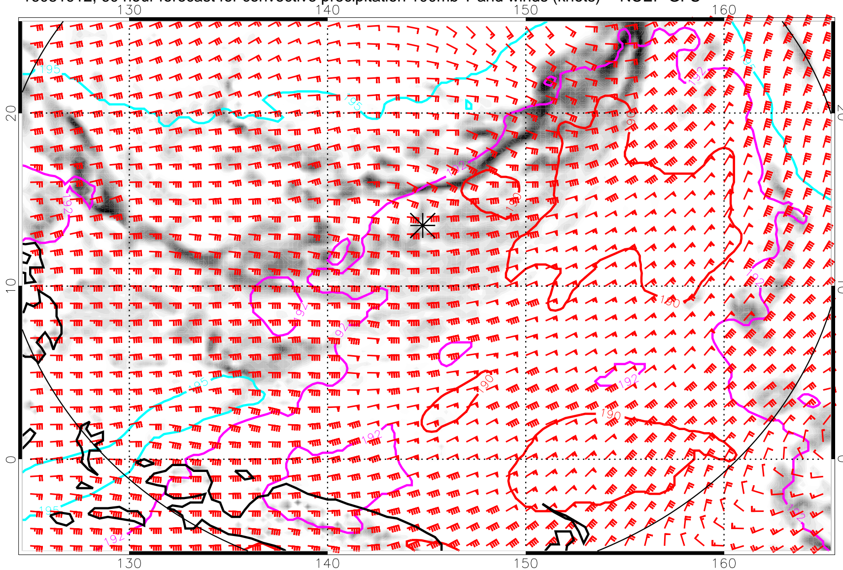
16081912, 60 hour forecast for convective precipitation 100mb T and winds (knots) -- NCEP GFS
