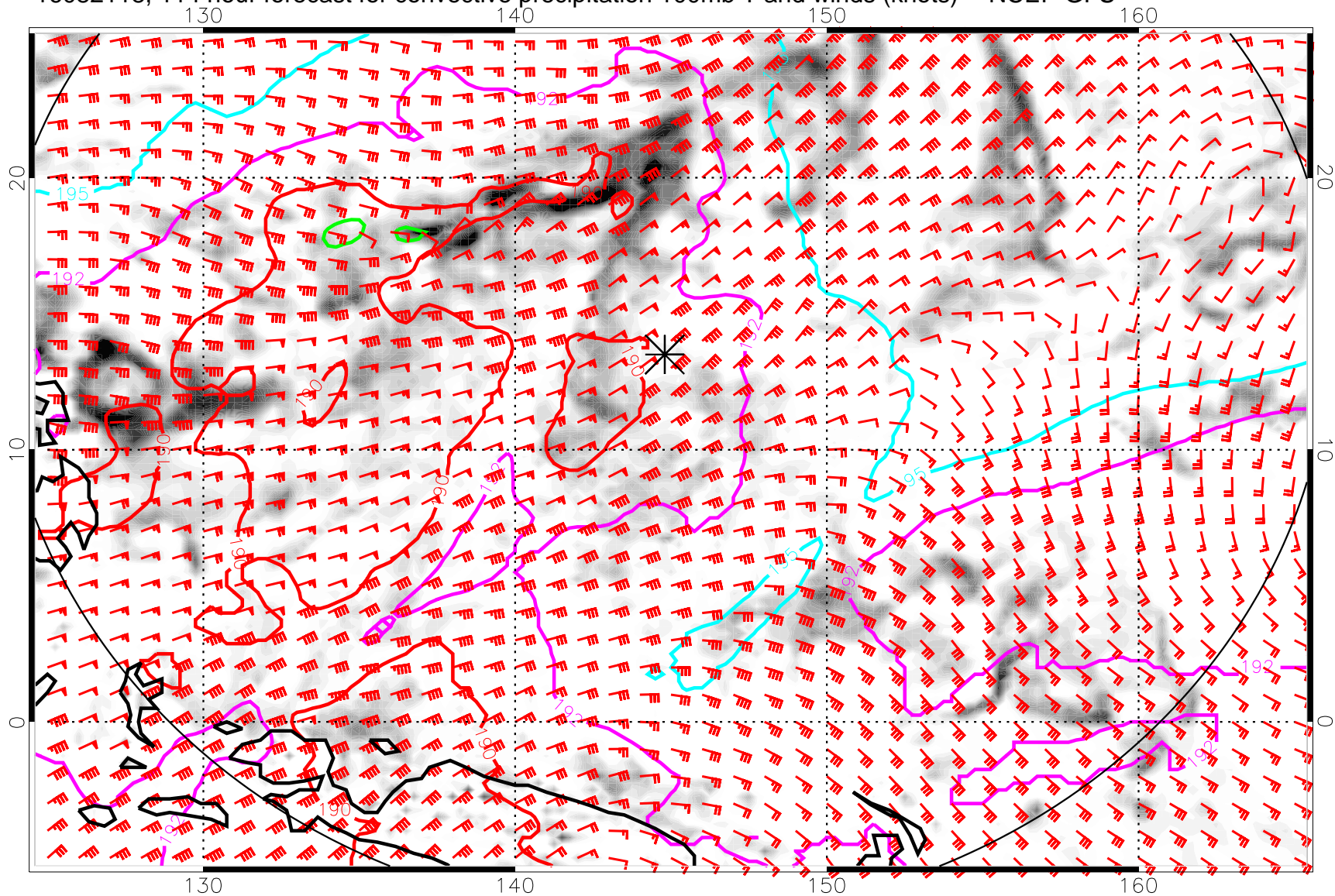
16082118, 114 hour forecast for convective precipitation 100mb T and winds (knots) -- NCEP GFS
