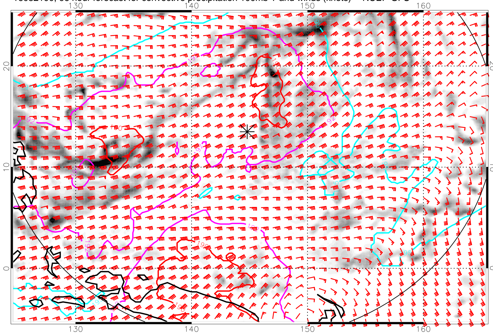
16082100, 96 hour forecast for convective precipitation 100mb T and winds (knots) -- NCEP GFS
