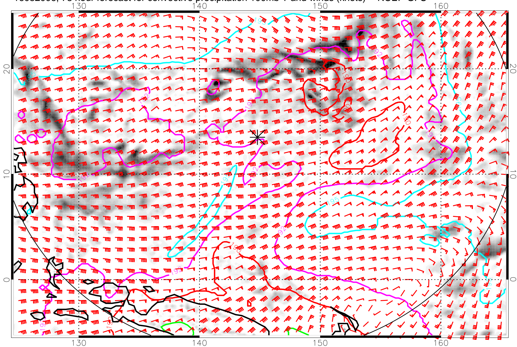
16082006, 78 hour forecast for convective precipitation 100mb T and winds (knots) -- NCEP GFS
