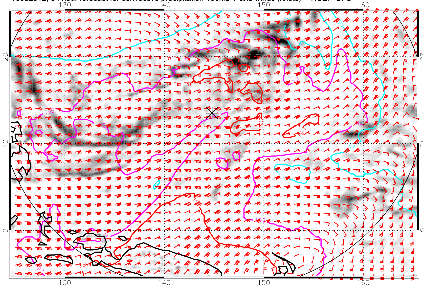
16082012, 84 hour forecast for convective precipitation 100mb T and winds (knots) -- NCEP GFS
