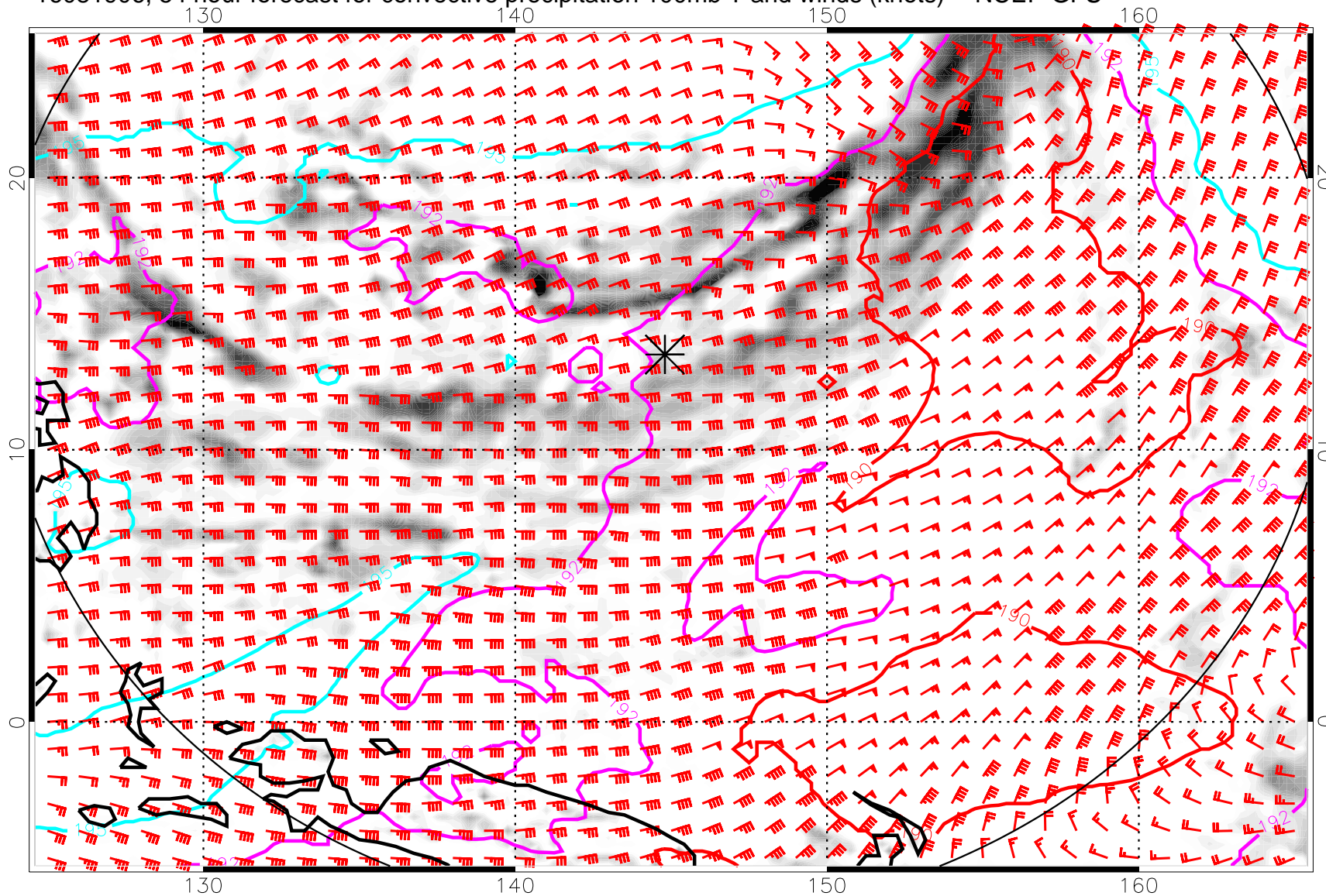
16081906, 54 hour forecast for convective precipitation 100mb T and winds (knots) -- NCEP GFS
