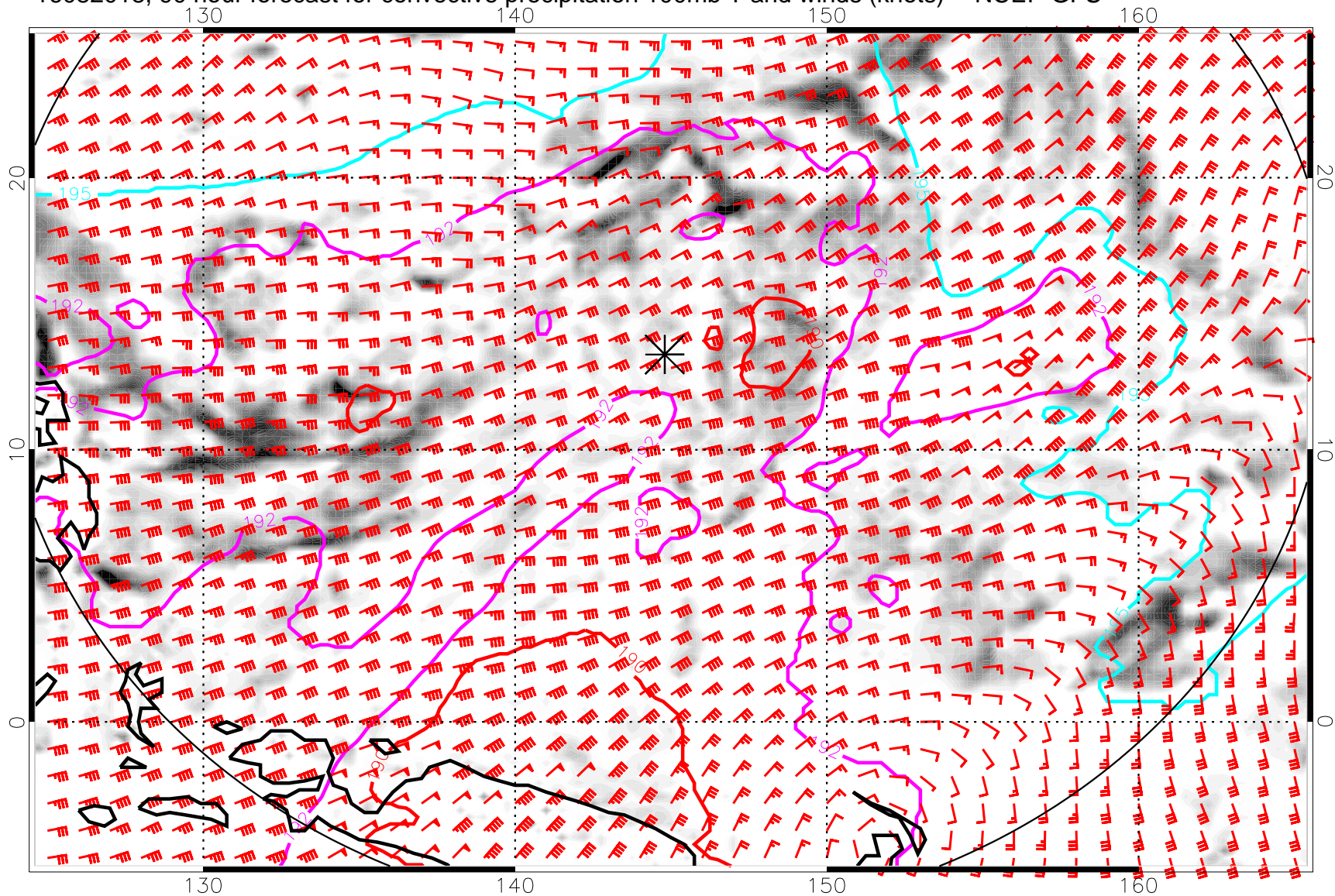
16082018, 90 hour forecast for convective precipitation 100mb T and winds (knots) -- NCEP GFS
