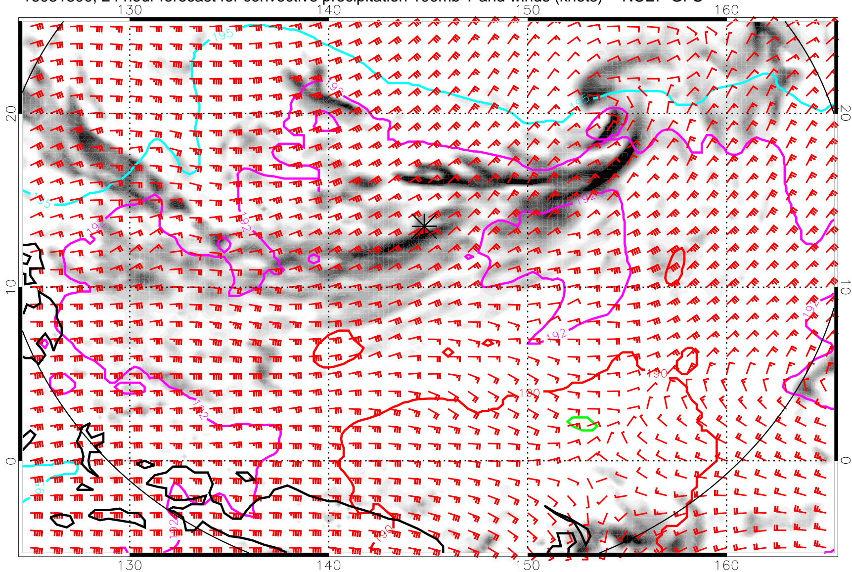
16081800, 24 hour forecast for convective precipitation 100mb T and winds (knots) -- NCEP GFS
