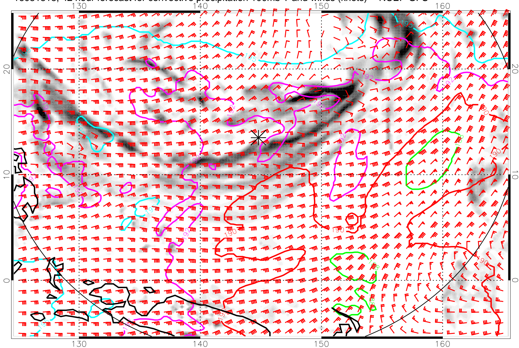
16081818, 42 hour forecast for convective precipitation 100mb T and winds (knots) -- NCEP GFS
