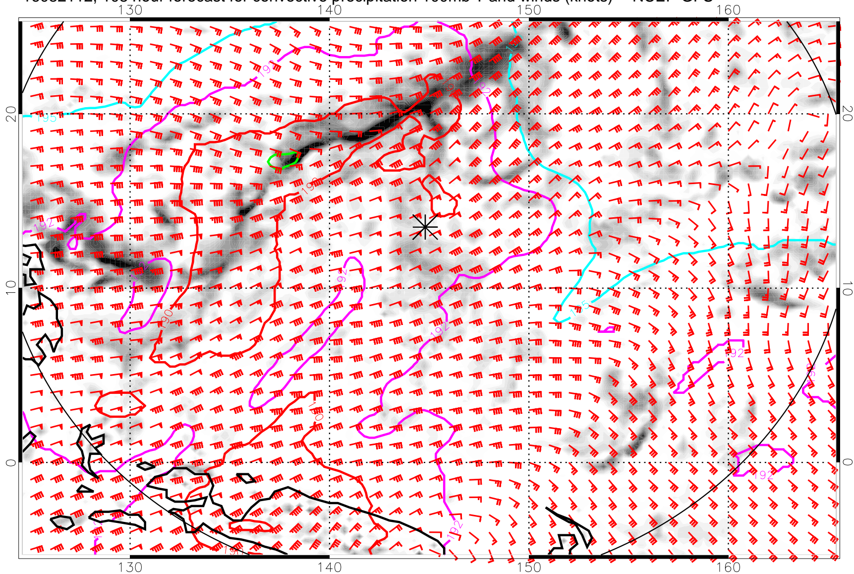
16082112, 108 hour forecast for convective precipitation 100mb T and winds (knots) -- NCEP GFS
