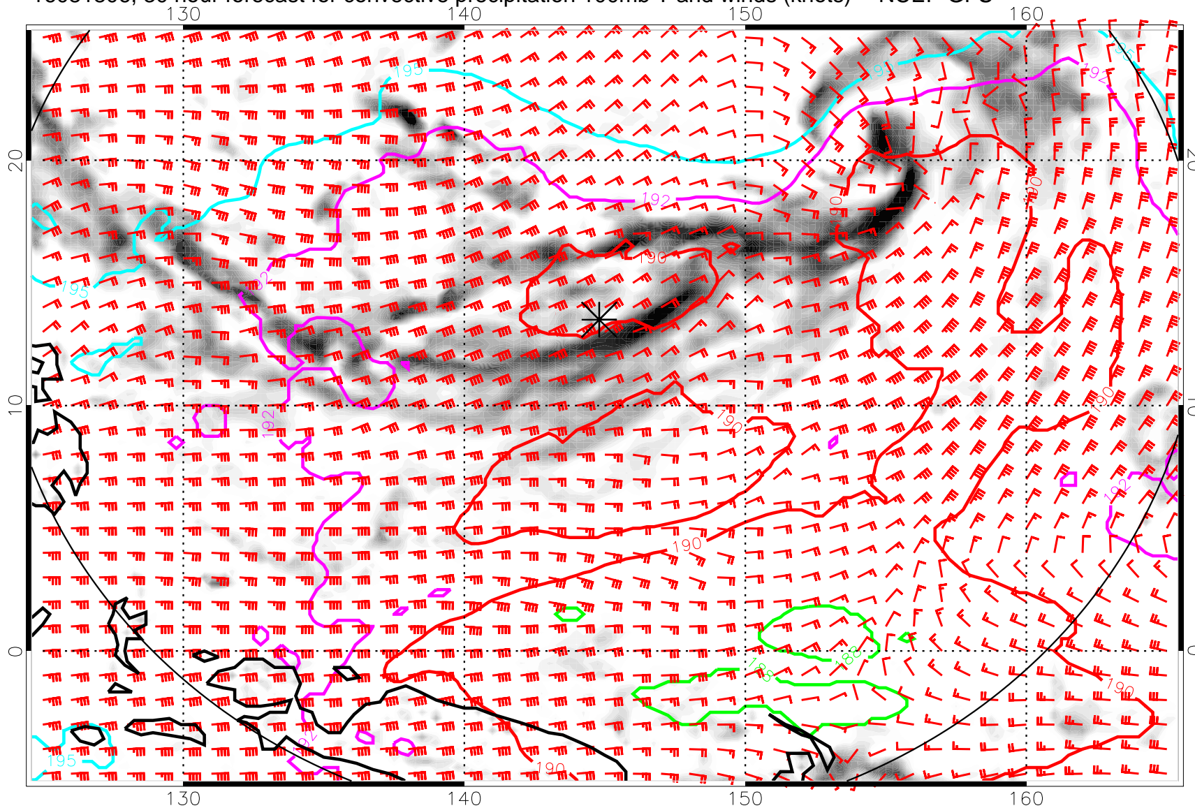
16081806, 30 hour forecast for convective precipitation 100mb T and winds (knots) -- NCEP GFS
