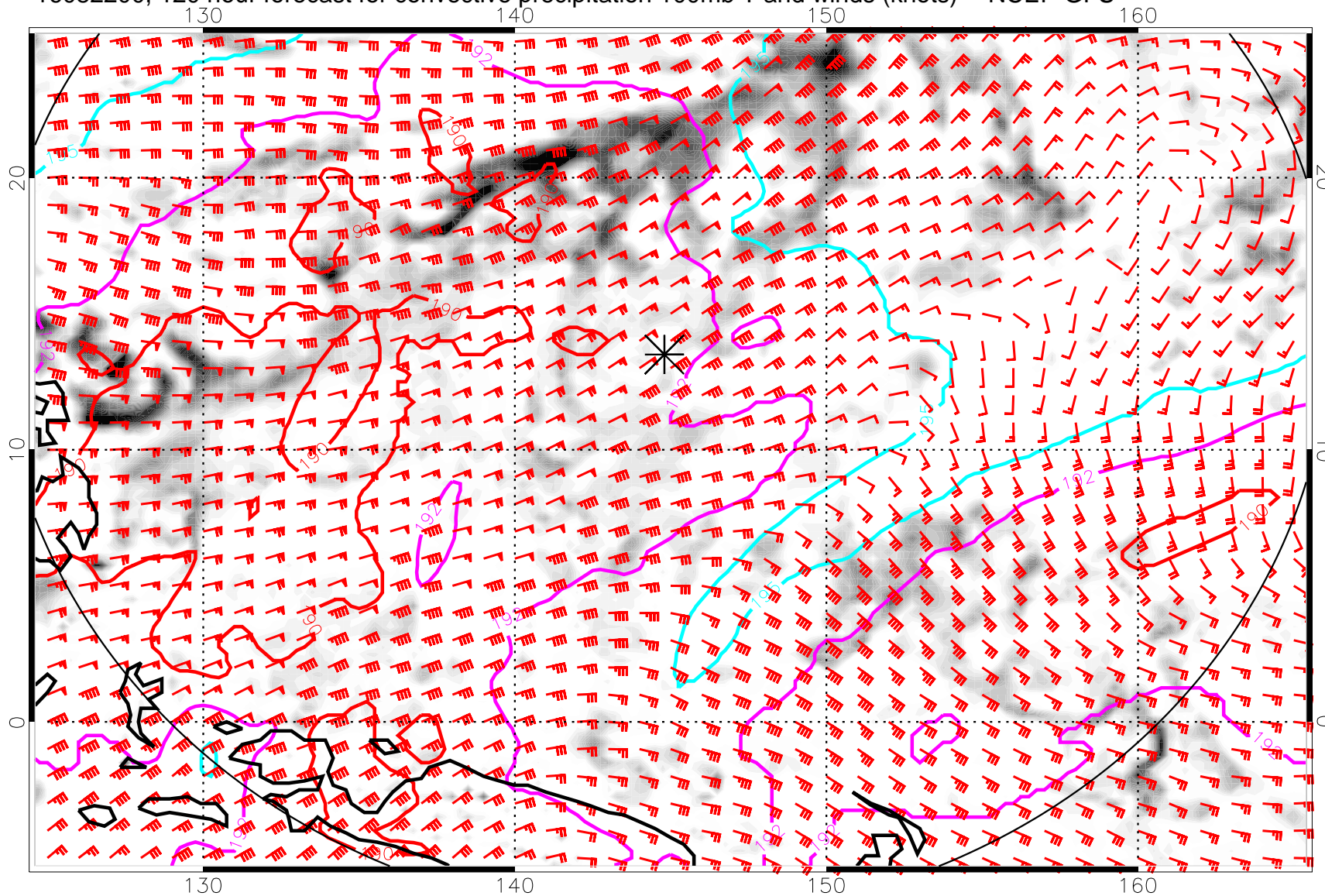
16082200, 120 hour forecast for convective precipitation 100mb T and winds (knots) -- NCEP GFS
