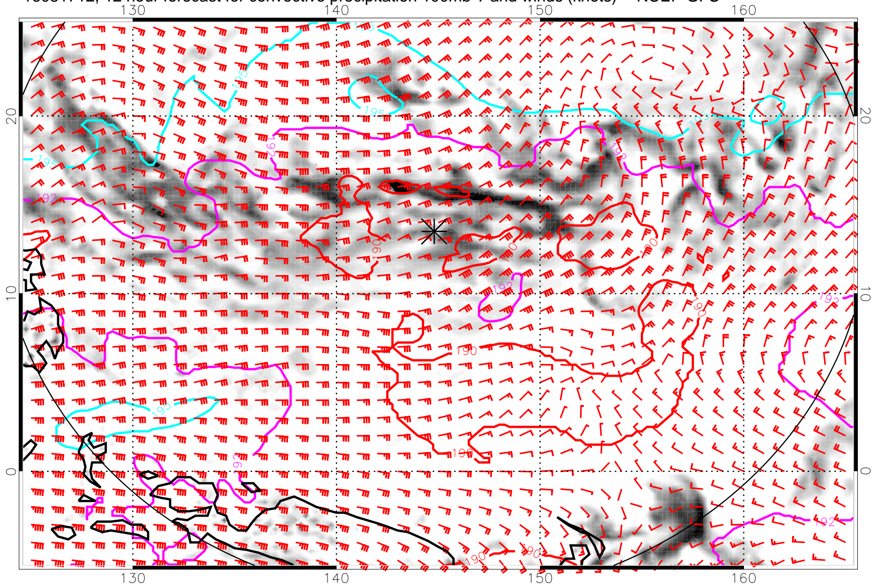
16081712, 12 hour forecast for convective precipitation 100mb T and winds (knots) -- NCEP GFS
