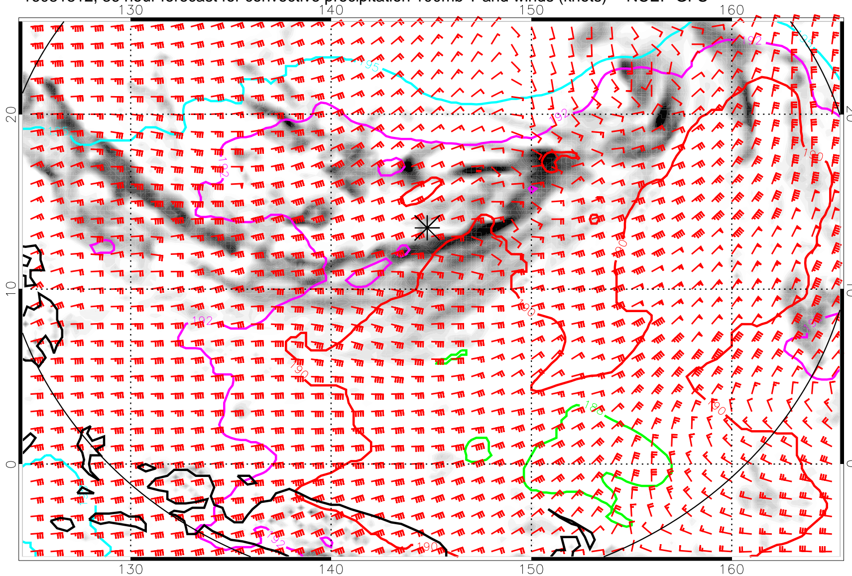
16081812, 36 hour forecast for convective precipitation 100mb T and winds (knots) -- NCEP GFS
