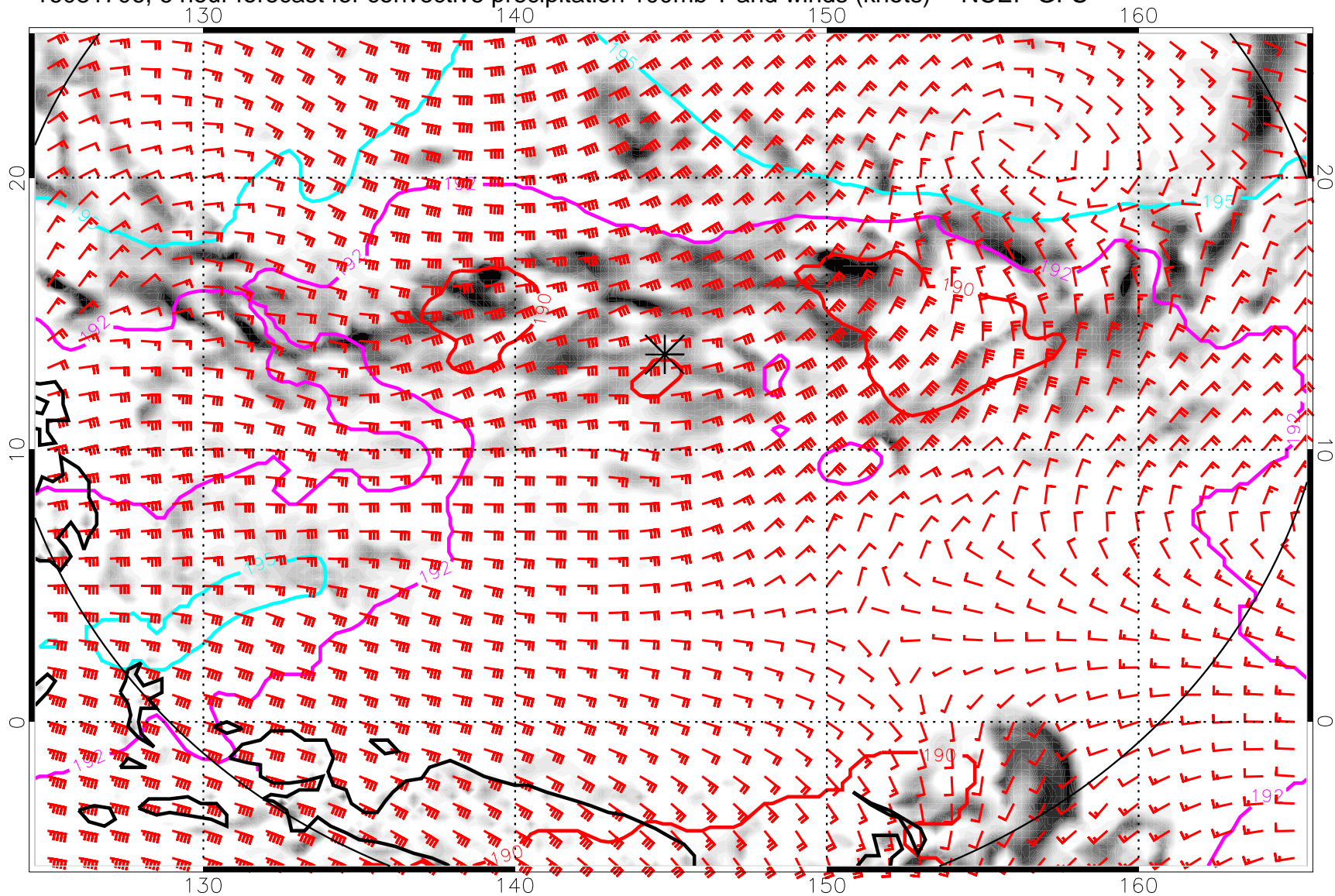
16081706, 6 hour forecast for convective precipitation 100mb T and winds (knots) -- NCEP GFS
