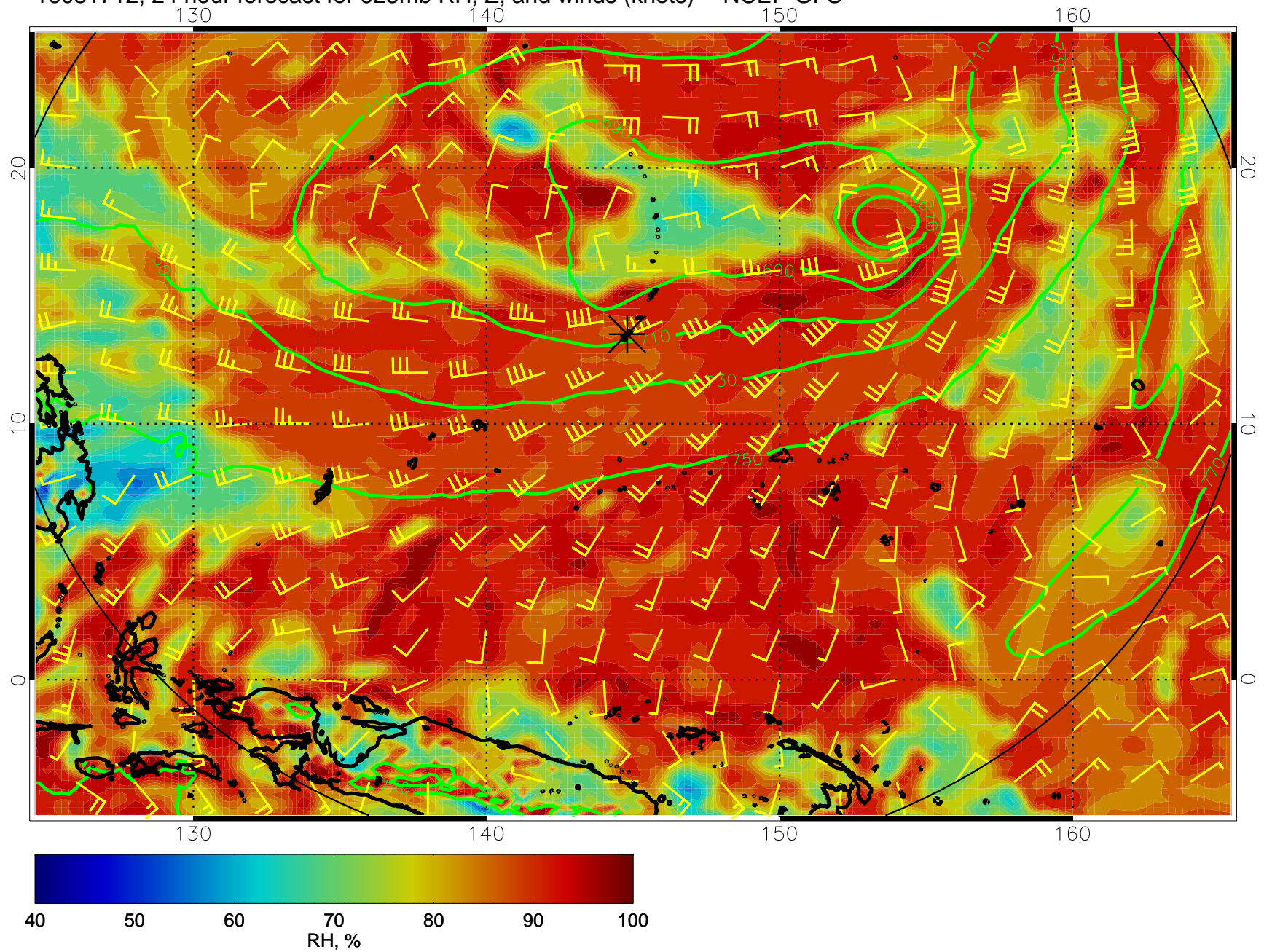
16081712, 24 hour forecast for 925mb RH, Z, and winds (knots) -- NCEP GFS
