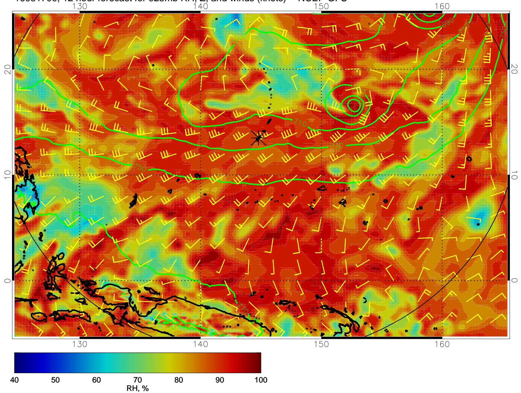
16081700, 12 hour forecast for 925mb RH, Z, and winds (knots) -- NCEP GFS
