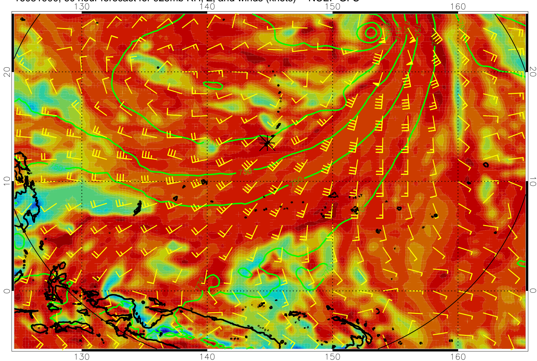
16081900, 60 hour forecast for 925mb RH, Z, and winds (knots) -- NCEP GFS
