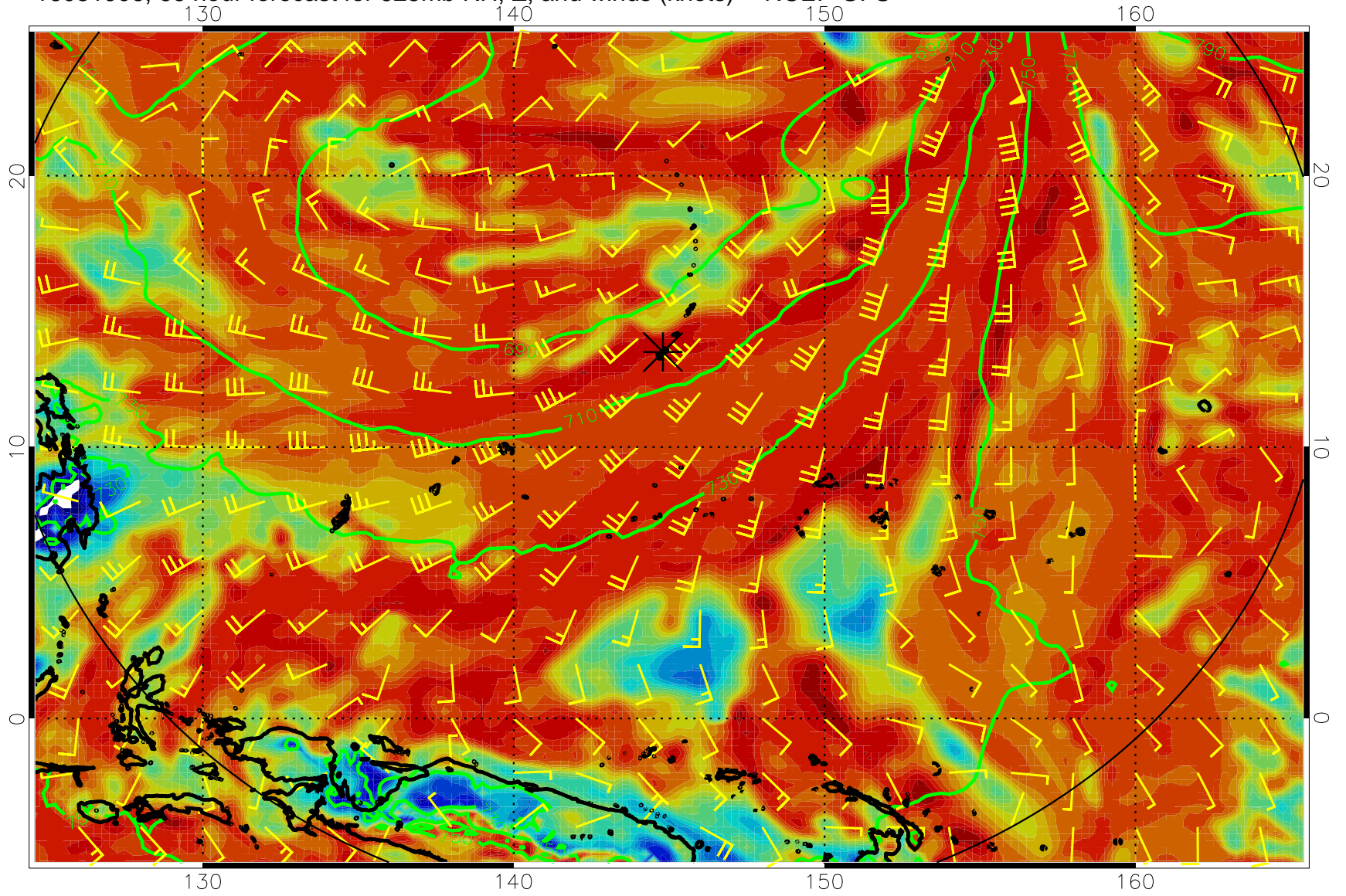
16081906, 66 hour forecast for 925mb RH, Z, and winds (knots) -- NCEP GFS
