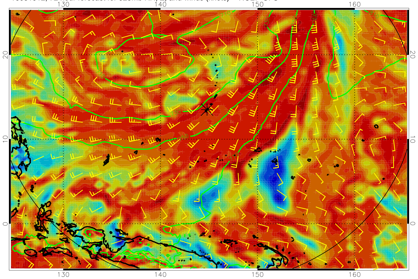
16081912, 72 hour forecast for 925mb RH, Z, and winds (knots) -- NCEP GFS
