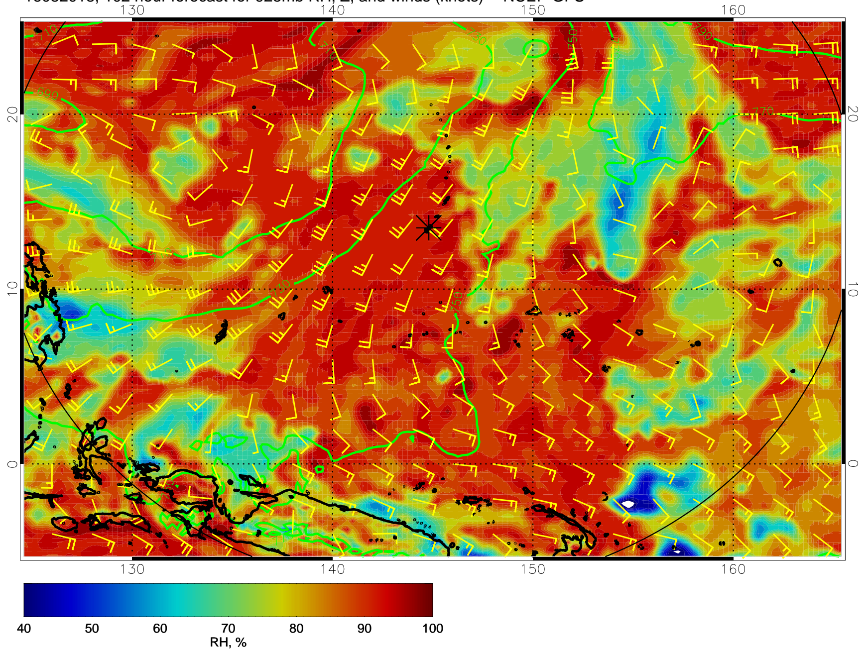
16082018, 102 hour forecast for 925mb RH, Z, and winds (knots) -- NCEP GFS
