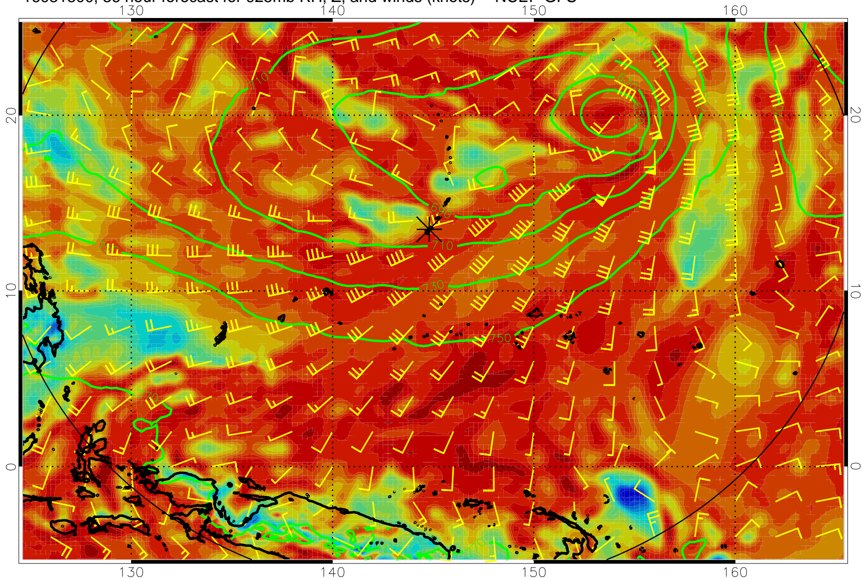
16081800, 36 hour forecast for 925mb RH, Z, and winds (knots) -- NCEP GFS
