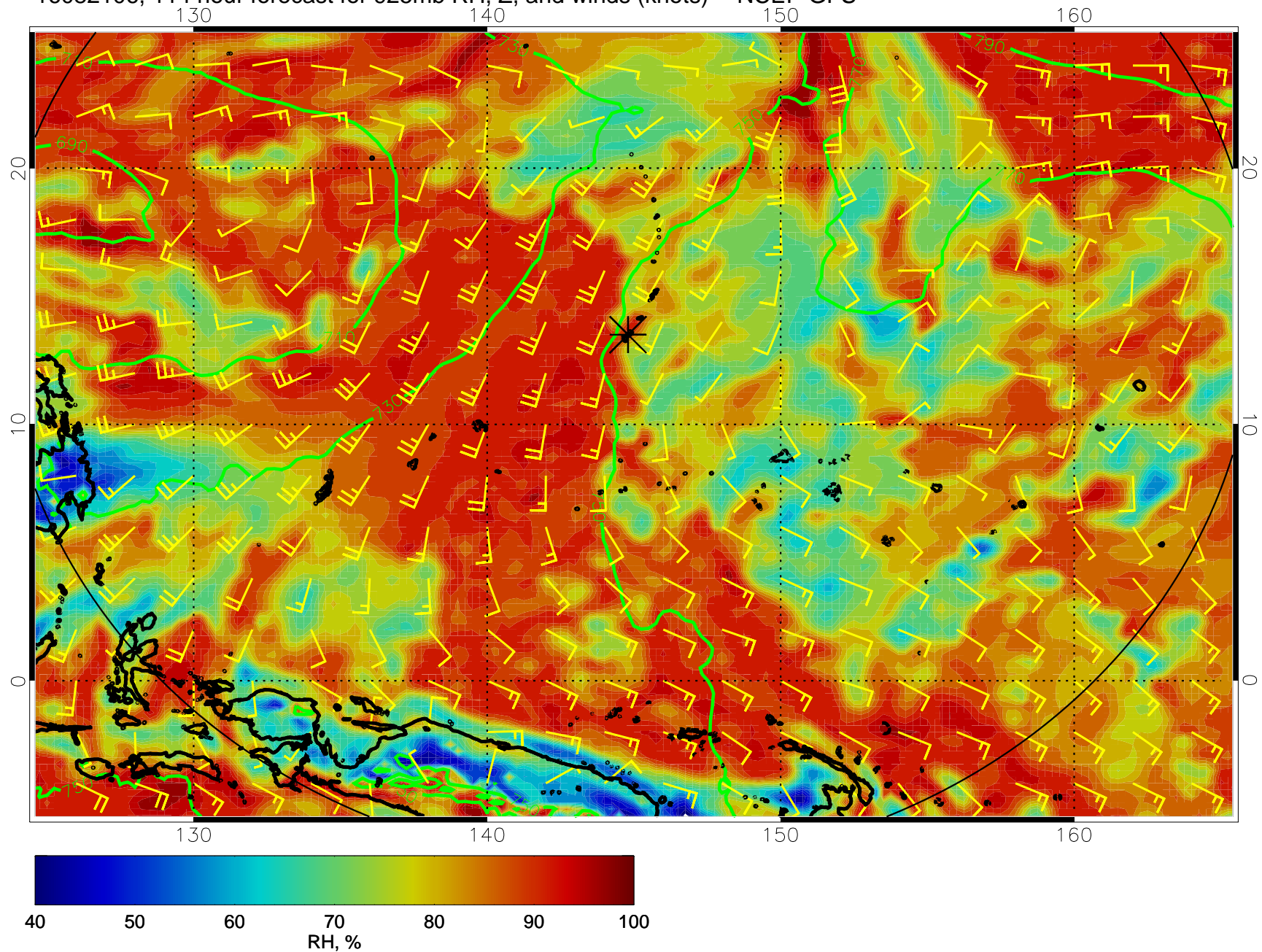
16082106, 114 hour forecast for 925mb RH, Z, and winds (knots) -- NCEP GFS
