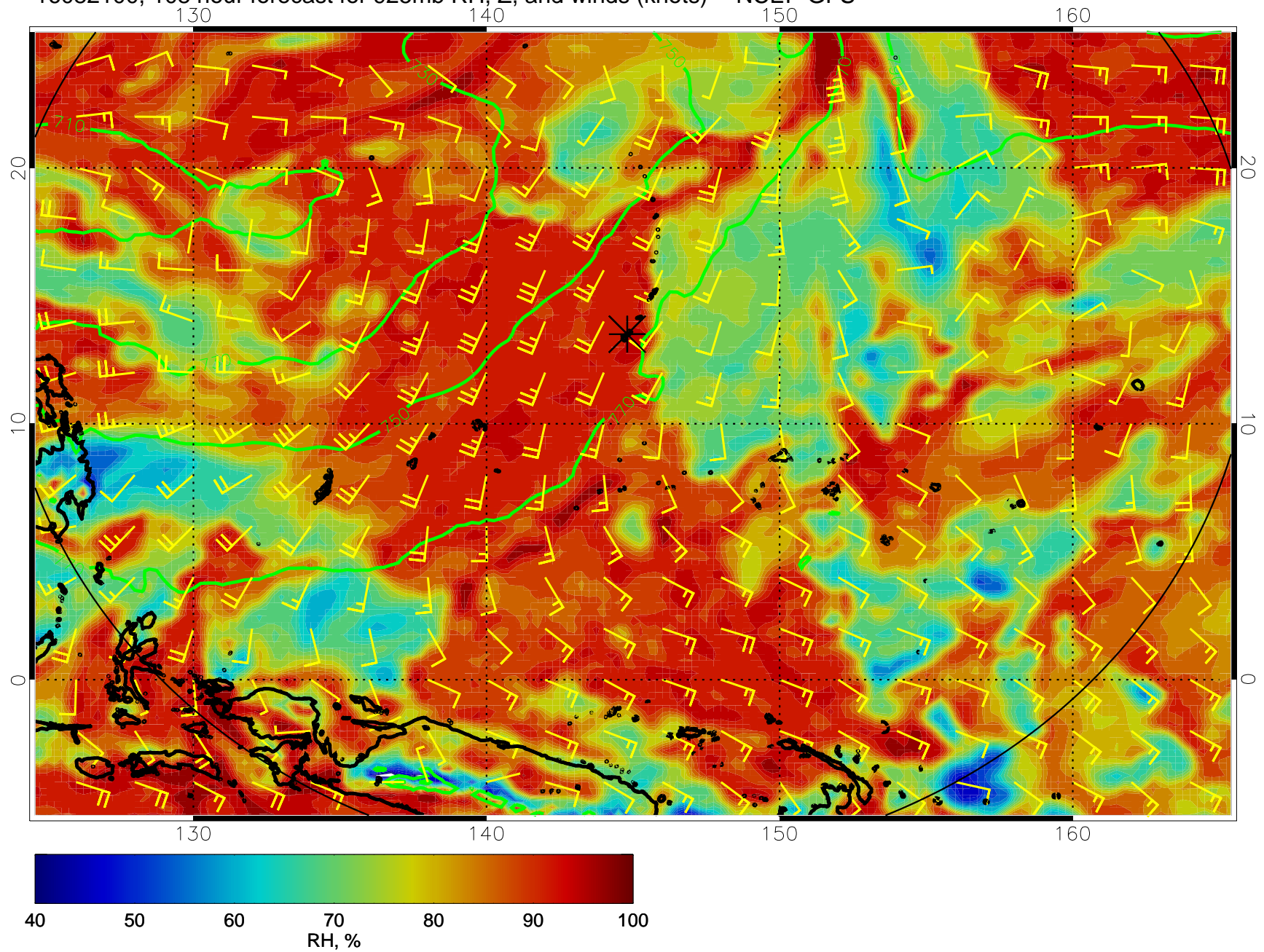
16082100, 108 hour forecast for 925mb RH, Z, and winds (knots) -- NCEP GFS
