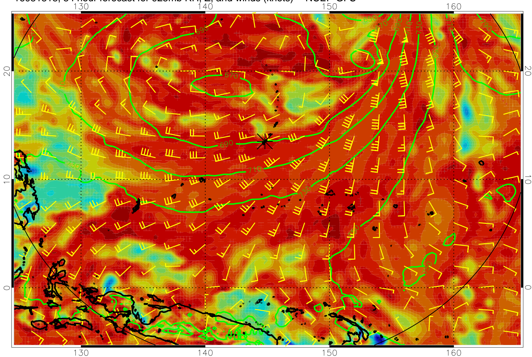
16081818, 54 hour forecast for 925mb RH, Z, and winds (knots) -- NCEP GFS
