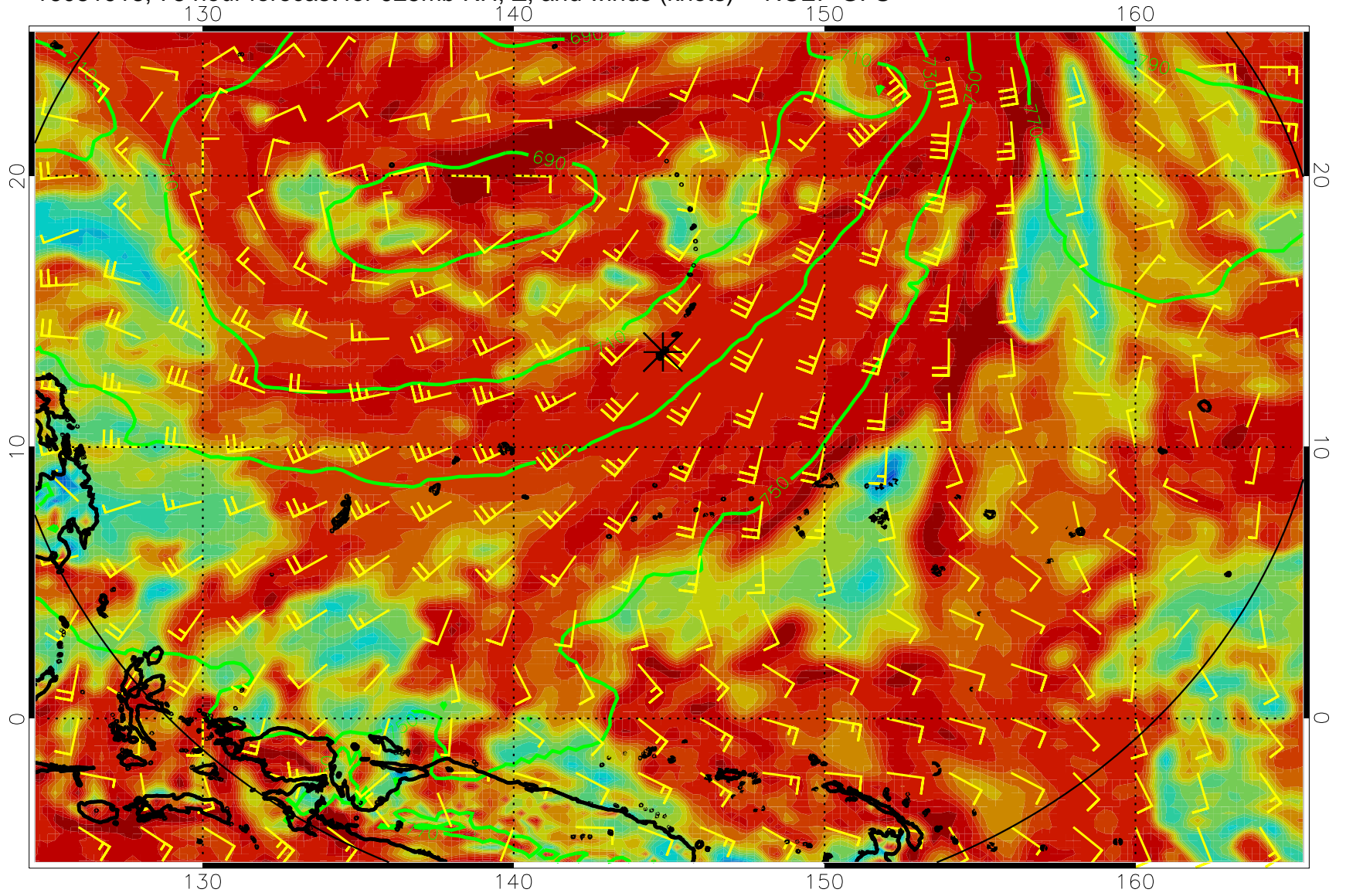
16081918, 78 hour forecast for 925mb RH, Z, and winds (knots) -- NCEP GFS
