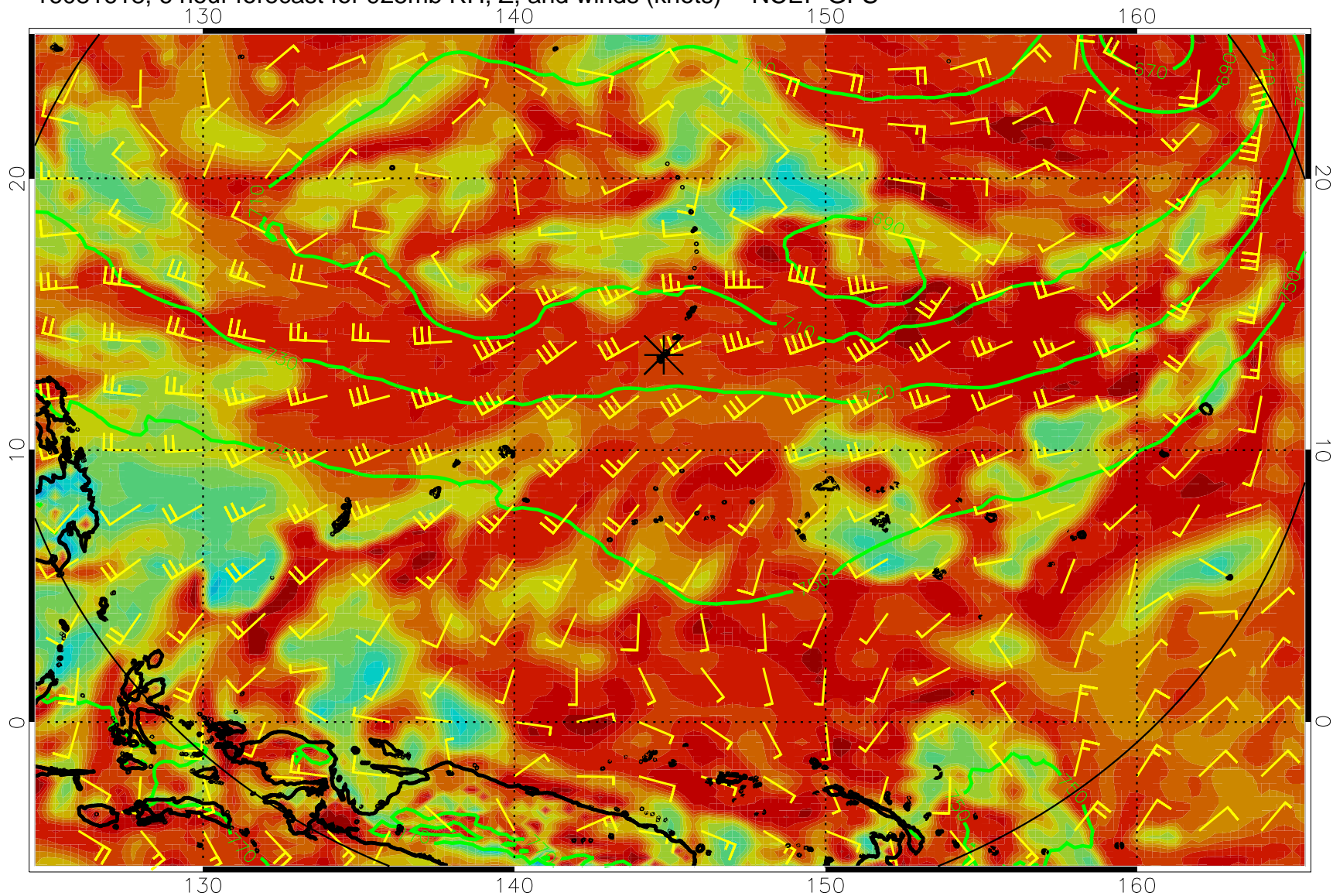
16081618, 6 hour forecast for 925mb RH, Z, and winds (knots) -- NCEP GFS
