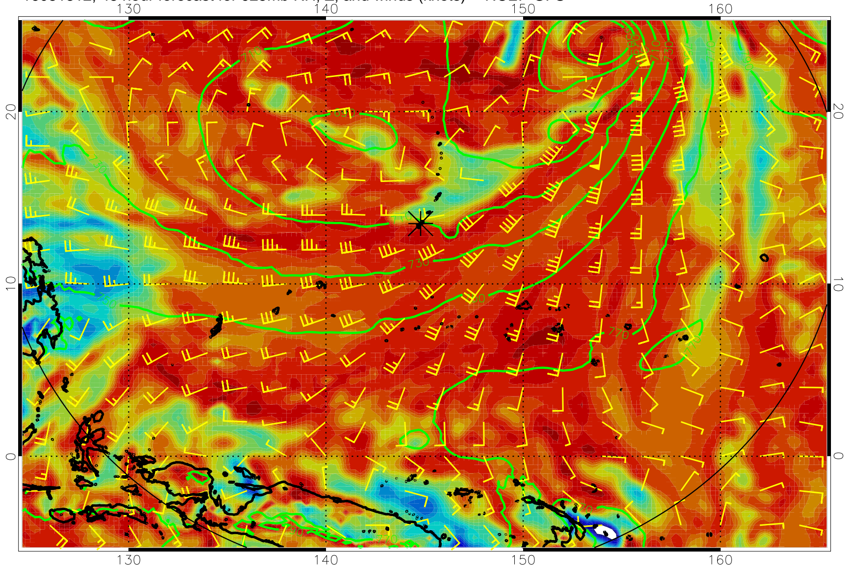
16081812, 48 hour forecast for 925mb RH, Z, and winds (knots) -- NCEP GFS
