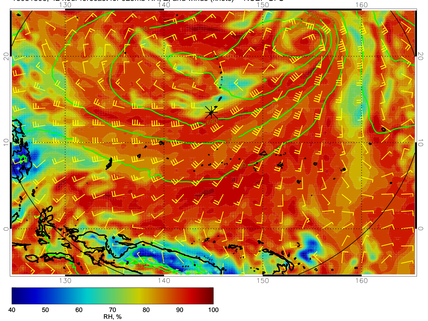
16081806, 42 hour forecast for 925mb RH, Z, and winds (knots) -- NCEP GFS
