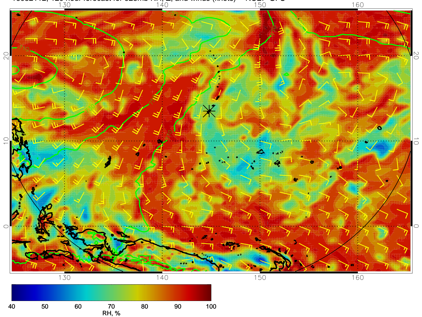
16082112, 120 hour forecast for 925mb RH, Z, and winds (knots) -- NCEP GFS
