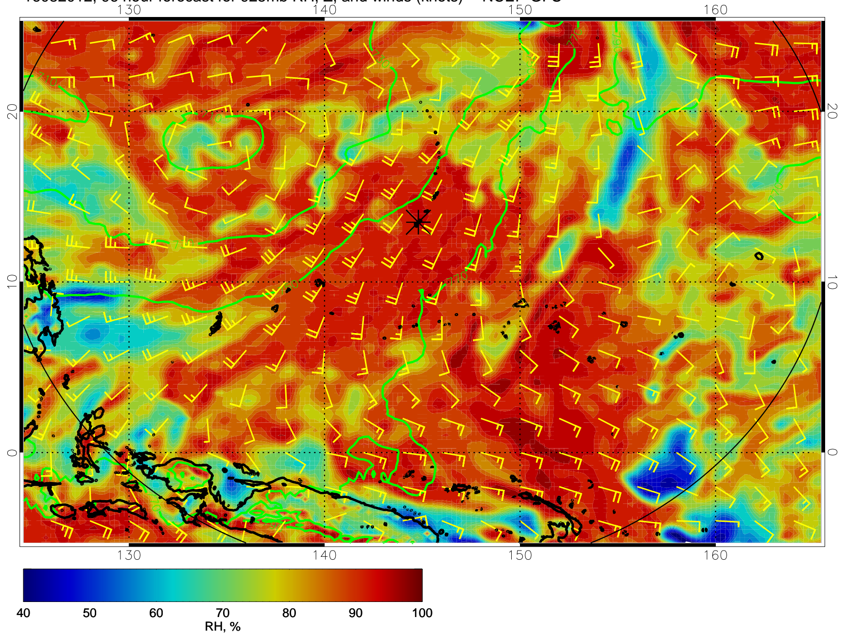
16082012, 96 hour forecast for 925mb RH, Z, and winds (knots) -- NCEP GFS
