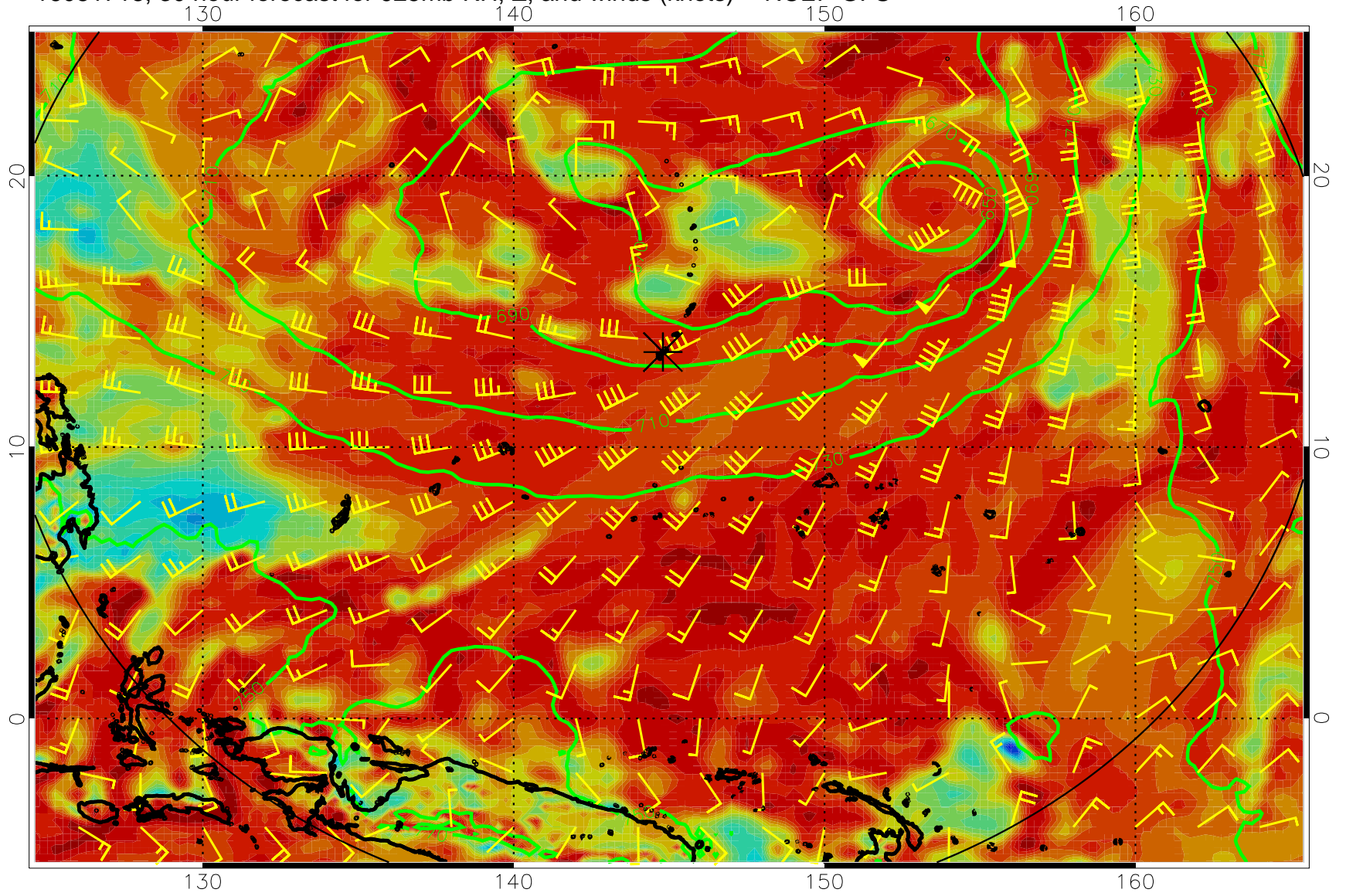
16081718, 30 hour forecast for 925mb RH, Z, and winds (knots) -- NCEP GFS
