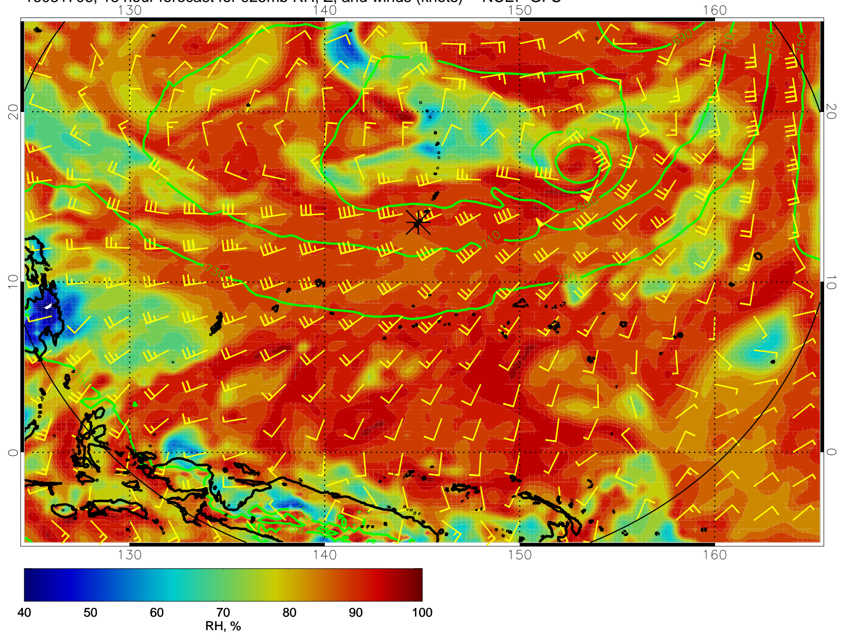
16081706, 18 hour forecast for 925mb RH, Z, and winds (knots) -- NCEP GFS
