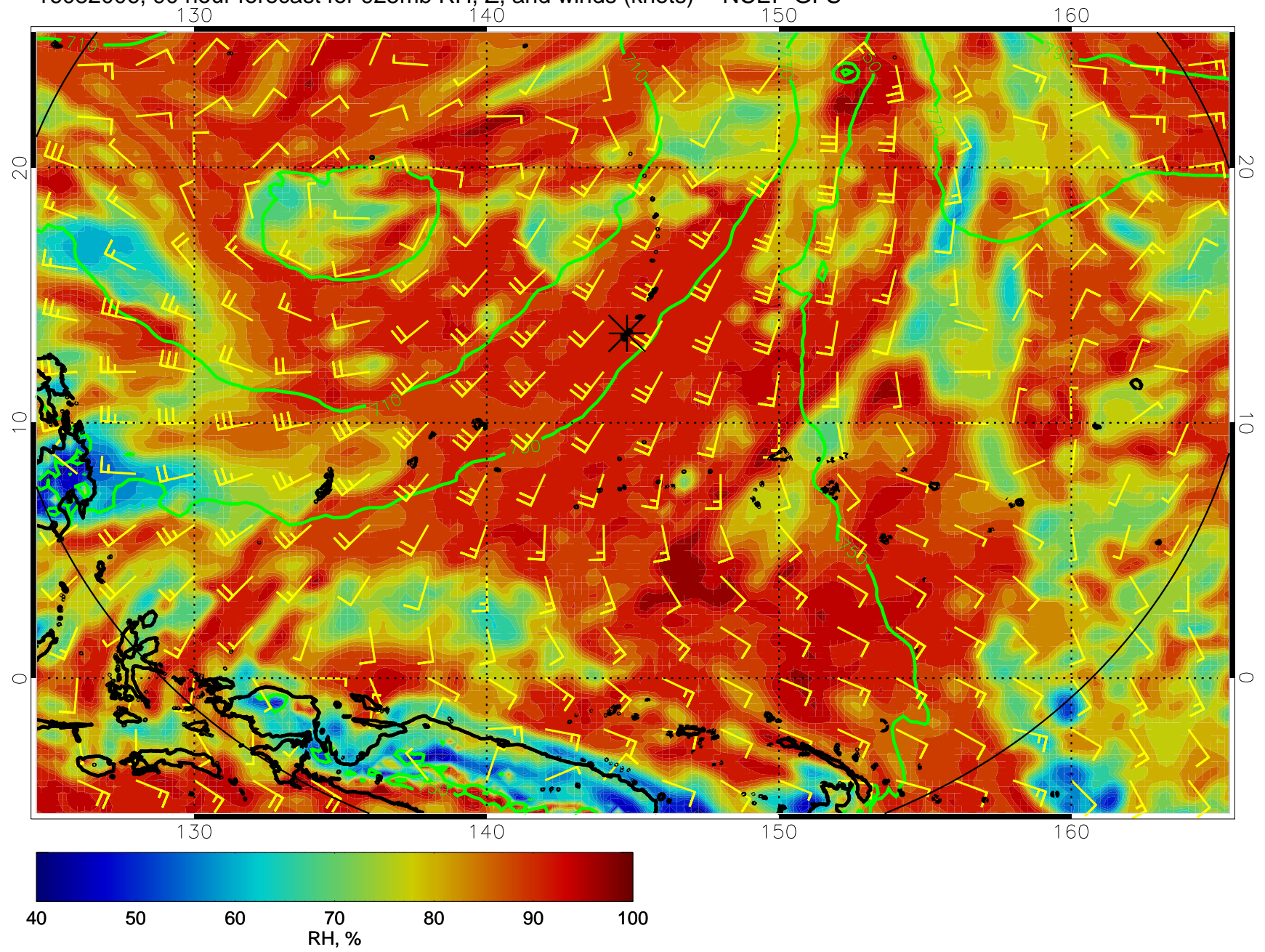
16082006, 90 hour forecast for 925mb RH, Z, and winds (knots) -- NCEP GFS
