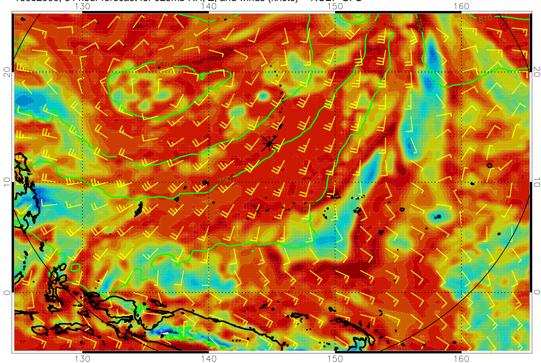
16082000, 84 hour forecast for 925mb RH, Z, and winds (knots) -- NCEP GFS
