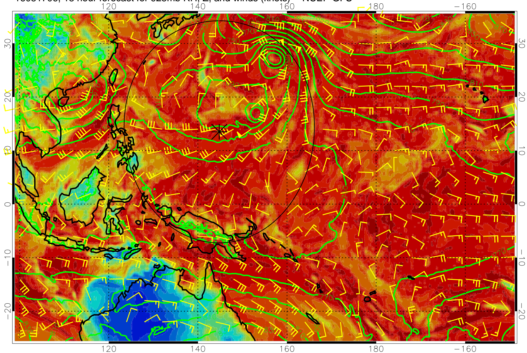
16081706, 18 hour forecast for 925mb RH, Z, and winds (knots) -- NCEP GFS
