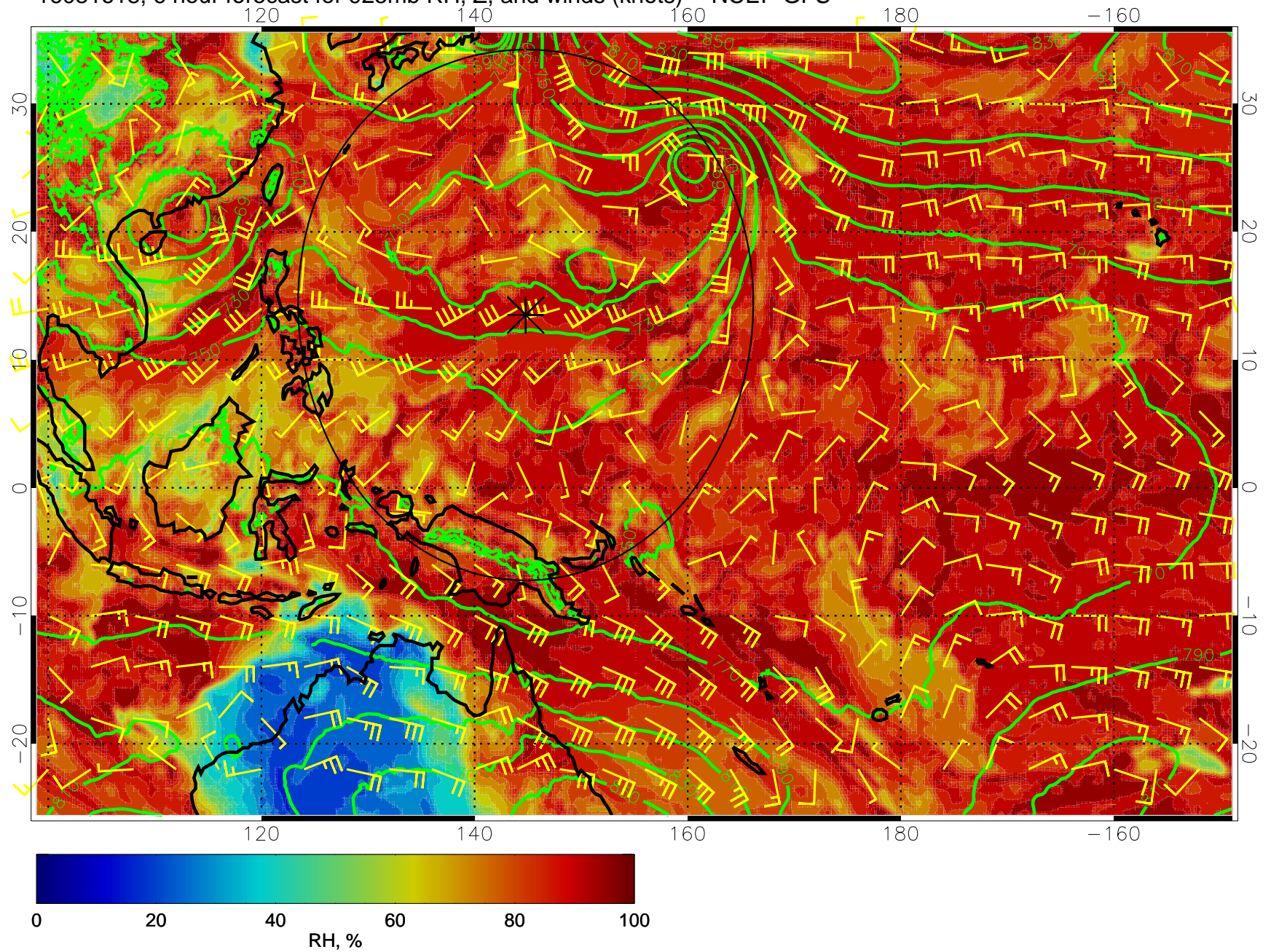
16081618, 6 hour forecast for 925mb RH, Z, and winds (knots) -- NCEP GFS
