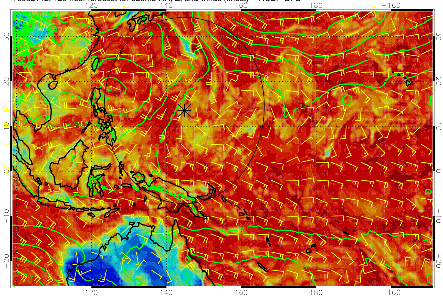
16082112, 120 hour forecast for 925mb RH, Z, and winds (knots) -- NCEP GFS
