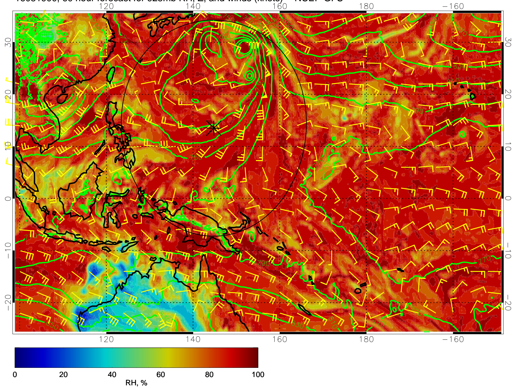
16081900, 60 hour forecast for 925mb RH, Z, and winds (knots) -- NCEP GFS
