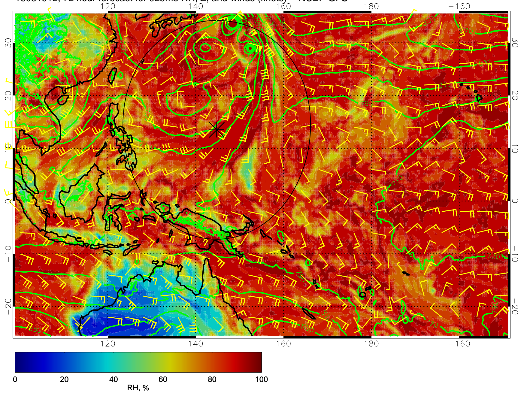
16081912, 72 hour forecast for 925mb RH, Z, and winds (knots) -- NCEP GFS
