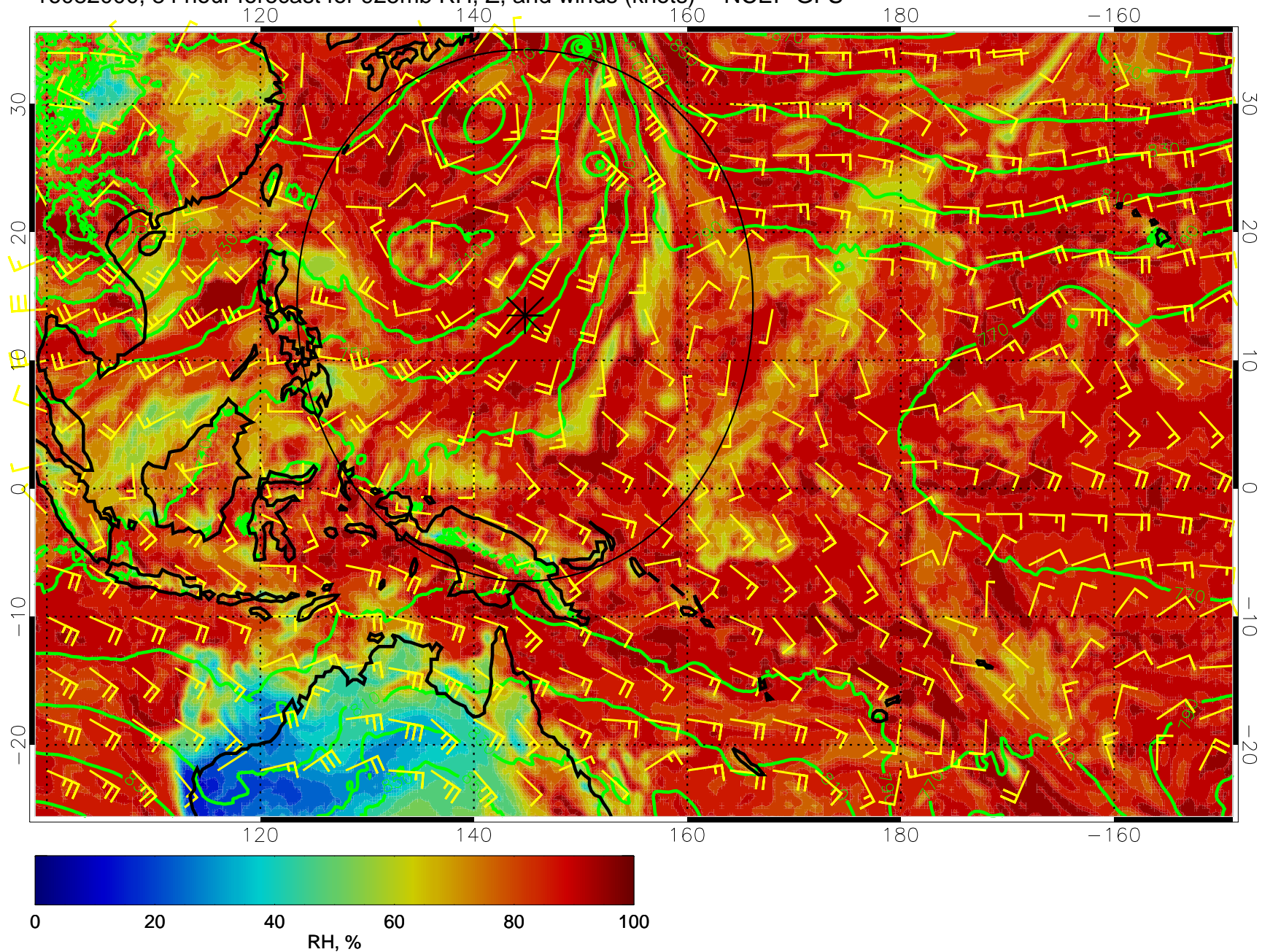
16082000, 84 hour forecast for 925mb RH, Z, and winds (knots) -- NCEP GFS
