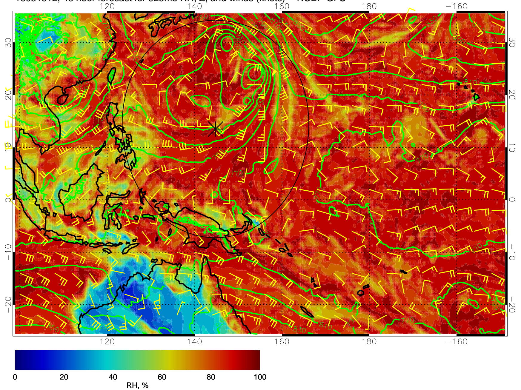
16081812, 48 hour forecast for 925mb RH, Z, and winds (knots) -- NCEP GFS
