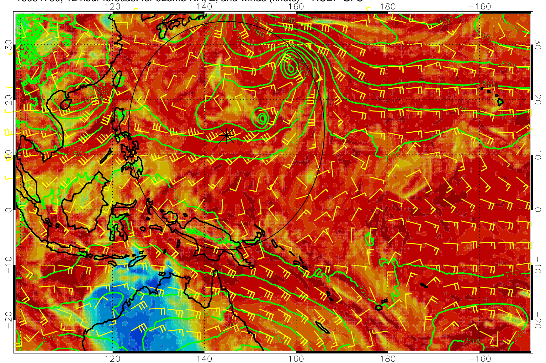
16081700, 12 hour forecast for 925mb RH, Z, and winds (knots) -- NCEP GFS
