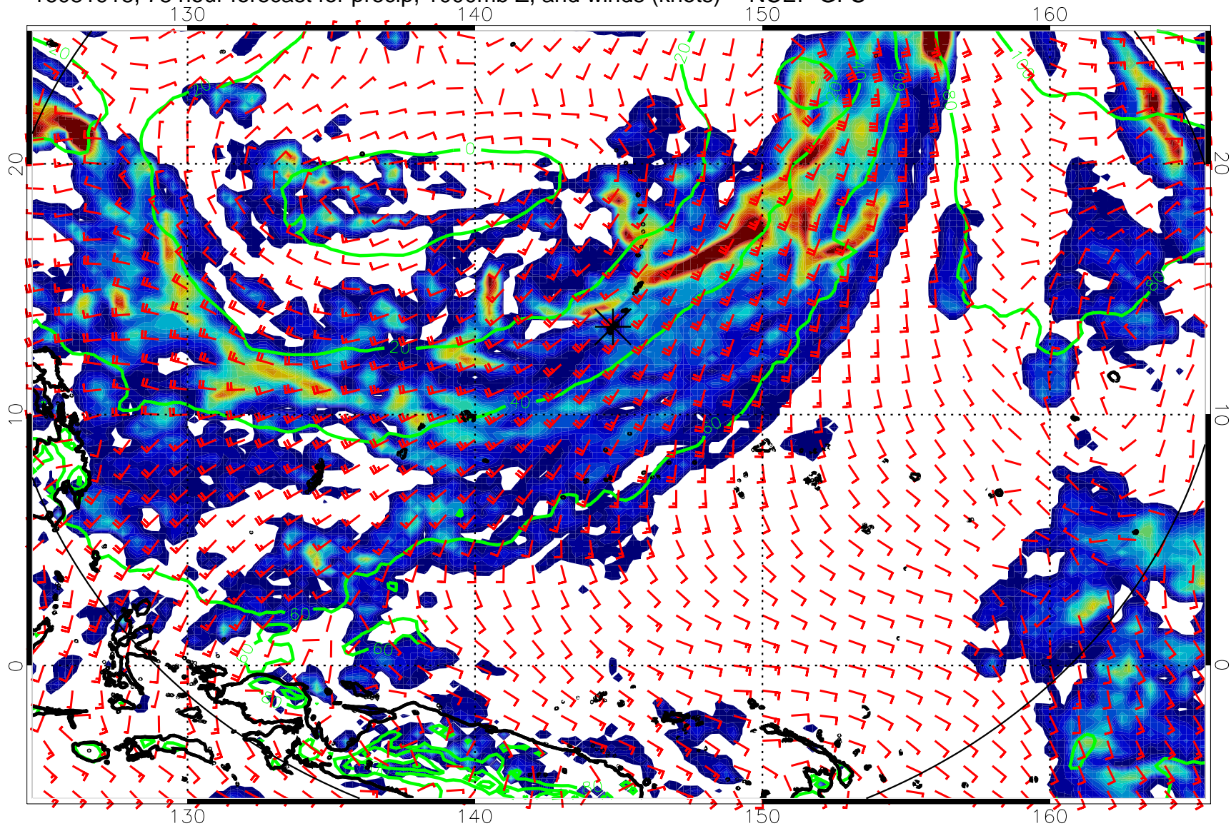
16081918, 78 hour forecast for precip, 1000mb Z, and winds (knots) -- NCEP GFS
