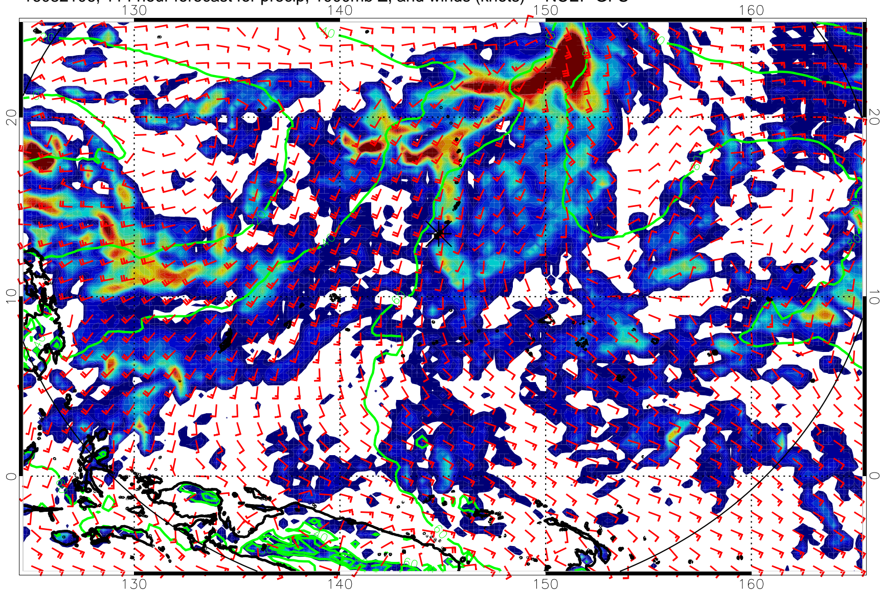
16082106, 114 hour forecast for precip, 1000mb Z, and winds (knots) -- NCEP GFS
