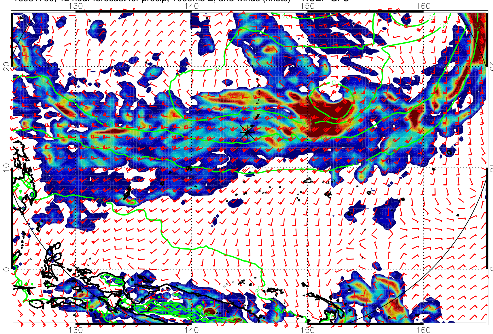
16081700, 12 hour forecast for precip, 1000mb Z, and winds (knots) -- NCEP GFS
