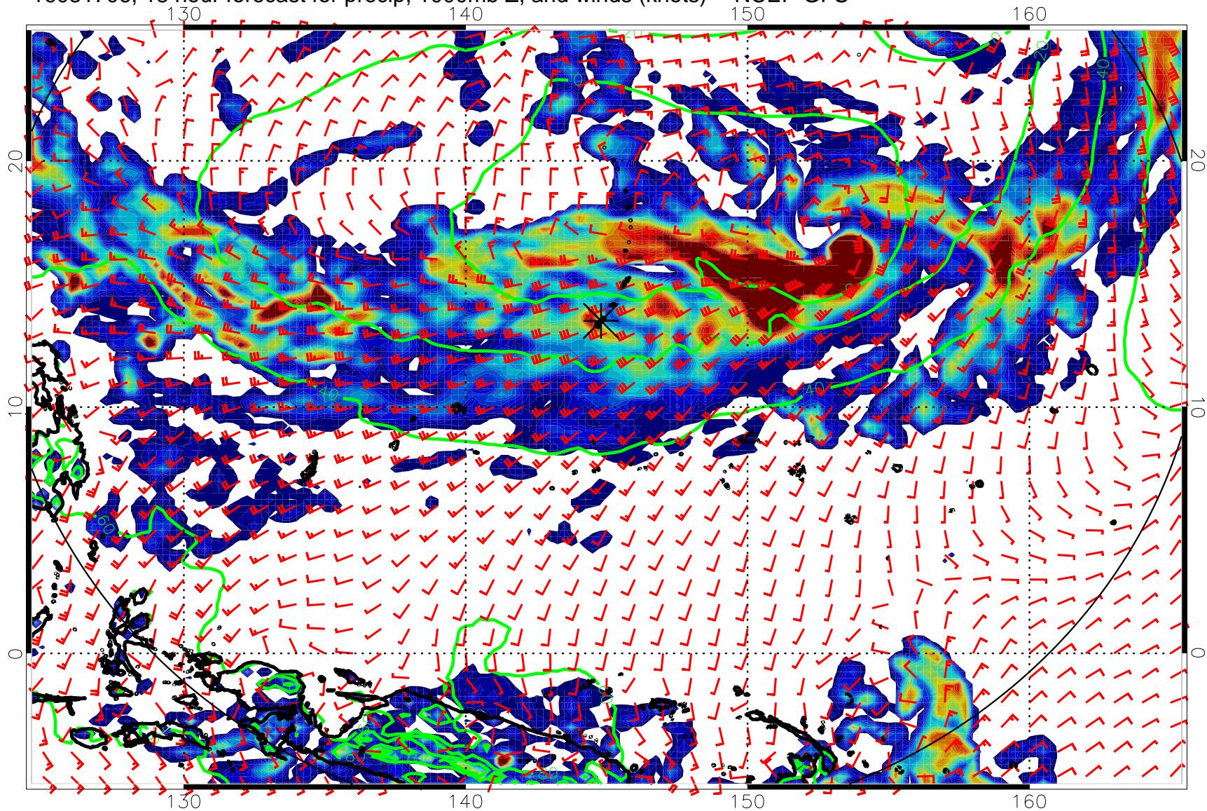
16081706, 18 hour forecast for precip, 1000mb Z, and winds (knots) -- NCEP GFS
