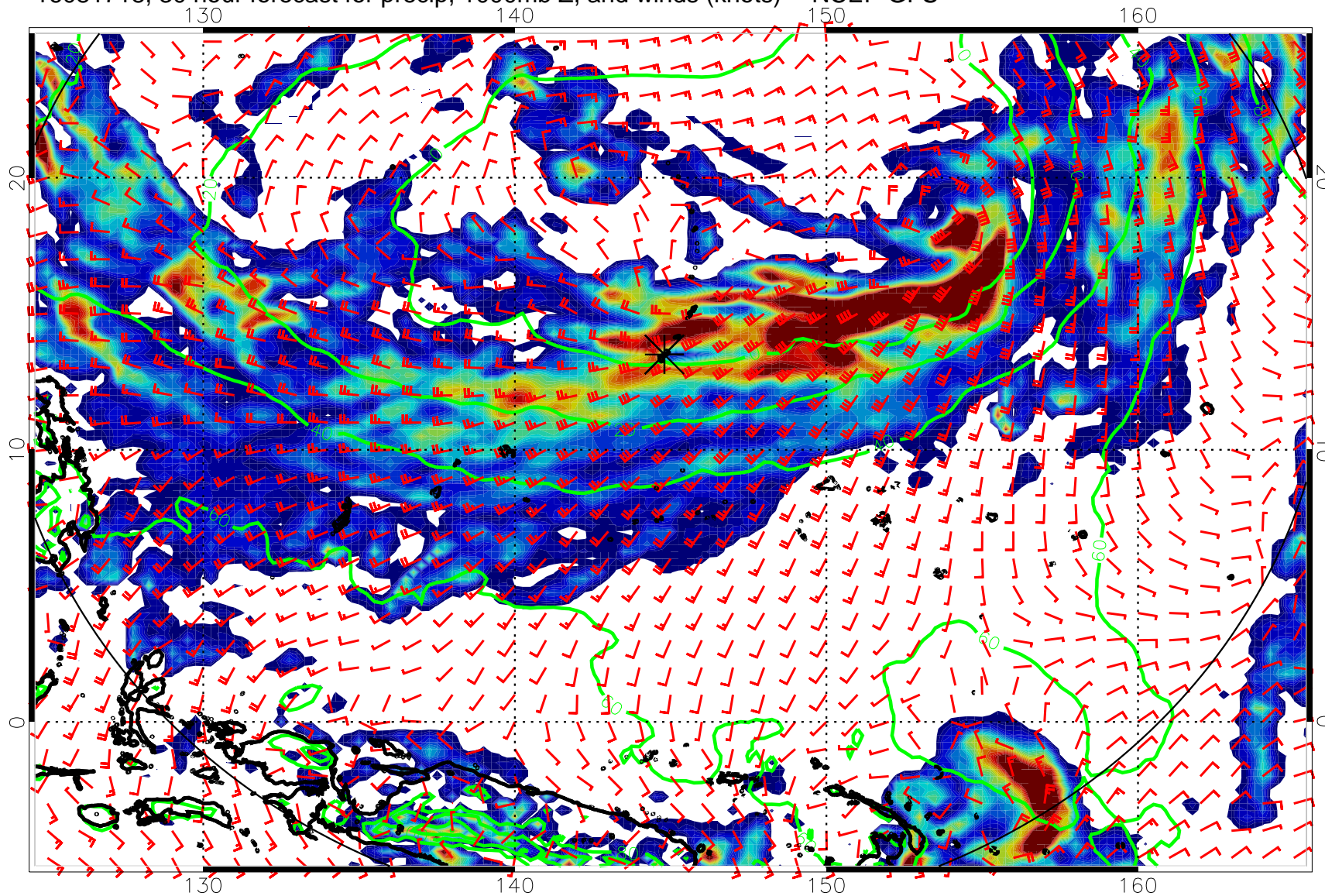
16081718, 30 hour forecast for precip, 1000mb Z, and winds (knots) -- NCEP GFS
