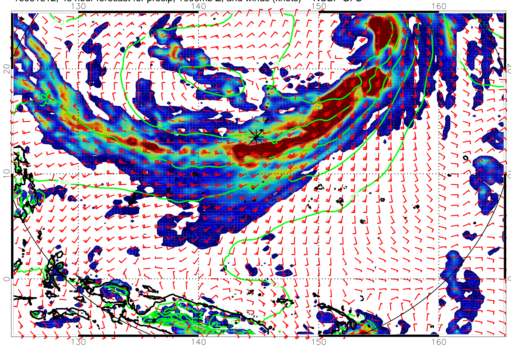
16081812, 48 hour forecast for precip, 1000mb Z, and winds (knots) -- NCEP GFS
