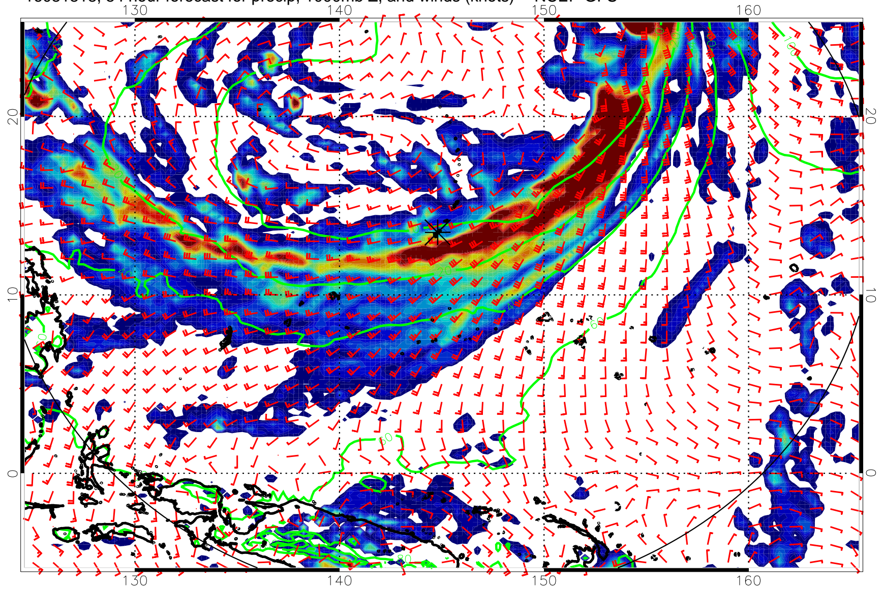
16081818, 54 hour forecast for precip, 1000mb Z, and winds (knots) -- NCEP GFS
