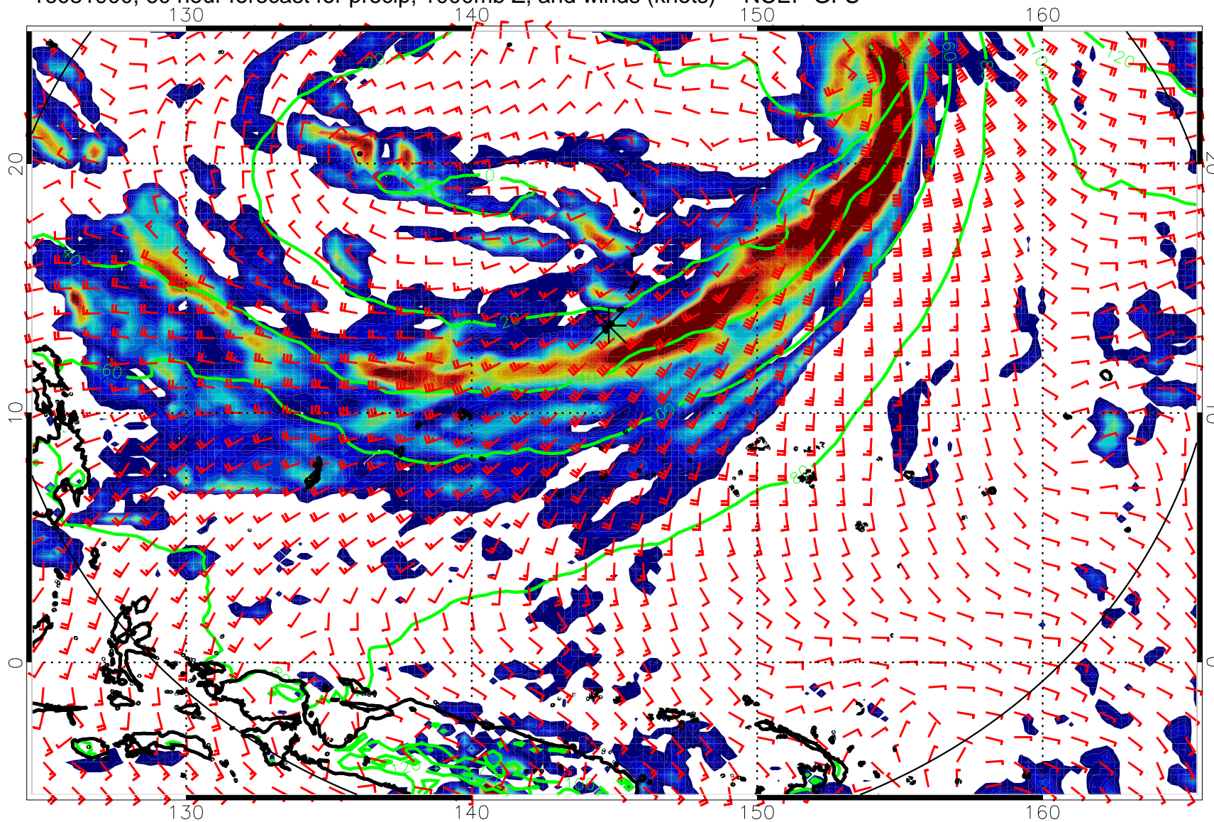
16081900, 60 hour forecast for precip, 1000mb Z, and winds (knots) -- NCEP GFS
