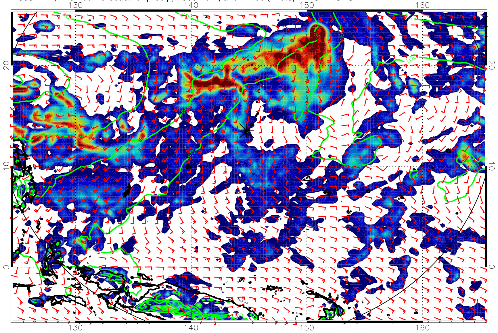
16082112, 120 hour forecast for precip, 1000mb Z, and winds (knots) -- NCEP GFS
