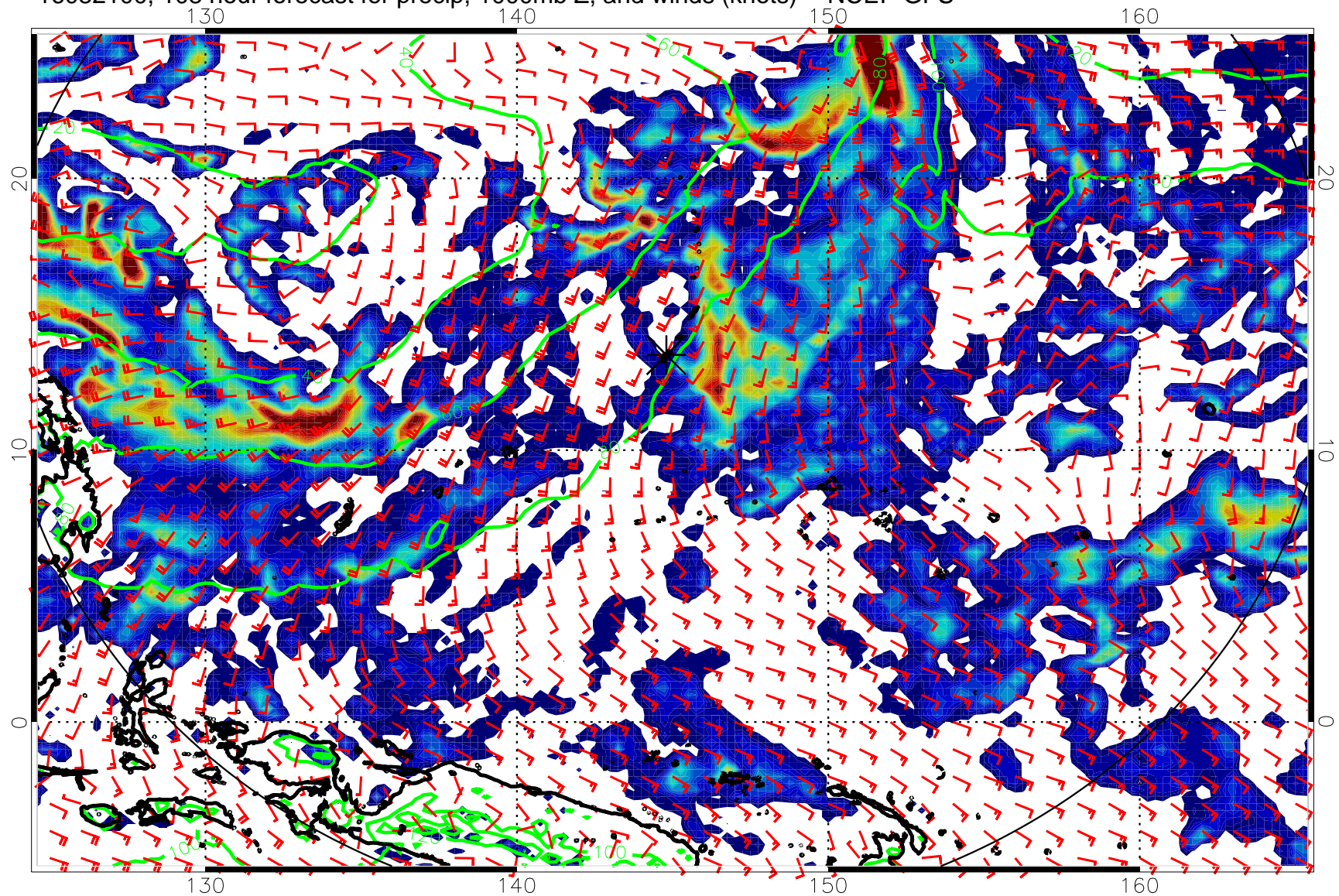
16082100, 108 hour forecast for precip, 1000mb Z, and winds (knots) -- NCEP GFS
