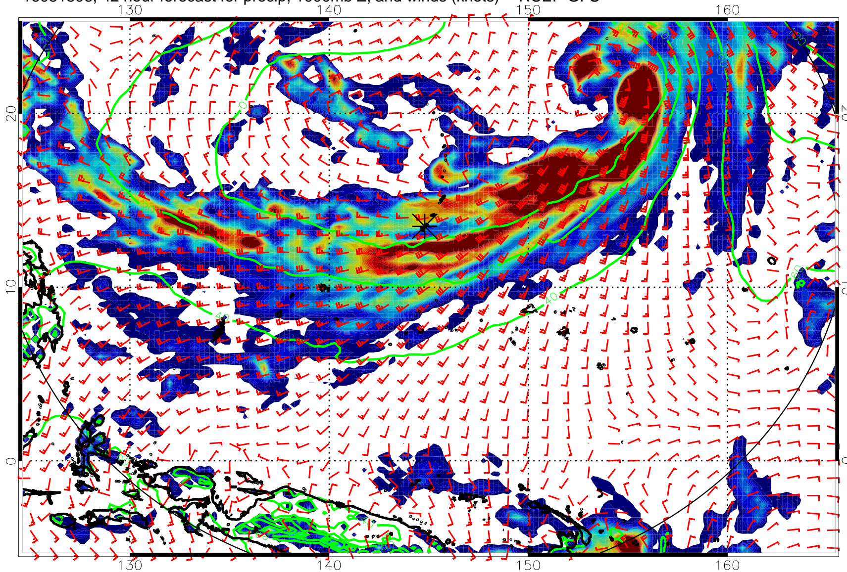
16081806, 42 hour forecast for precip, 1000mb Z, and winds (knots) -- NCEP GFS
