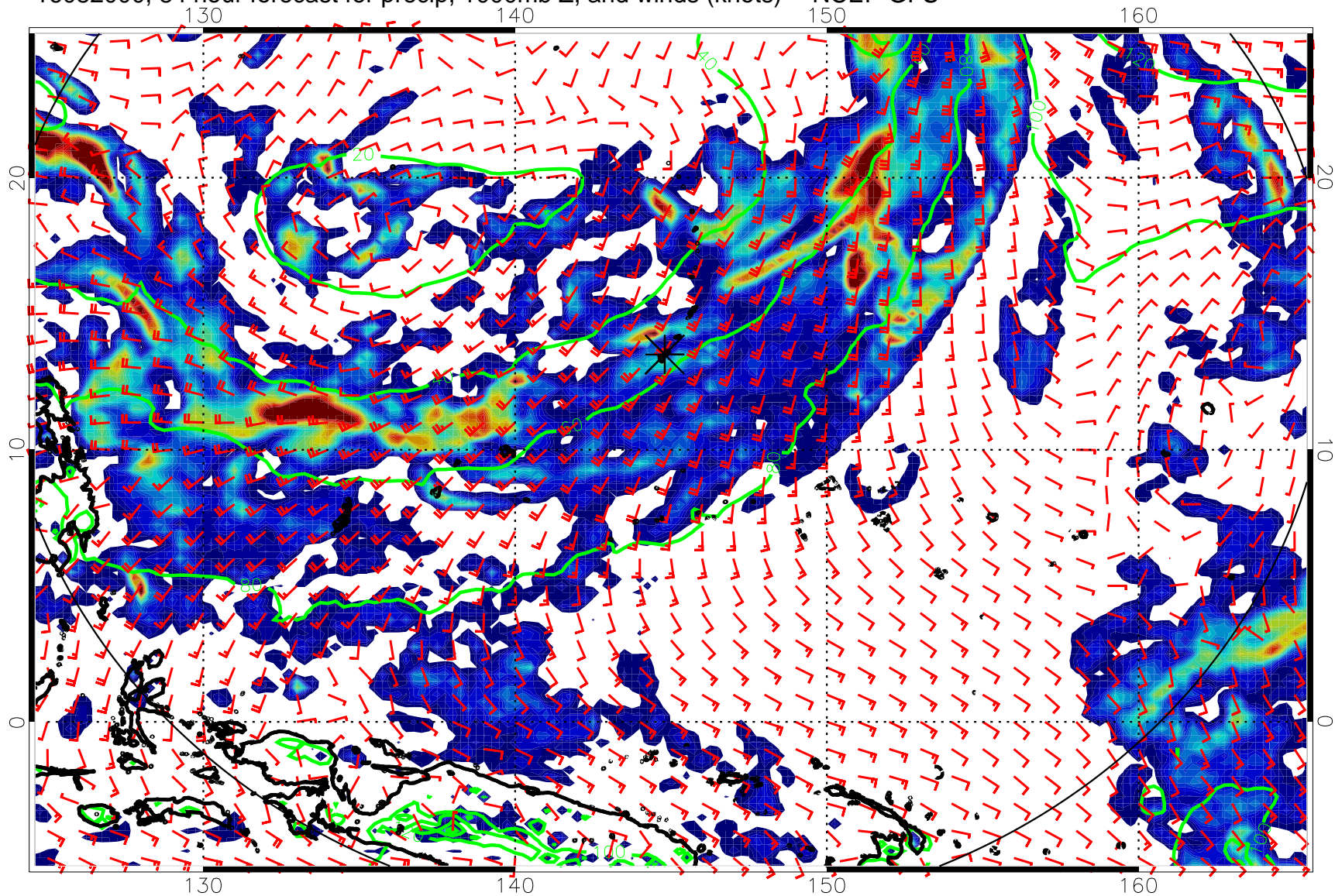
16082000, 84 hour forecast for precip, 1000mb Z, and winds (knots) -- NCEP GFS
