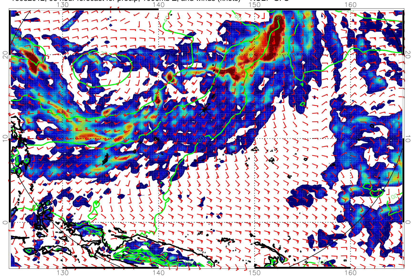
16082012, 96 hour forecast for precip, 1000mb Z, and winds (knots) -- NCEP GFS
