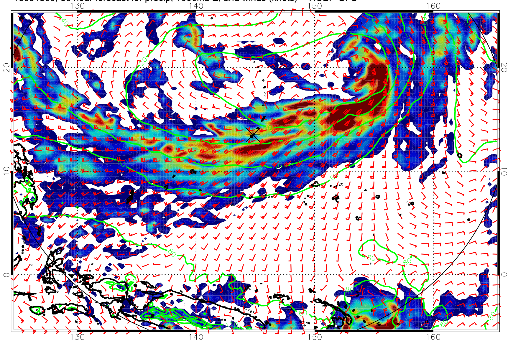
16081800, 36 hour forecast for precip, 1000mb Z, and winds (knots) -- NCEP GFS
