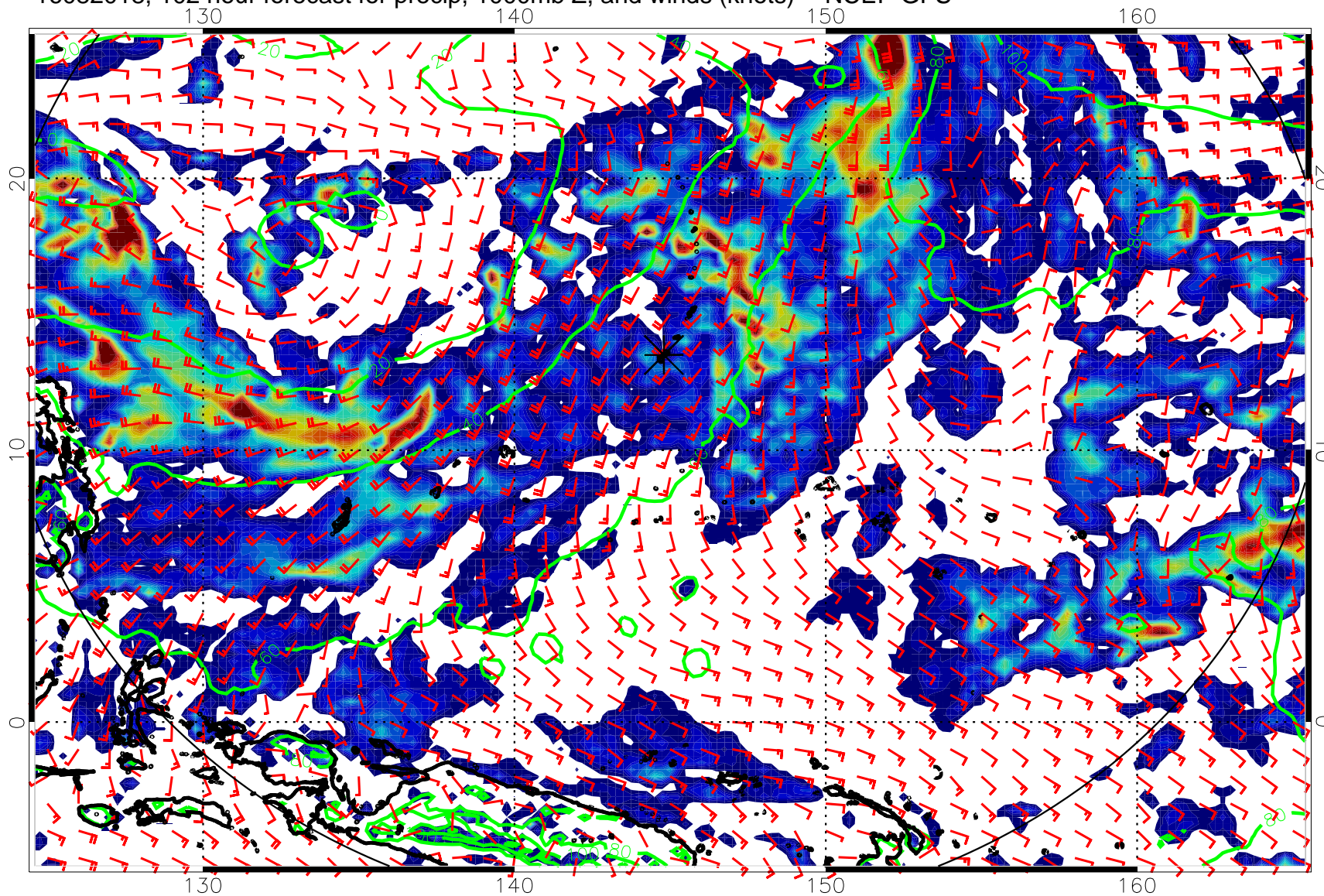
16082018, 102 hour forecast for precip, 1000mb Z, and winds (knots) -- NCEP GFS
