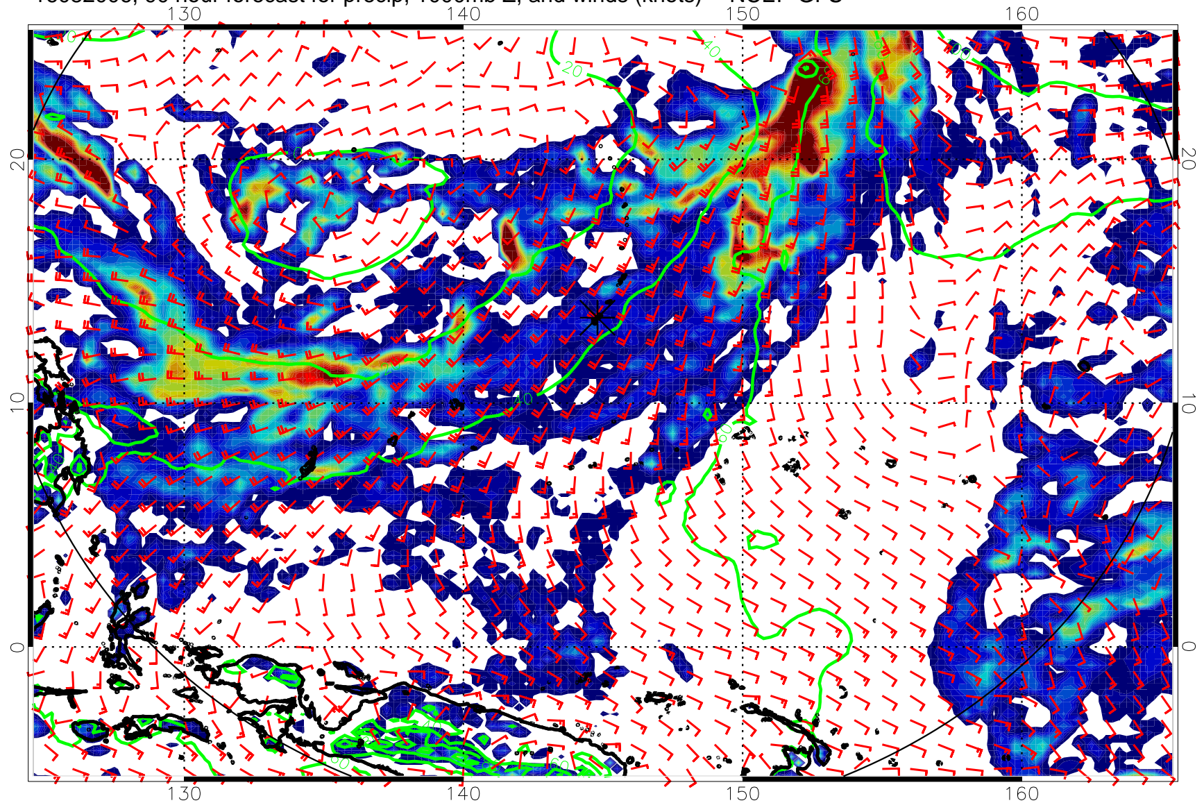
16082006, 90 hour forecast for precip, 1000mb Z, and winds (knots) -- NCEP GFS
