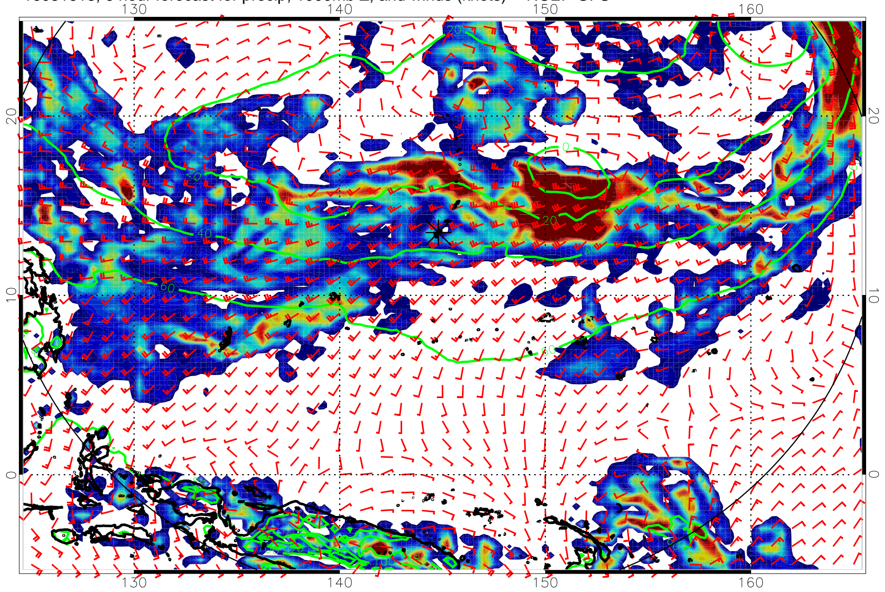
16081618, 6 hour forecast for precip, 1000mb Z, and winds (knots) -- NCEP GFS
