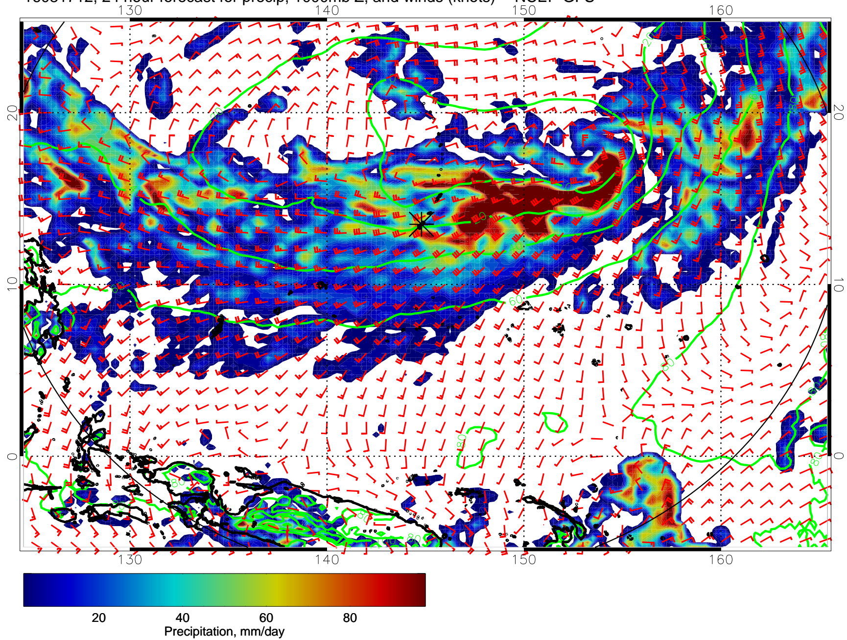
16081712, 24 hour forecast for precip, 1000mb Z, and winds (knots) -- NCEP GFS
