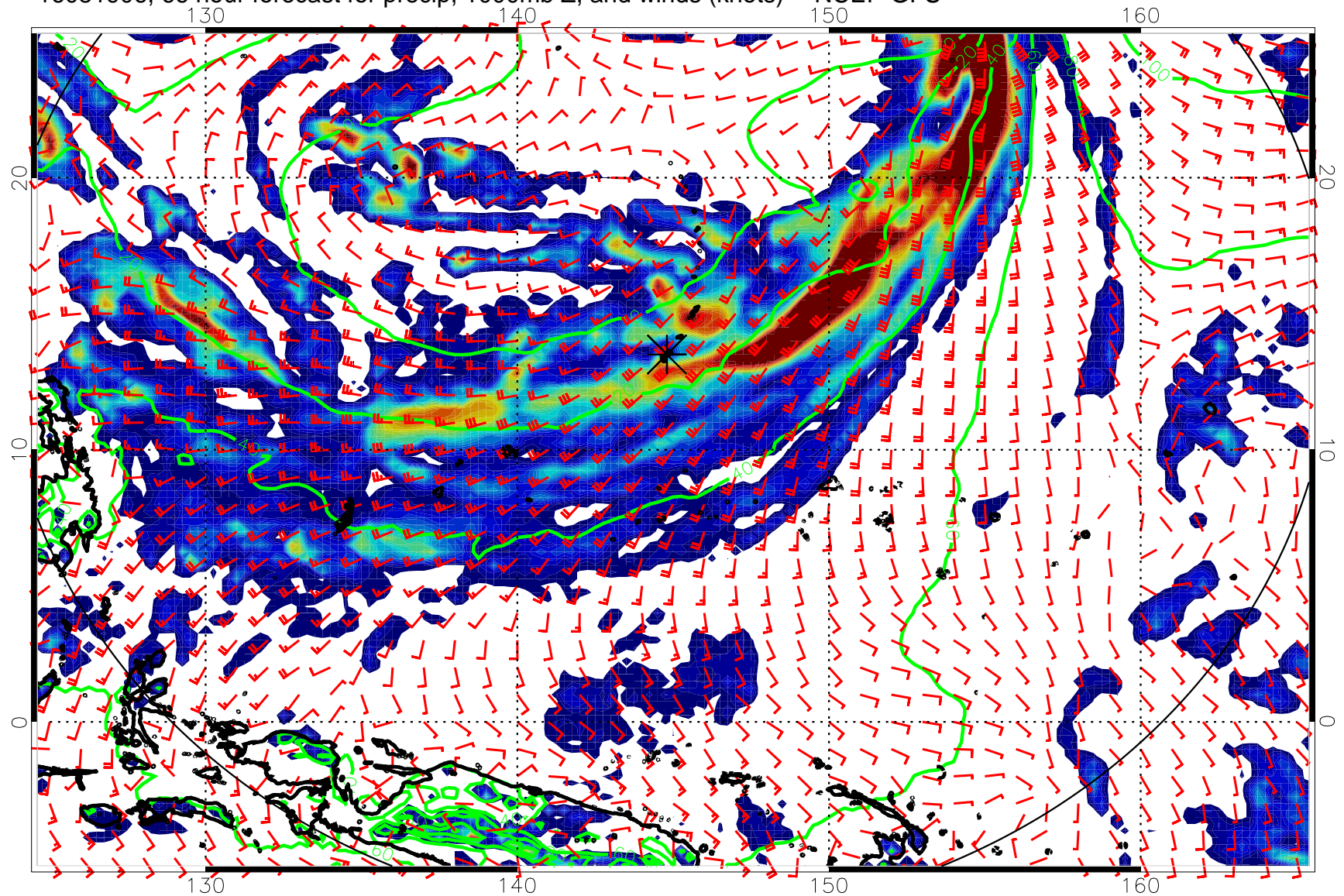
16081906, 66 hour forecast for precip, 1000mb Z, and winds (knots) -- NCEP GFS
