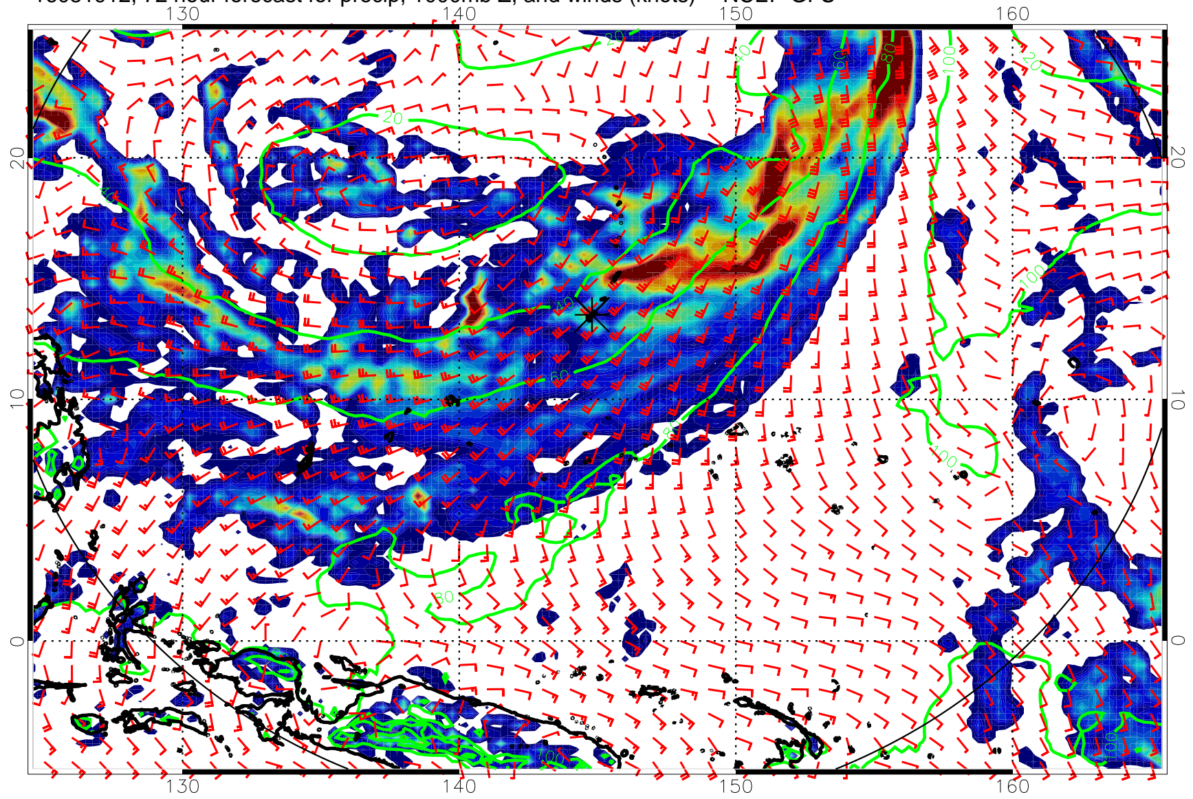
16081912, 72 hour forecast for precip, 1000mb Z, and winds (knots) -- NCEP GFS
