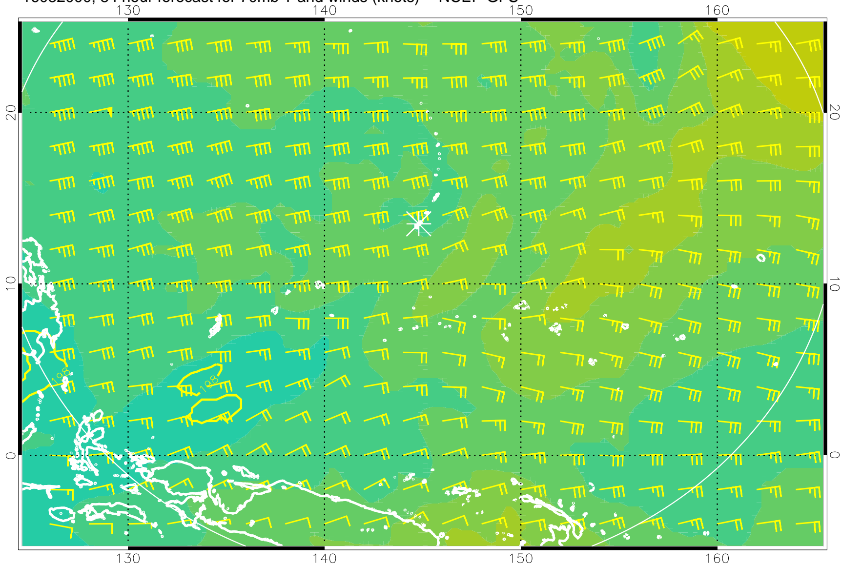
16082000, 84 hour forecast for 70mb T and winds (knots) -- NCEP GFS
