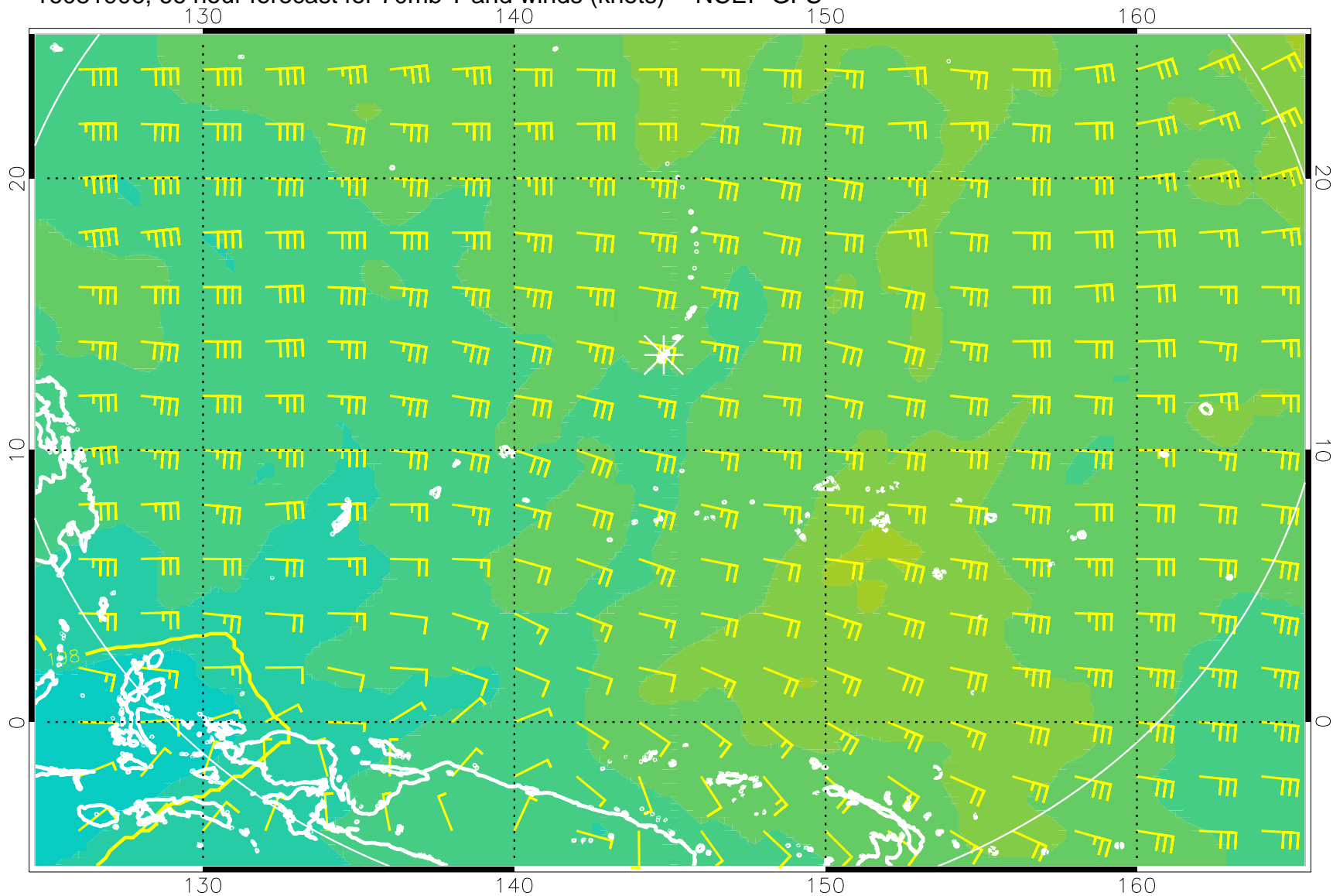
16081906, 66 hour forecast for 70mb T and winds (knots) -- NCEP GFS
