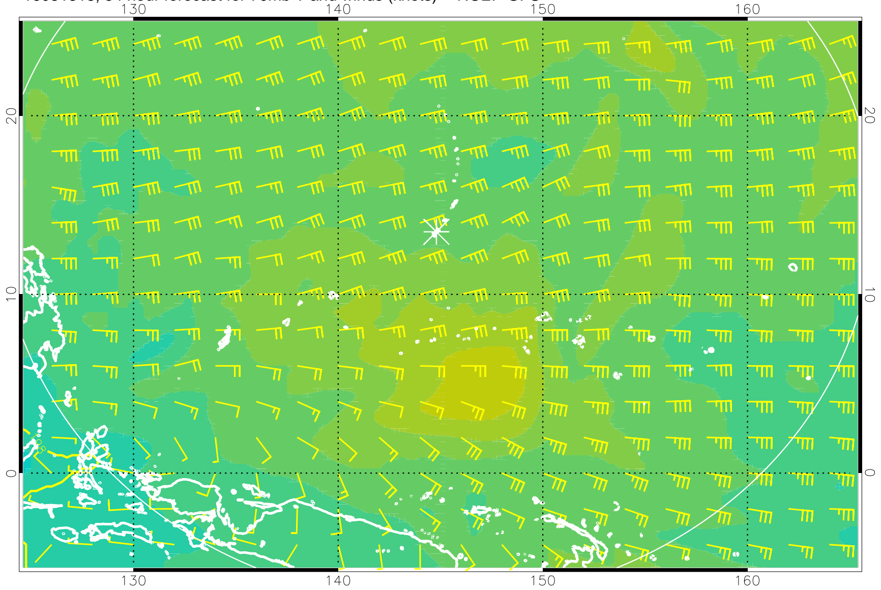
16081818, 54 hour forecast for 70mb T and winds (knots) -- NCEP GFS
