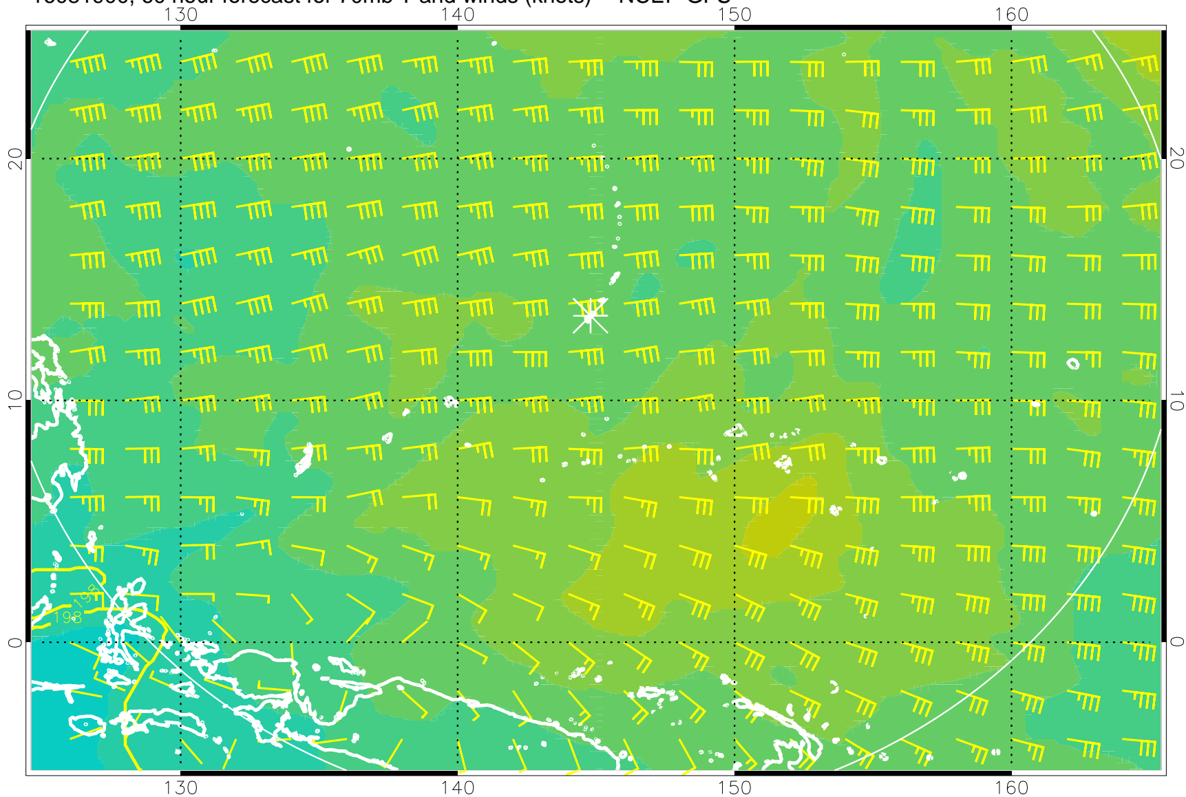
16081900, 60 hour forecast for 70mb T and winds (knots) -- NCEP GFS
