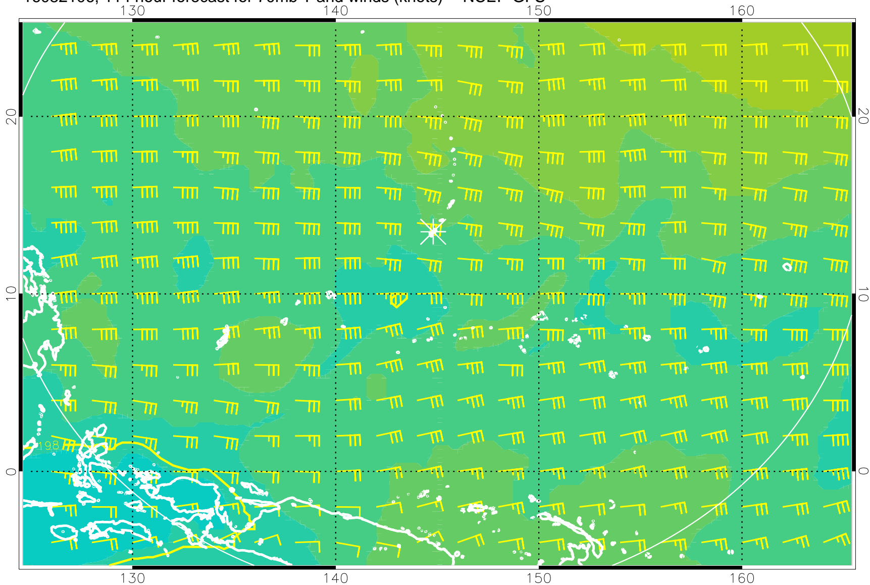
16082106, 114 hour forecast for 70mb T and winds (knots) -- NCEP GFS
