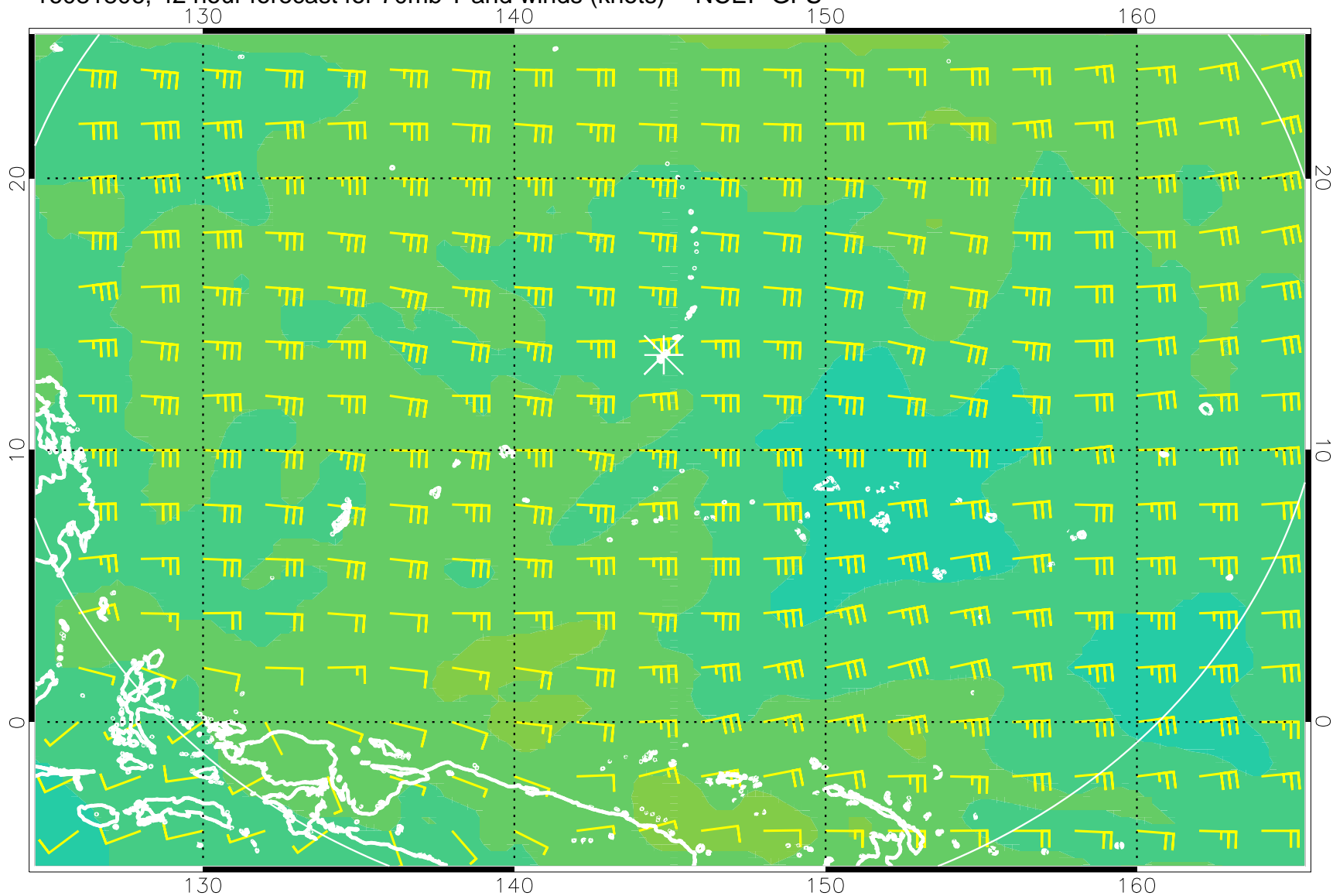
16081806, 42 hour forecast for 70mb T and winds (knots) -- NCEP GFS
