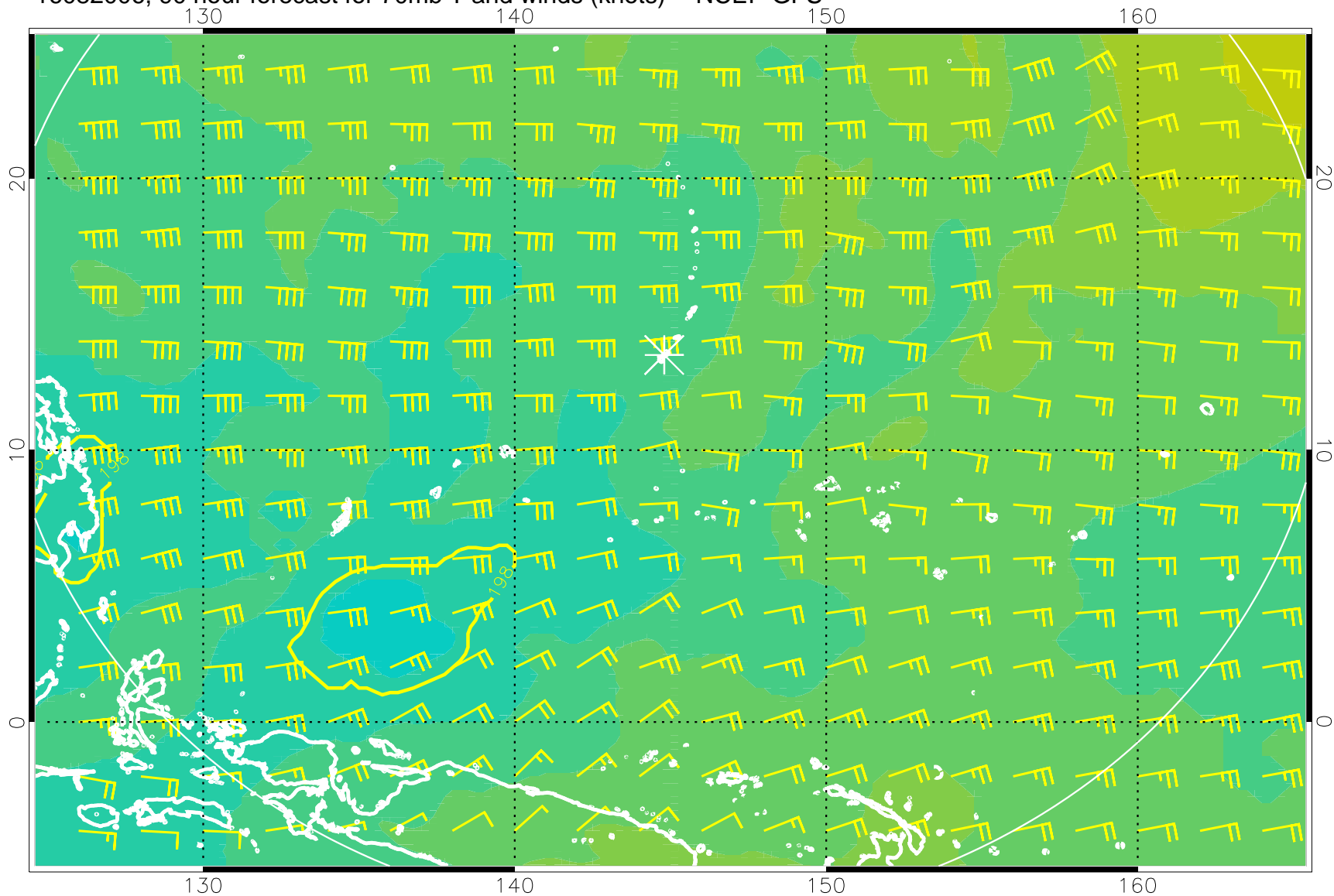
16082006, 90 hour forecast for 70mb T and winds (knots) -- NCEP GFS
