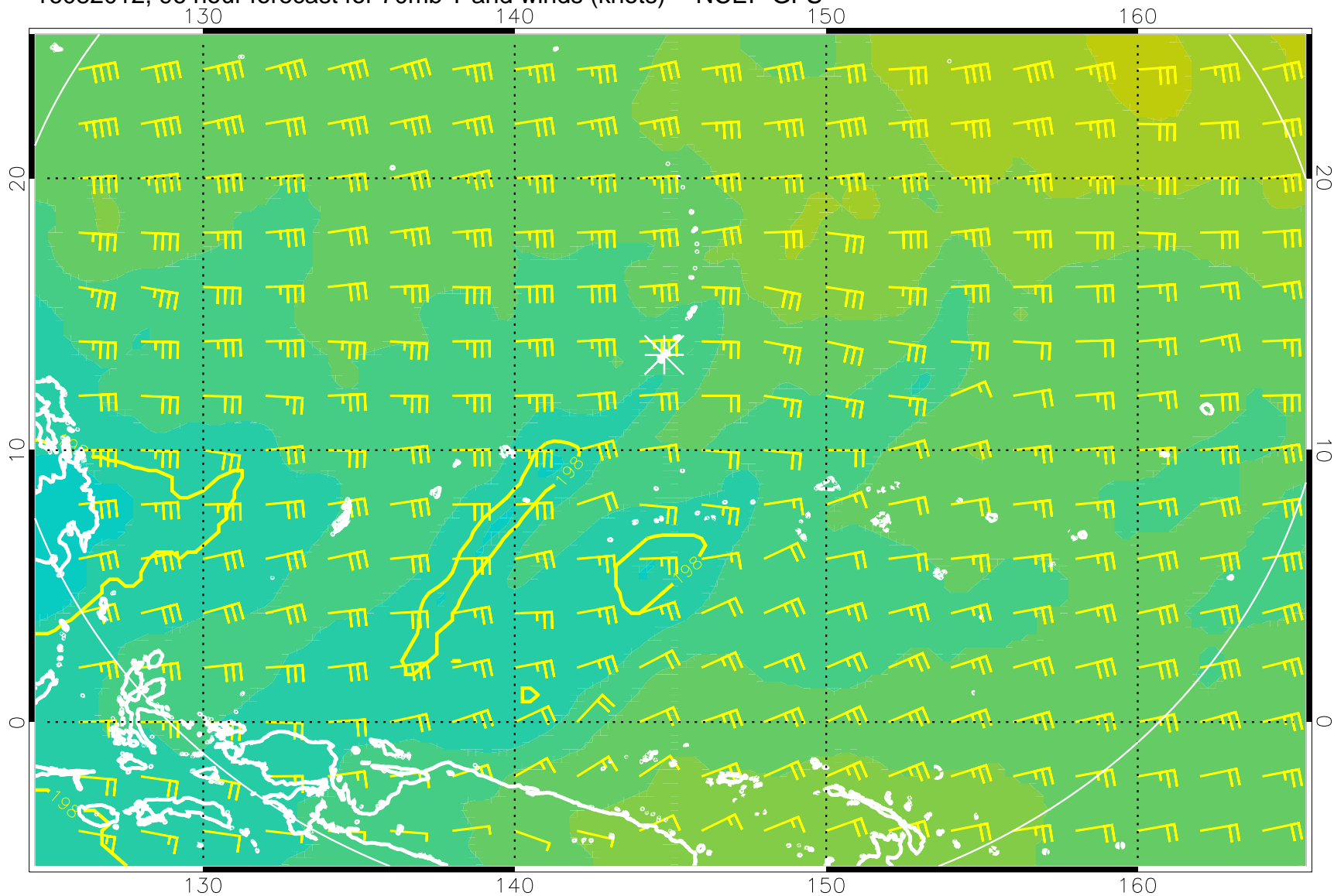
16082012, 96 hour forecast for 70mb T and winds (knots) -- NCEP GFS
