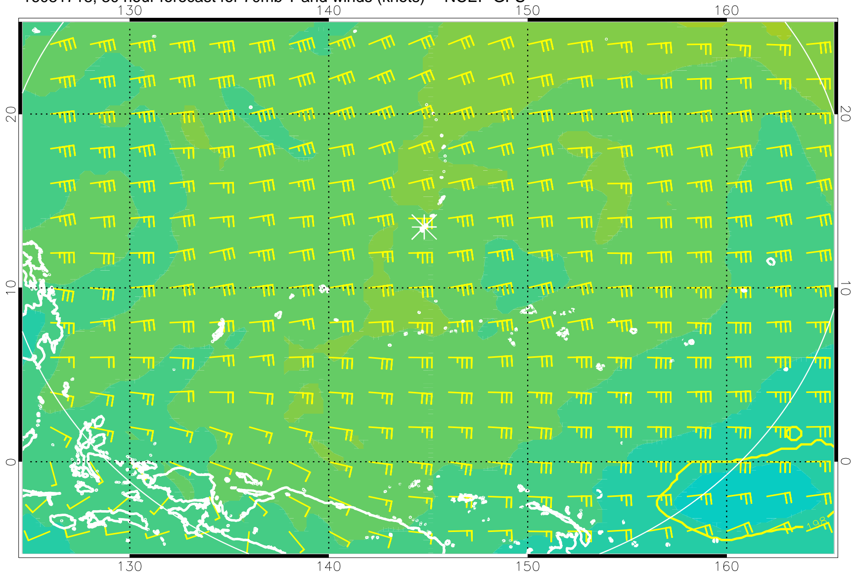
16081718, 30 hour forecast for 70mb T and winds (knots) -- NCEP GFS
