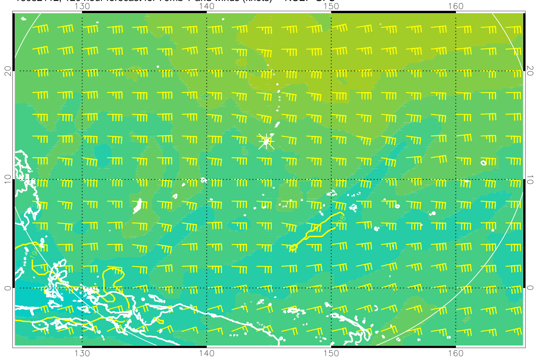
16082112, 120 hour forecast for 70mb T and winds (knots) -- NCEP GFS
