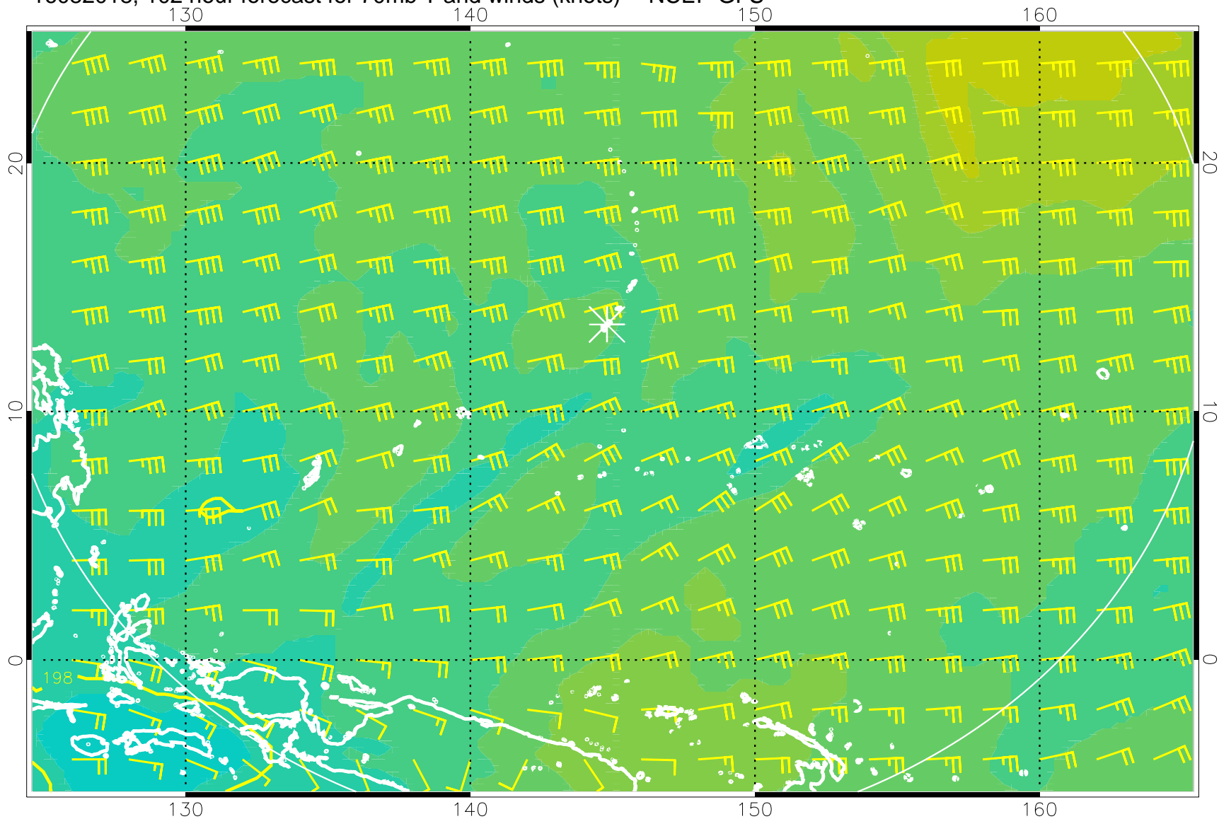
16082018, 102 hour forecast for 70mb T and winds (knots) -- NCEP GFS
