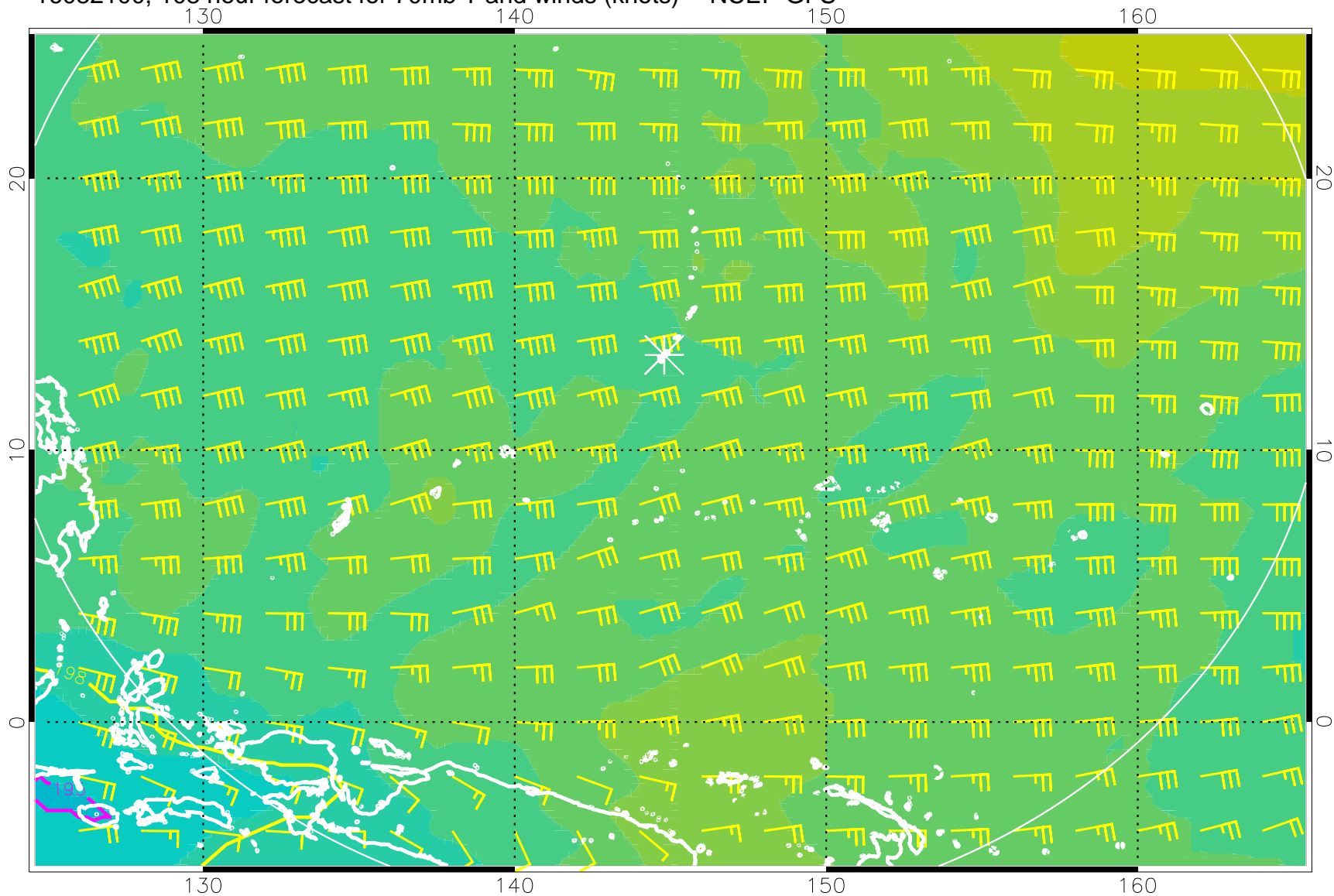
16082100, 108 hour forecast for 70mb T and winds (knots) -- NCEP GFS
