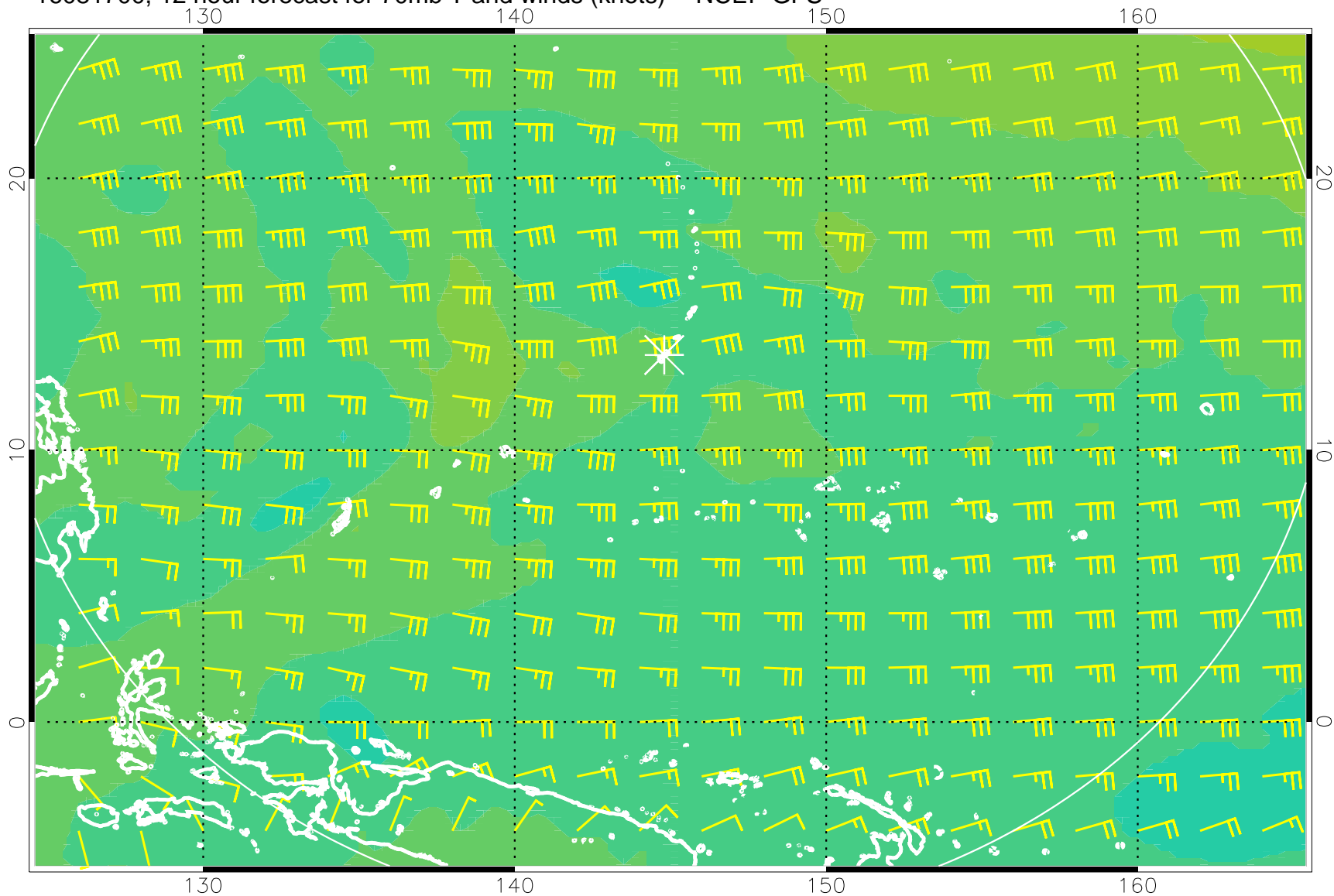
16081700, 12 hour forecast for 70mb T and winds (knots) -- NCEP GFS
