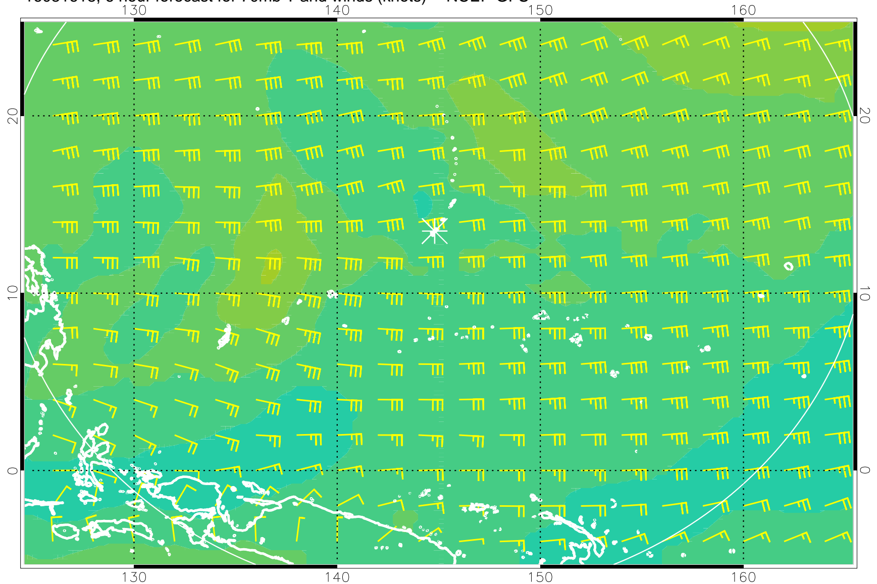
16081618, 6 hour forecast for 70mb T and winds (knots) -- NCEP GFS
