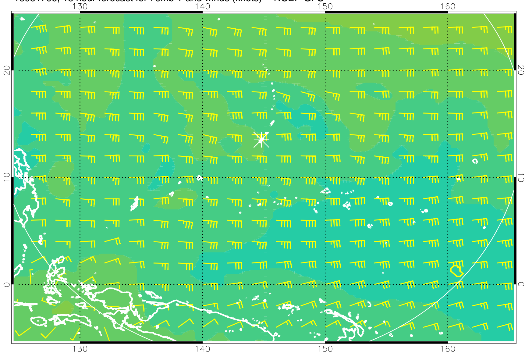
16081706, 18 hour forecast for 70mb T and winds (knots) -- NCEP GFS
