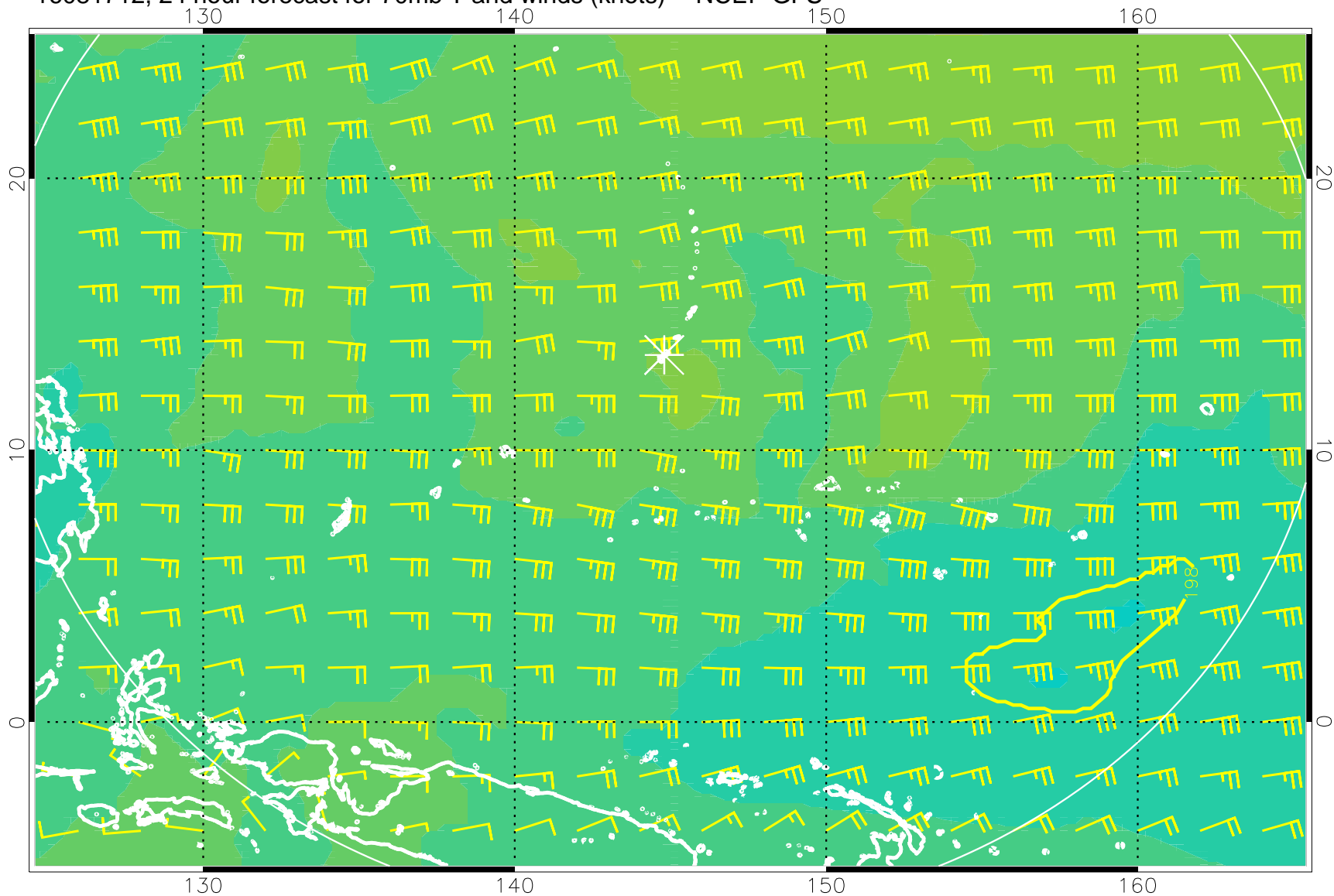
16081712, 24 hour forecast for 70mb T and winds (knots) -- NCEP GFS
