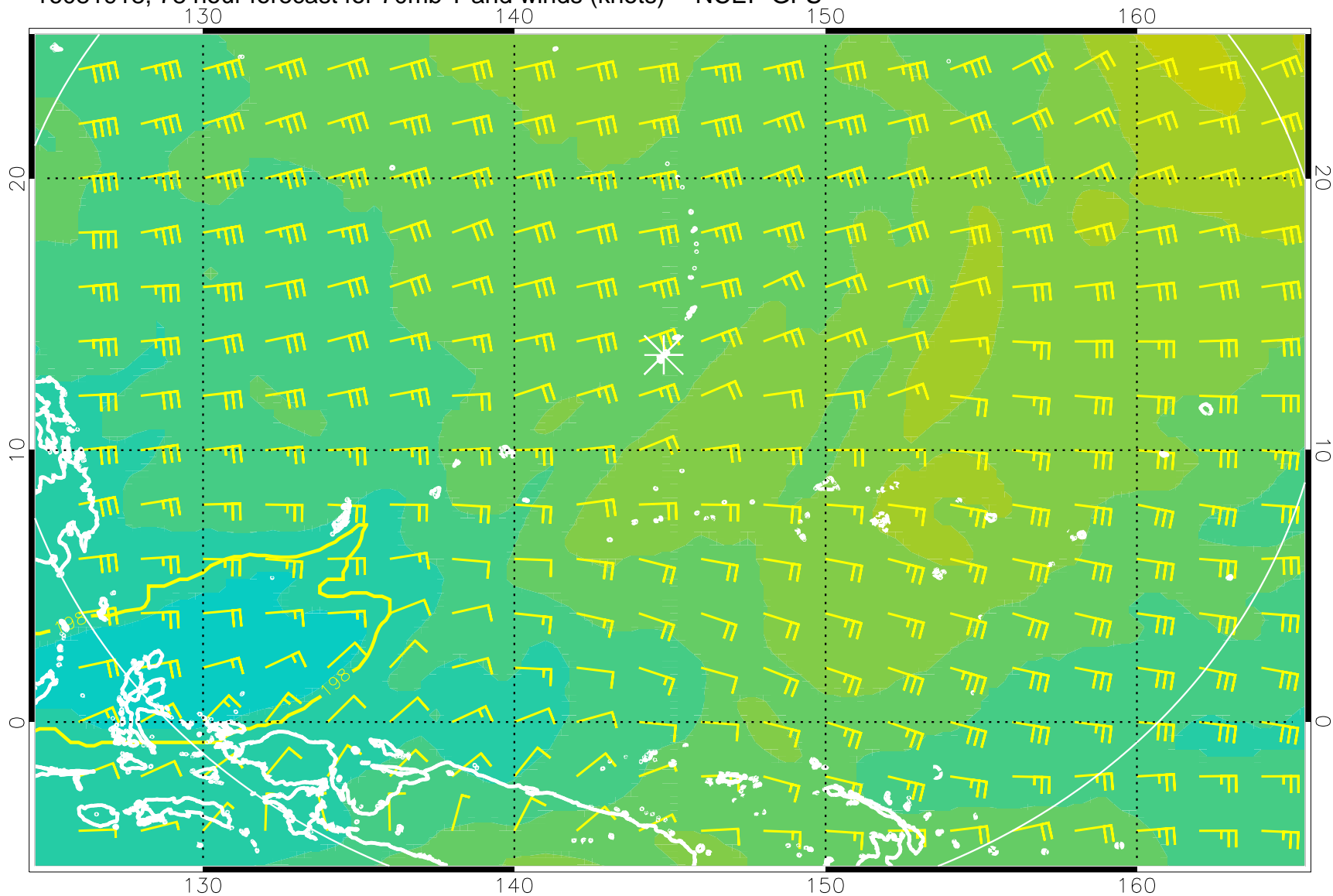
16081918, 78 hour forecast for 70mb T and winds (knots) -- NCEP GFS
