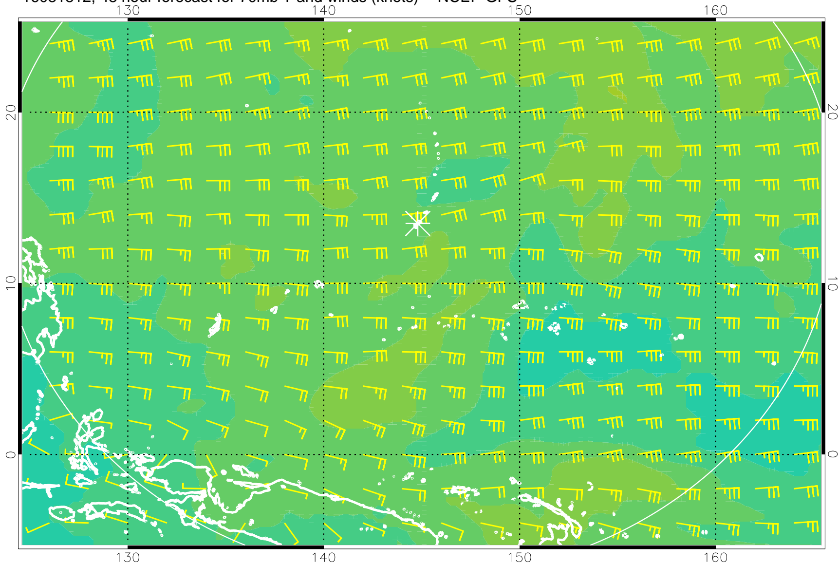
16081812, 48 hour forecast for 70mb T and winds (knots) -- NCEP GFS
