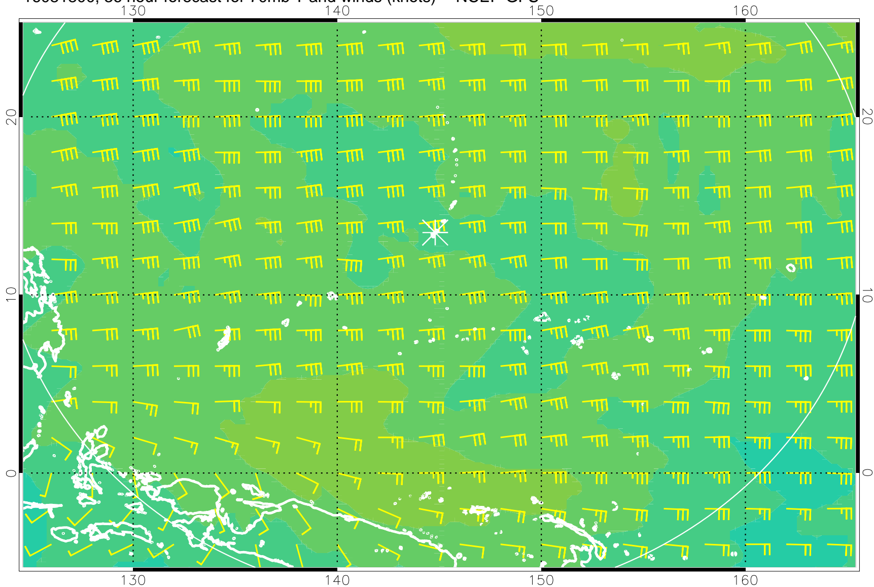
16081800, 36 hour forecast for 70mb T and winds (knots) -- NCEP GFS
