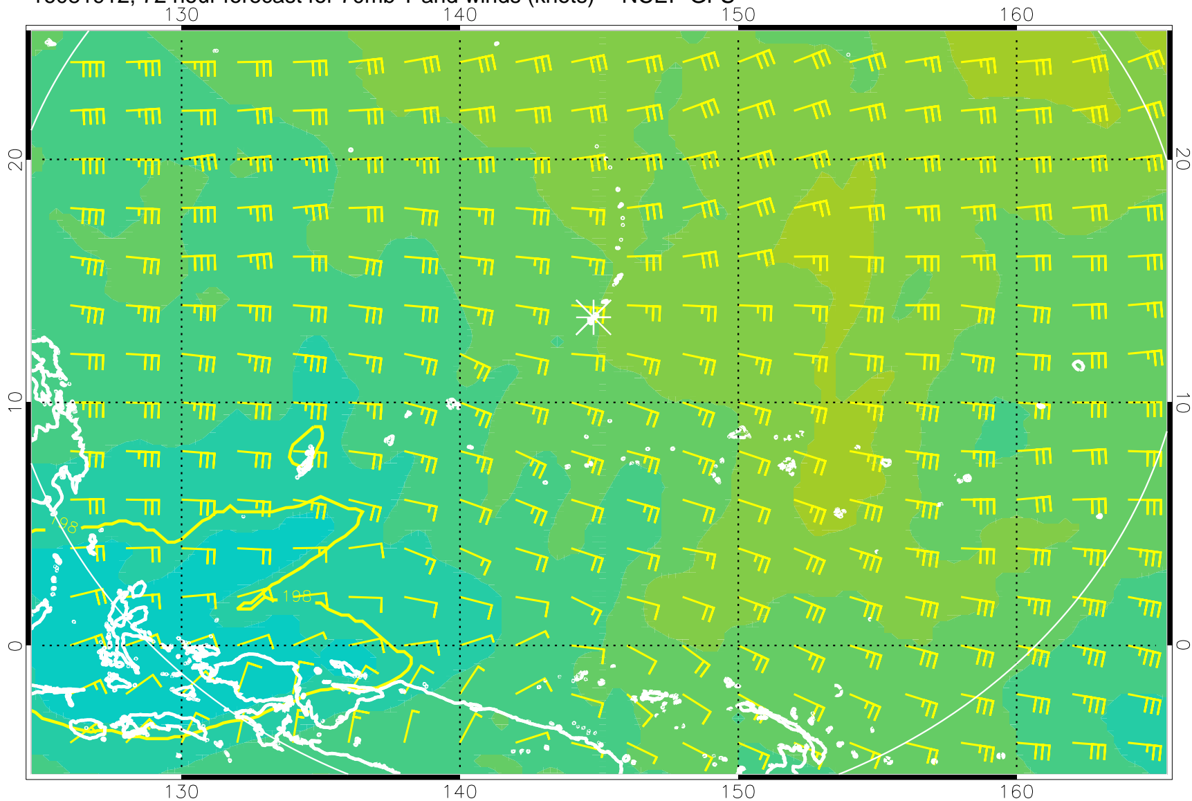
16081912, 72 hour forecast for 70mb T and winds (knots) -- NCEP GFS
