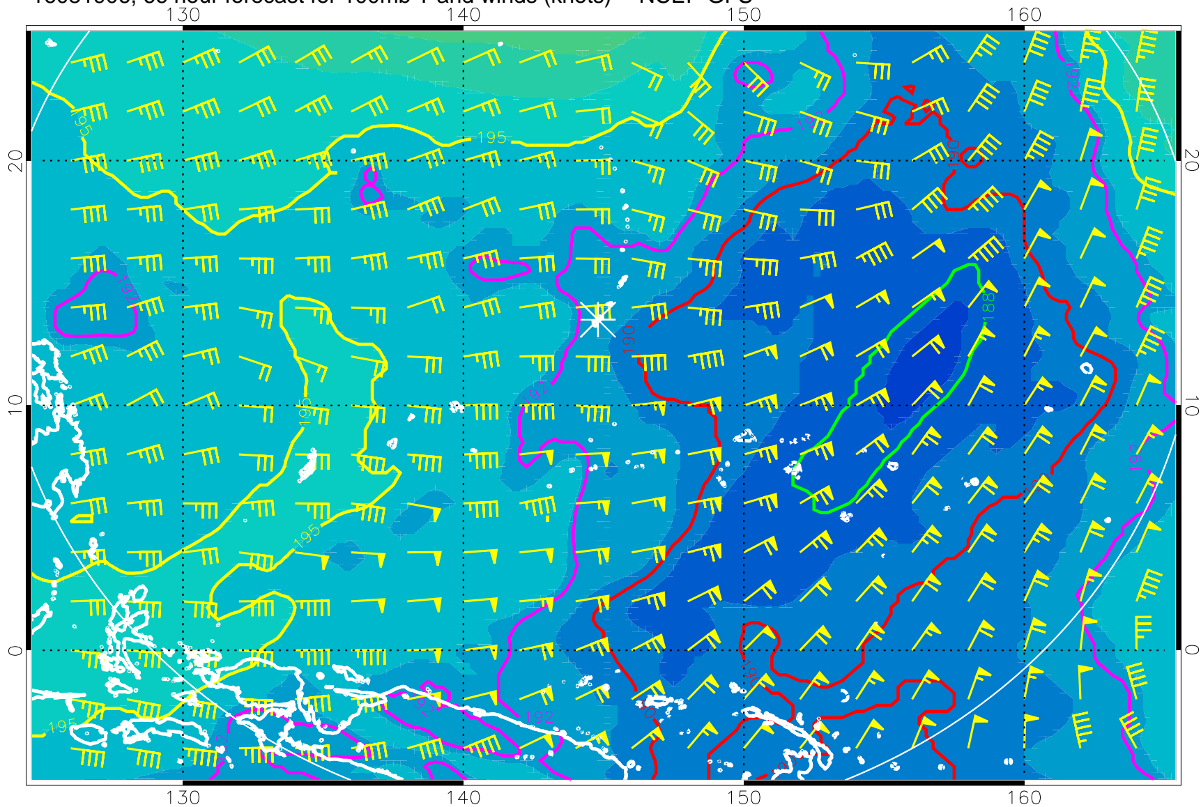
16081906, 66 hour forecast for 100mb T and winds (knots) -- NCEP GFS
