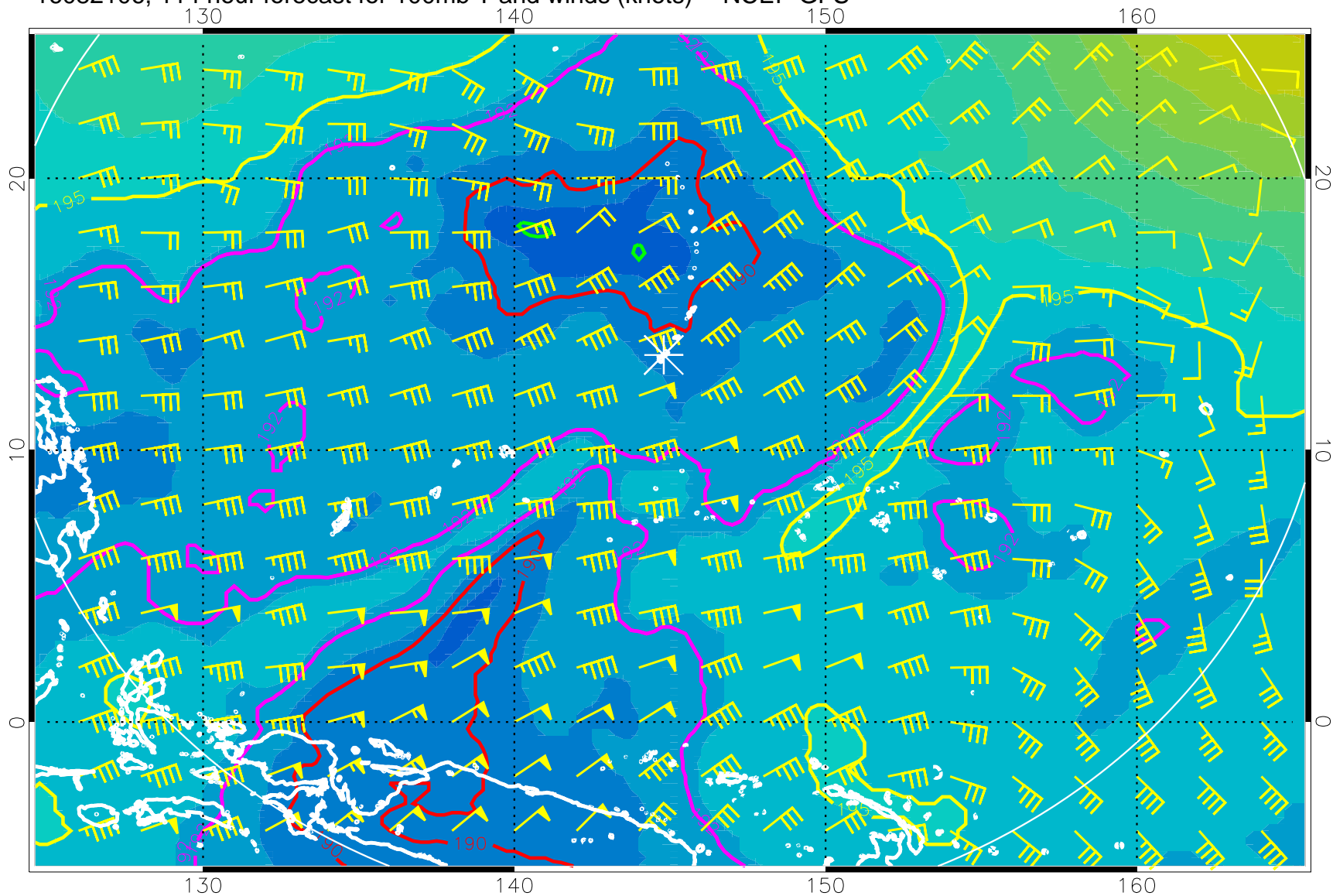
16082106, 114 hour forecast for 100mb T and winds (knots) -- NCEP GFS
