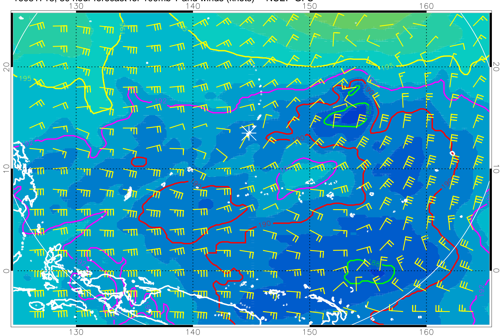
16081718, 30 hour forecast for 100mb T and winds (knots) -- NCEP GFS
