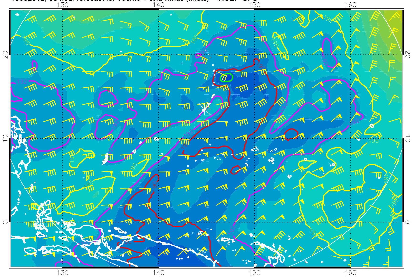
16082012, 96 hour forecast for 100mb T and winds (knots) -- NCEP GFS
