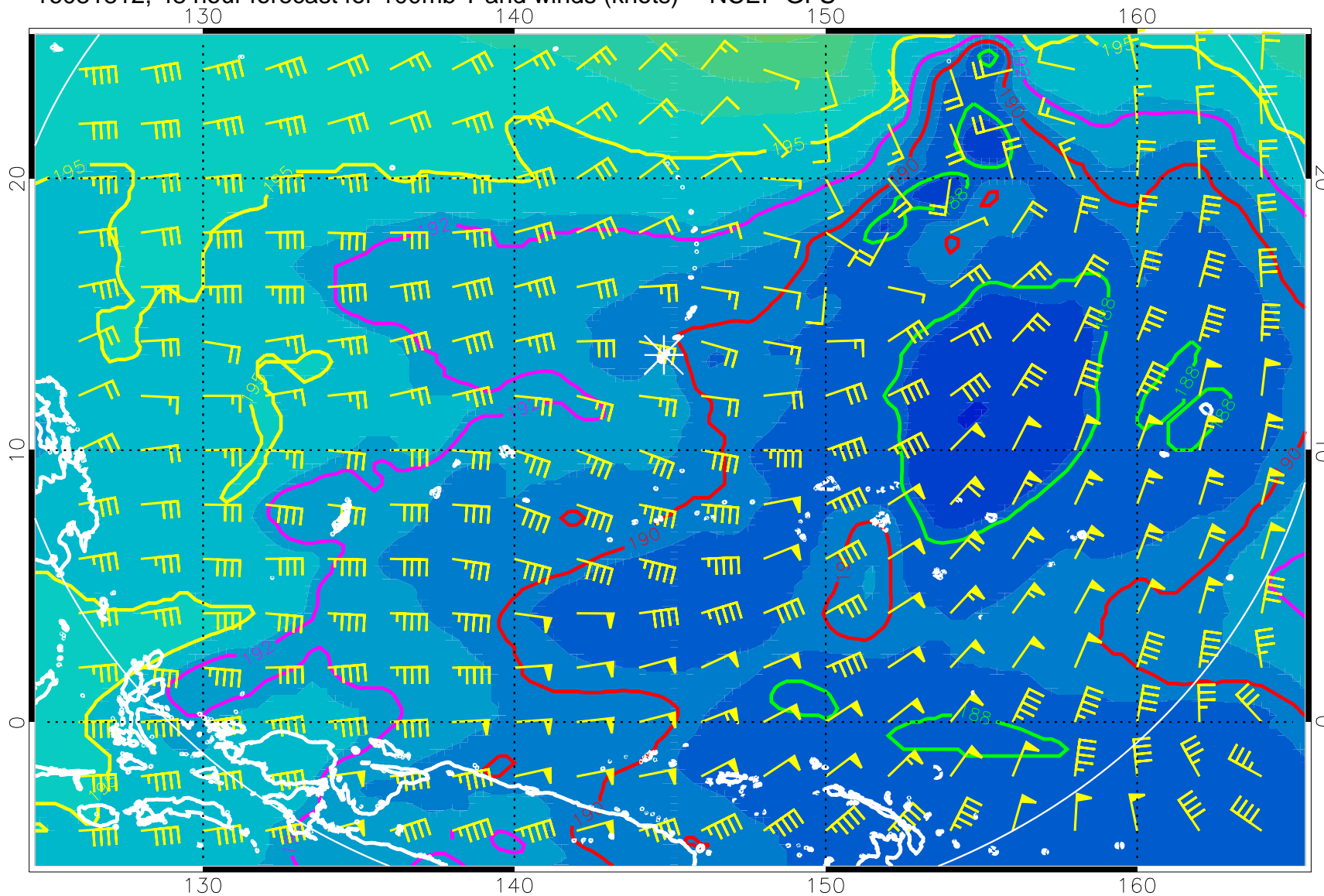
16081812, 48 hour forecast for 100mb T and winds (knots) -- NCEP GFS
