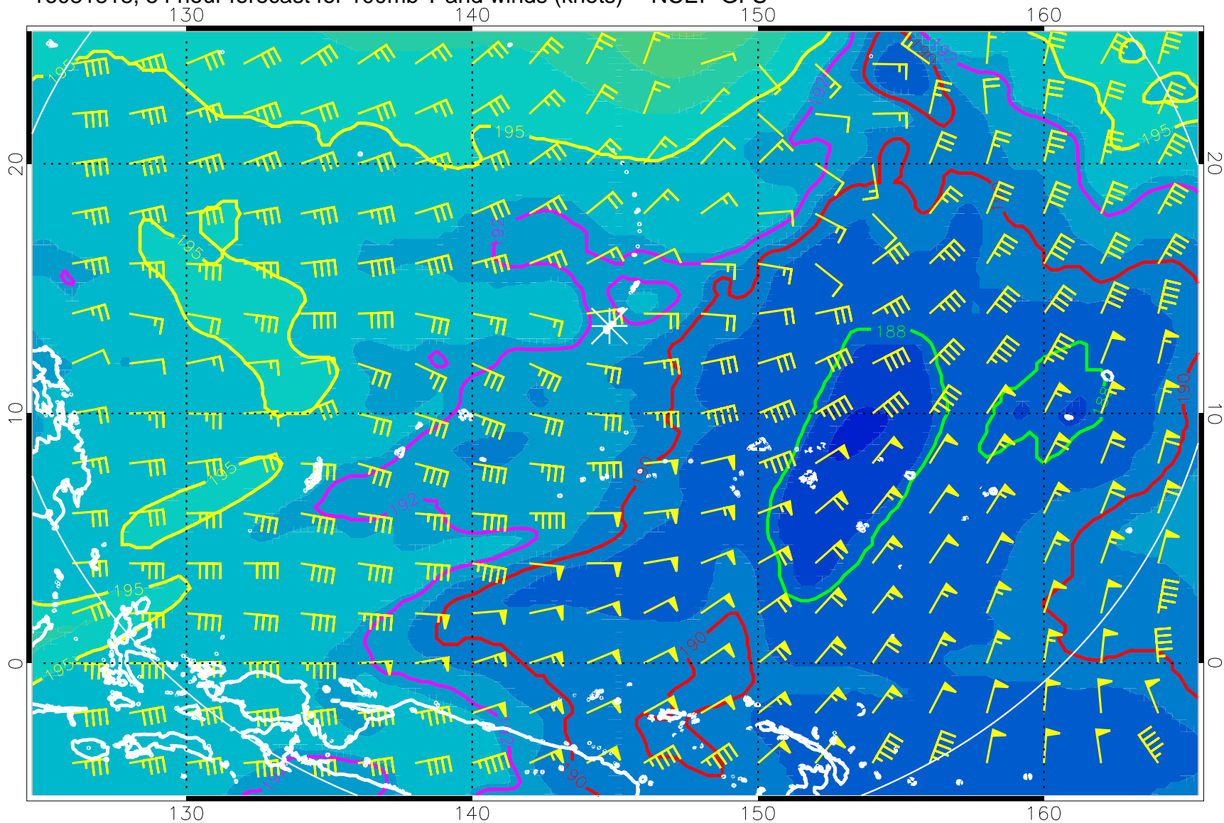
16081818, 54 hour forecast for 100mb T and winds (knots) -- NCEP GFS
