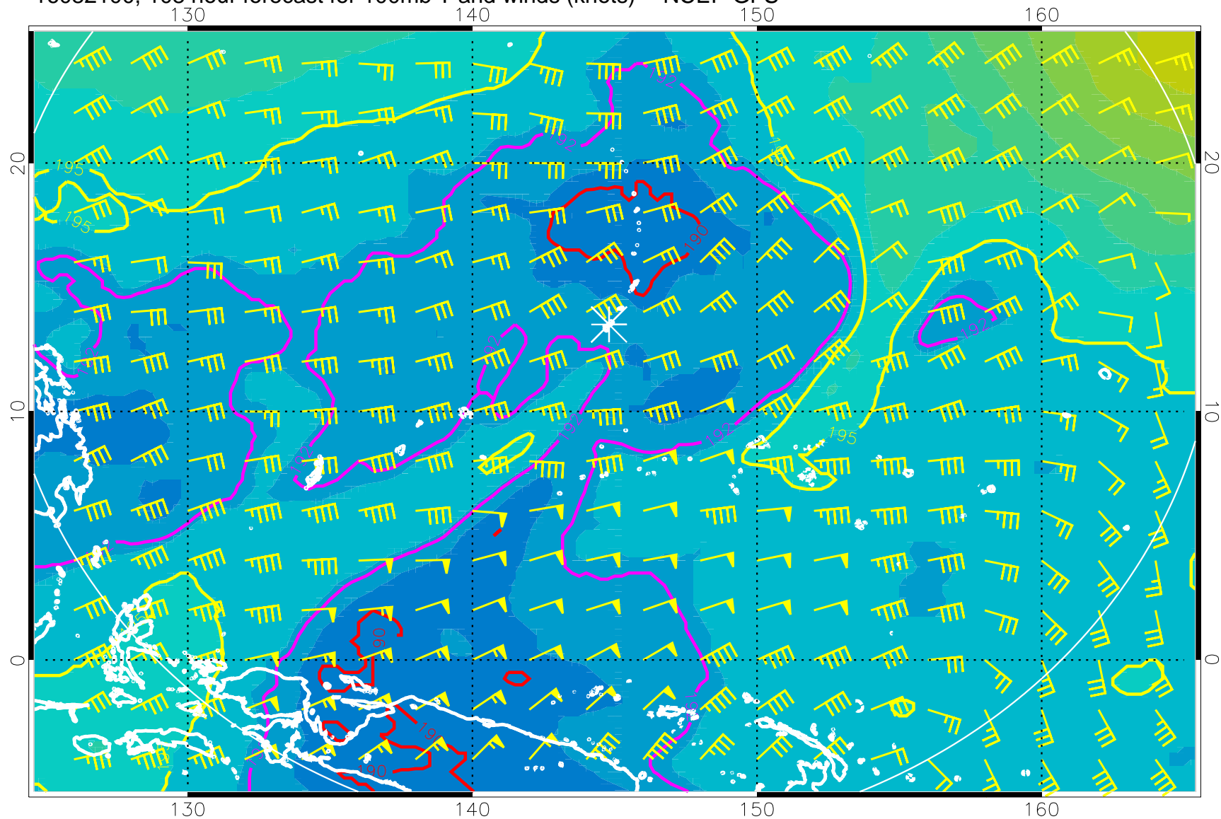
16082100, 108 hour forecast for 100mb T and winds (knots) -- NCEP GFS
