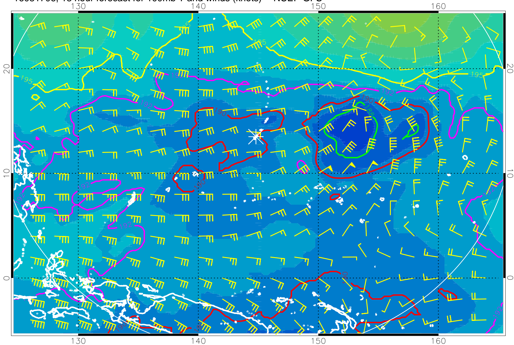
16081706, 18 hour forecast for 100mb T and winds (knots) -- NCEP GFS
