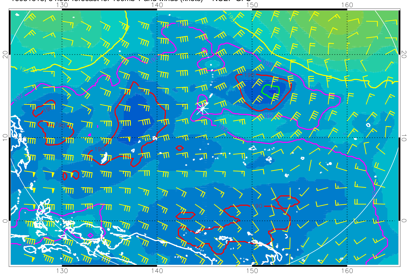
16081618, 6 hour forecast for 100mb T and winds (knots) -- NCEP GFS
