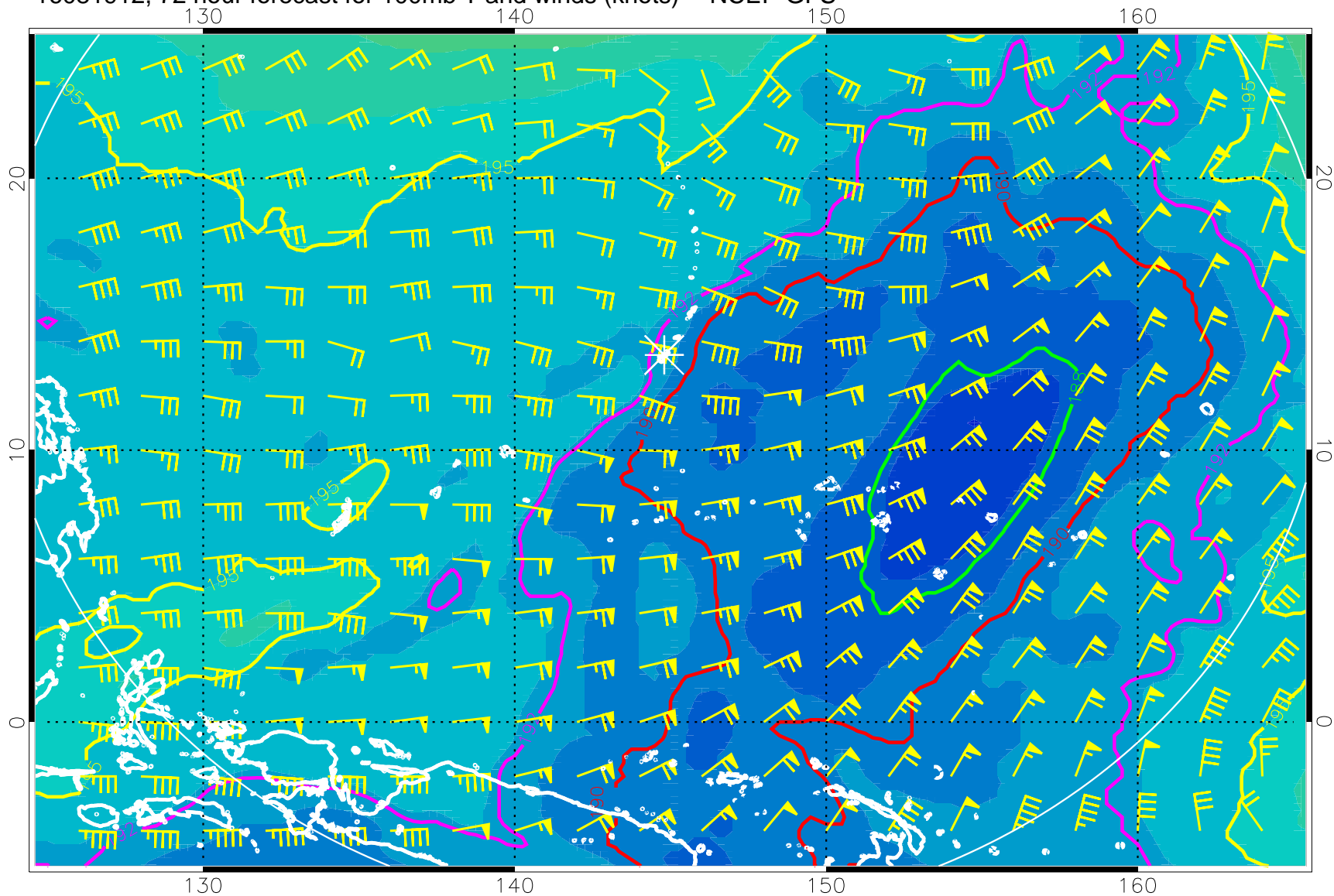
16081912, 72 hour forecast for 100mb T and winds (knots) -- NCEP GFS
