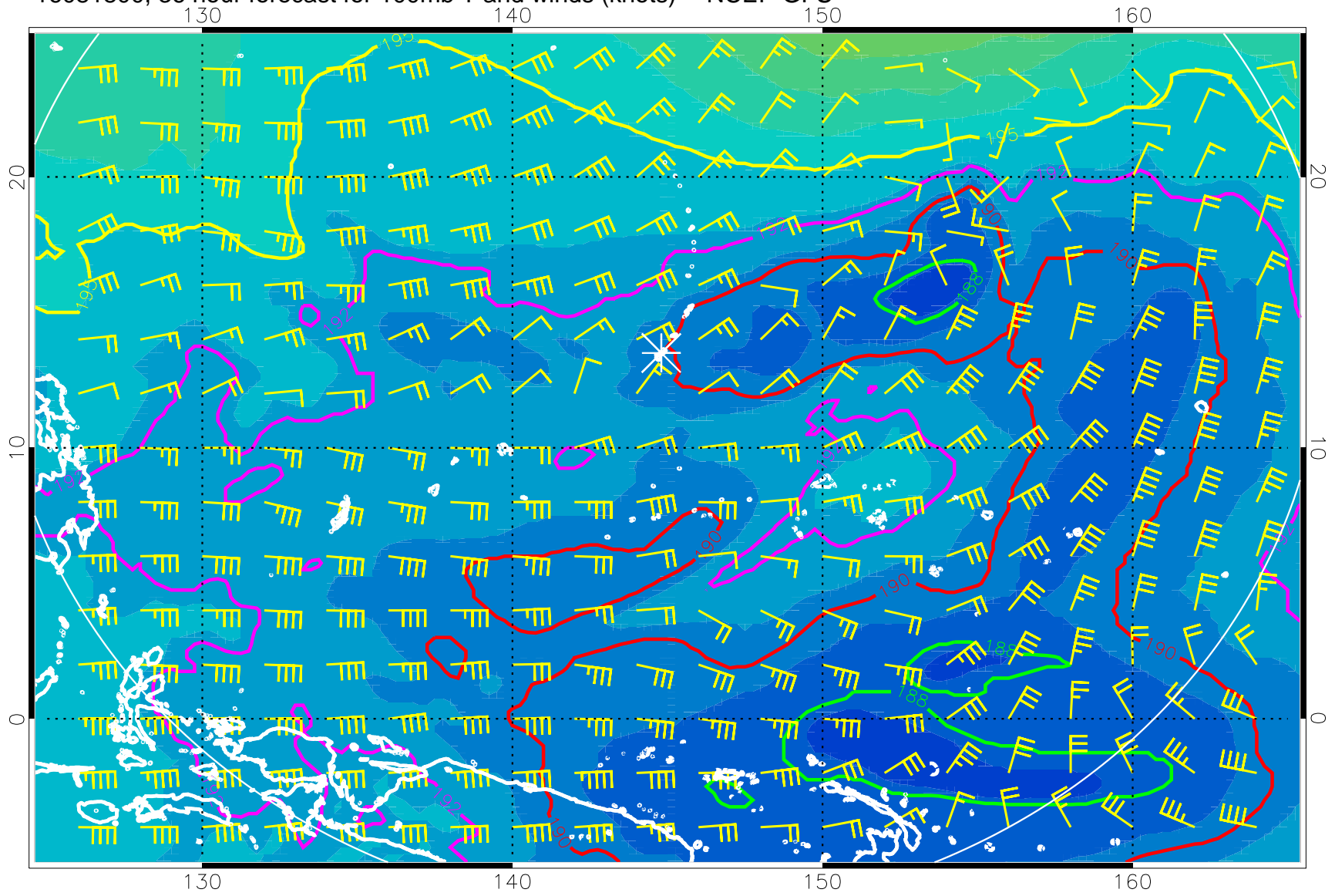
16081800, 36 hour forecast for 100mb T and winds (knots) -- NCEP GFS
