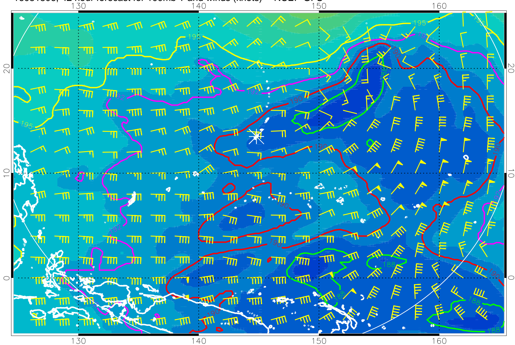
16081806, 42 hour forecast for 100mb T and winds (knots) -- NCEP GFS
