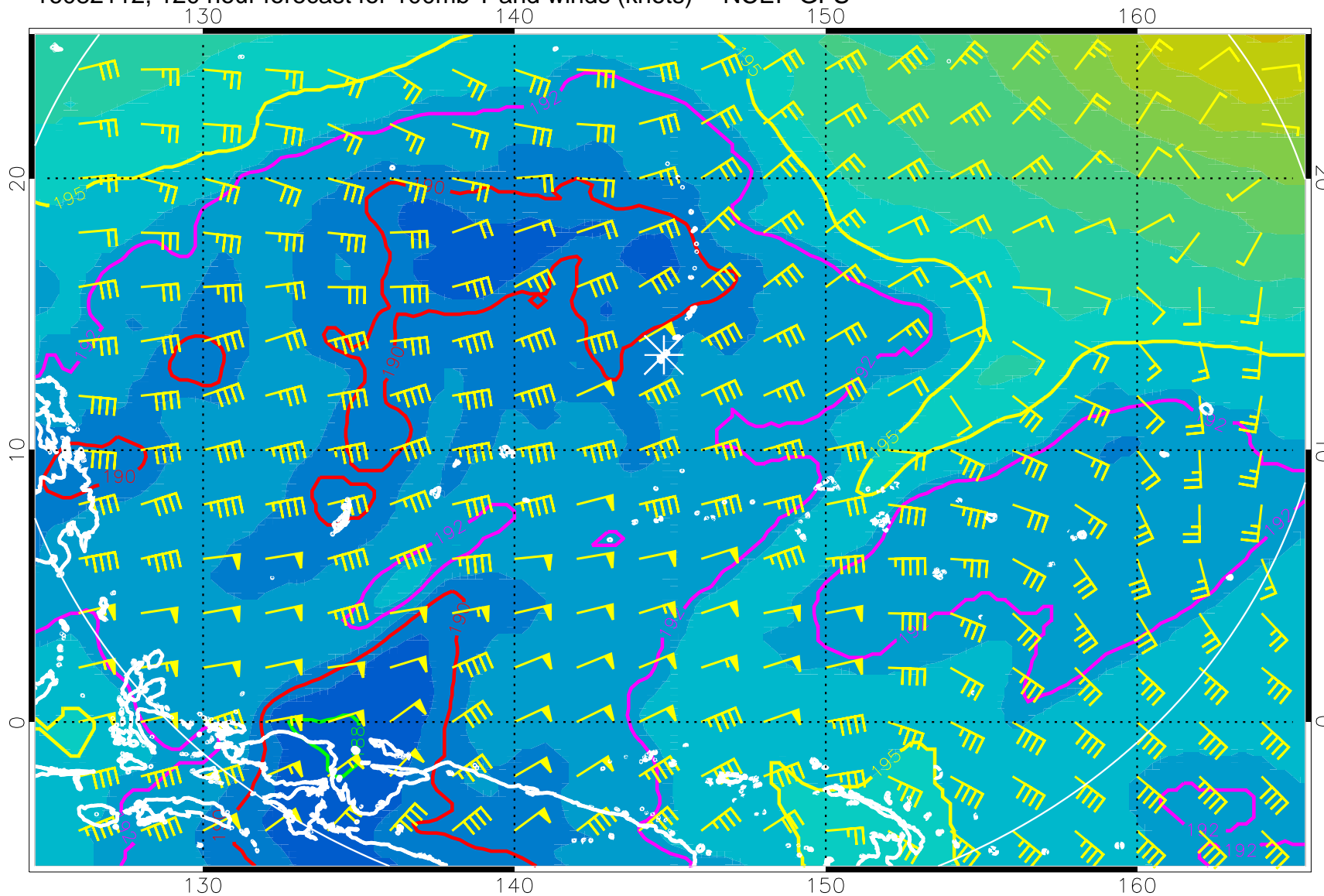
16082112, 120 hour forecast for 100mb T and winds (knots) -- NCEP GFS
