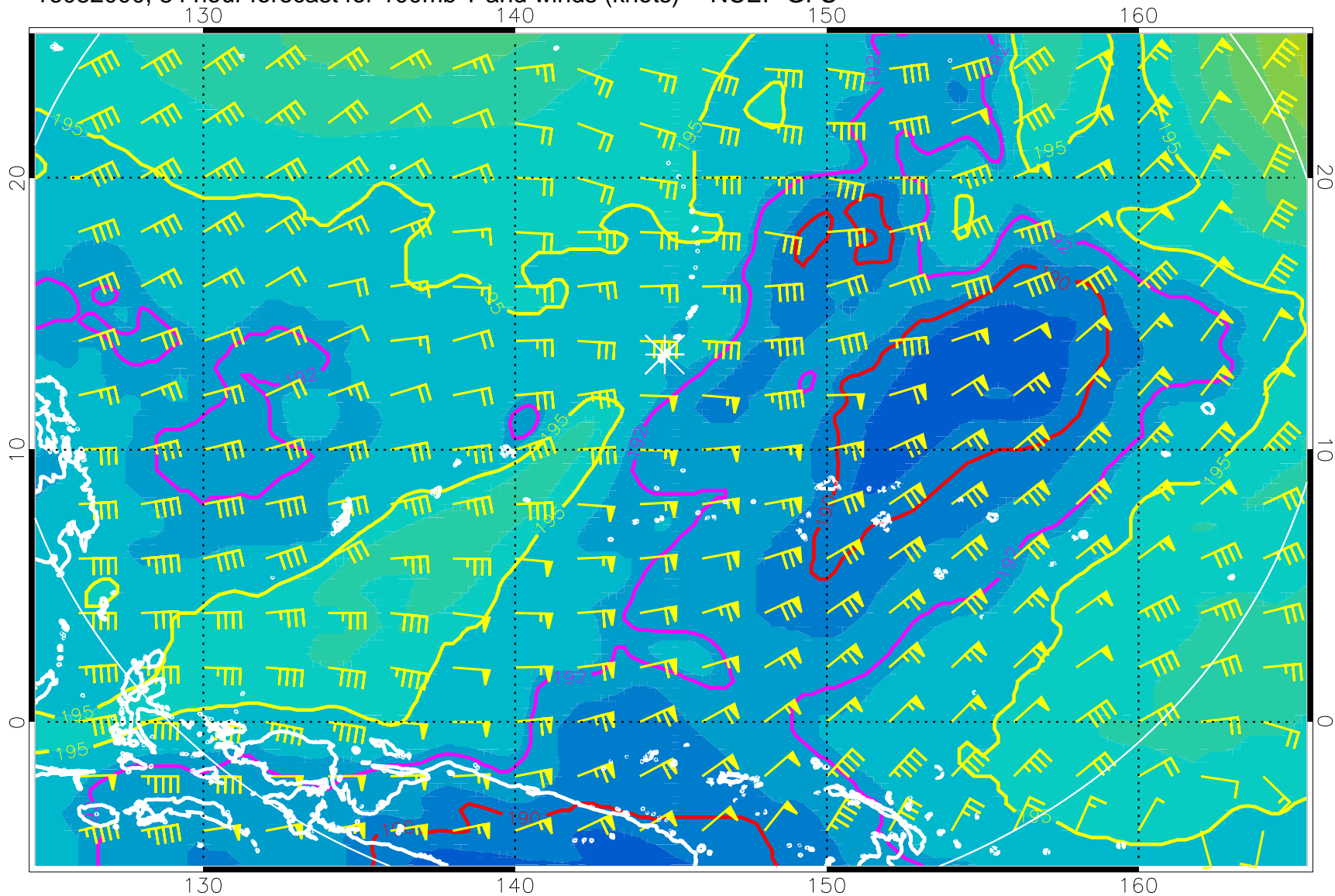
16082000, 84 hour forecast for 100mb T and winds (knots) -- NCEP GFS
