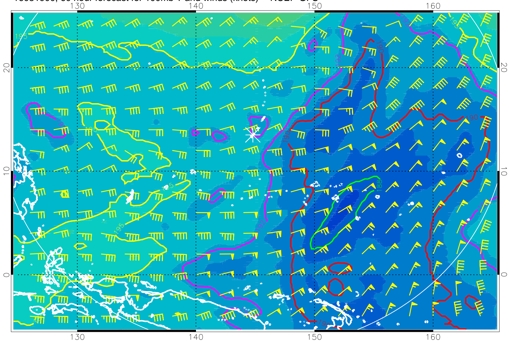
16081900, 60 hour forecast for 100mb T and winds (knots) -- NCEP GFS
