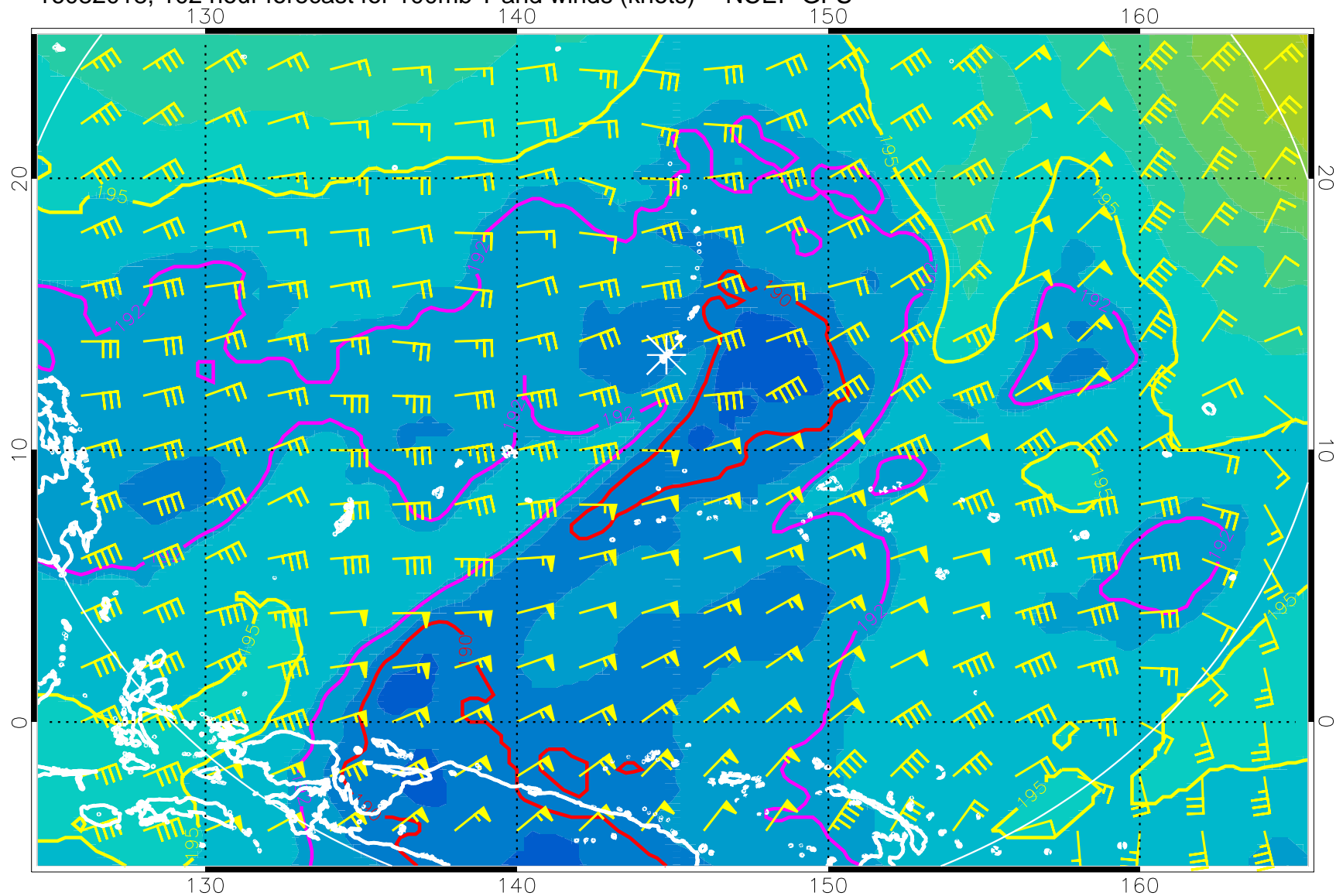
16082018, 102 hour forecast for 100mb T and winds (knots) -- NCEP GFS
