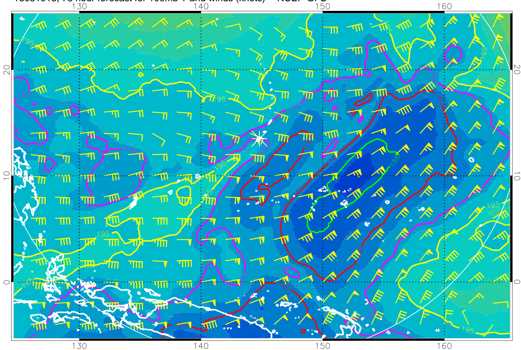
16081918, 78 hour forecast for 100mb T and winds (knots) -- NCEP GFS
