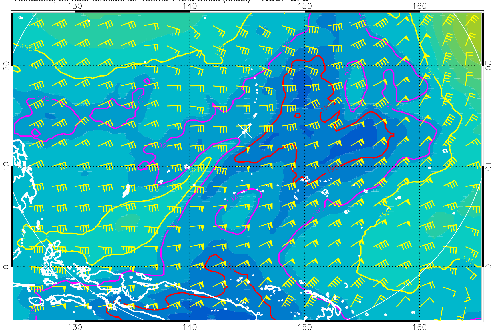
16082006, 90 hour forecast for 100mb T and winds (knots) -- NCEP GFS
