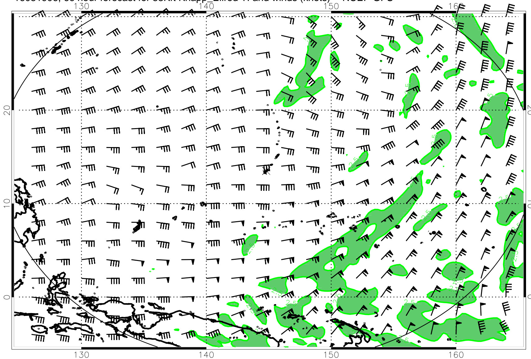
16081906, 66 hour forecast for 53Kft Knapp_Ellrod TI and winds (knots) -- NCEP GFS
