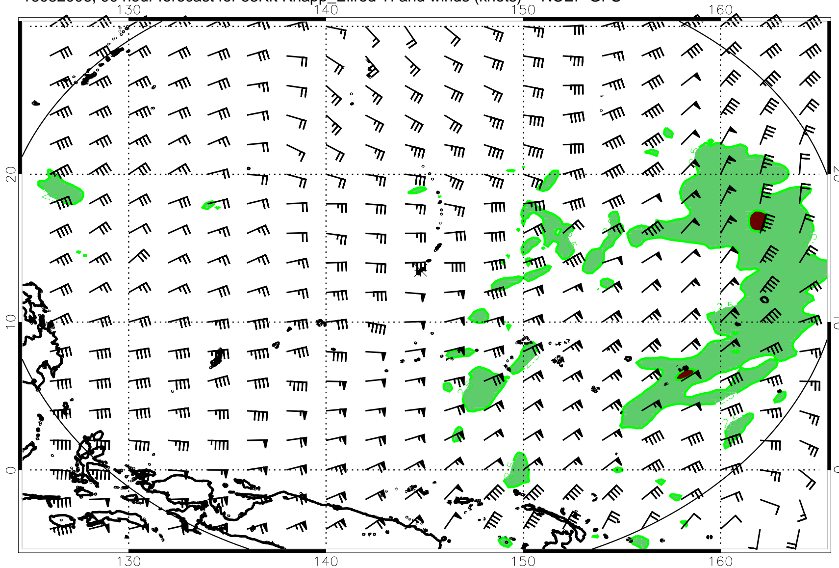
16082006, 90 hour forecast for 53Kft Knapp_Ellrod TI and winds (knots) -- NCEP GFS
