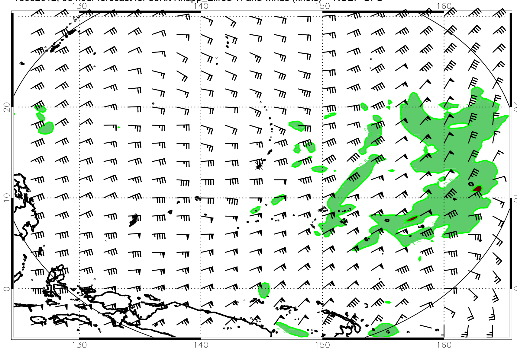
16082012, 96 hour forecast for 53Kft Knapp_Ellrod TI and winds (knots) -- NCEP GFS
