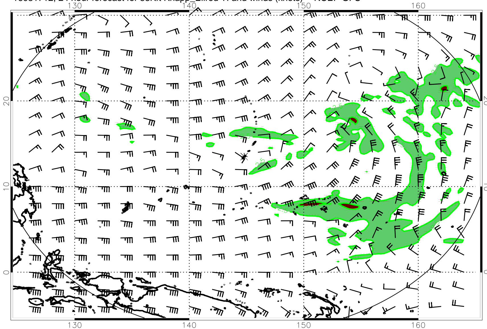
16081712, 24 hour forecast for 53Kft Knapp_Ellrod TI and winds (knots) -- NCEP GFS
