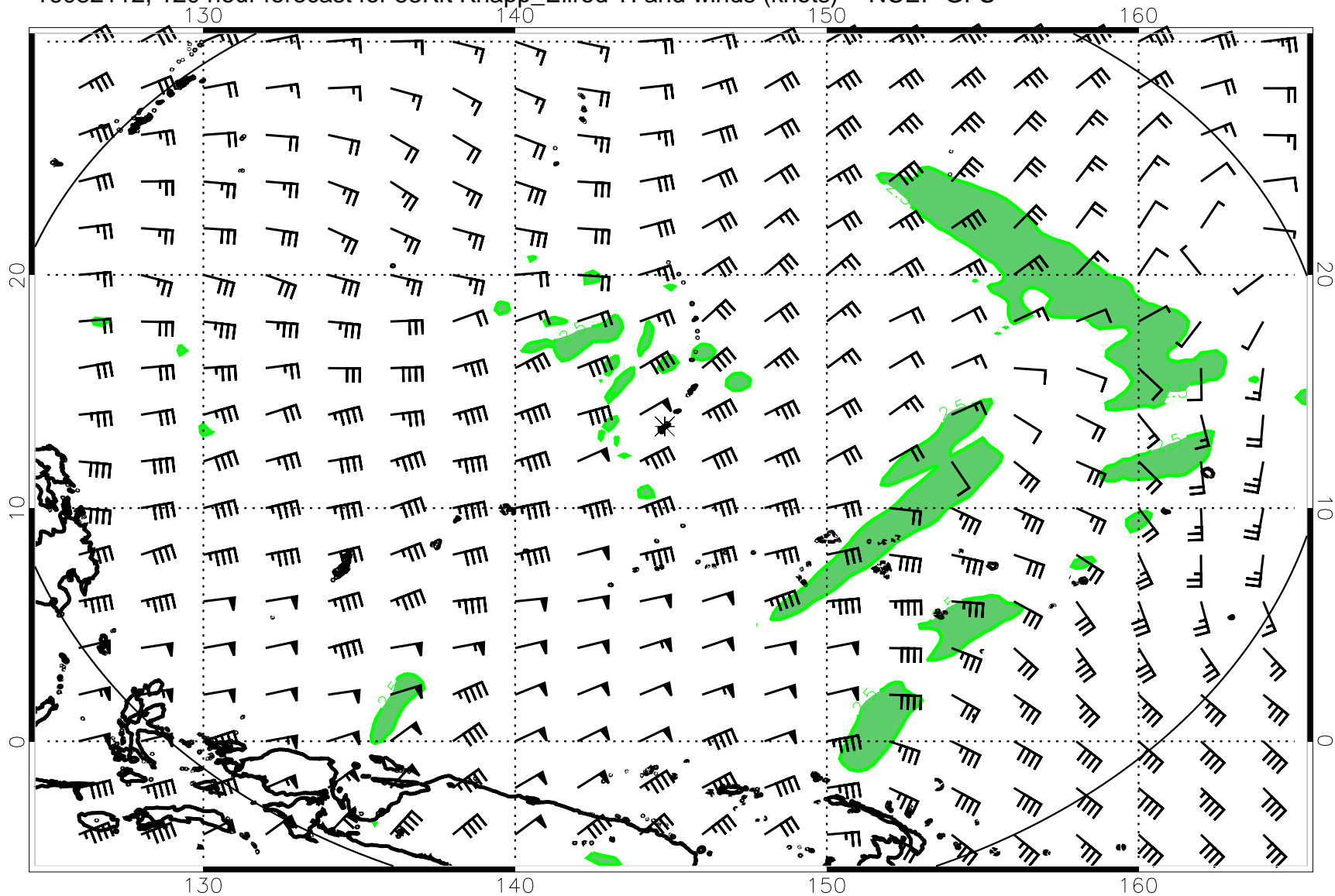
16082112, 120 hour forecast for 53Kft Knapp_Ellrod TI and winds (knots) -- NCEP GFS
