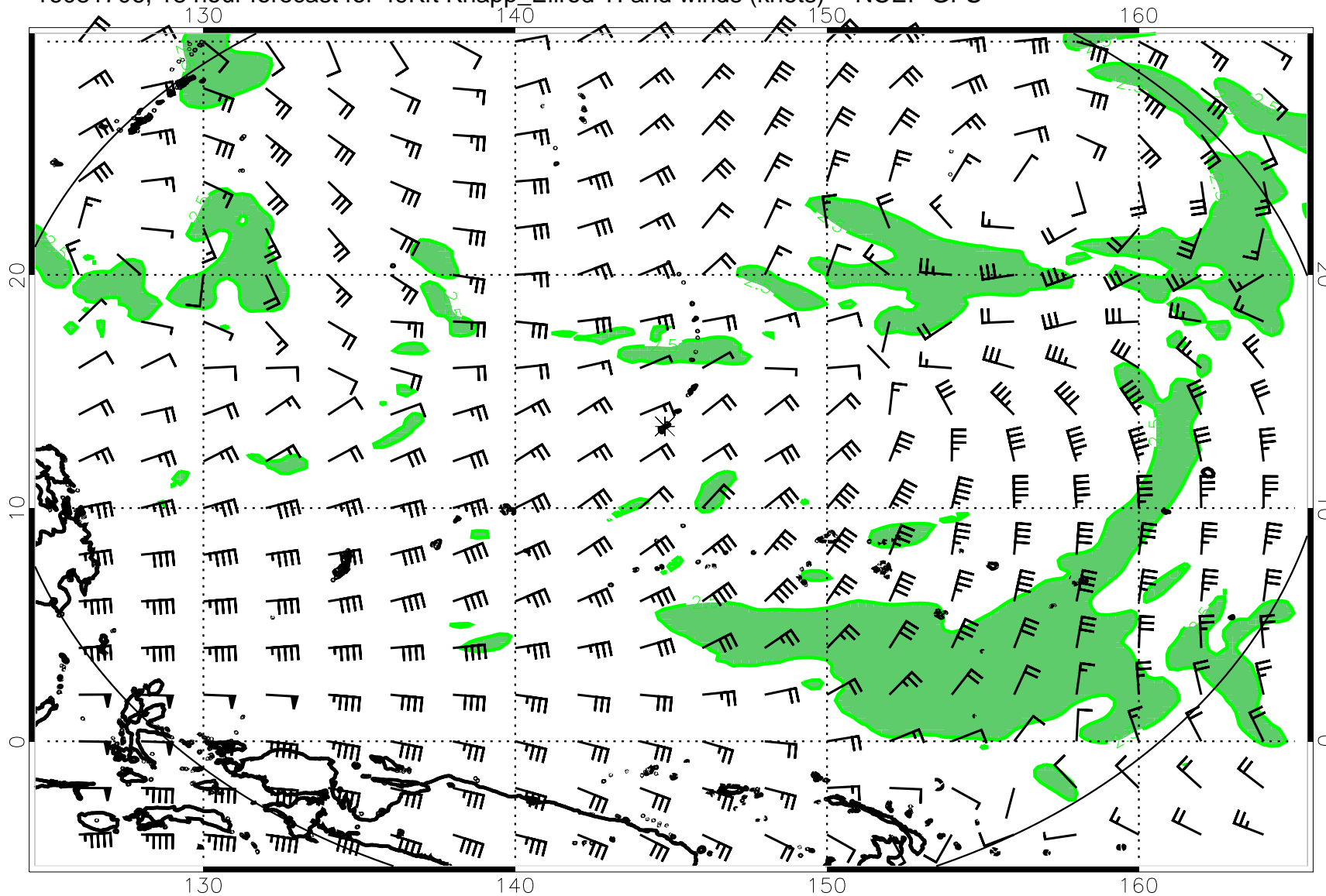
16081706, 18 hour forecast for 49Kft Knapp_Ellrod TI and winds (knots) -- NCEP GFS
