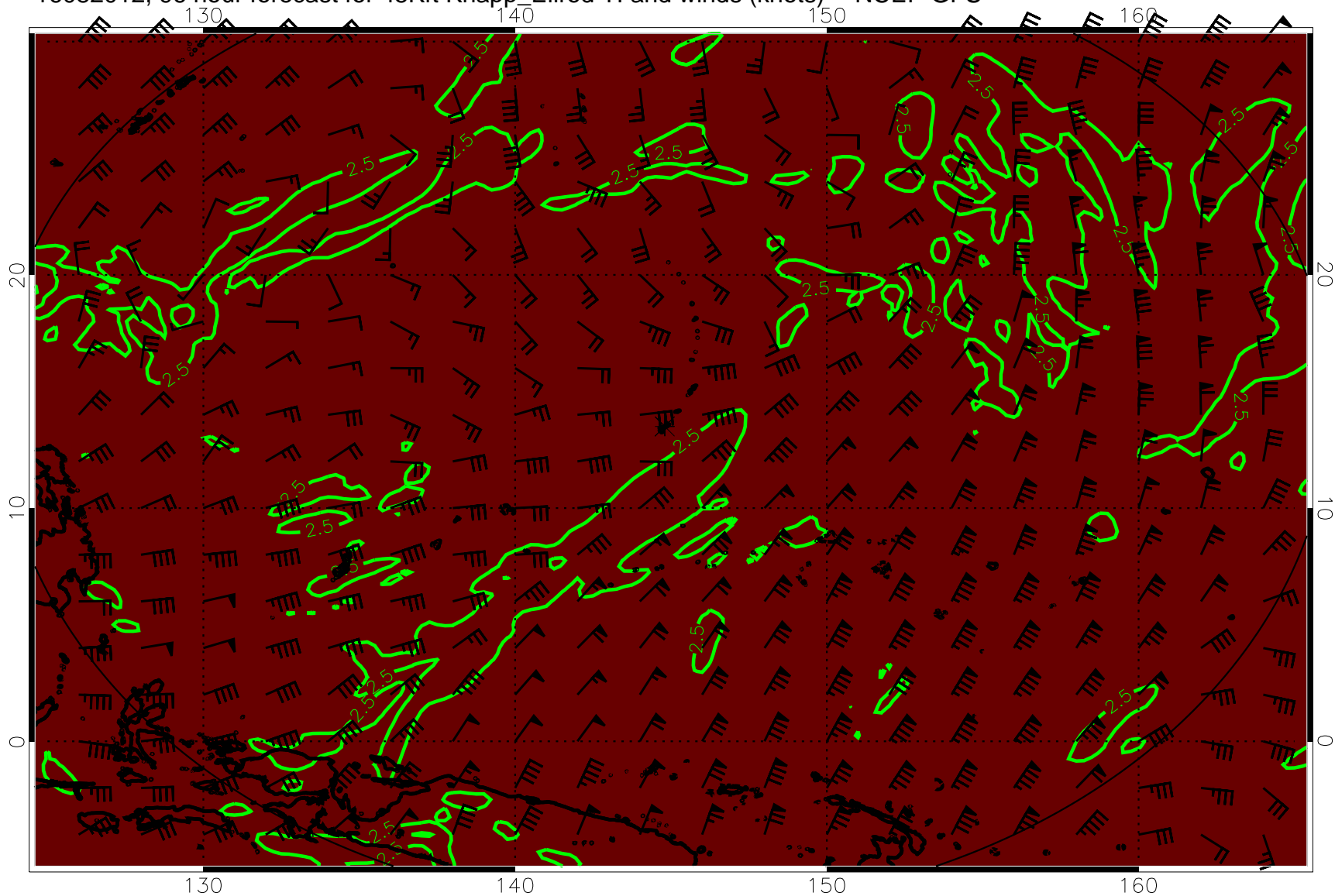
16082012, 96 hour forecast for 45Kft Knapp_Ellrod TI and winds (knots) -- NCEP GFS
