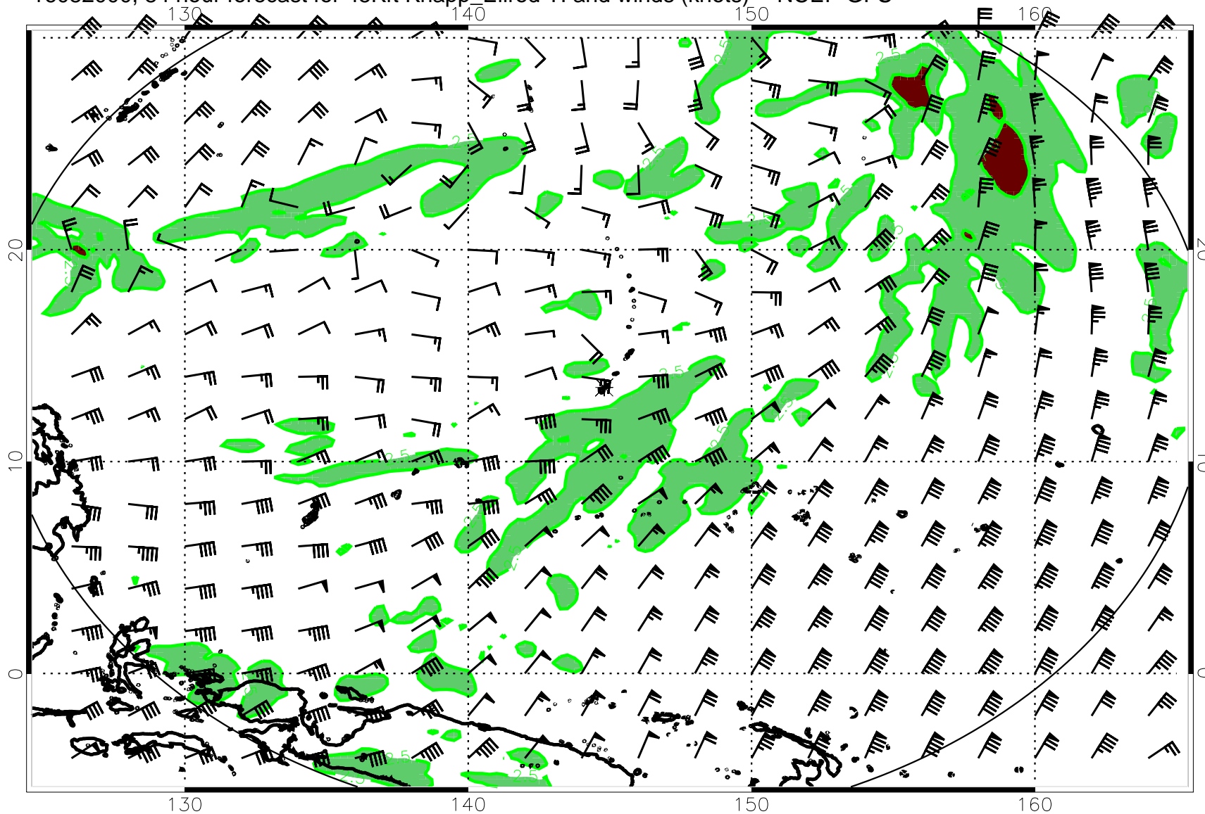
16082000, 84 hour forecast for 45Kft Knapp_Ellrod TI and winds (knots) -- NCEP GFS
