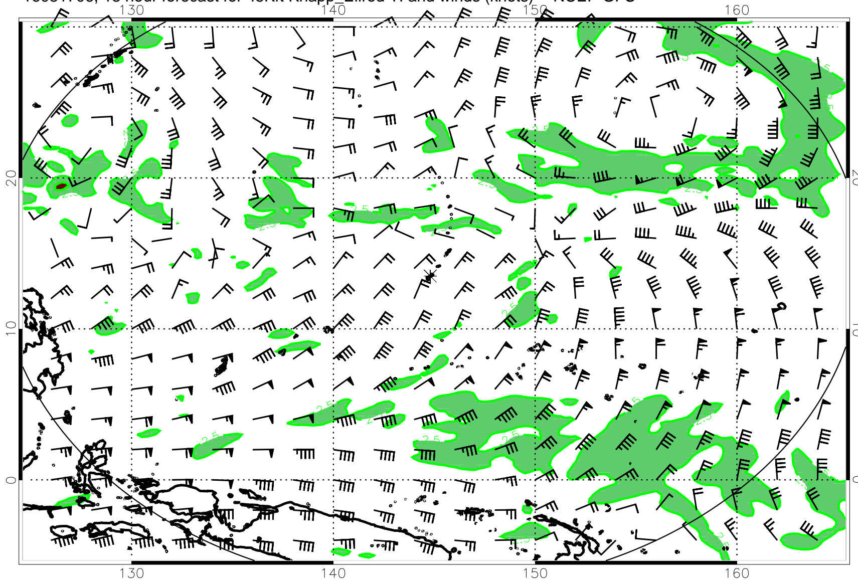
16081706, 18 hour forecast for 45Kft Knapp_Ellrod TI and winds (knots) -- NCEP GFS
