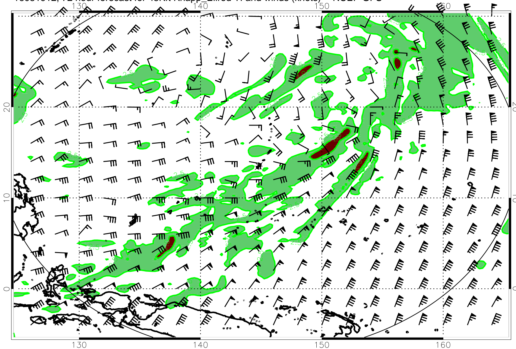
16081912, 72 hour forecast for 45Kft Knapp_Ellrod TI and winds (knots) -- NCEP GFS
