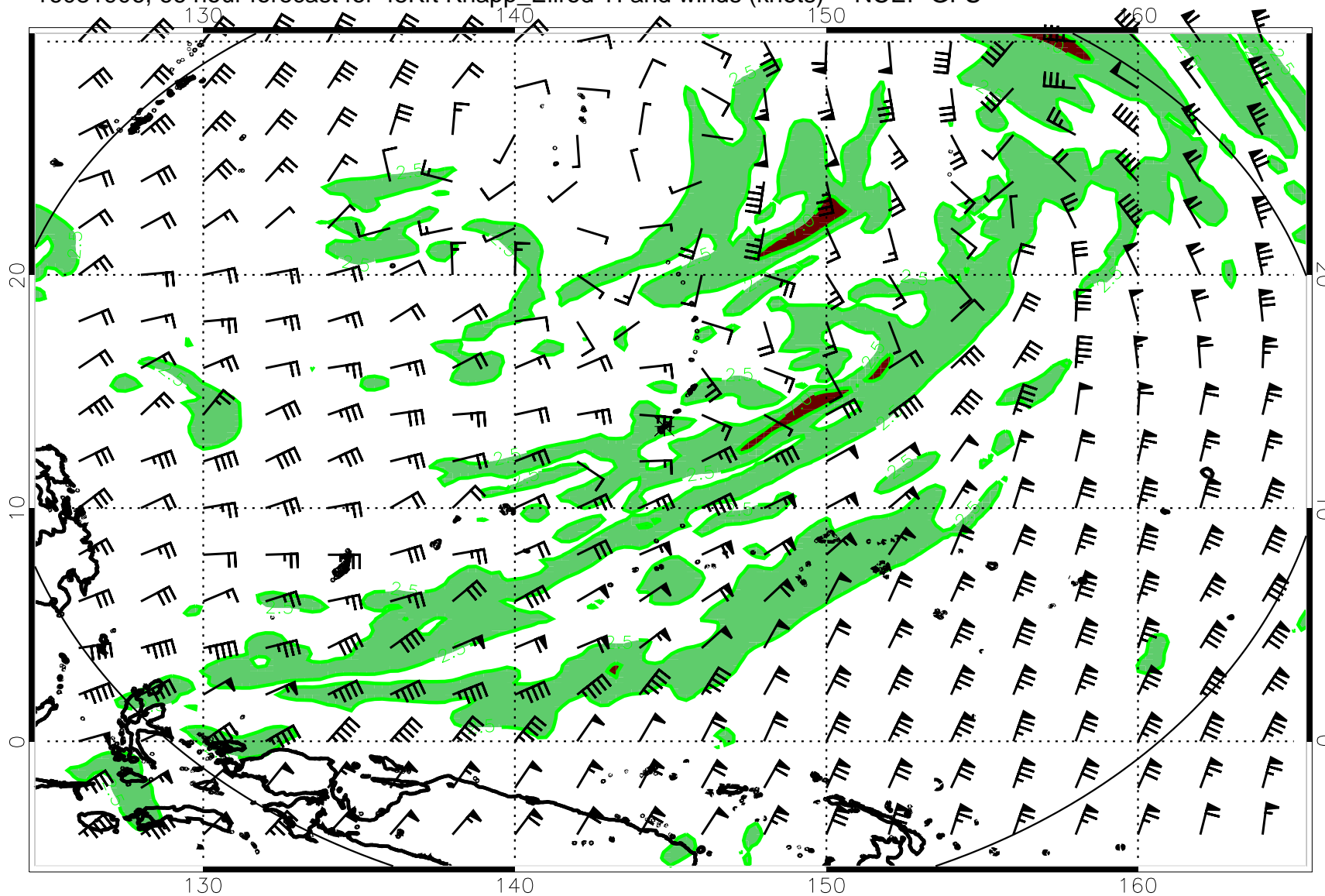
16081906, 66 hour forecast for 45Kft Knapp_Ellrod TI and winds (knots) -- NCEP GFS
