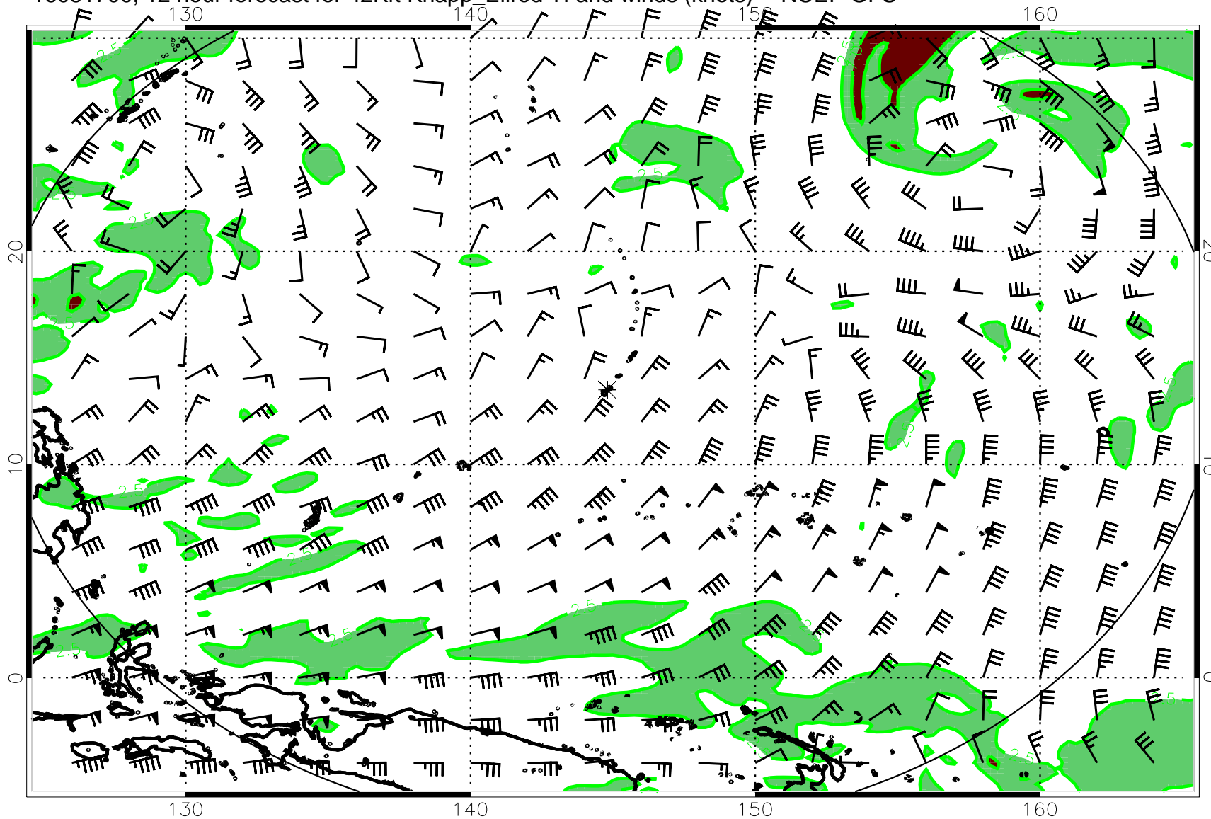
16081700, 12 hour forecast for 42Kft Knapp_Ellrod TI and winds (knots) -- NCEP GFS
