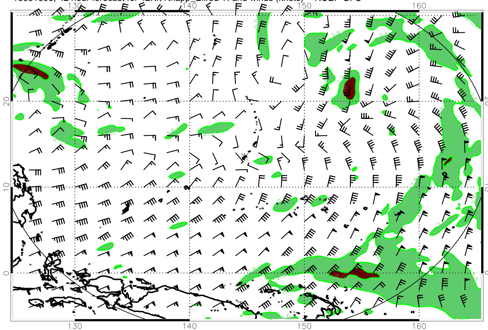
16081806, 42 hour forecast for 42Kft Knapp_Ellrod TI and winds (knots) -- NCEP GFS
