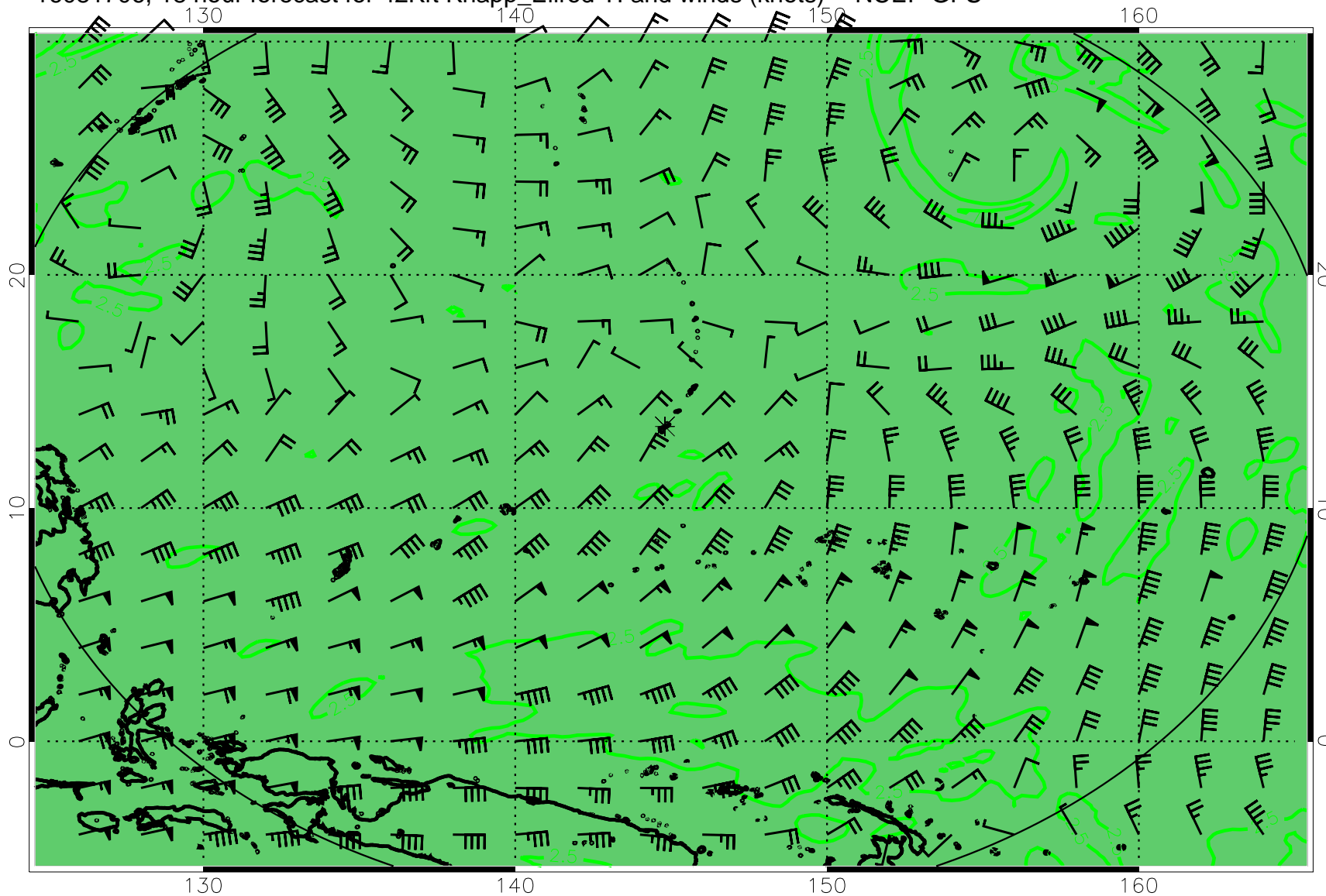
16081706, 18 hour forecast for 42Kft Knapp_Ellrod TI and winds (knots) -- NCEP GFS
