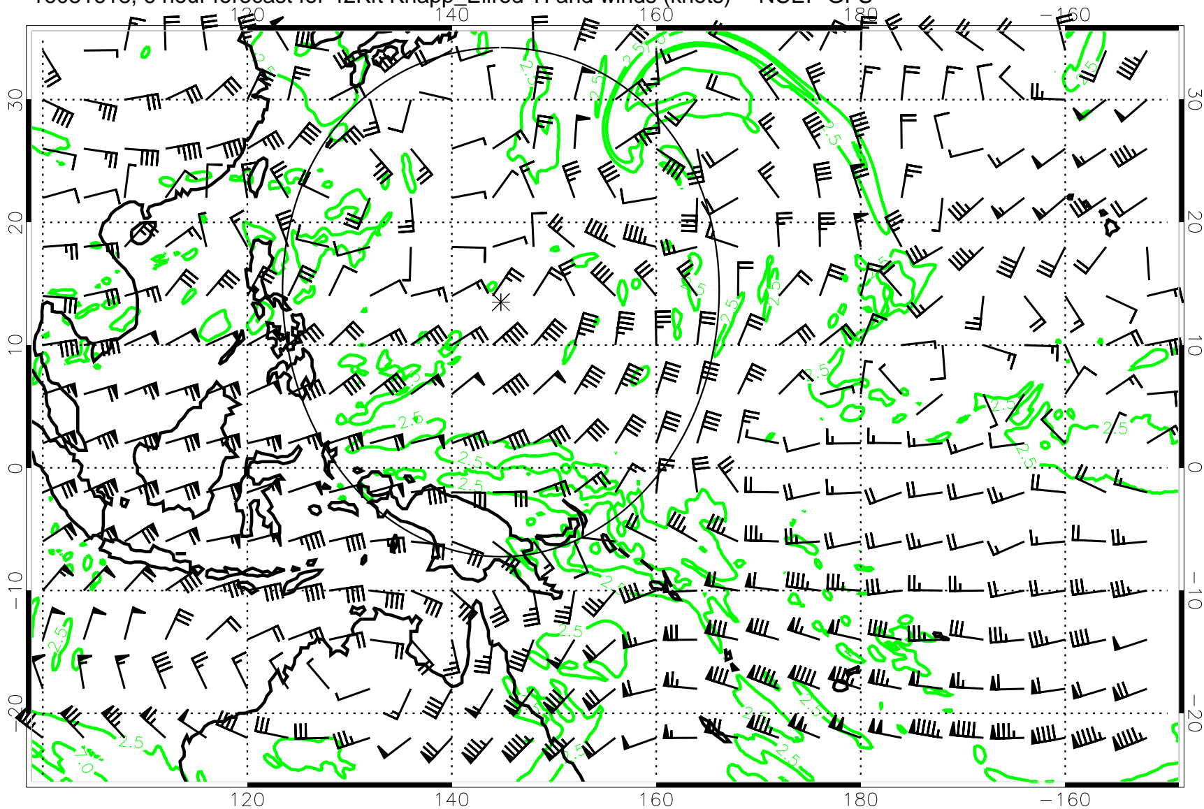
16081618, 6 hour forecast for 42Kft Knapp_Ellrod TI and winds (knots) -- NCEP GFS
