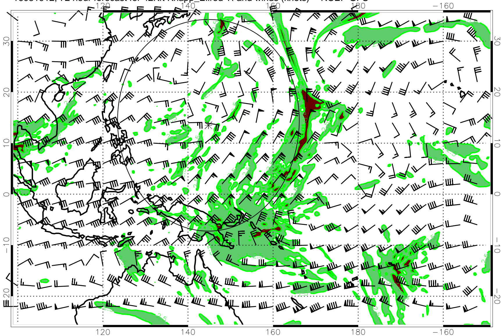
16081912, 72 hour forecast for 42Kft Knapp_Ellrod TI and winds (knots) -- NCEP GFS
