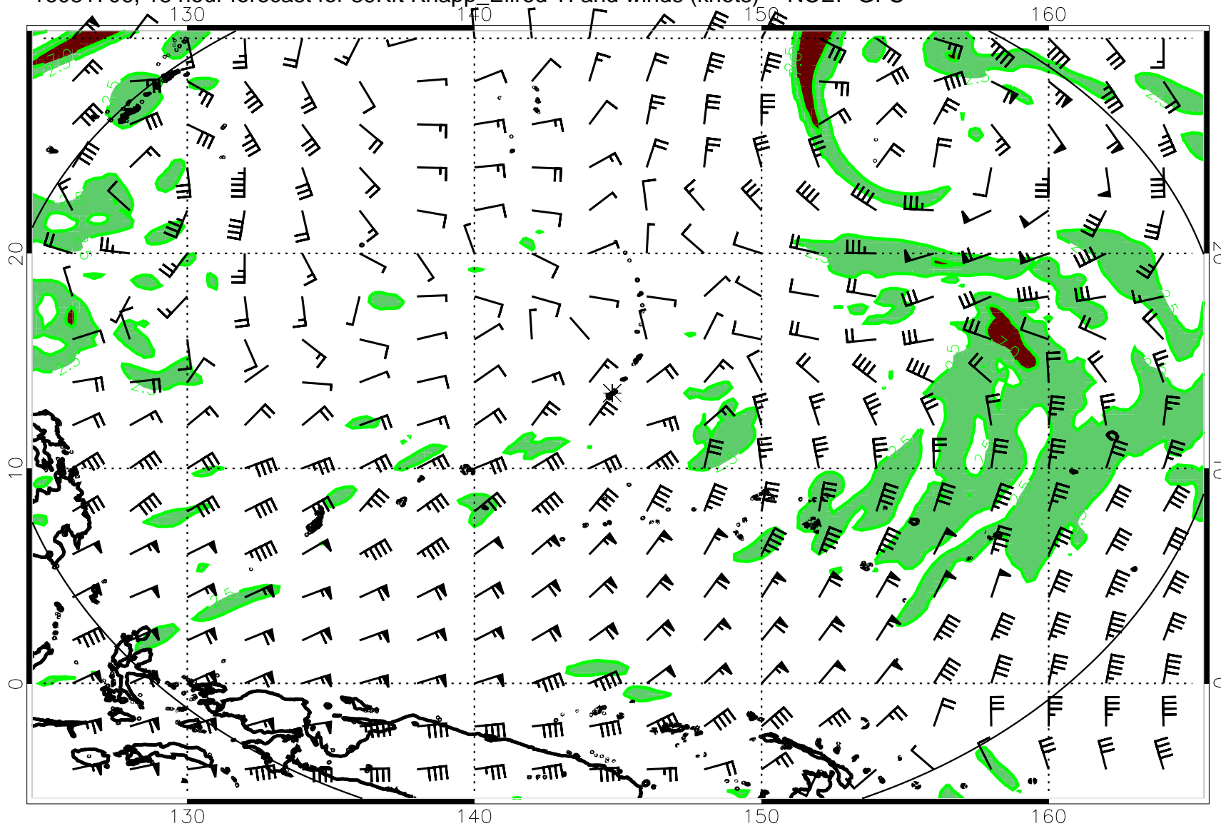
16081706, 18 hour forecast for 39Kft Knapp_Ellrod TI and winds (knots) -- NCEP GFS
