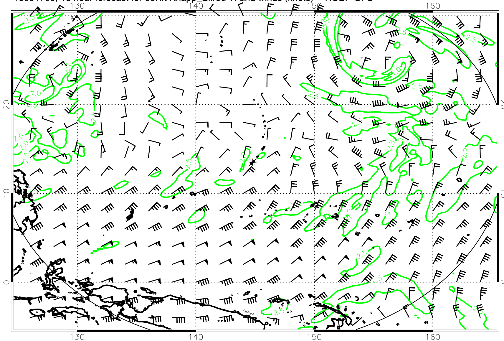
16081706, 18 hour forecast for 36Kft Knapp_Ellrod TI and winds (knots) -- NCEP GFS
