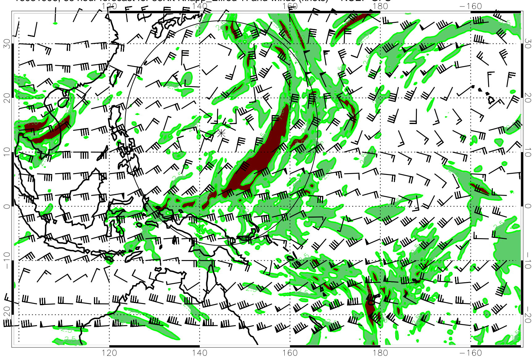
16081906, 66 hour forecast for 36Kft Knapp_Ellrod TI and winds (knots) -- NCEP GFS
