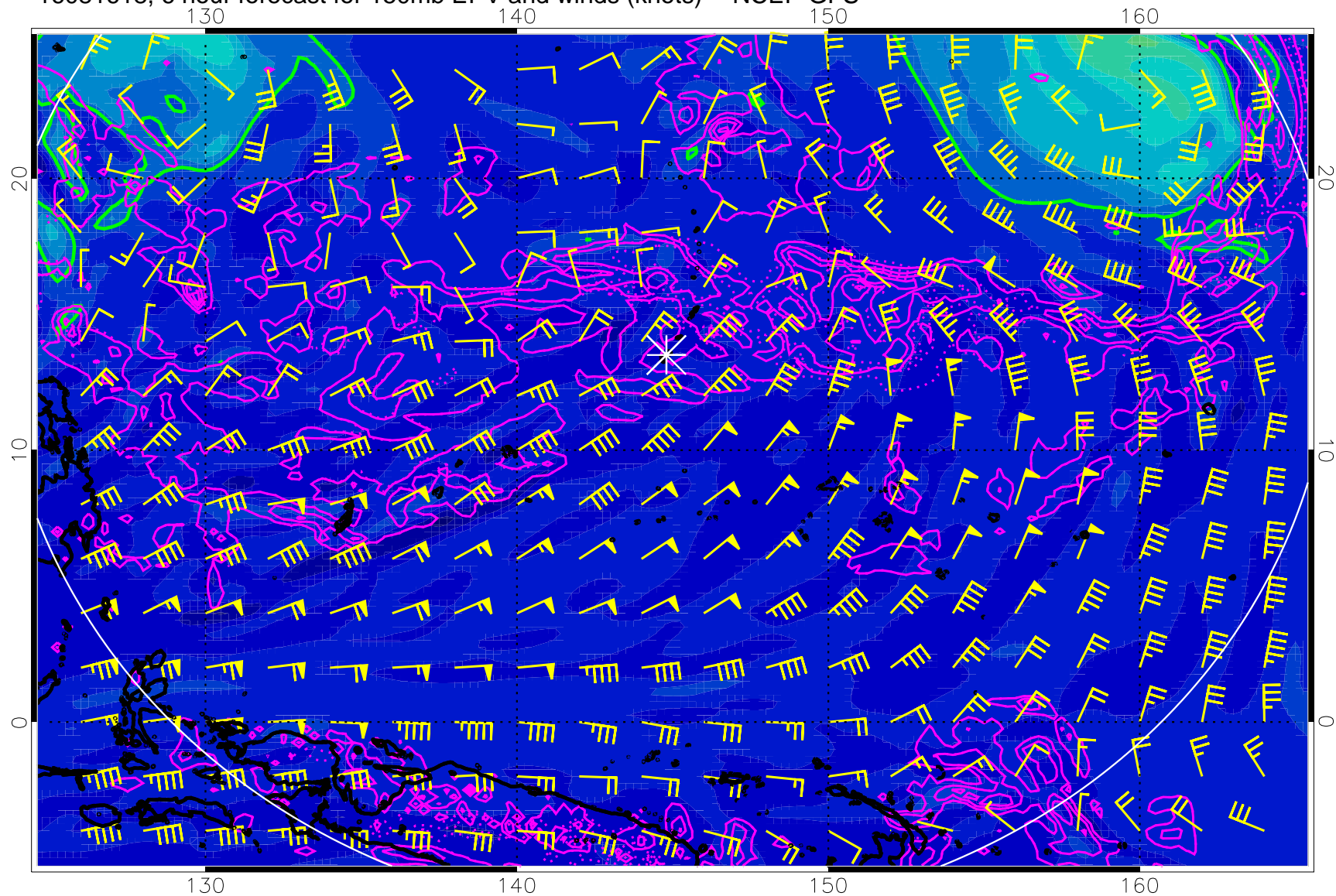
16081618, 6 hour forecast for 150mb EPV and winds (knots) -- NCEP GFS
