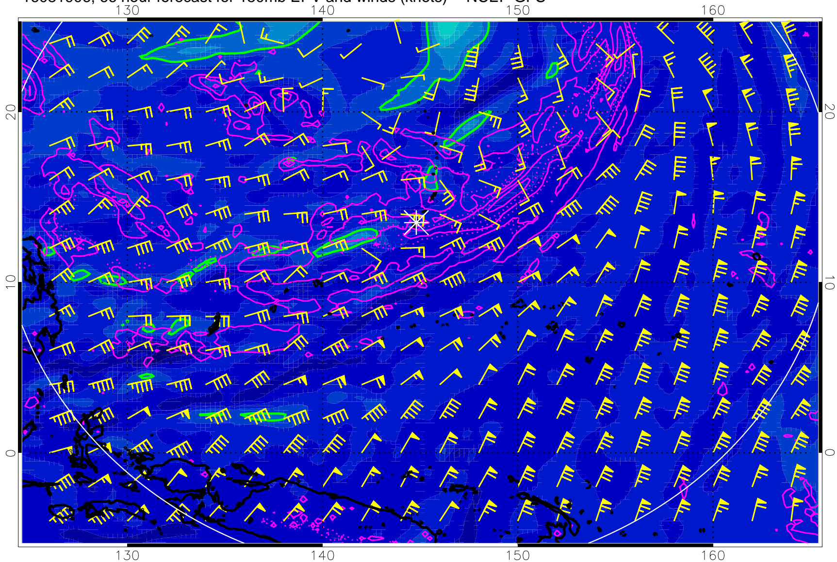
16081906, 66 hour forecast for 150mb EPV and winds (knots) -- NCEP GFS
