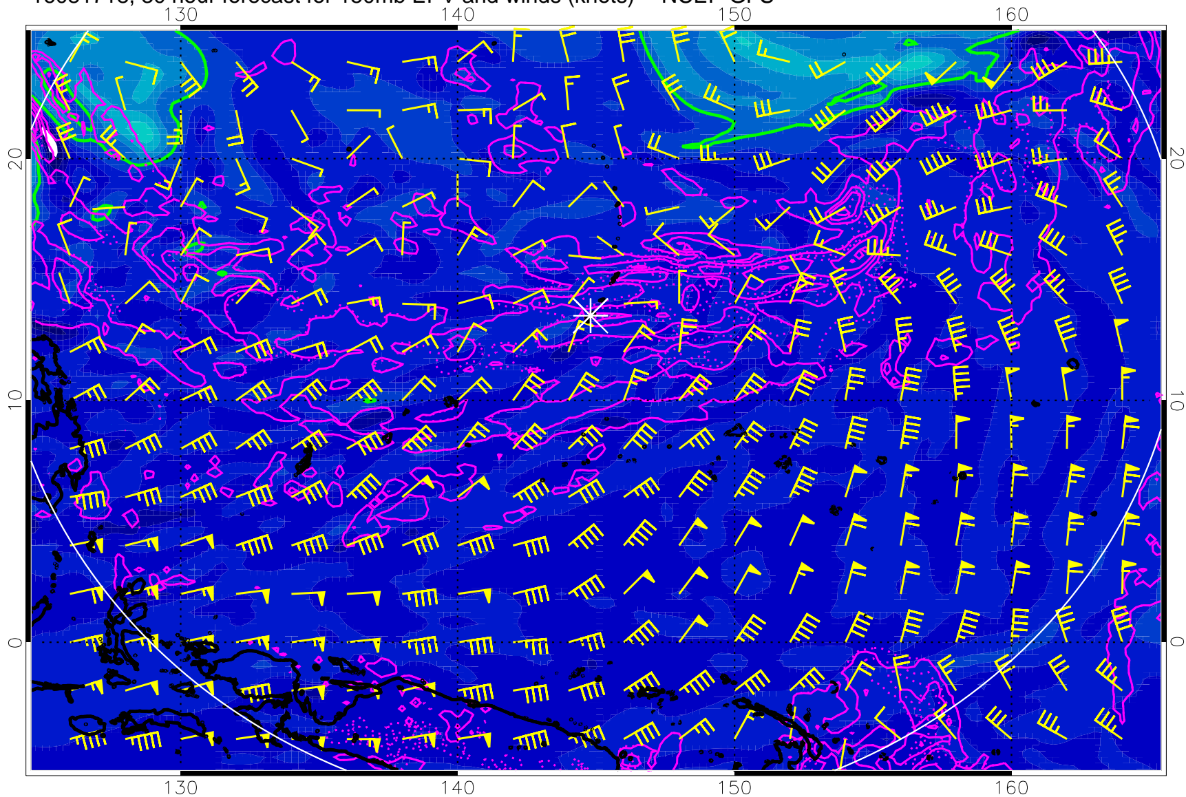
16081718, 30 hour forecast for 150mb EPV and winds (knots) -- NCEP GFS
