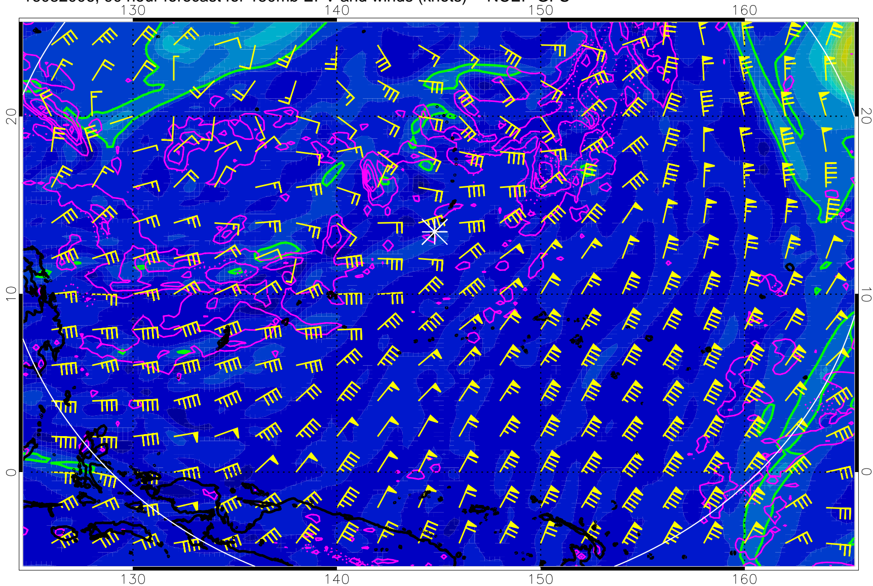
16082006, 90 hour forecast for 150mb EPV and winds (knots) -- NCEP GFS
