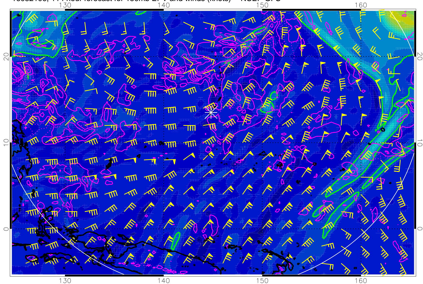
16082106, 114 hour forecast for 150mb EPV and winds (knots) -- NCEP GFS
