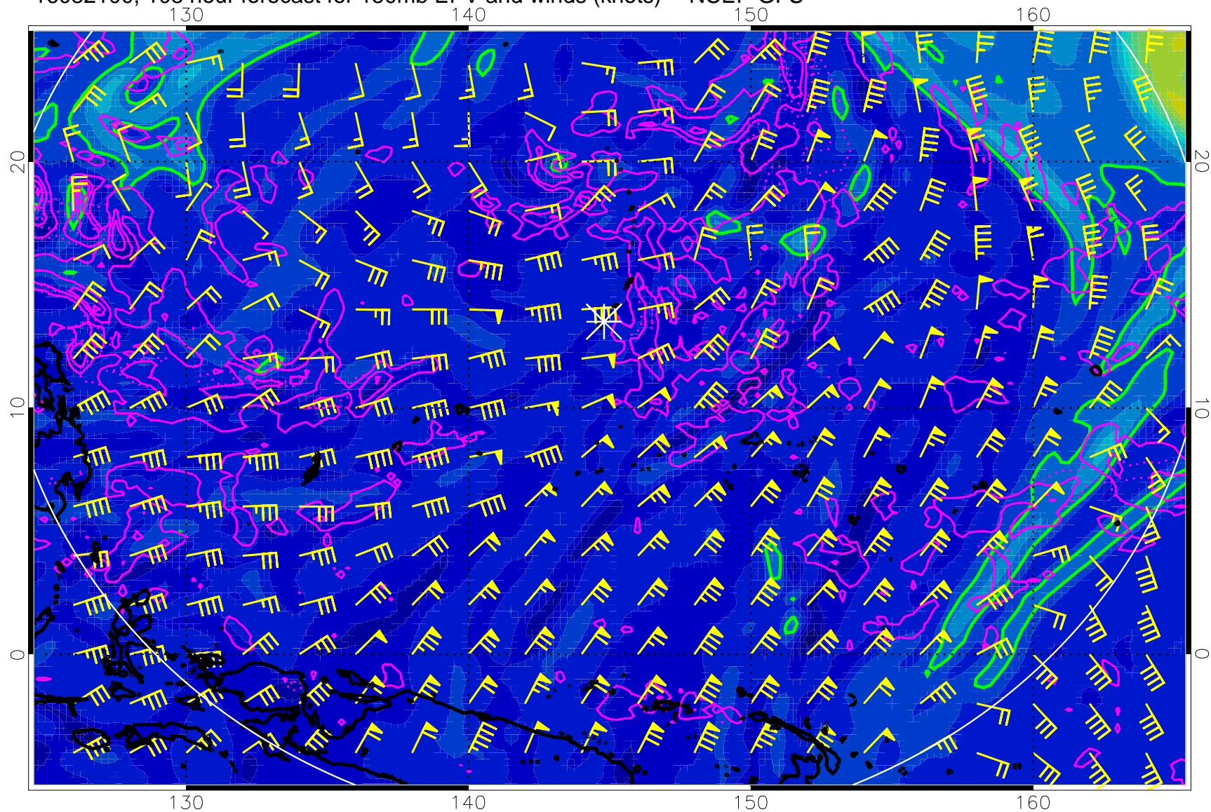
16082100, 108 hour forecast for 150mb EPV and winds (knots) -- NCEP GFS
