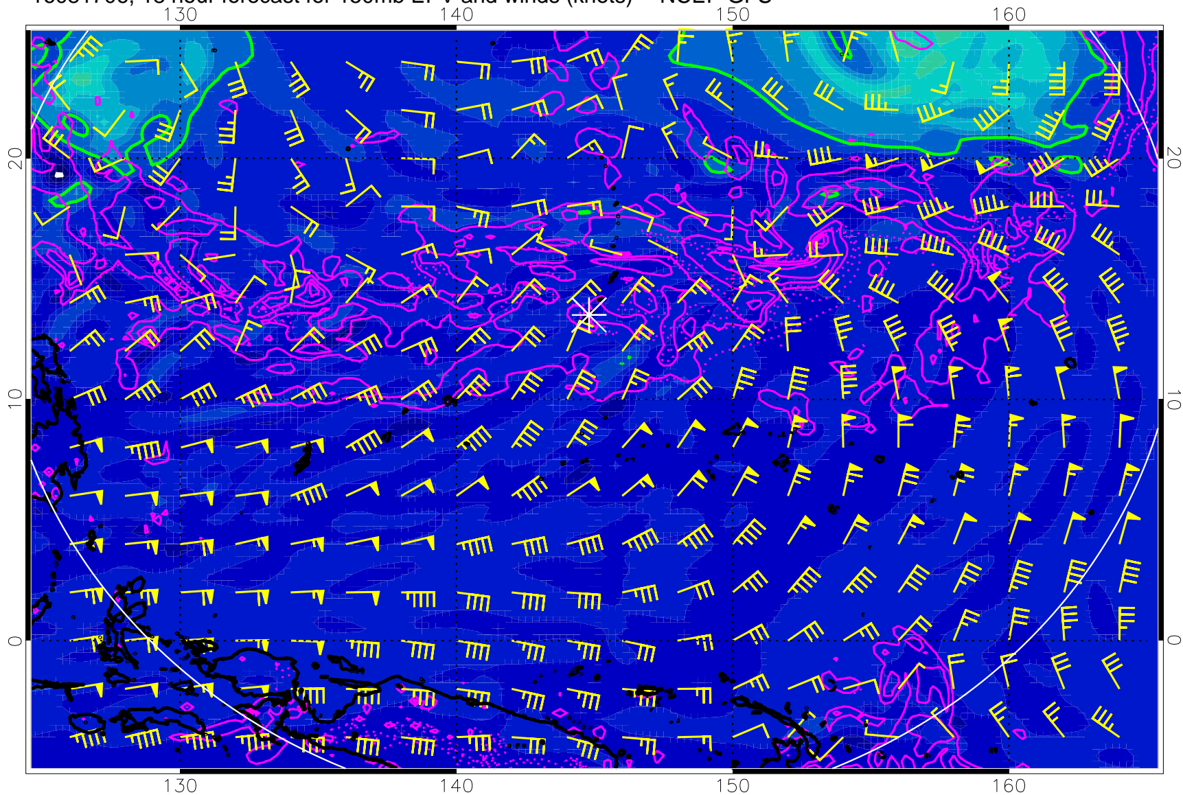
16081706, 18 hour forecast for 150mb EPV and winds (knots) -- NCEP GFS
