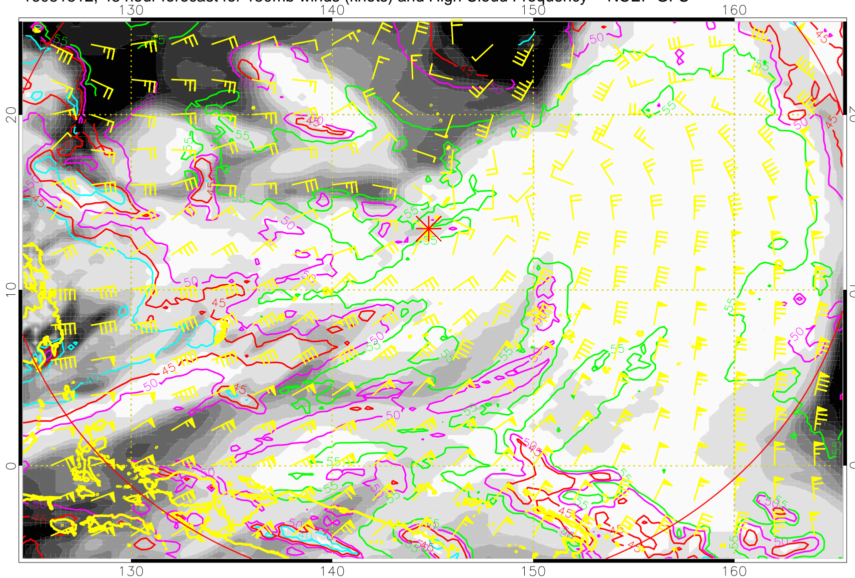
16081812, 48 hour forecast for 150mb winds (knots) and High Cloud Frequency -- NCEP GFS
