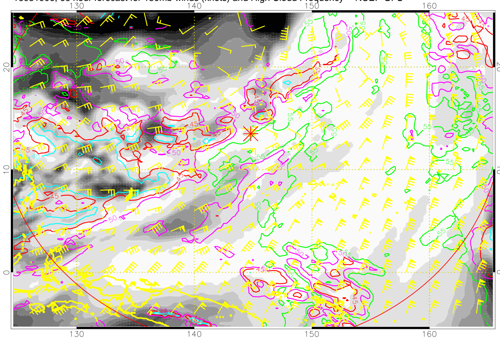
16081906, 66 hour forecast for 150mb winds (knots) and High Cloud Frequency -- NCEP GFS
