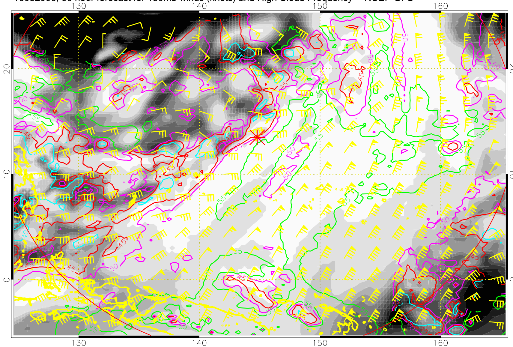
16082006, 90 hour forecast for 150mb winds (knots) and High Cloud Frequency -- NCEP GFS
