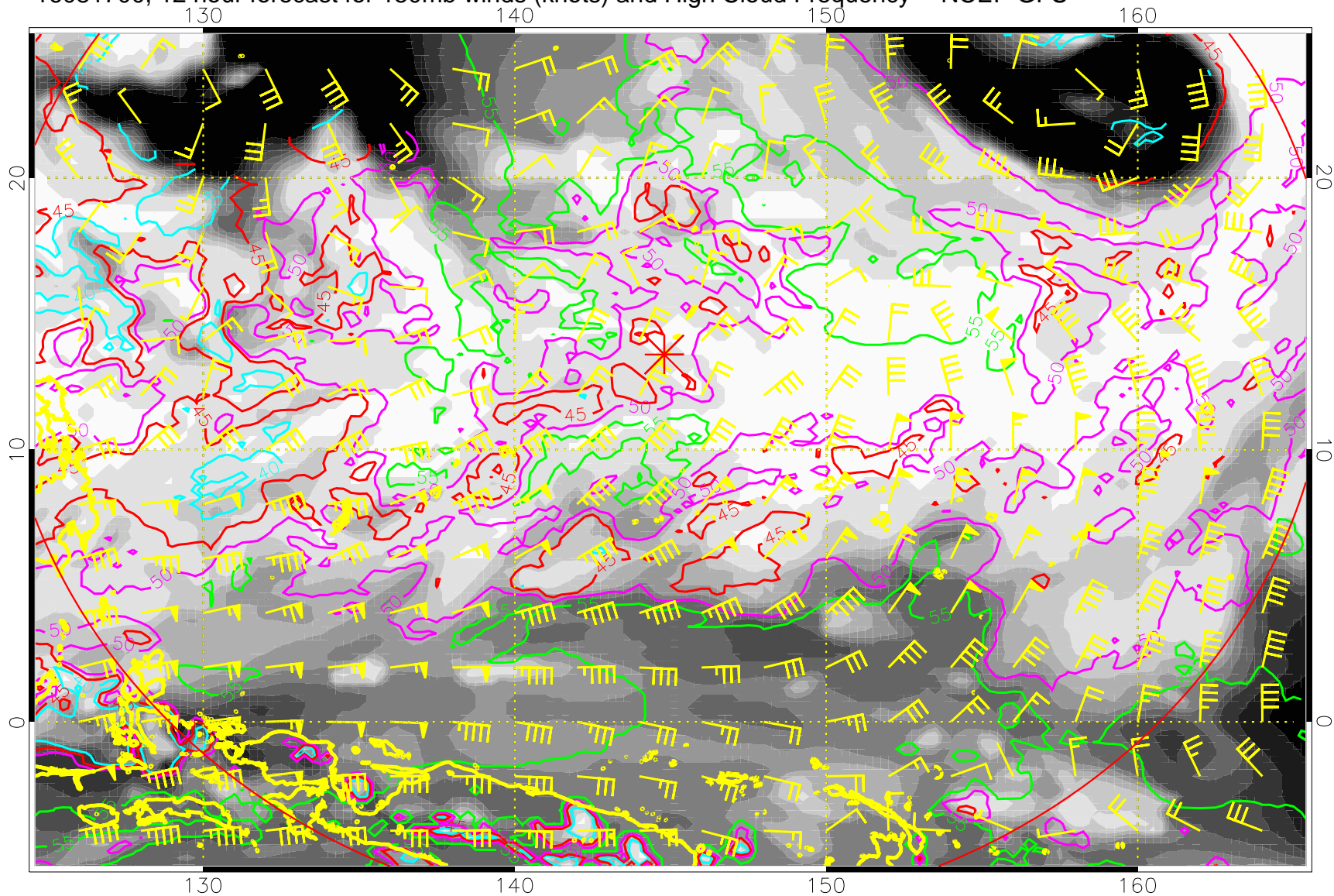
16081700, 12 hour forecast for 150mb winds (knots) and High Cloud Frequency -- NCEP GFS
