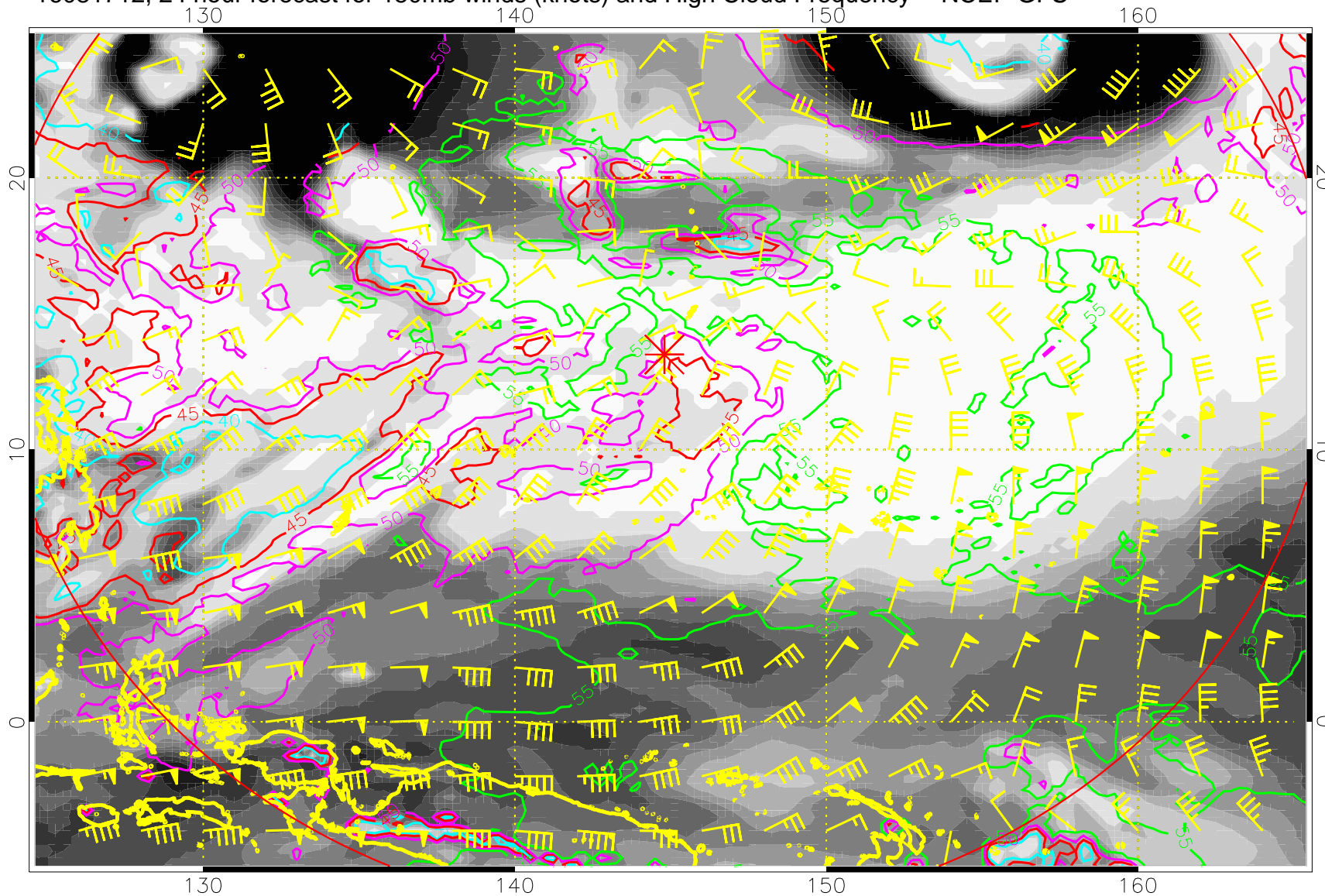
16081712, 24 hour forecast for 150mb winds (knots) and High Cloud Frequency -- NCEP GFS
