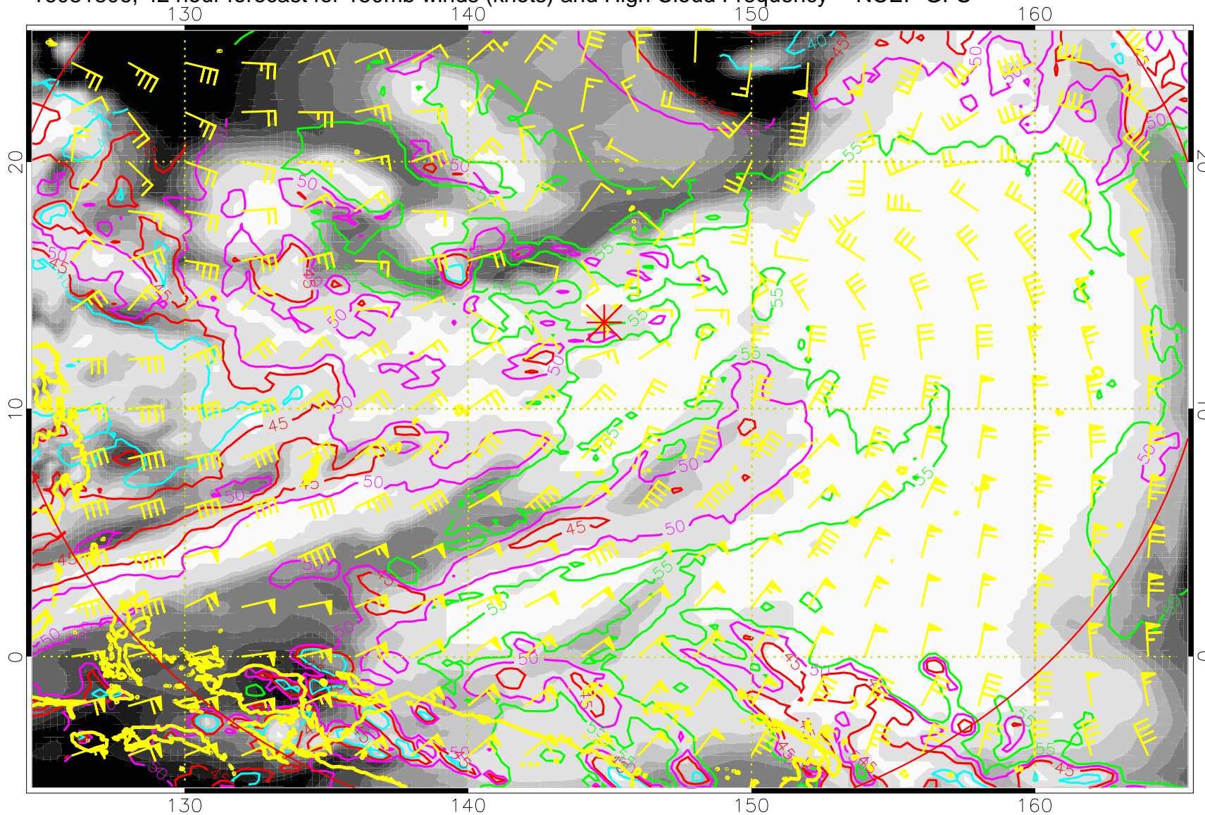
16081806, 42 hour forecast for 150mb winds (knots) and High Cloud Frequency -- NCEP GFS
