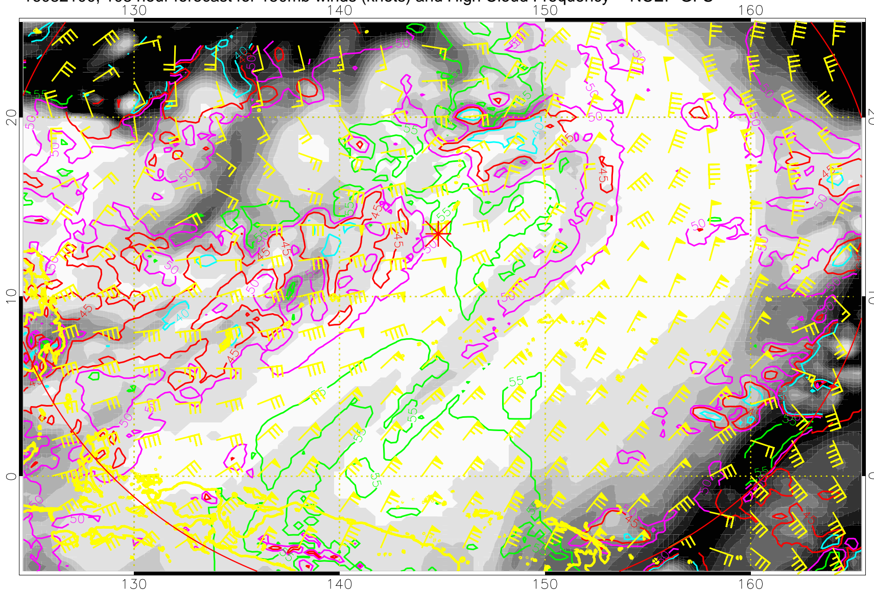
16082100, 108 hour forecast for 150mb winds (knots) and High Cloud Frequency -- NCEP GFS
