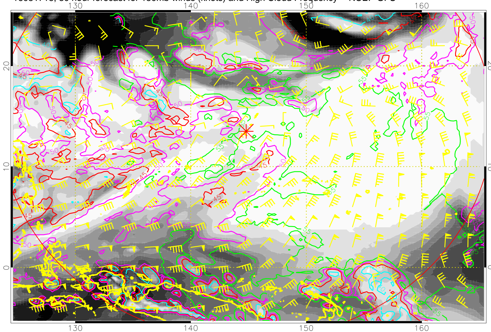
16081718, 30 hour forecast for 150mb winds (knots) and High Cloud Frequency -- NCEP GFS
