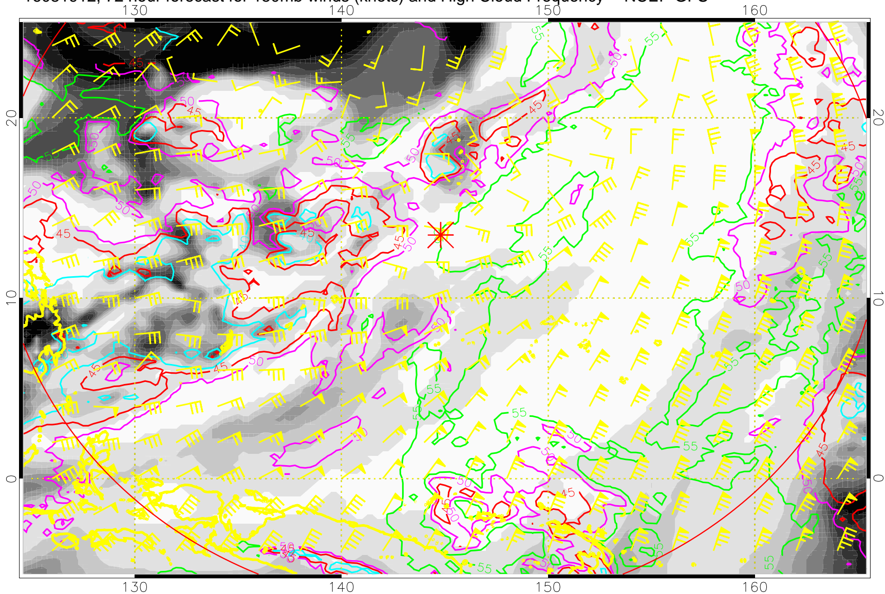
16081912, 72 hour forecast for 150mb winds (knots) and High Cloud Frequency -- NCEP GFS
