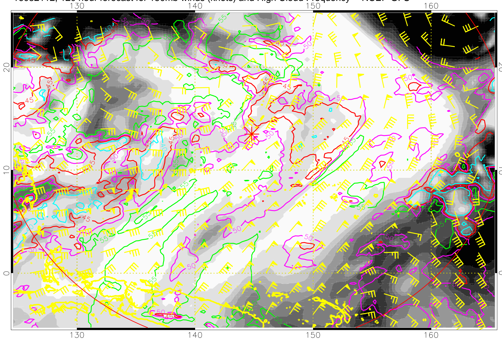
16082112, 120 hour forecast for 150mb winds (knots) and High Cloud Frequency -- NCEP GFS
