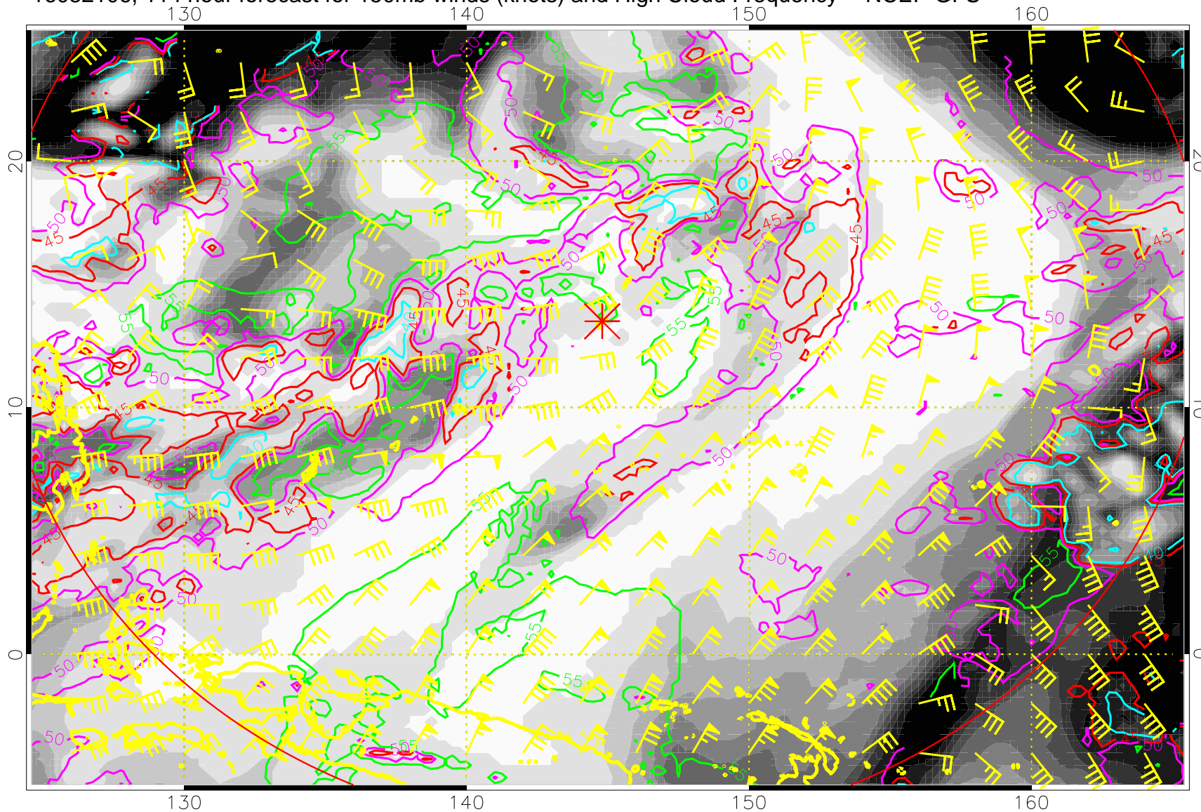
16082106, 114 hour forecast for 150mb winds (knots) and High Cloud Frequency -- NCEP GFS
