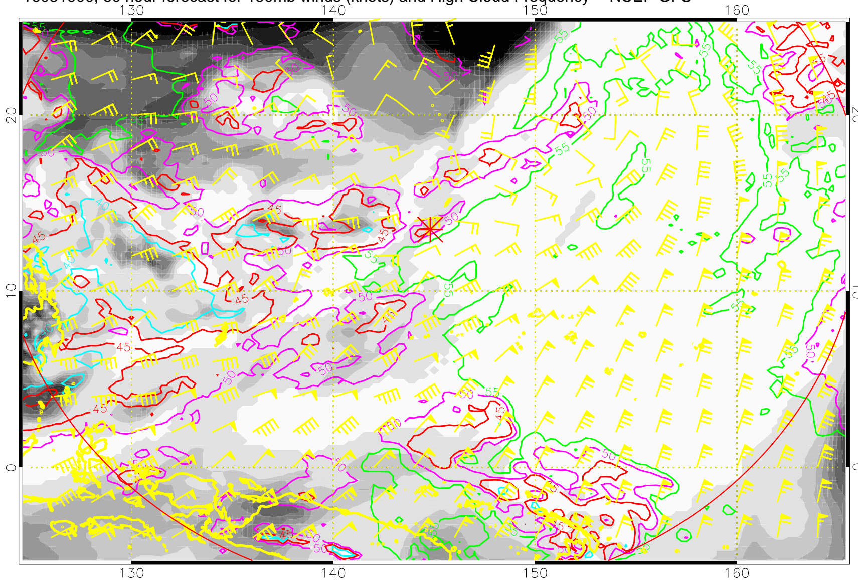
16081900, 60 hour forecast for 150mb winds (knots) and High Cloud Frequency -- NCEP GFS
