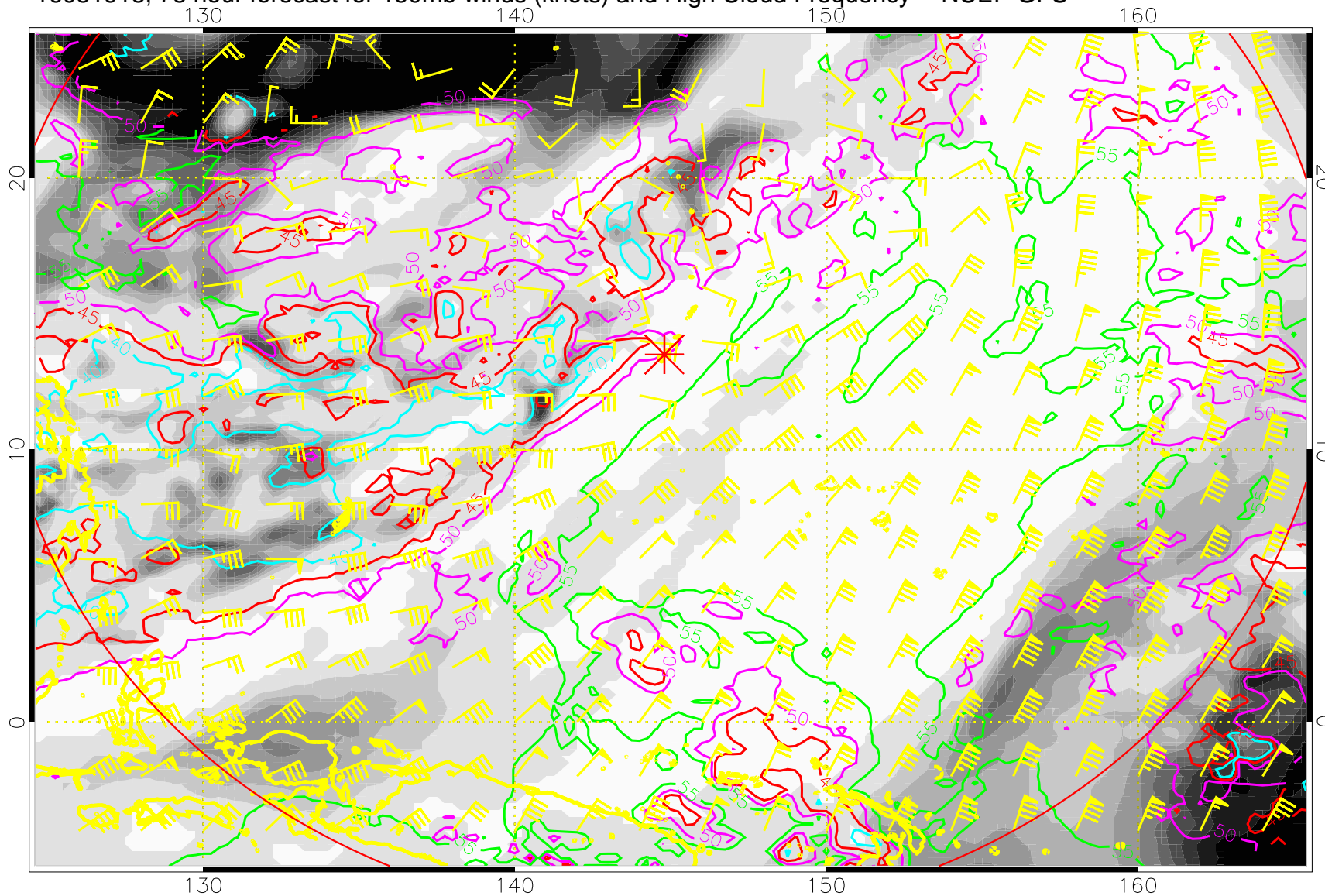
16081918, 78 hour forecast for 150mb winds (knots) and High Cloud Frequency -- NCEP GFS
