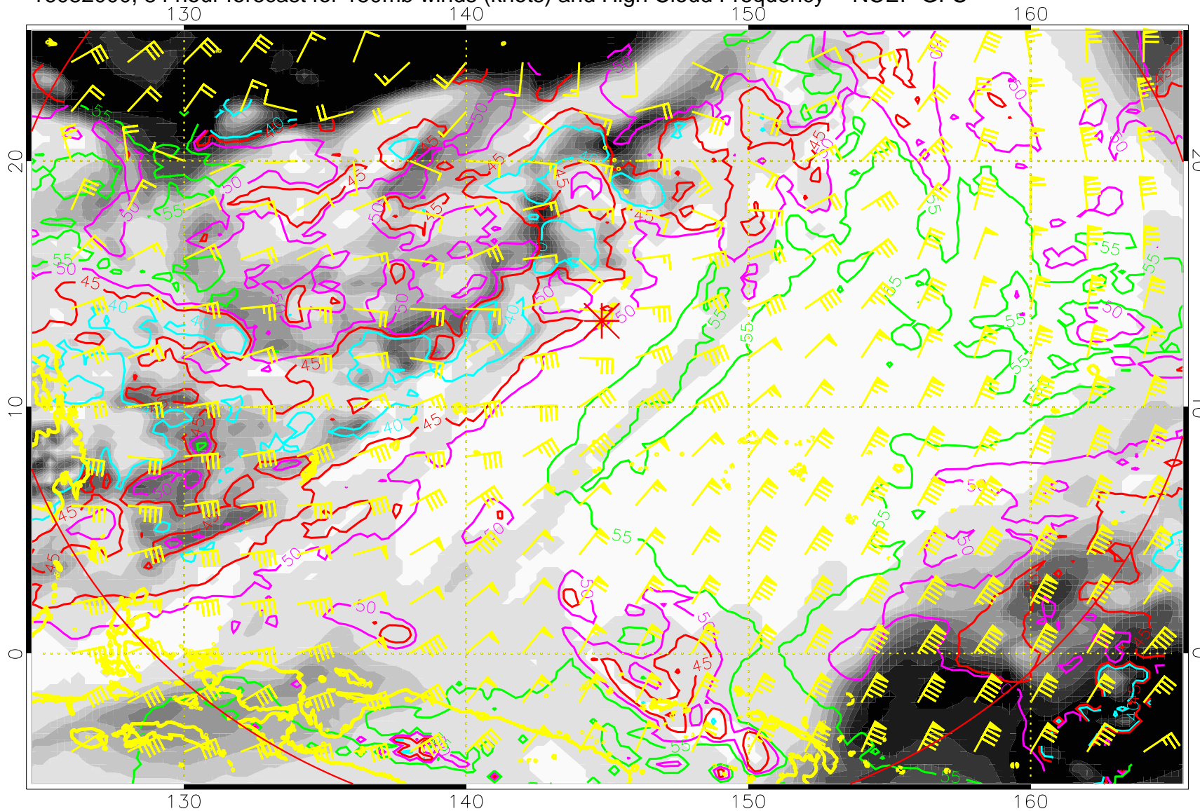
16082000, 84 hour forecast for 150mb winds (knots) and High Cloud Frequency -- NCEP GFS
