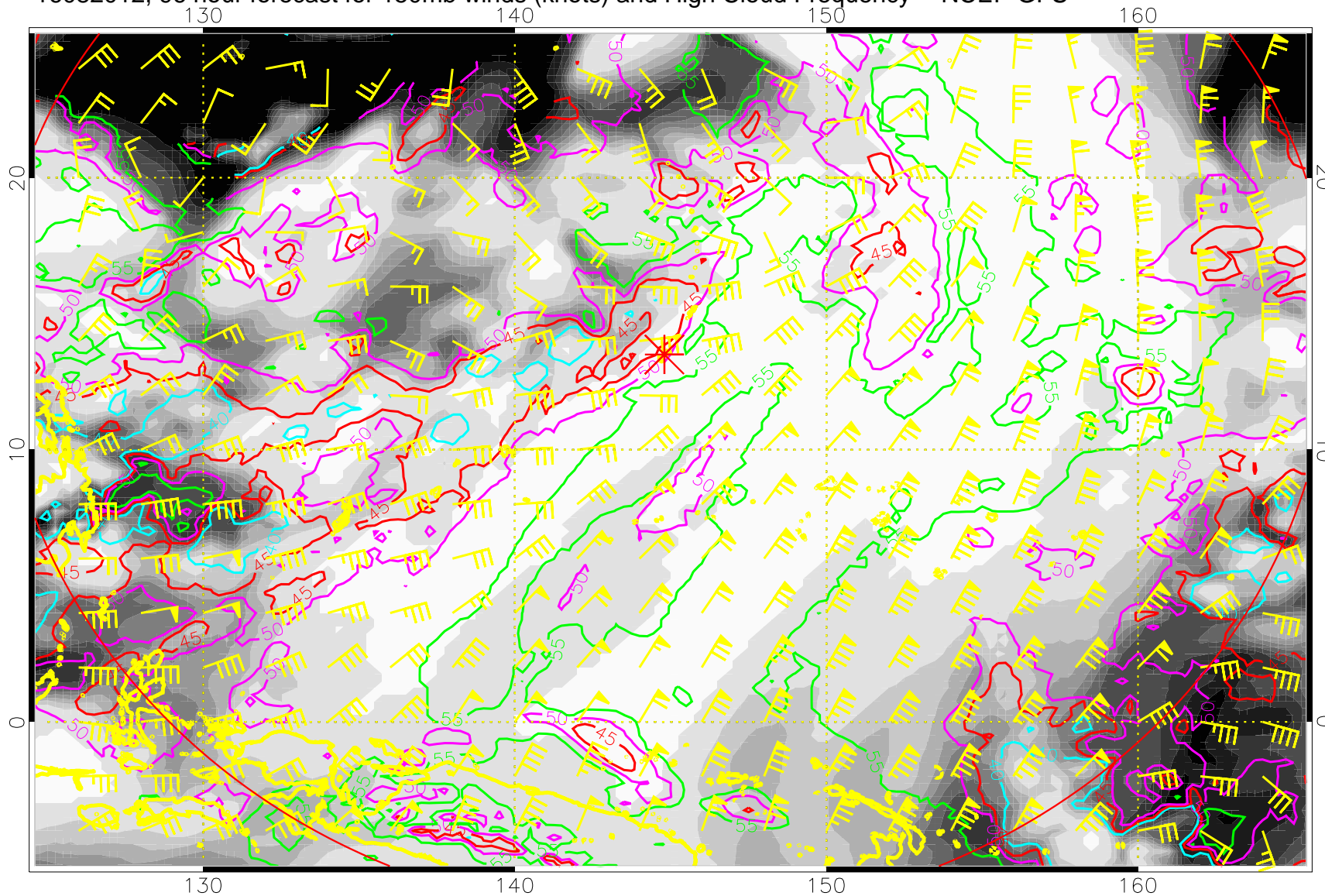
16082012, 96 hour forecast for 150mb winds (knots) and High Cloud Frequency -- NCEP GFS
