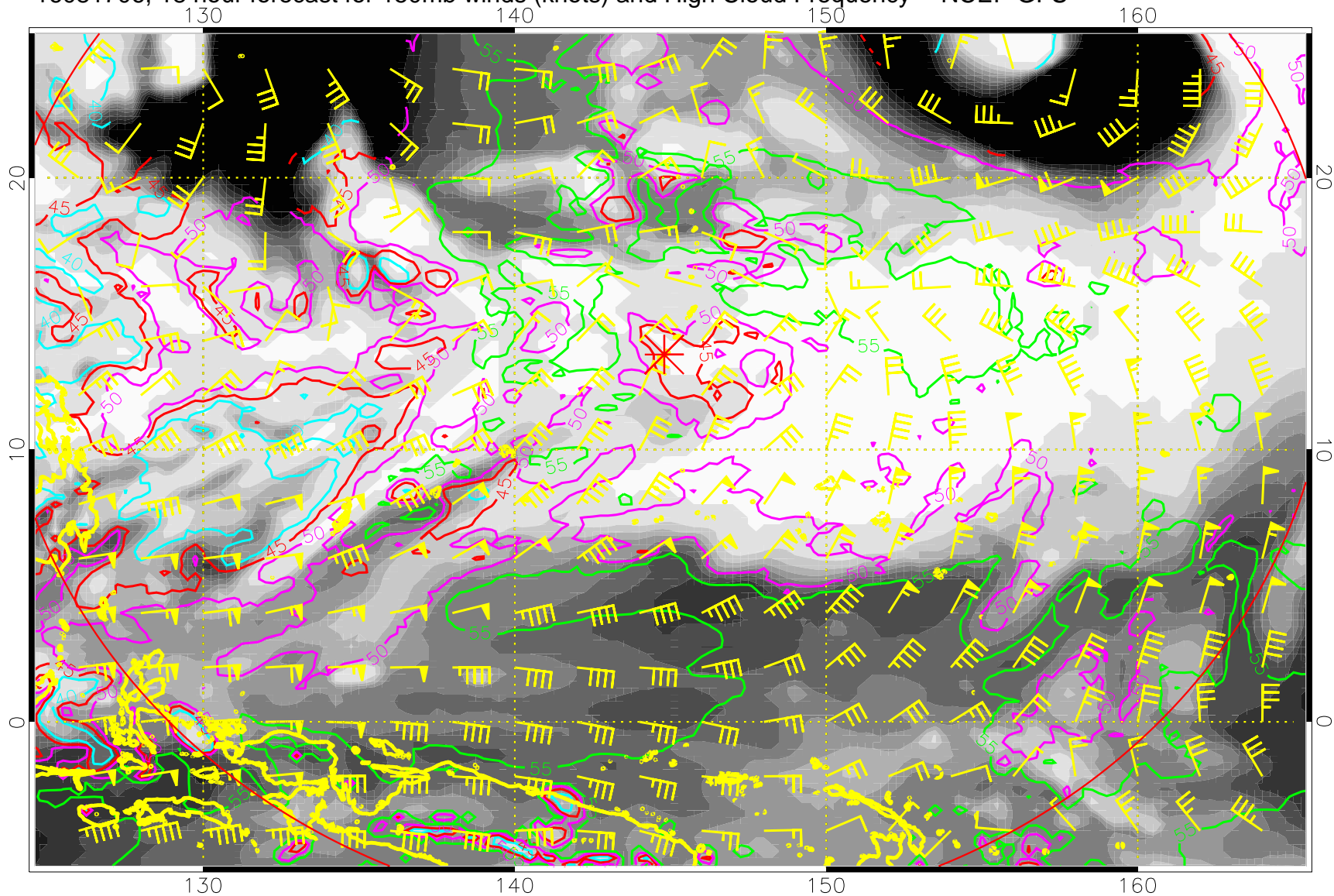
16081706, 18 hour forecast for 150mb winds (knots) and High Cloud Frequency -- NCEP GFS
