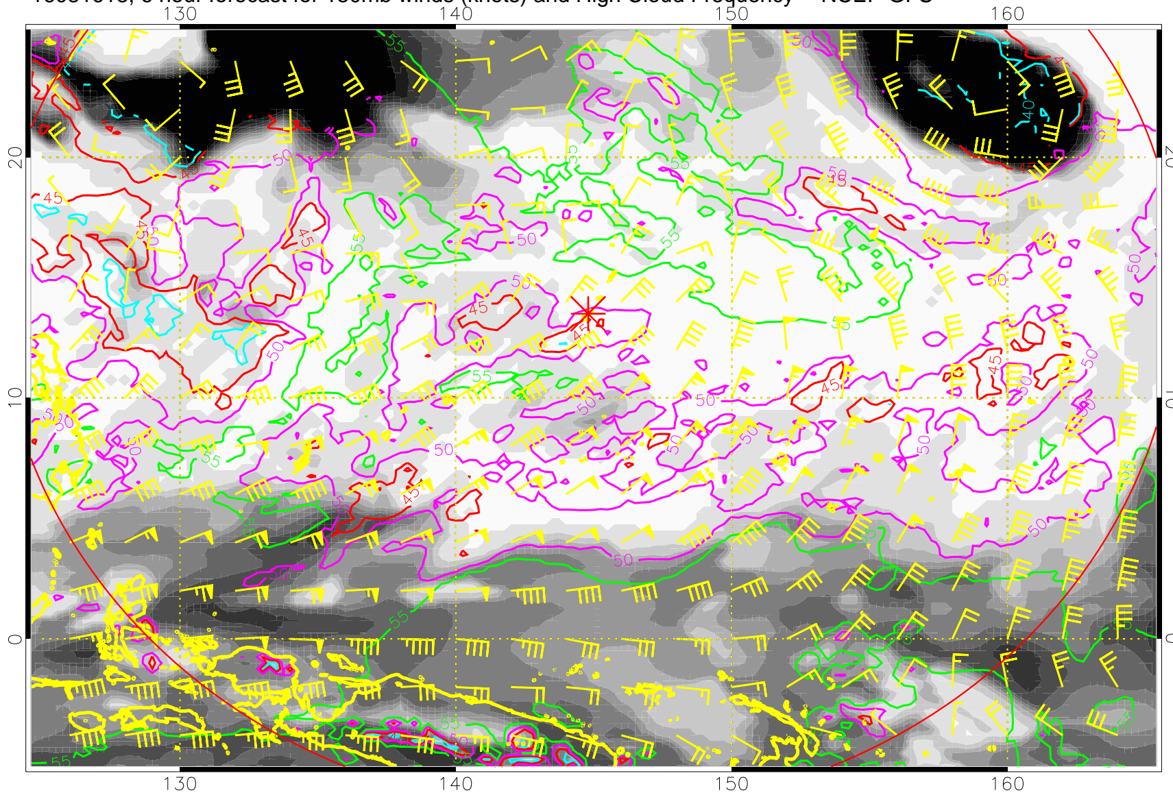
16081618, 6 hour forecast for 150mb winds (knots) and High Cloud Frequency -- NCEP GFS
