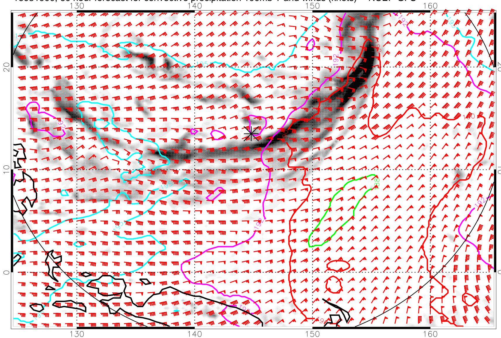
16081900, 60 hour forecast for convective precipitation 100mb T and winds (knots) -- NCEP GFS
