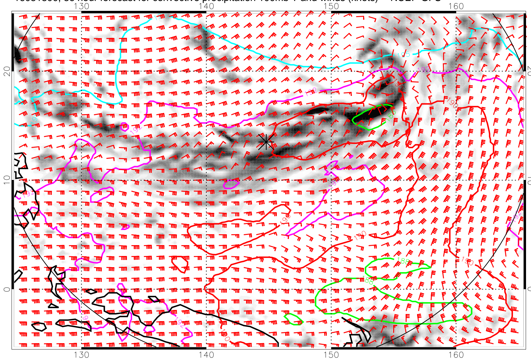
16081800, 36 hour forecast for convective precipitation 100mb T and winds (knots) -- NCEP GFS
