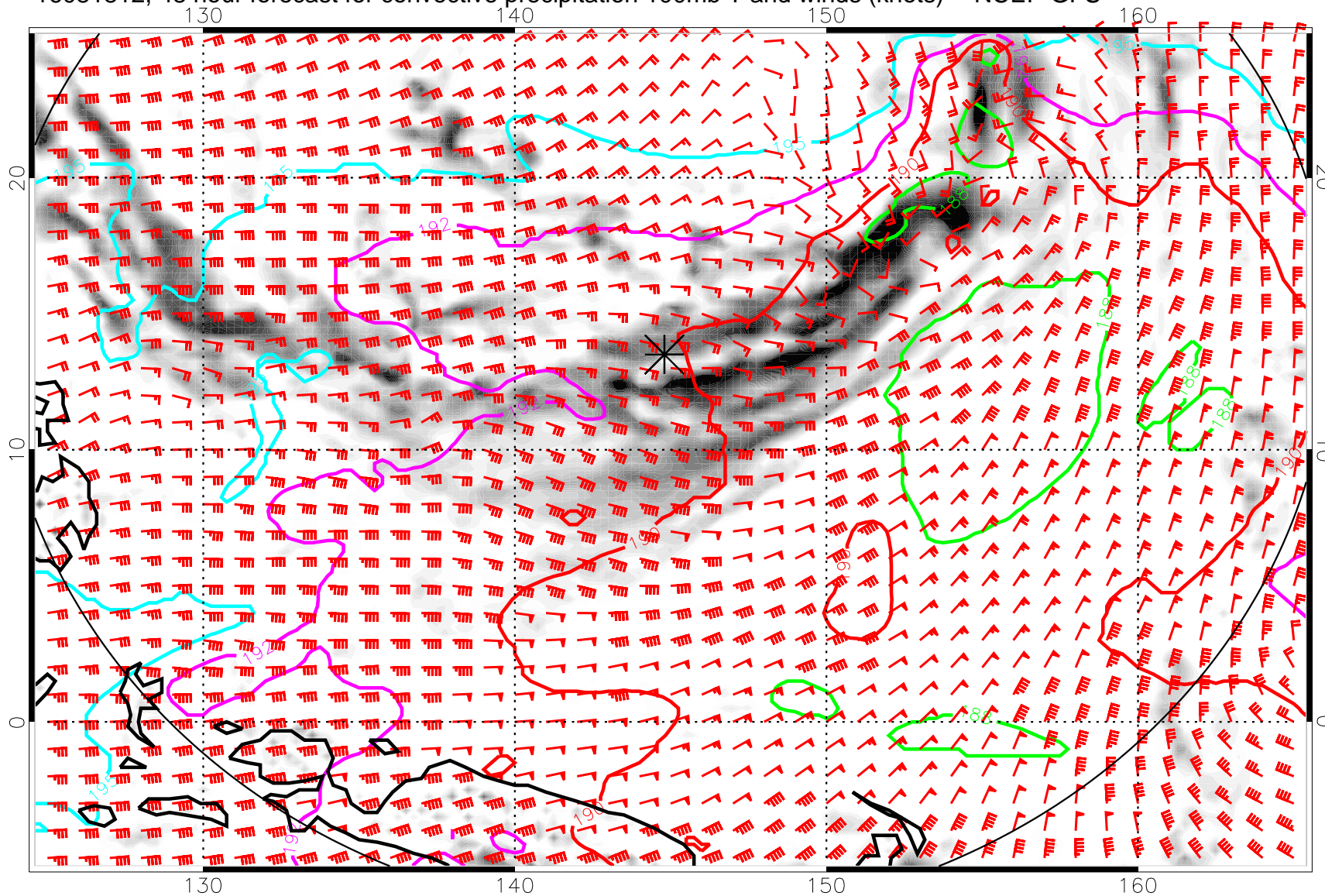
16081812, 48 hour forecast for convective precipitation 100mb T and winds (knots) -- NCEP GFS
