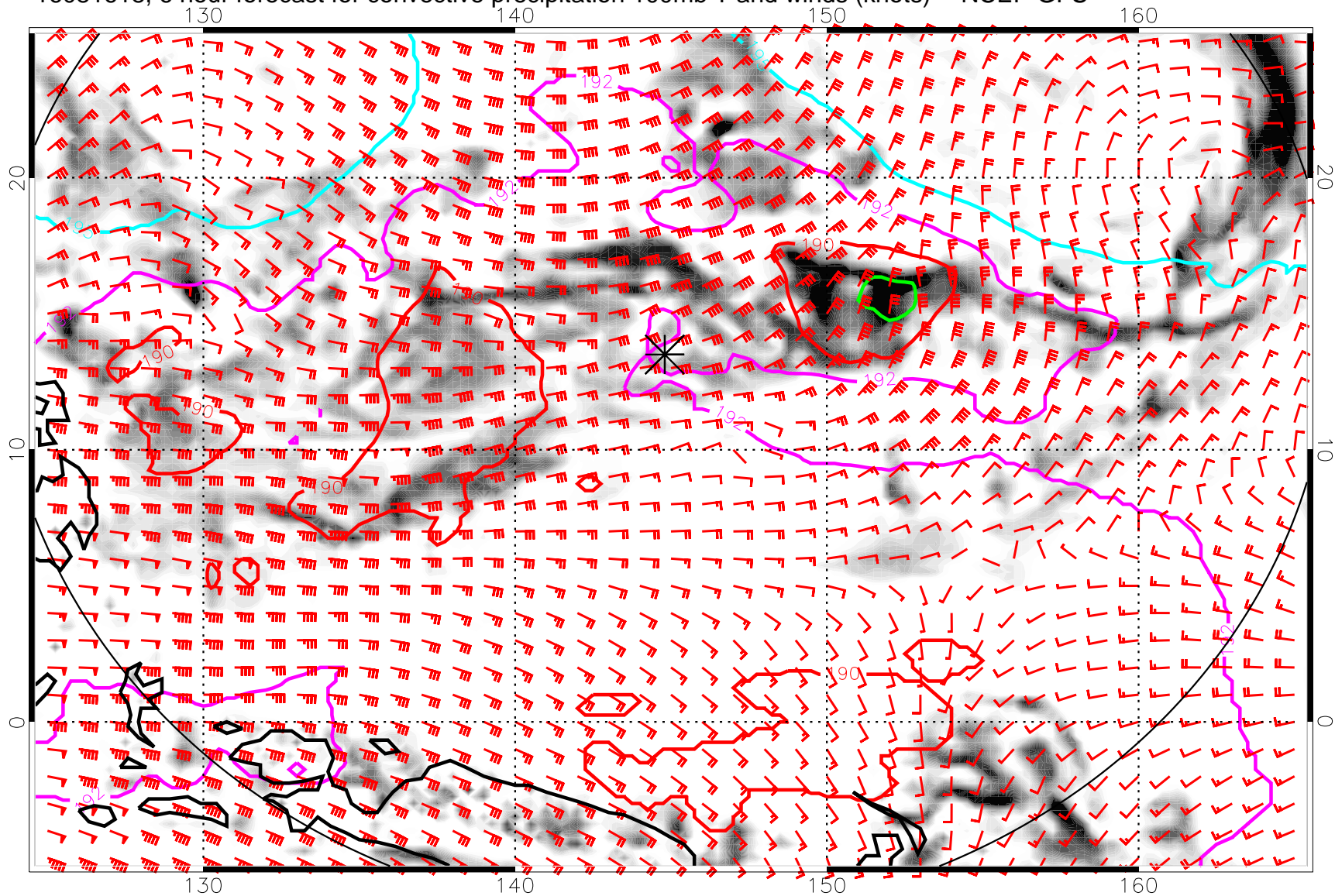
16081618, 6 hour forecast for convective precipitation 100mb T and winds (knots) -- NCEP GFS
