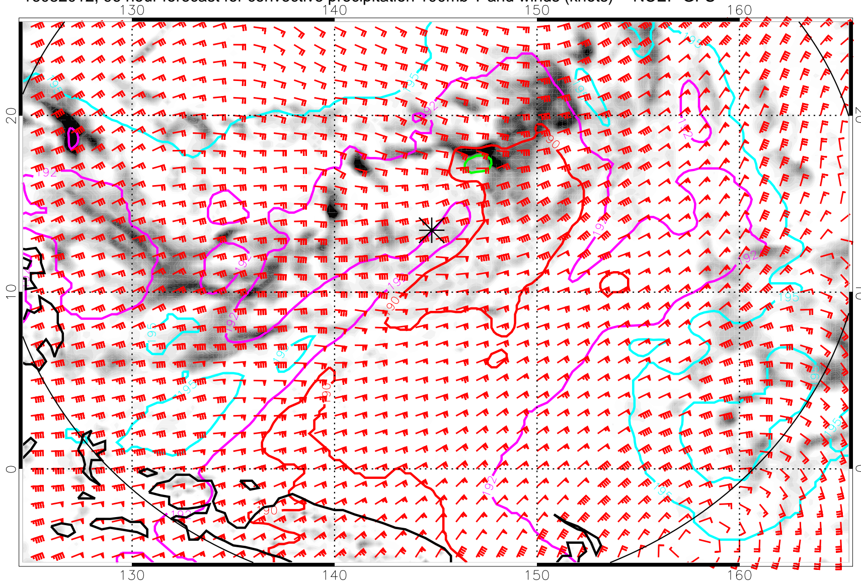
16082012, 96 hour forecast for convective precipitation 100mb T and winds (knots) -- NCEP GFS
