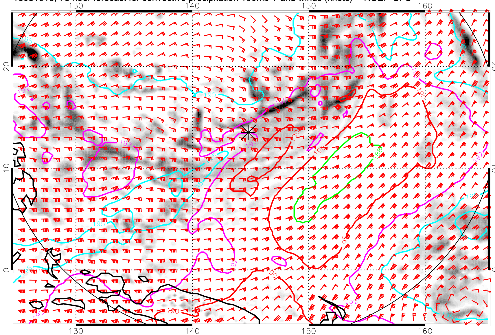
16081918, 78 hour forecast for convective precipitation 100mb T and winds (knots) -- NCEP GFS
