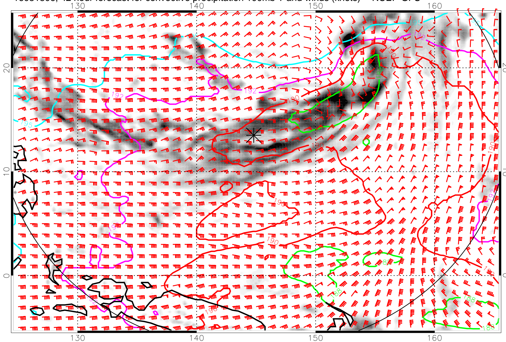
16081806, 42 hour forecast for convective precipitation 100mb T and winds (knots) -- NCEP GFS
