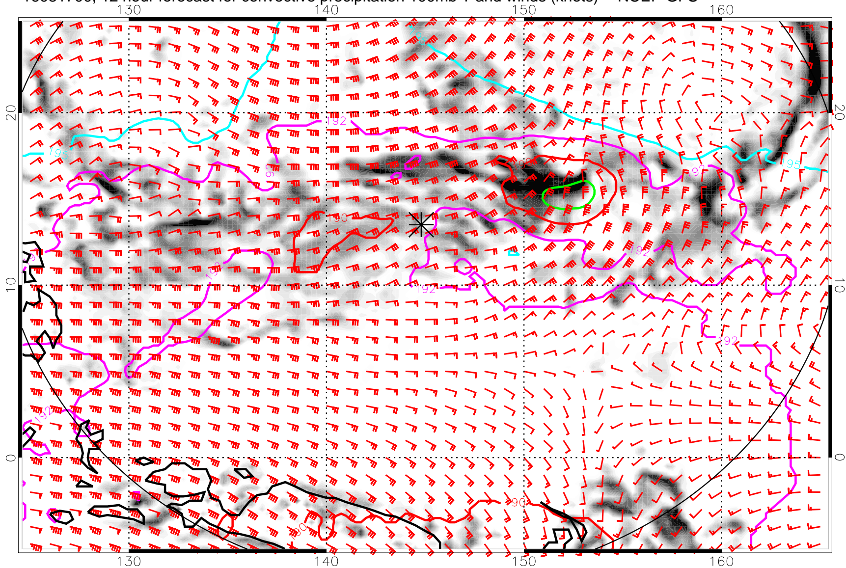
16081700, 12 hour forecast for convective precipitation 100mb T and winds (knots) -- NCEP GFS
