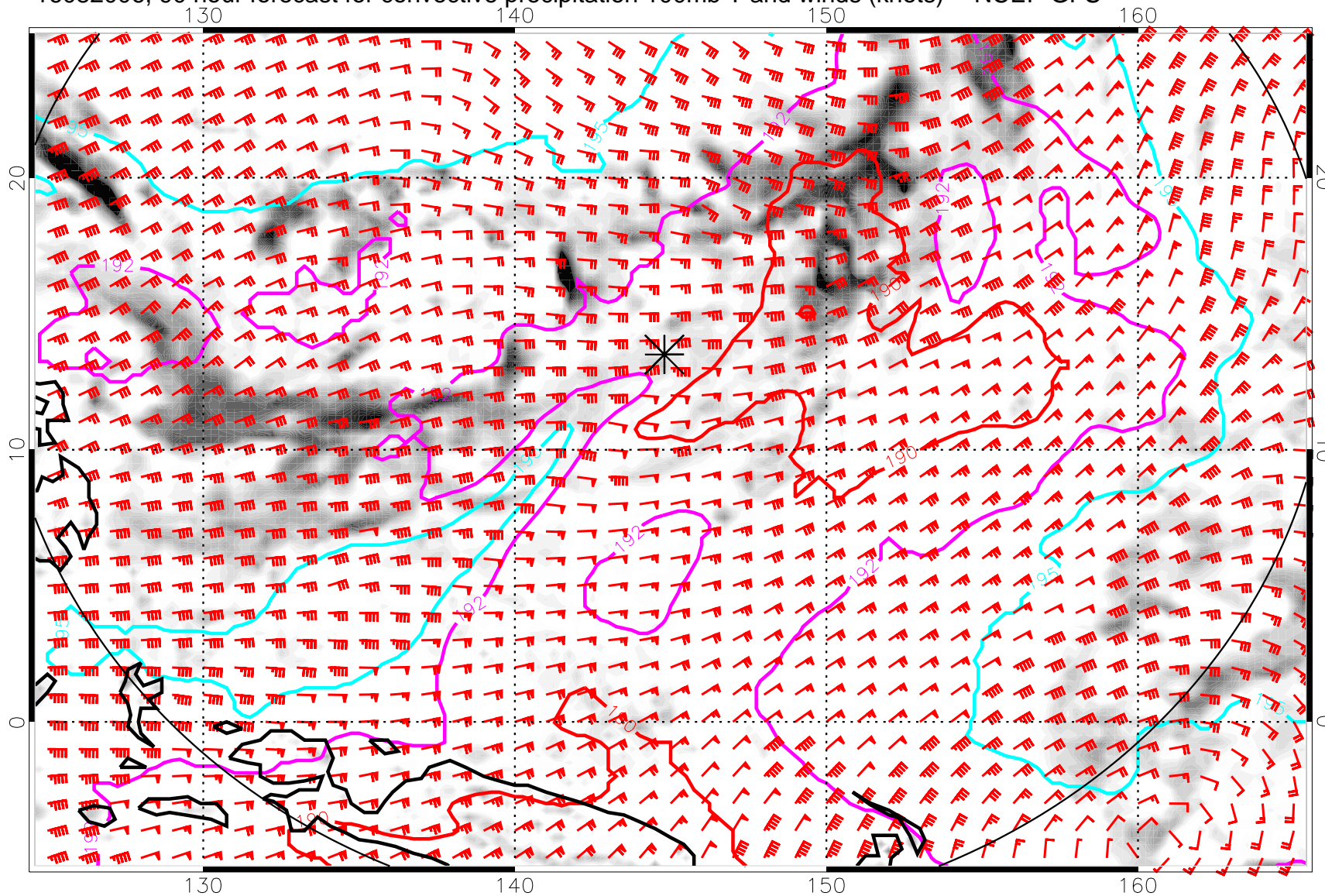
16082006, 90 hour forecast for convective precipitation 100mb T and winds (knots) -- NCEP GFS
