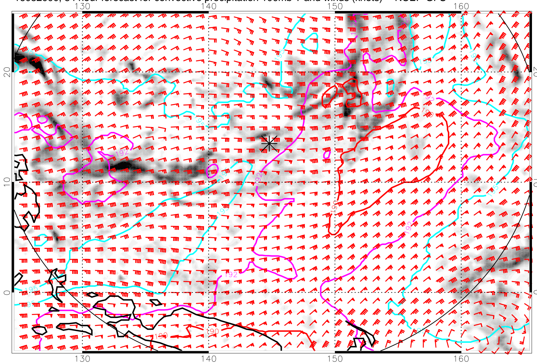
16082000, 84 hour forecast for convective precipitation 100mb T and winds (knots) -- NCEP GFS
