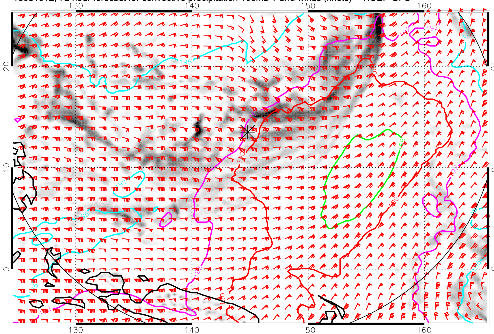
16081912, 72 hour forecast for convective precipitation 100mb T and winds (knots) -- NCEP GFS
