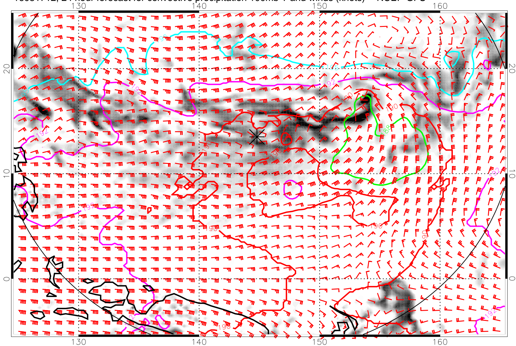
16081712, 24 hour forecast for convective precipitation 100mb T and winds (knots) -- NCEP GFS
