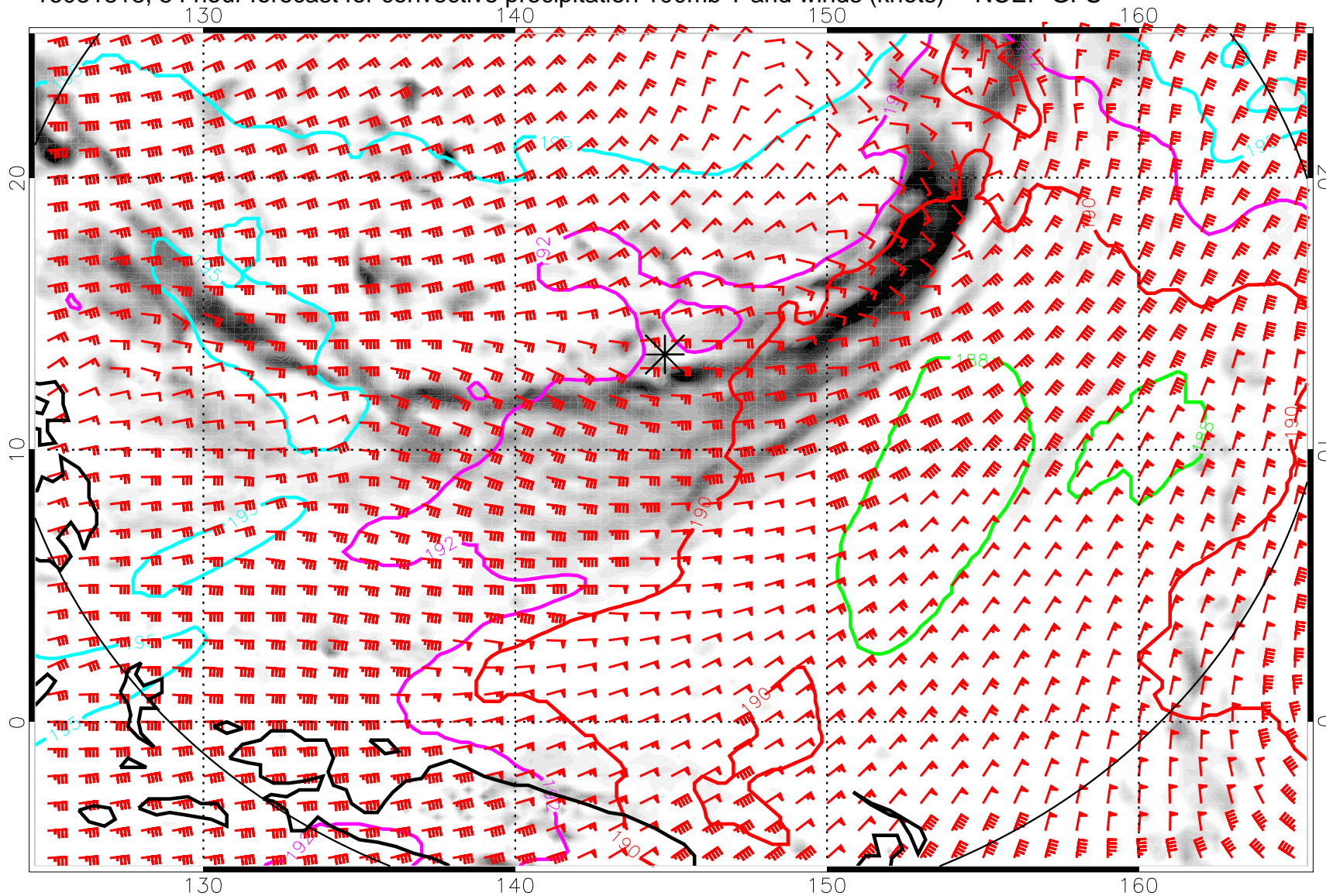
16081818, 54 hour forecast for convective precipitation 100mb T and winds (knots) -- NCEP GFS
