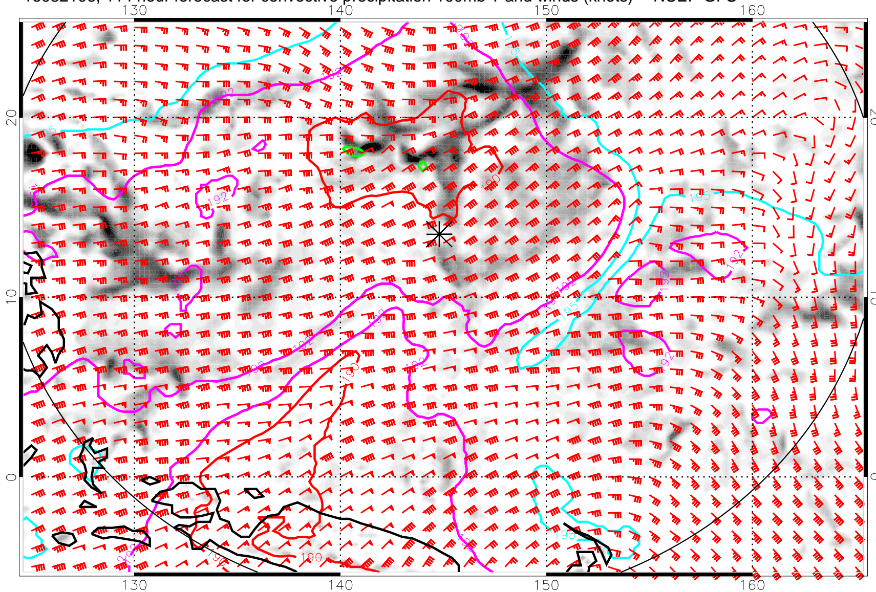
16082106, 114 hour forecast for convective precipitation 100mb T and winds (knots) -- NCEP GFS
