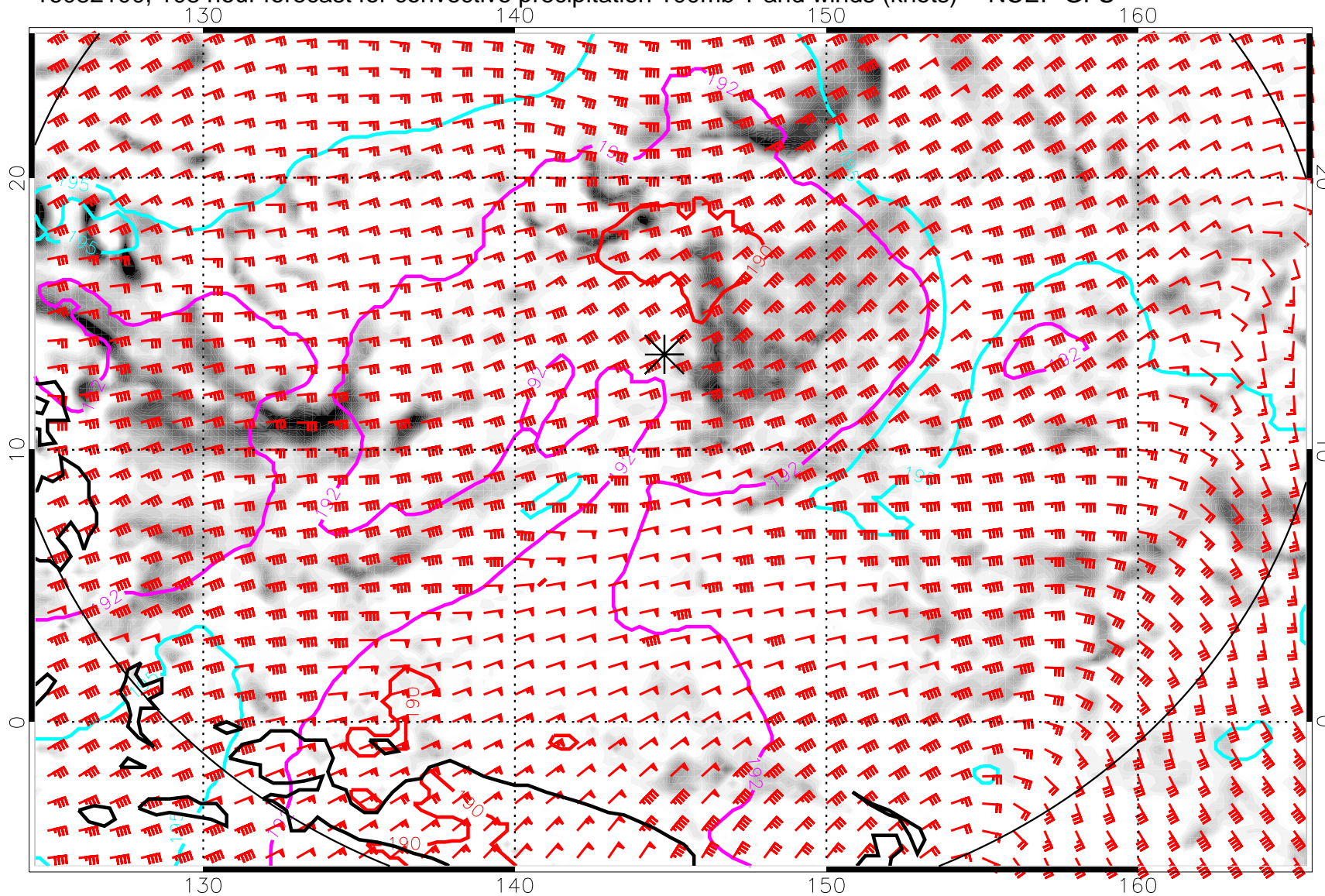
16082100, 108 hour forecast for convective precipitation 100mb T and winds (knots) -- NCEP GFS
