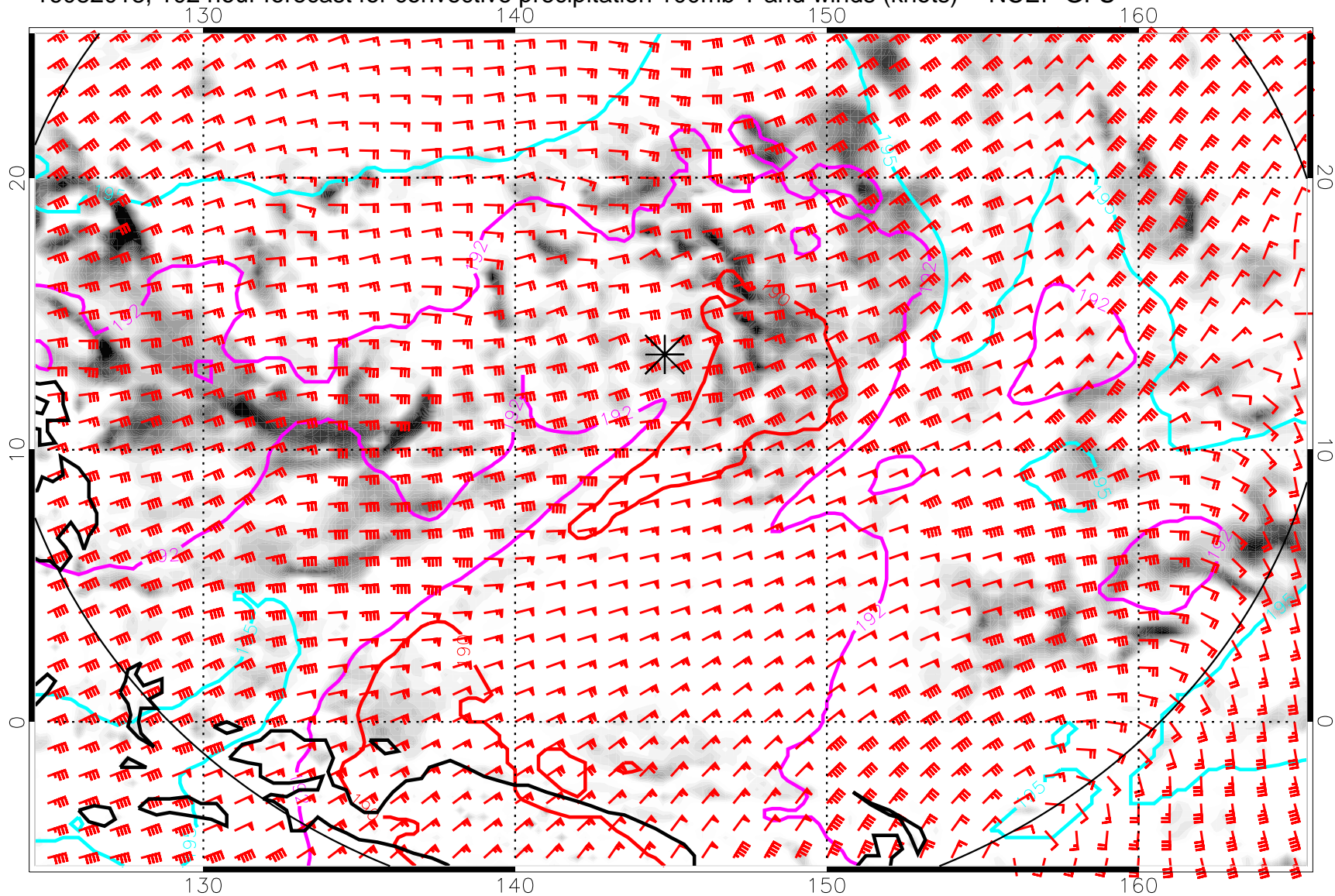
16082018, 102 hour forecast for convective precipitation 100mb T and winds (knots) -- NCEP GFS
