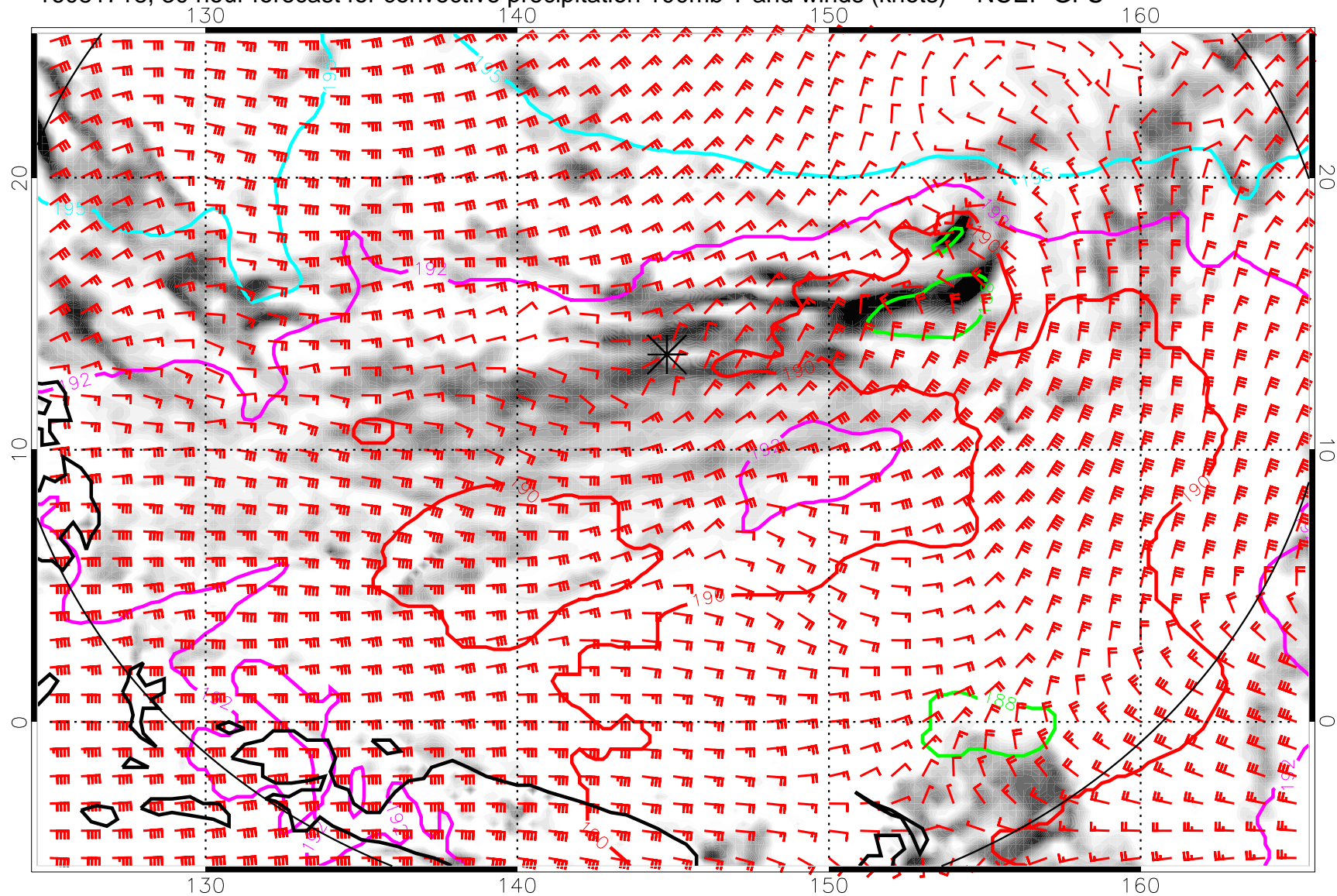
16081718, 30 hour forecast for convective precipitation 100mb T and winds (knots) -- NCEP GFS
