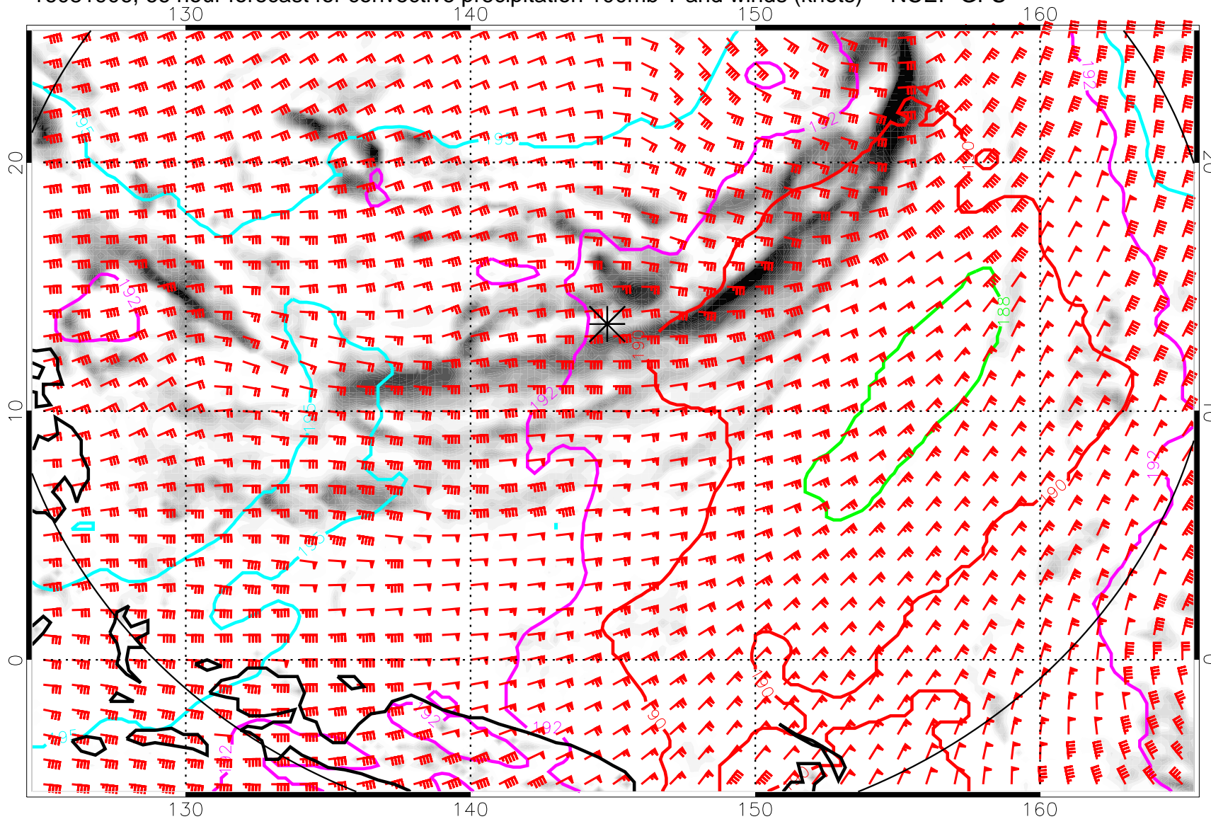
16081906, 66 hour forecast for convective precipitation 100mb T and winds (knots) -- NCEP GFS
