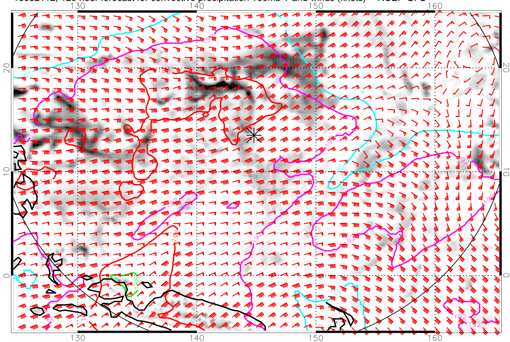
16082112, 120 hour forecast for convective precipitation 100mb T and winds (knots) -- NCEP GFS
