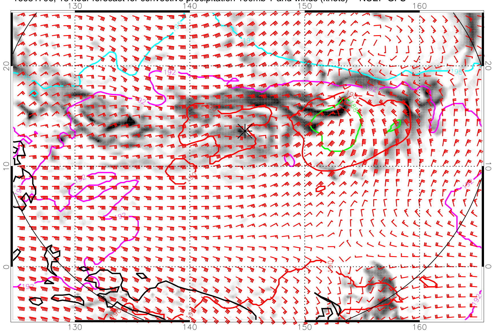
16081706, 18 hour forecast for convective precipitation 100mb T and winds (knots) -- NCEP GFS
