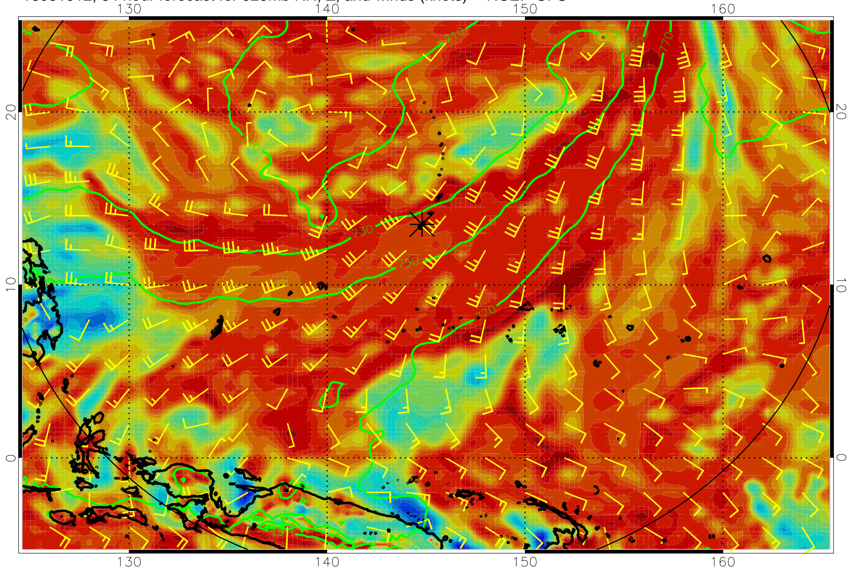
16081912, 84 hour forecast for 925mb RH, Z, and winds (knots) -- NCEP GFS
