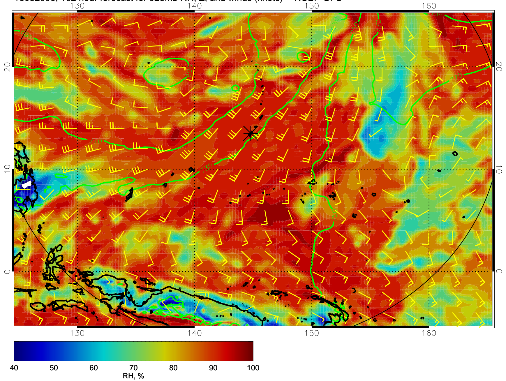
16082006, 102 hour forecast for 925mb RH, Z, and winds (knots) -- NCEP GFS
