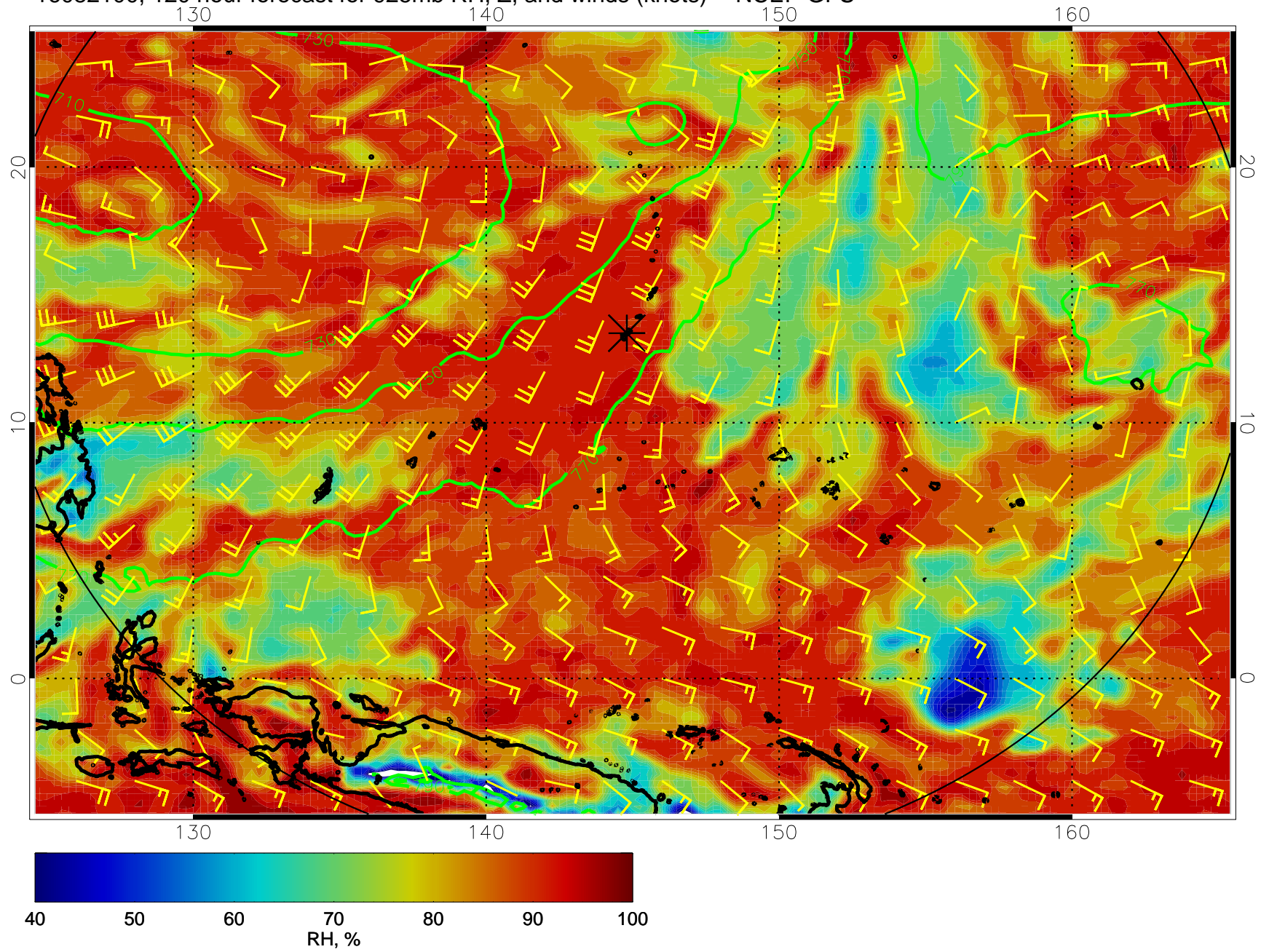
16082100, 120 hour forecast for 925mb RH, Z, and winds (knots) -- NCEP GFS
