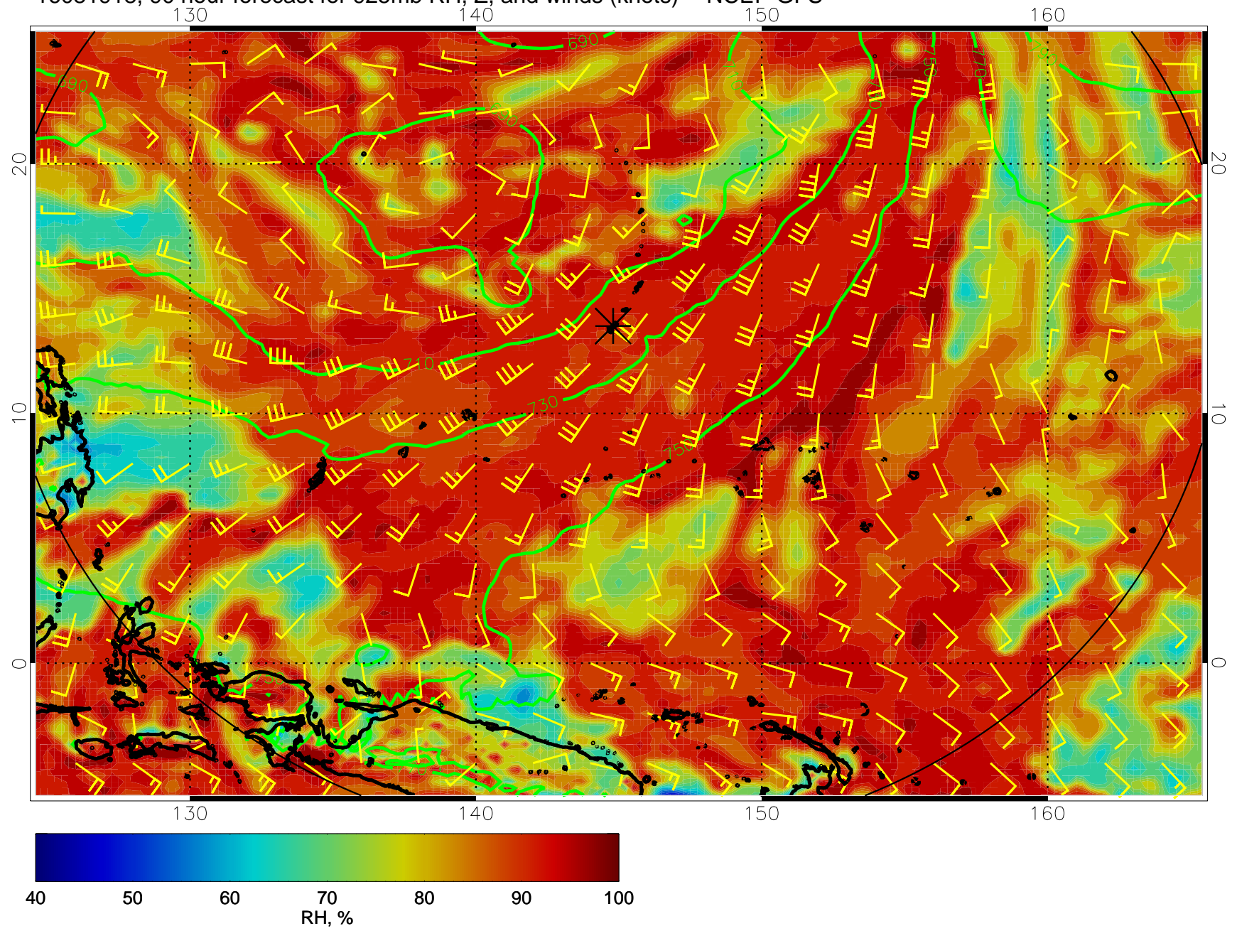
16081918, 90 hour forecast for 925mb RH, Z, and winds (knots) -- NCEP GFS
