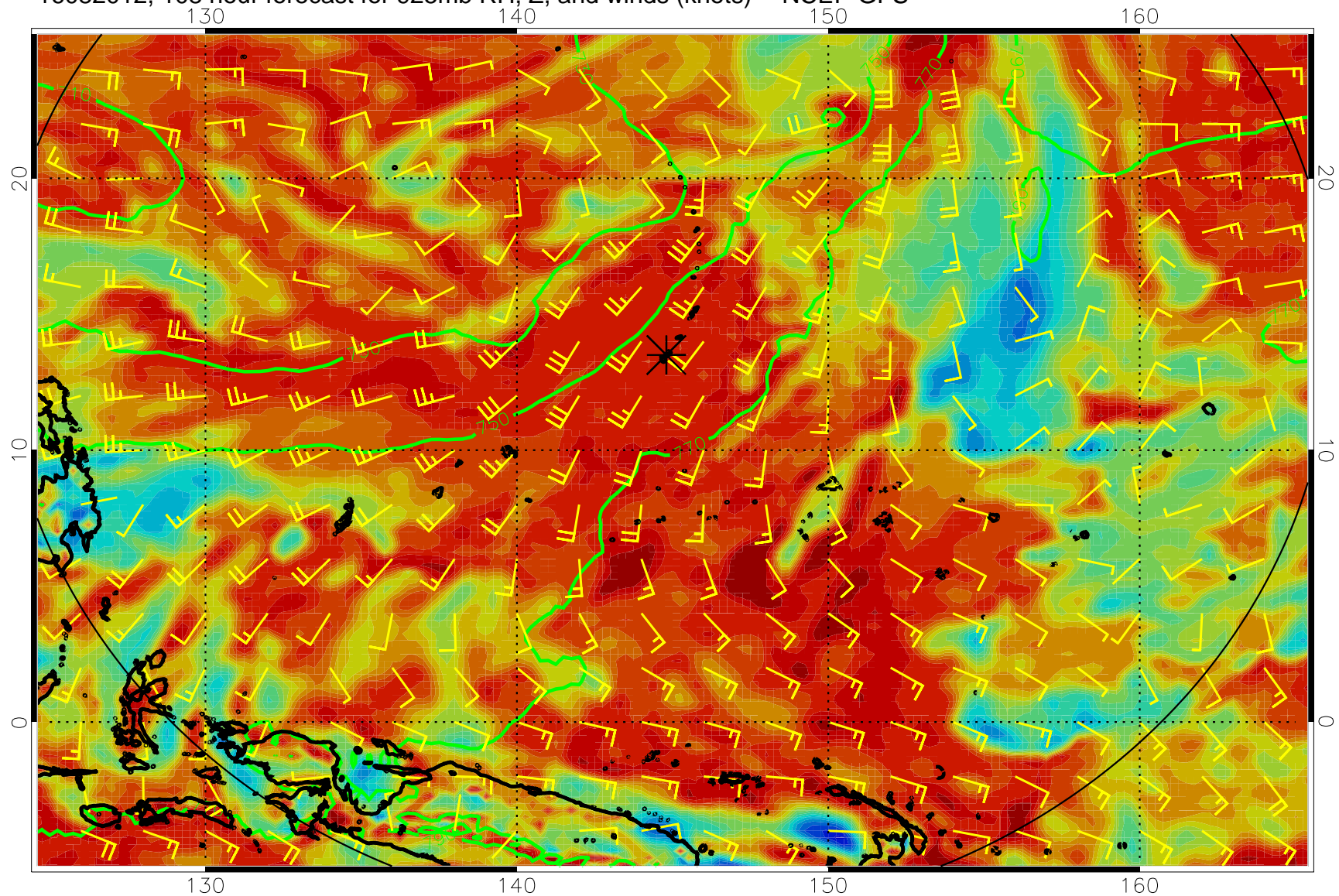
16082012, 108 hour forecast for 925mb RH, Z, and winds (knots) -- NCEP GFS
