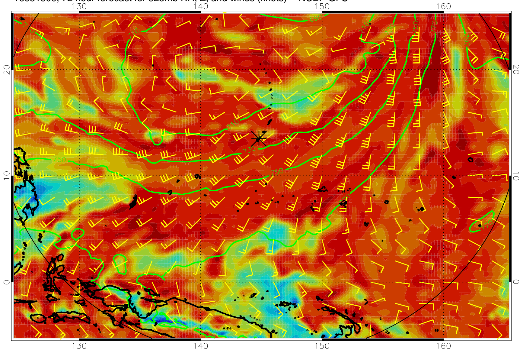
16081900, 72 hour forecast for 925mb RH, Z, and winds (knots) -- NCEP GFS
