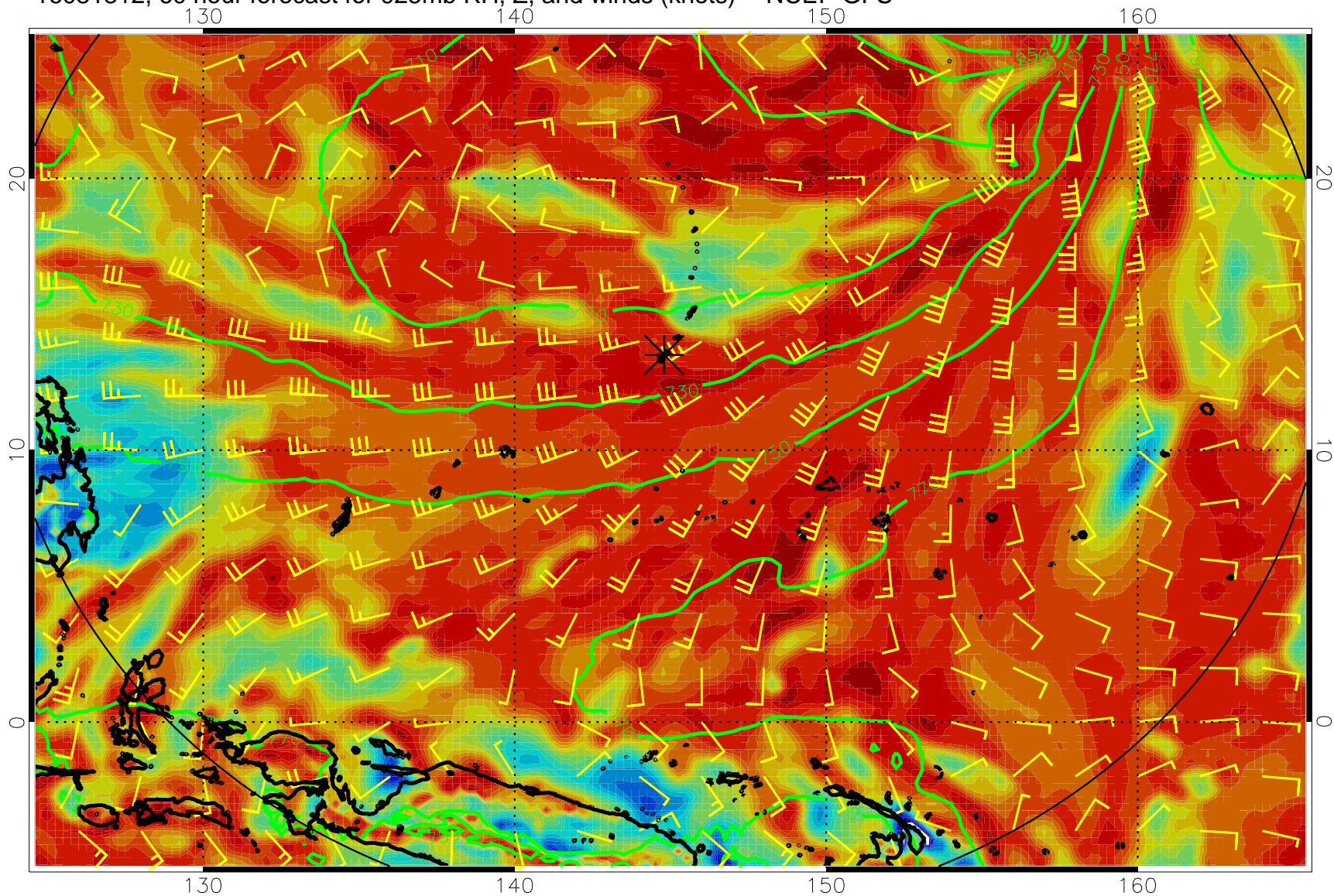
16081812, 60 hour forecast for 925mb RH, Z, and winds (knots) -- NCEP GFS
