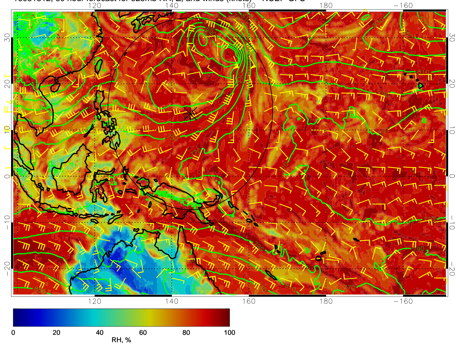
16081812, 60 hour forecast for 925mb RH, Z, and winds (knots) -- NCEP GFS
