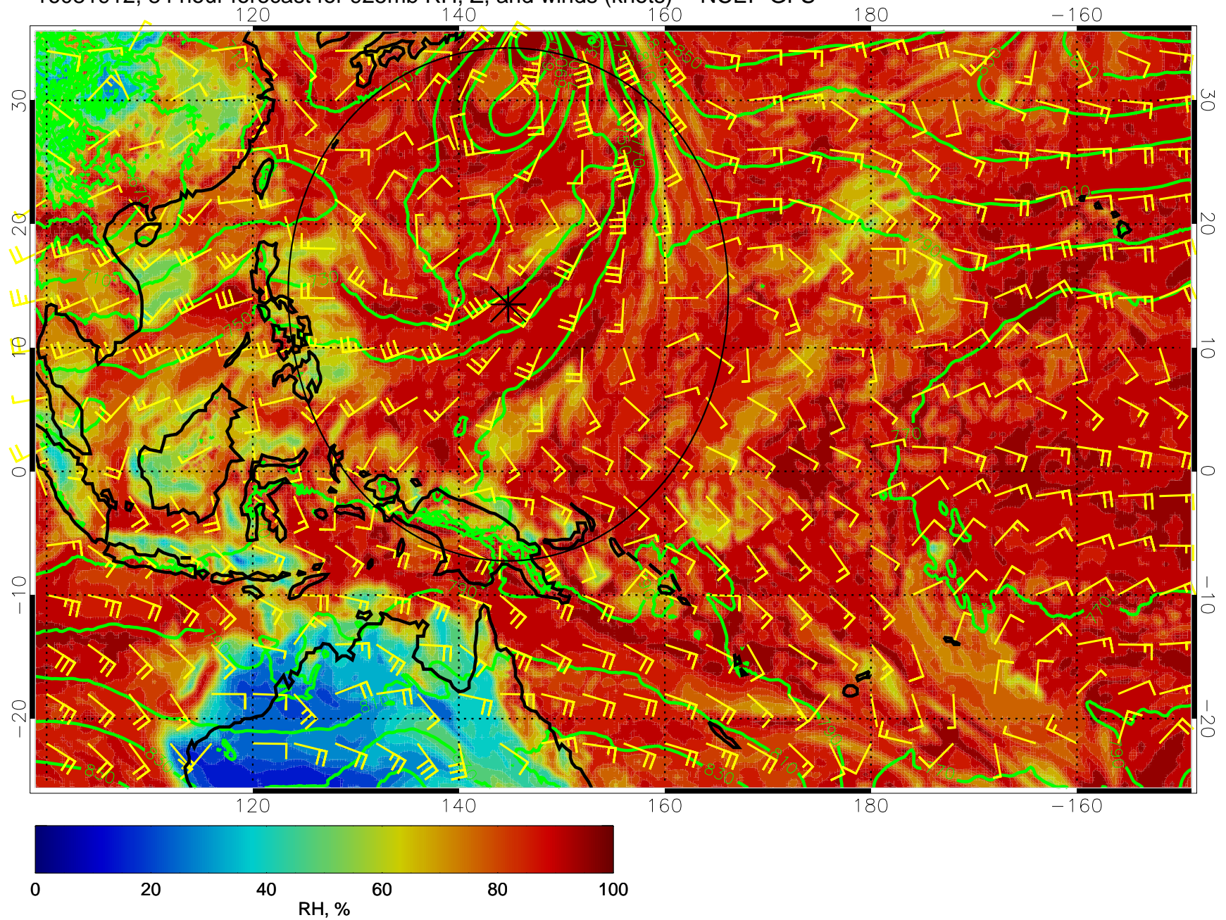
16081912, 84 hour forecast for 925mb RH, Z, and winds (knots) -- NCEP GFS
