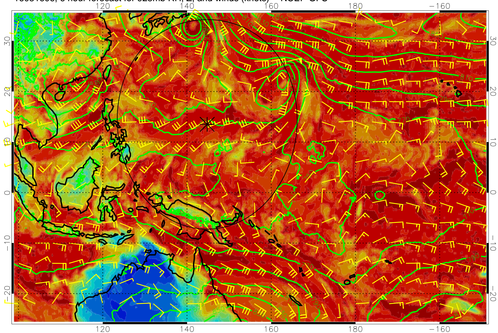
16081606, 6 hour forecast for 925mb RH, Z, and winds (knots) -- NCEP GFS
