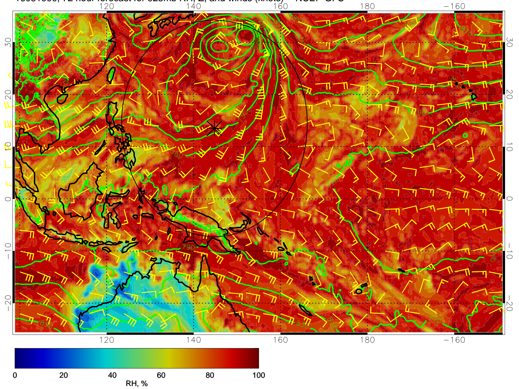
16081900, 72 hour forecast for 925mb RH, Z, and winds (knots) -- NCEP GFS
