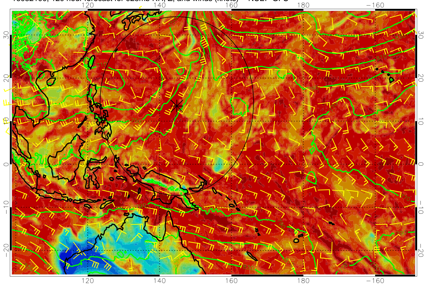
16082100, 120 hour forecast for 925mb RH, Z, and winds (knots) -- NCEP GFS
