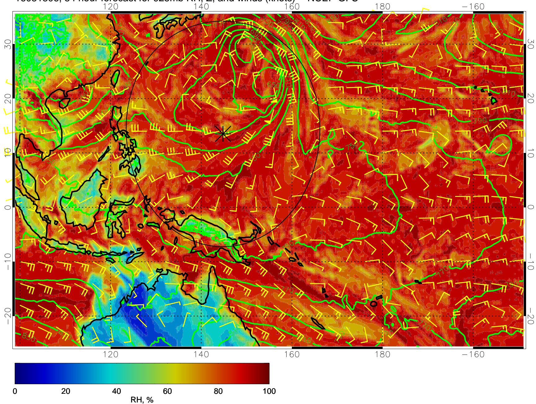
16081806, 54 hour forecast for 925mb RH, Z, and winds (knots) -- NCEP GFS
