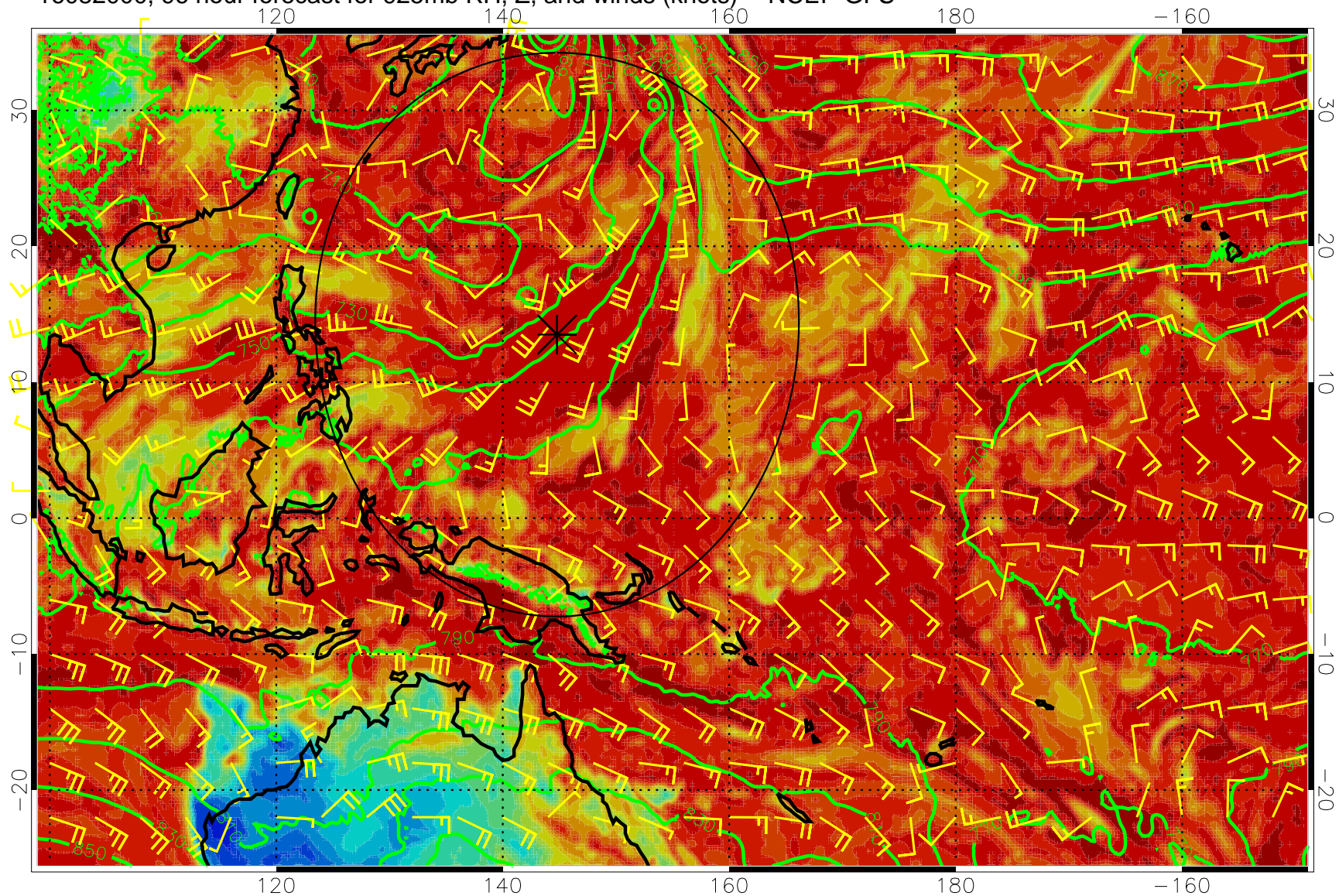
16082000, 96 hour forecast for 925mb RH, Z, and winds (knots) -- NCEP GFS
