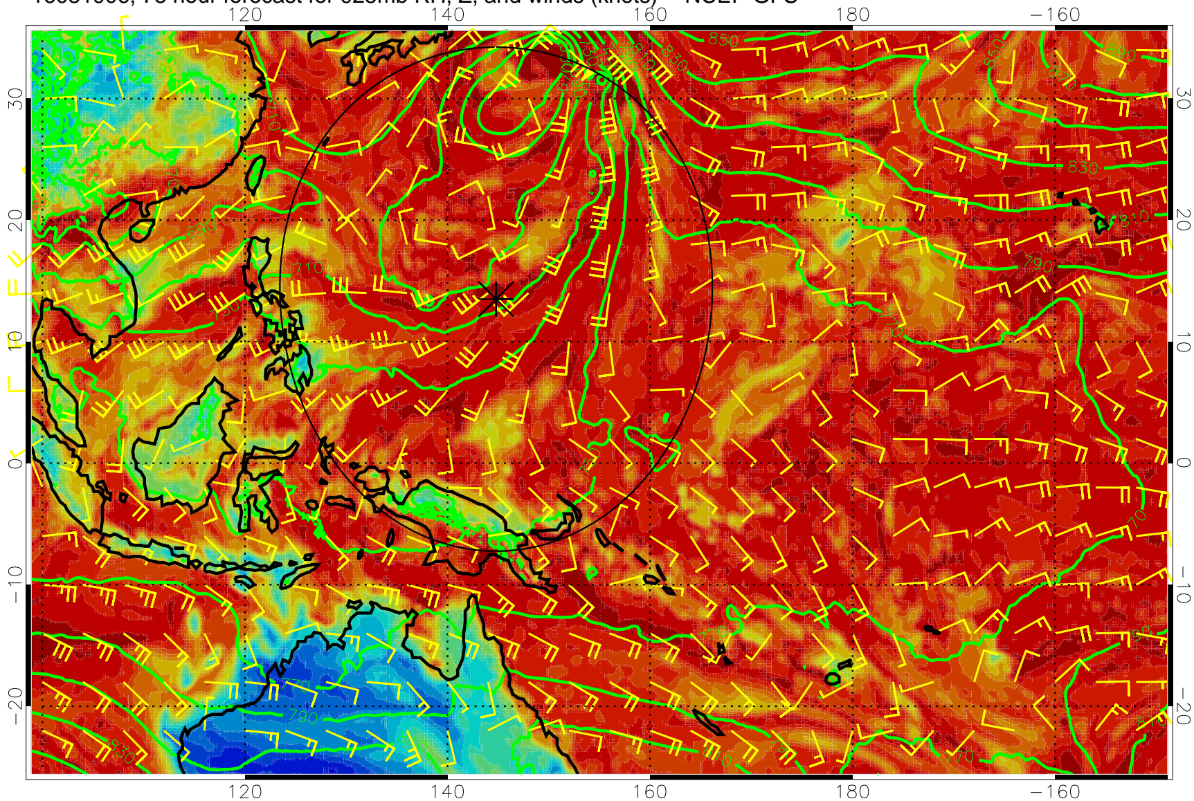
16081906, 78 hour forecast for 925mb RH, Z, and winds (knots) -- NCEP GFS
