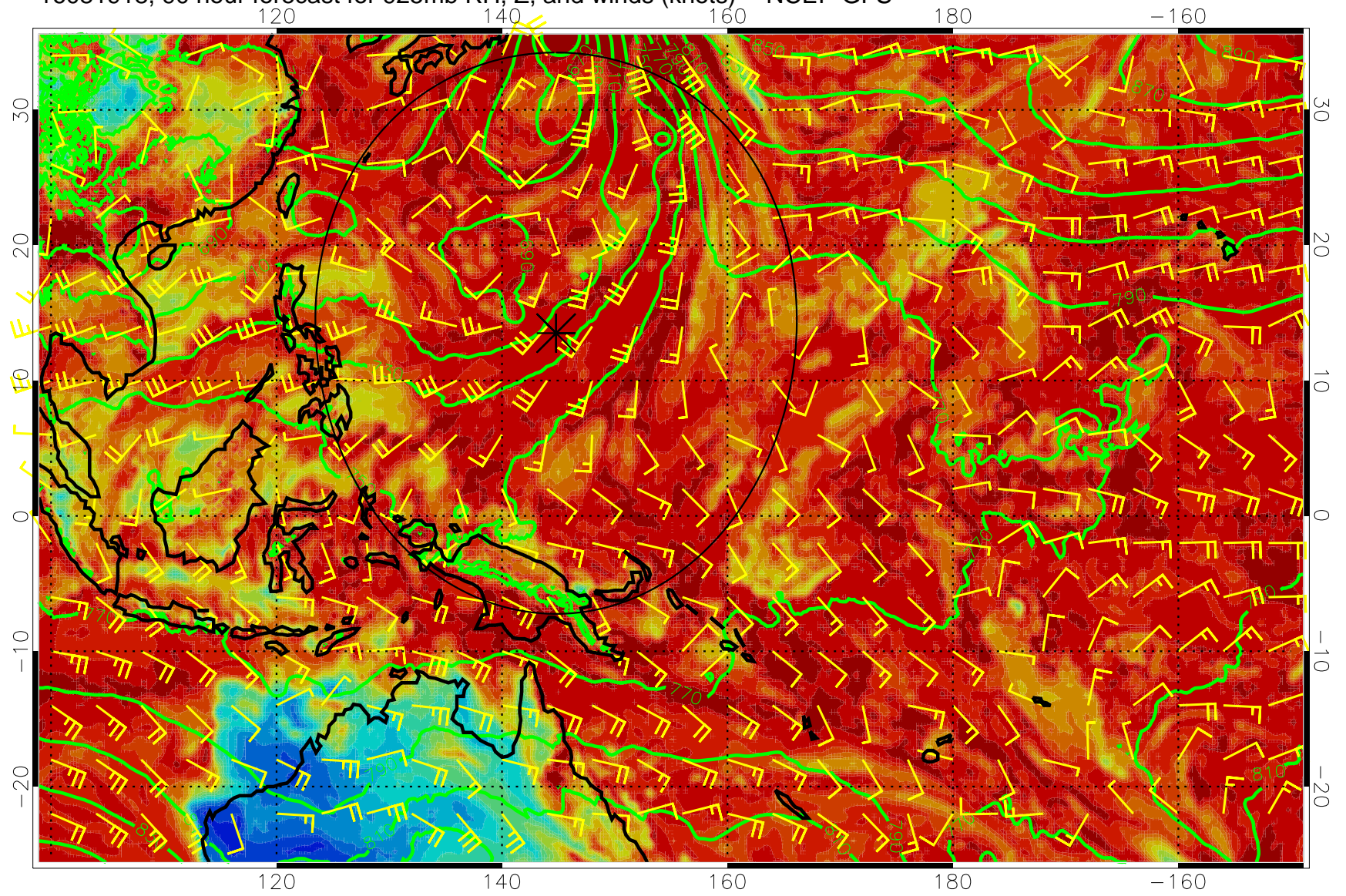
16081918, 90 hour forecast for 925mb RH, Z, and winds (knots) -- NCEP GFS
