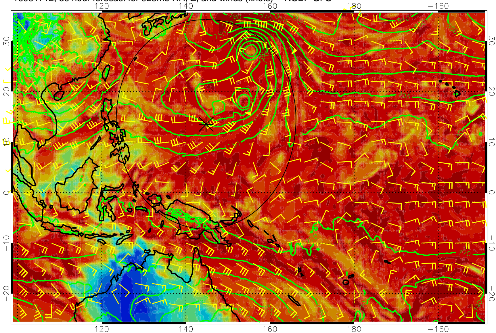
16081712, 36 hour forecast for 925mb RH, Z, and winds (knots) -- NCEP GFS
