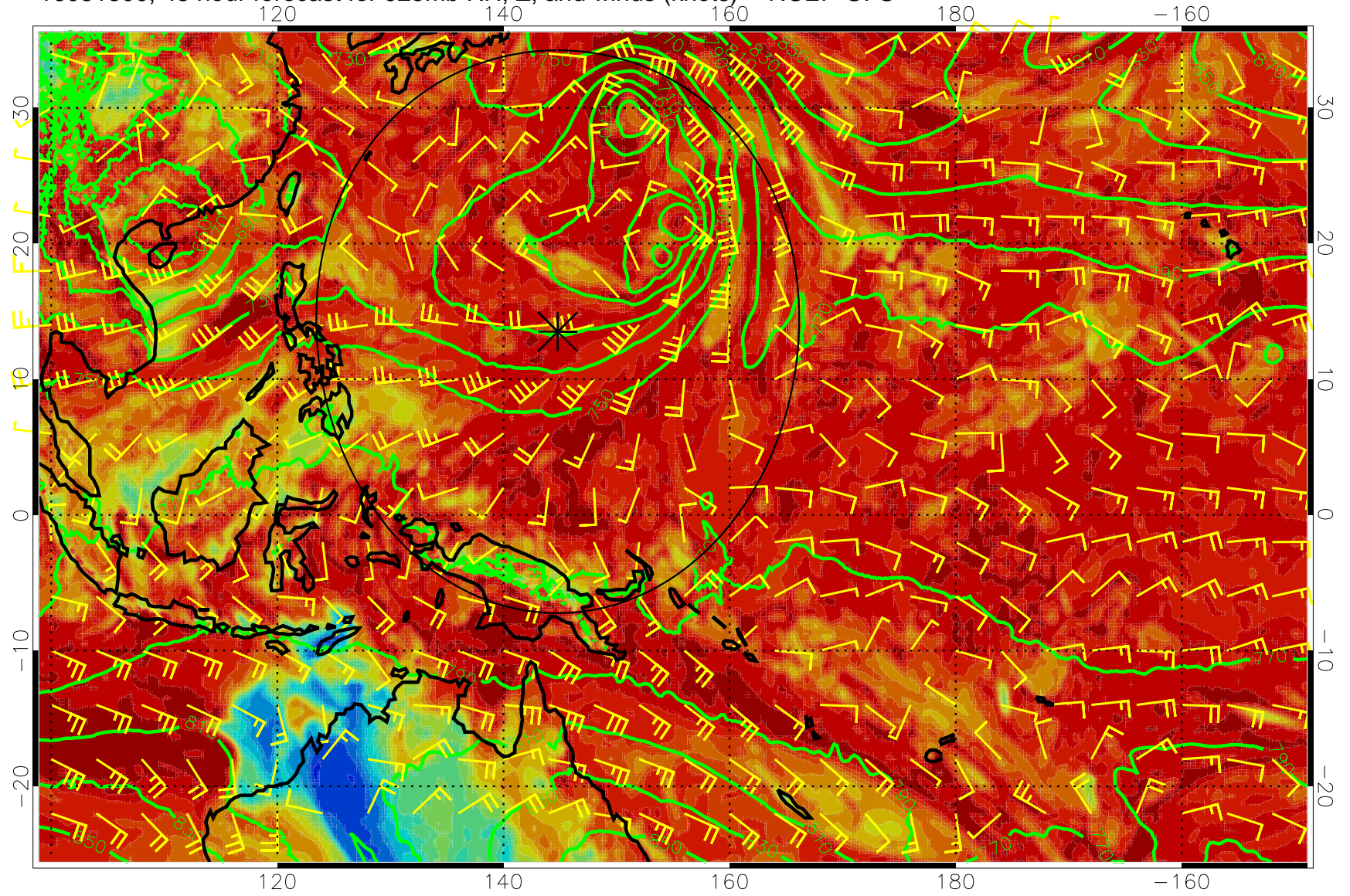
16081800, 48 hour forecast for 925mb RH, Z, and winds (knots) -- NCEP GFS
