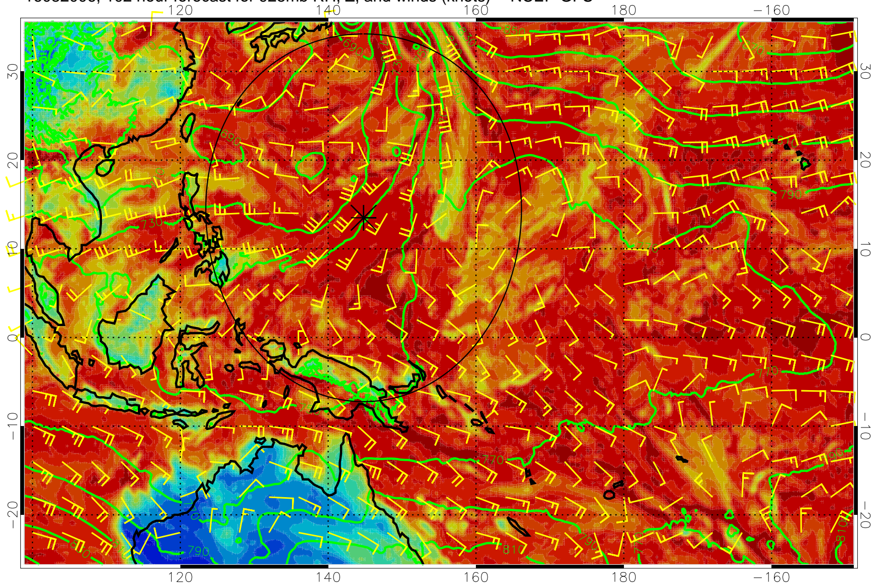
16082006, 102 hour forecast for 925mb RH, Z, and winds (knots) -- NCEP GFS
