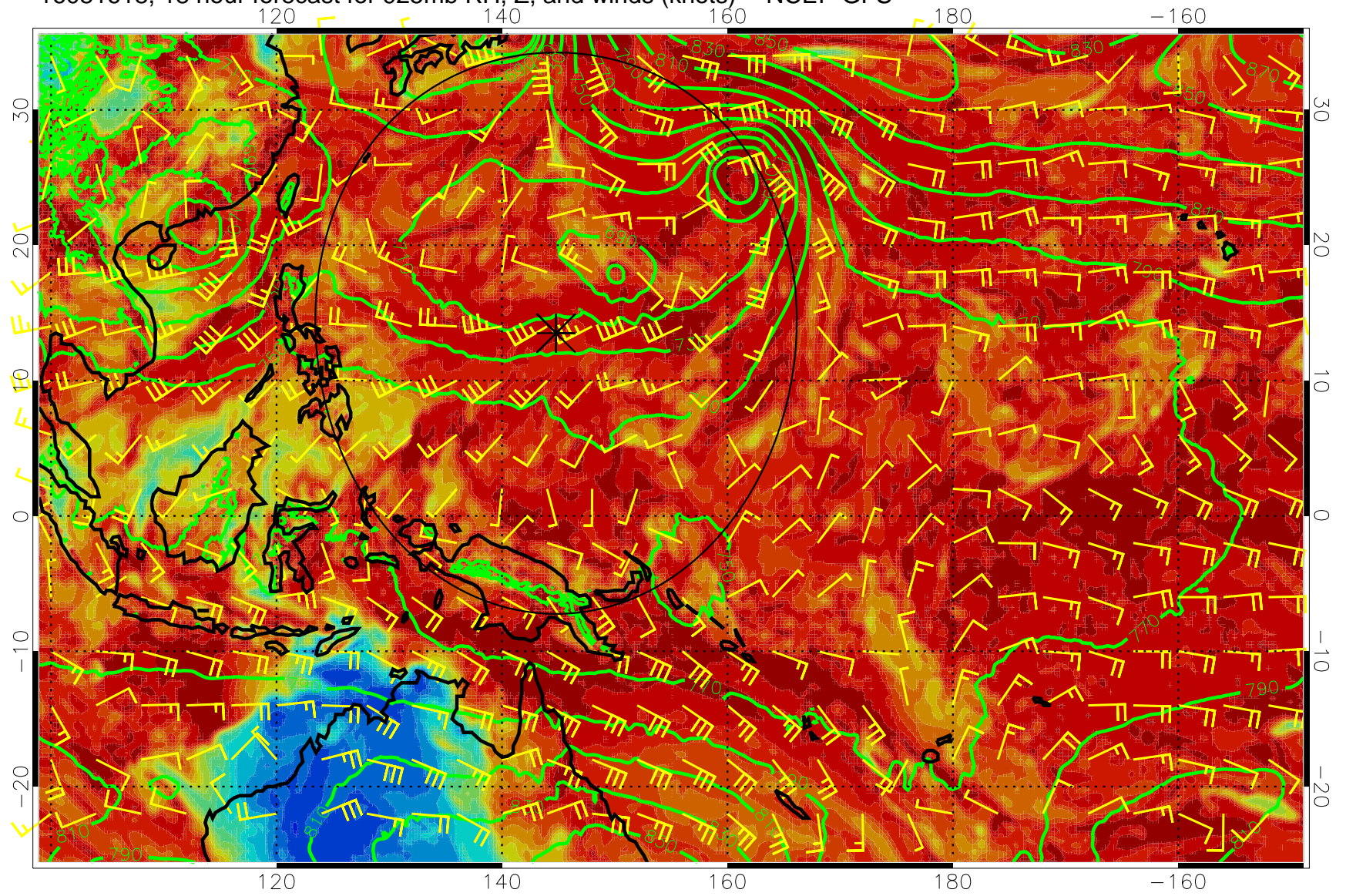
16081618, 18 hour forecast for 925mb RH, Z, and winds (knots) -- NCEP GFS
