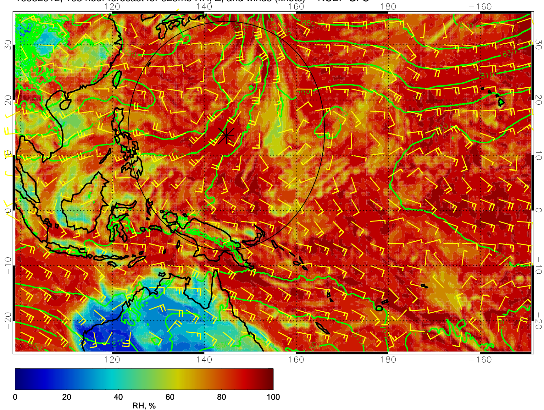
16082012, 108 hour forecast for 925mb RH, Z, and winds (knots) -- NCEP GFS
