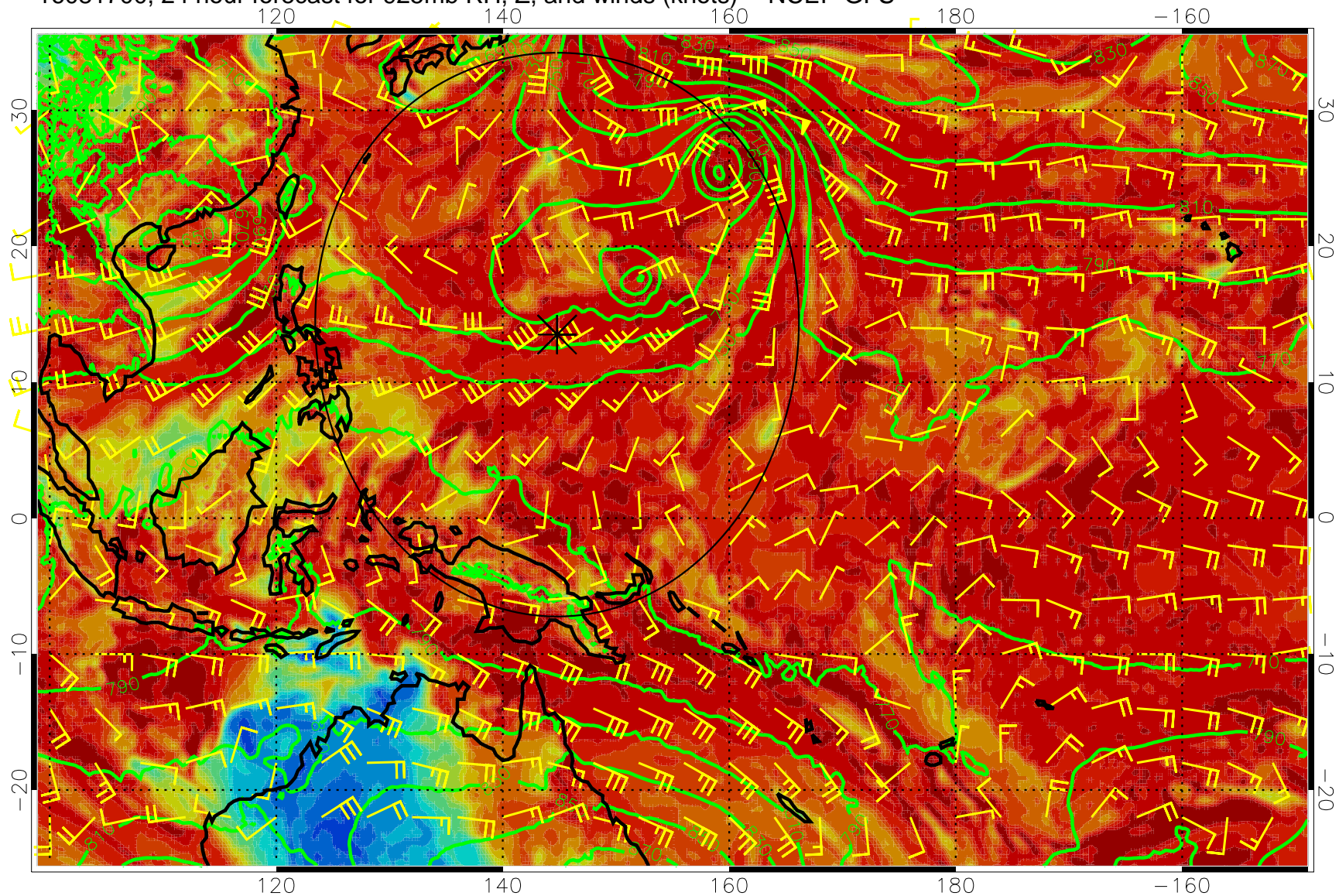
16081700, 24 hour forecast for 925mb RH, Z, and winds (knots) -- NCEP GFS
