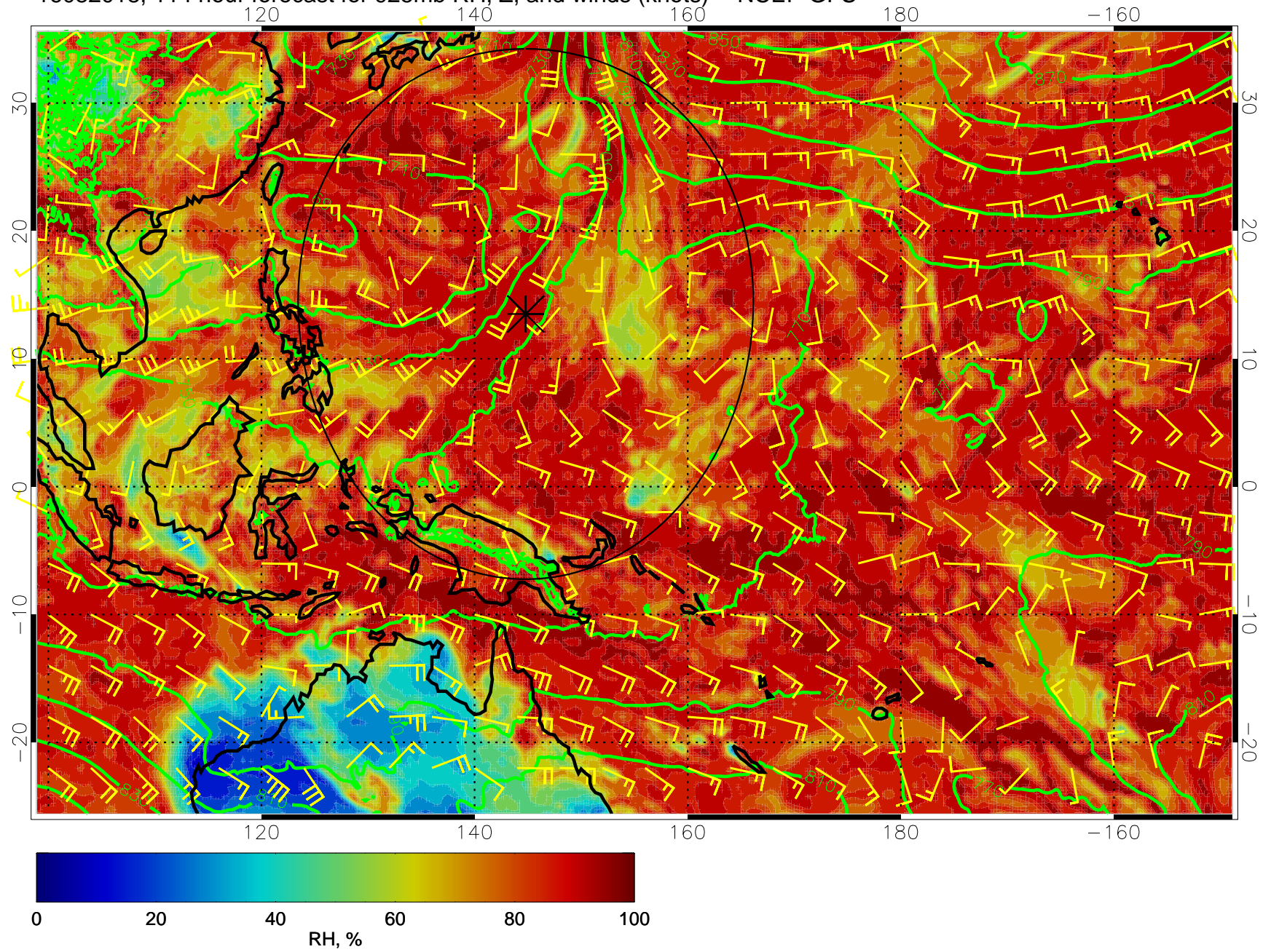
16082018, 114 hour forecast for 925mb RH, Z, and winds (knots) -- NCEP GFS
