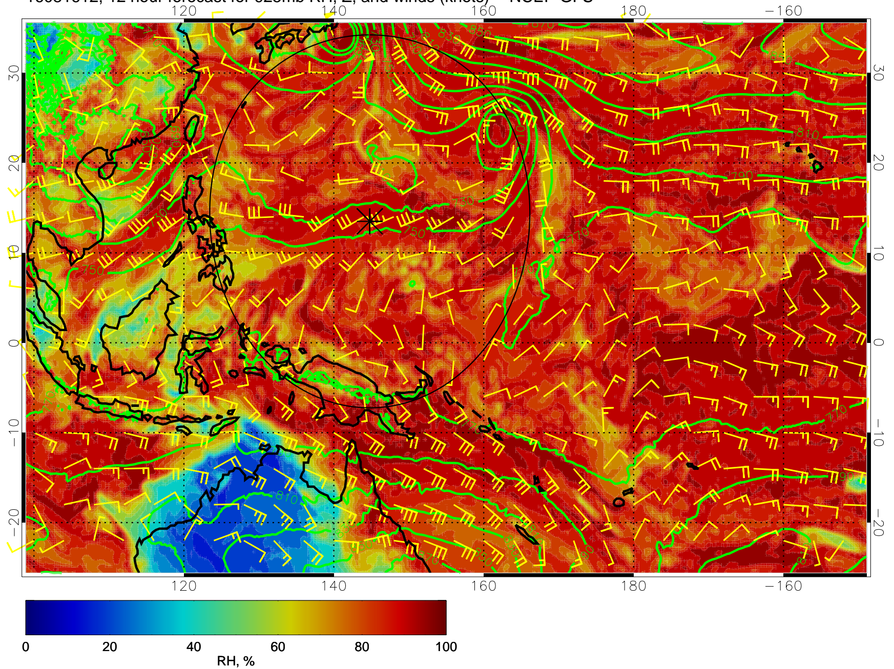
16081612, 12 hour forecast for 925mb RH, Z, and winds (knots) -- NCEP GFS
