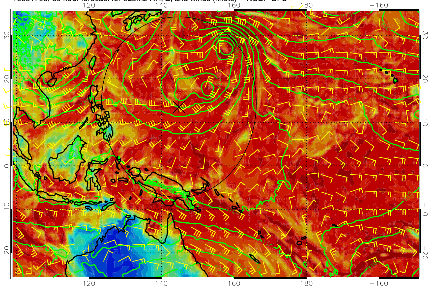
16081706, 30 hour forecast for 925mb RH, Z, and winds (knots) -- NCEP GFS
