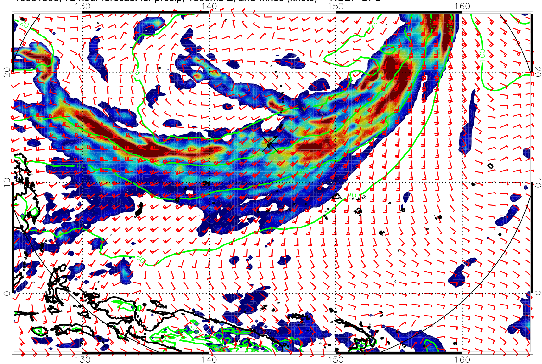
16081900, 72 hour forecast for precip, 1000mb Z, and winds (knots) -- NCEP GFS
