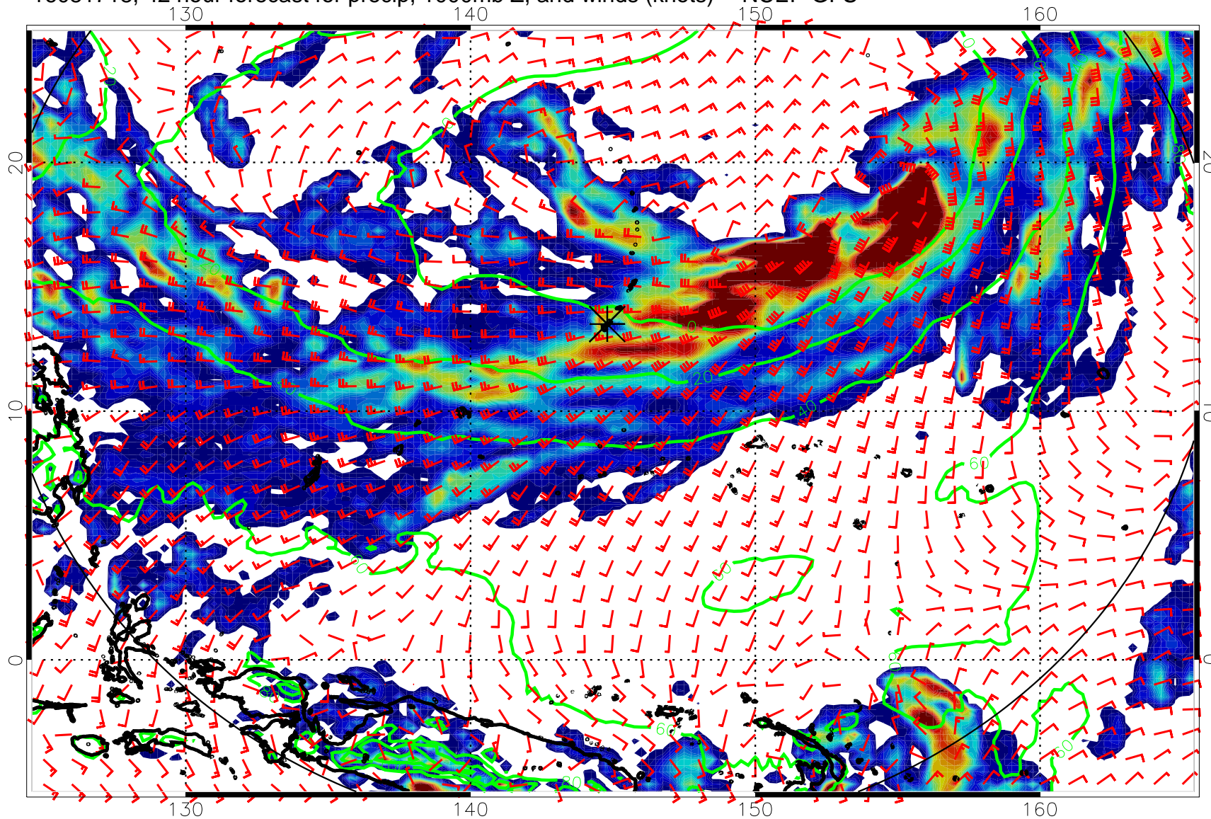
16081718, 42 hour forecast for precip, 1000mb Z, and winds (knots) -- NCEP GFS
