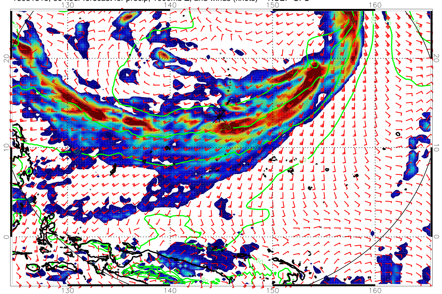
16081818, 66 hour forecast for precip, 1000mb Z, and winds (knots) -- NCEP GFS
