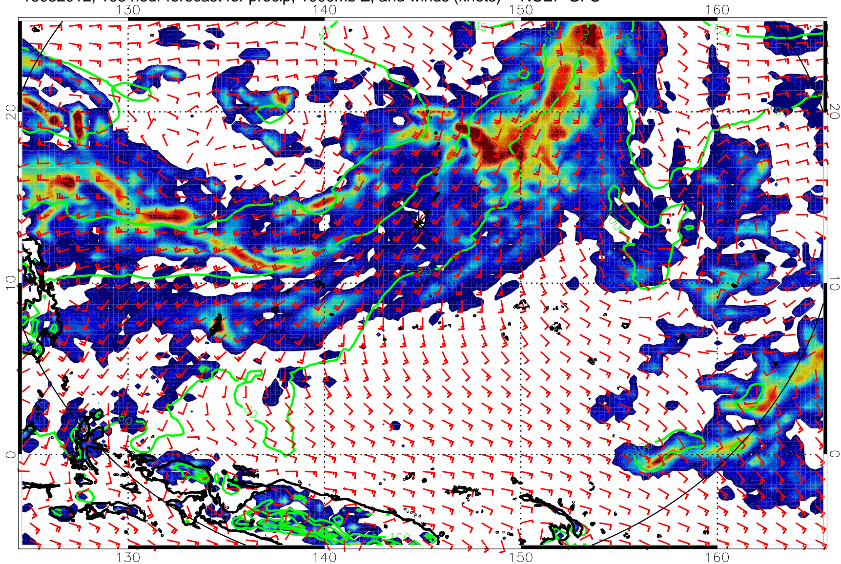
16082012, 108 hour forecast for precip, 1000mb Z, and winds (knots) -- NCEP GFS
