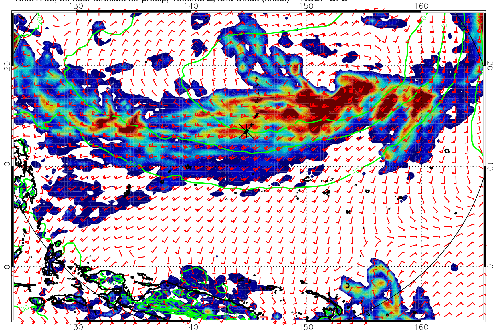
16081706, 30 hour forecast for precip, 1000mb Z, and winds (knots) -- NCEP GFS
