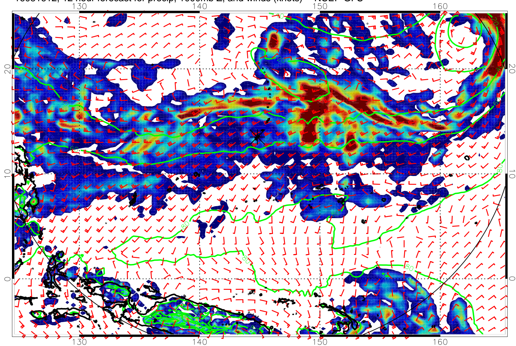
16081612, 12 hour forecast for precip, 1000mb Z, and winds (knots) -- NCEP GFS
