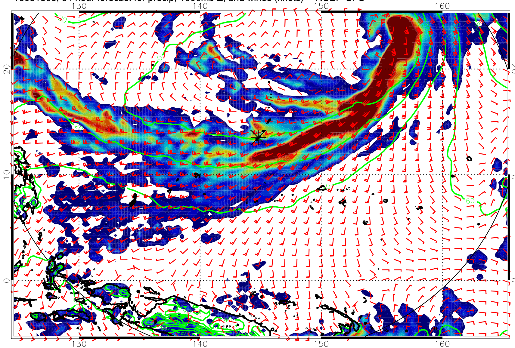
16081806, 54 hour forecast for precip, 1000mb Z, and winds (knots) -- NCEP GFS
