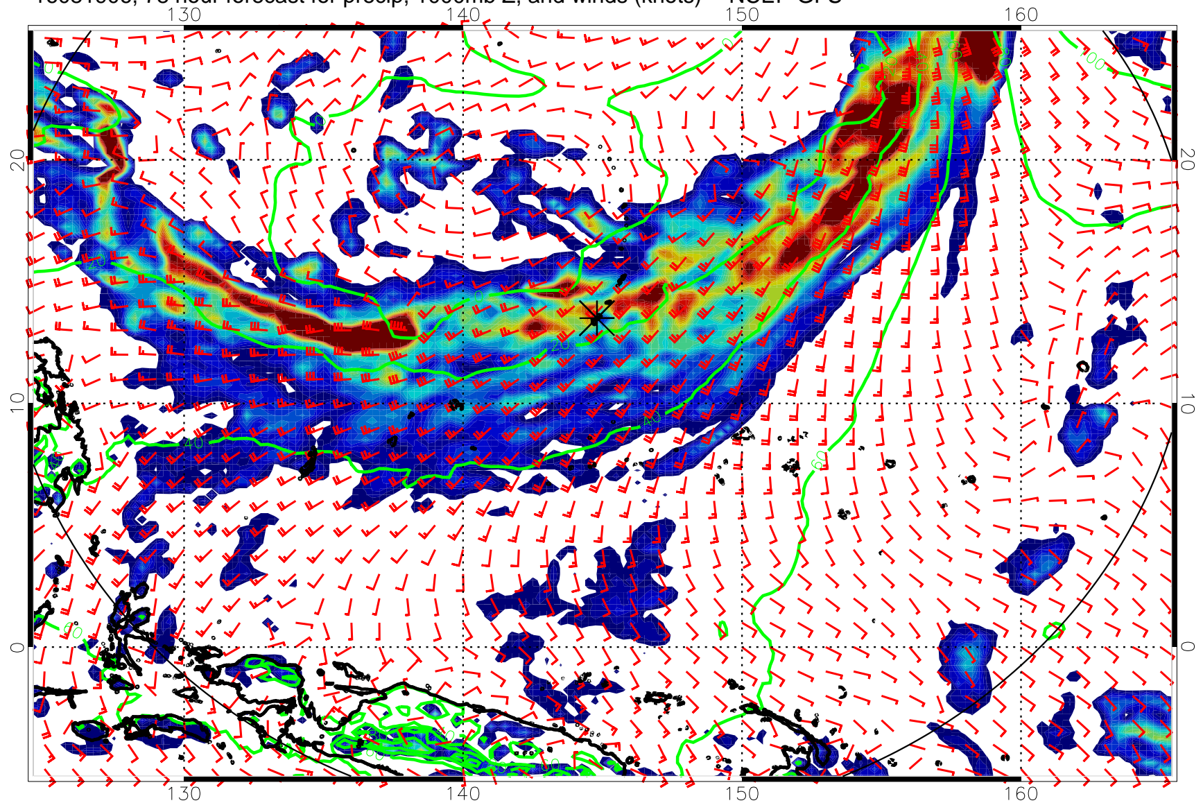
16081906, 78 hour forecast for precip, 1000mb Z, and winds (knots) -- NCEP GFS
