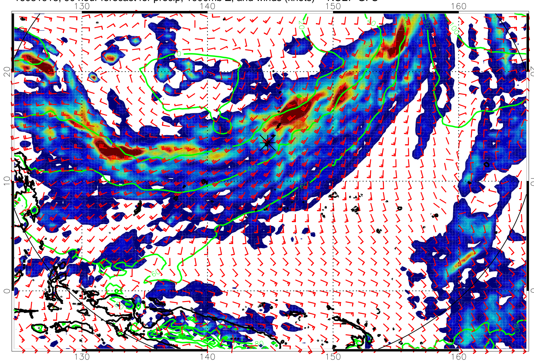
16081918, 90 hour forecast for precip, 1000mb Z, and winds (knots) -- NCEP GFS
