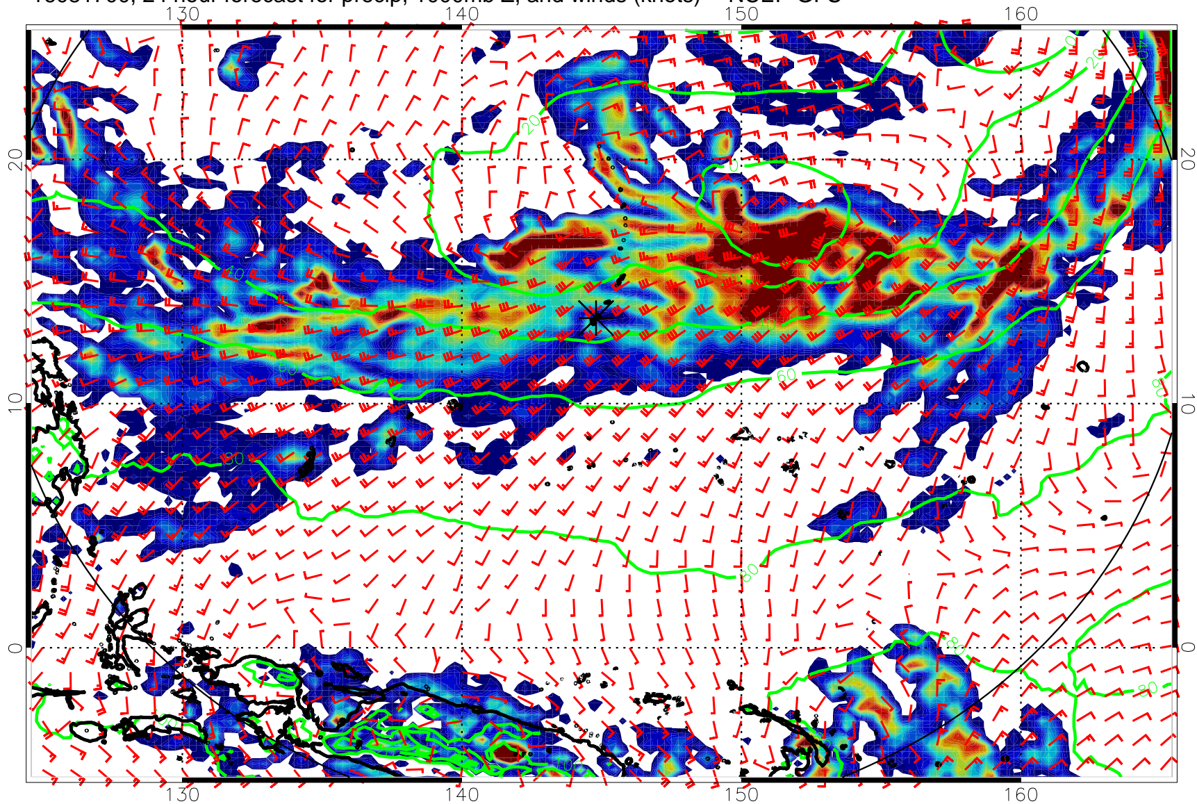
16081700, 24 hour forecast for precip, 1000mb Z, and winds (knots) -- NCEP GFS
