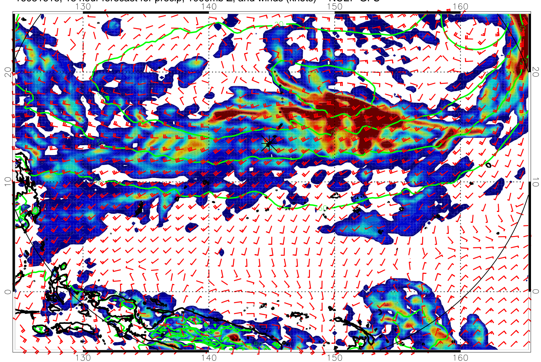
16081618, 18 hour forecast for precip, 1000mb Z, and winds (knots) -- NCEP GFS
