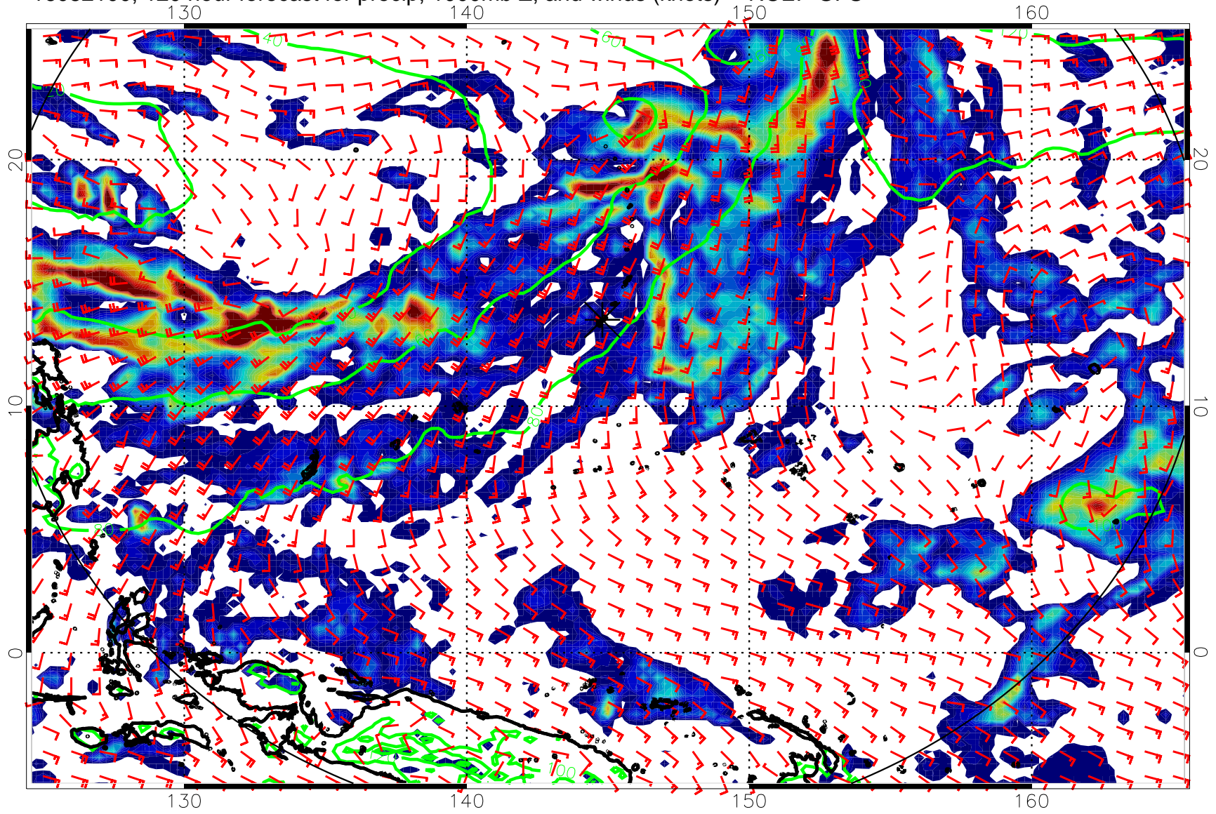
16082100, 120 hour forecast for precip, 1000mb Z, and winds (knots) -- NCEP GFS
