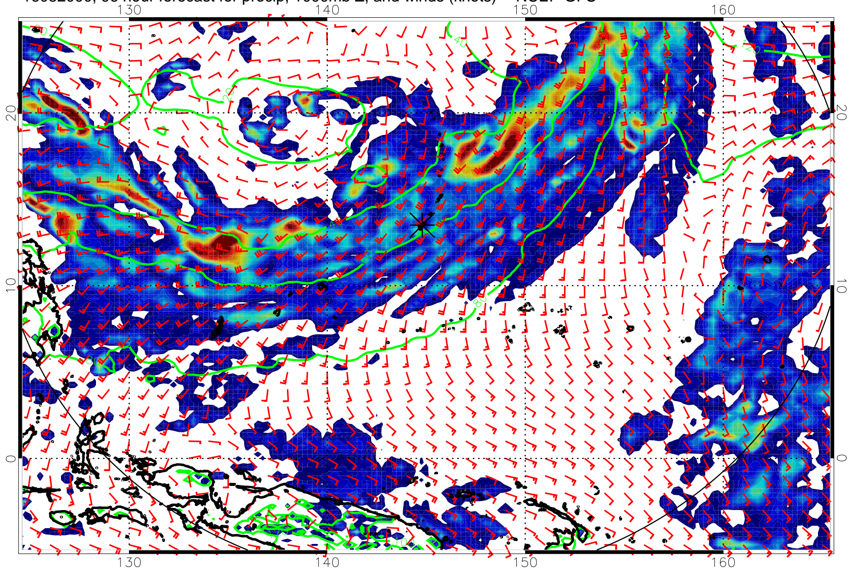
16082000, 96 hour forecast for precip, 1000mb Z, and winds (knots) -- NCEP GFS
