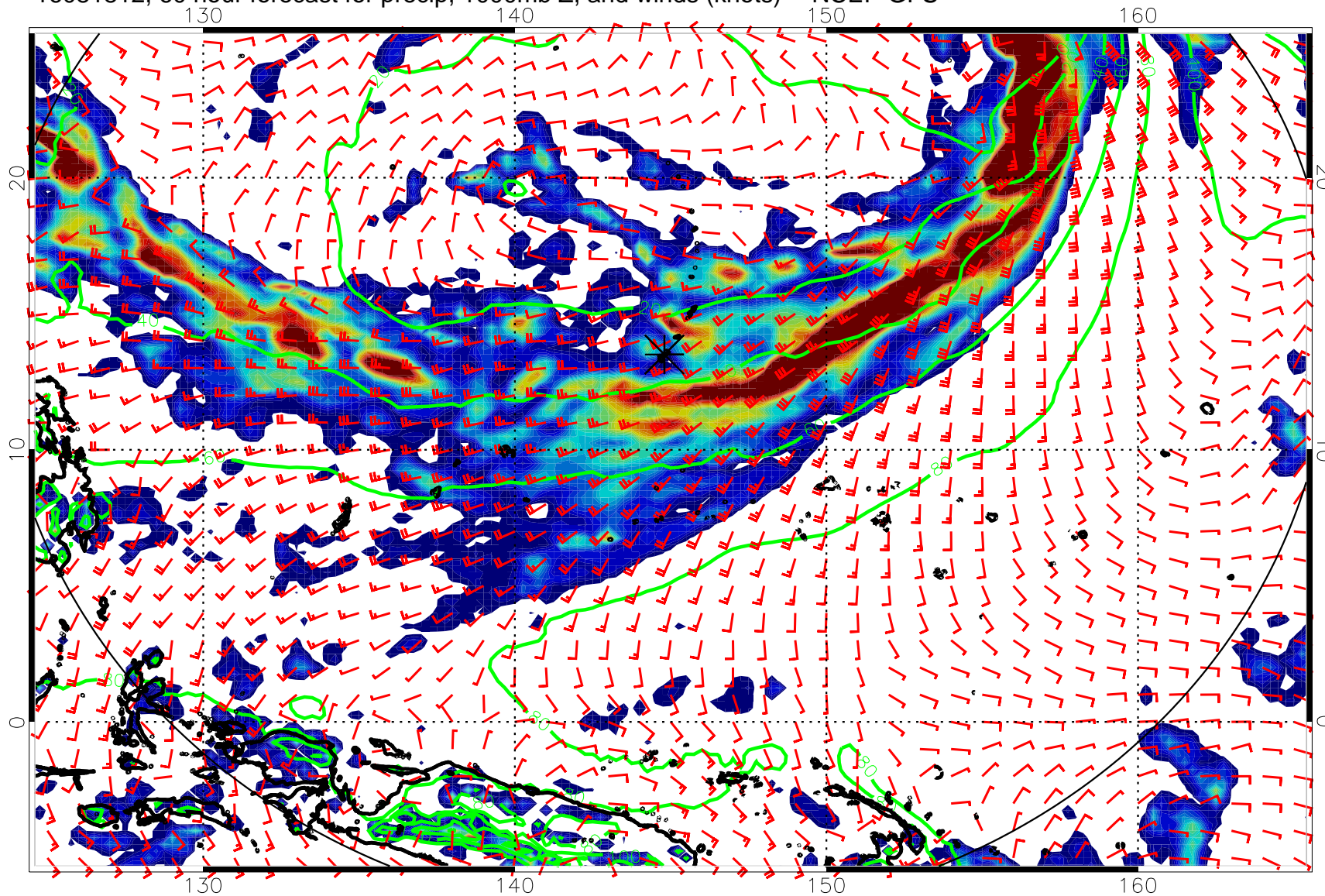
16081812, 60 hour forecast for precip, 1000mb Z, and winds (knots) -- NCEP GFS
