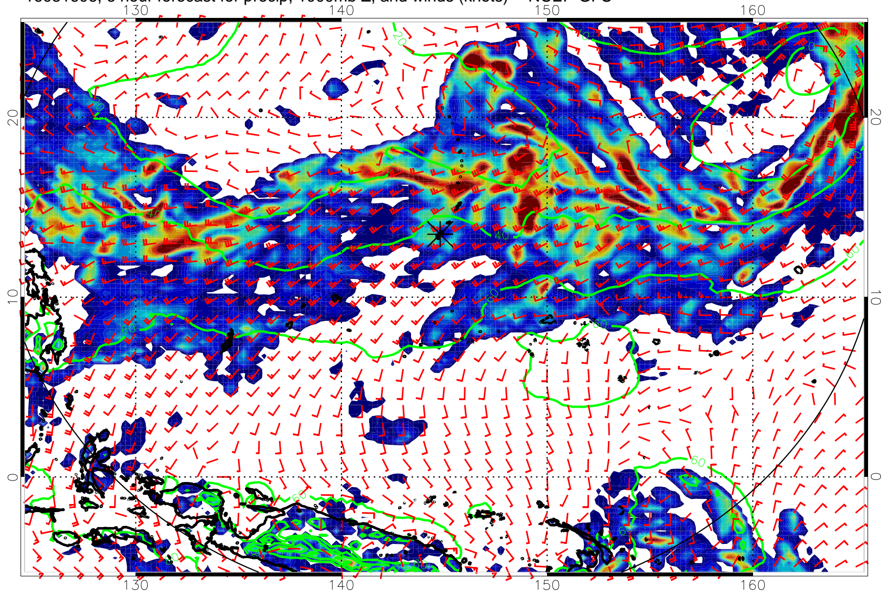
16081606, 6 hour forecast for precip, 1000mb Z, and winds (knots) -- NCEP GFS
