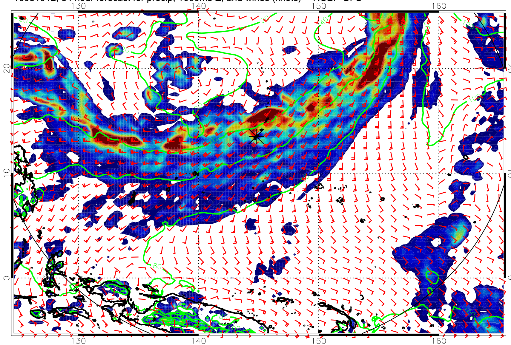
16081912, 84 hour forecast for precip, 1000mb Z, and winds (knots) -- NCEP GFS
