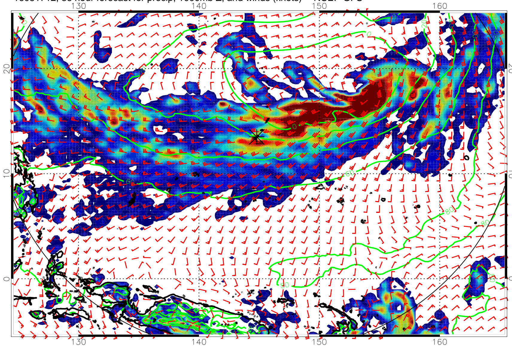
16081712, 36 hour forecast for precip, 1000mb Z, and winds (knots) -- NCEP GFS
