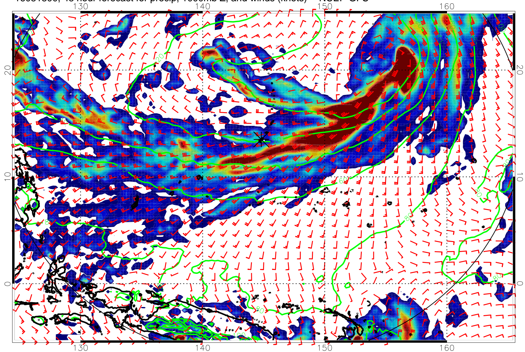
16081800, 48 hour forecast for precip, 1000mb Z, and winds (knots) -- NCEP GFS
