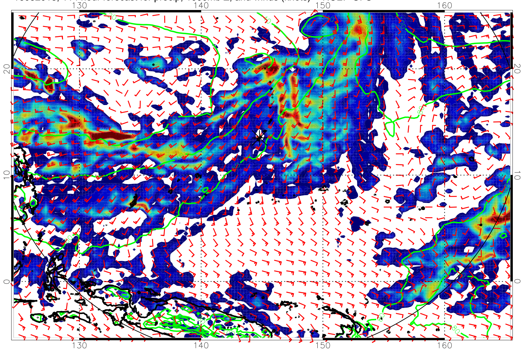
16082018, 114 hour forecast for precip, 1000mb Z, and winds (knots) -- NCEP GFS
