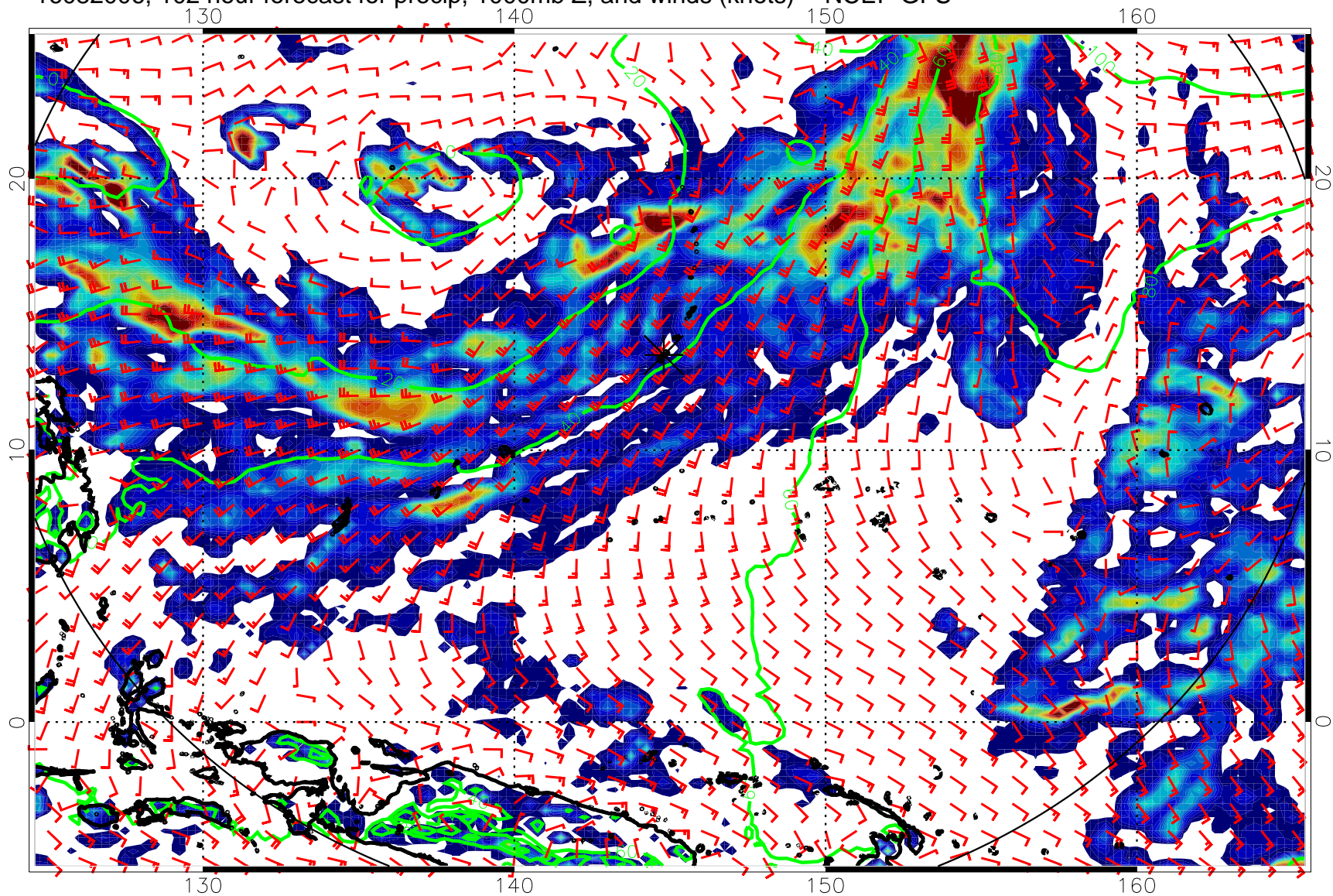
16082006, 102 hour forecast for precip, 1000mb Z, and winds (knots) -- NCEP GFS
