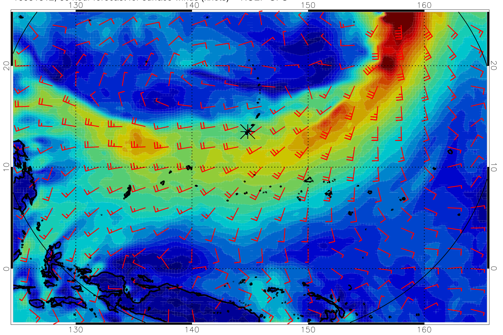
16081812, 60 hour forecast for surface winds (knots) -- NCEP GFS
