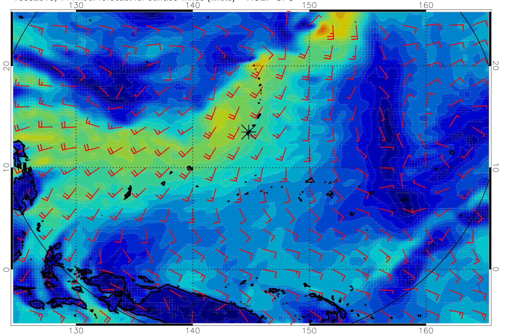
16082018, 114 hour forecast for surface winds (knots) -- NCEP GFS
