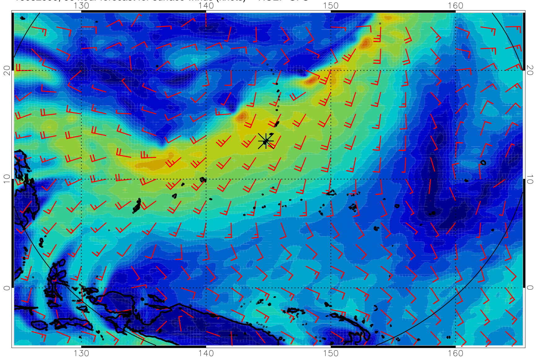
16082000, 96 hour forecast for surface winds (knots) -- NCEP GFS
