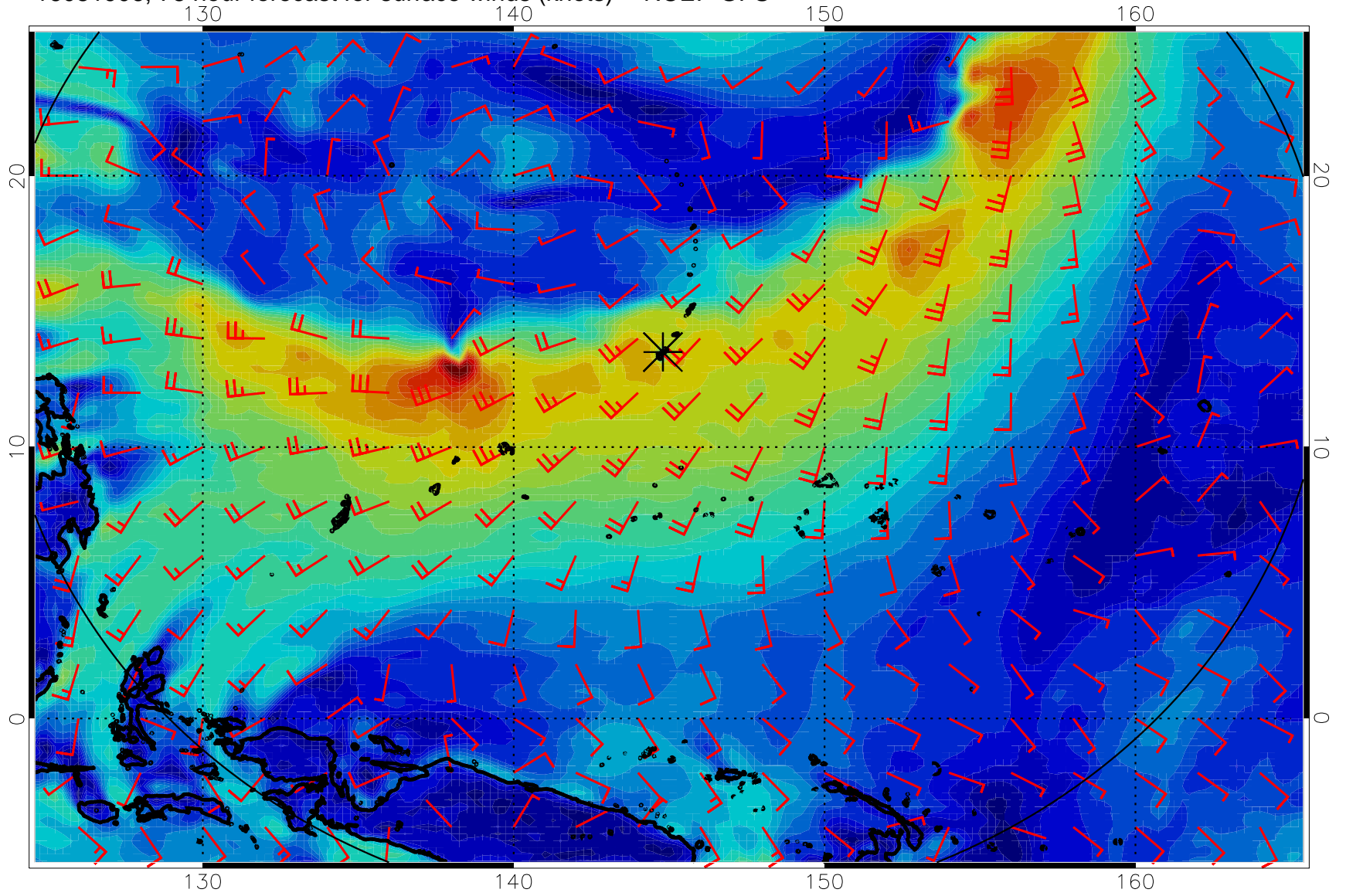
16081906, 78 hour forecast for surface winds (knots) -- NCEP GFS
