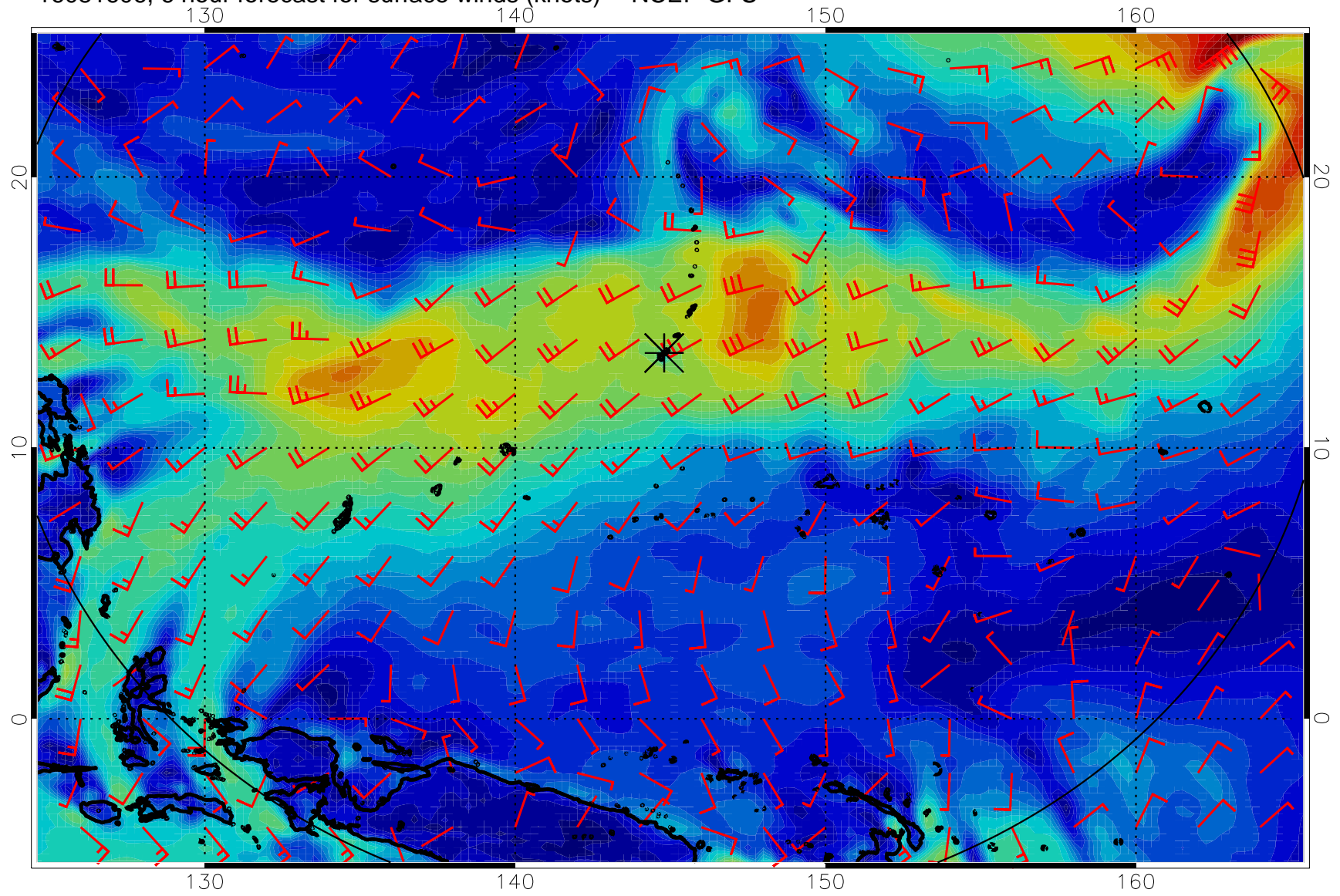
16081606, 6 hour forecast for surface winds (knots) -- NCEP GFS
