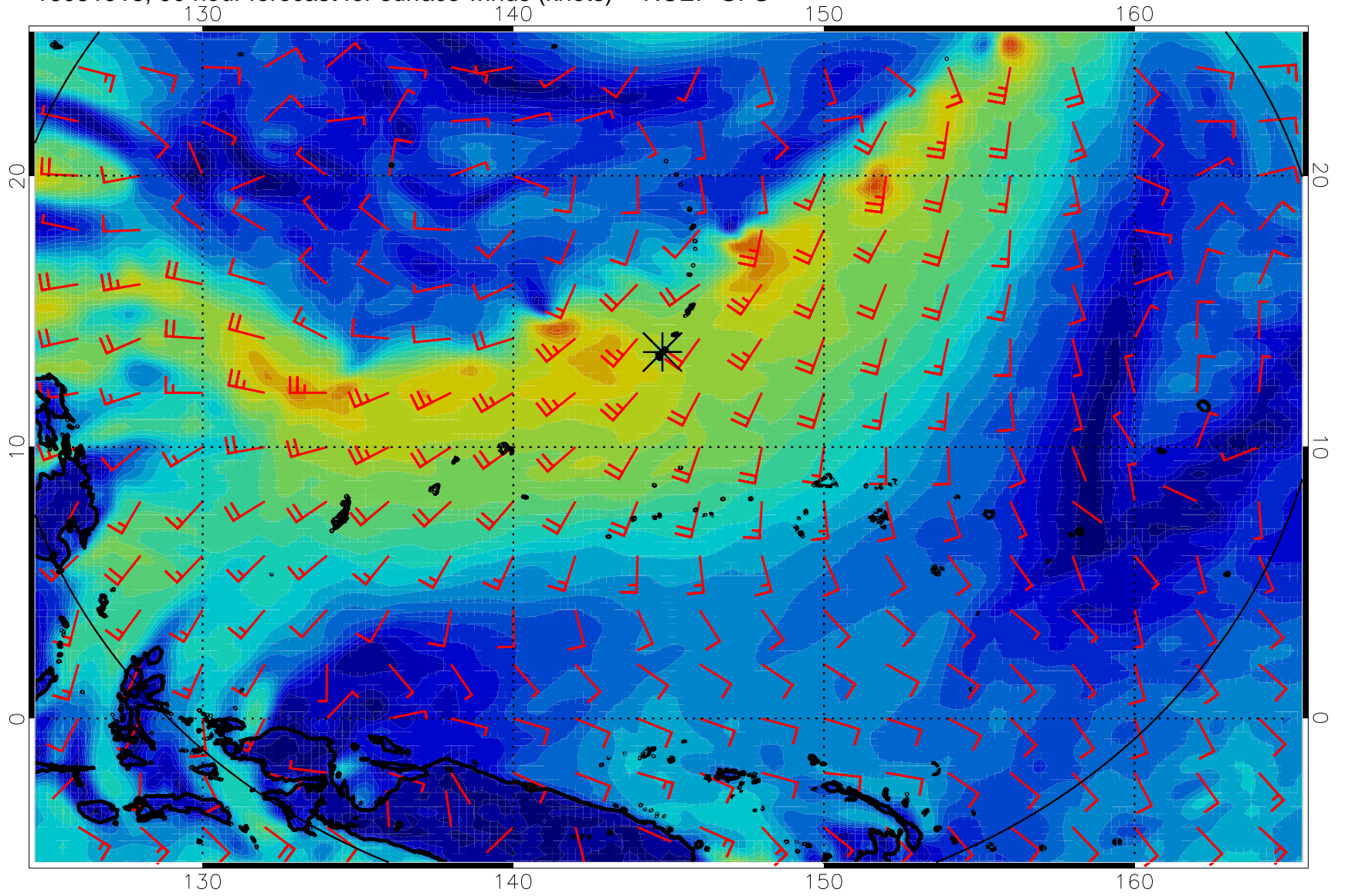
16081918, 90 hour forecast for surface winds (knots) -- NCEP GFS
