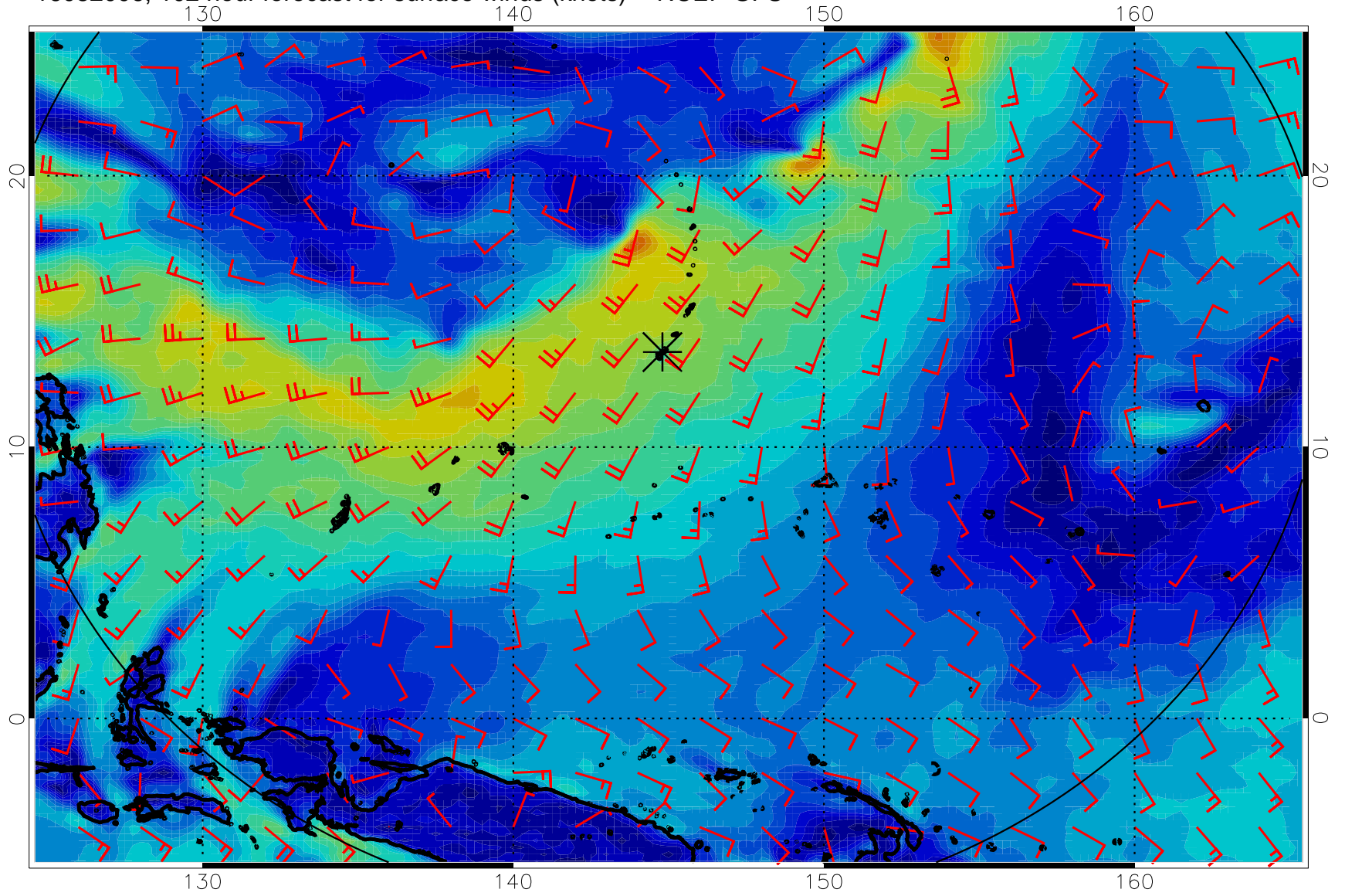
16082006, 102 hour forecast for surface winds (knots) -- NCEP GFS
