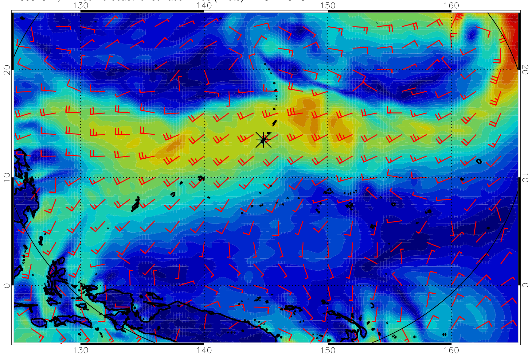
16081612, 12 hour forecast for surface winds (knots) -- NCEP GFS
