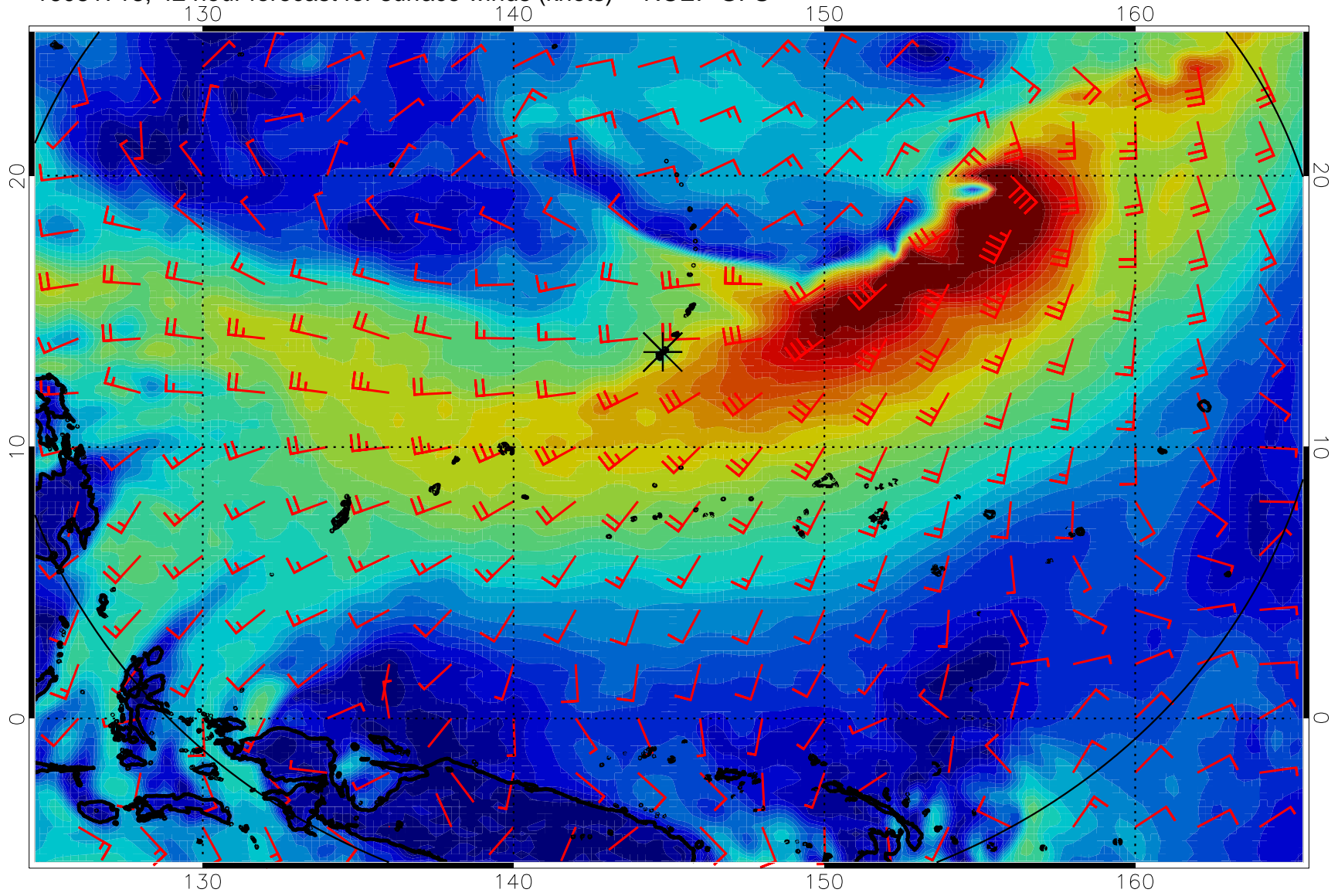
16081718, 42 hour forecast for surface winds (knots) -- NCEP GFS
