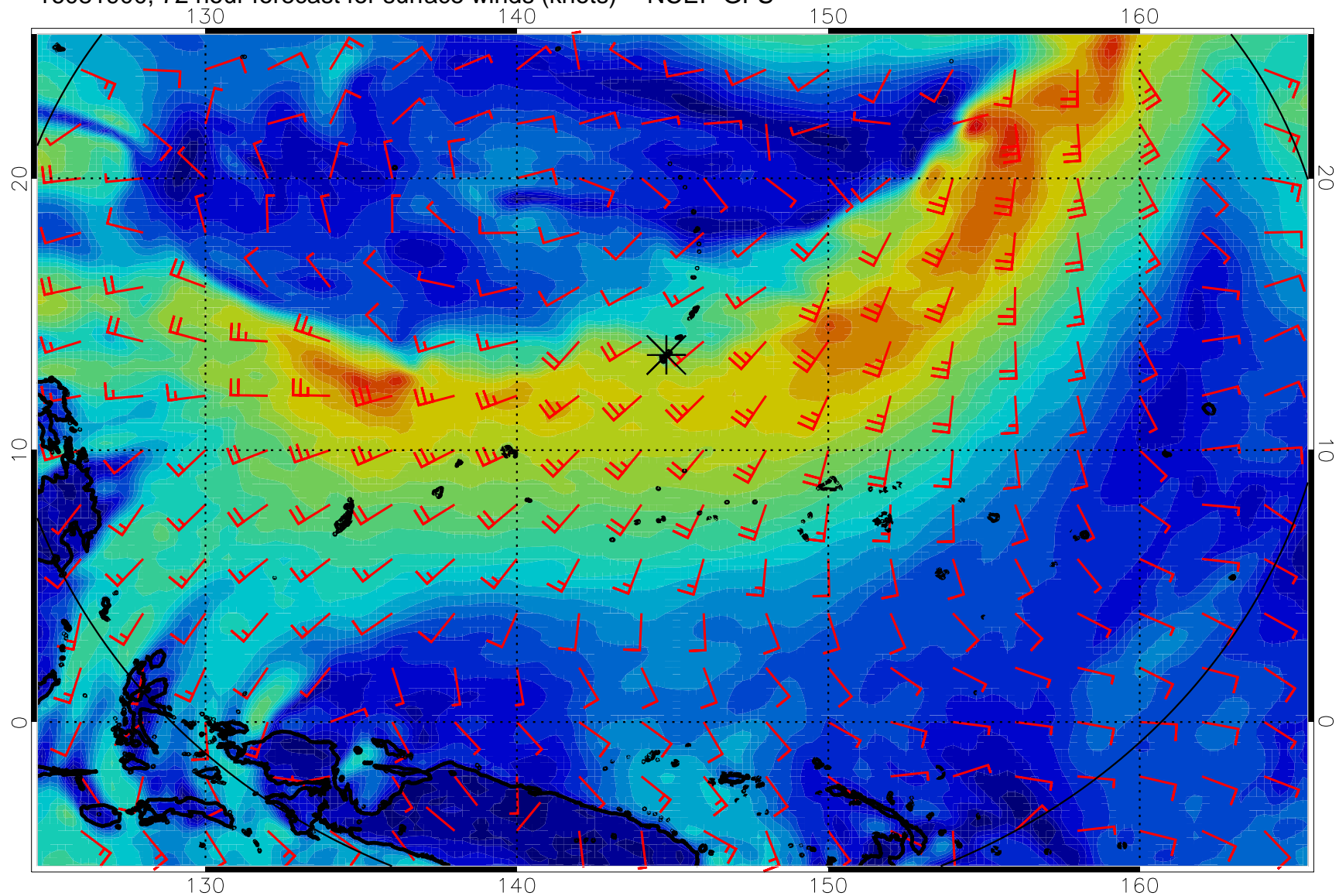
16081900, 72 hour forecast for surface winds (knots) -- NCEP GFS
