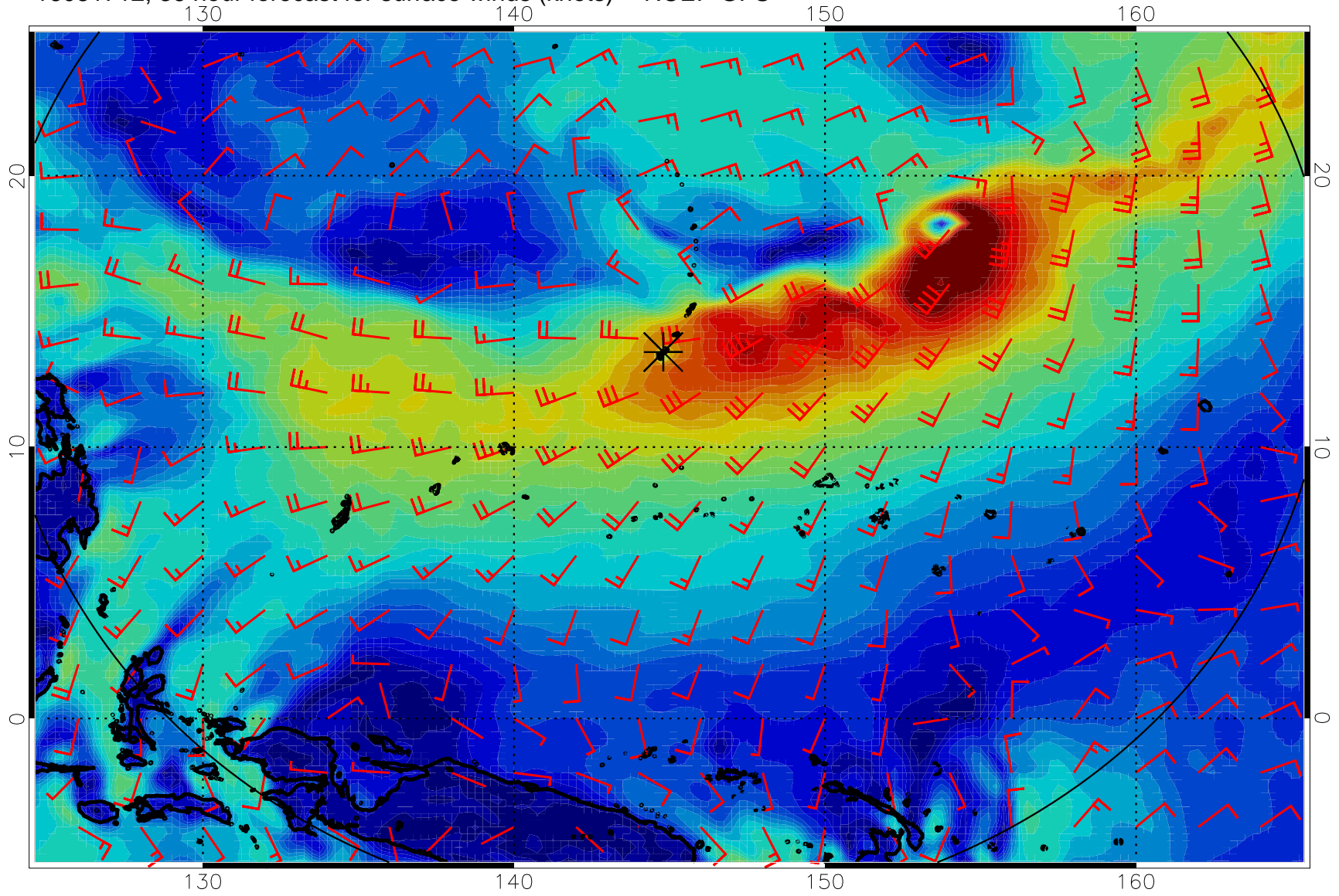
16081712, 36 hour forecast for surface winds (knots) -- NCEP GFS
