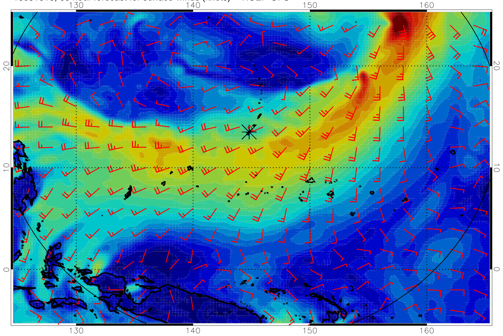
16081818, 66 hour forecast for surface winds (knots) -- NCEP GFS
