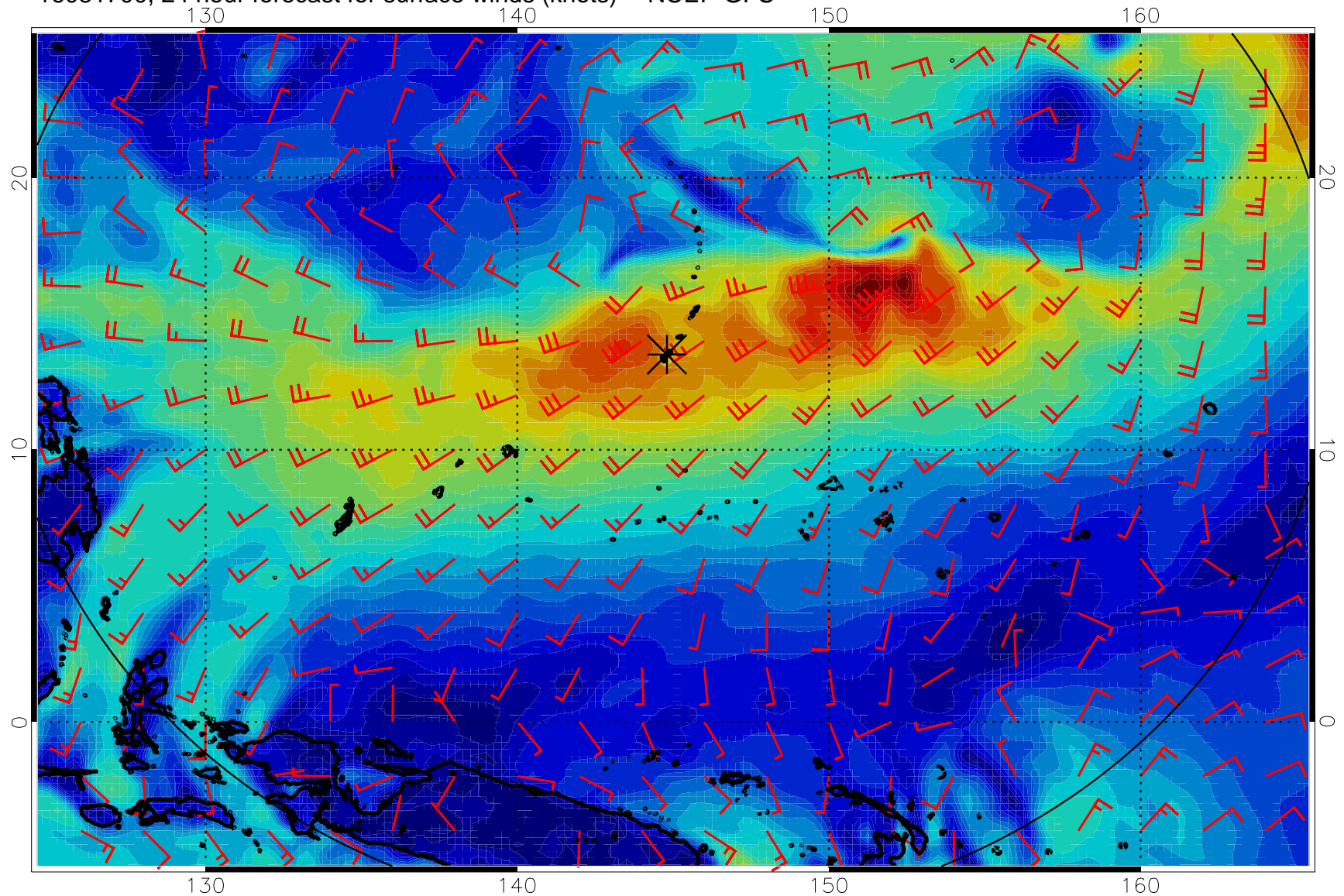
16081700, 24 hour forecast for surface winds (knots) -- NCEP GFS
