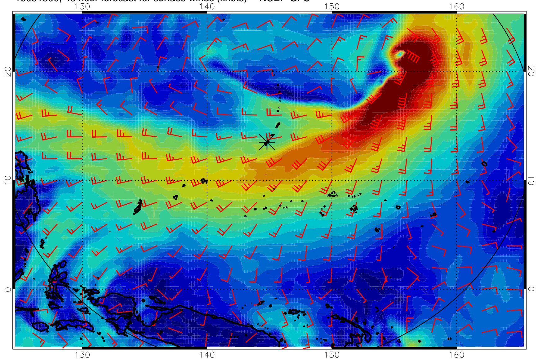
16081800, 48 hour forecast for surface winds (knots) -- NCEP GFS
