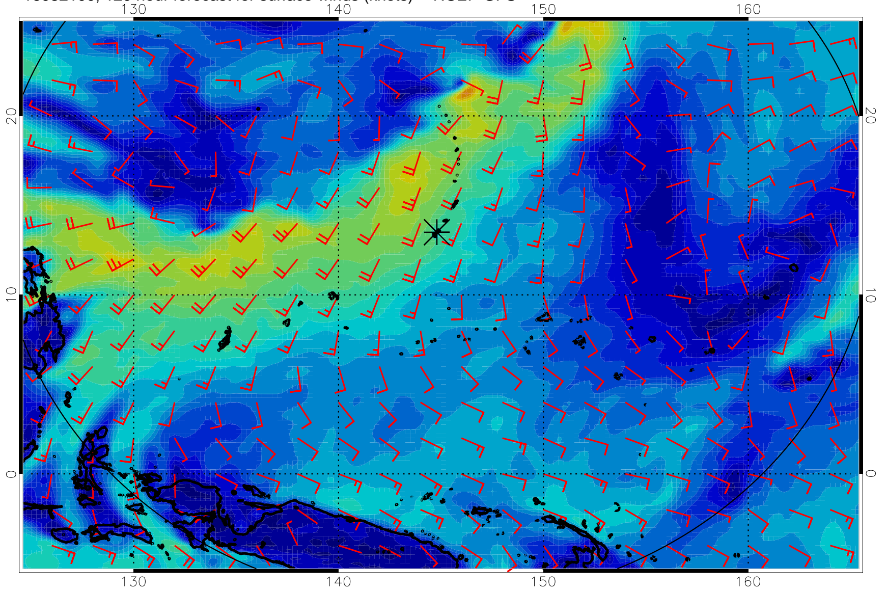
16082100, 120 hour forecast for surface winds (knots) -- NCEP GFS
