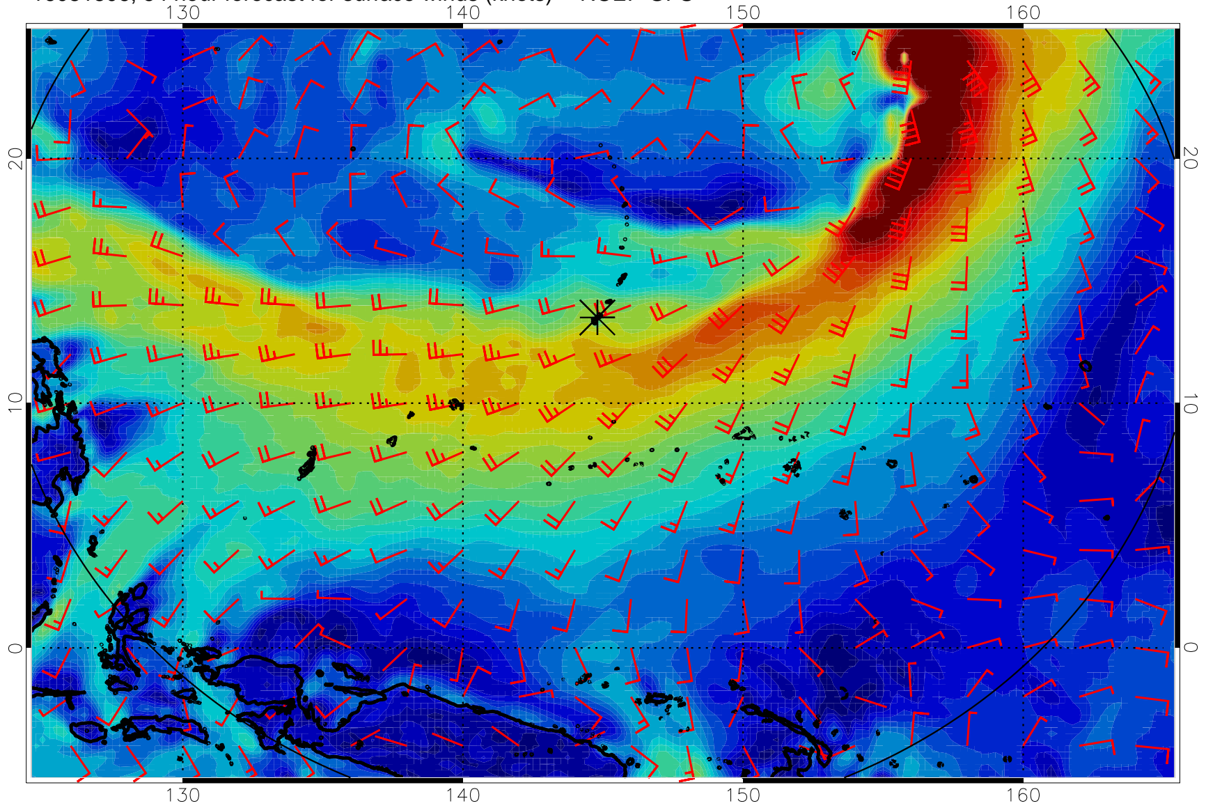
16081806, 54 hour forecast for surface winds (knots) -- NCEP GFS
