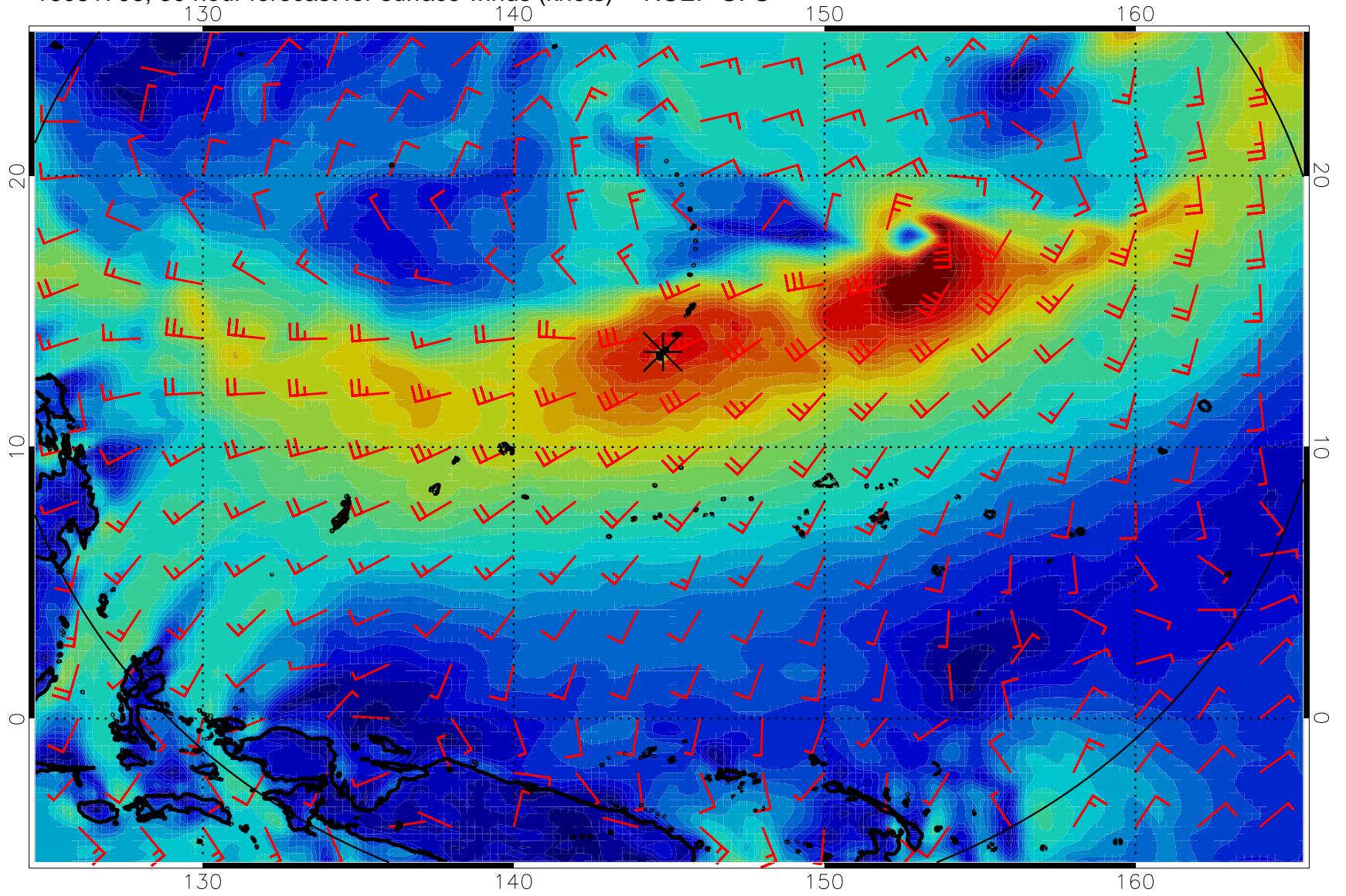
16081706, 30 hour forecast for surface winds (knots) -- NCEP GFS
