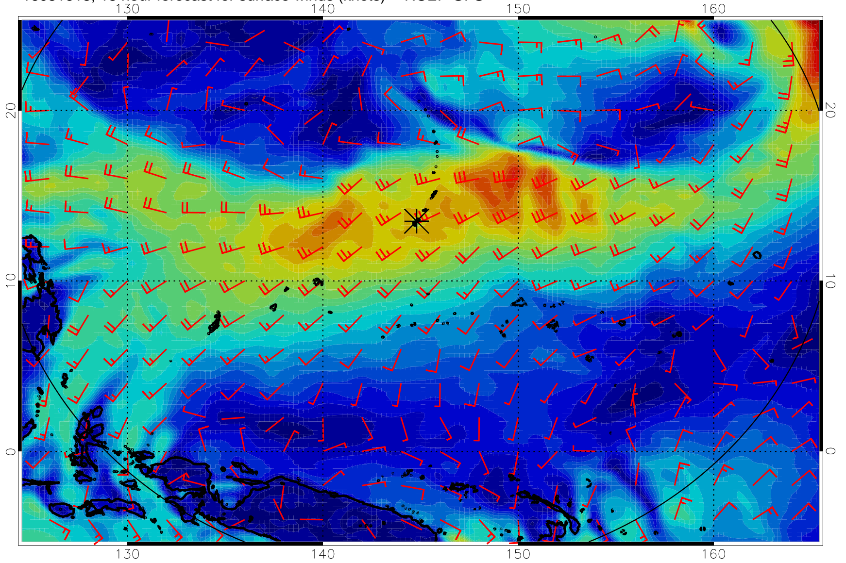
16081618, 18 hour forecast for surface winds (knots) -- NCEP GFS
