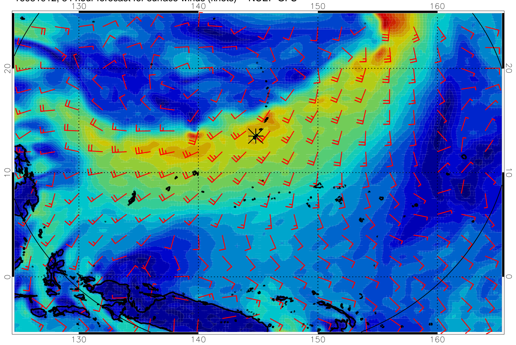
16081912, 84 hour forecast for surface winds (knots) -- NCEP GFS
