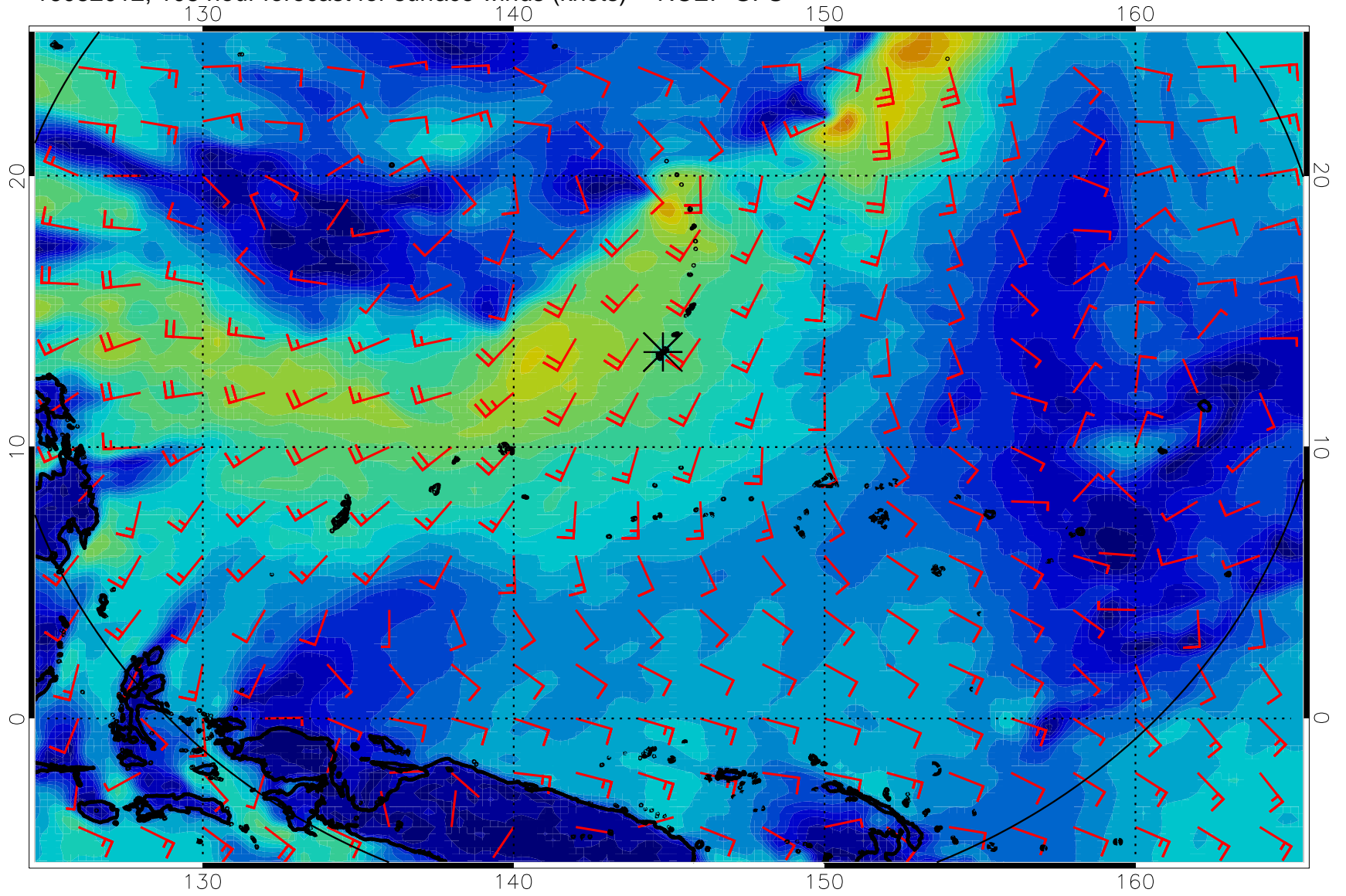
16082012, 108 hour forecast for surface winds (knots) -- NCEP GFS
