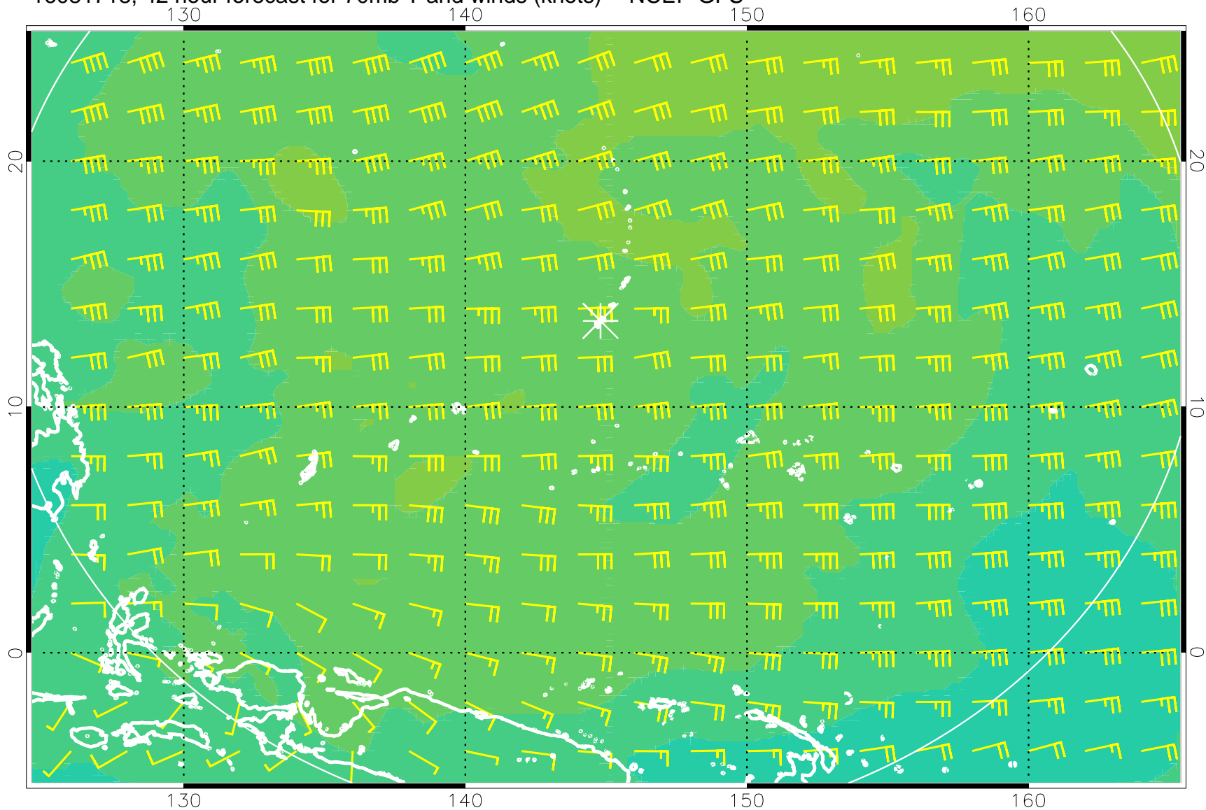
16081718, 42 hour forecast for 70mb T and winds (knots) -- NCEP GFS
