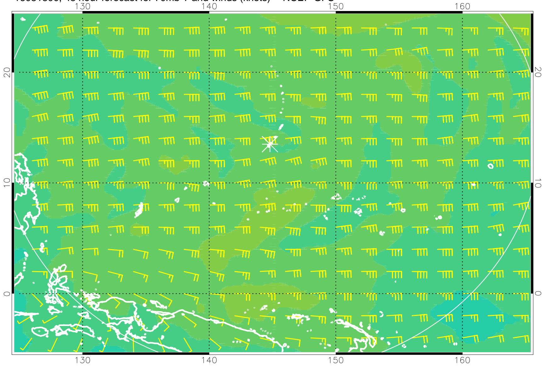
16081800, 48 hour forecast for 70mb T and winds (knots) -- NCEP GFS
