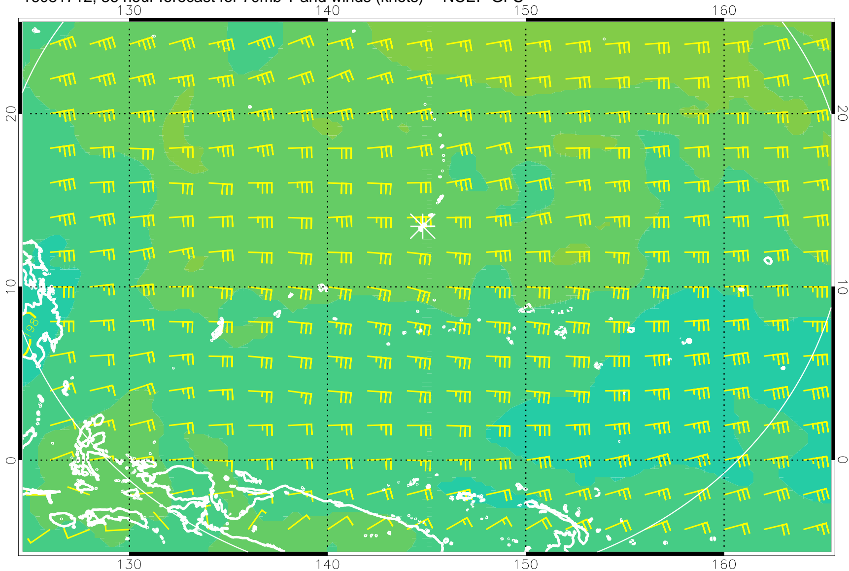
16081712, 36 hour forecast for 70mb T and winds (knots) -- NCEP GFS
