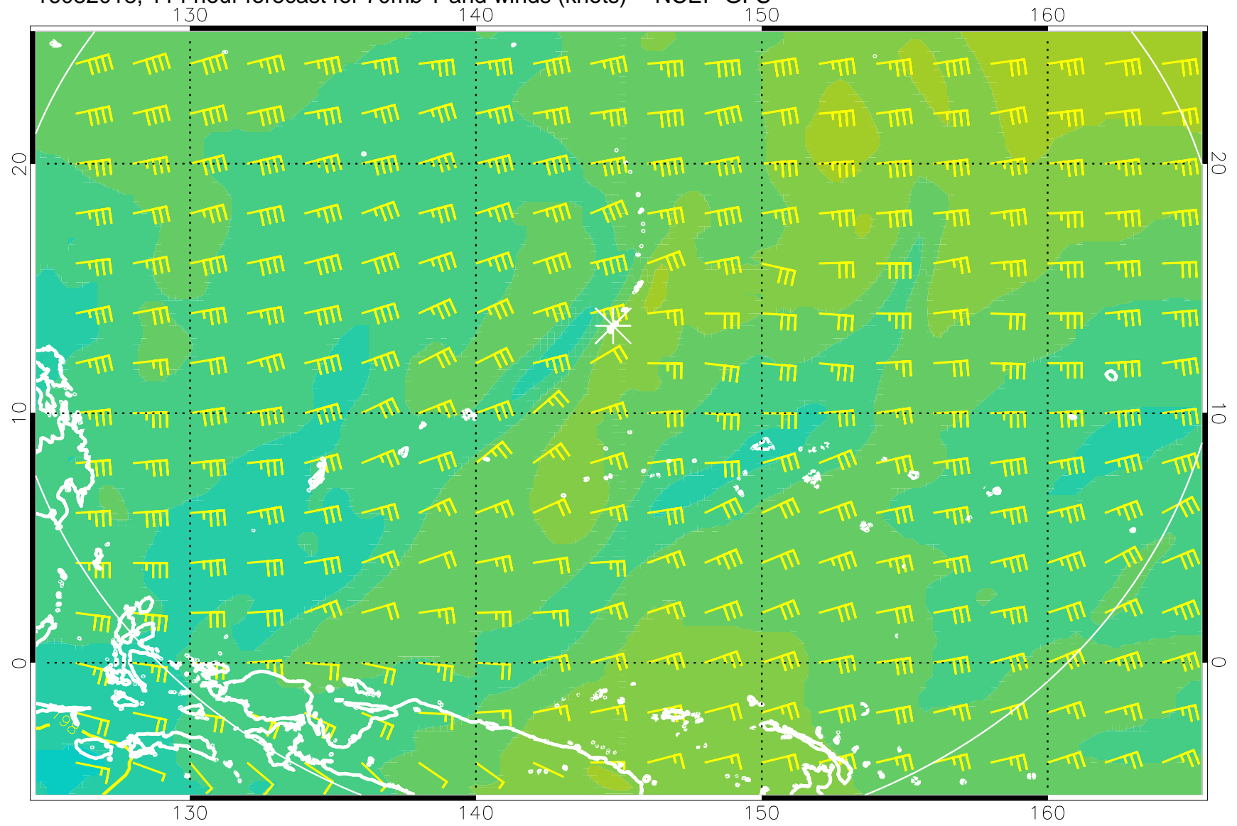
16082018, 114 hour forecast for 70mb T and winds (knots) -- NCEP GFS
