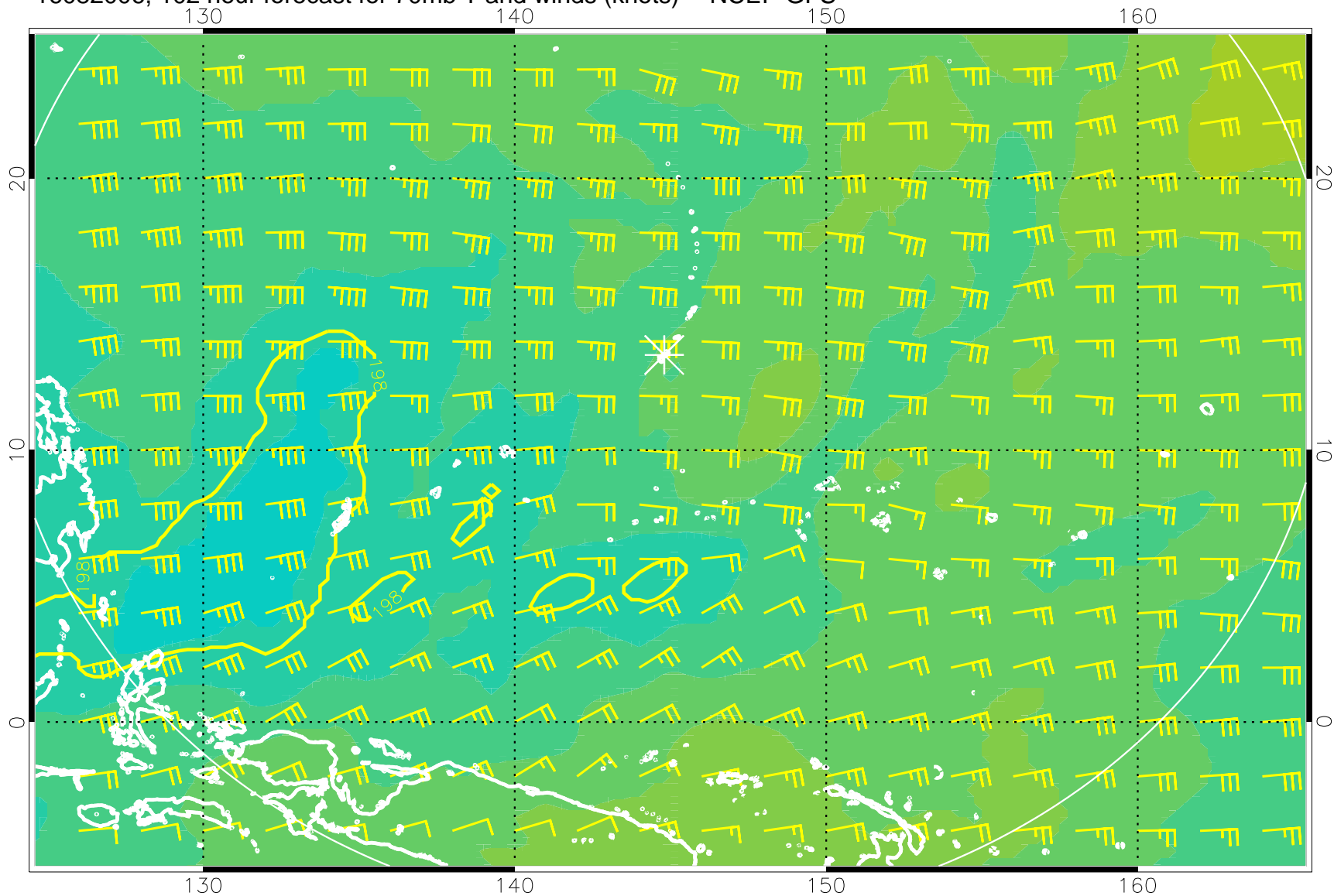
16082006, 102 hour forecast for 70mb T and winds (knots) -- NCEP GFS
