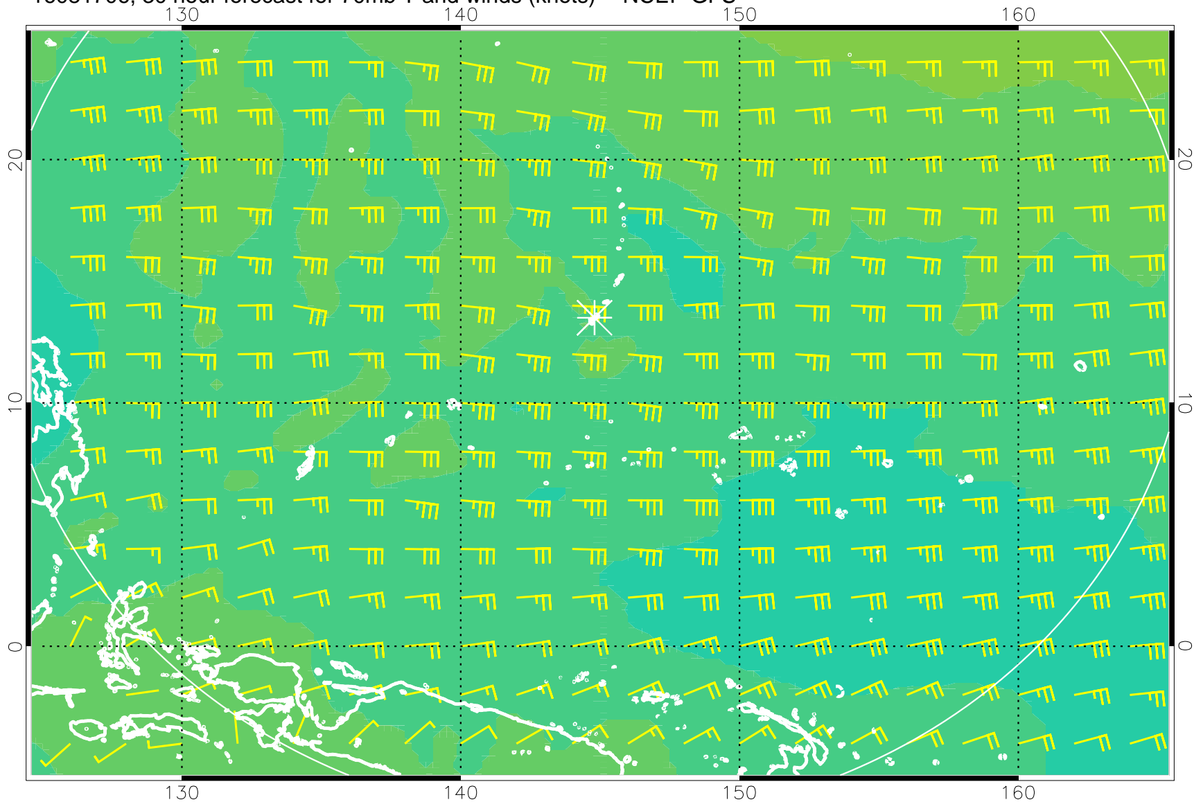
16081706, 30 hour forecast for 70mb T and winds (knots) -- NCEP GFS
