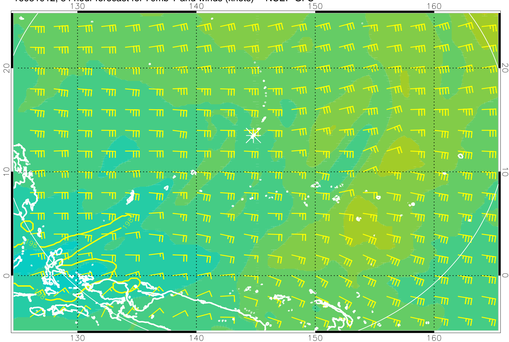
16081912, 84 hour forecast for 70mb T and winds (knots) -- NCEP GFS
