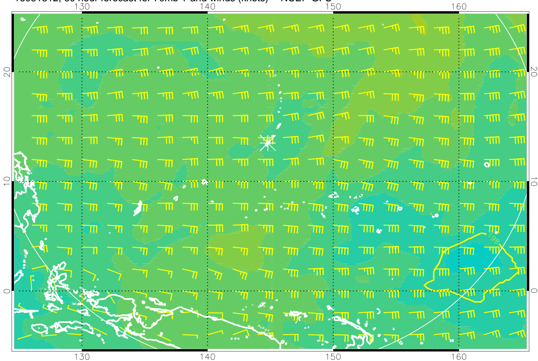
16081812, 60 hour forecast for 70mb T and winds (knots) -- NCEP GFS
