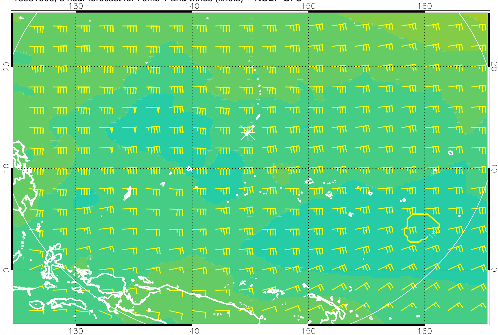
16081606, 6 hour forecast for 70mb T and winds (knots) -- NCEP GFS
