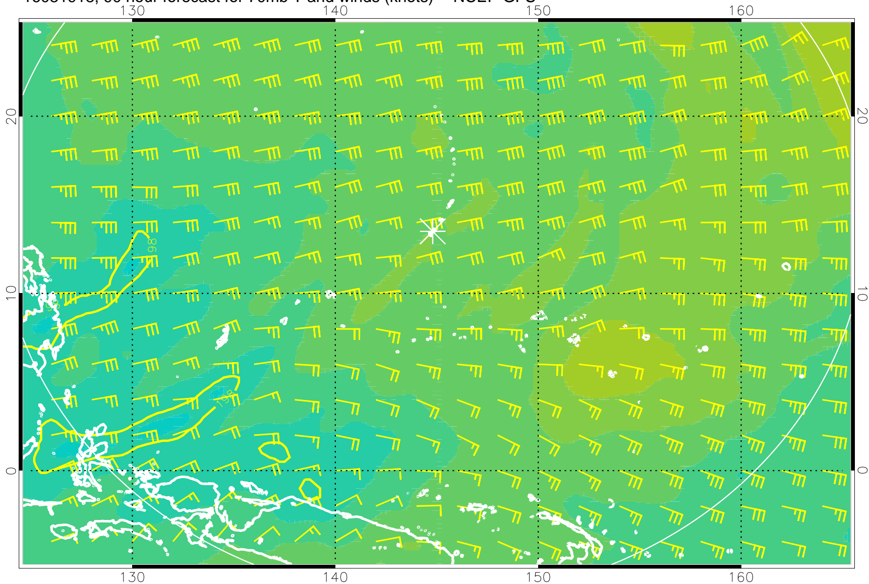
16081918, 90 hour forecast for 70mb T and winds (knots) -- NCEP GFS
