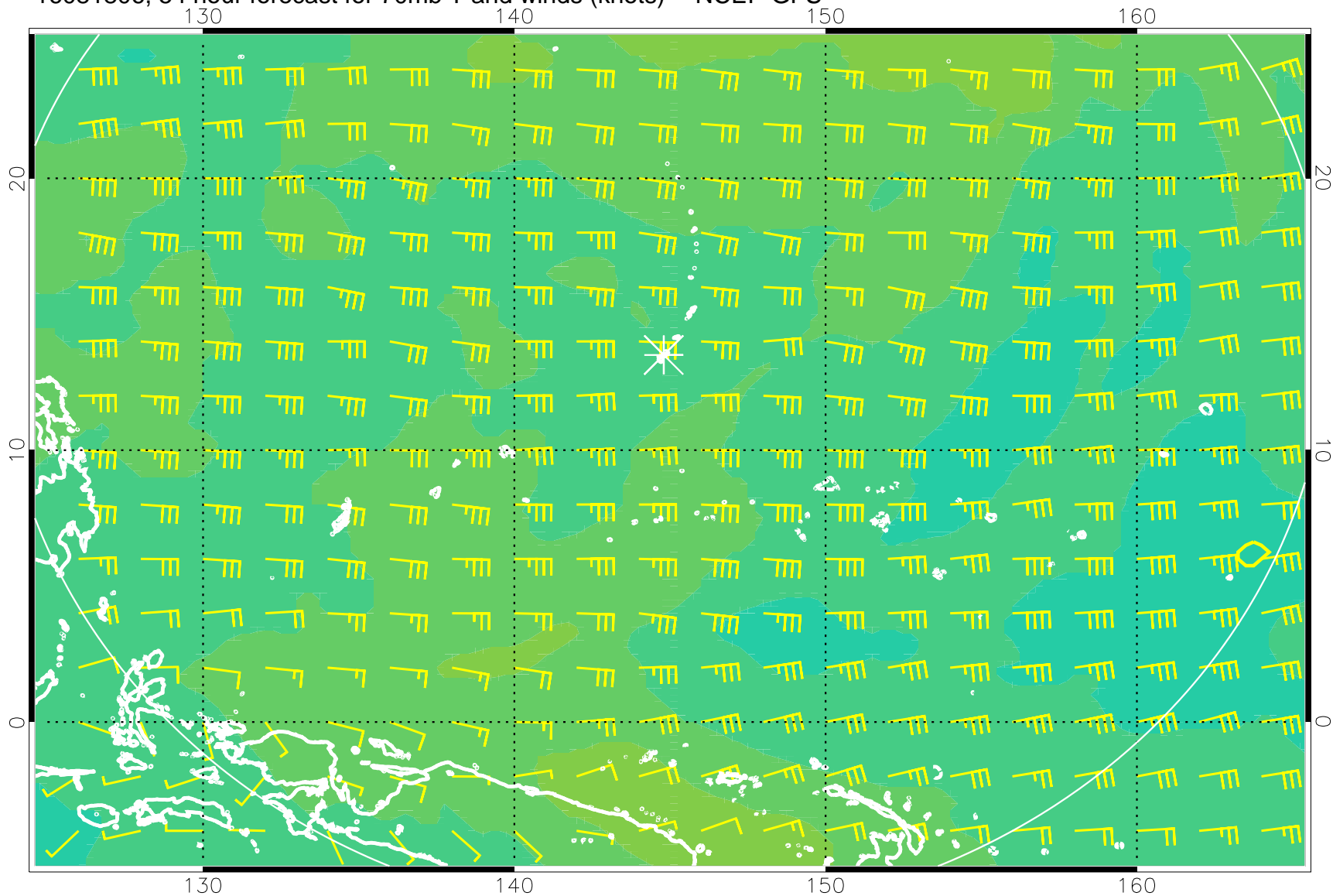
16081806, 54 hour forecast for 70mb T and winds (knots) -- NCEP GFS
