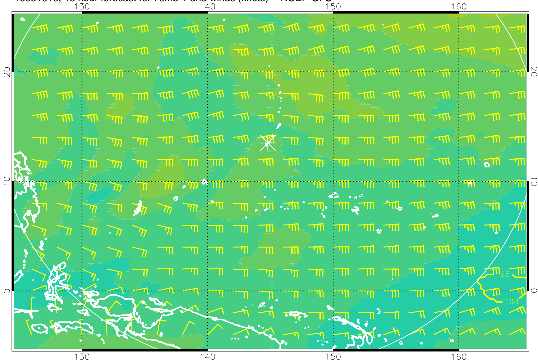
16081618, 18 hour forecast for 70mb T and winds (knots) -- NCEP GFS
