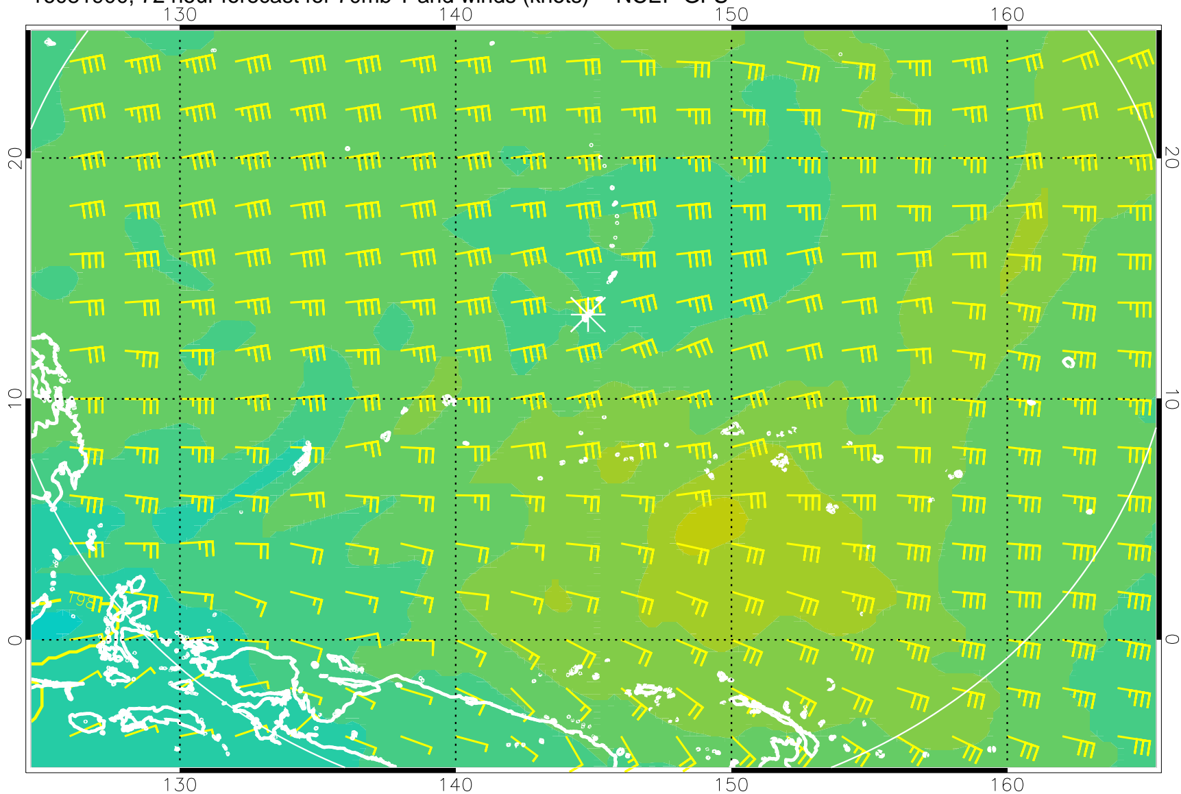
16081900, 72 hour forecast for 70mb T and winds (knots) -- NCEP GFS
