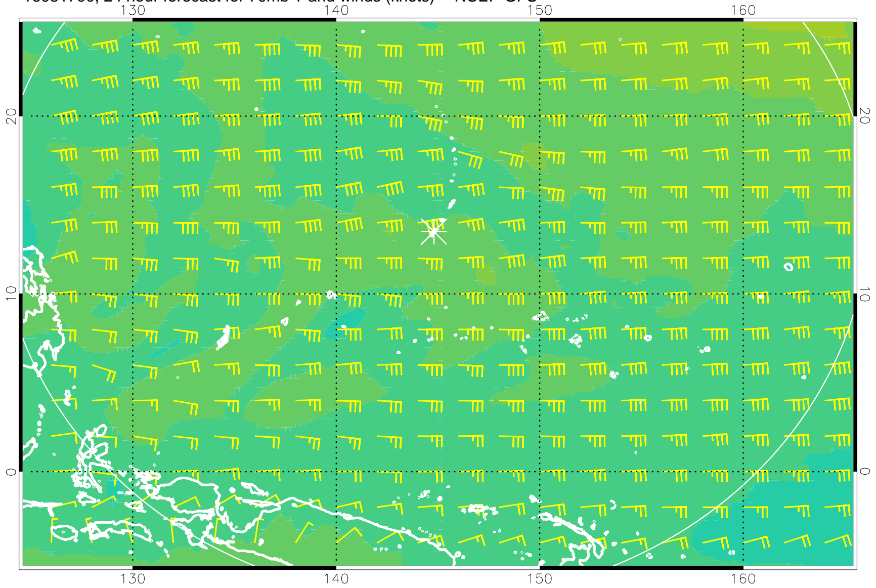
16081700, 24 hour forecast for 70mb T and winds (knots) -- NCEP GFS
