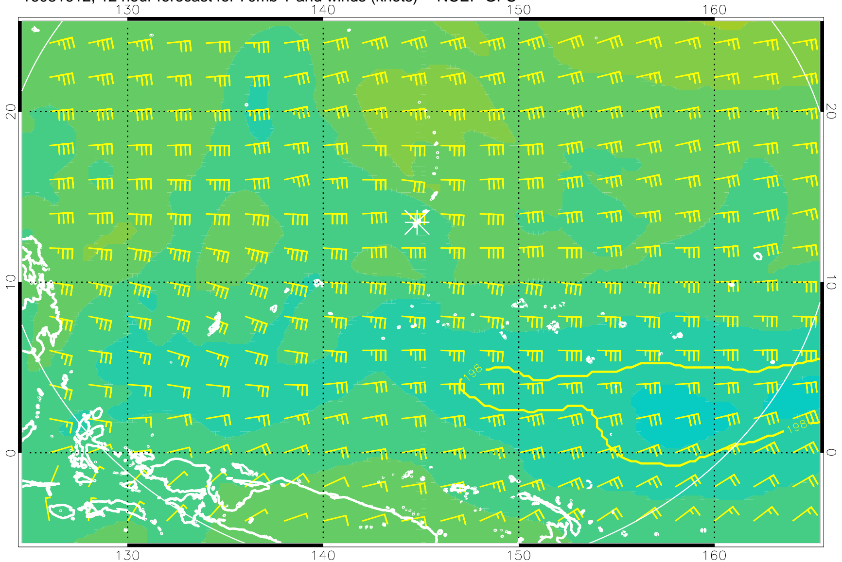
16081612, 12 hour forecast for 70mb T and winds (knots) -- NCEP GFS
