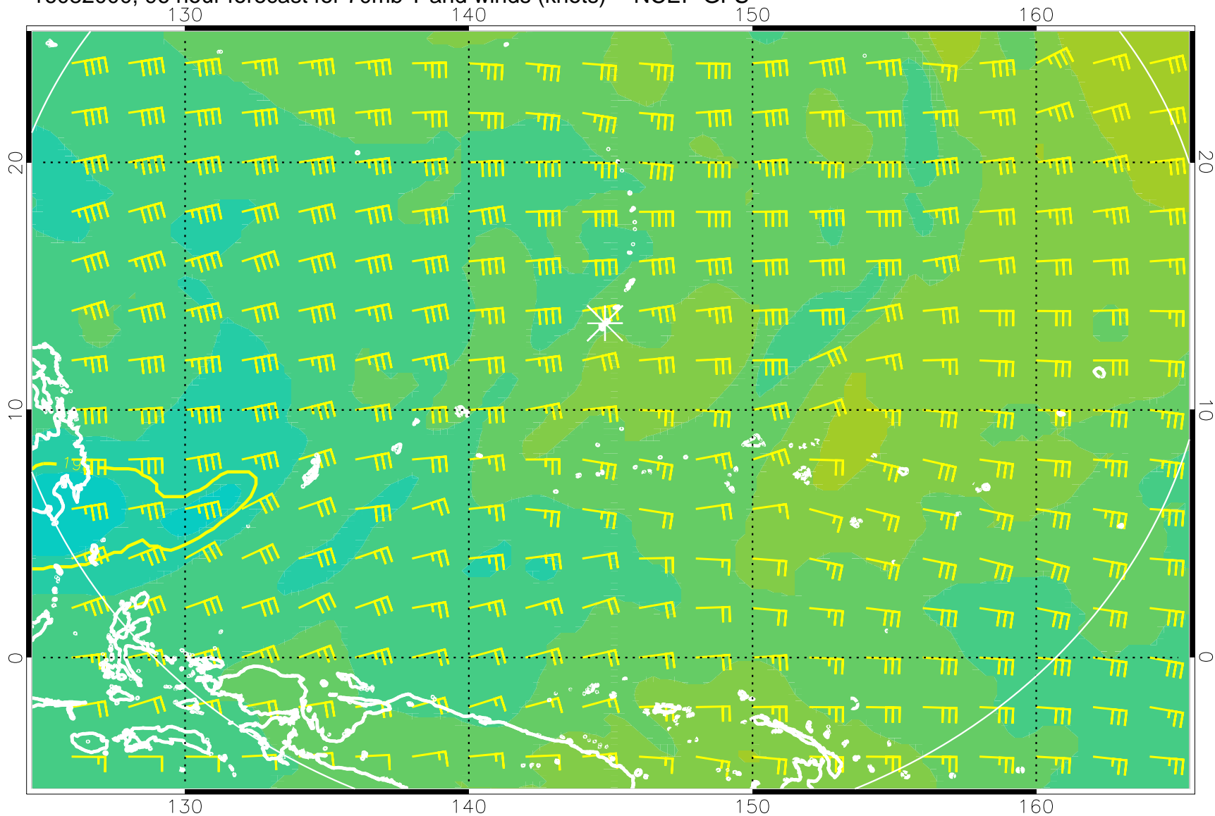
16082000, 96 hour forecast for 70mb T and winds (knots) -- NCEP GFS
