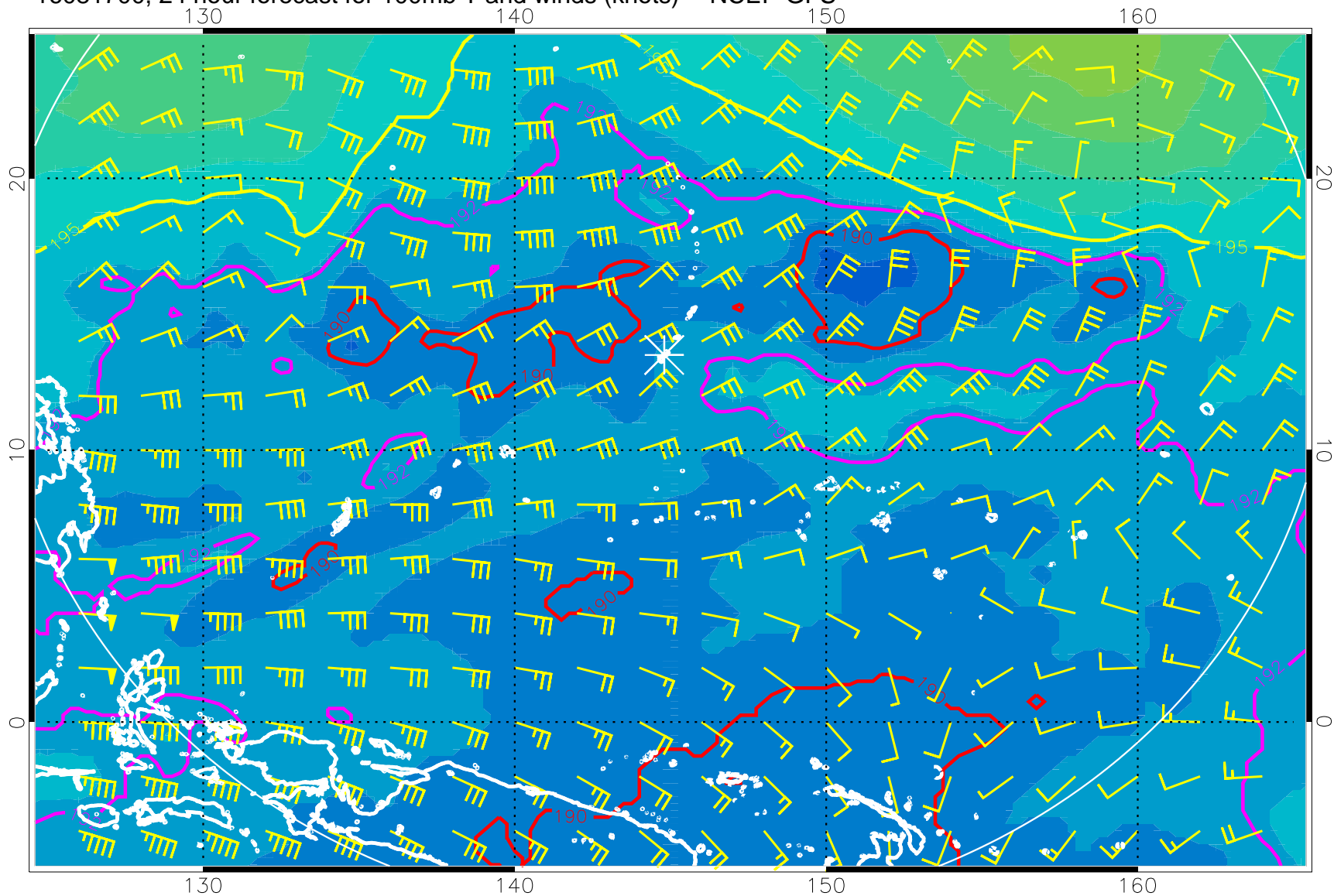
16081700, 24 hour forecast for 100mb T and winds (knots) -- NCEP GFS
