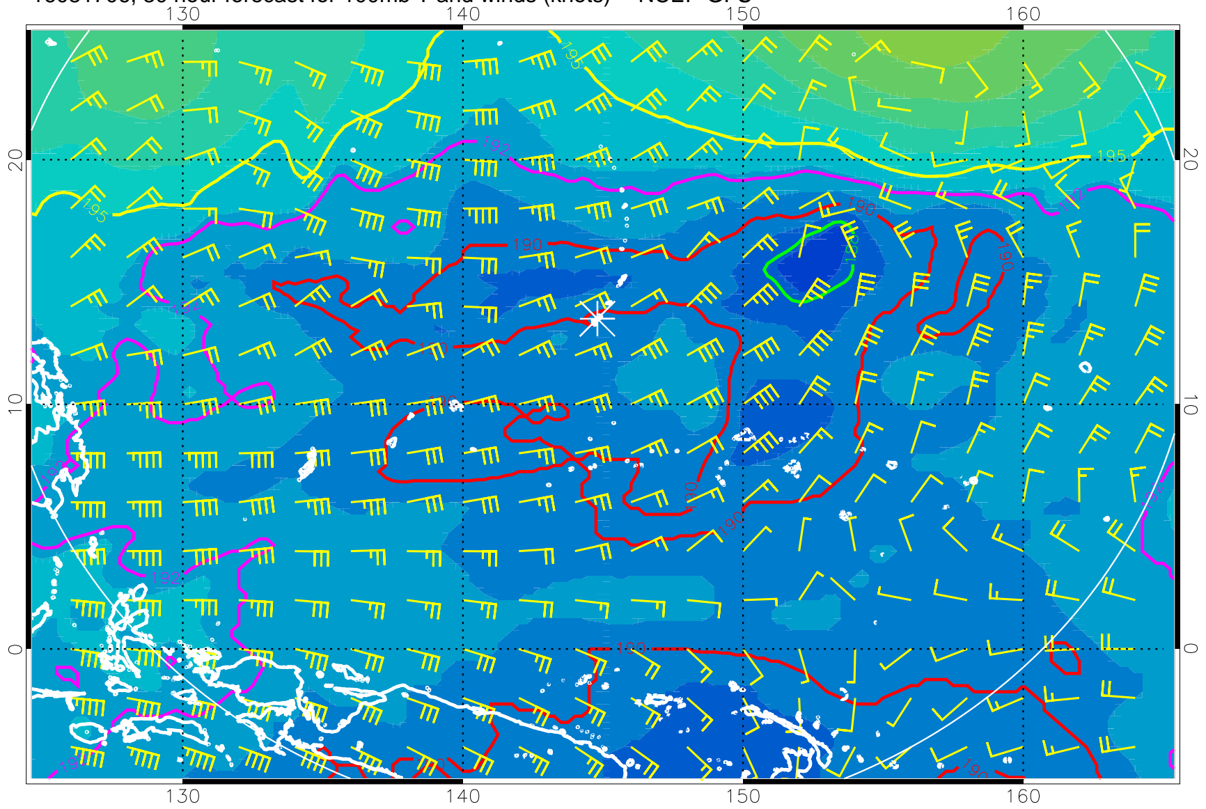
16081706, 30 hour forecast for 100mb T and winds (knots) -- NCEP GFS
