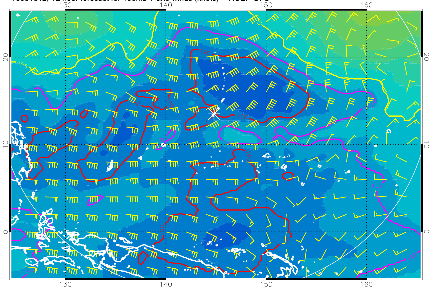
16081612, 12 hour forecast for 100mb T and winds (knots) -- NCEP GFS
