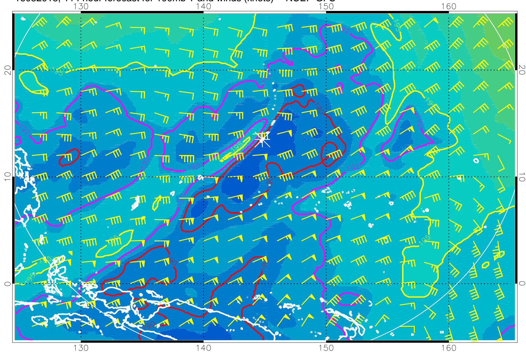
16082018, 114 hour forecast for 100mb T and winds (knots) -- NCEP GFS
