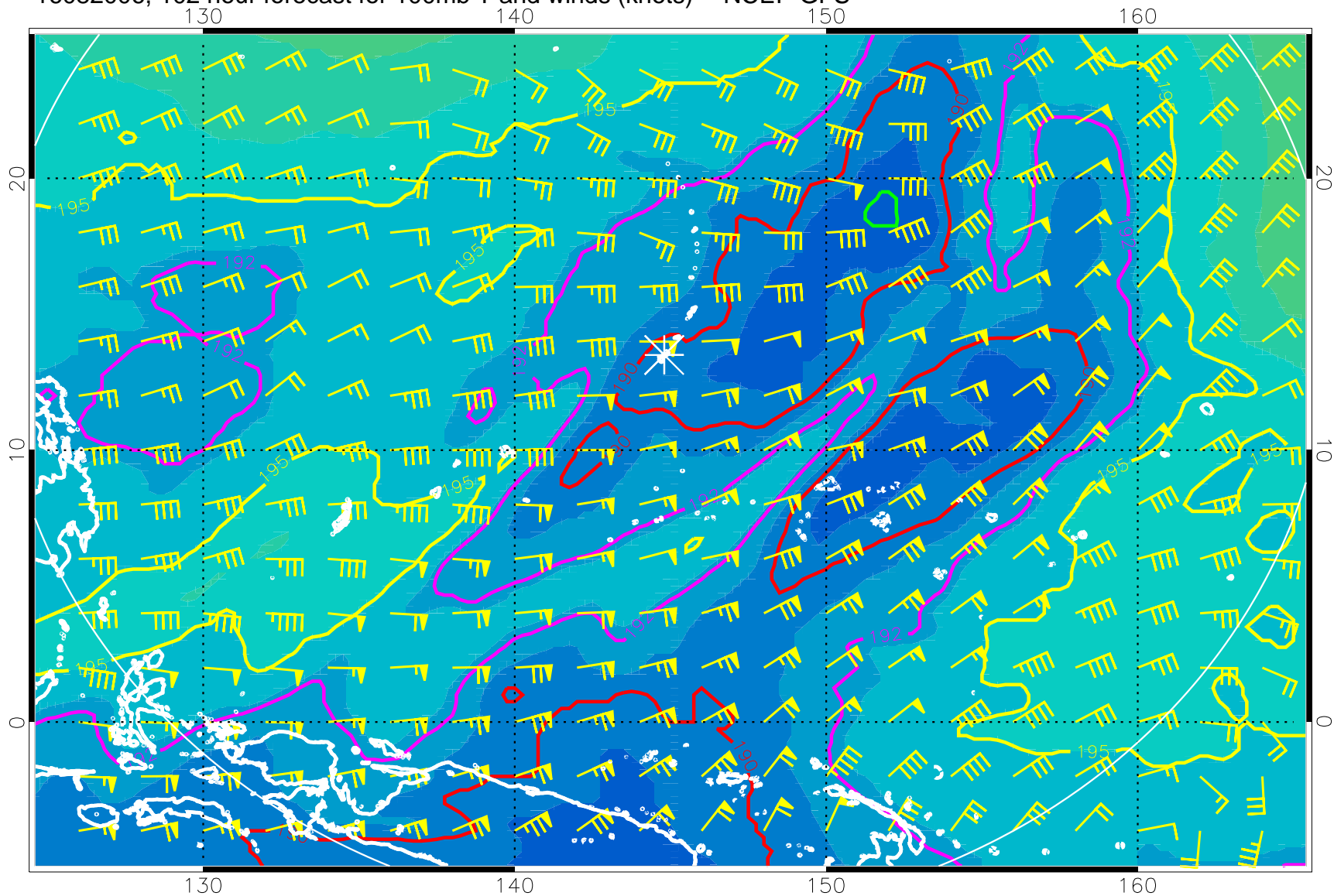
16082006, 102 hour forecast for 100mb T and winds (knots) -- NCEP GFS
