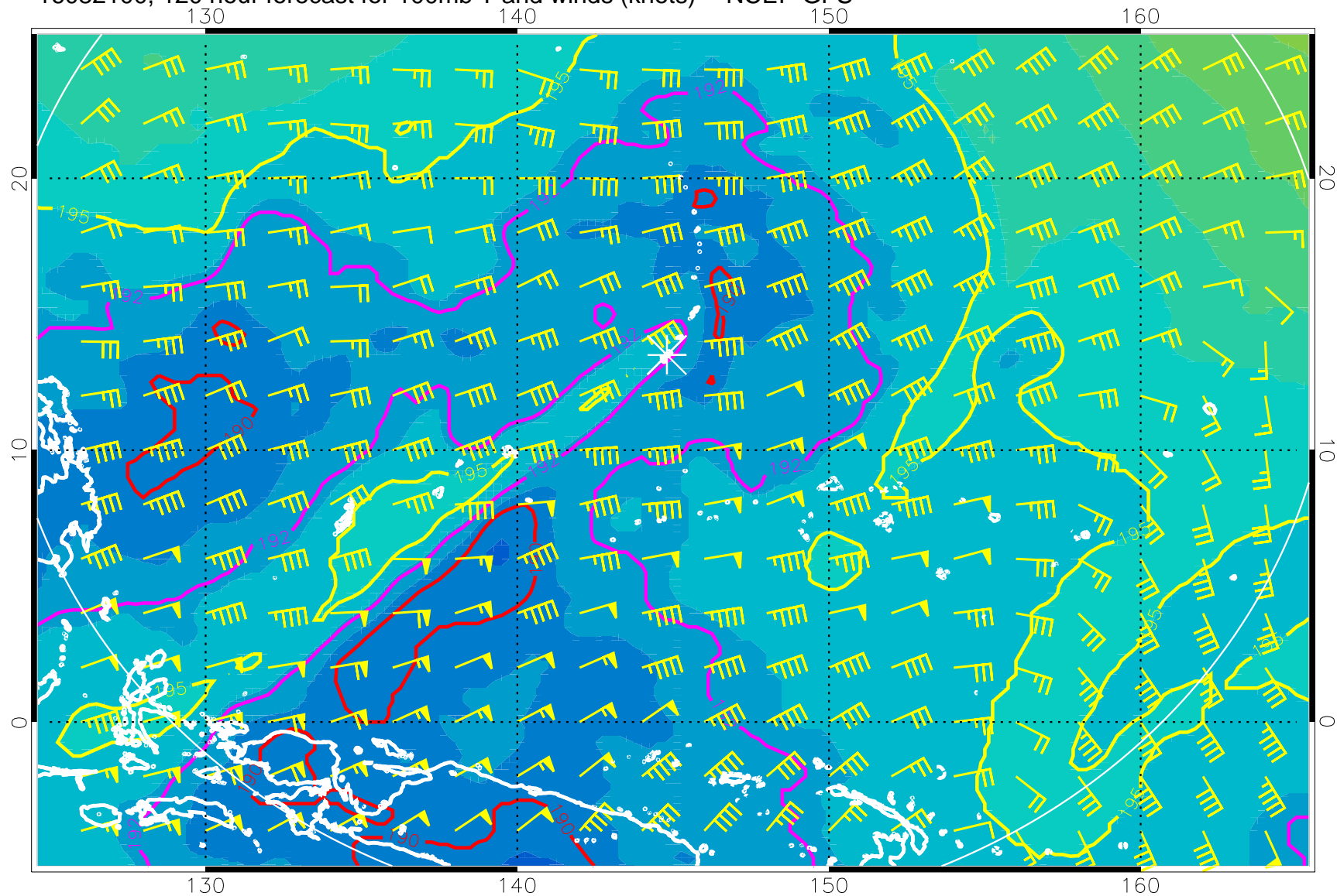
16082100, 120 hour forecast for 100mb T and winds (knots) -- NCEP GFS
