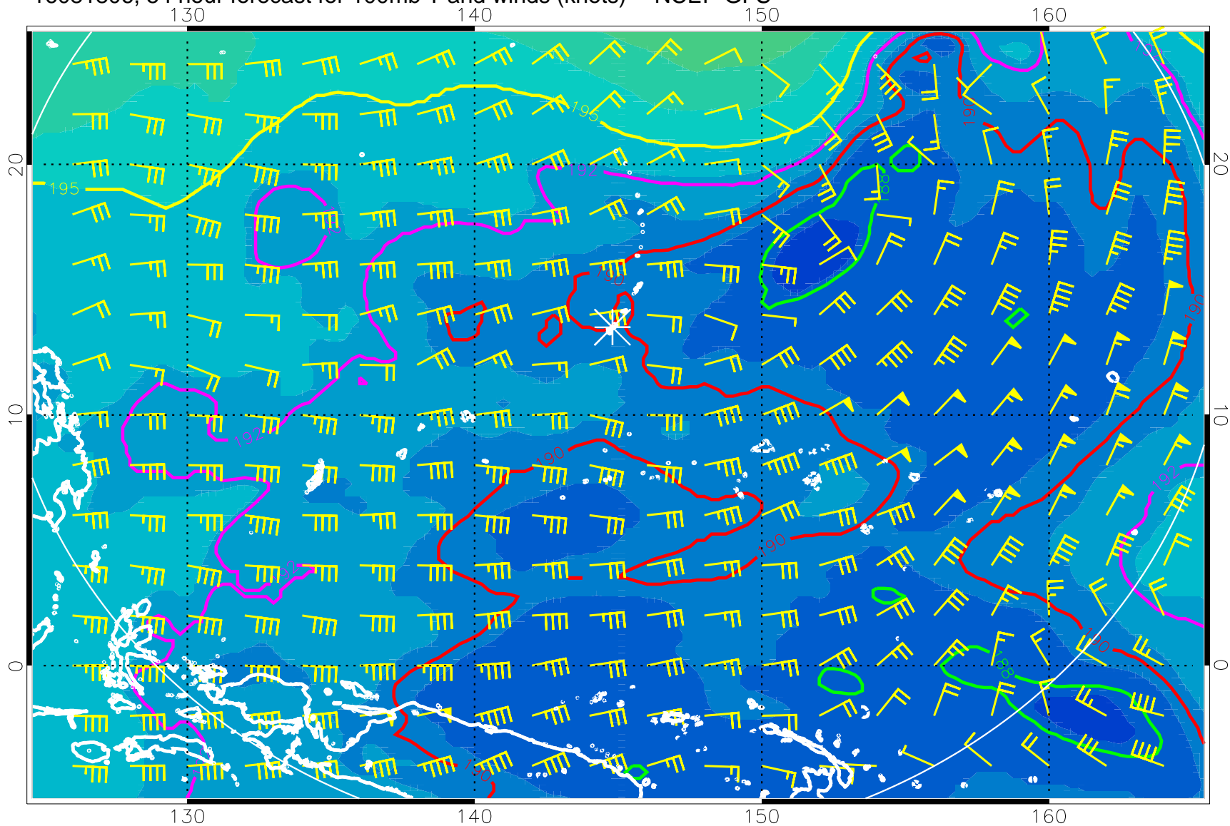
16081806, 54 hour forecast for 100mb T and winds (knots) -- NCEP GFS
