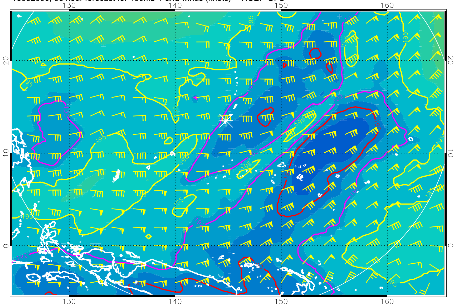
16082000, 96 hour forecast for 100mb T and winds (knots) -- NCEP GFS
