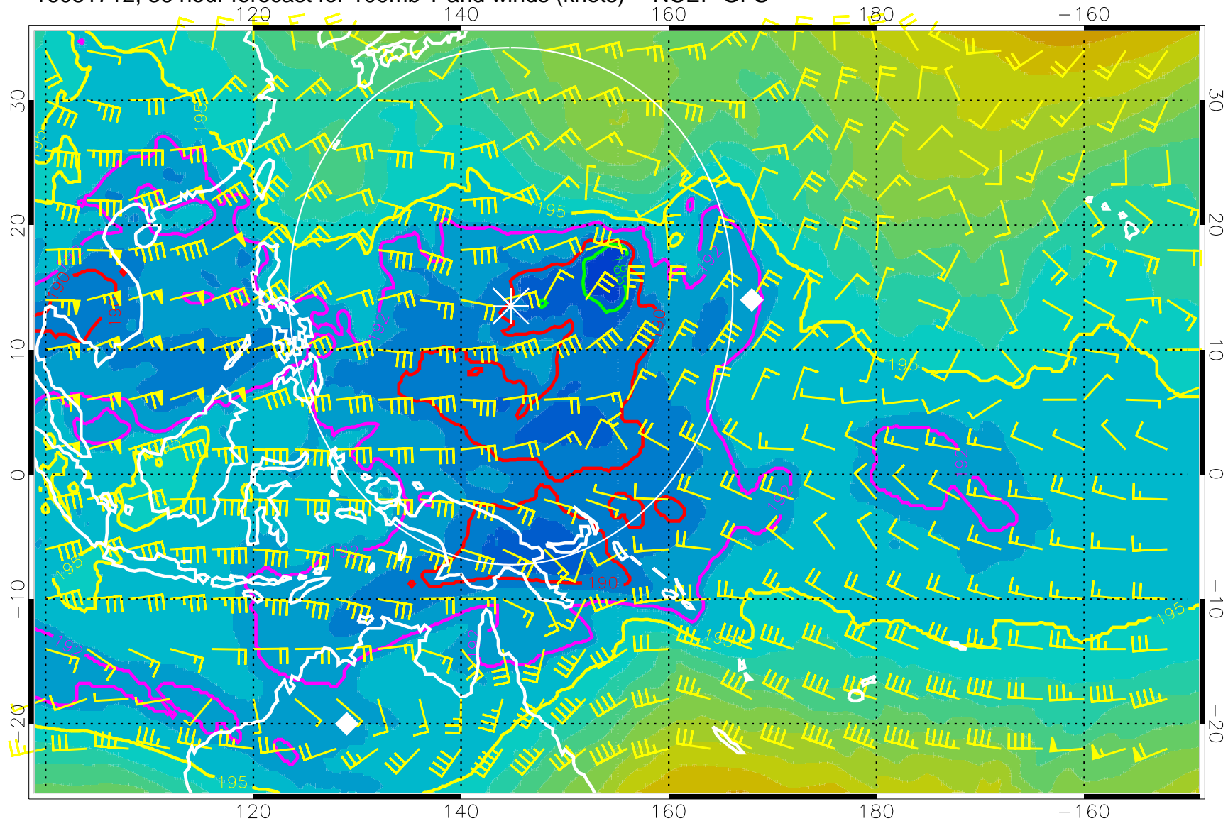
16081712, 36 hour forecast for 100mb T and winds (knots) -- NCEP GFS
