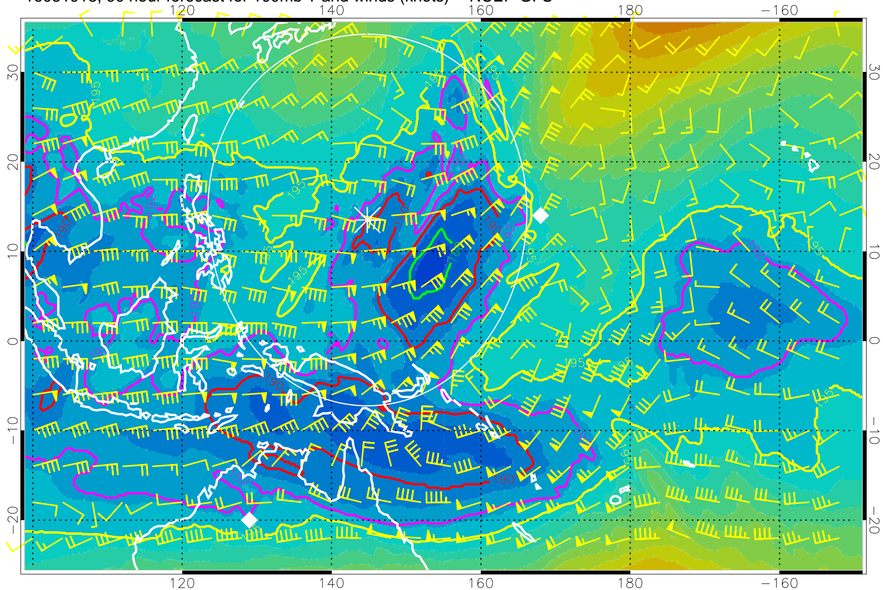
16081918, 90 hour forecast for 100mb T and winds (knots) -- NCEP GFS
