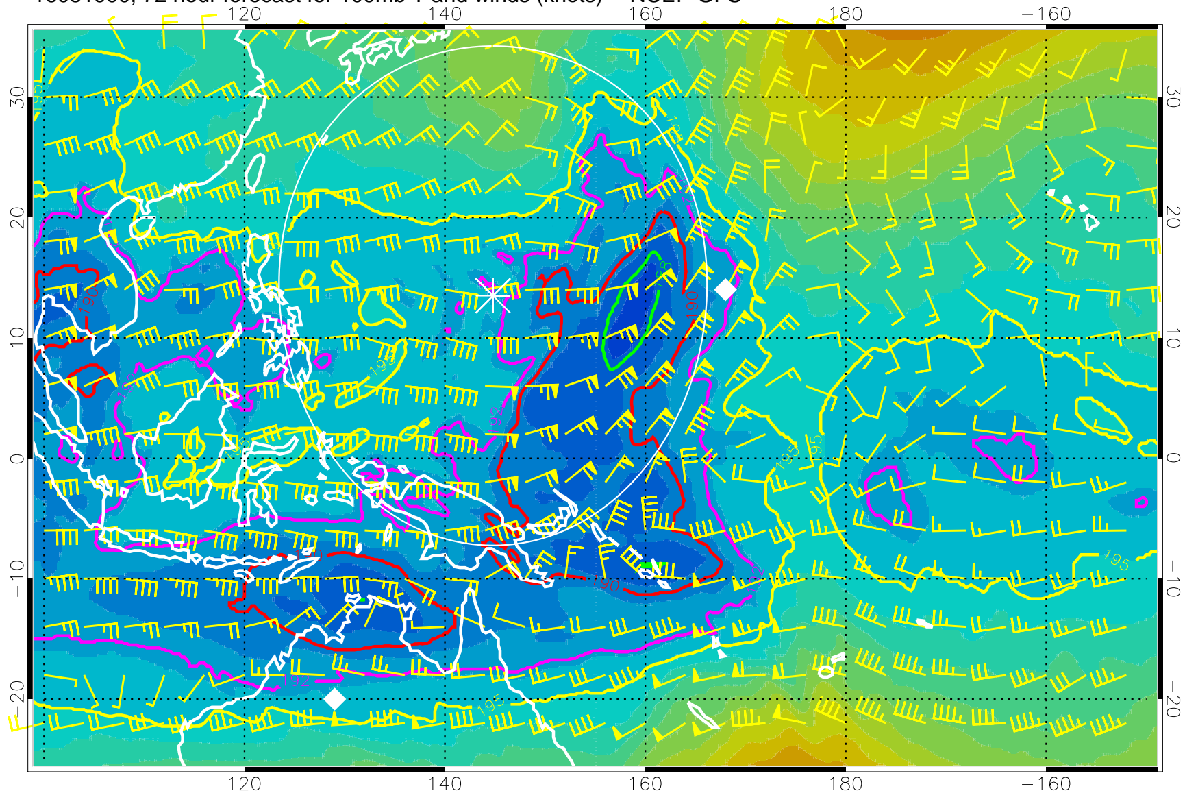
16081900, 72 hour forecast for 100mb T and winds (knots) -- NCEP GFS
