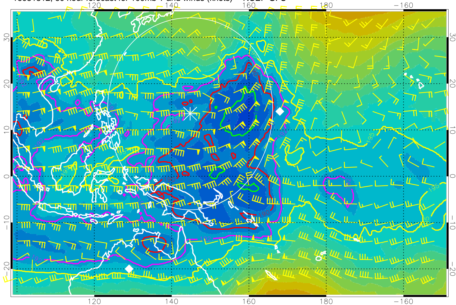
16081812, 60 hour forecast for 100mb T and winds (knots) -- NCEP GFS
