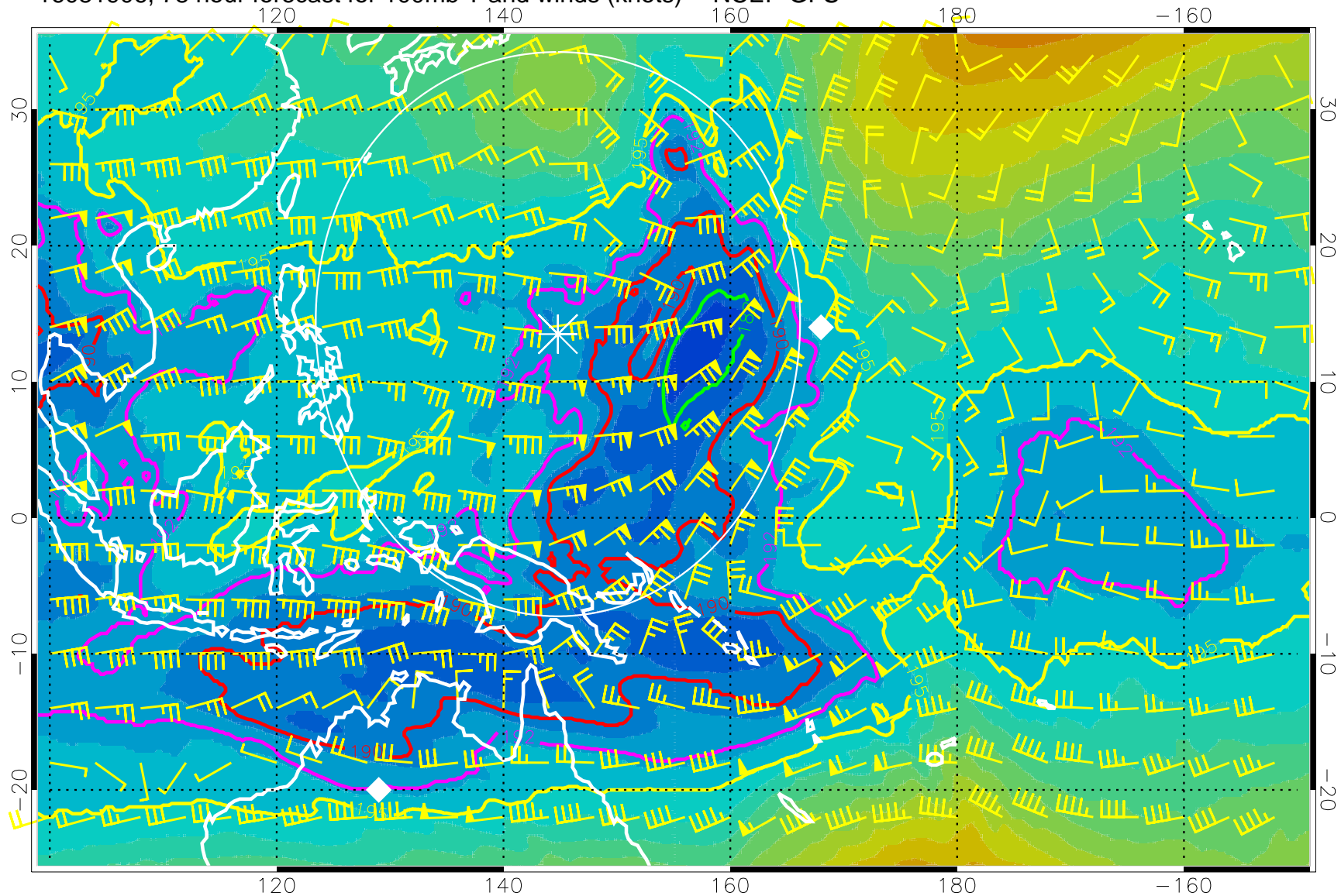
16081906, 78 hour forecast for 100mb T and winds (knots) -- NCEP GFS
