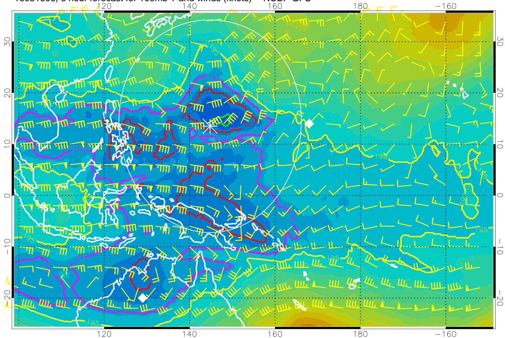
16081606, 6 hour forecast for 100mb T and winds (knots) -- NCEP GFS
