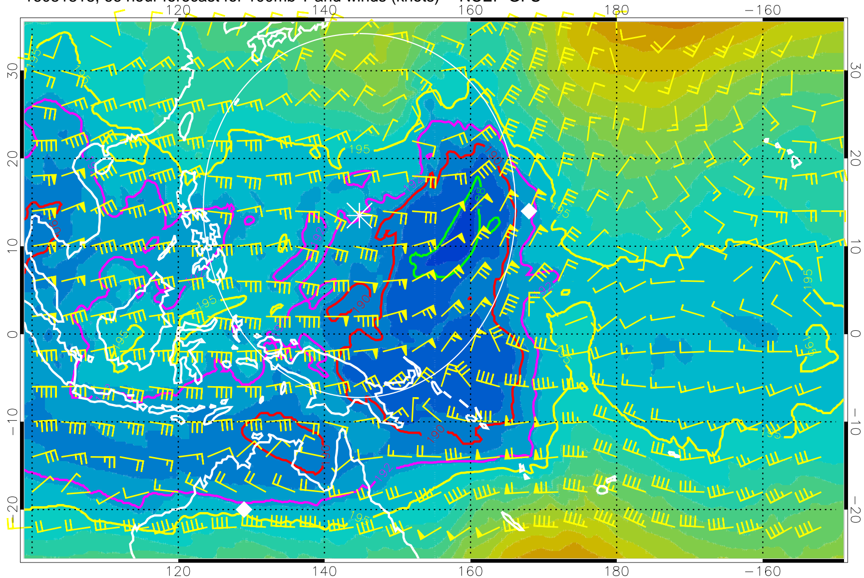
16081818, 66 hour forecast for 100mb T and winds (knots) -- NCEP GFS
