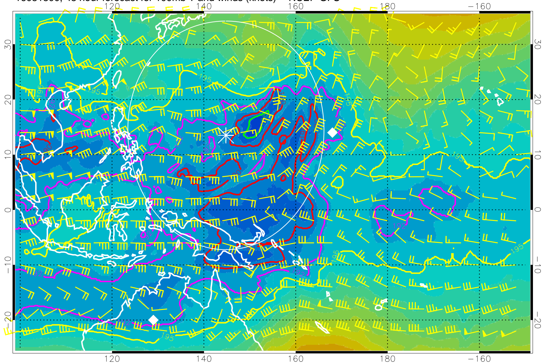
16081800, 48 hour forecast for 100mb T and winds (knots) -- NCEP GFS
