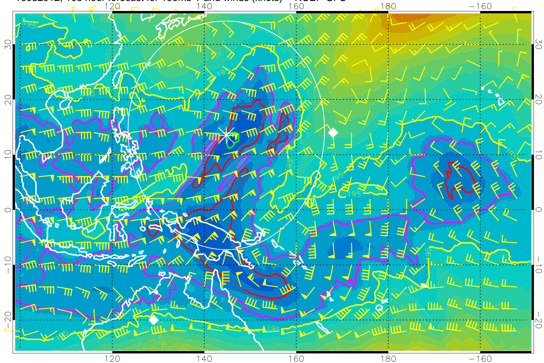
16082012, 108 hour forecast for 100mb T and winds (knots) -- NCEP GFS
