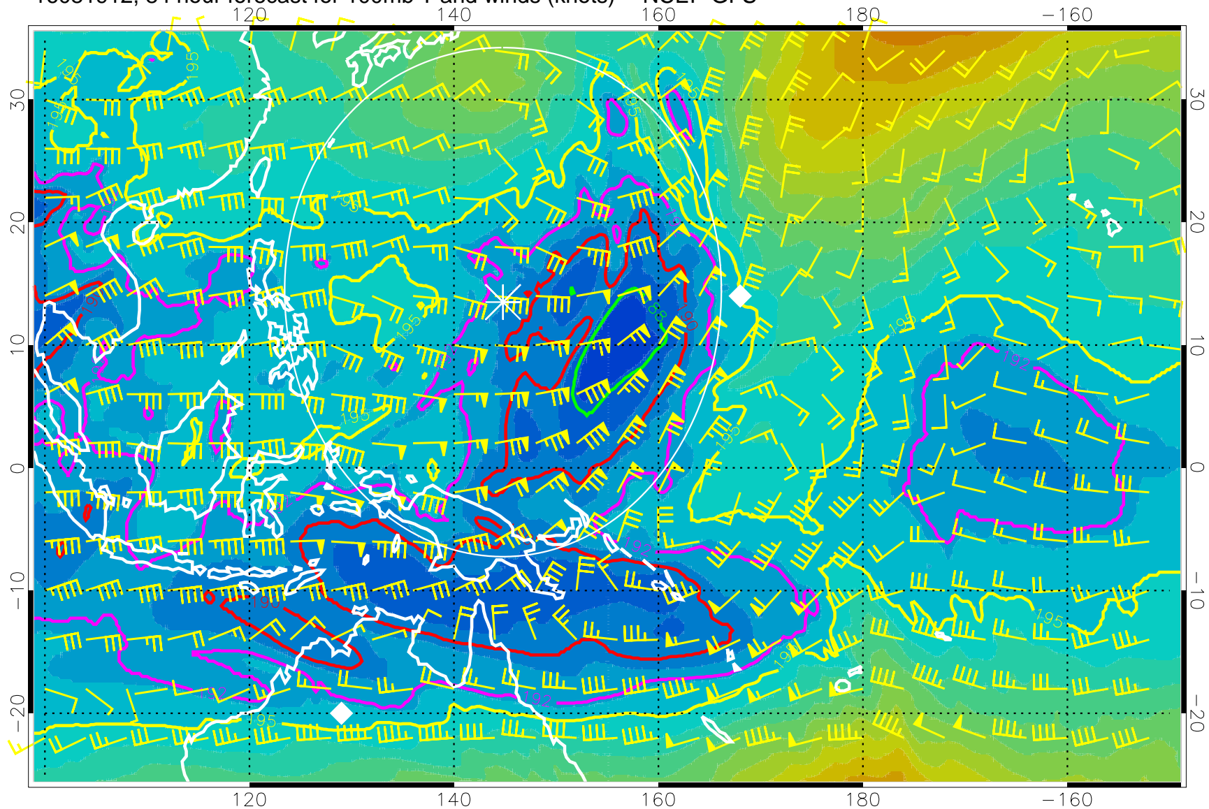
16081912, 84 hour forecast for 100mb T and winds (knots) -- NCEP GFS
