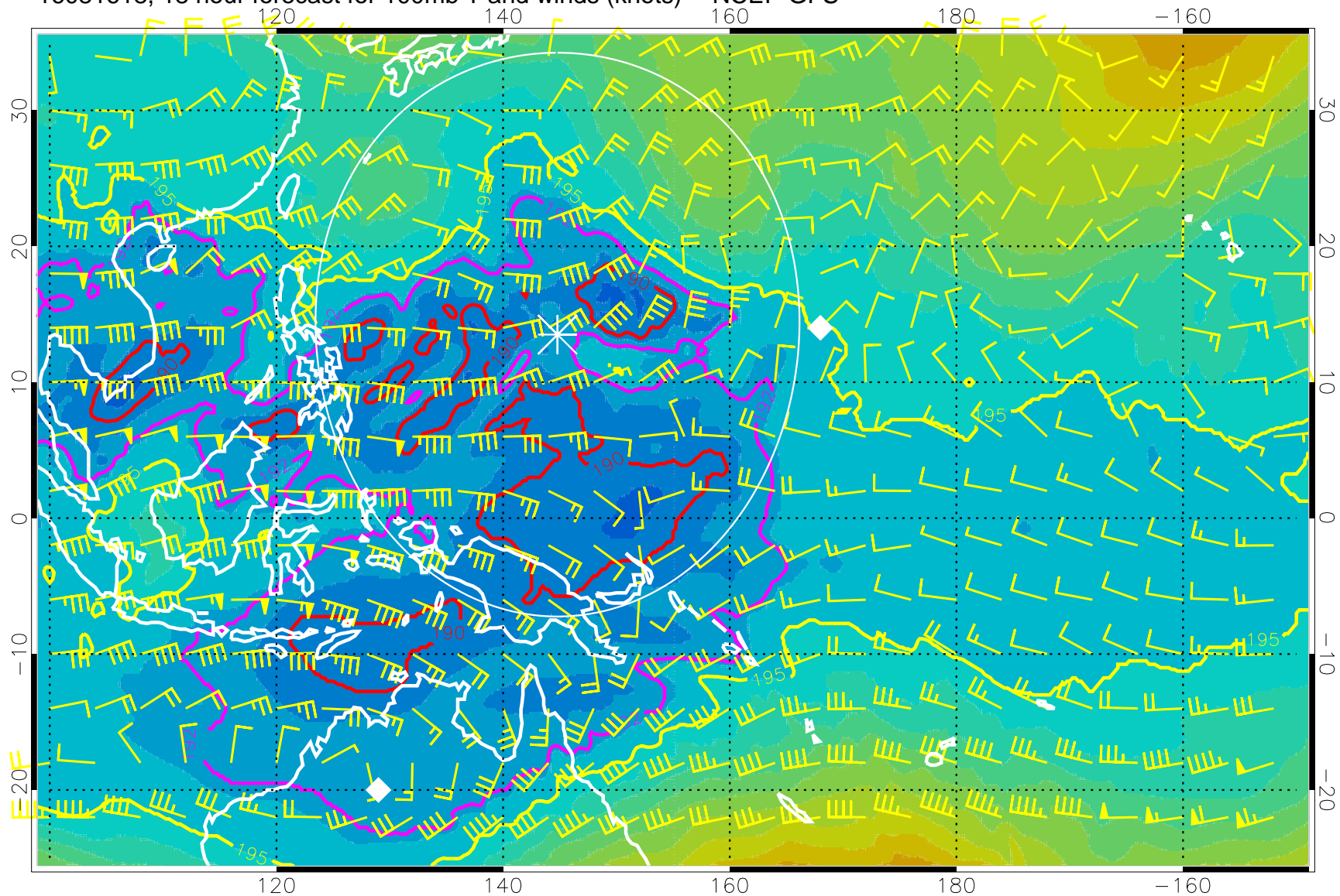
16081618, 18 hour forecast for 100mb T and winds (knots) -- NCEP GFS
