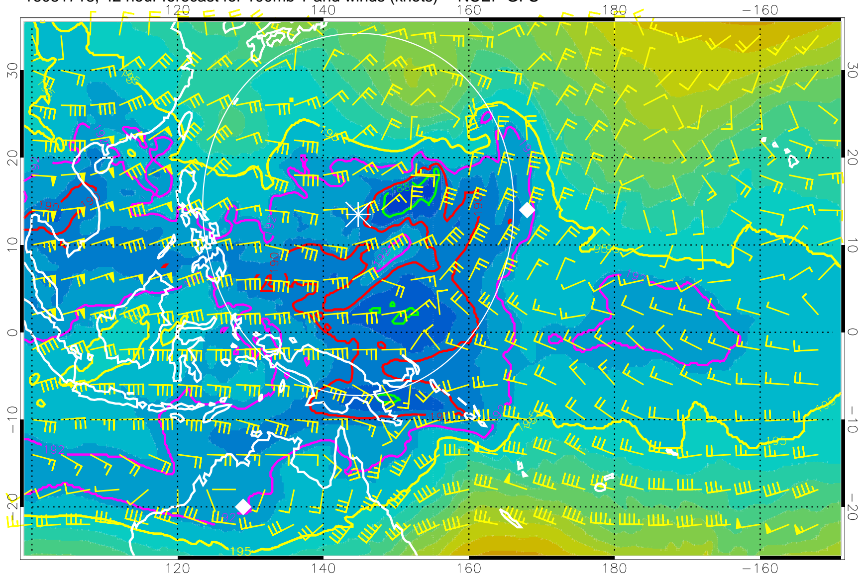
16081718, 42 hour forecast for 100mb T and winds (knots) -- NCEP GFS
