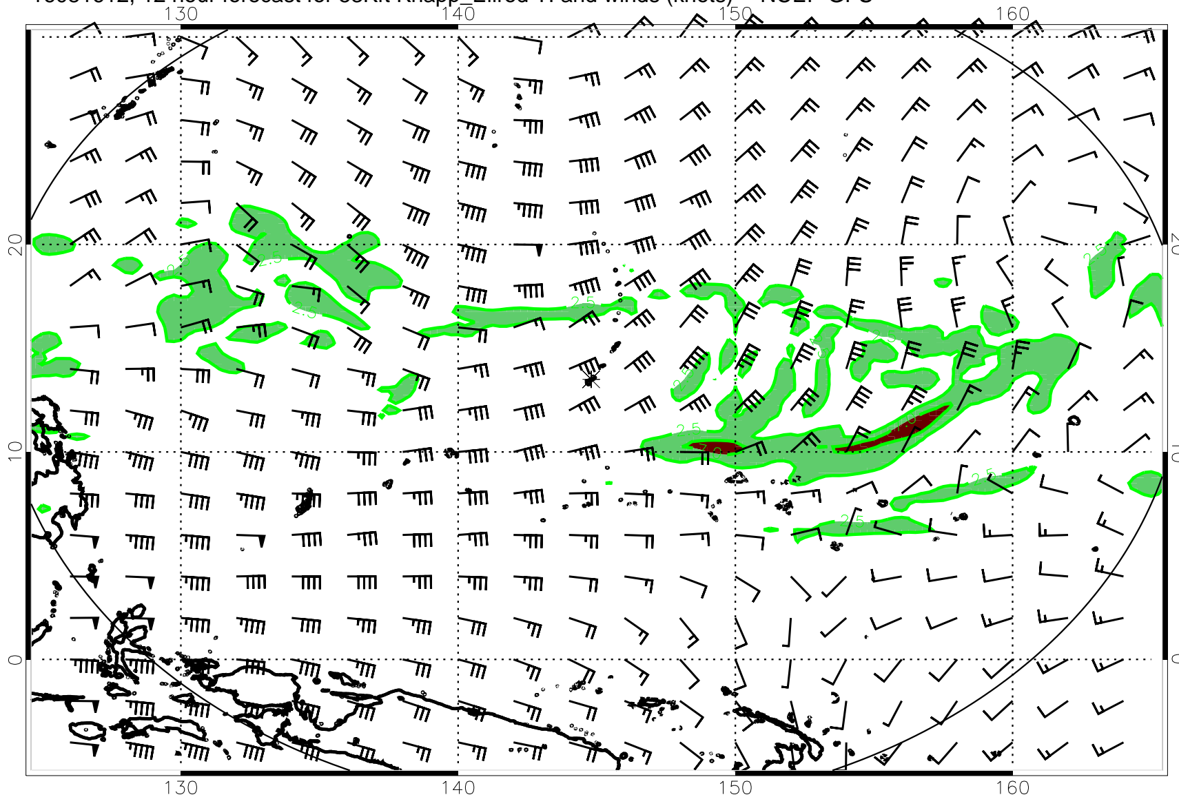
16081612, 12 hour forecast for 53Kft Knapp_Ellrod TI and winds (knots) -- NCEP GFS
