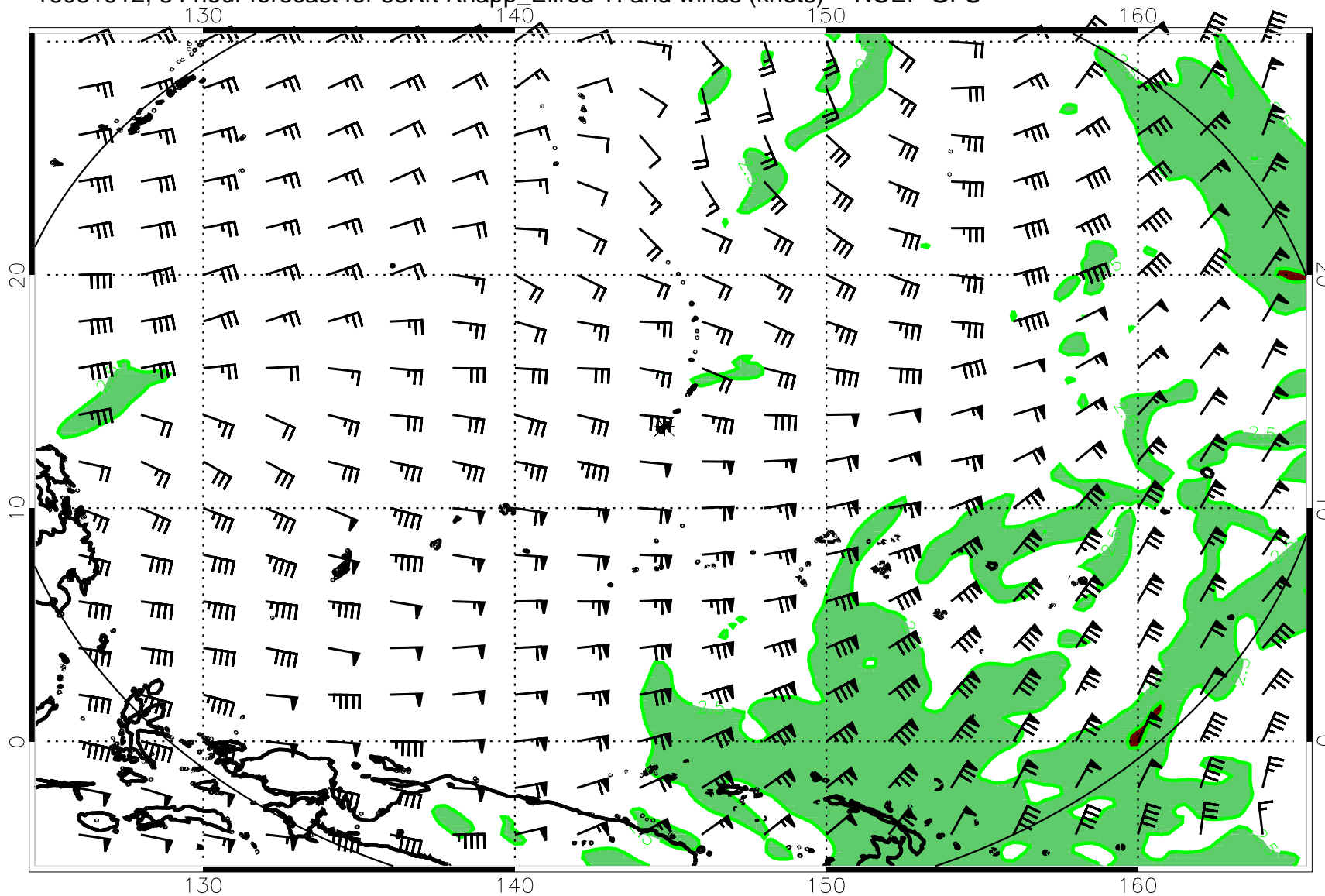
16081912, 84 hour forecast for 53Kft Knapp_Ellrod TI and winds (knots) -- NCEP GFS
