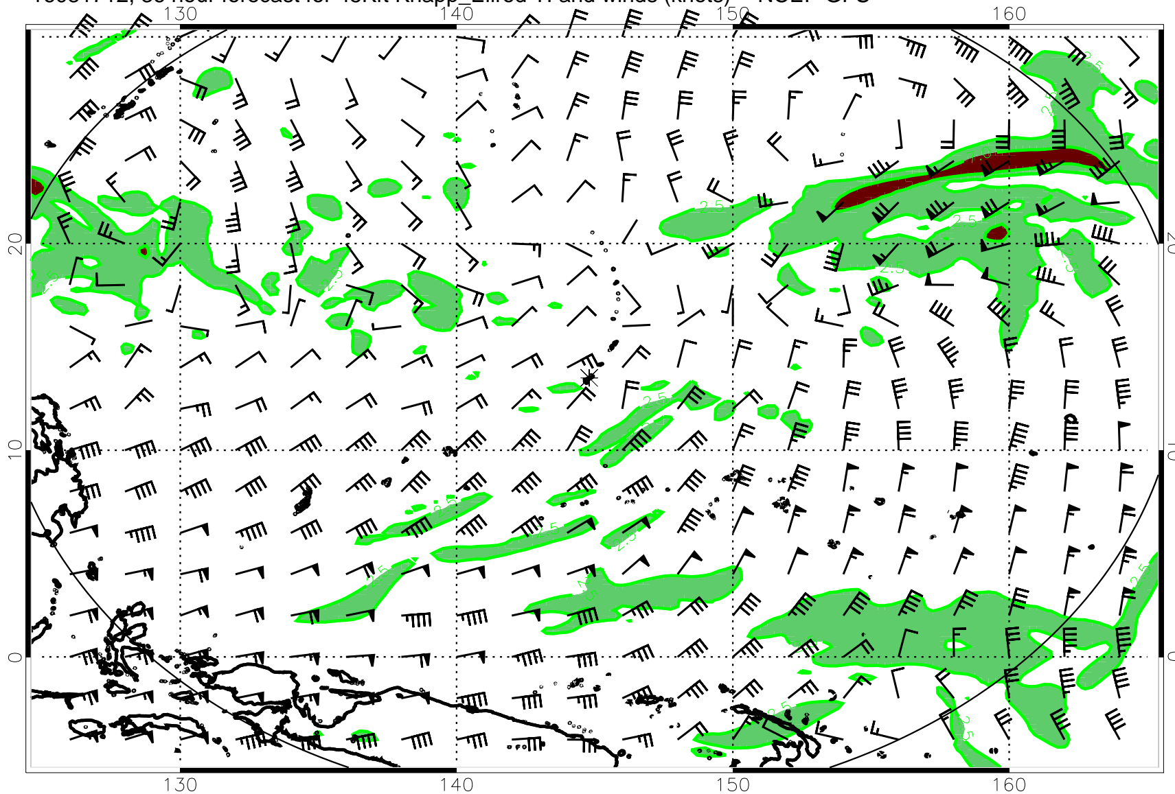
16081712, 36 hour forecast for 45Kft Knapp_Ellrod TI and winds (knots) -- NCEP GFS
