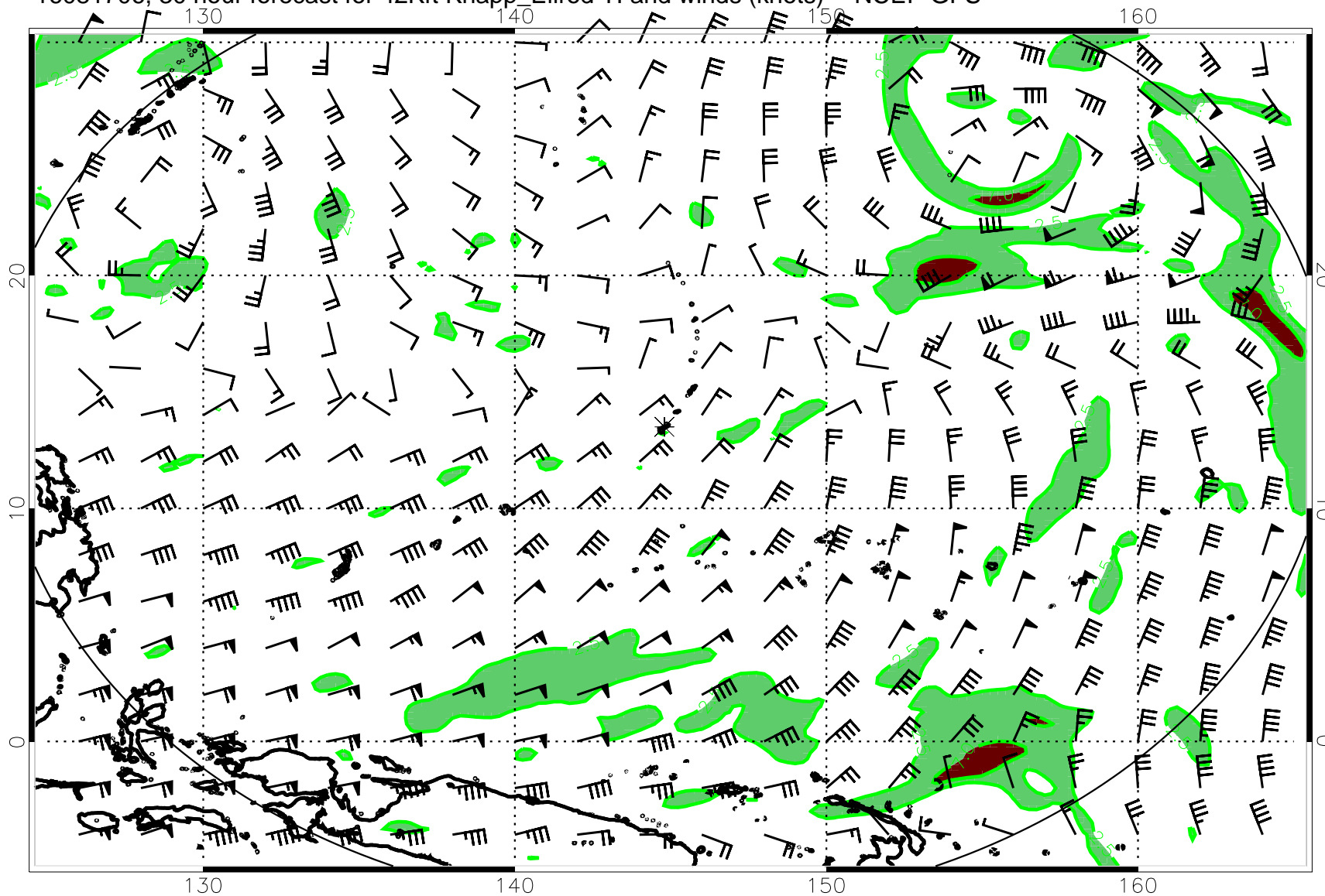
16081706, 30 hour forecast for 42Kft Knapp_Ellrod TI and winds (knots) -- NCEP GFS
