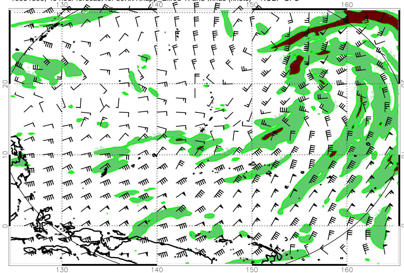
16081800, 48 hour forecast for 39Kft Knapp_Ellrod TI and winds (knots) -- NCEP GFS
