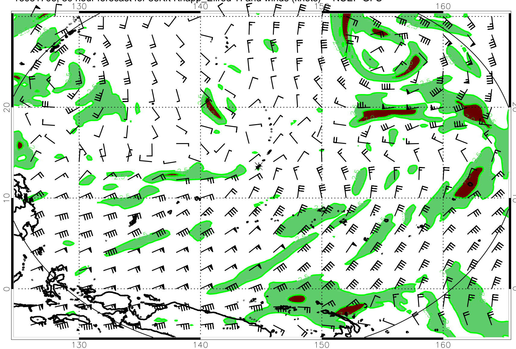
16081706, 30 hour forecast for 36Kft Knapp_Ellrod TI and winds (knots) -- NCEP GFS
