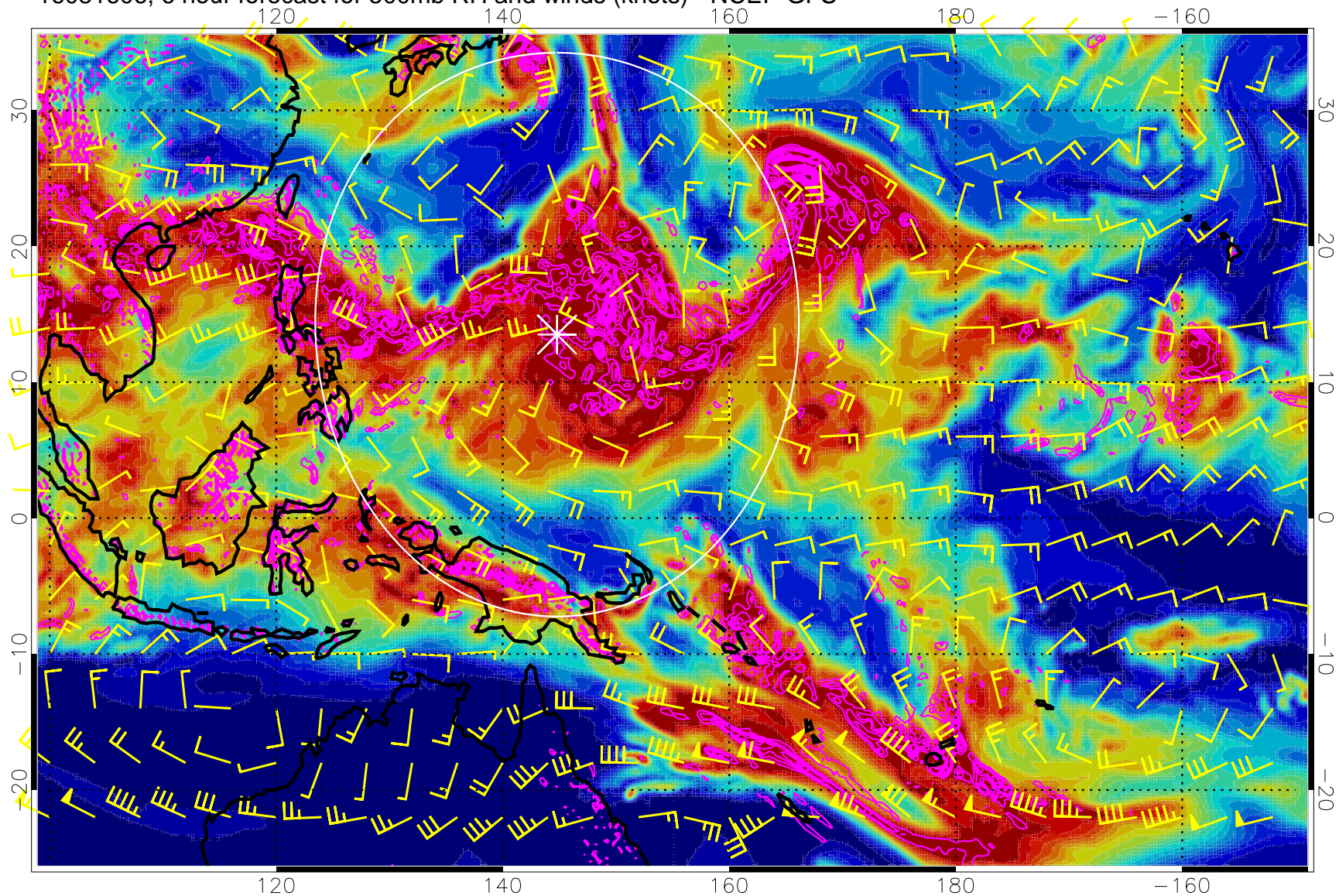
16081606, 6 hour forecast for 500mb RH and winds (knots) - NCEP GFS
