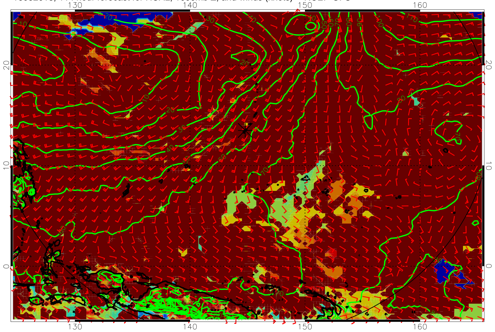
16082018, 114 hour forecast for HCAL, 1000mb Z, and winds (knots) -- NCEP GFS
