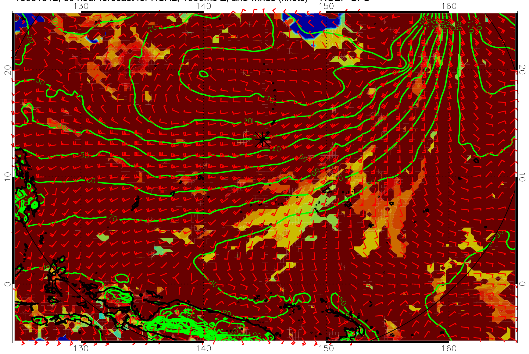
16081812, 60 hour forecast for HCAL, 1000mb Z, and winds (knots) -- NCEP GFS
