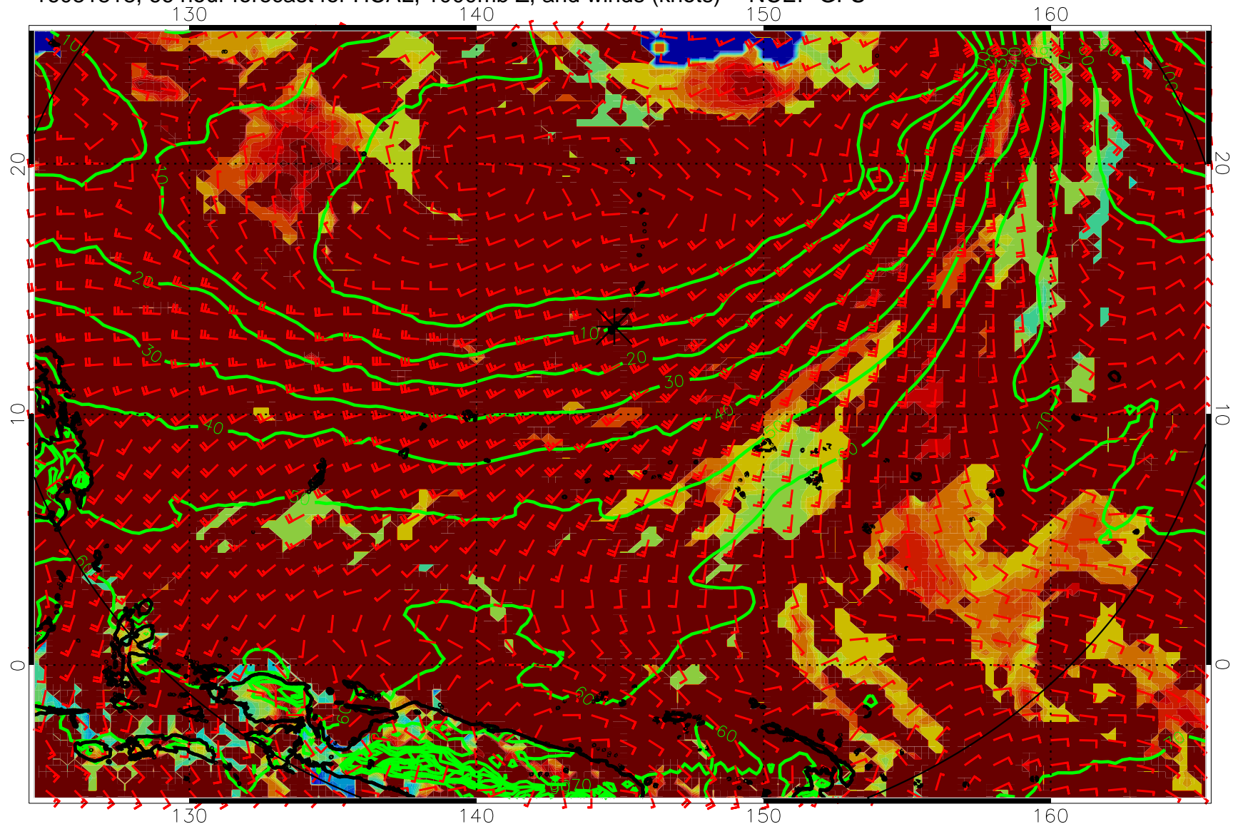
16081818, 66 hour forecast for HCAL, 1000mb Z, and winds (knots) -- NCEP GFS
