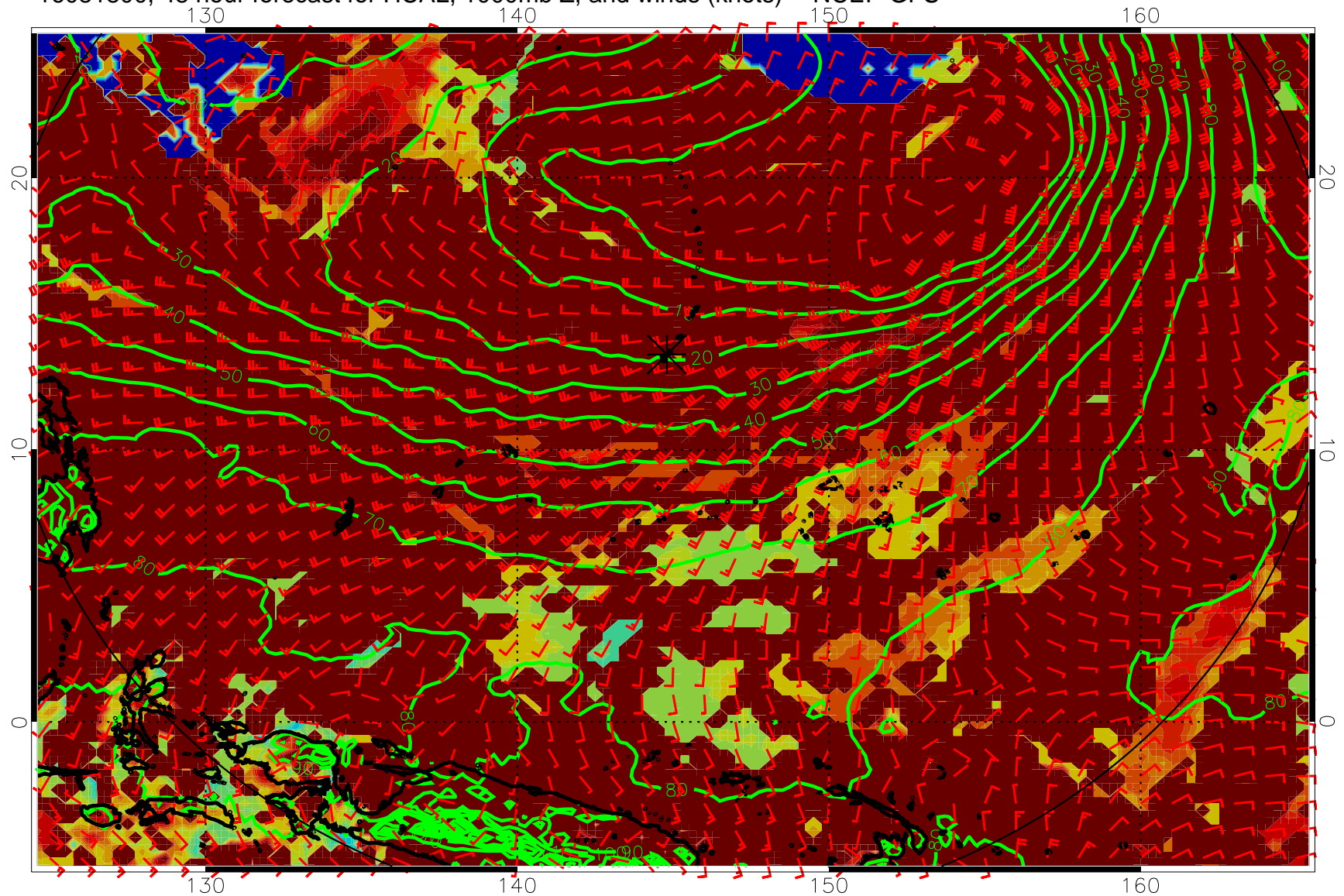
16081800, 48 hour forecast for HCAL, 1000mb Z, and winds (knots) -- NCEP GFS
