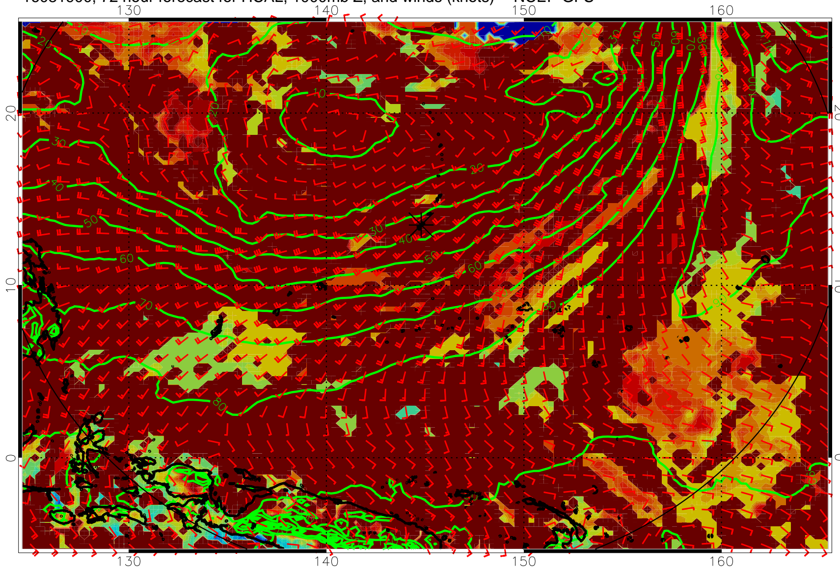
16081900, 72 hour forecast for HCAL, 1000mb Z, and winds (knots) -- NCEP GFS
