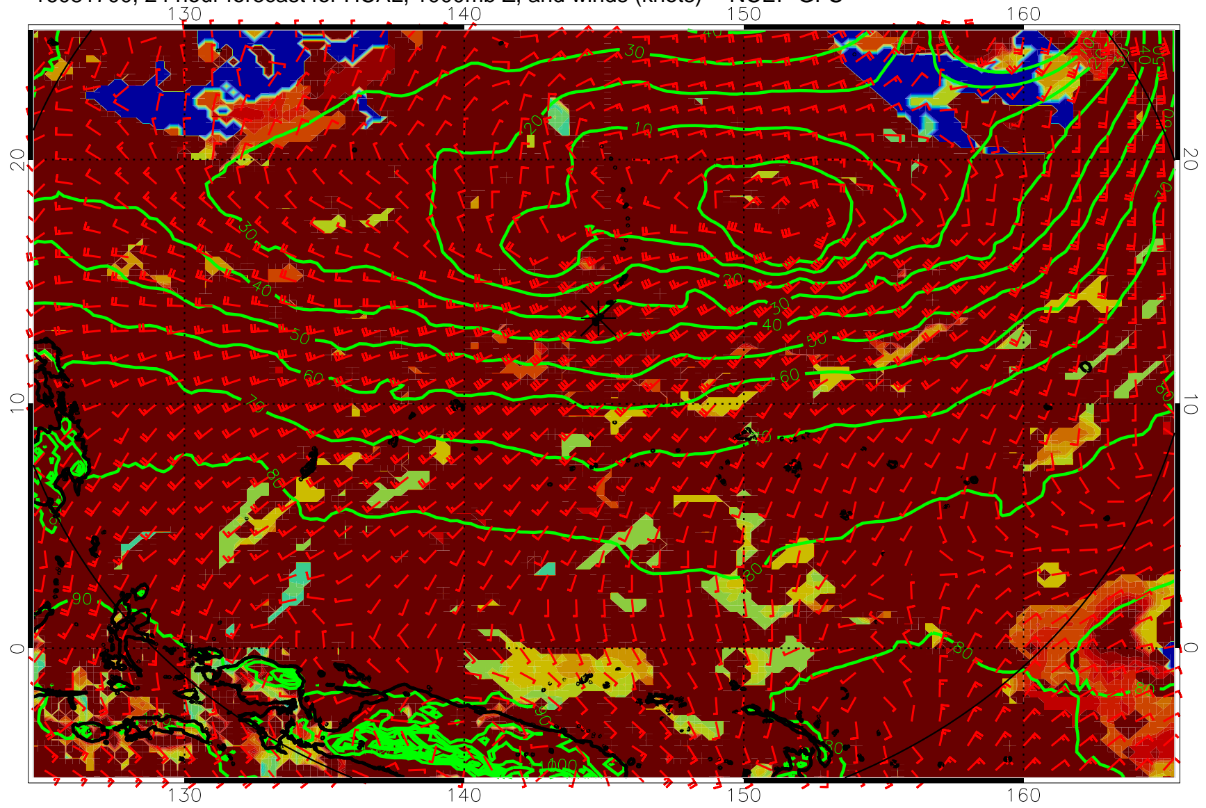
16081700, 24 hour forecast for HCAL, 1000mb Z, and winds (knots) -- NCEP GFS
