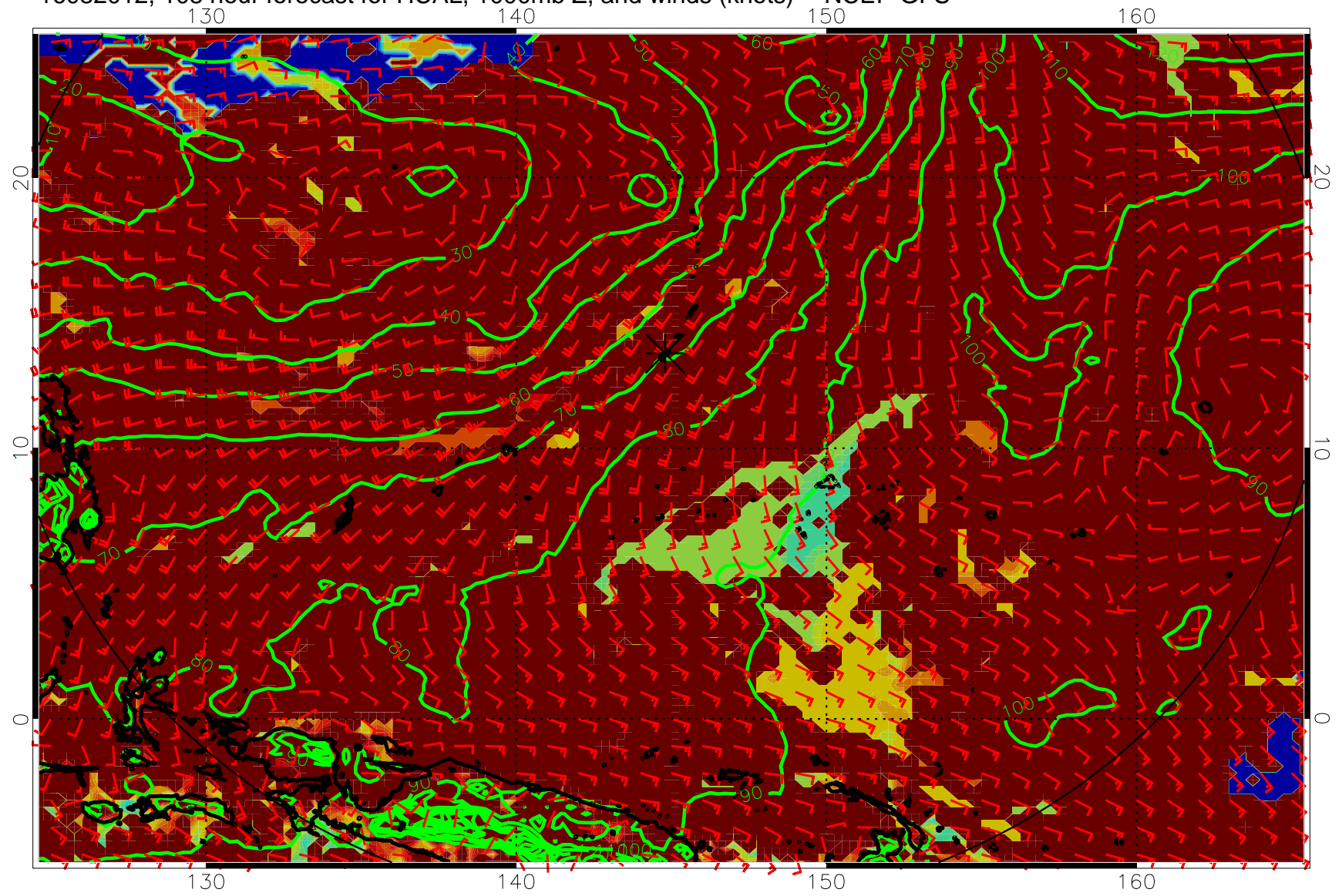
16082012, 108 hour forecast for HCAL, 1000mb Z, and winds (knots) -- NCEP GFS
