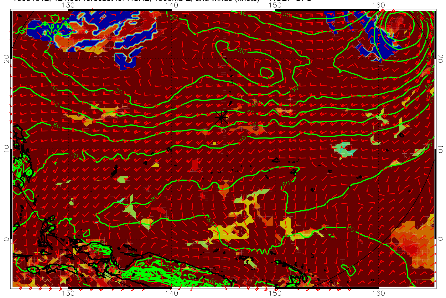
16081612, 12 hour forecast for HCAL, 1000mb Z, and winds (knots) -- NCEP GFS
