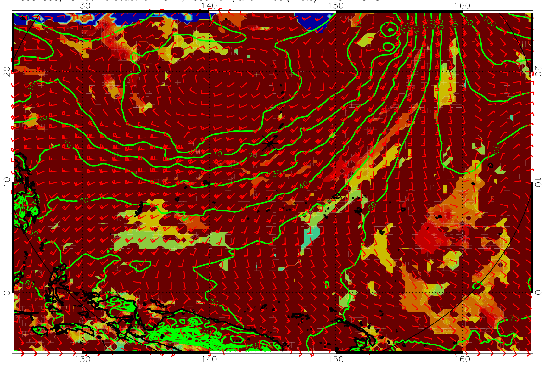
16081906, 78 hour forecast for HCAL, 1000mb Z, and winds (knots) -- NCEP GFS
