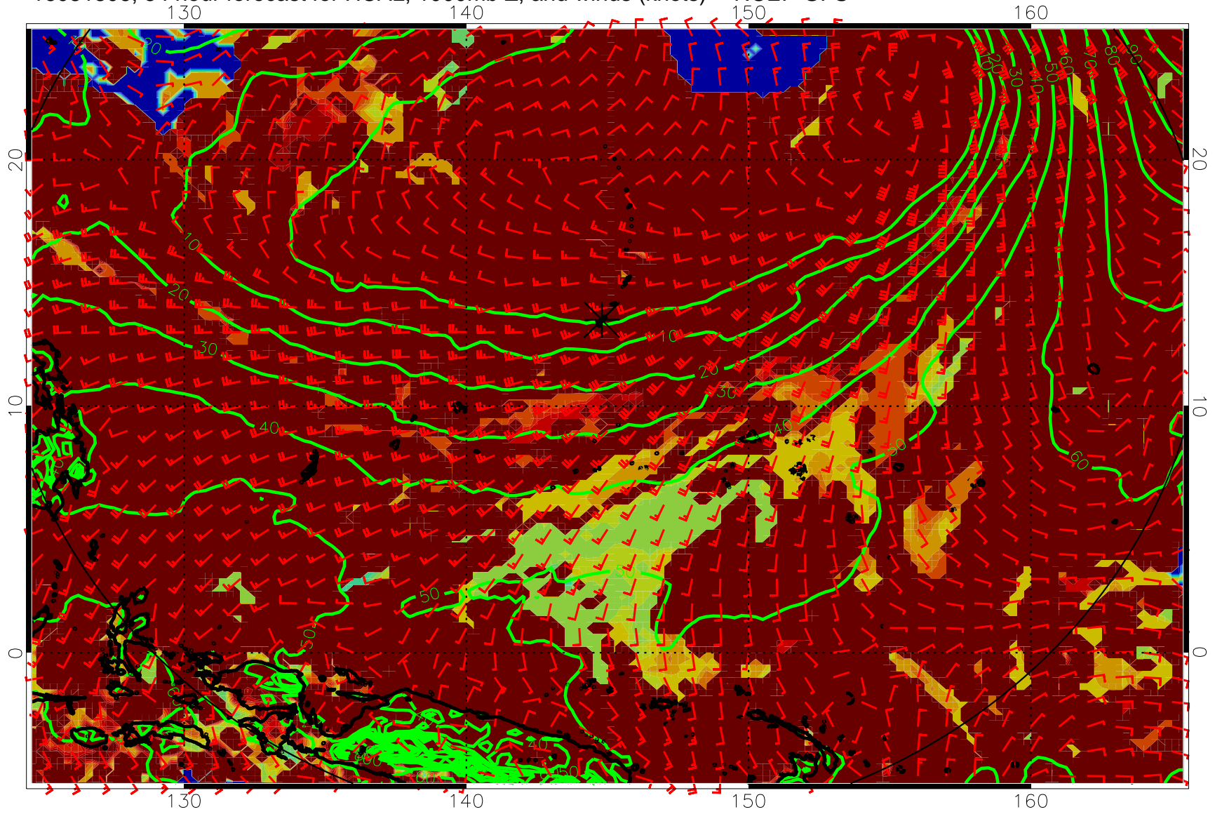
16081806, 54 hour forecast for HCAL, 1000mb Z, and winds (knots) -- NCEP GFS
