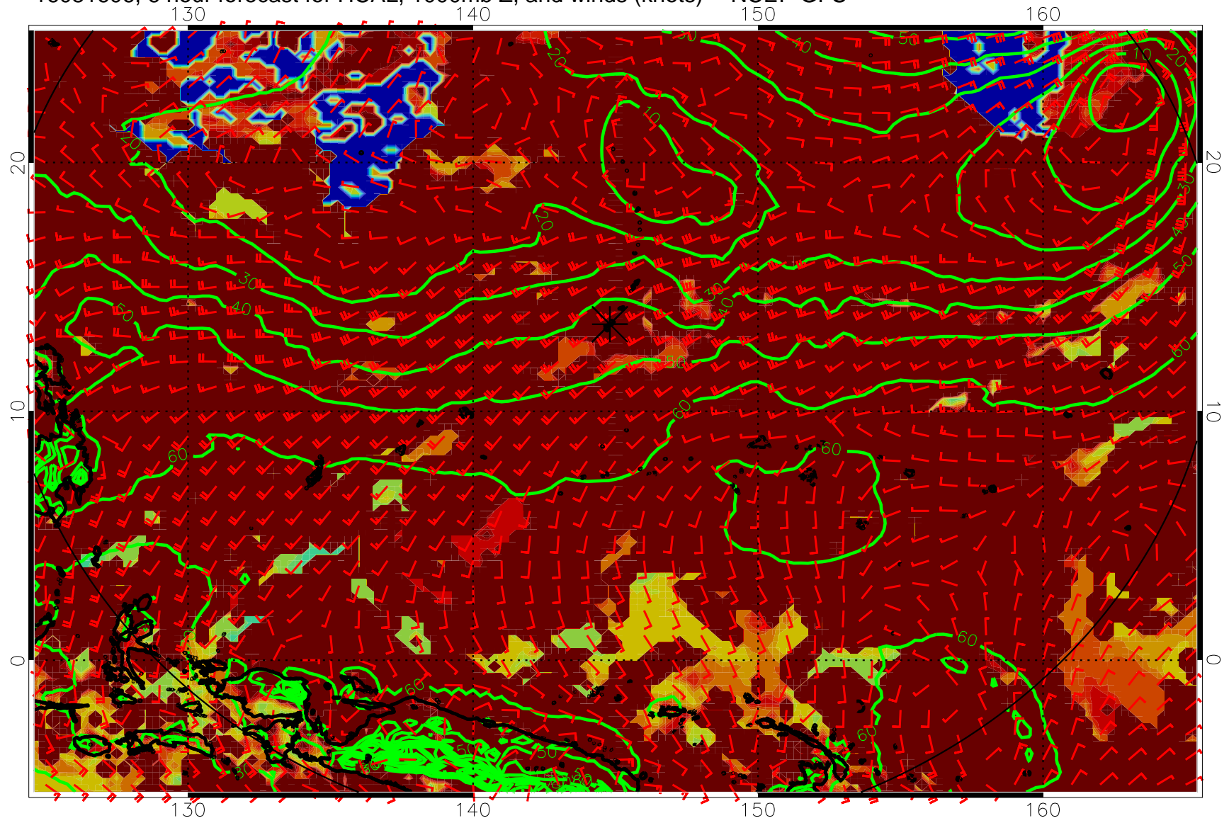
16081606, 6 hour forecast for HCAL, 1000mb Z, and winds (knots) -- NCEP GFS
