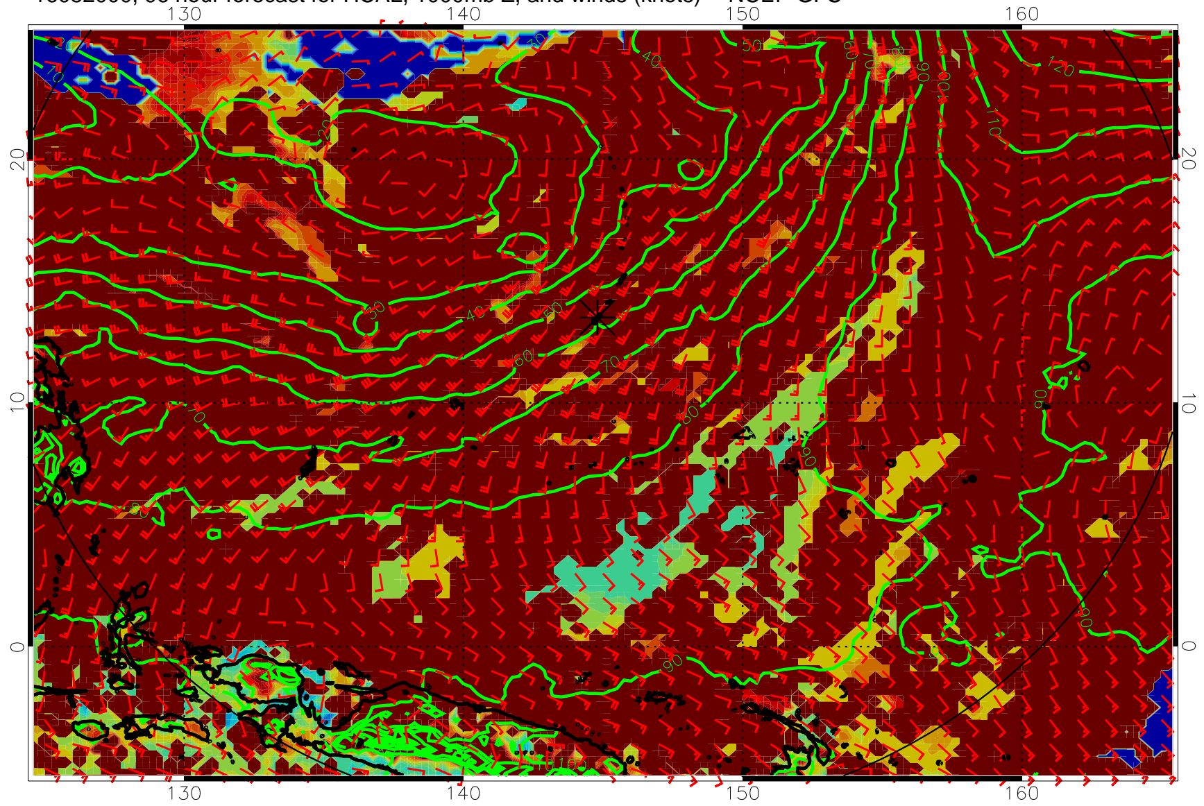
16082000, 96 hour forecast for HCAL, 1000mb Z, and winds (knots) -- NCEP GFS
