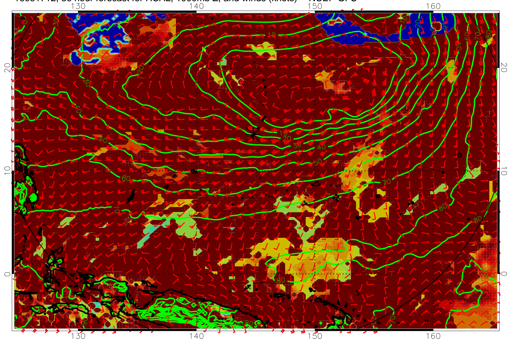
16081712, 36 hour forecast for HCAL, 1000mb Z, and winds (knots) -- NCEP GFS
