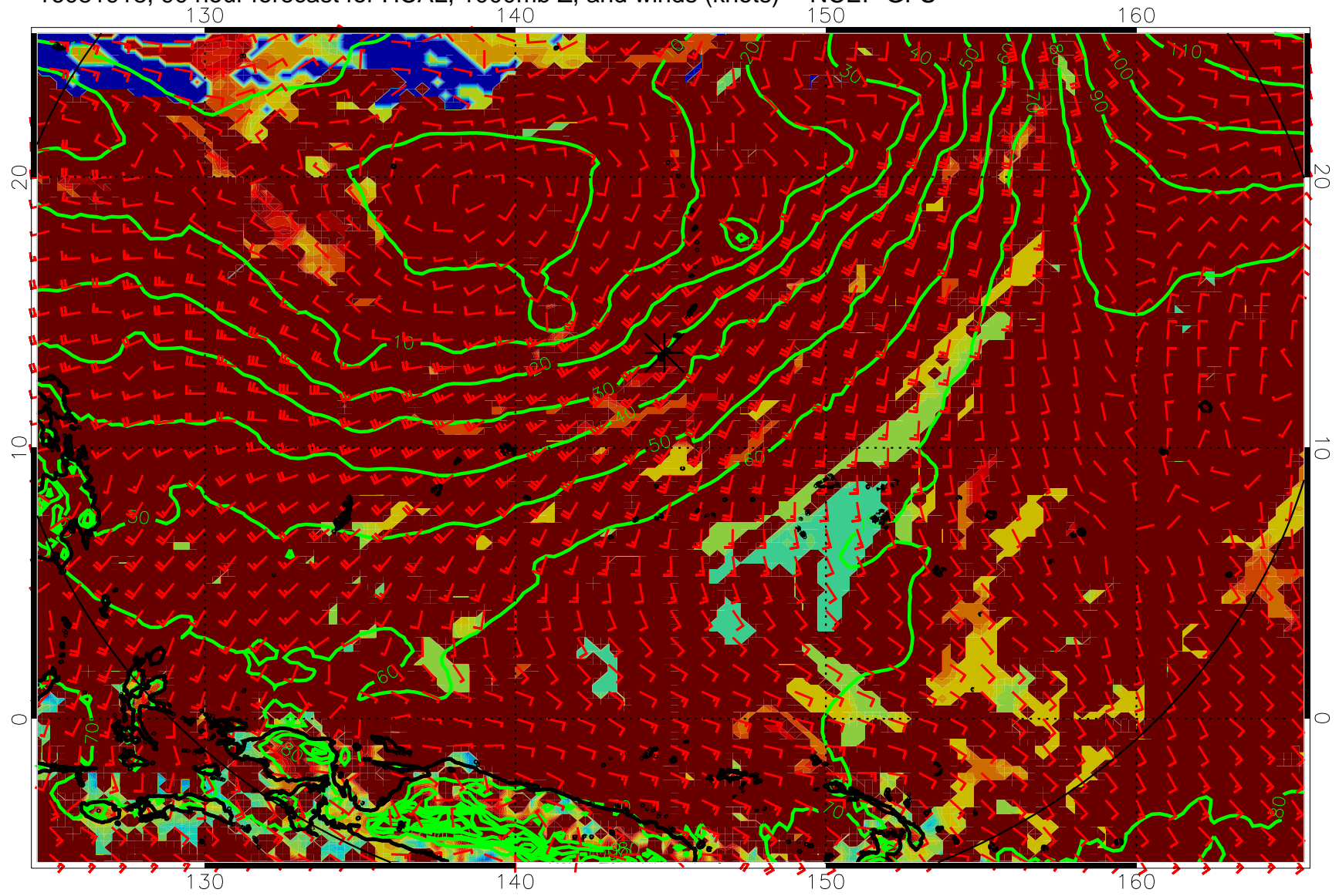
16081918, 90 hour forecast for HCAL, 1000mb Z, and winds (knots) -- NCEP GFS
