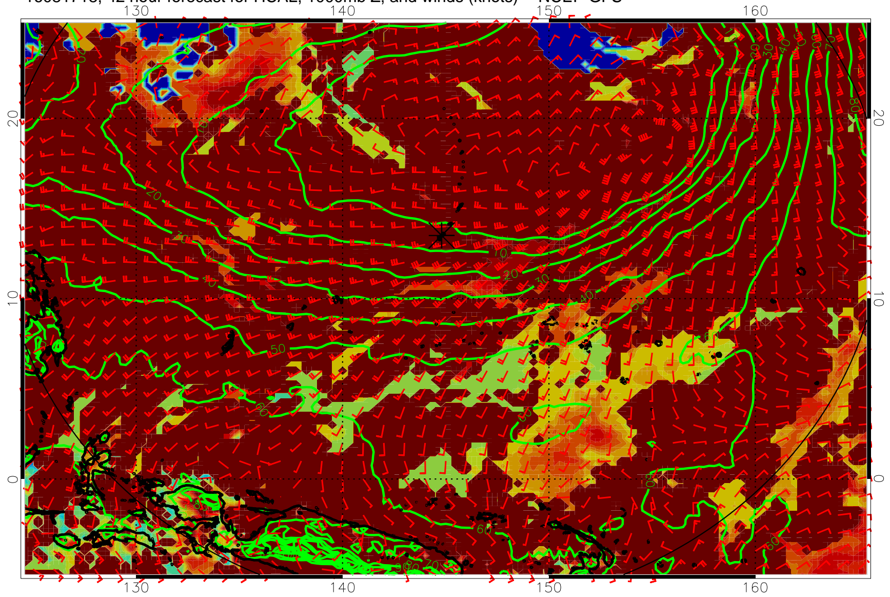
16081718, 42 hour forecast for HCAL, 1000mb Z, and winds (knots) -- NCEP GFS
