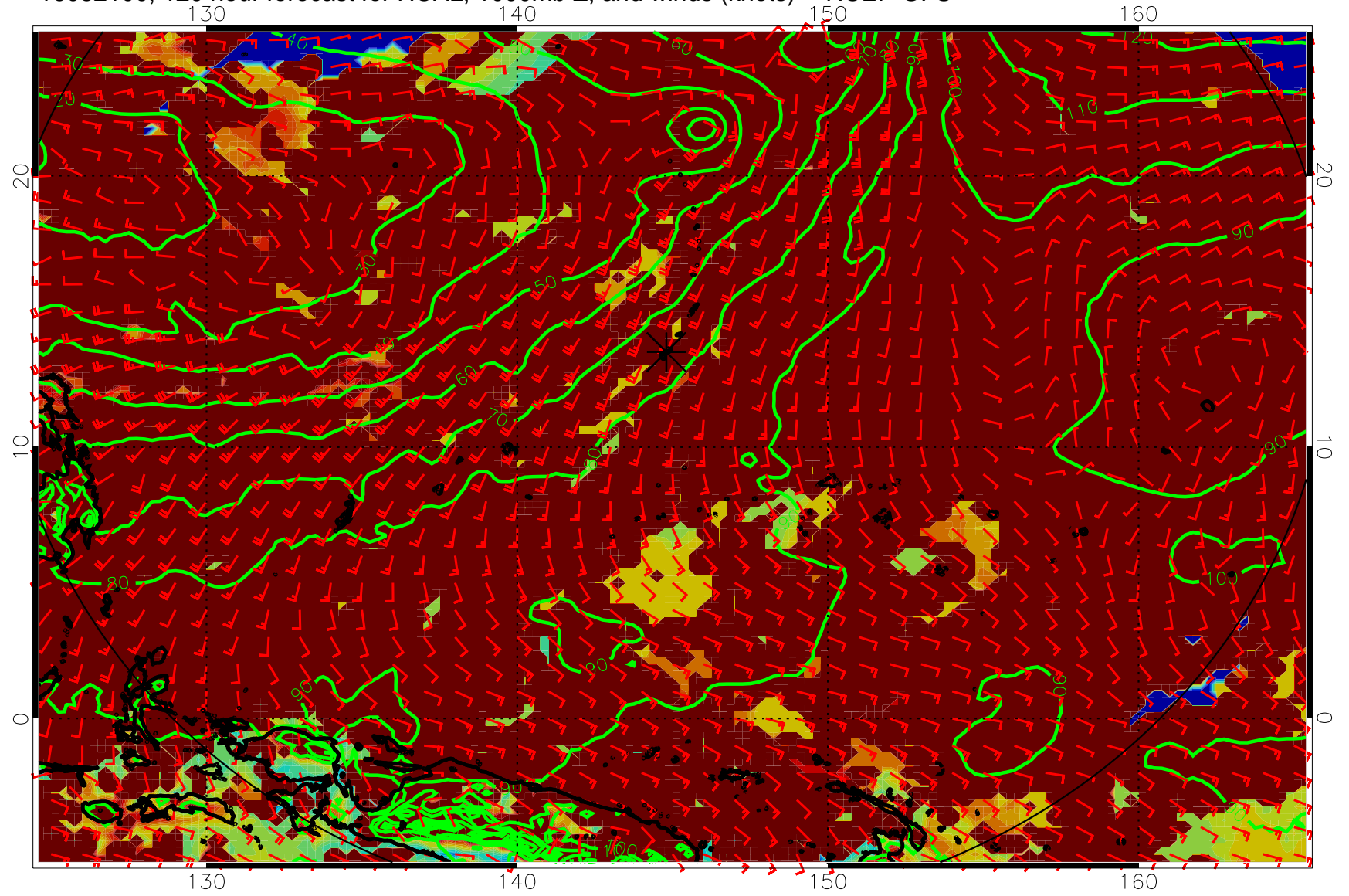
16082100, 120 hour forecast for HCAL, 1000mb Z, and winds (knots) -- NCEP GFS
