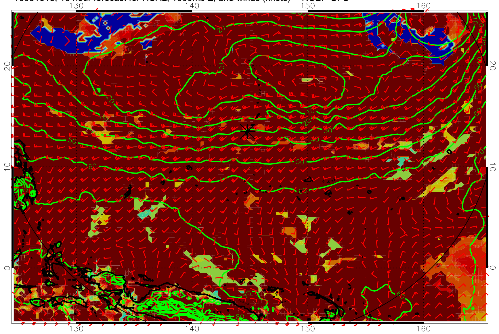
16081618, 18 hour forecast for HCAL, 1000mb Z, and winds (knots) -- NCEP GFS
