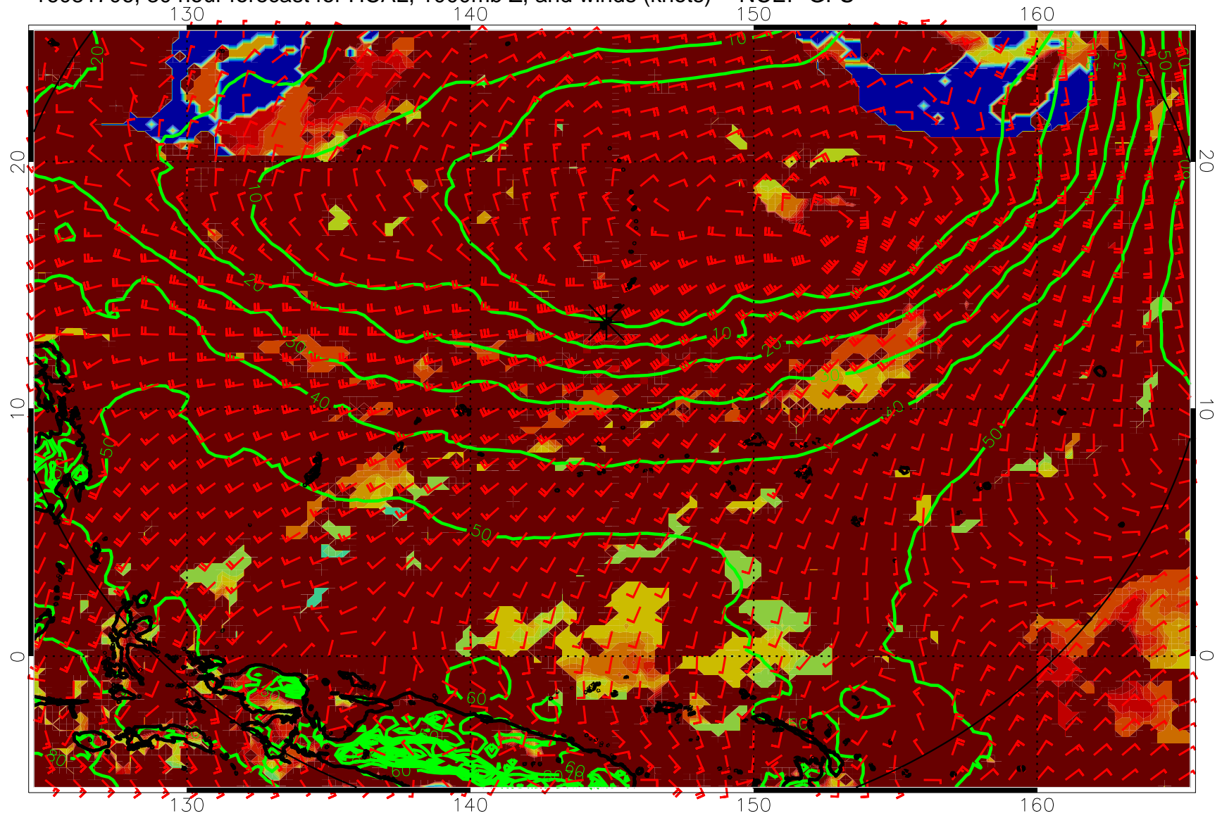
16081706, 30 hour forecast for HCAL, 1000mb Z, and winds (knots) -- NCEP GFS
