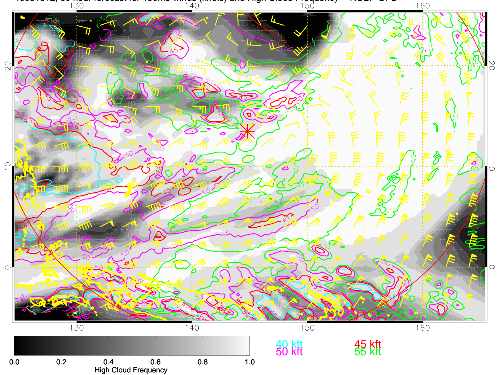
16081812, 60 hour forecast for 150mb winds (knots) and High Cloud Frequency -- NCEP GFS
