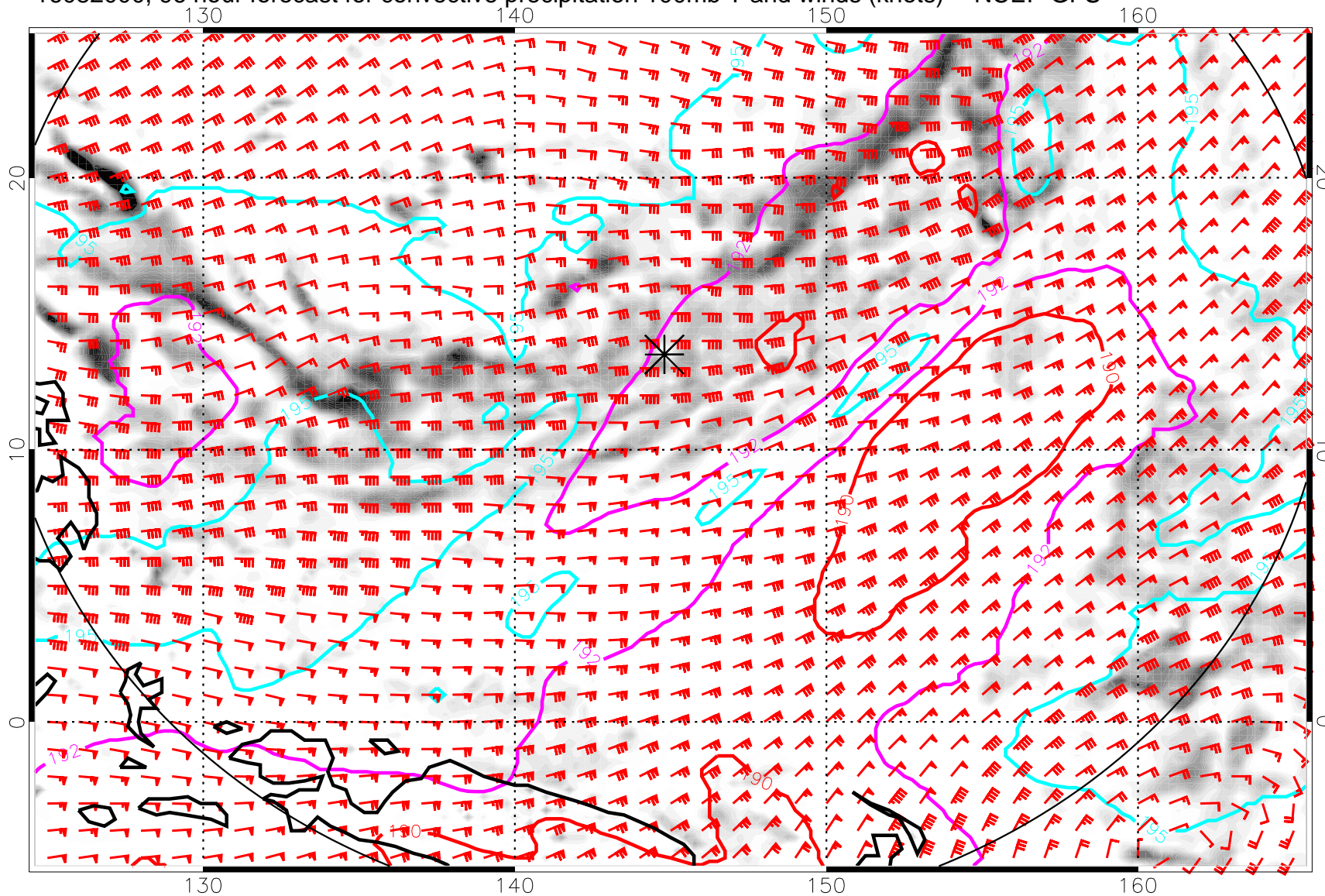
16082000, 96 hour forecast for convective precipitation 100mb T and winds (knots) -- NCEP GFS
