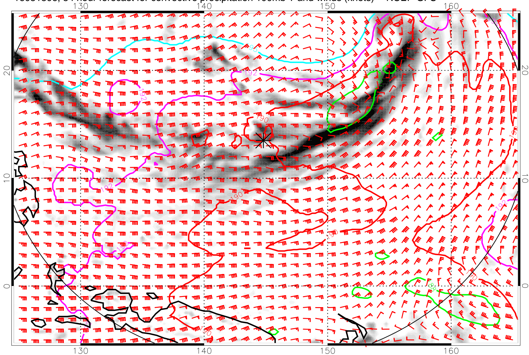
16081806, 54 hour forecast for convective precipitation 100mb T and winds (knots) -- NCEP GFS
