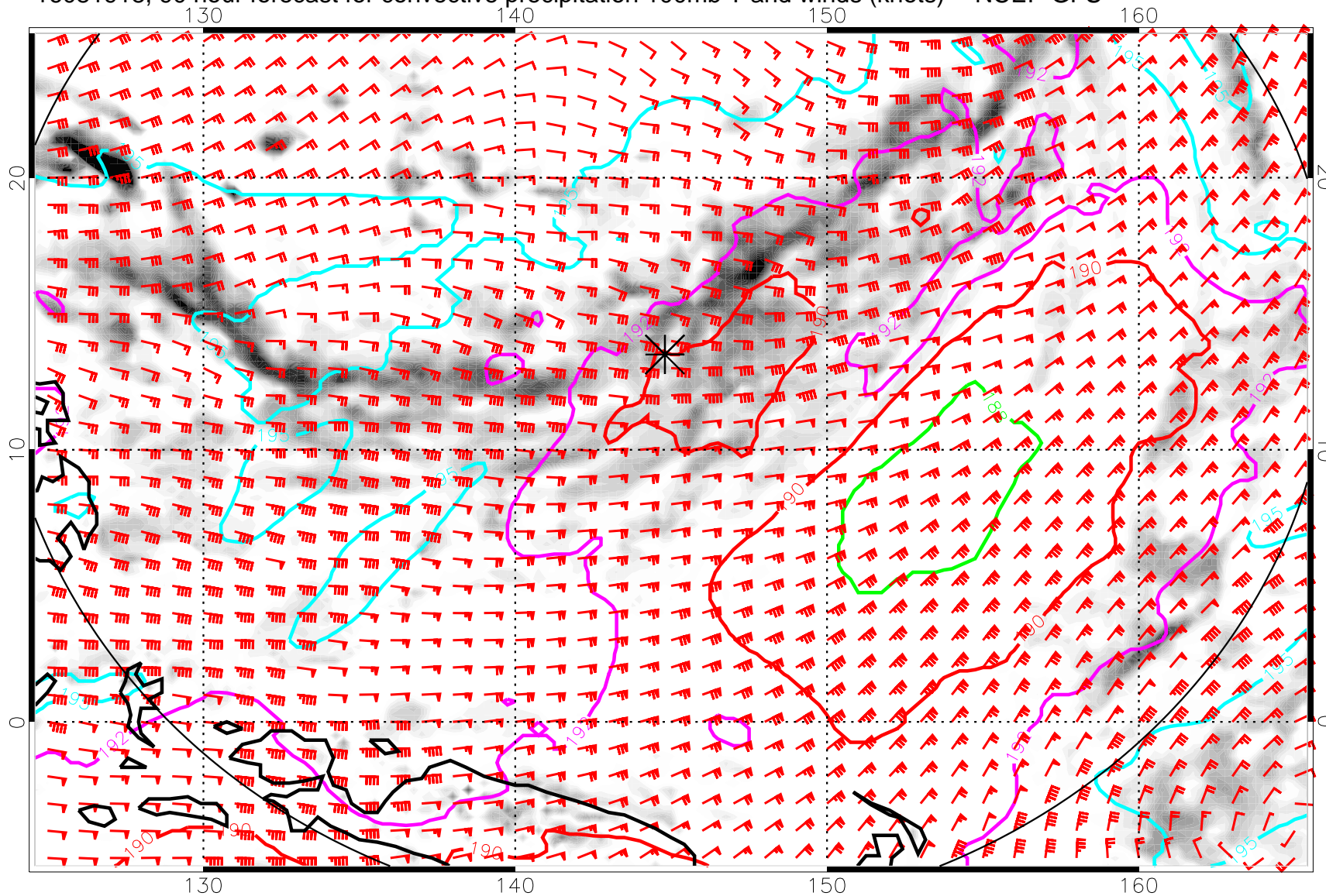
16081918, 90 hour forecast for convective precipitation 100mb T and winds (knots) -- NCEP GFS
