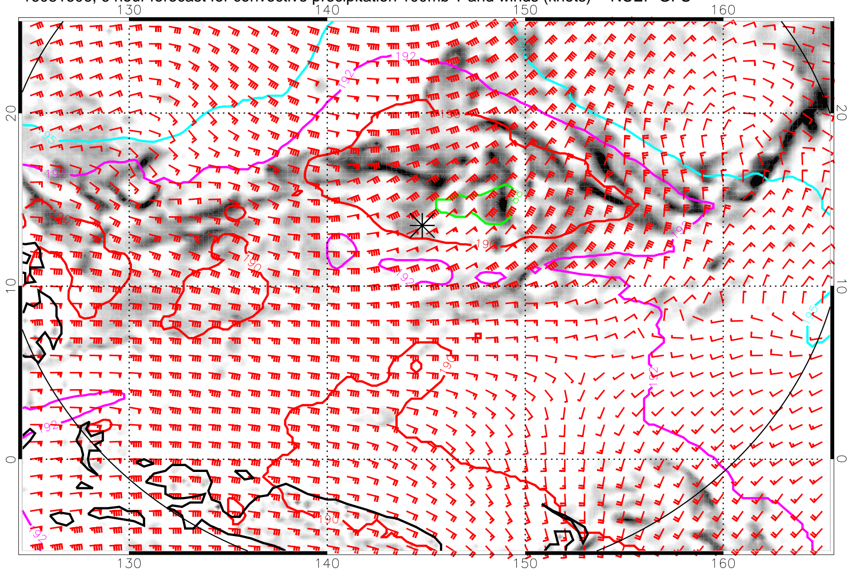
16081606, 6 hour forecast for convective precipitation 100mb T and winds (knots) -- NCEP GFS
