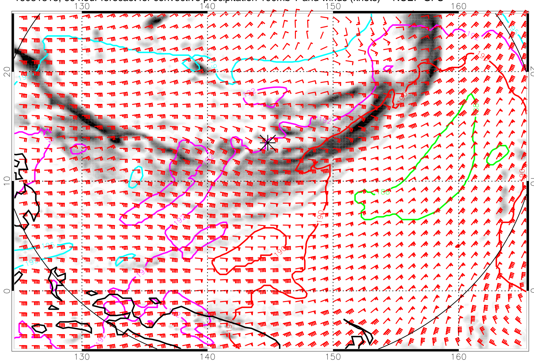
16081818, 66 hour forecast for convective precipitation 100mb T and winds (knots) -- NCEP GFS
