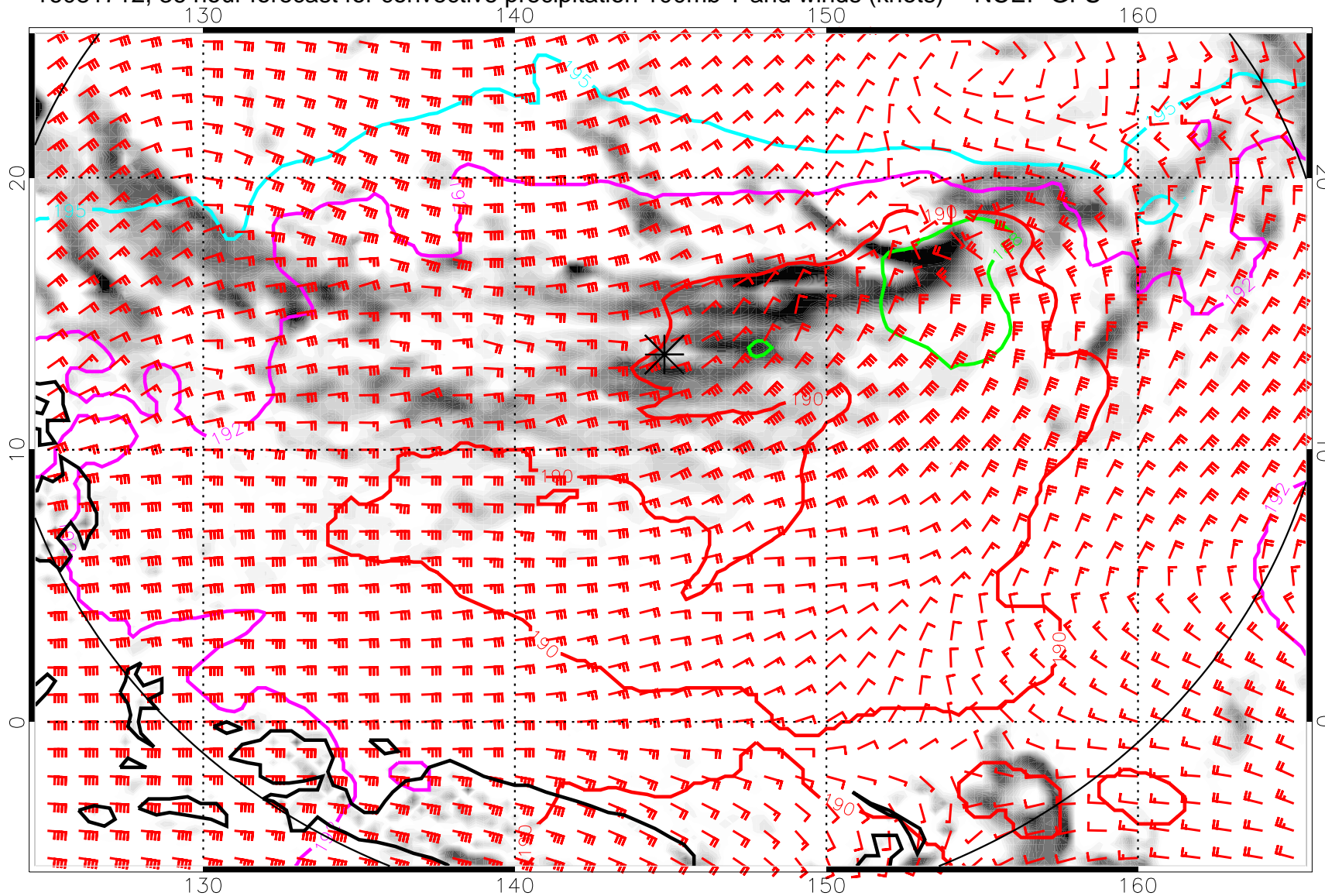
16081712, 36 hour forecast for convective precipitation 100mb T and winds (knots) -- NCEP GFS
