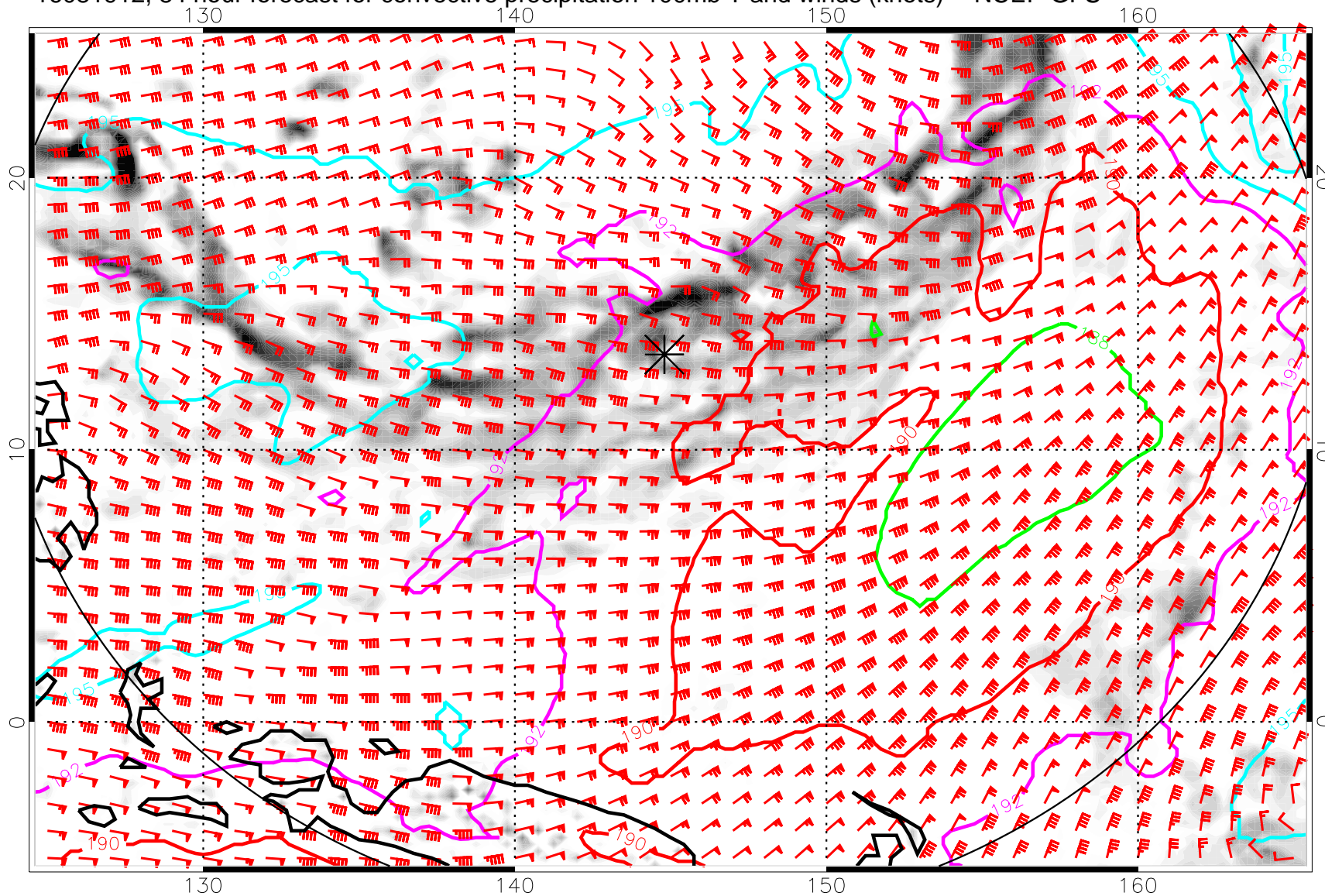
16081912, 84 hour forecast for convective precipitation 100mb T and winds (knots) -- NCEP GFS
