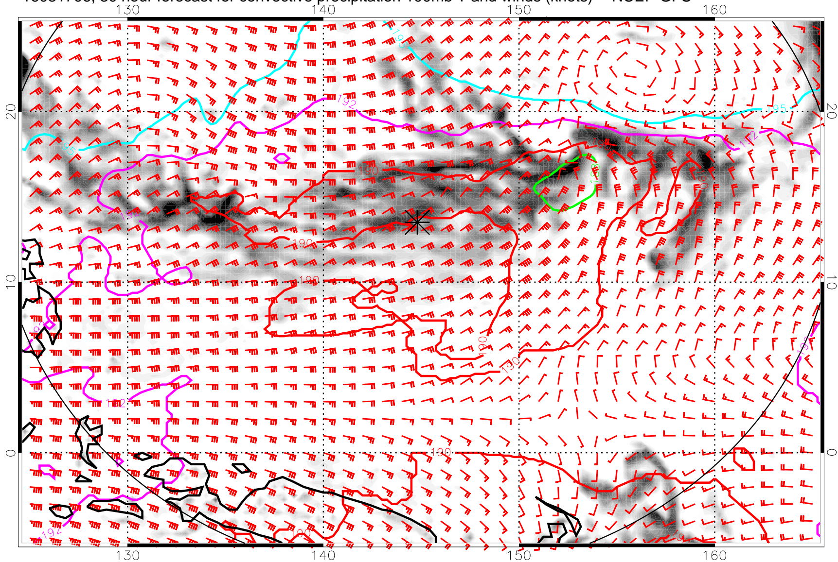
16081706, 30 hour forecast for convective precipitation 100mb T and winds (knots) -- NCEP GFS
