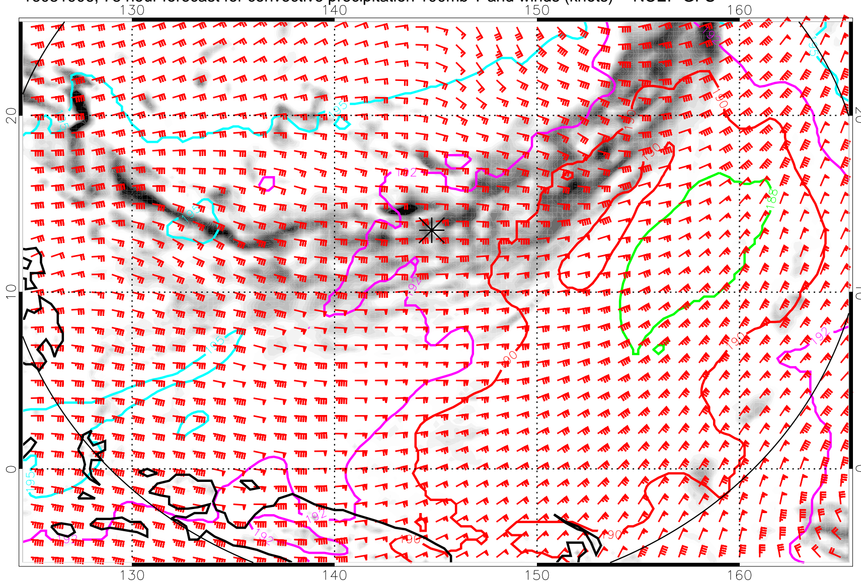
16081906, 78 hour forecast for convective precipitation 100mb T and winds (knots) -- NCEP GFS
