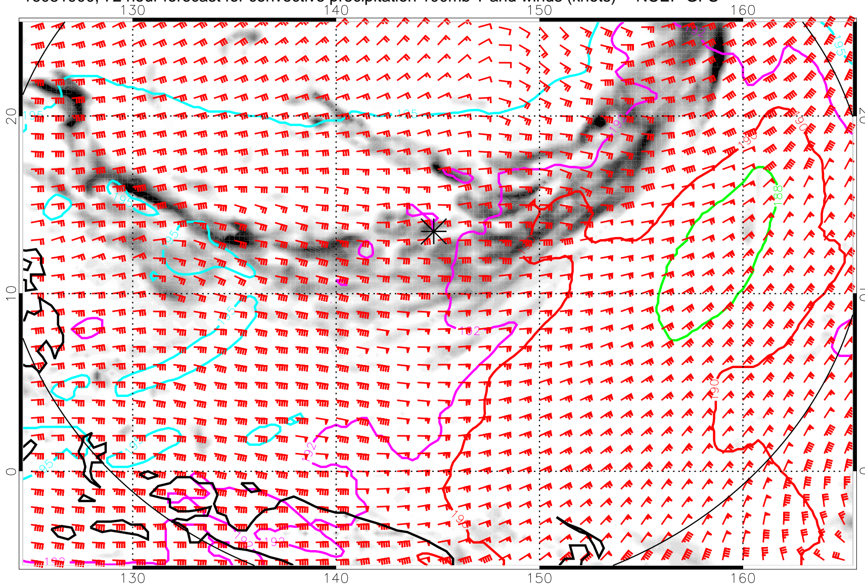
16081900, 72 hour forecast for convective precipitation 100mb T and winds (knots) -- NCEP GFS
