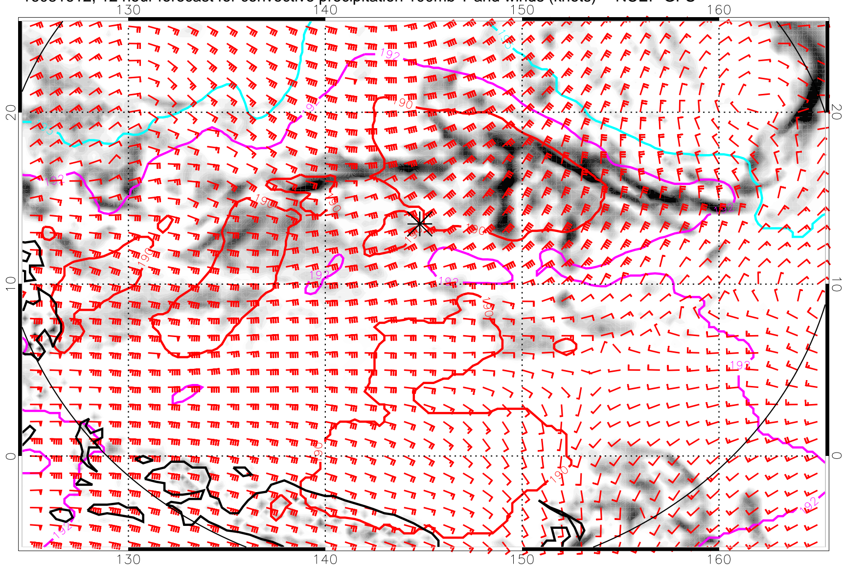
16081612, 12 hour forecast for convective precipitation 100mb T and winds (knots) -- NCEP GFS
