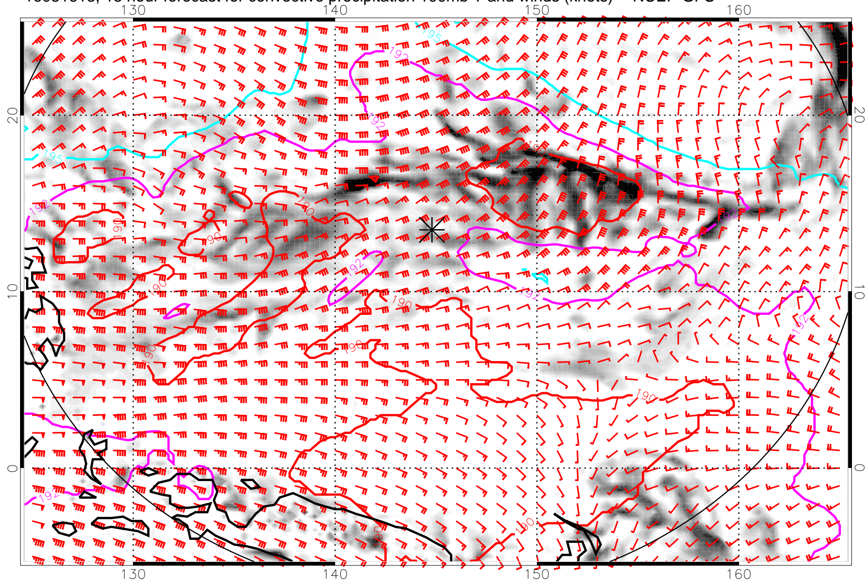
16081618, 18 hour forecast for convective precipitation 100mb T and winds (knots) -- NCEP GFS
