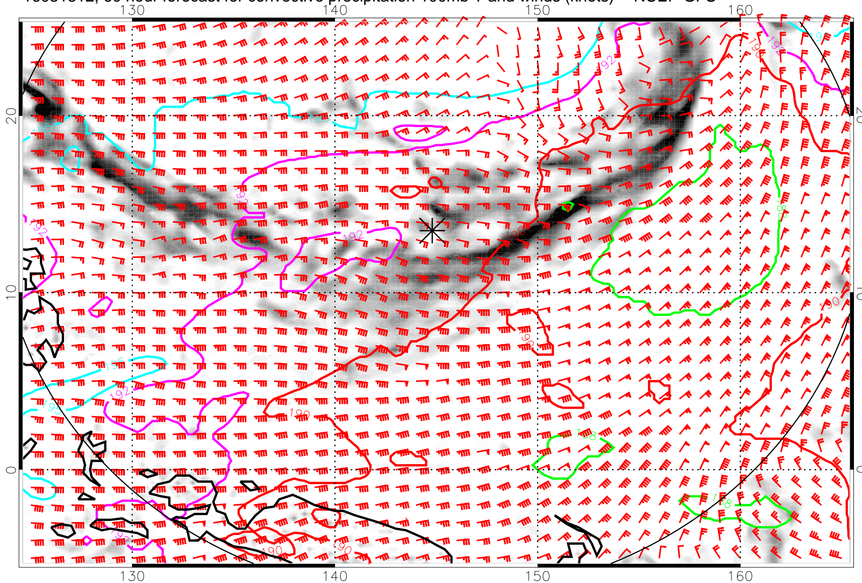
16081812, 60 hour forecast for convective precipitation 100mb T and winds (knots) -- NCEP GFS
