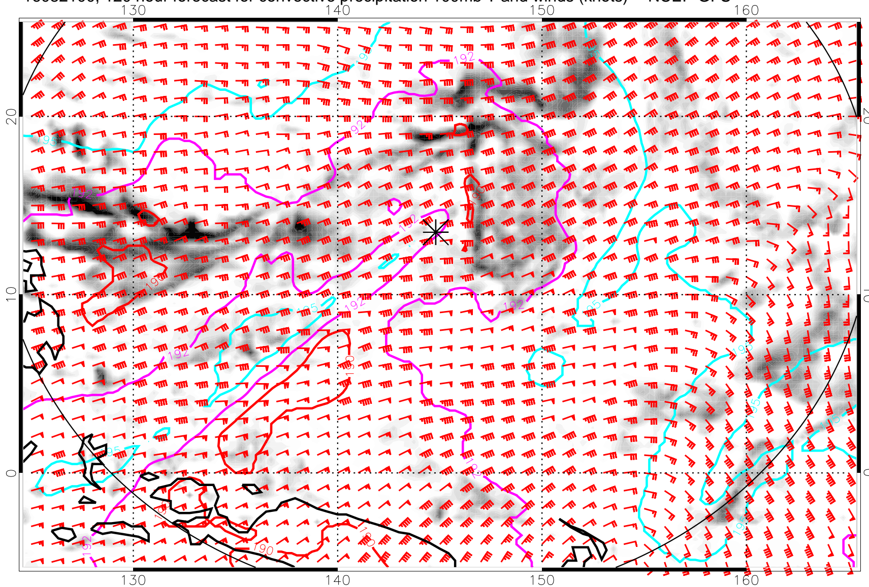
16082100, 120 hour forecast for convective precipitation 100mb T and winds (knots) -- NCEP GFS
