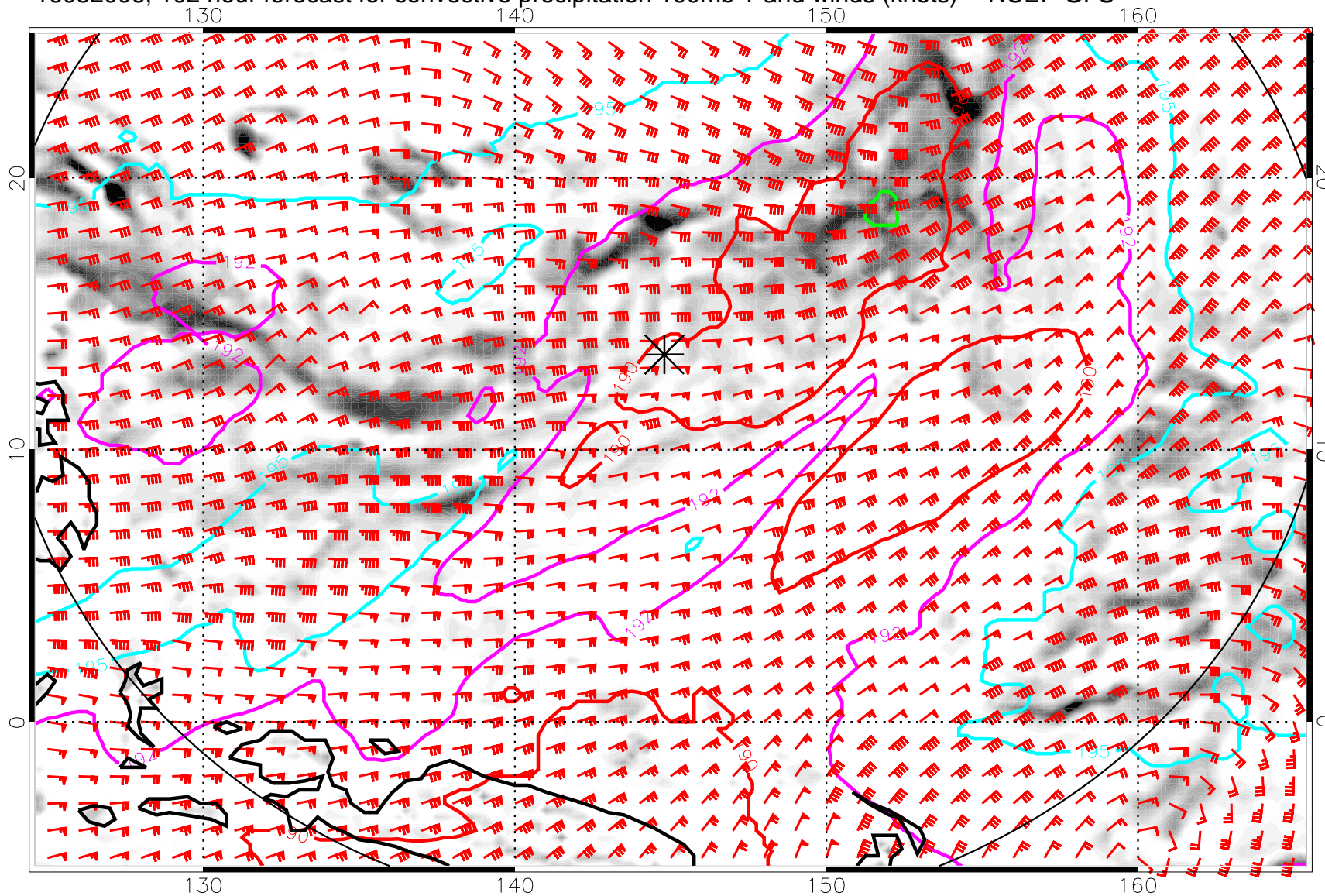
16082006, 102 hour forecast for convective precipitation 100mb T and winds (knots) -- NCEP GFS
