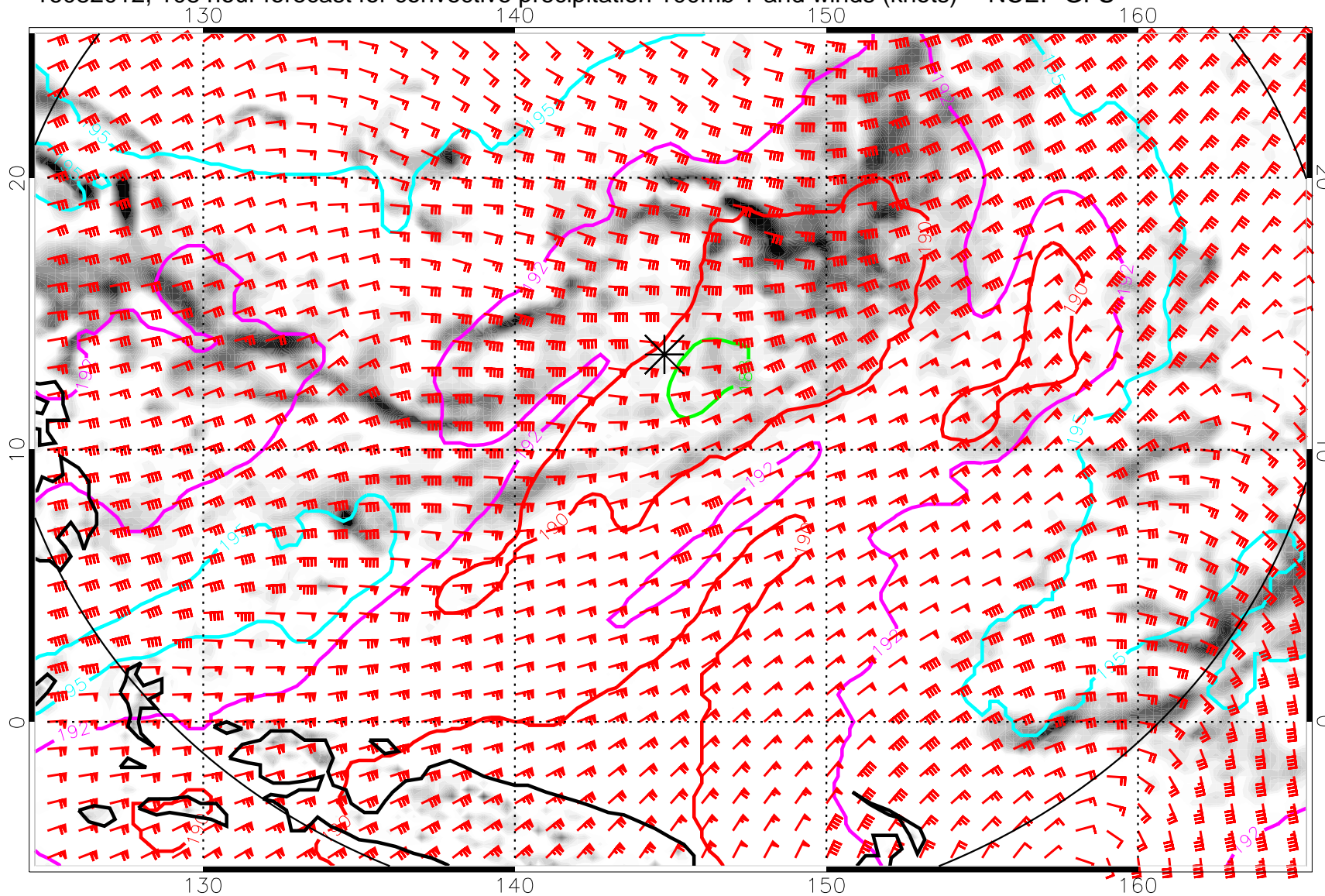
16082012, 108 hour forecast for convective precipitation 100mb T and winds (knots) -- NCEP GFS
