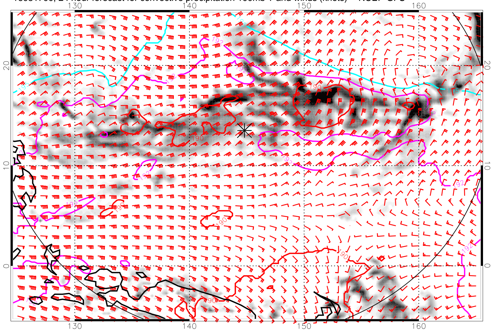
16081700, 24 hour forecast for convective precipitation 100mb T and winds (knots) -- NCEP GFS
