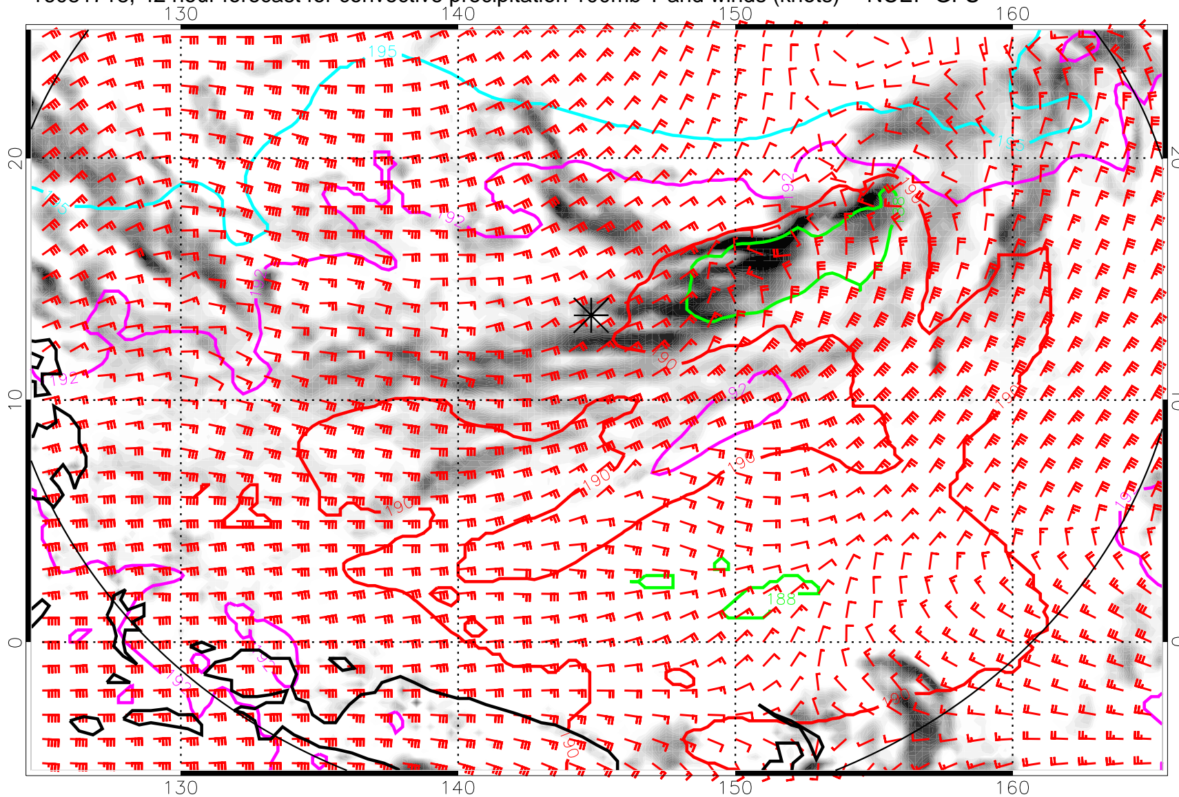
16081718, 42 hour forecast for convective precipitation 100mb T and winds (knots) -- NCEP GFS
