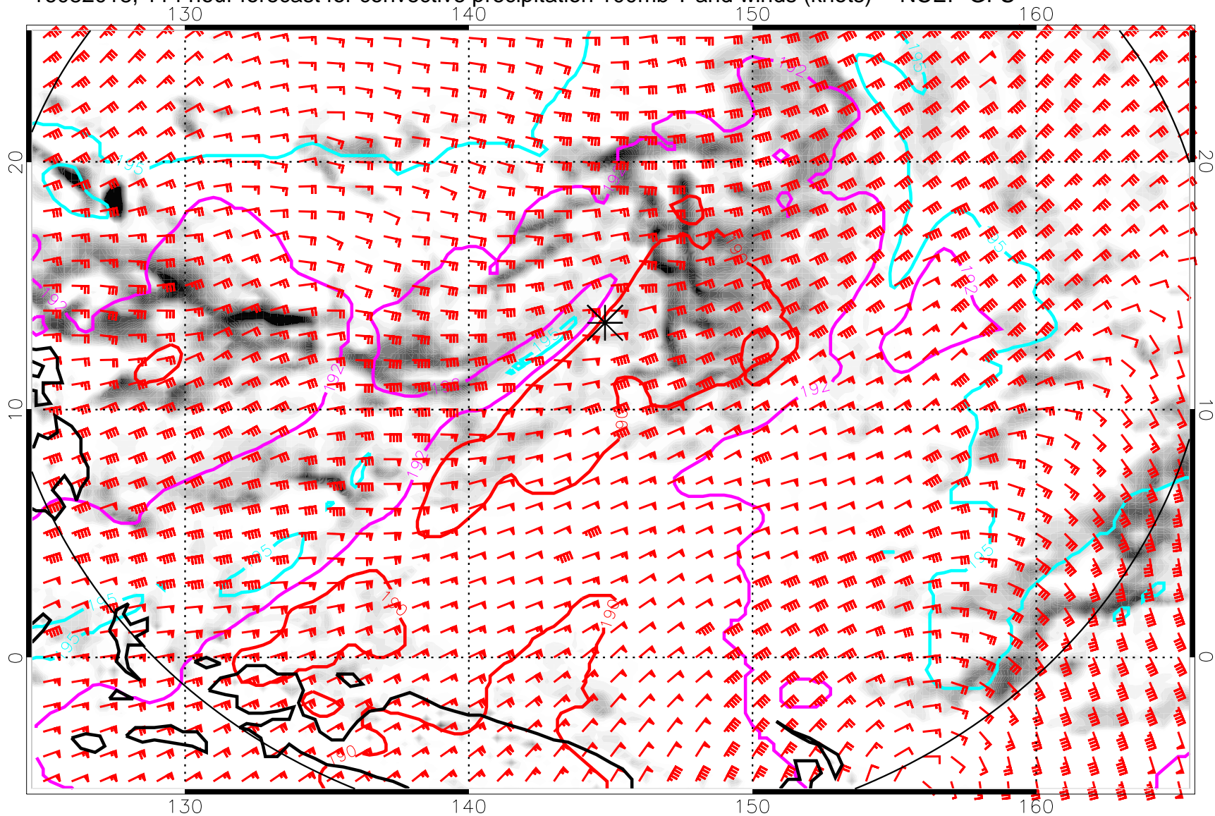
16082018, 114 hour forecast for convective precipitation 100mb T and winds (knots) -- NCEP GFS
