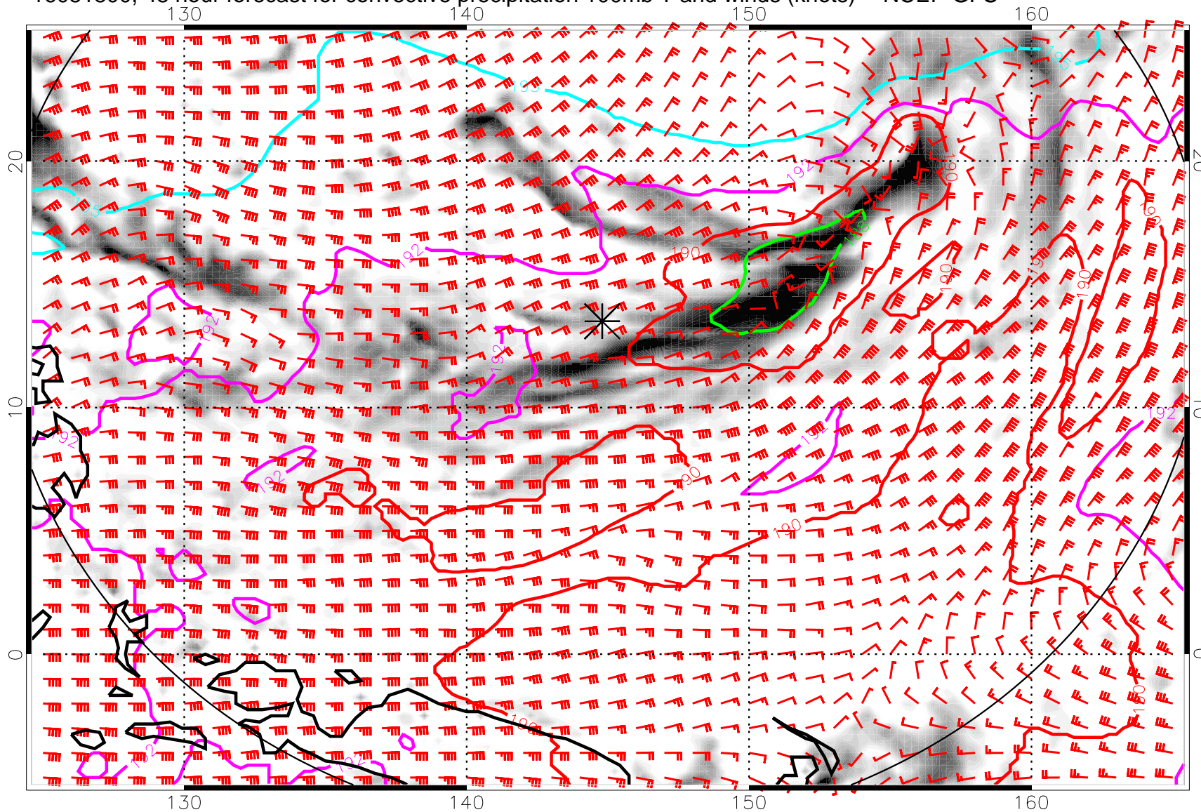
16081800, 48 hour forecast for convective precipitation 100mb T and winds (knots) -- NCEP GFS
